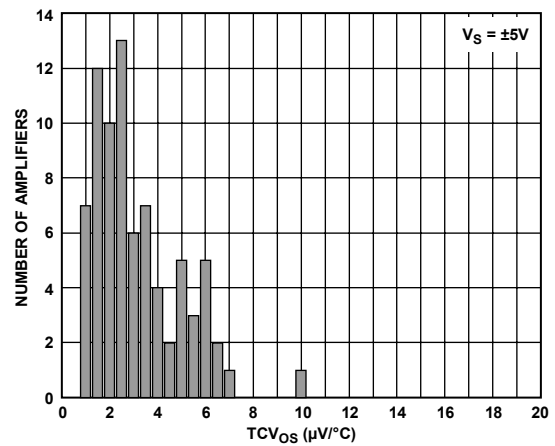
Figure 11. Offset Voltage Drift Distribution, V_S = \pm 5 V
