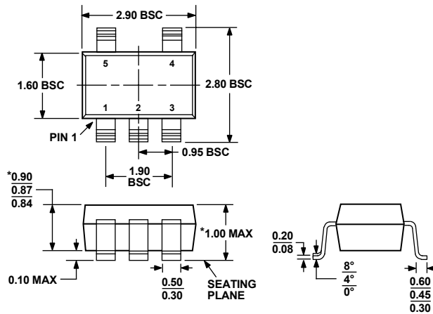
Figure 36. 5-Lead Thin Small Outline Transistor Package [TSOT] (UJ-5)
