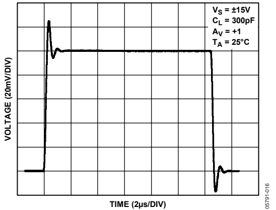
Figure 15. Small Signal Transient Response, V_S = \pm 15 V
