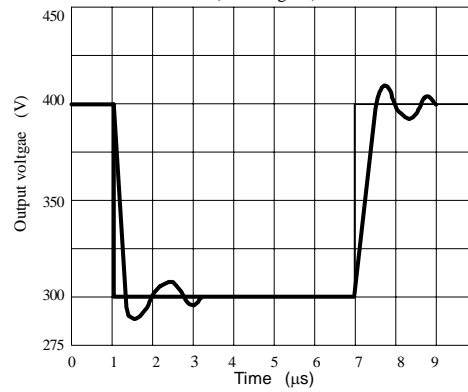
Fig.10 Output Characteristics current sourcing
