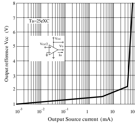
Fig.12 Current Limiting
