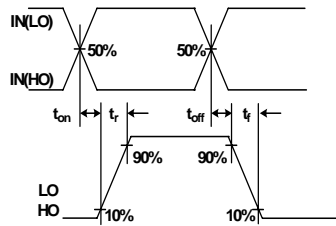
Figure 3. Switching Time Waveform Definitions
