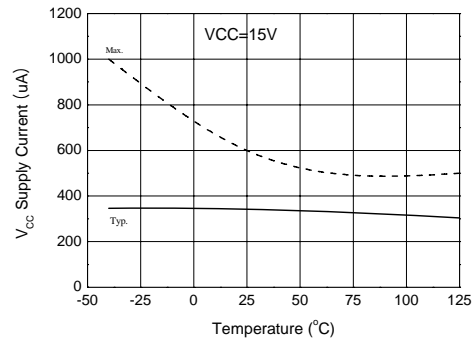
Figure 22. VCC Supply Current vs Temperature
