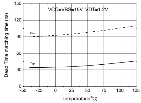
Figure 31. Deadtime Matching Time vs Temperature
