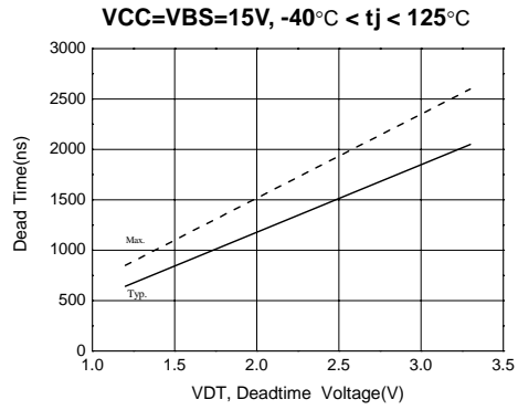
Figure 2. Dead Time VS VDT
