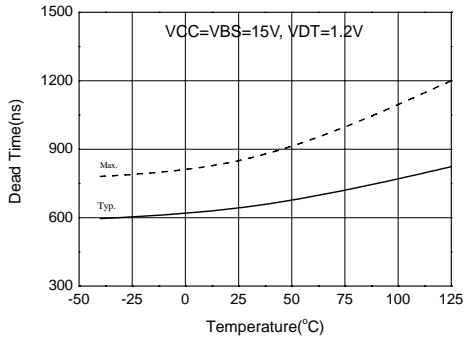
Figure 30. Deadtime vs Temperature
