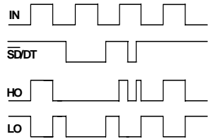
Figure 1. Input/output Timing Diagram
