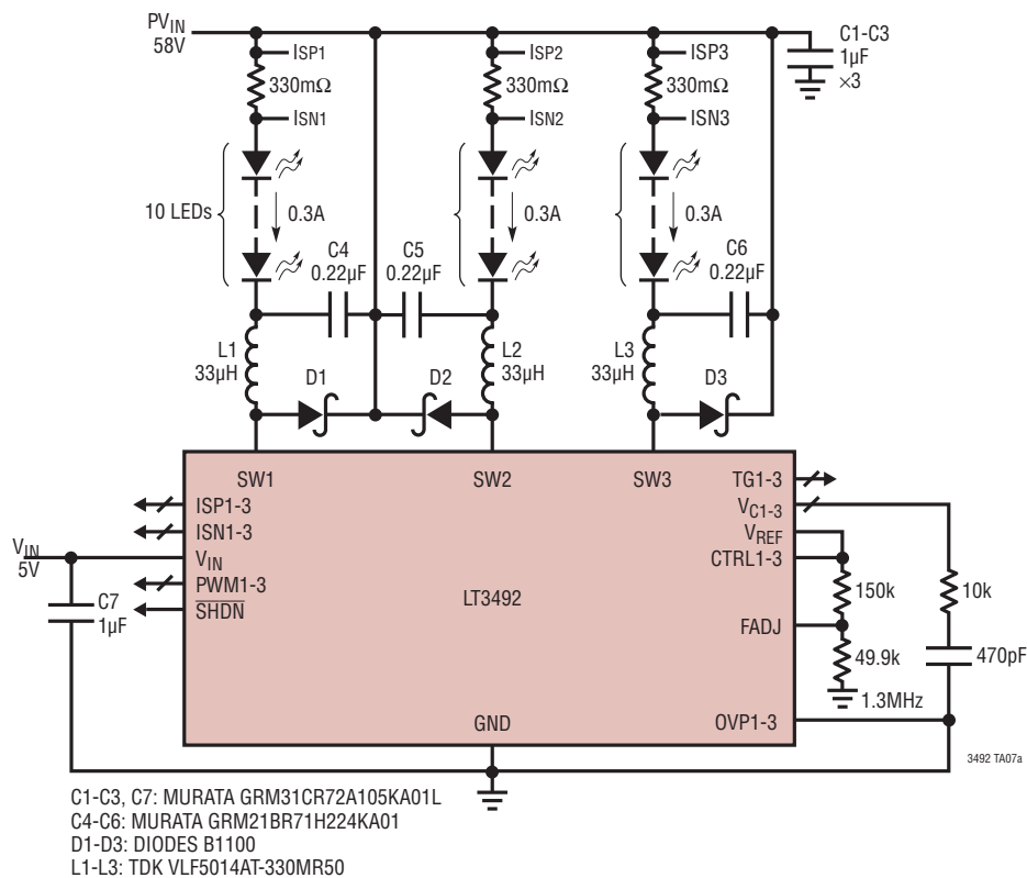
Minimum BOM Buck Mode LED Driver
