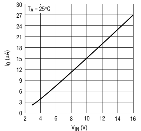
Shutdown Quiescent Current ( I_Q = 0V)
