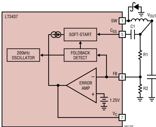
Figure 2. Feedback Network
