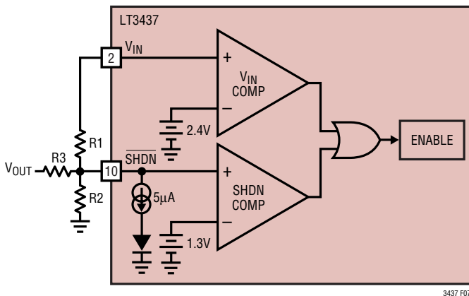
Figure 7. Undervoltage Lockout
