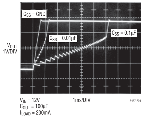
Figure 4. V_{OUT} dV/dt
