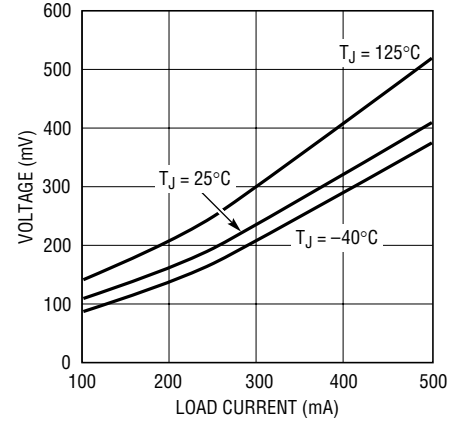
Switch On Voltage ( V_{CESAT} )
