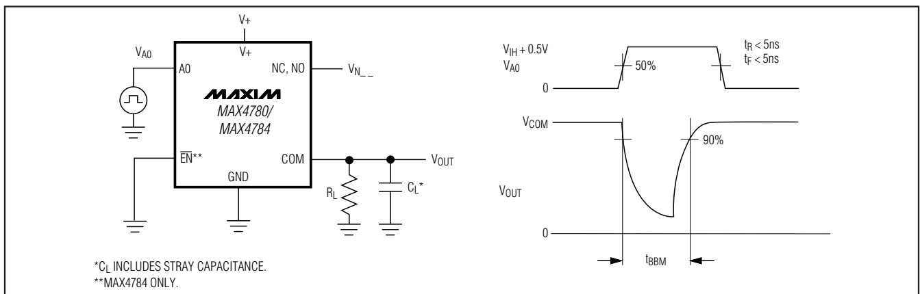
Figure 2. Break-Before-Make Interval
