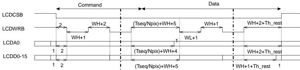
Figure 4-1 MAIN LCD data transfer waveform (Unit : tSCLK)
