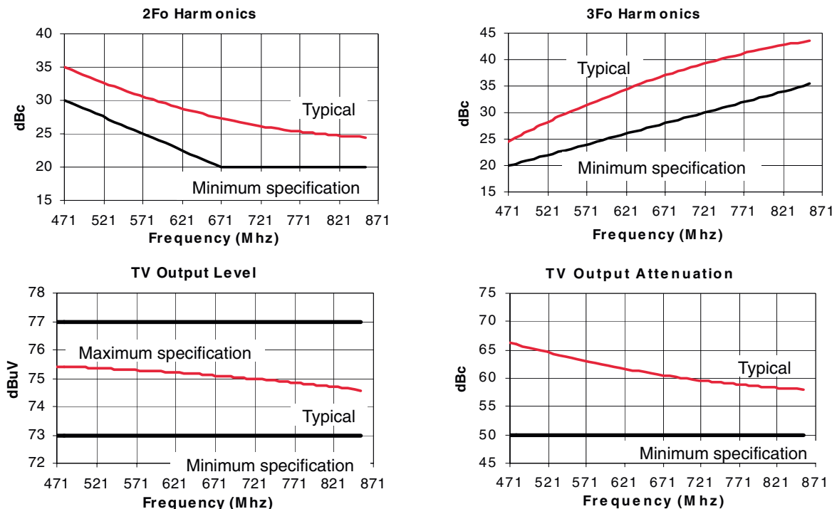
Figure 3. Typical Performance
