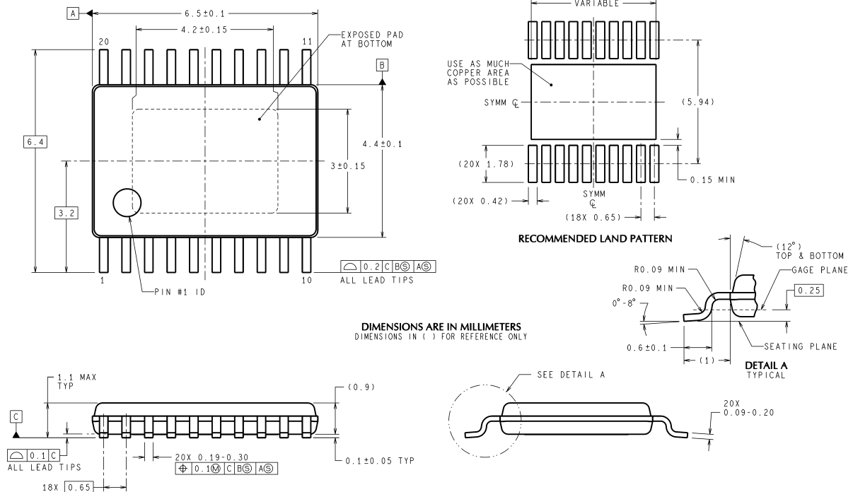
Exposed-DAP TSSOP Package Order Number LM4884MH NS Package Number MXA20A for Exposed-DAP TSSOP
