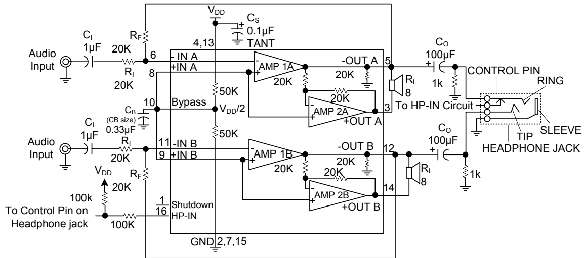
Figure 1. Typical Audio Amplifier Application Circuit
