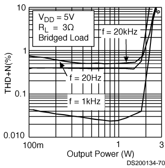
LM4839MTE THD+N vs Output Power
