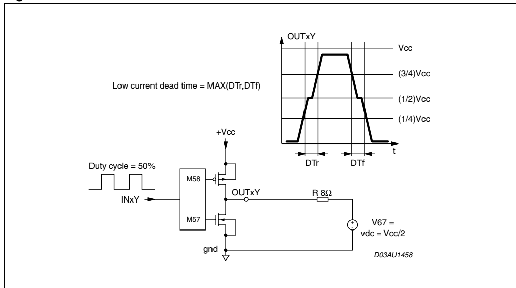
Figure 2. Test circuit
