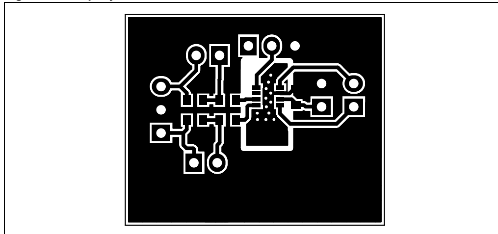
Figure 69. Top layer
