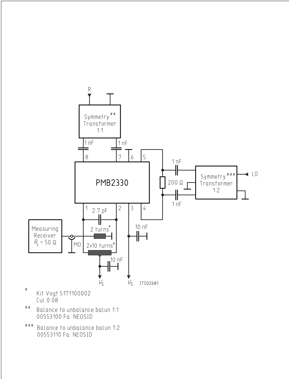
Test Circuit
