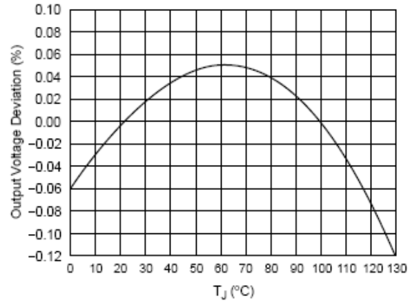
Figure 2. Reference Voltage vs Temperature
