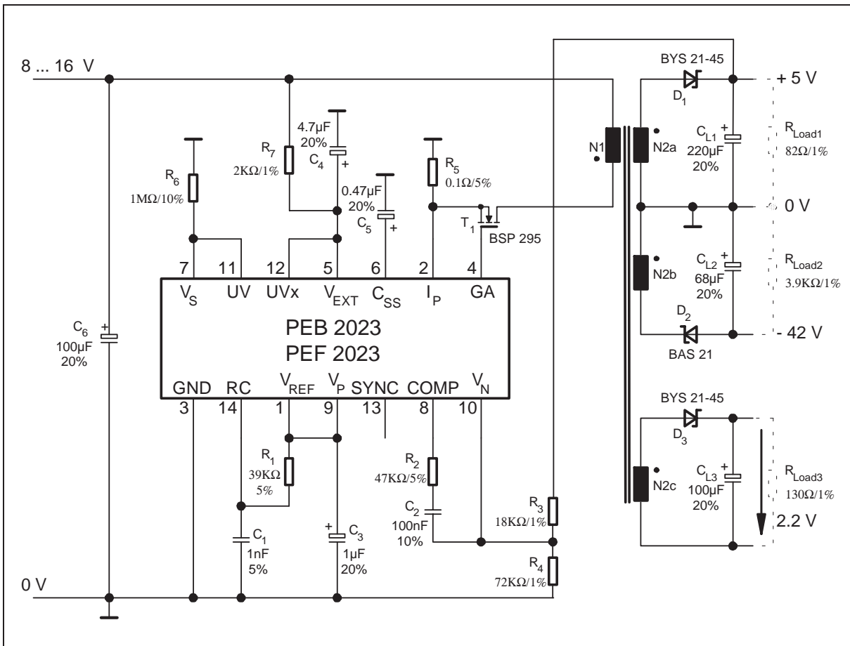
Figure 6 PEB/F 2023 in a non-isolated Flyback Configuration
