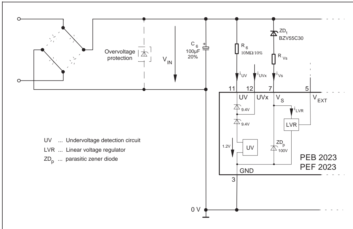
Figure 7 PEB/F 2023 Surge Protection
