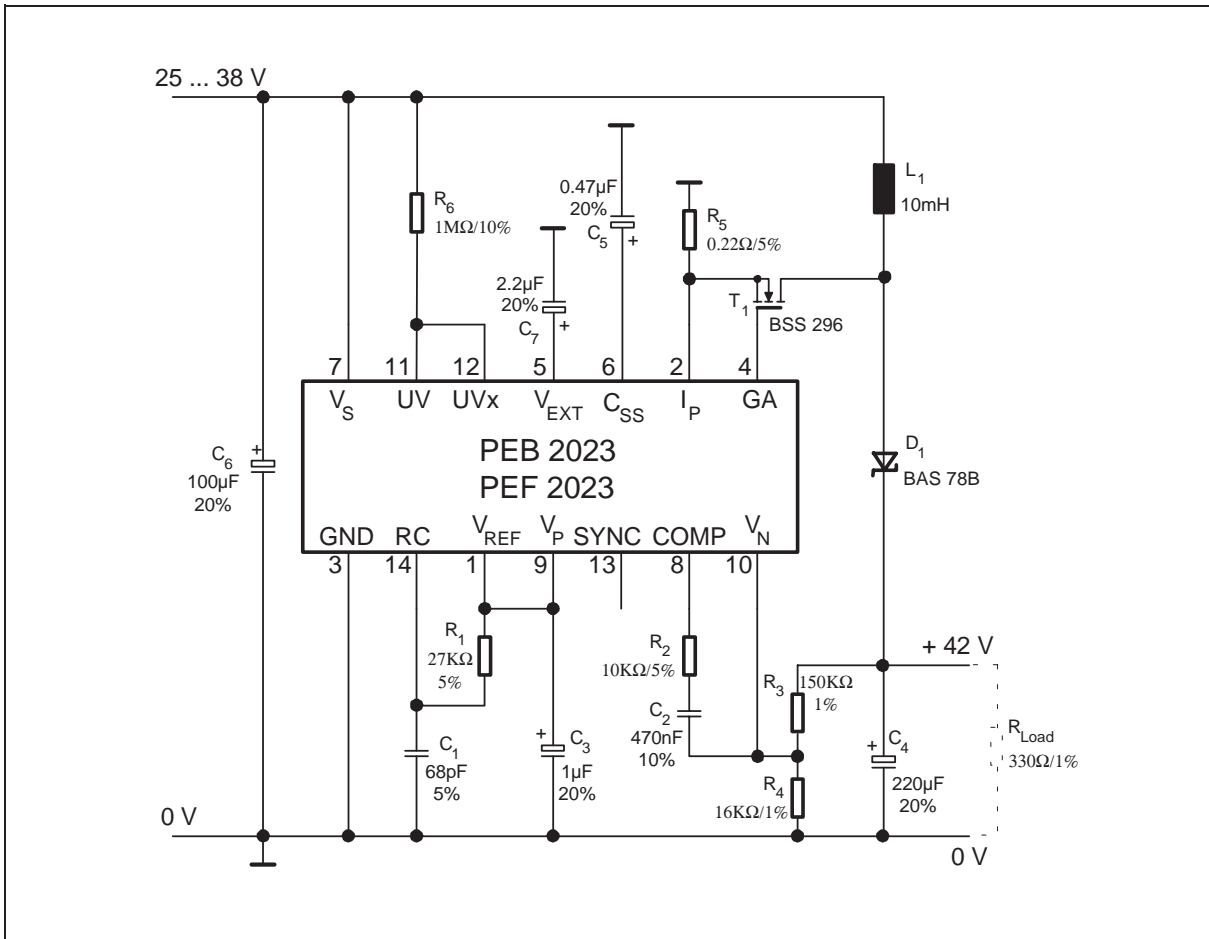
Figure 5 PEB/F 2023 in a non-isolated Minimum Configuration
