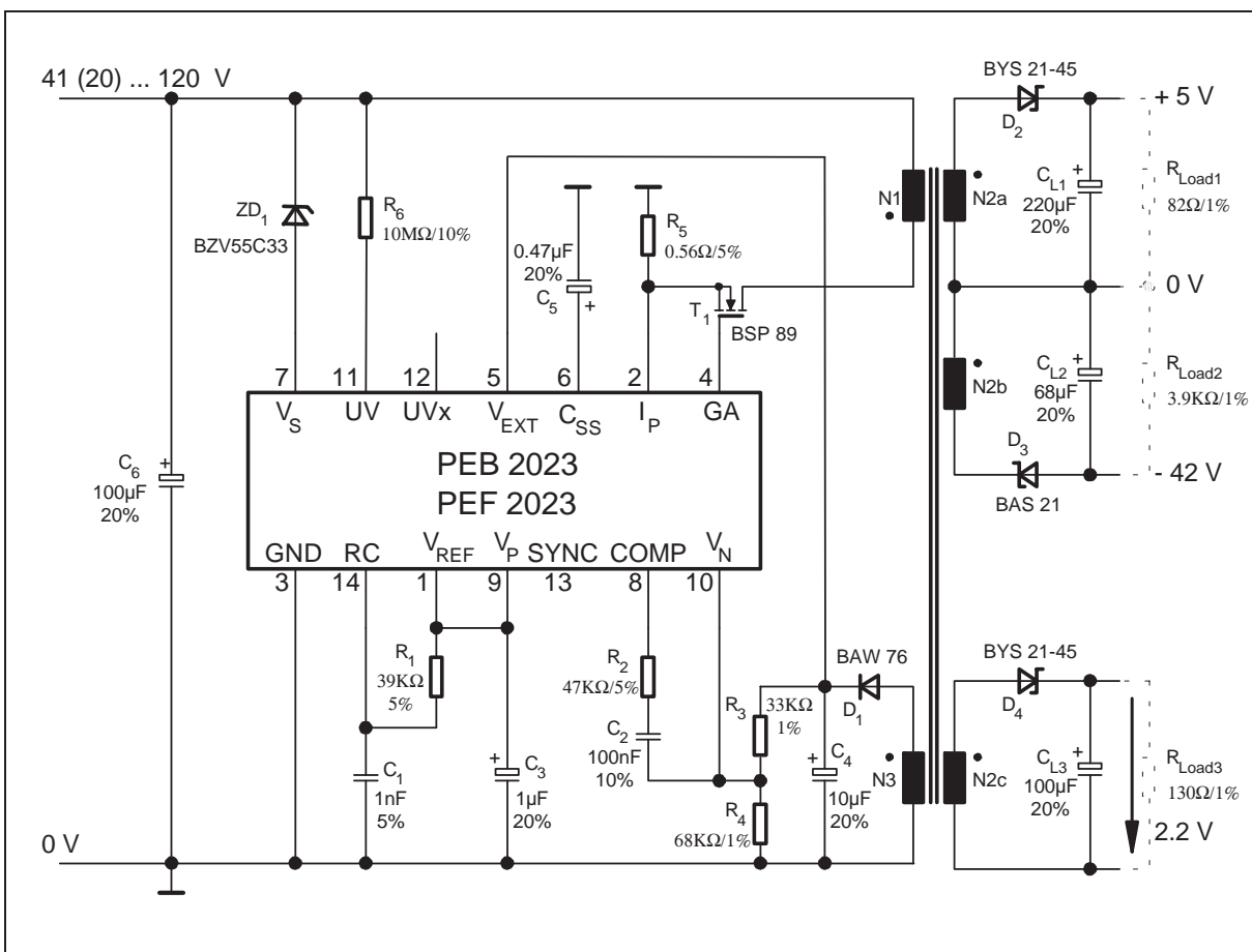
Figure 4 PEB/F 2023 in Flyback Configuration with Transformer Isolation
