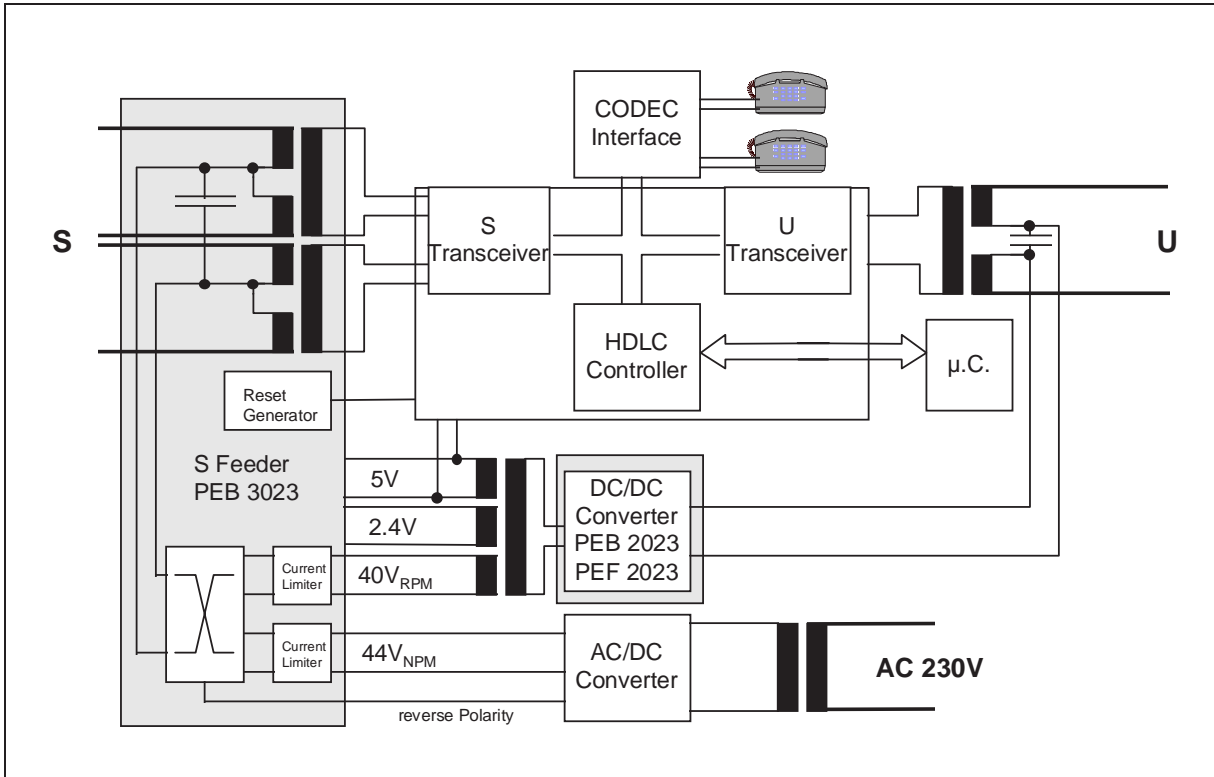
Figure 3 PEB/F 2023 in ISDN-Concept
