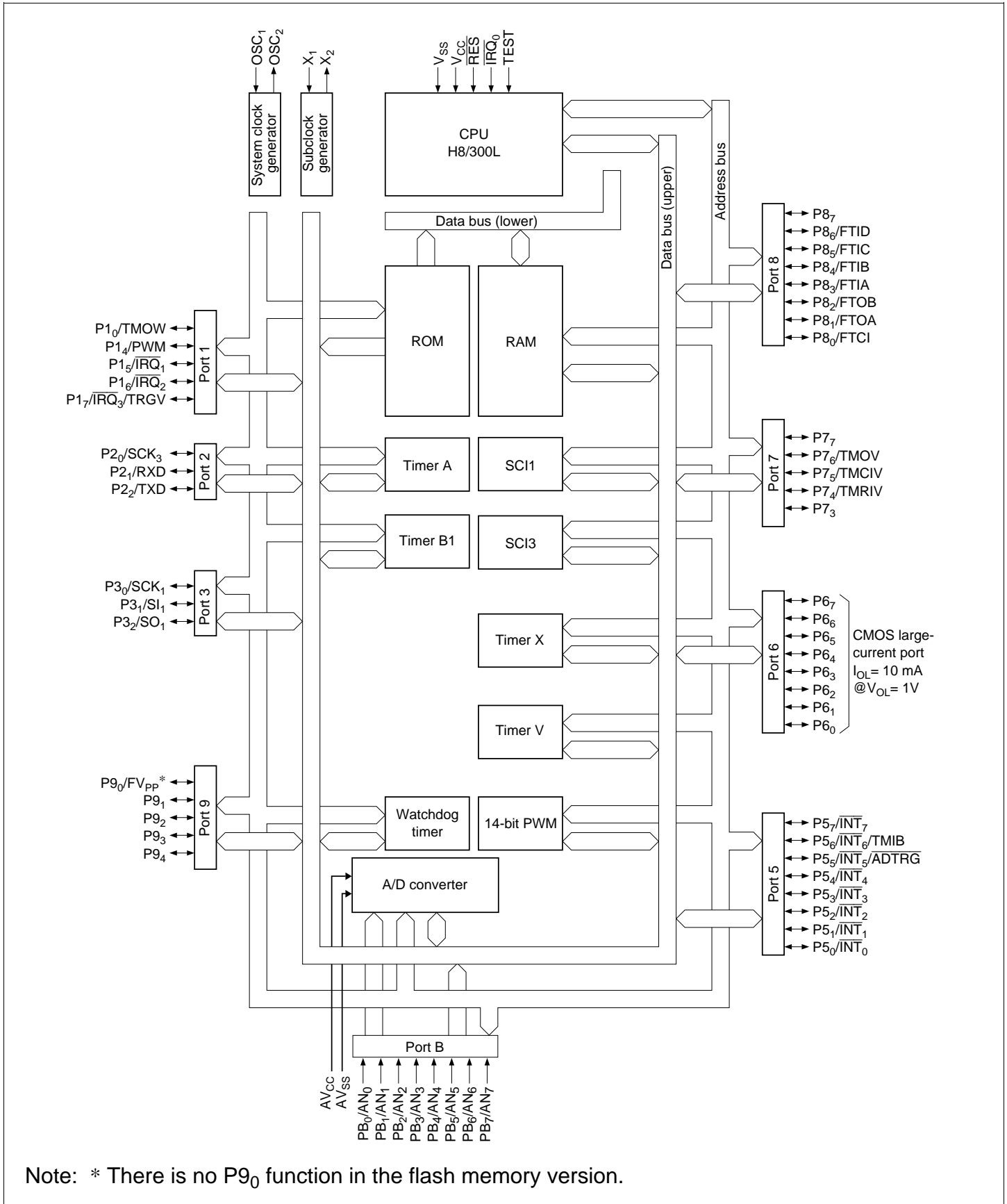
Figure 1.1 Block Diagram
