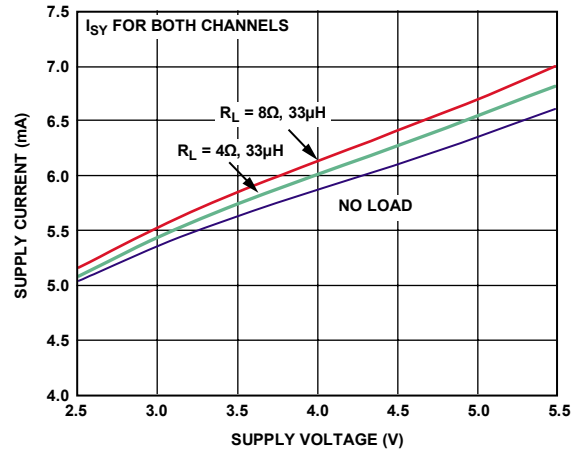
Figure 13. Supply Current vs. Supply Voltage, No Load
