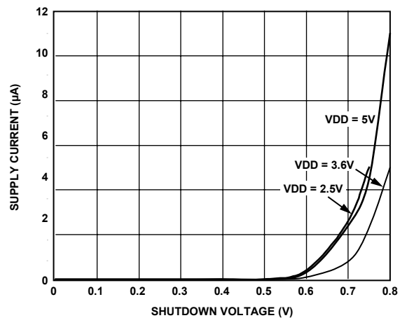
Figure 14. Supply Current vs. Shutdown Voltage
