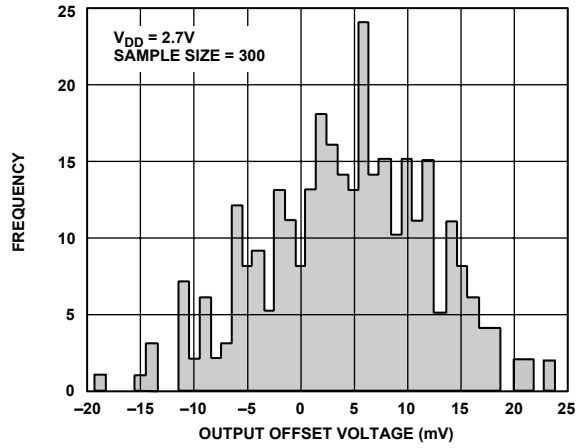
Figure 36. Output Offset Voltage Distribution
