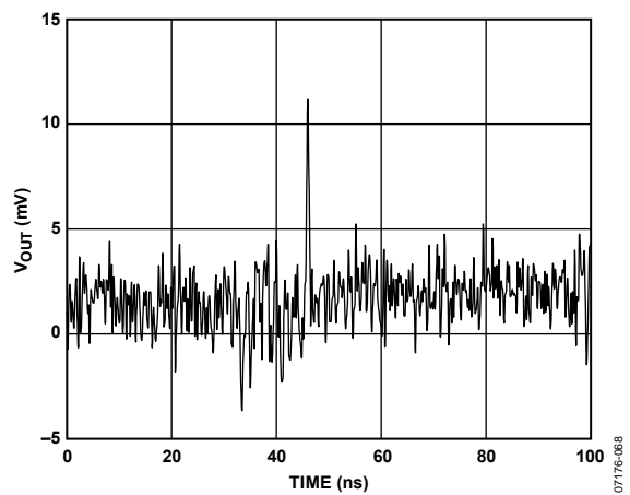
Figure 40. ADV3200 OSD Switching Glitch
