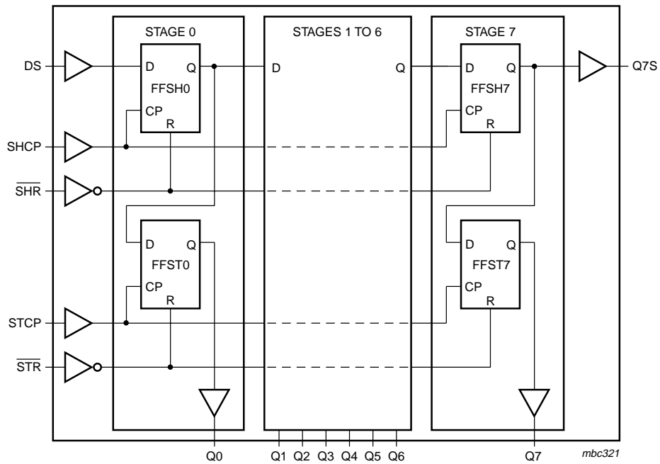
Fig 4. Logic diagram
