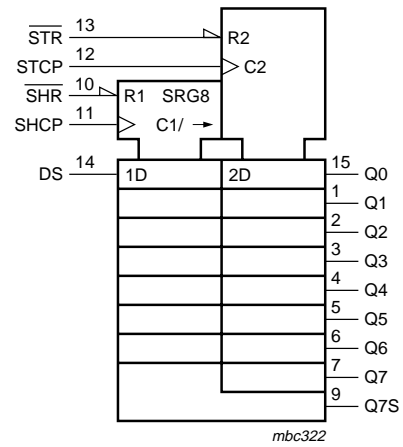
Fig 3. IEC logic symbol
