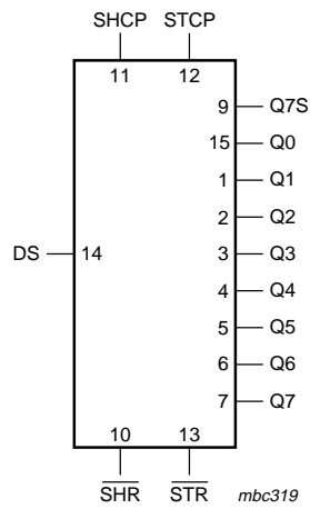
Fig 2. Logic symbol
