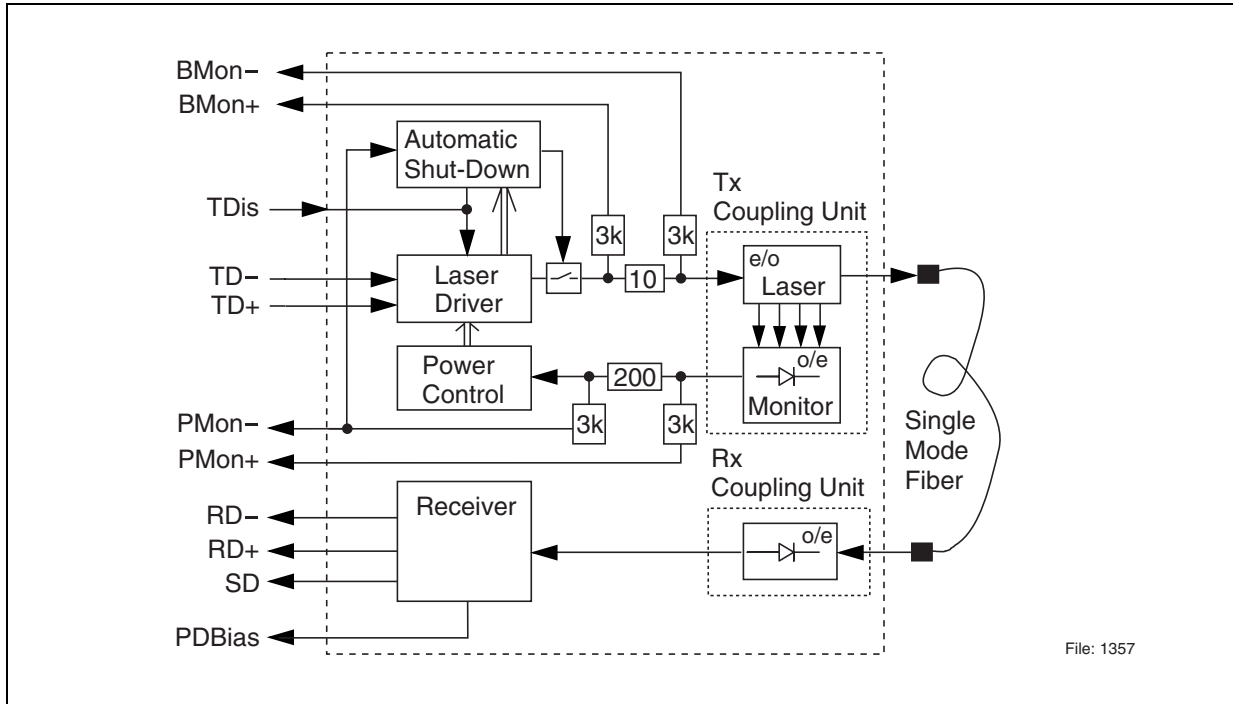
Figure 10 Functional Diagram 2x10 Pin Rows
