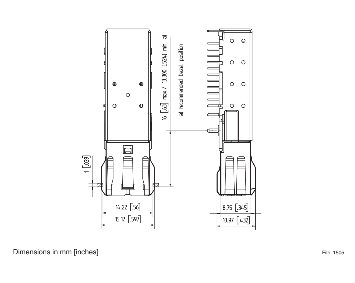
Figure 20 Non-standard Collar
