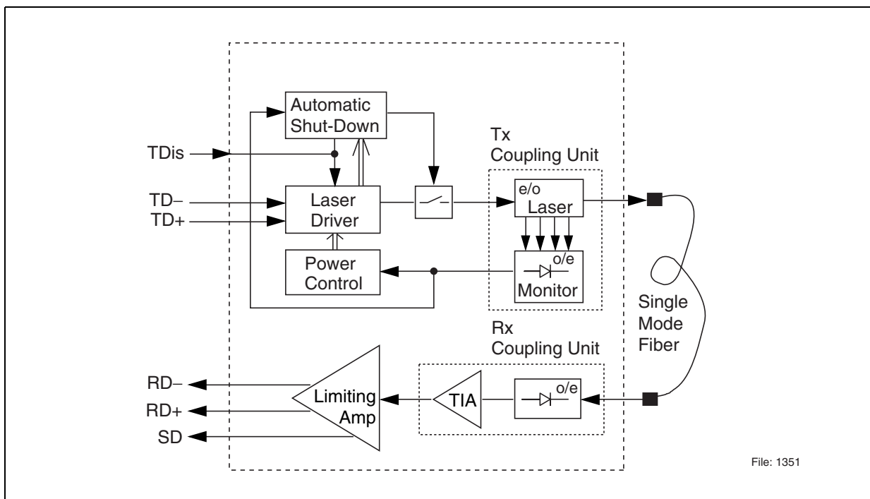
Figure 11 Functional Diagram 2x5 Pin Rows
