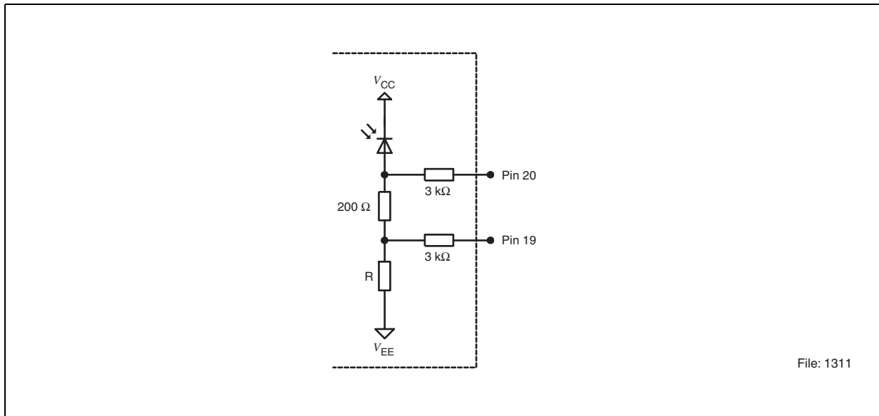
Figure 8 Power Monitor – Transceiver Internal
