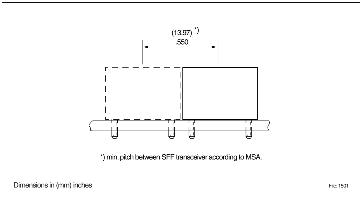
Figure 12 Transceiver Pitch
