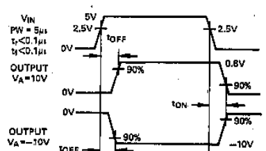
Figure 4. Standard DTL, TTL, RTL
