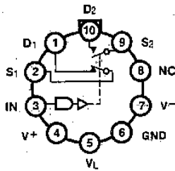
(OUTLINE DWG TO-100)
