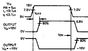
Figure 3. High Level Logic
