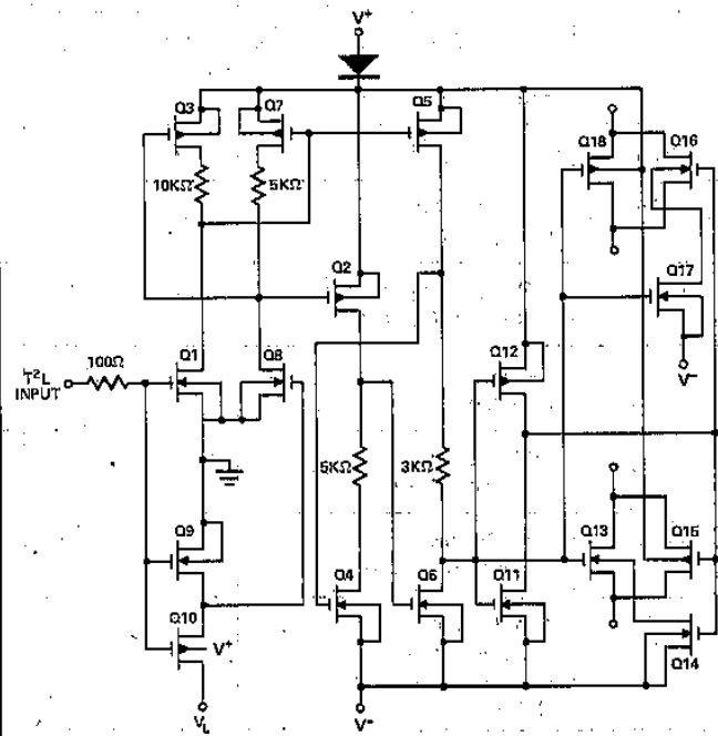
FIGURE 1. Typical Driver/Gate — IH5142
