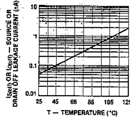
I_{S(off)} or I_{D(off)} vs Temperature*
