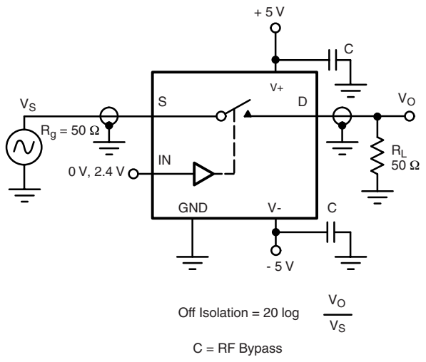
Figure 5. Off-Isolation
