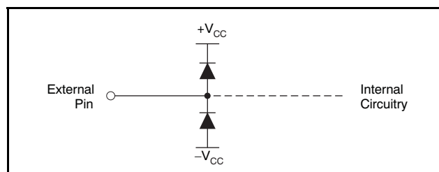
Figure 55. Internal ESD Protection
