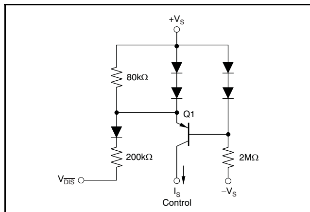
Figure 54. Simplified Disable Control Circuit
