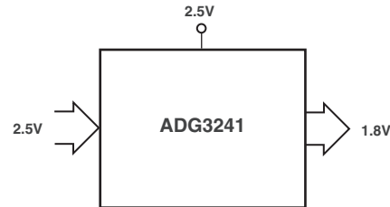
Figure 7. 2.5 V to 1.8 V Voltage Translation, \overline{SEL} = 2.5 V _{CC}
