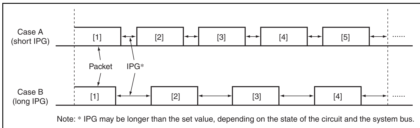
Figure 11.7 Changing IPG and Transmission Efficiency
