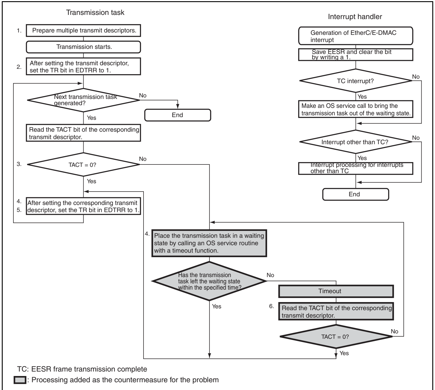
Figure 12.10 Method of Adding Timeout Processing
