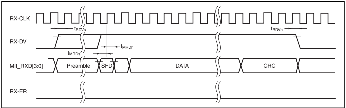
Figure 21.45 MII Reception Timing (Normal Operation)
