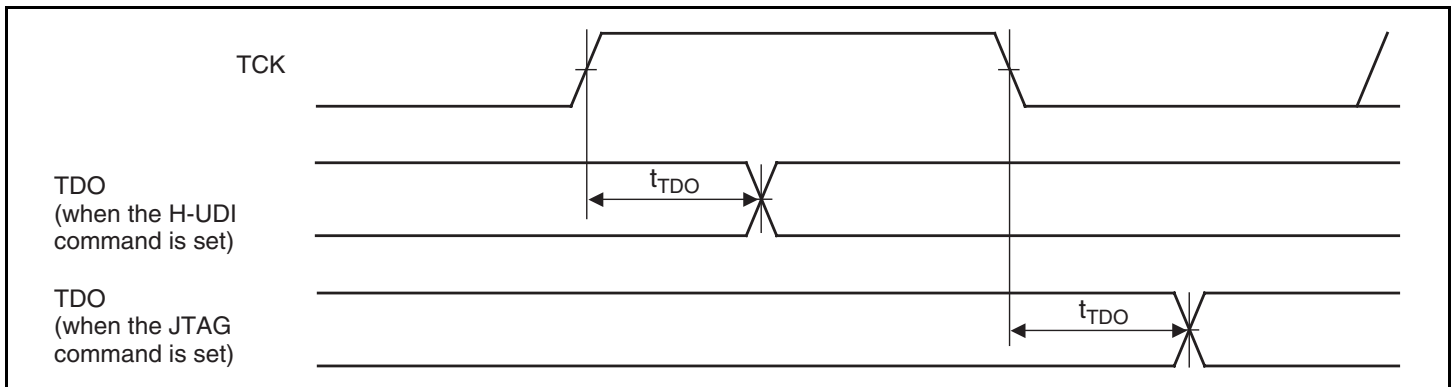
Figure 19.3 H-UDI Data Transfer Timing
