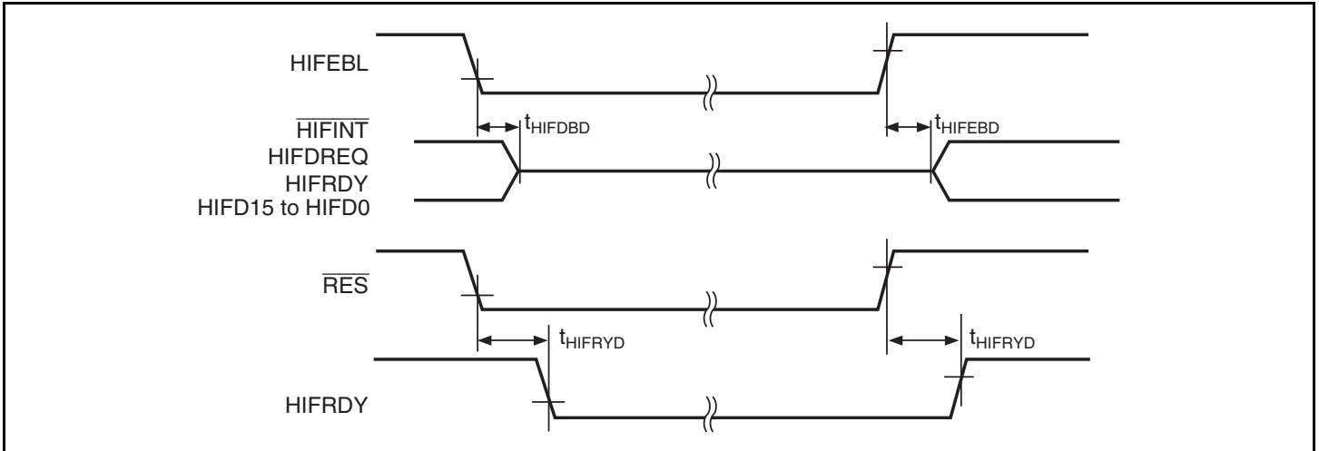
Figure 21.42 HIFRDY and HIF Pin Enable/Disable Timing
