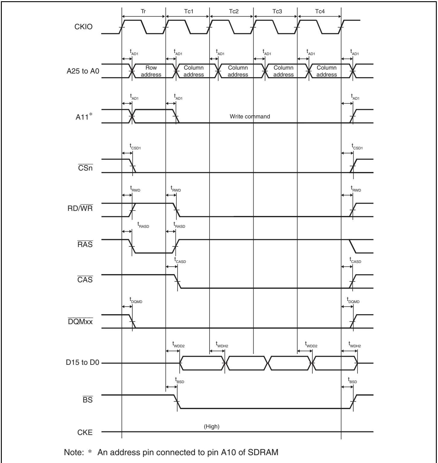
Figure 21.27 Synchronous DRAM Burst Write Bus Cycle (Single Write × 4) (Bank Active Mode: ACT + WRITE Commands, WTRCD = 0 Cycle, TRWL = 0 Cycle)
