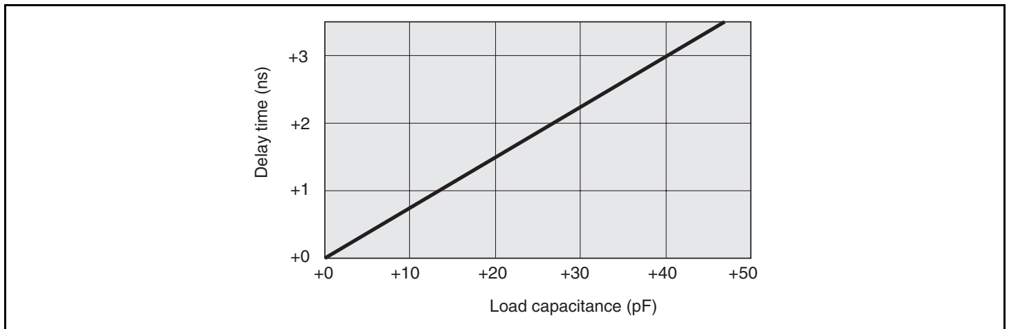
Figure 21.55 Load Capacitance versus Delay Time
