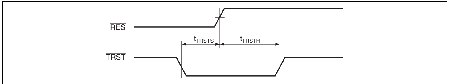
Figure 21.52 TCK Input Timing in Reset Hold State
