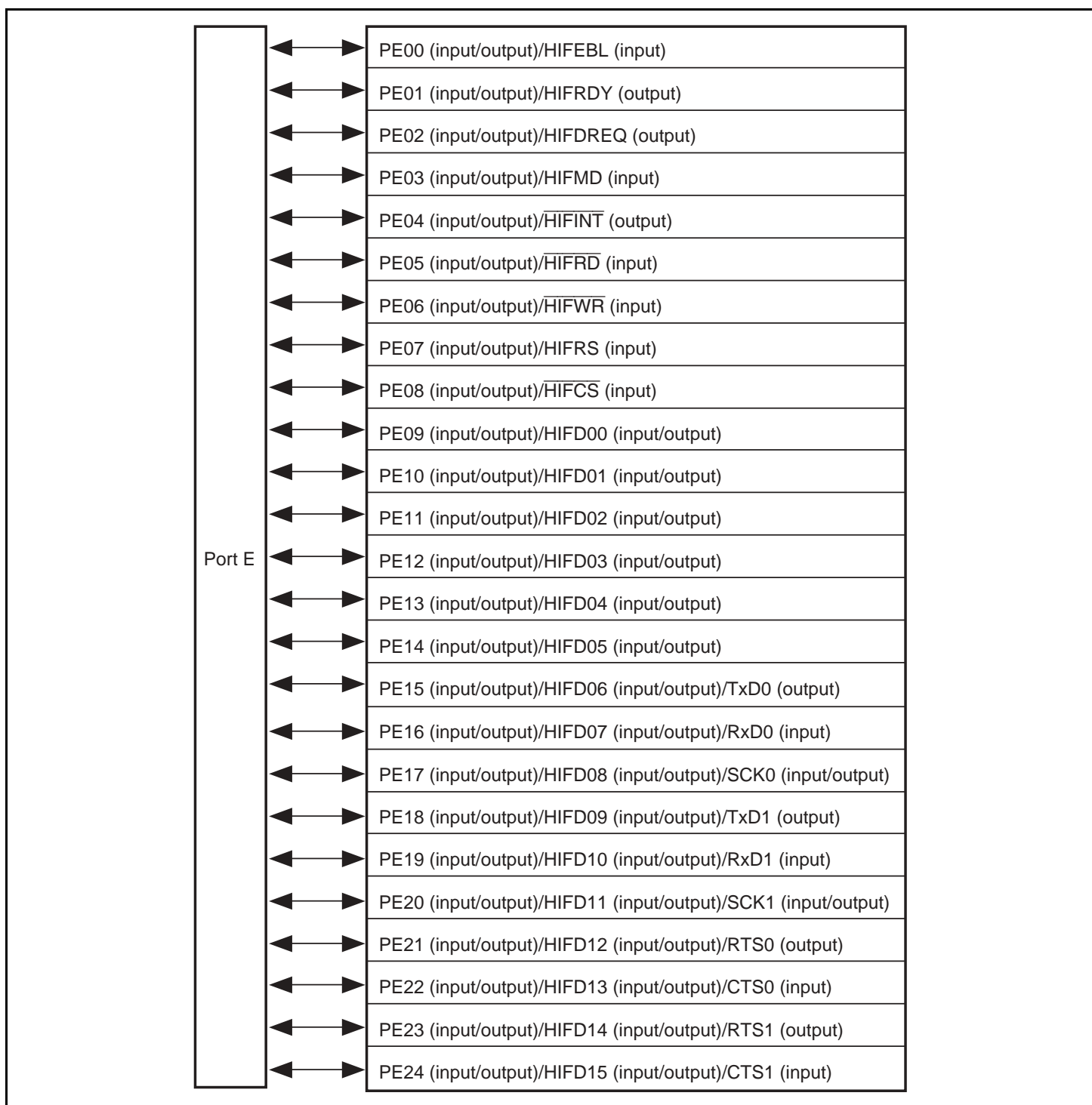
Figure 17.5 Port E
