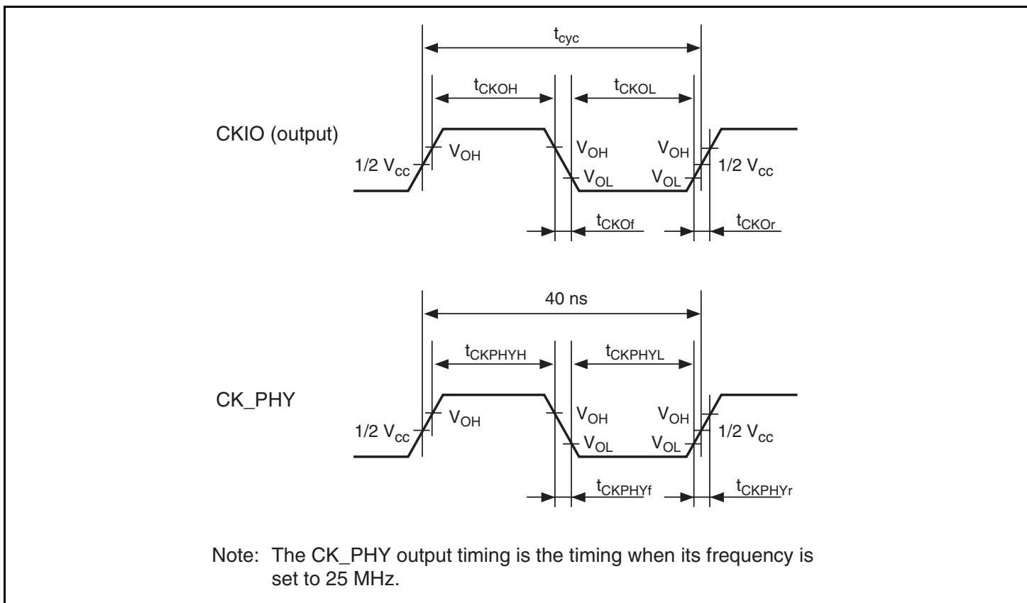
Figure 21.2 CKIO and CK_PHY Clock Output Timings
