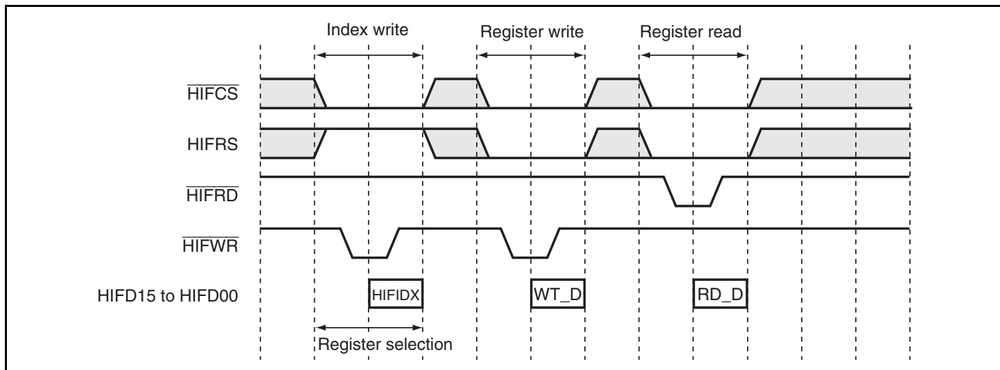
Figure 15.5 HIF Register Settings
