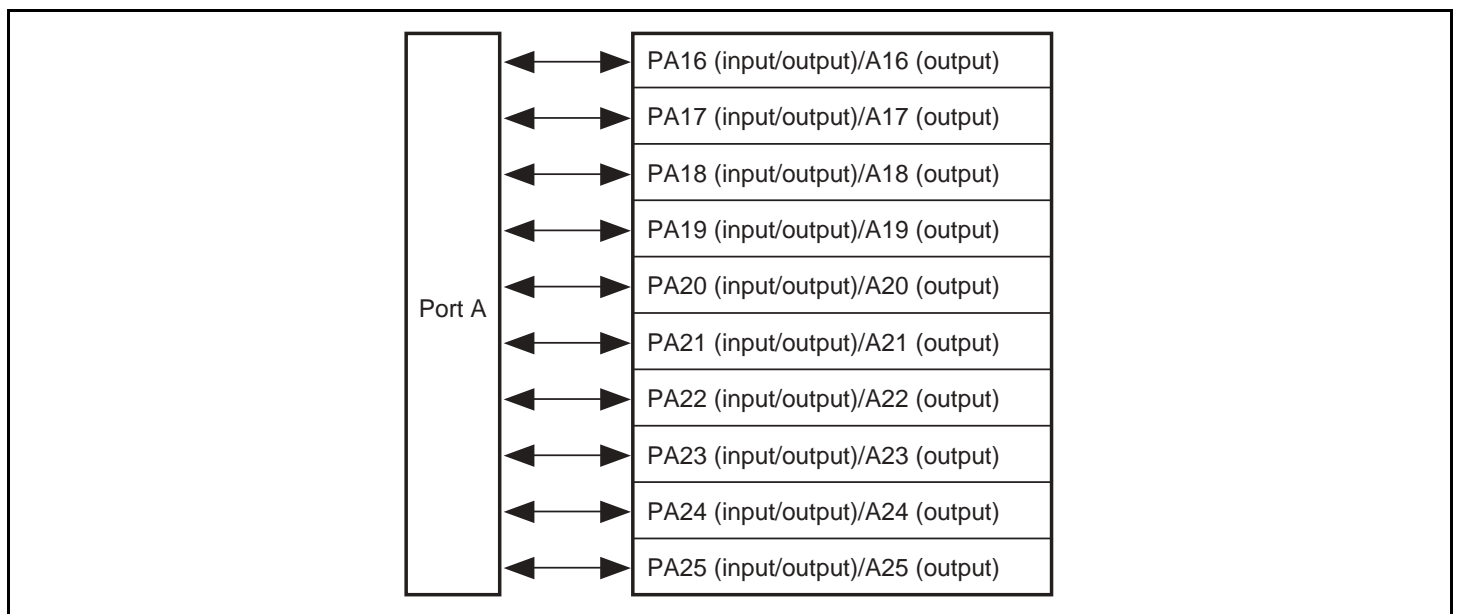
Figure 17.1 Port A
