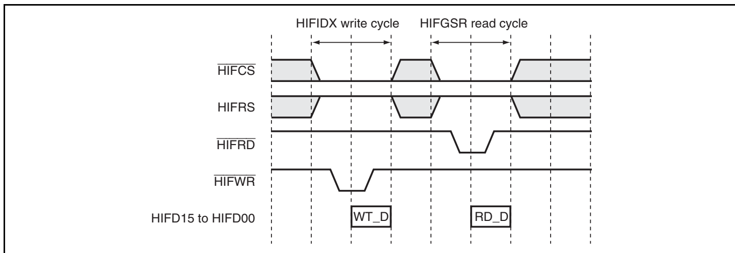
Figure 15.4 HIFIDX Write and HIFGSR Read
