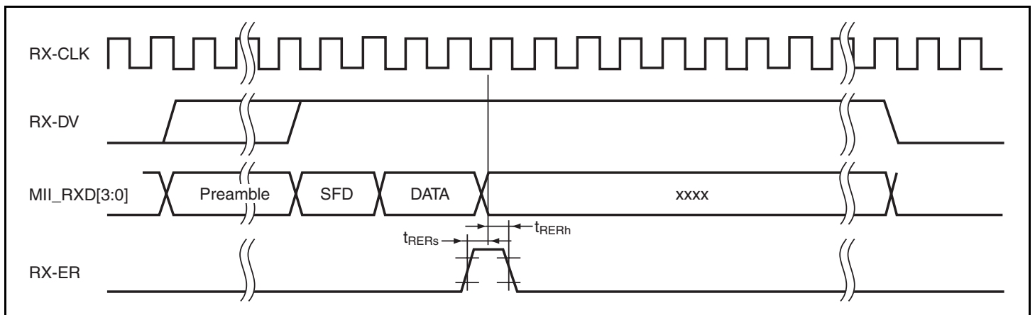
Figure 21.46 MII Reception Timing (Error Occurred)
