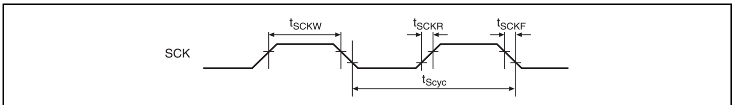
Figure 21.37 SCK Input Clock Timing
