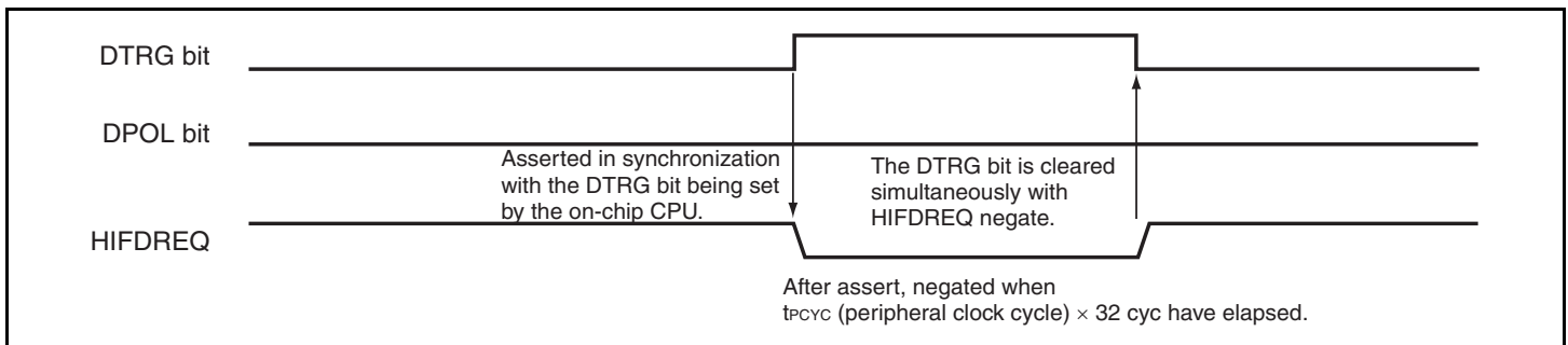
Figure 15.10 HIFDREQ Timing (When DMD = 1 and DPOL = 0 )
