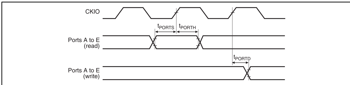
Figure 21.39 I/O Port Timing
