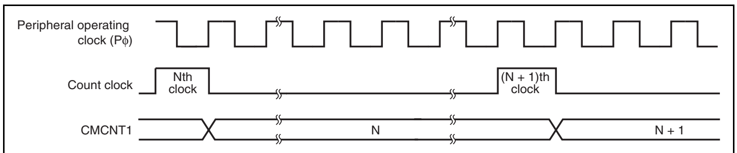
Figure 13.3 Count Timing
