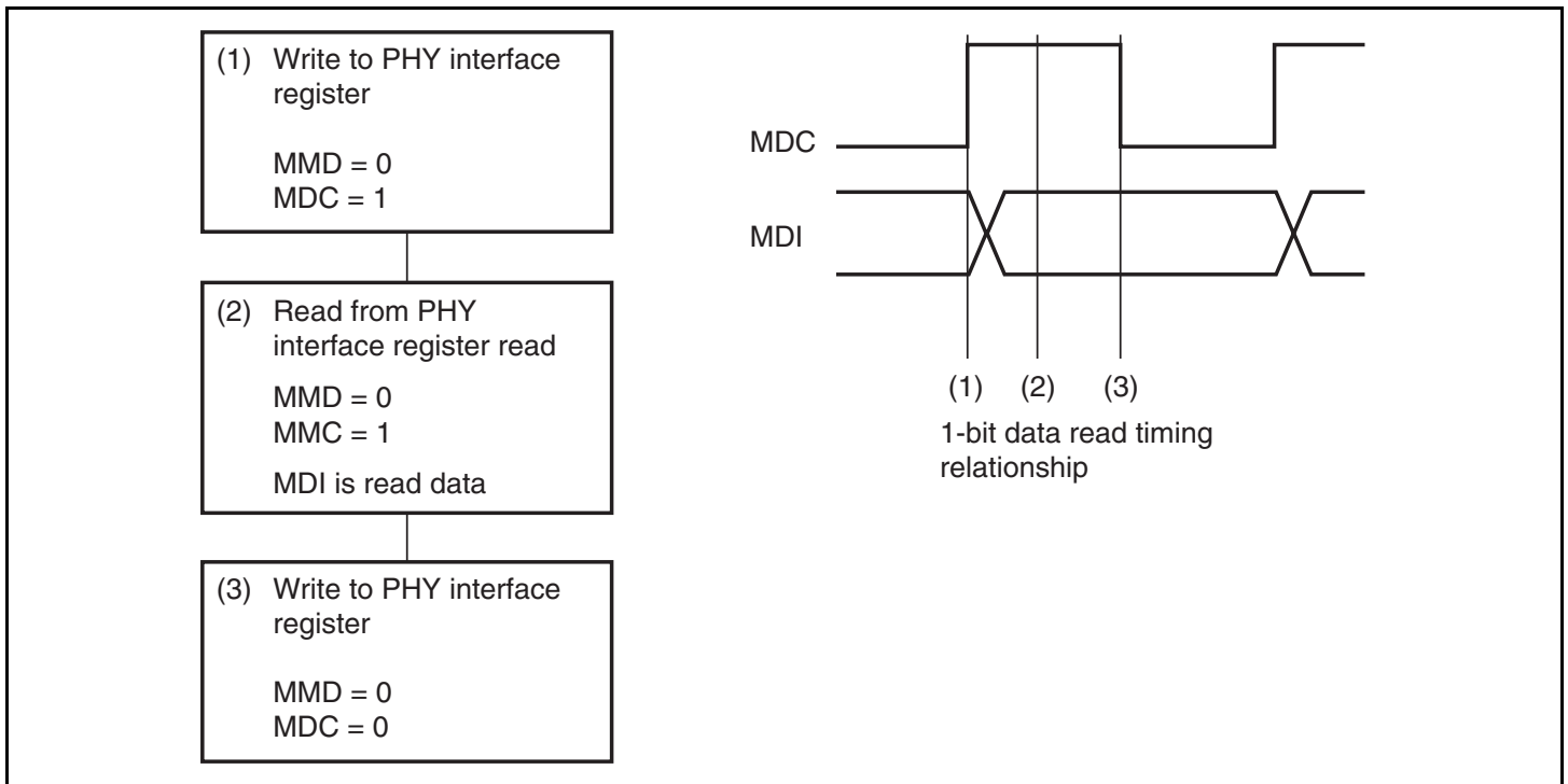
Figure 11.6 (3) 1-Bit Data Read Flowchart
