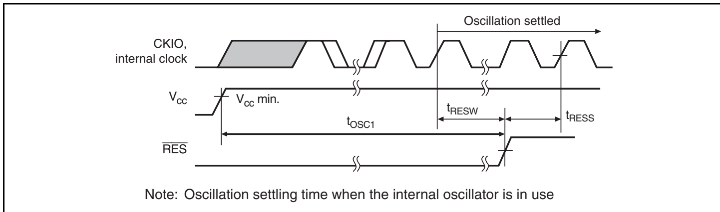
Figure 21.3 Oscillation Settling Timing after Power-On
