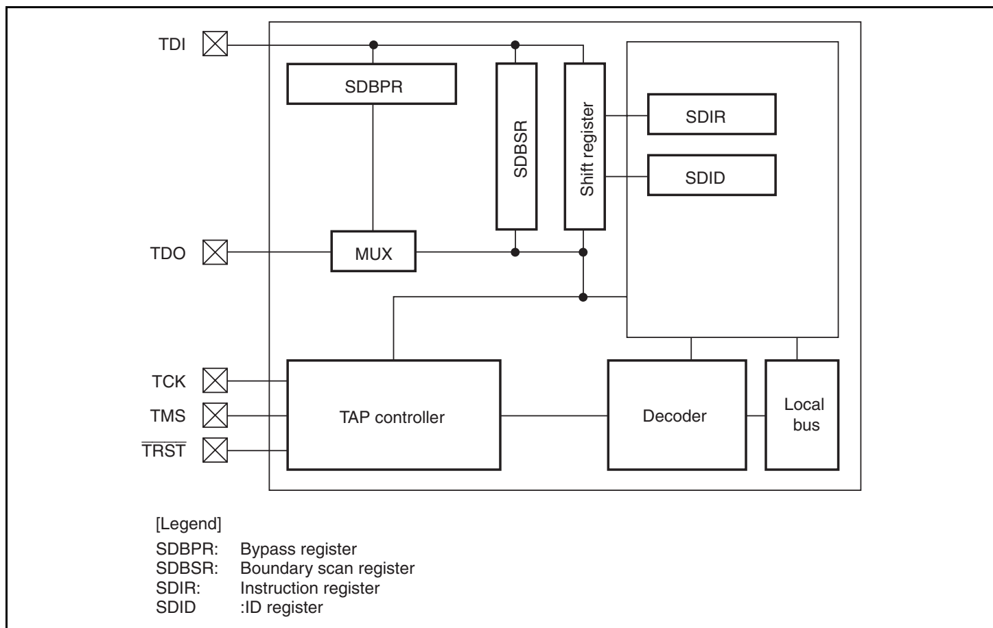
Figure 19.1 Block Diagram of H-UDI
