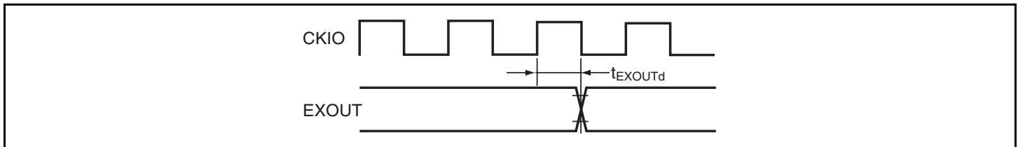
Figure 21.50 EXOUT Output Timing
