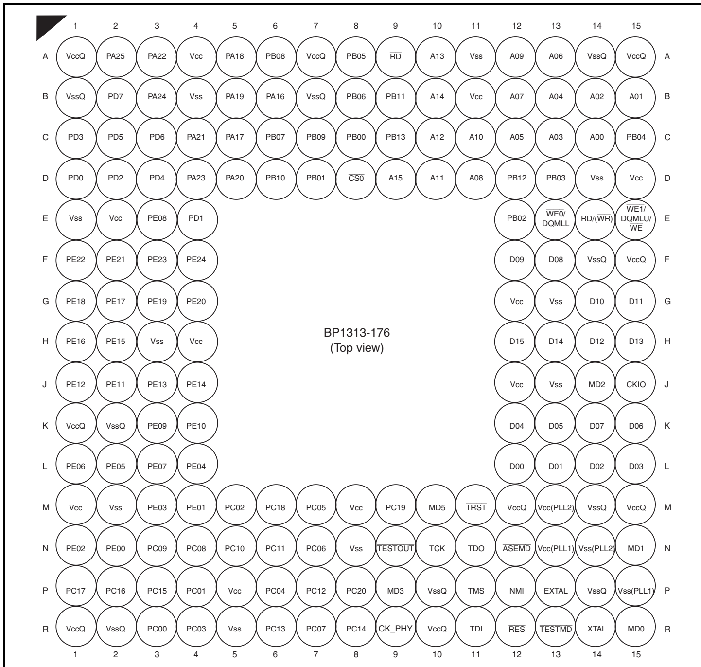
Figure 1.2 Pin Assignments
