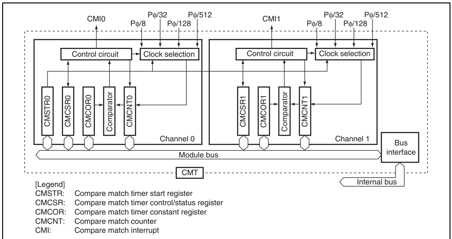
Figure 13.1 Block Diagram of Compare Match Timer
