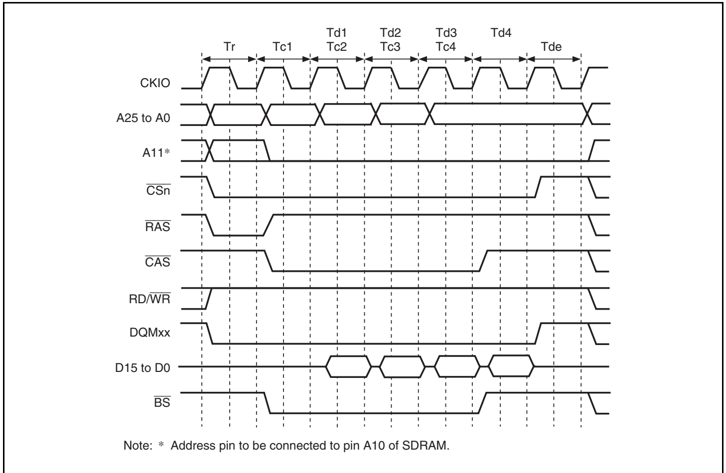
Figure 7.17 Burst Read Timing (No Auto Precharge)
