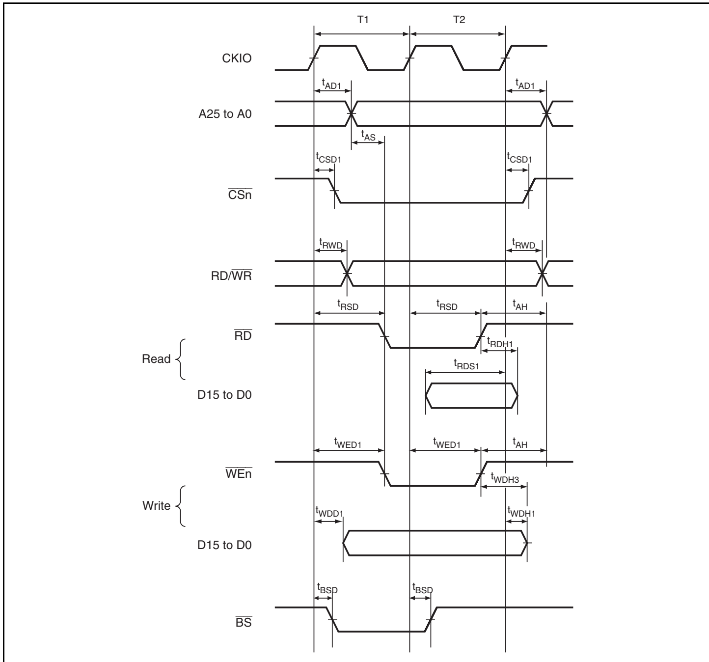
Figure 21.10 Basic Bus Timing: No Wait Cycle
