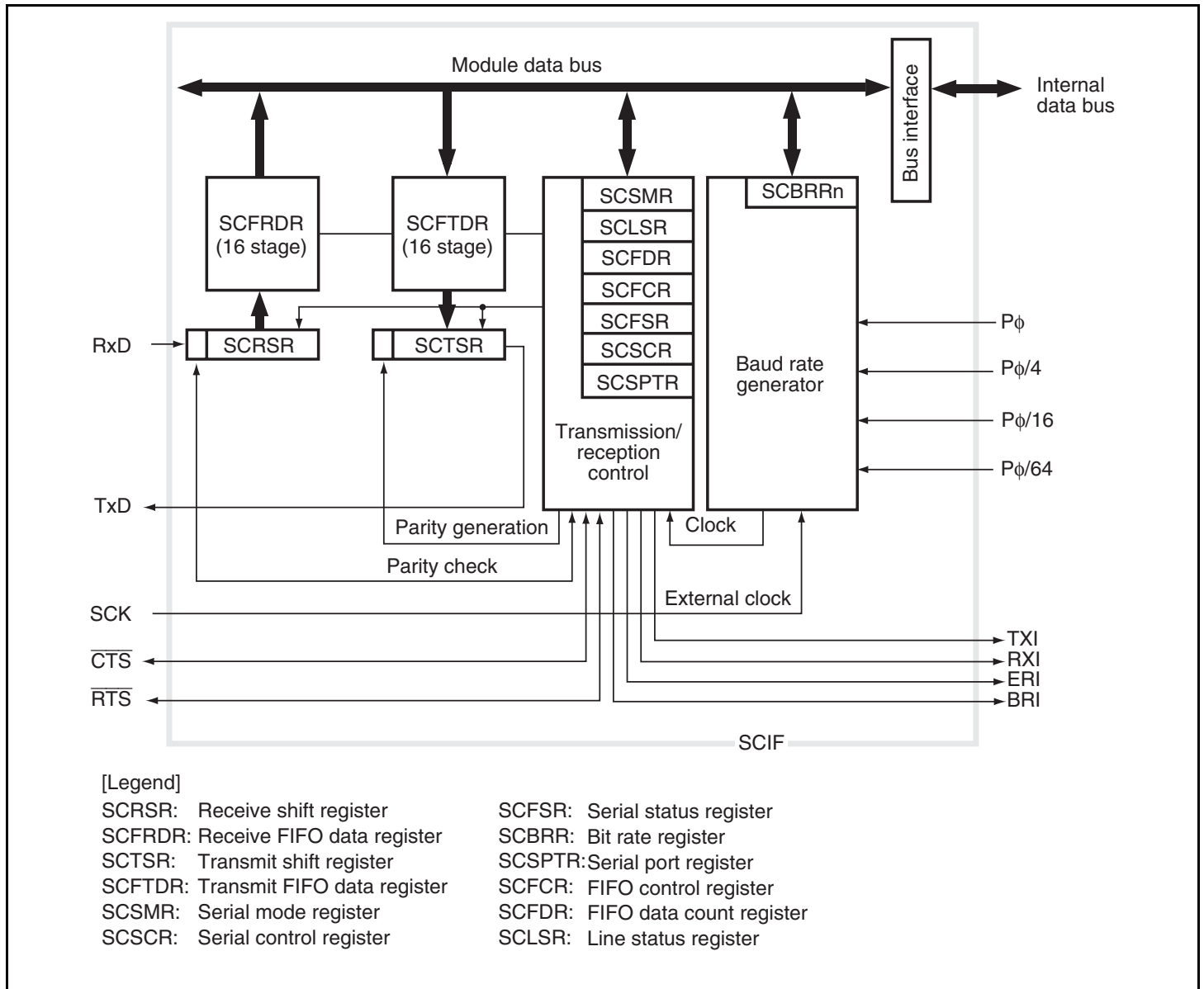
Figure 14.1 Block Diagram of SCIF
