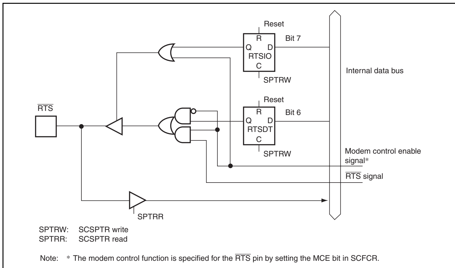
Figure 14.19 RTSIO Bit, RTSDT bit, and \overline{\text{RTS}} Pin
