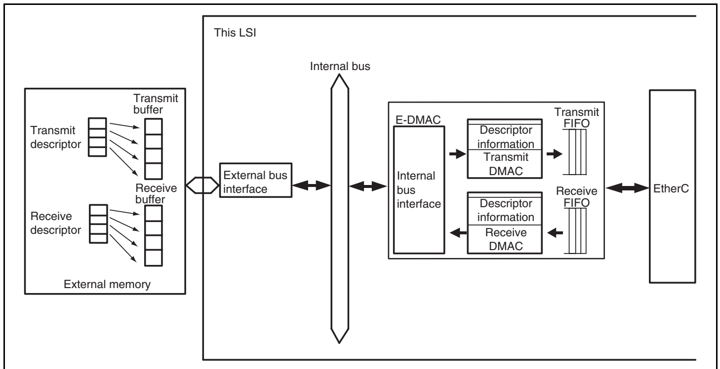
Figure 12.1 Configuration of E-DMAC, and Descriptors and Buffers
