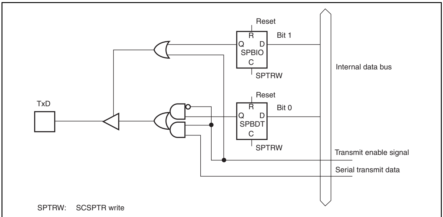
Figure 14.22 SPBIO Bit, SPBDT bit, and TxD Pin
