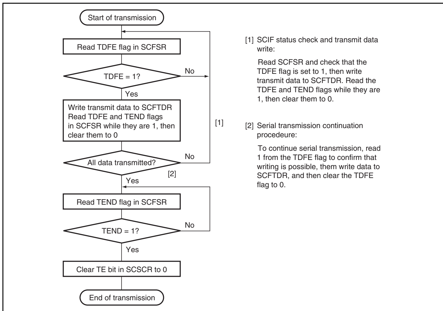
Figure 14.13 Sample Flowchart for Transmitting Serial Data
