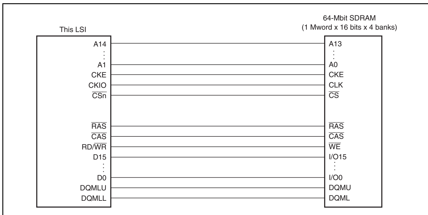
Figure 7.11 Example of 16-Bit Data-Width SDRAM Connection
