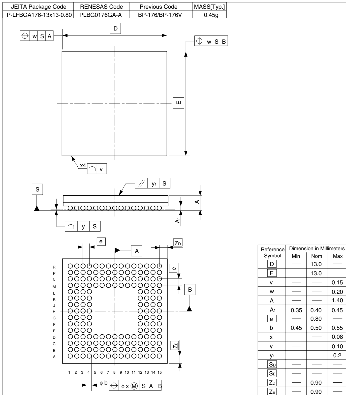
Figure C.1 Package Dimensions (BP-176)
