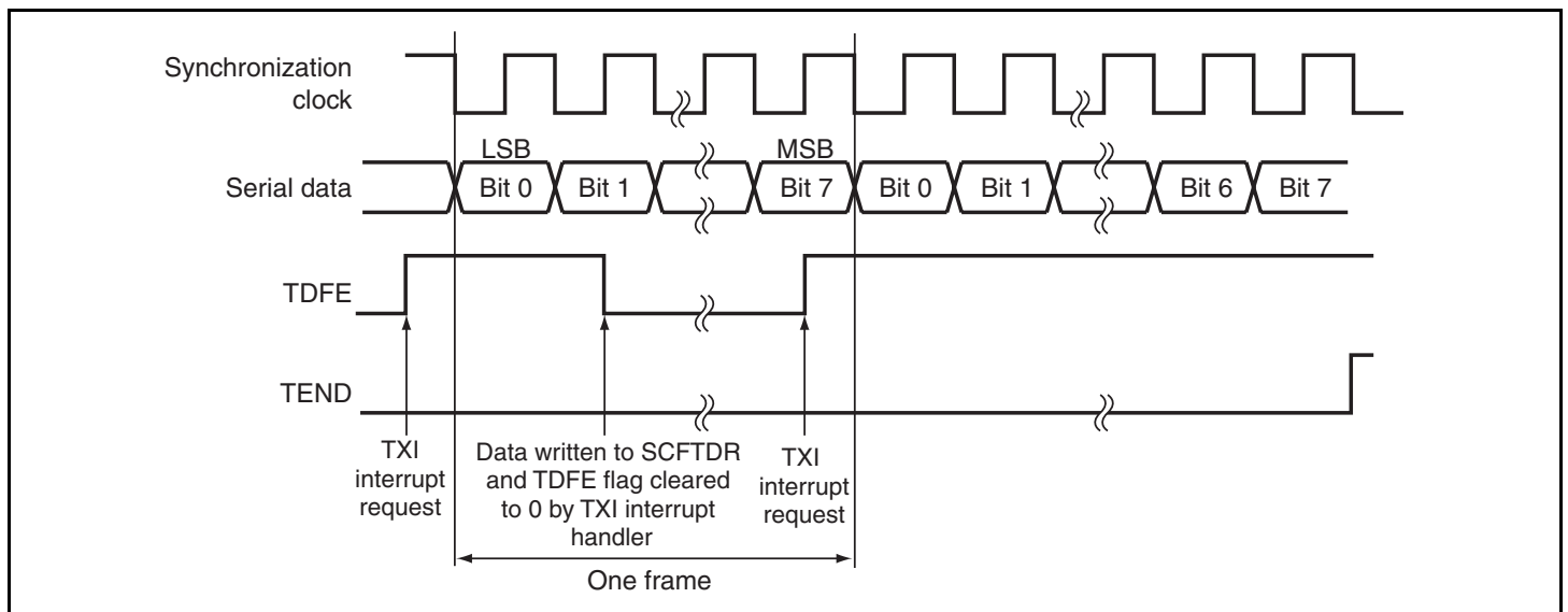
Figure 14.14 Example of SCIF Transmit Operation
