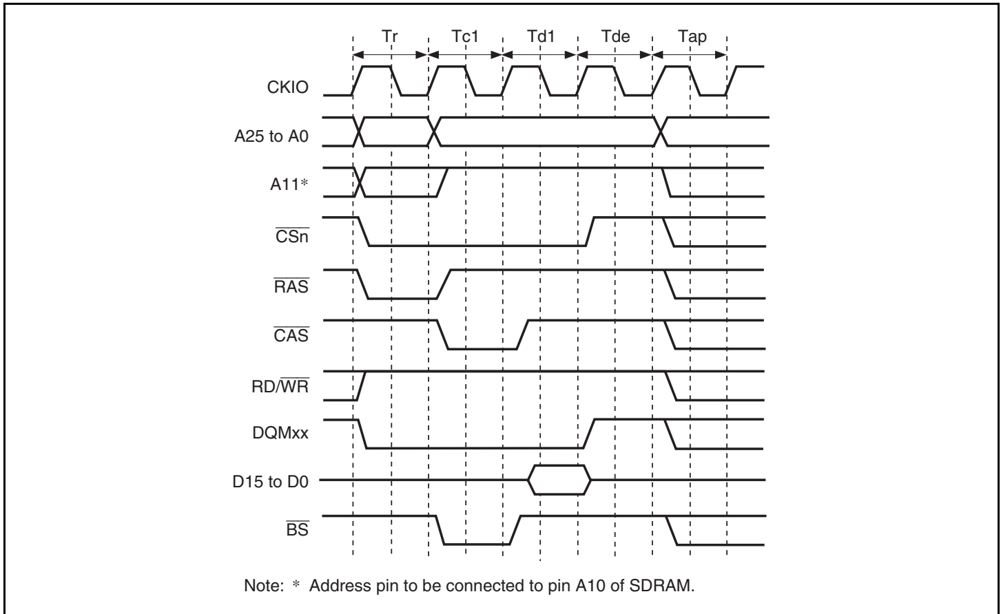
Figure 7.14 Basic Timing for Single Read (Auto Precharge)
