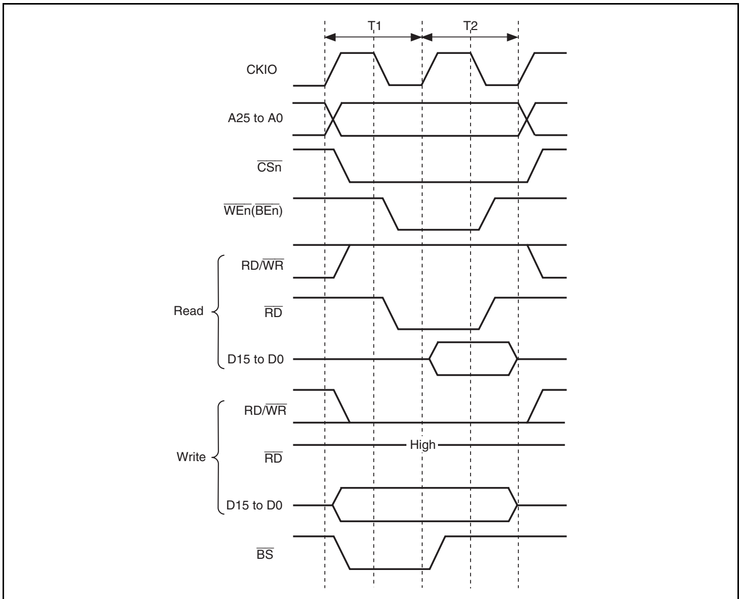
Figure 7.26 Basic Access Timing for Byte-Selection SRAM (BAS = 0)
