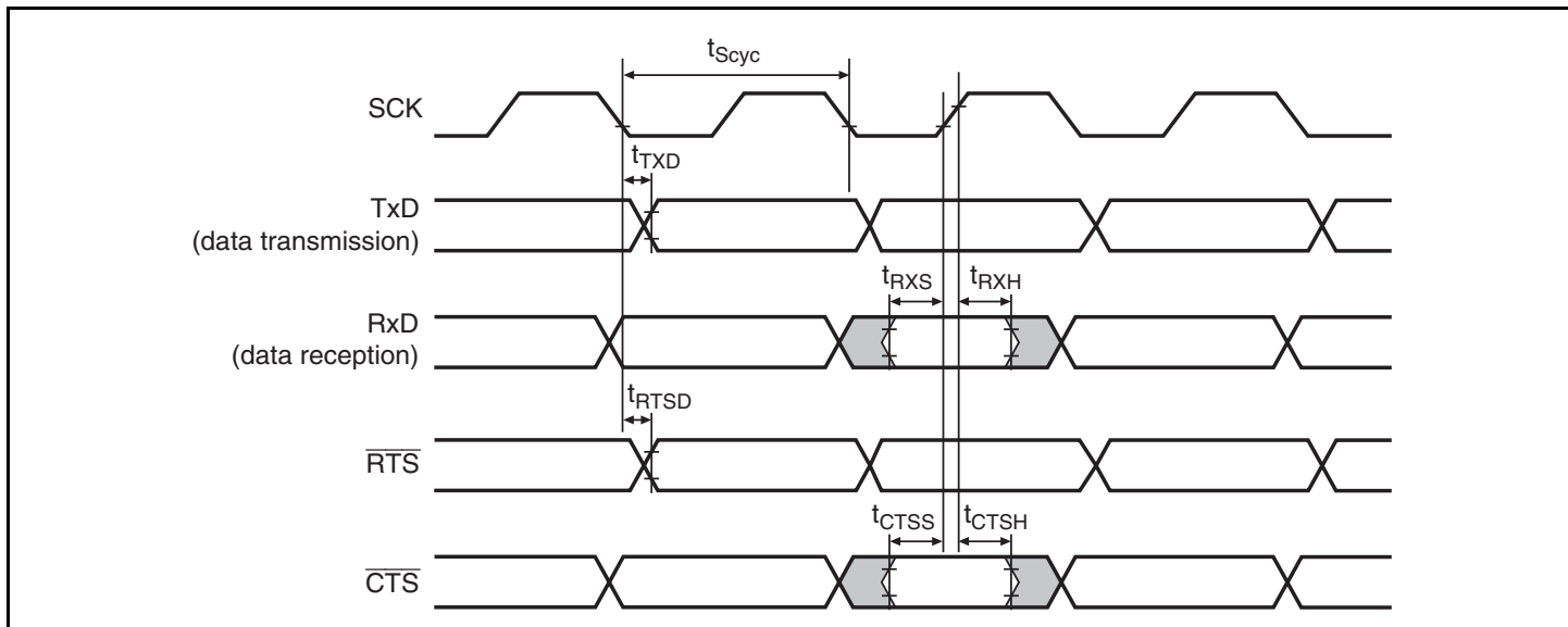
Figure 21.38 SCI Input/Output Timing in Clocked Synchronous Mode
