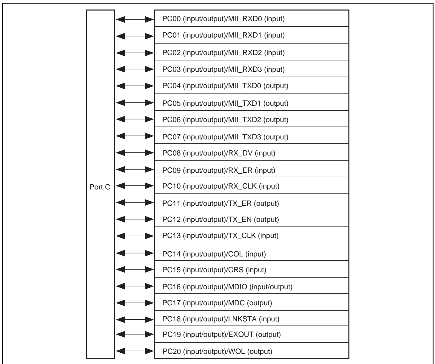
Figure 17.3 Port C
