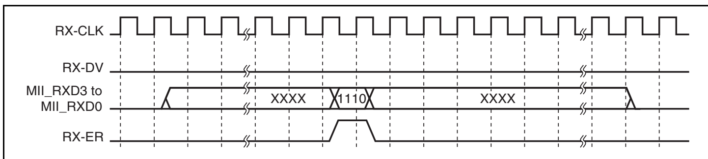
Figure 11.4 (6) MII Fame Receive Timing (Reception Error (2))
