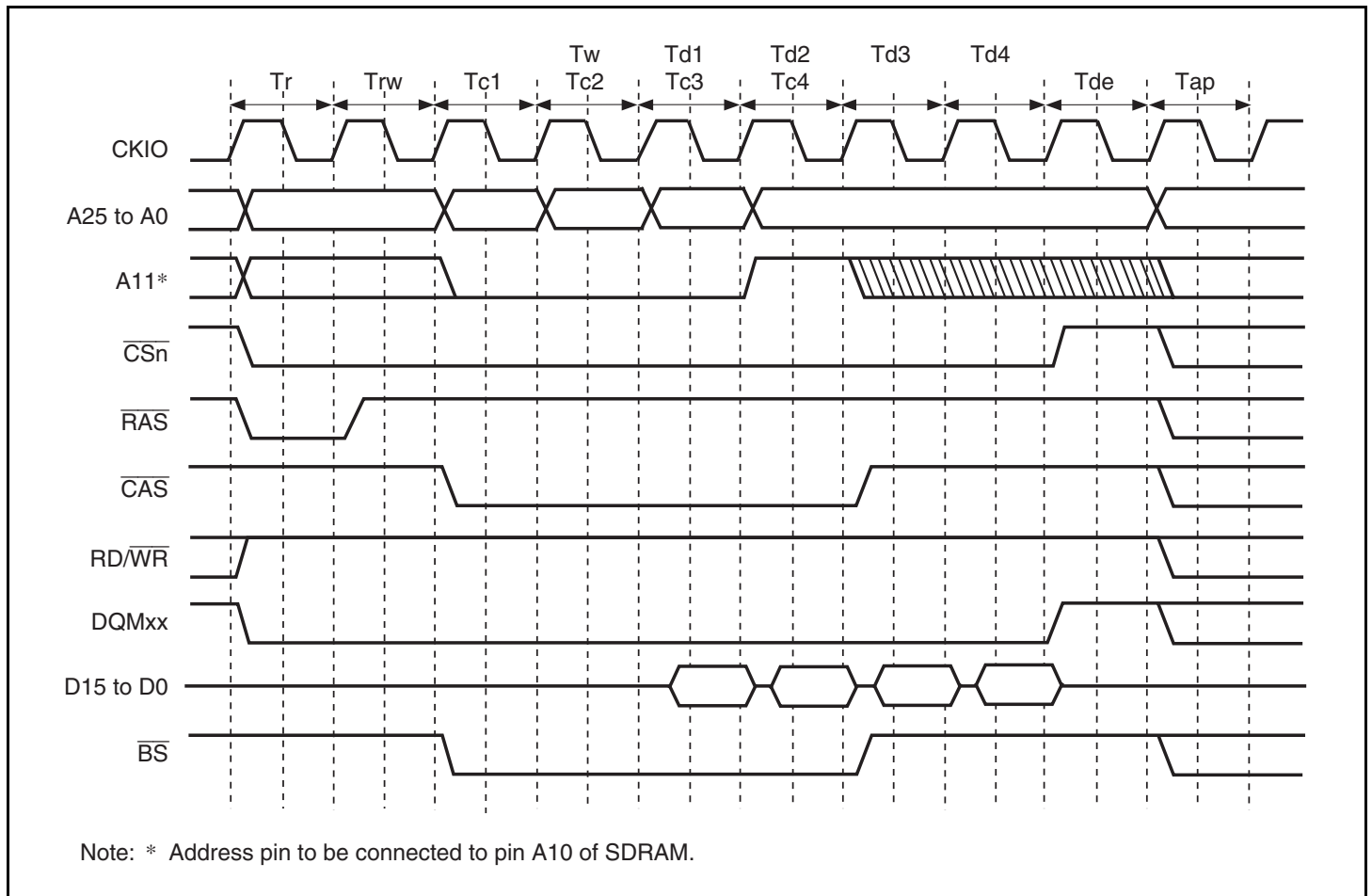
Figure 7.13 Burst Read Wait Specification Timing (Auto Precharge)
