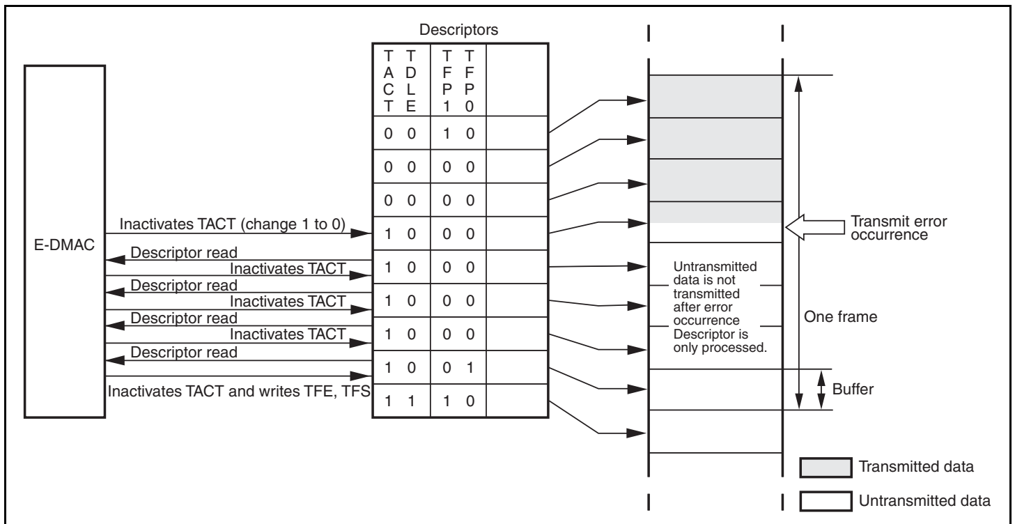
Figure 12.6 E-DMAC Operation after Transmit Error
