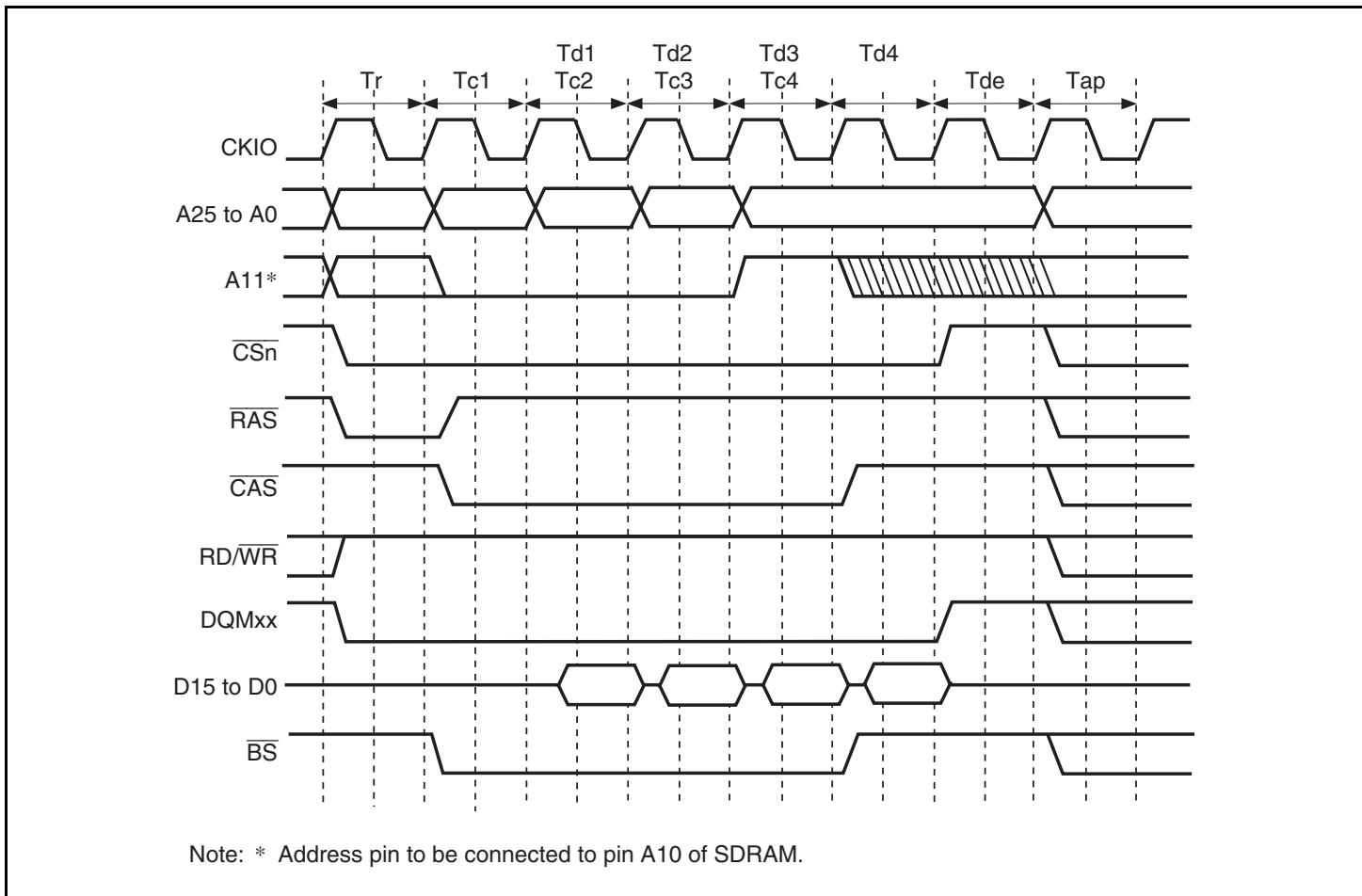
Figure 7.12 Burst Read Basic Timing (Auto Precharge)
