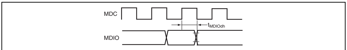
Figure 21.48 MDIO Output Timing
