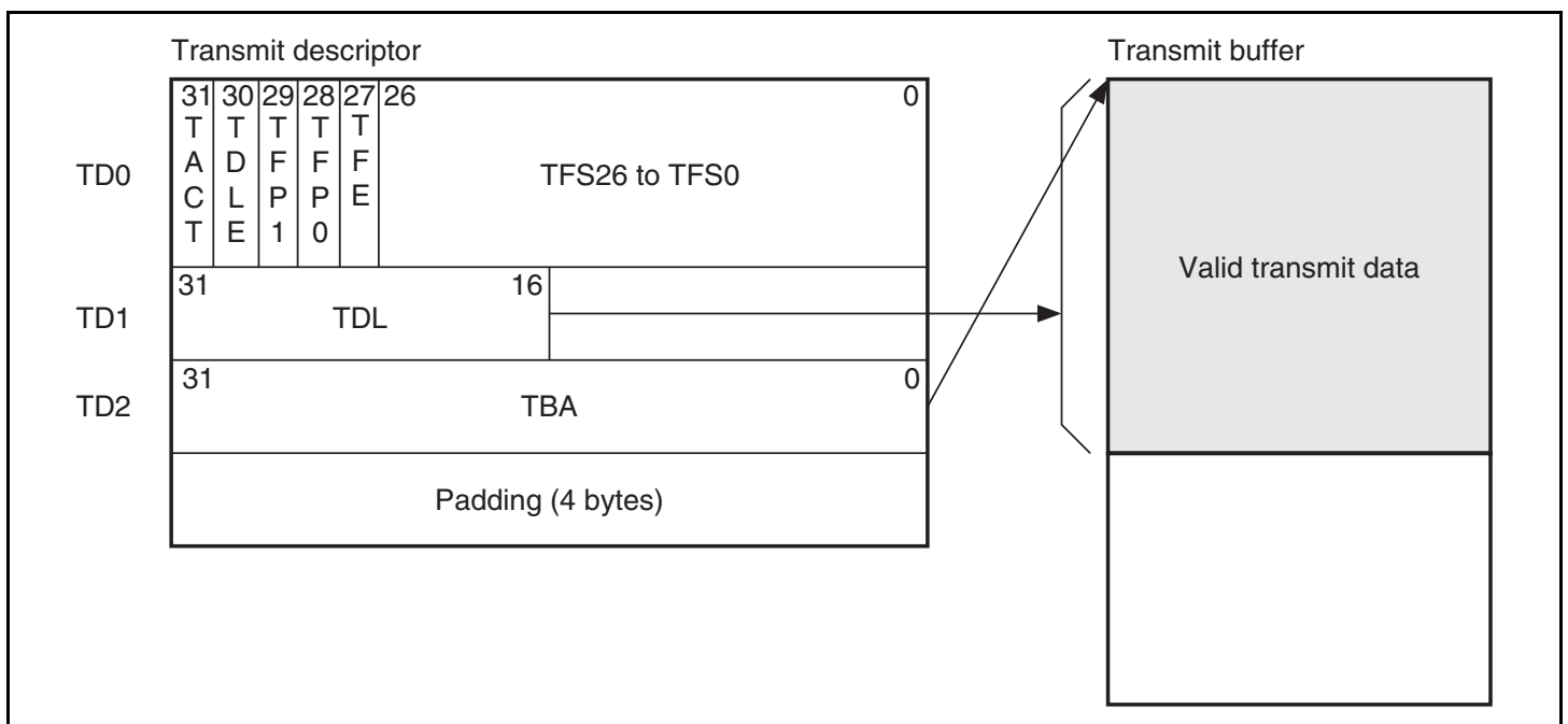
Figure 12.2 Relationship between Transmit Descriptor and Transmit Buffer
