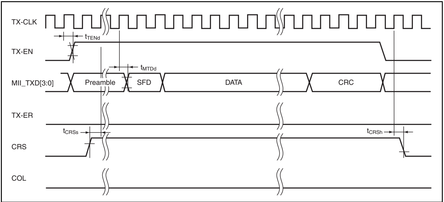
Figure 21.43 MII Transmission Timing (Normal Operation)
