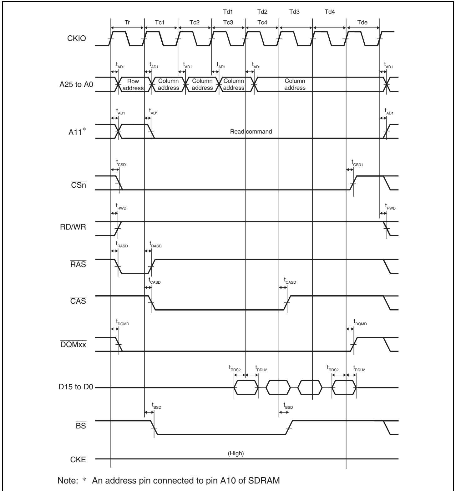
Figure 21.24 Synchronous DRAM Burst Read Bus Cycle (Single Read × 4) (Bank Active Mode: ACT + READ Commands, CAS Latency = 2, WTRCD = 0 Cycle)
