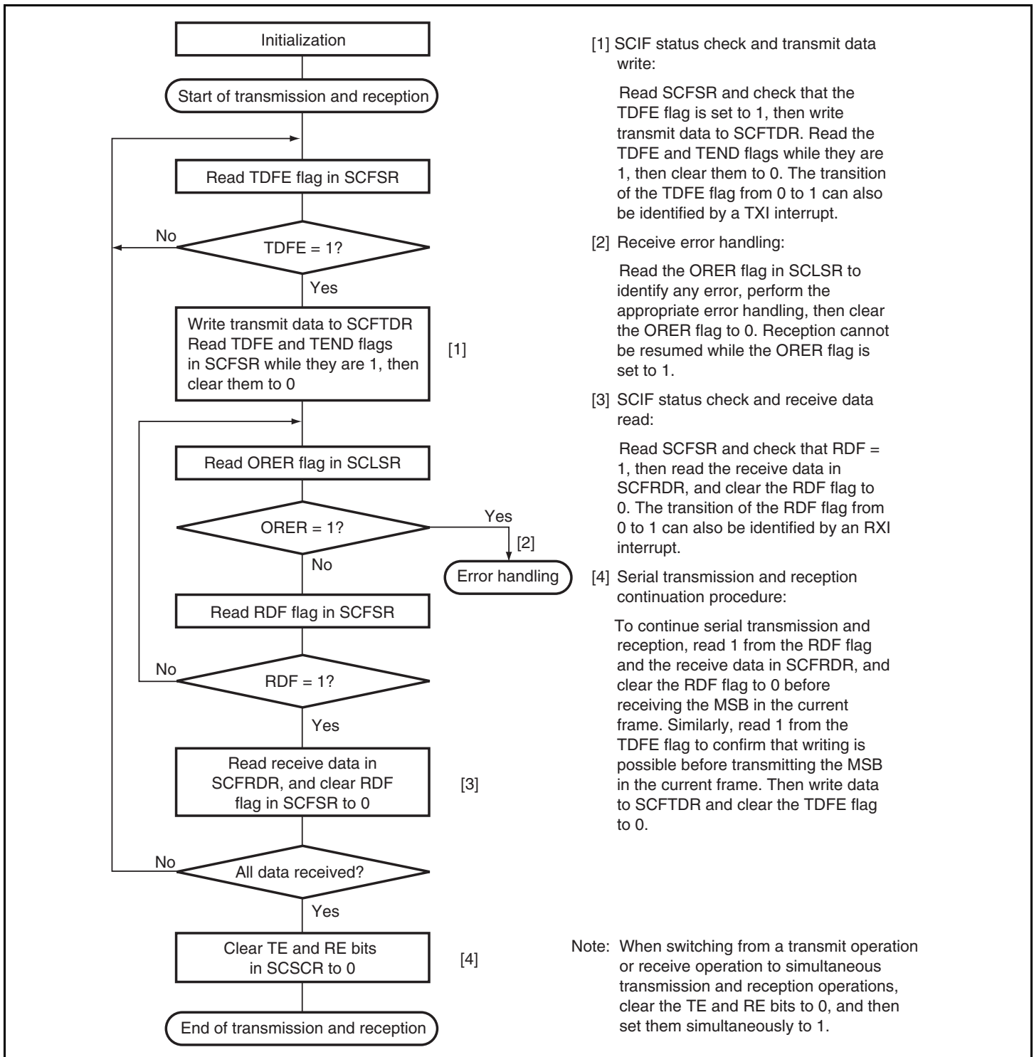
Figure 14.18 Sample Flowchart for Transmitting/Receiving Serial Data
