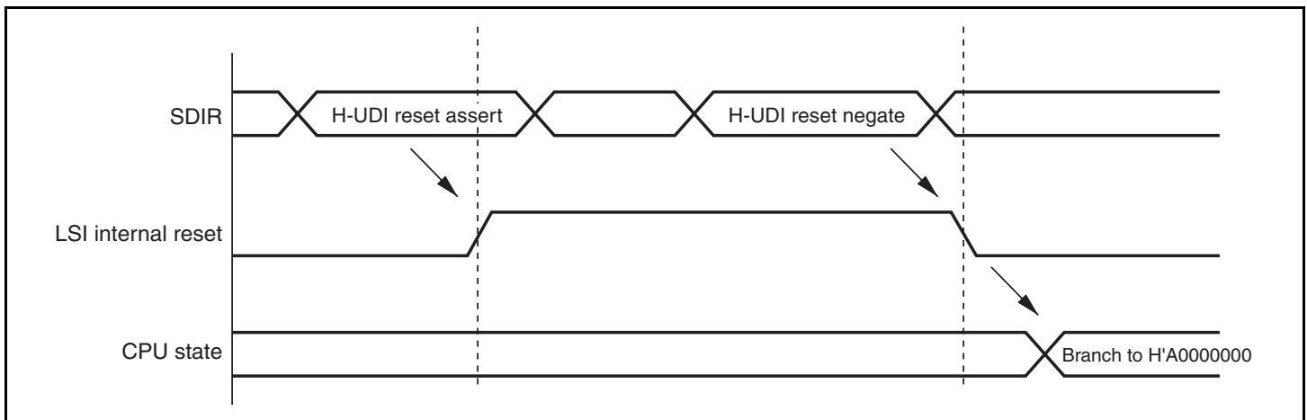
Figure 19.4 H-UDI Reset
