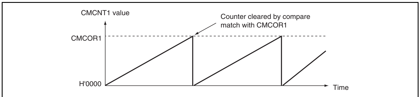
Figure 13.2 Counter Operation
