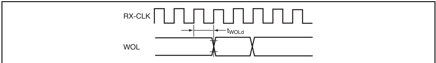
Figure 21.49 WOL Output Timing
