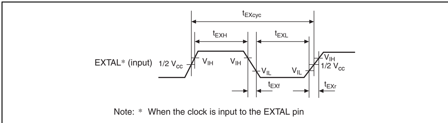
Figure 21.1 External Clock Input Timing
