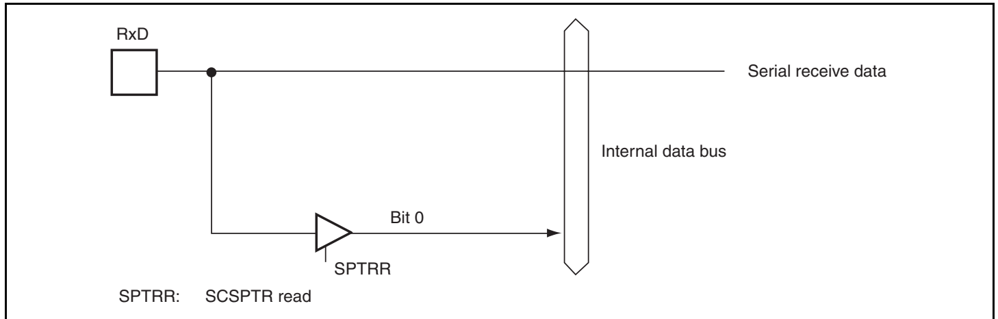
Figure 14.23 SPBDT bit and RxD Pin
