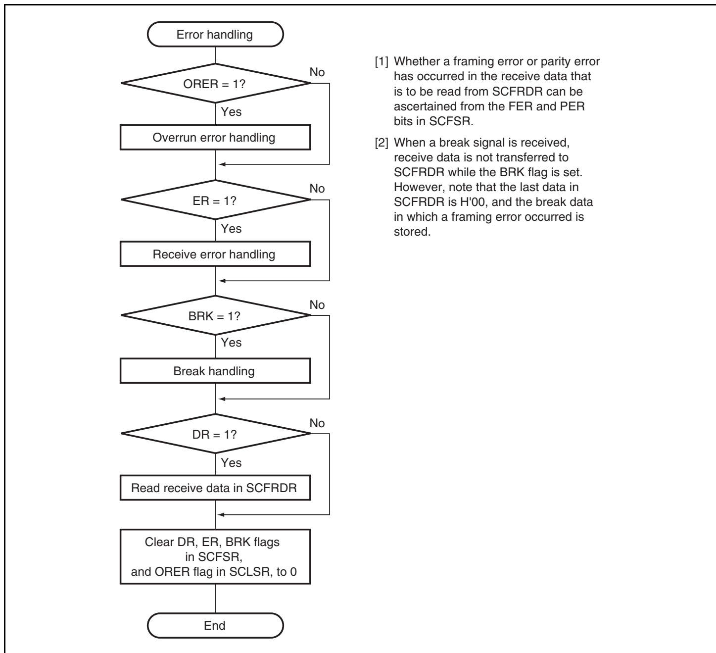
Figure 14.8 Sample Flowchart for Receiving Serial Data (cont)
