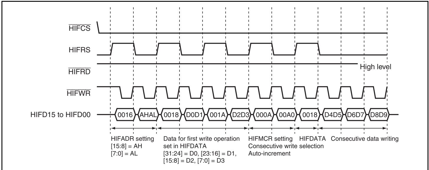
Figure 15.6 Consecutive Data Writing to HIFRAM
