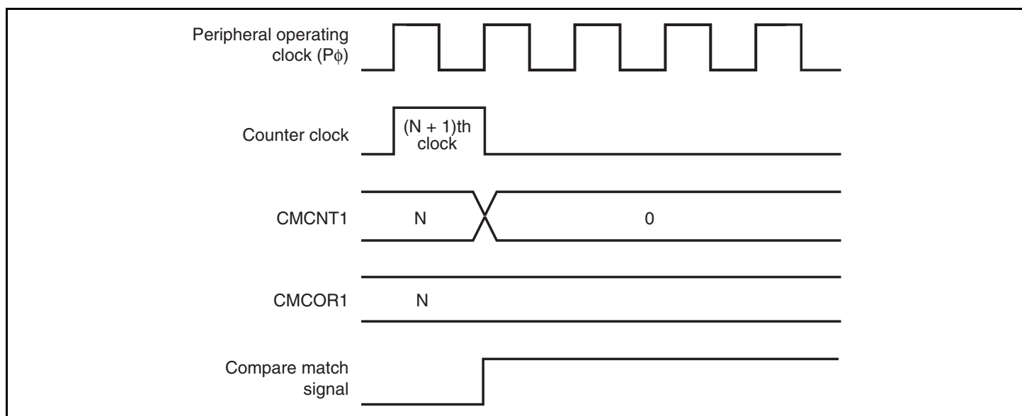
Figure 13.4 Timing of CMF Setting
