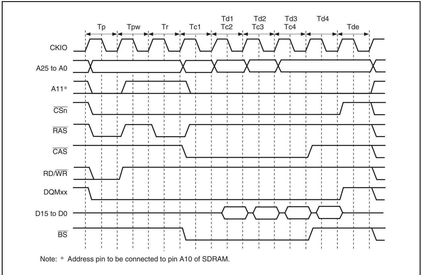
Figure 7.19 Burst Read Timing (Bank Active, Different Row Addresses)
