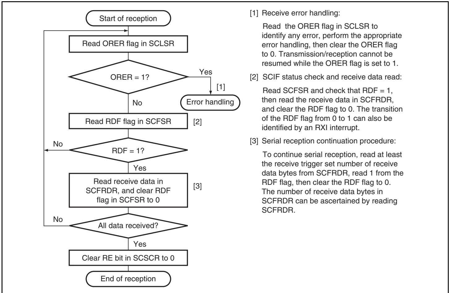
Figure 14.15 Sample Flowchart for Receiving Serial Data (1)
