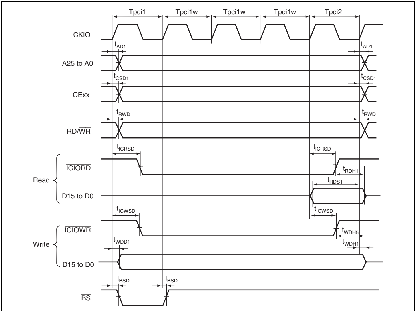
Figure 21.35 PCMCIA I/O Card Interface Bus Timing
