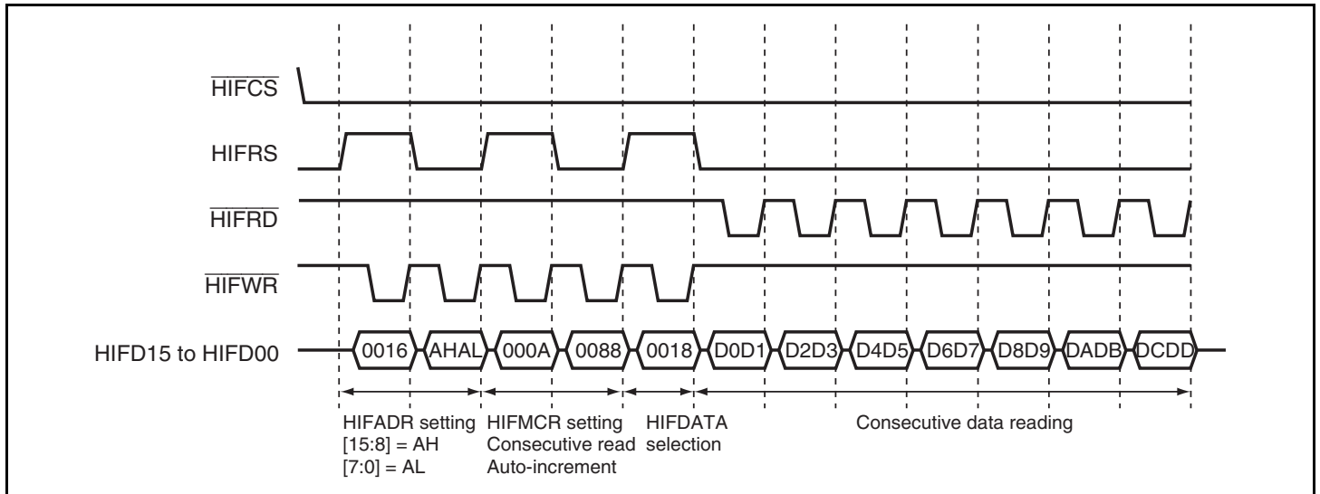
Figure 15.7 Consecutive Data Reading from HIFRAM
