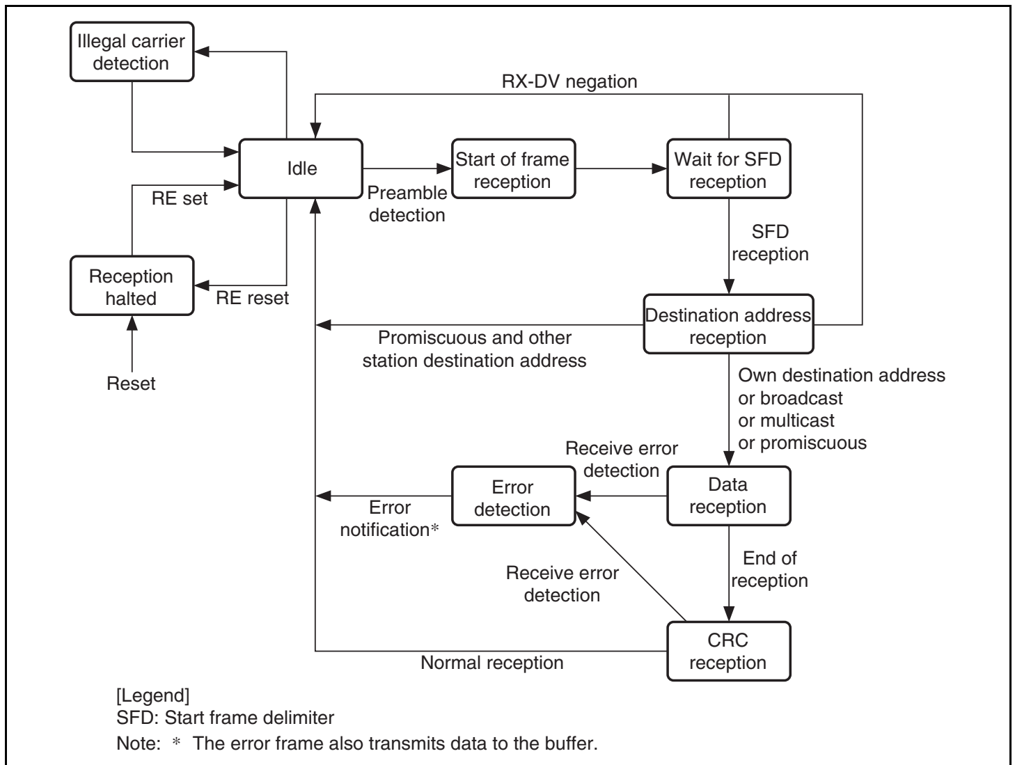
Figure 11.3 EtherC Receiver State Transmissions
