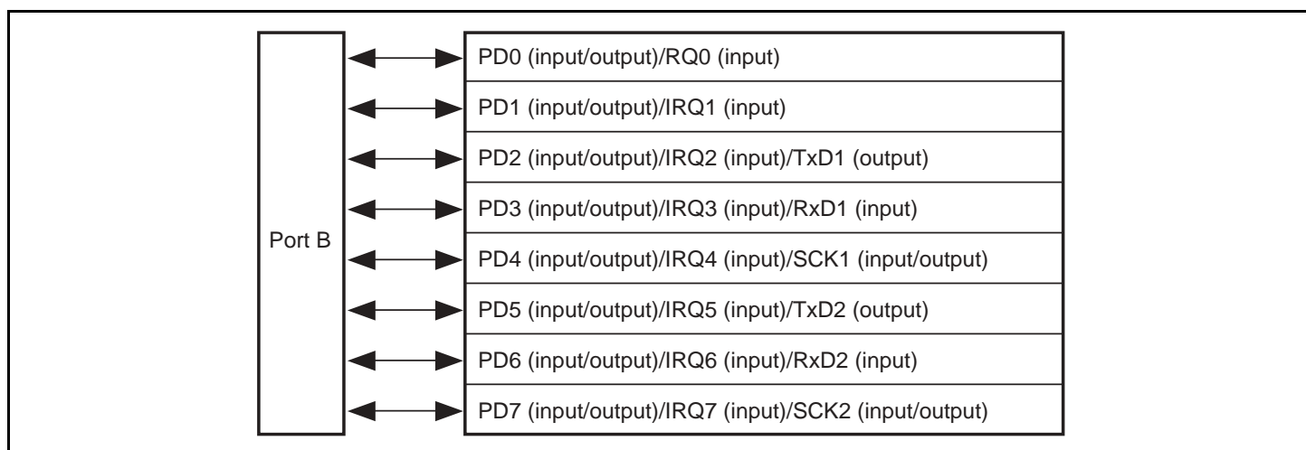
Figure 17.4 Port D
