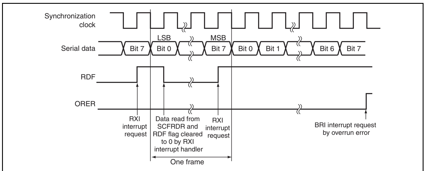
Figure 14.17 Example of SCIF Receive Operation
