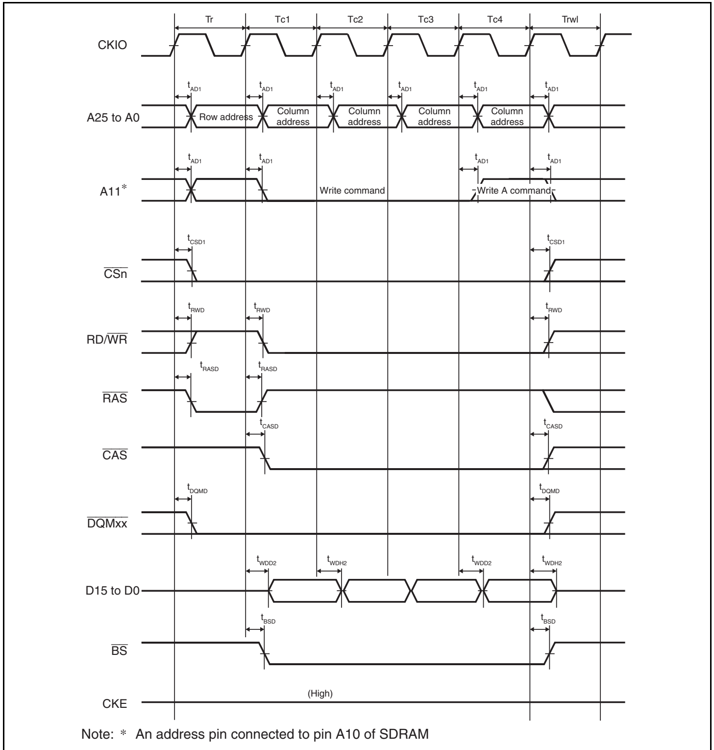
Figure 21.22 Synchronous DRAM Burst Write Bus Cycle (Single Write × 4) (Auto-Precharge, WTRCD = 0 Cycle, TRWL = 1 Cycle)
