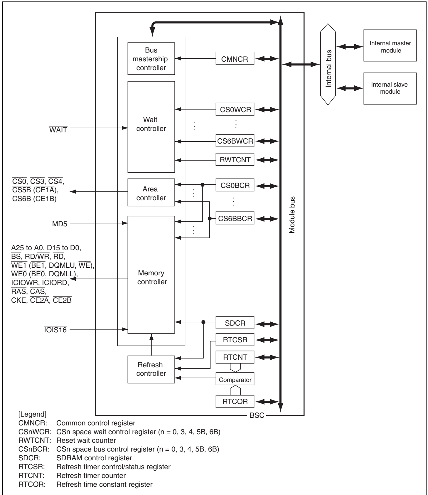
Figure 7.1 Block Diagram of BSC
