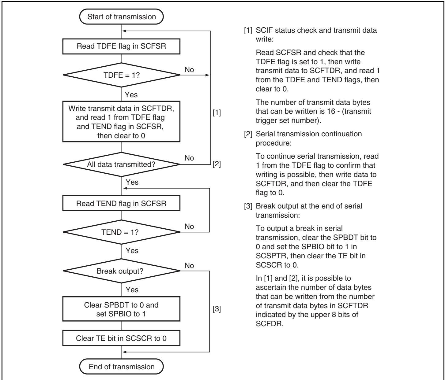
Figure 14.4 Sample Flowchart for Transmitting Serial Data
