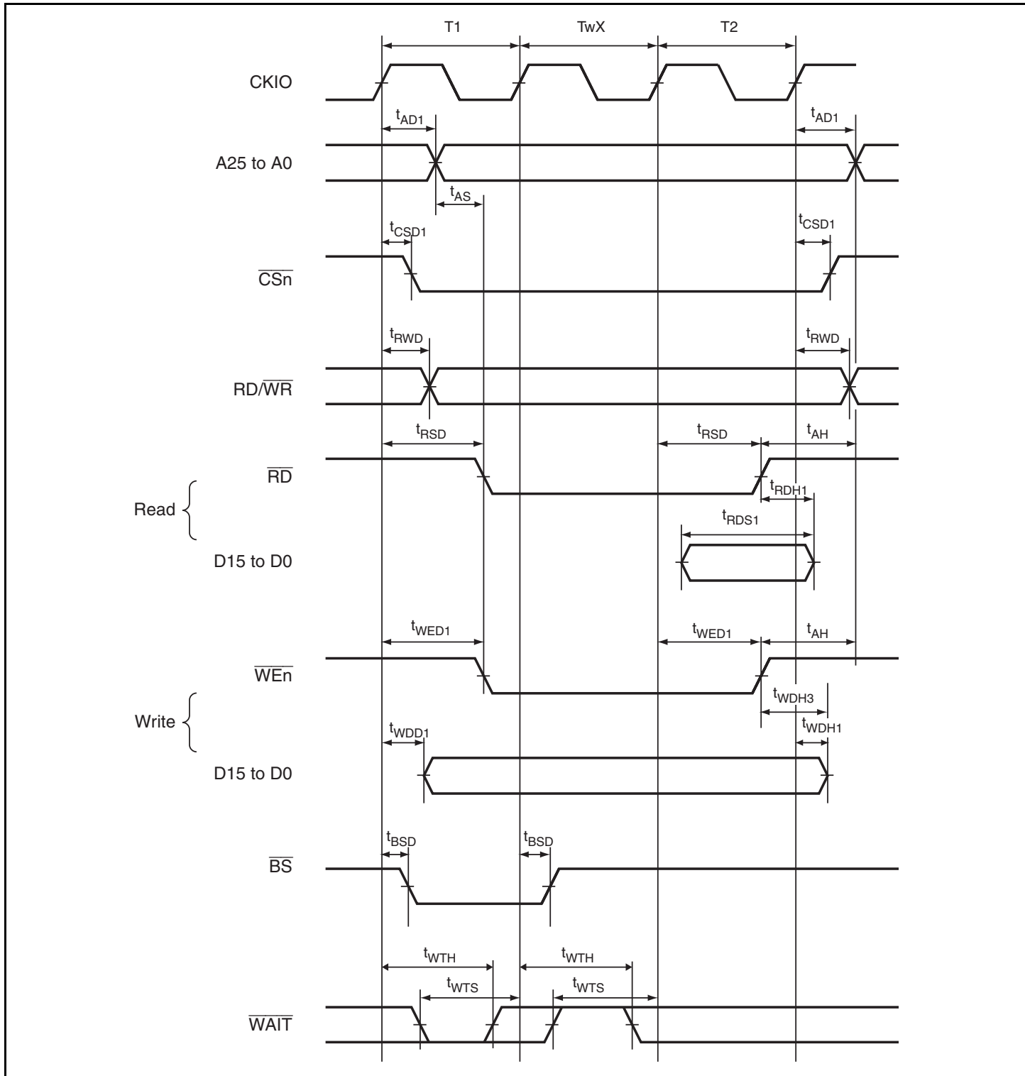
Figure 21.12 Basic Bus Timing: One External Wait Cycle
