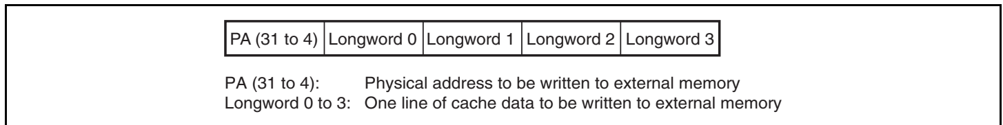
Figure 3.3 Write-Back Buffer Configuration
