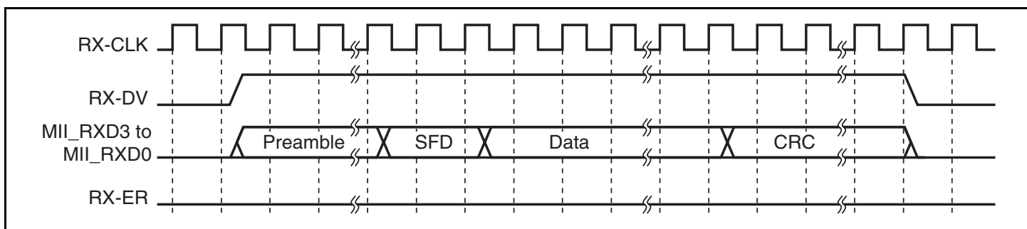
Figure 11.4 (4) MII Frame Receive Timing (Normal Reception)
