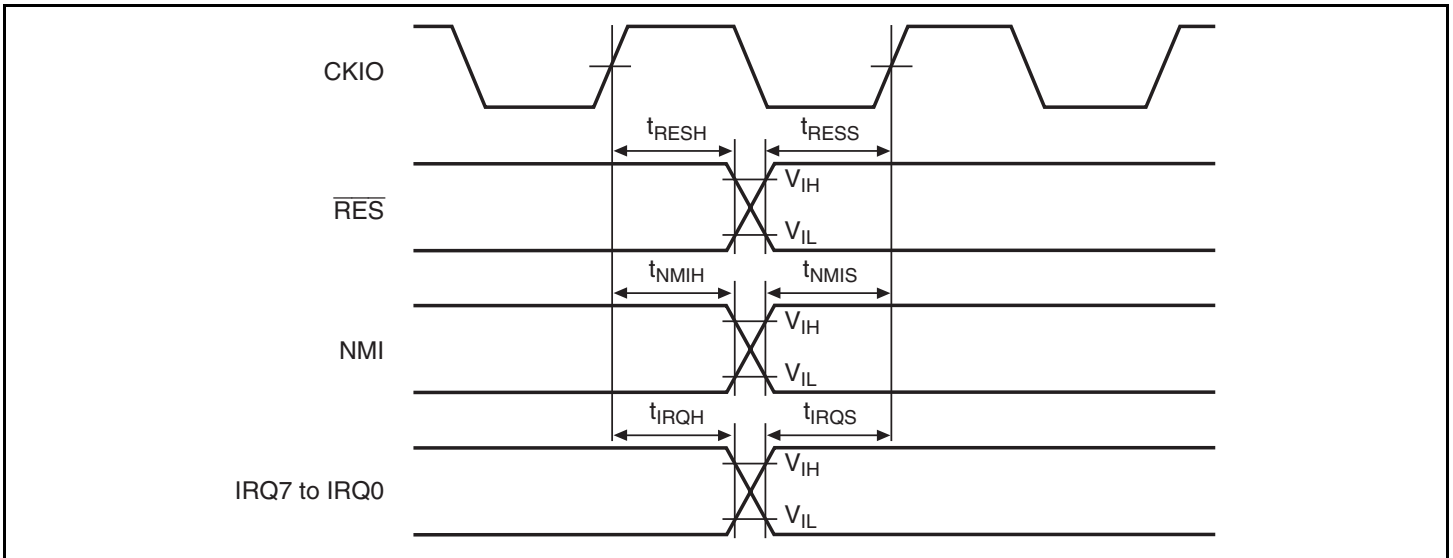
Figure 21.8 Interrupt Input Timing
