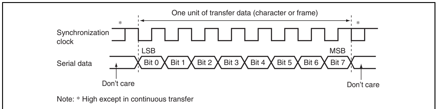
Figure 14.11 Data Format in Synchronous Communication
