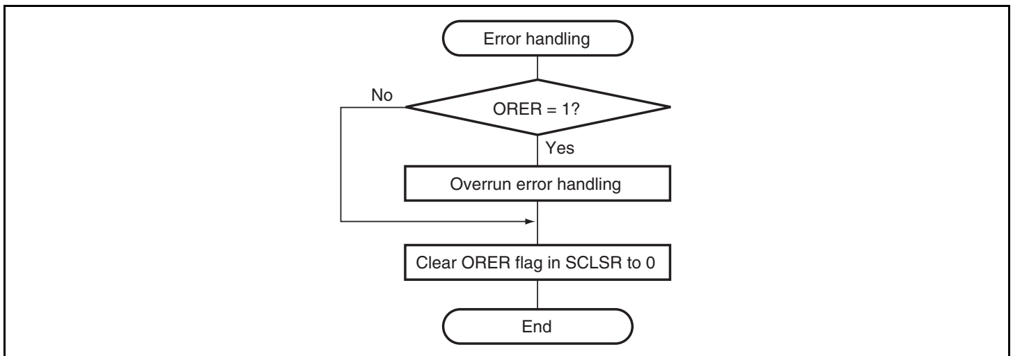
Figure 14.16 Sample Flowchart for Receiving Serial Data (2)
