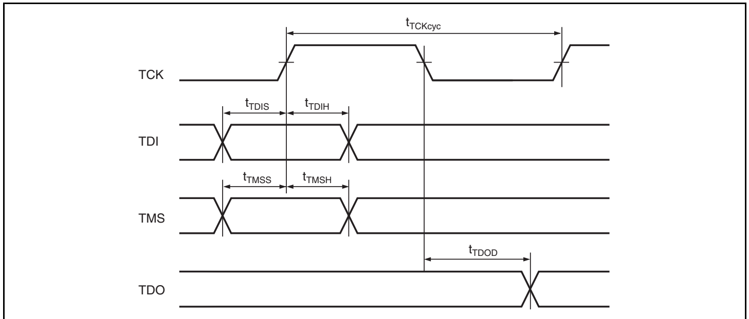
Figure 21.53 H-UDI Data Transmission Timing
