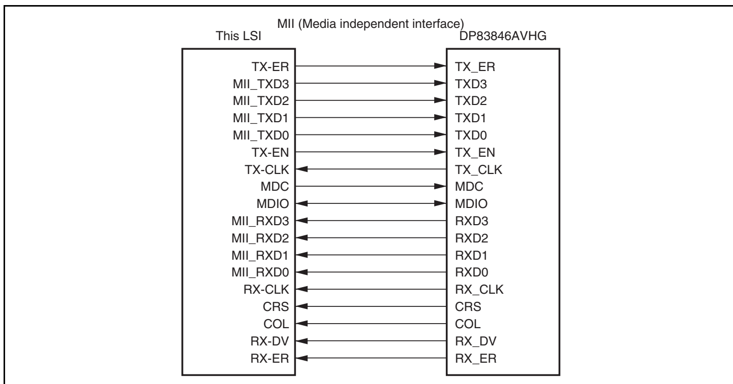
Figure 11.8 Example of Connection to DP83846AVHG
