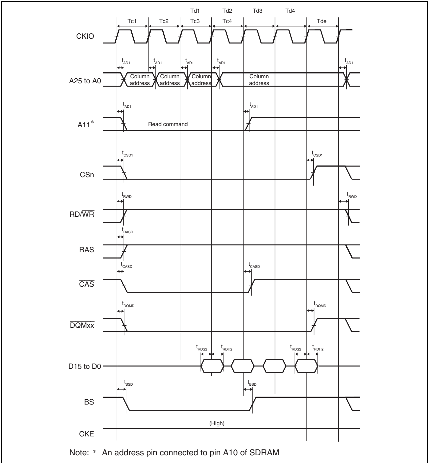
Figure 21.25 Synchronous DRAM Burst Read Bus Cycle (Single Read × 4) (Bank Active Mode: READ Command, Same Row Address, CAS Latency = 2, WTRCD = 0 Cycle)
