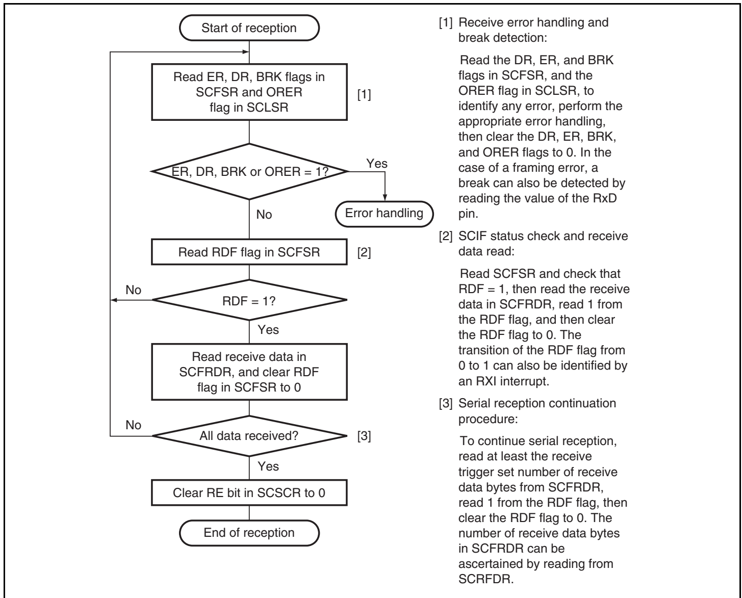
Figure 14.7 Sample Flowchart for Receiving Serial Data
