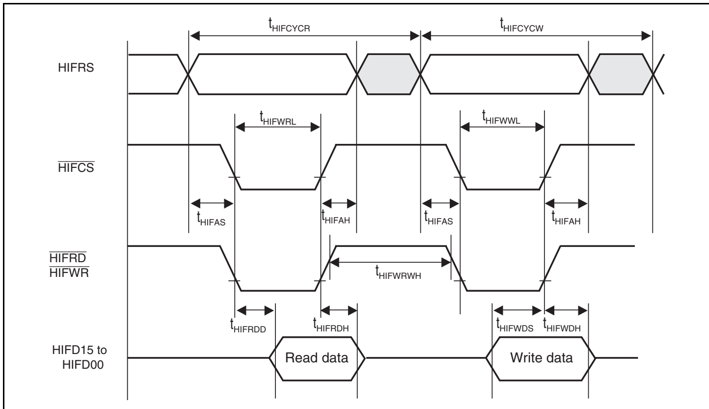
Figure 21.40 HIF Access Timing
