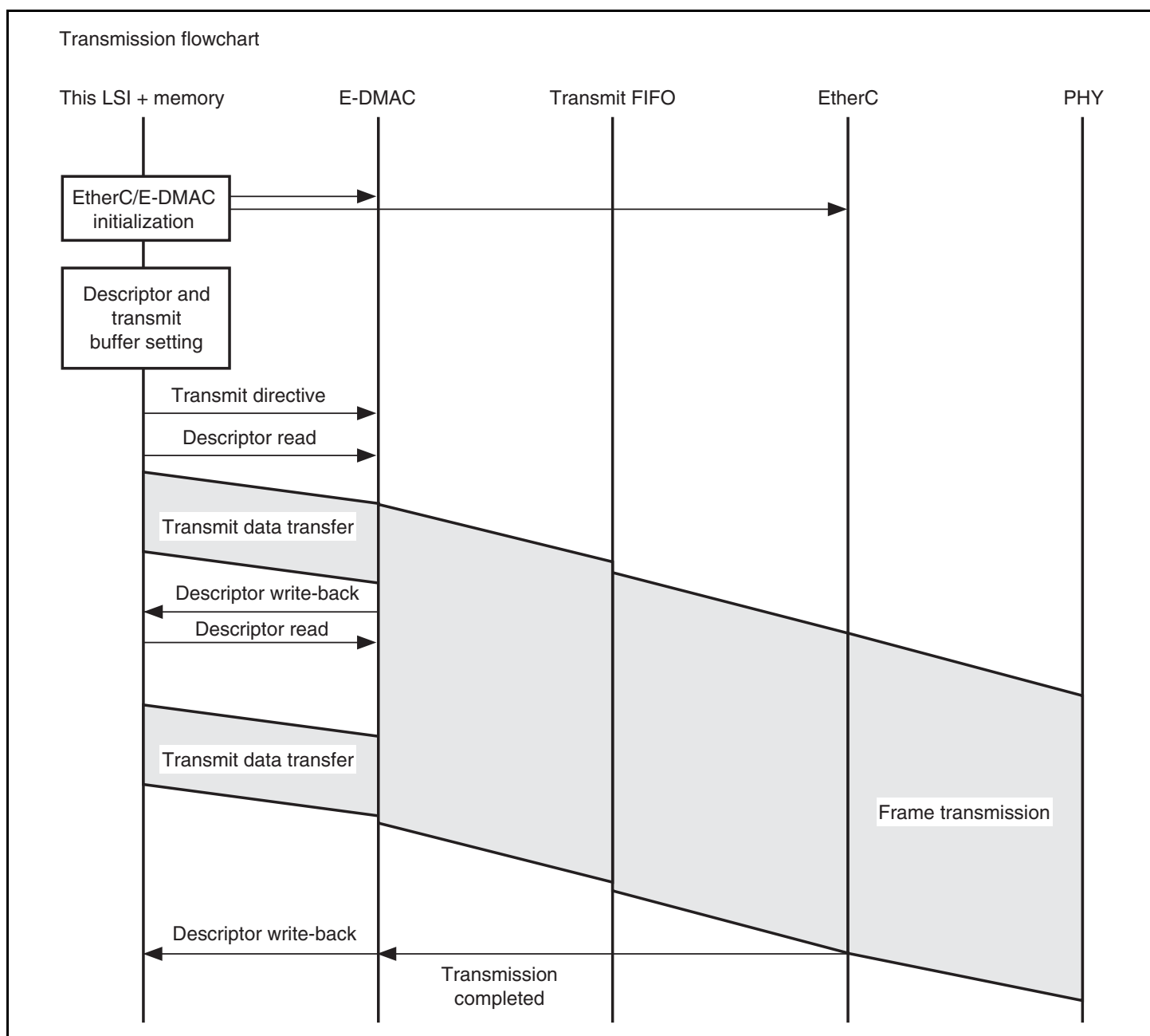
Figure 12.4 Sample Transmission Flowchart
