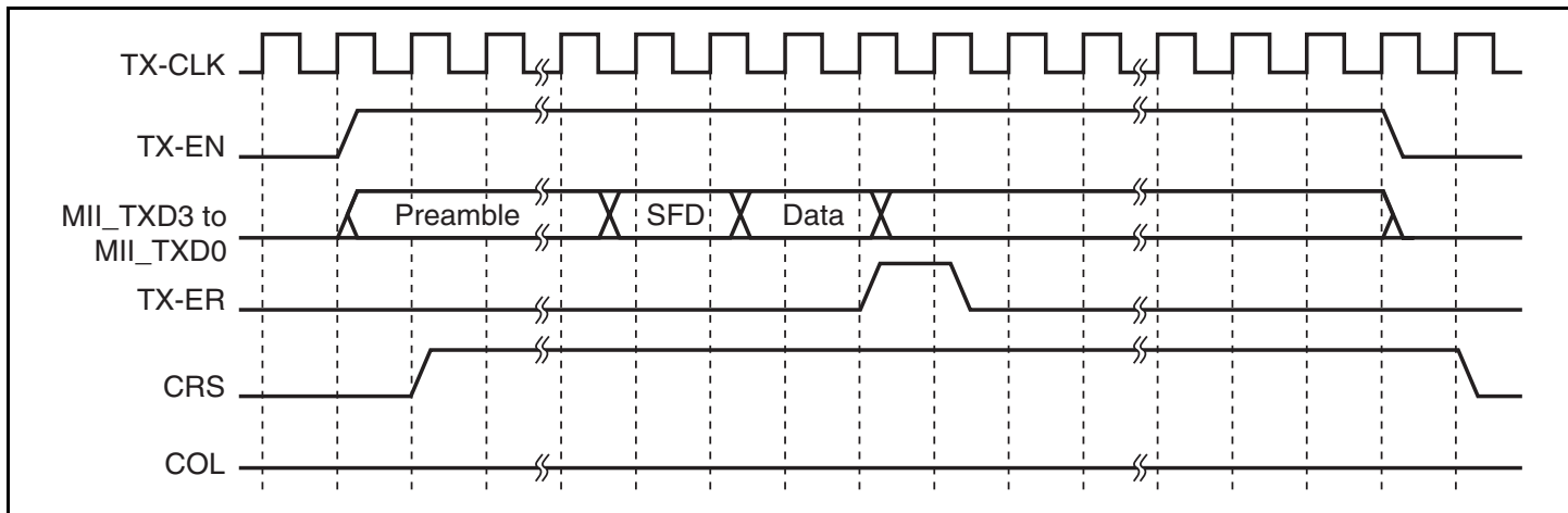
Figure 11.4 (3) MII Frame Transmit Timing (Transmit Error)
