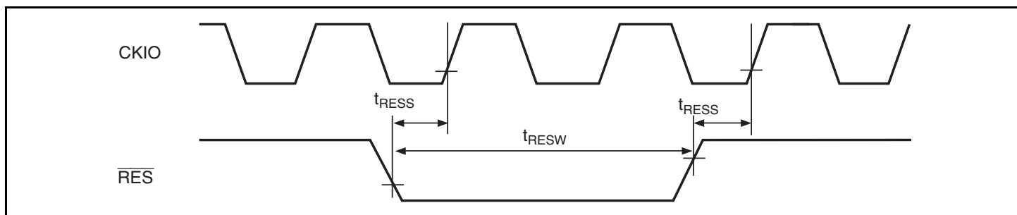
Figure 21.7 Reset Input Timing
