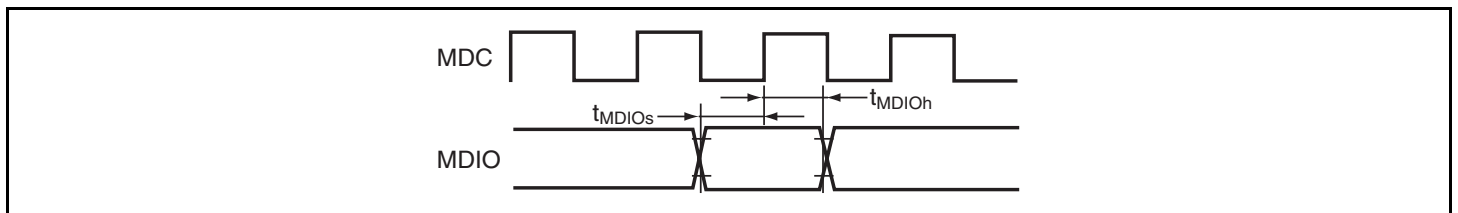
Figure 21.47 MDIO Input Timing
