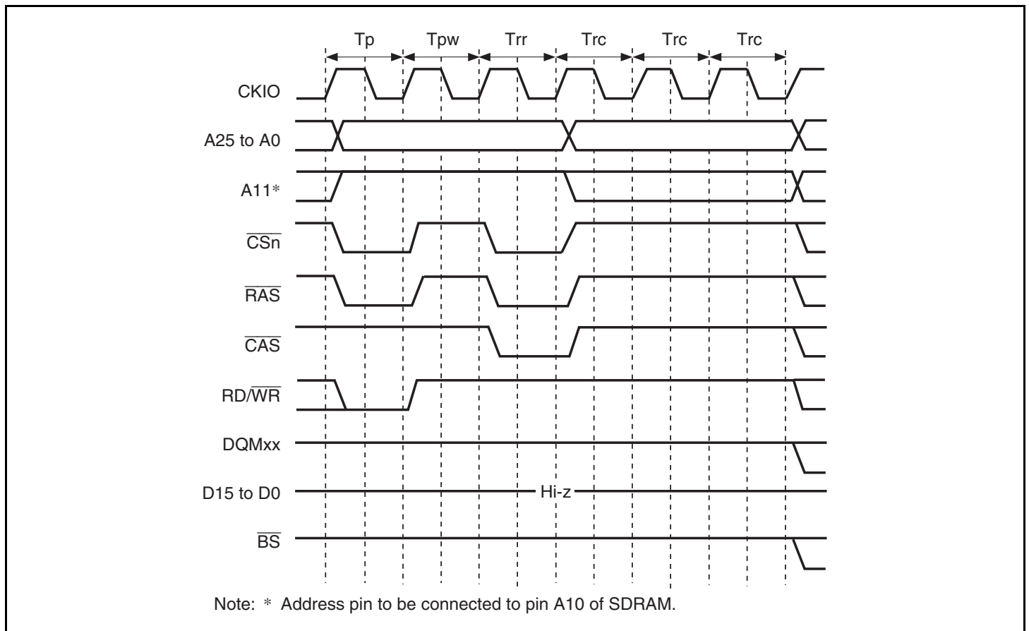
Figure 7.23 Auto-Refreshing Timing
