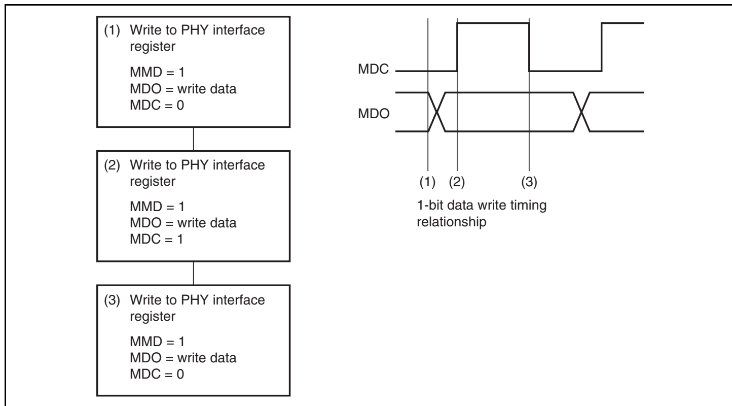
Figure 11.6 (1) 1-Bit Data Write Flowchart
