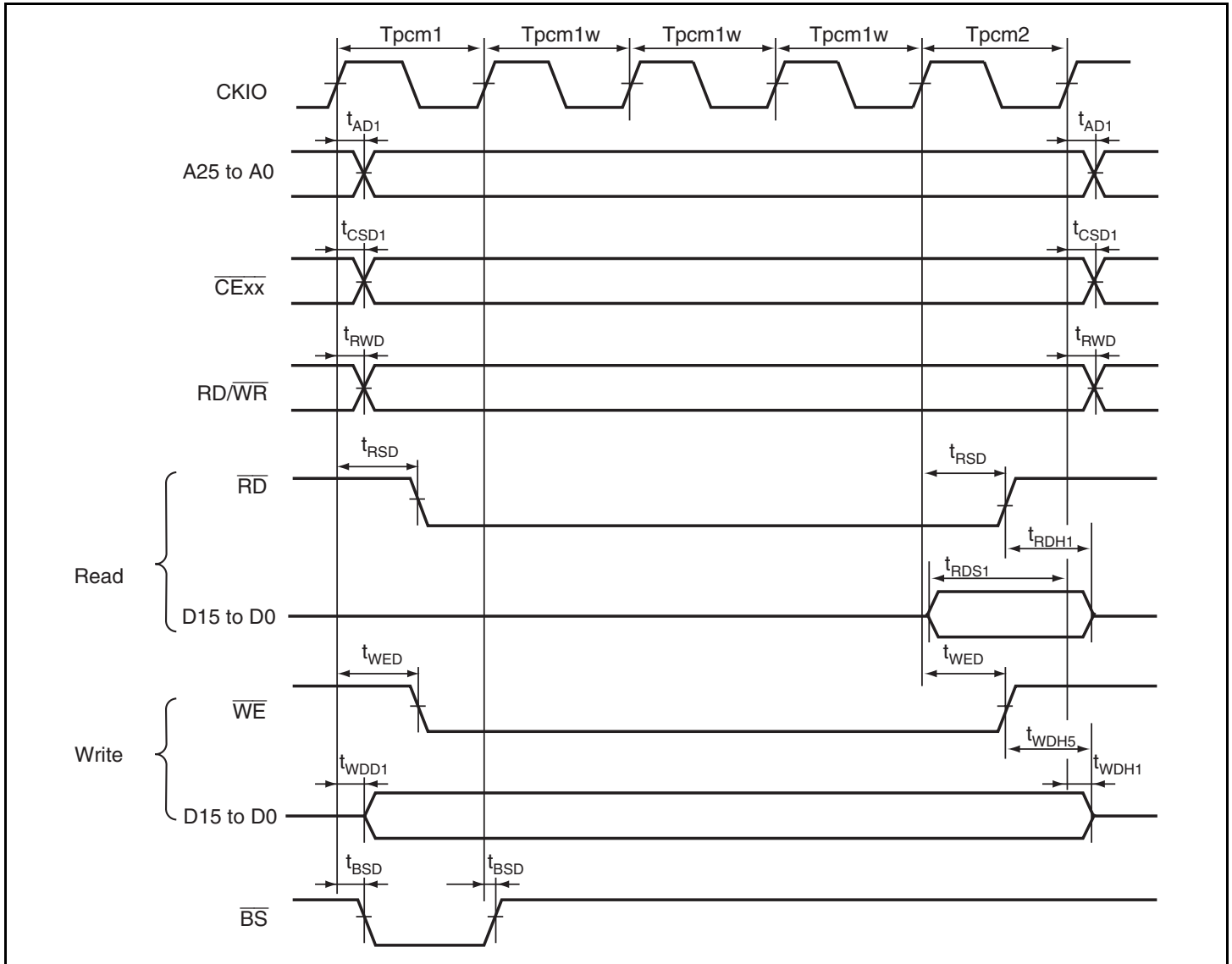
Figure 21.33 PCMCIA Memory Card Interface Bus Timing
