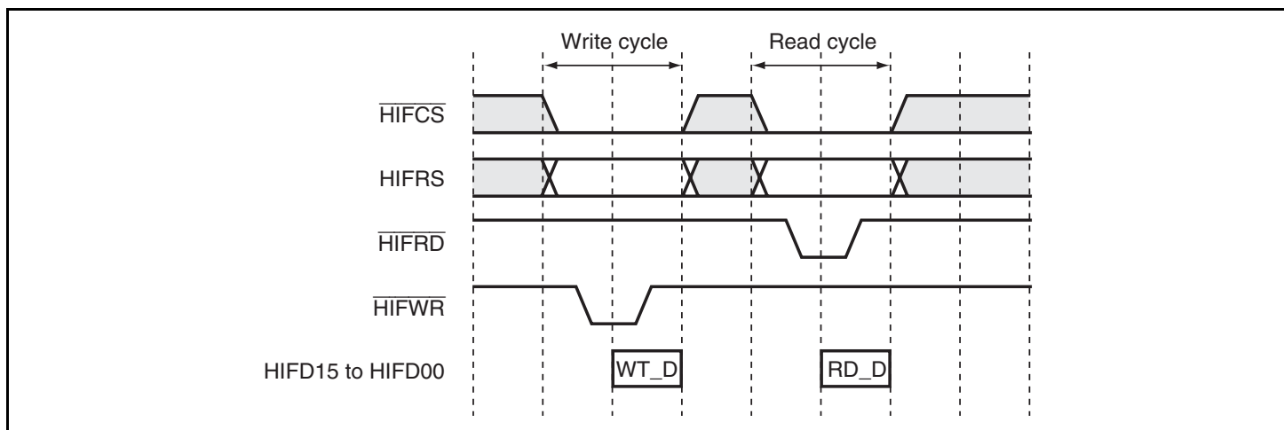
Figure 15.3 Basic Timing for HIF Interface
