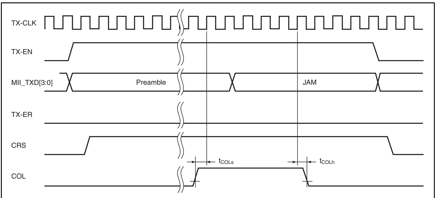
Figure 21.44 MII Transmission Timing (Collision Occurred)
