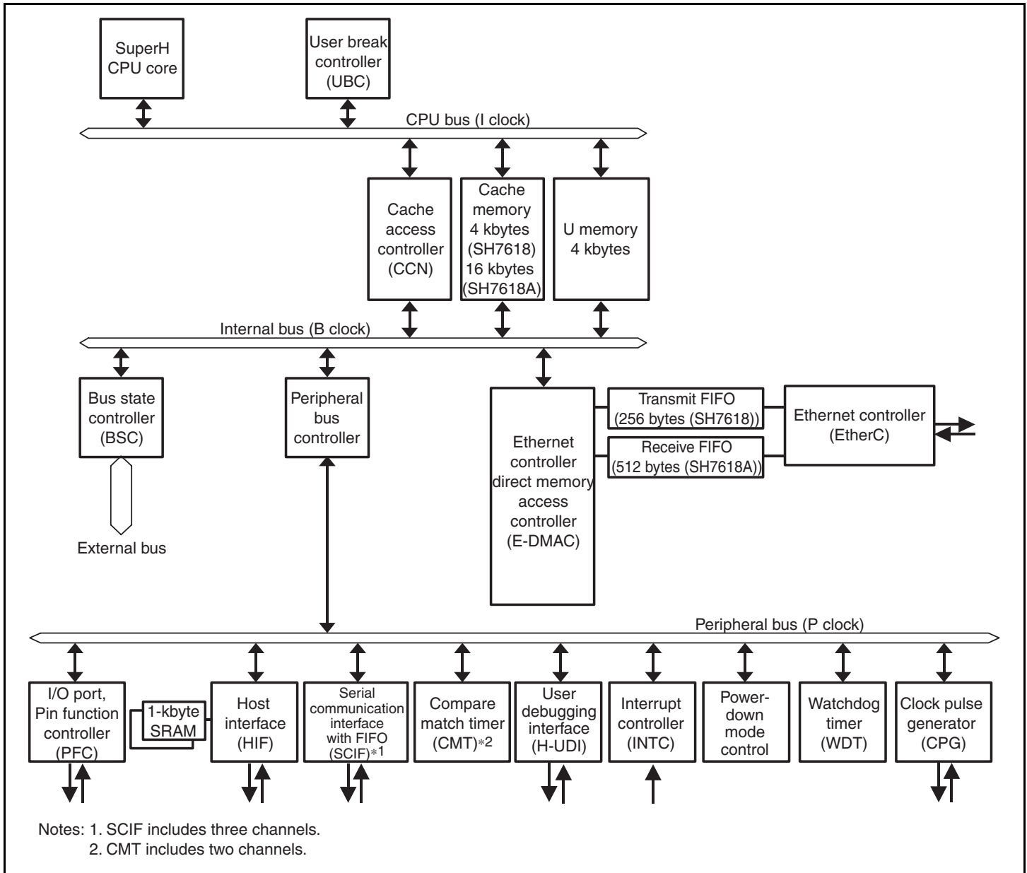
Figure 1.1 Block Diagram
