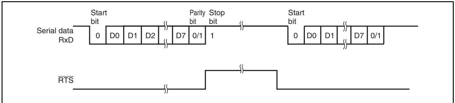
Figure 14.10 Example of Operation Using Modem Control ( \overline{\text{RTS}} )
