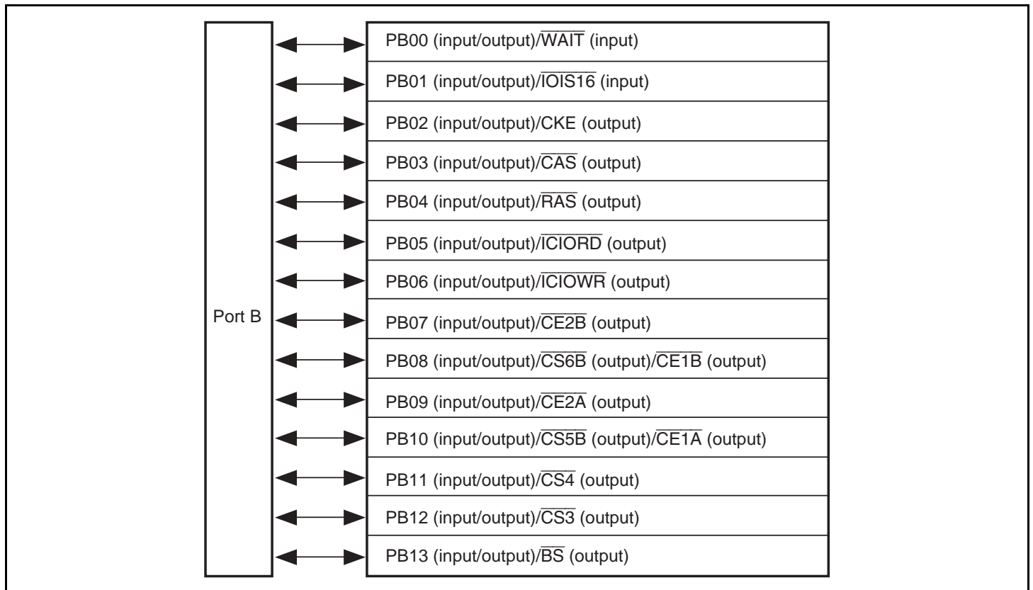
Figure 17.2 Port B
