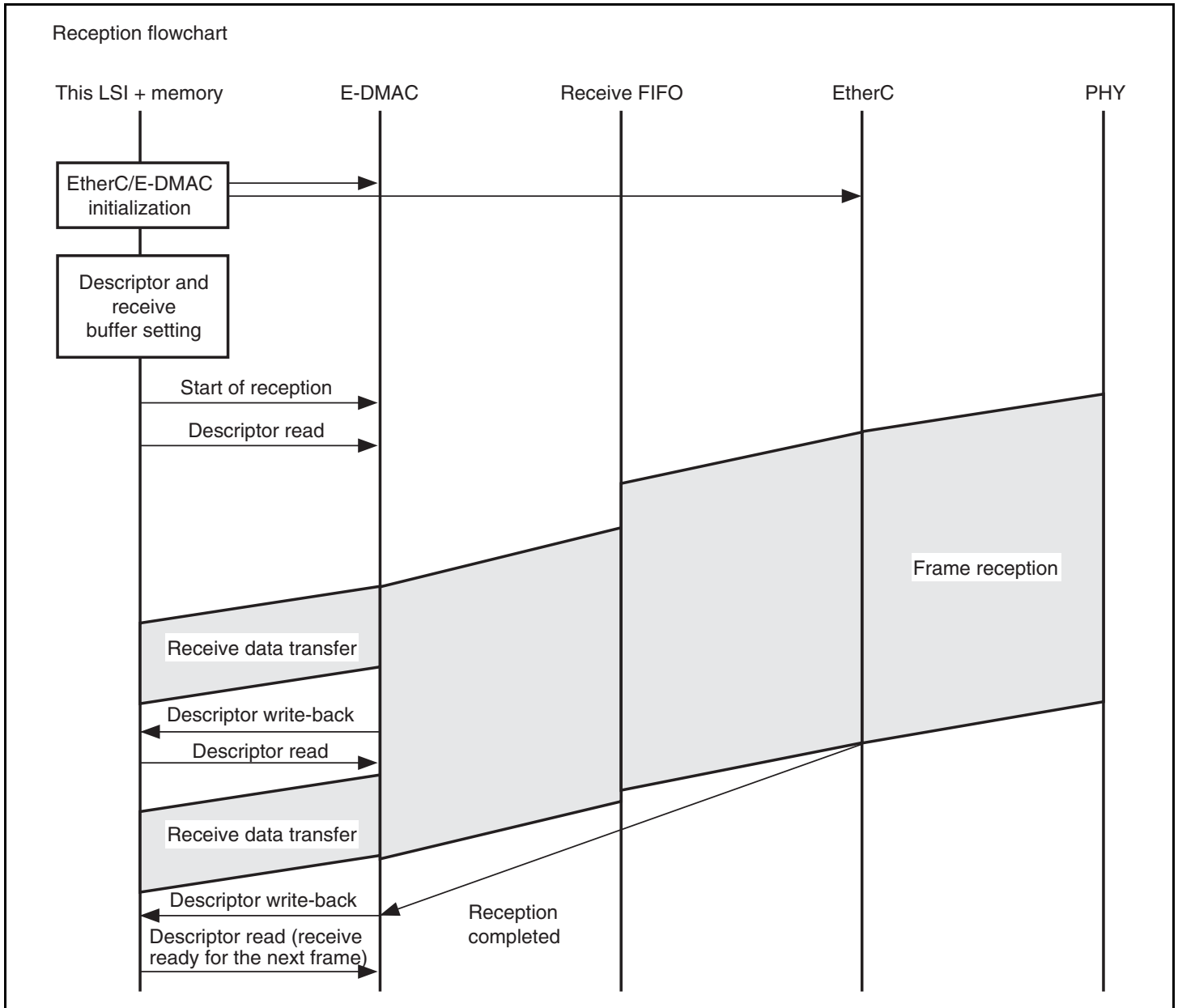
Figure 12.5 Sample Reception Flowchart
