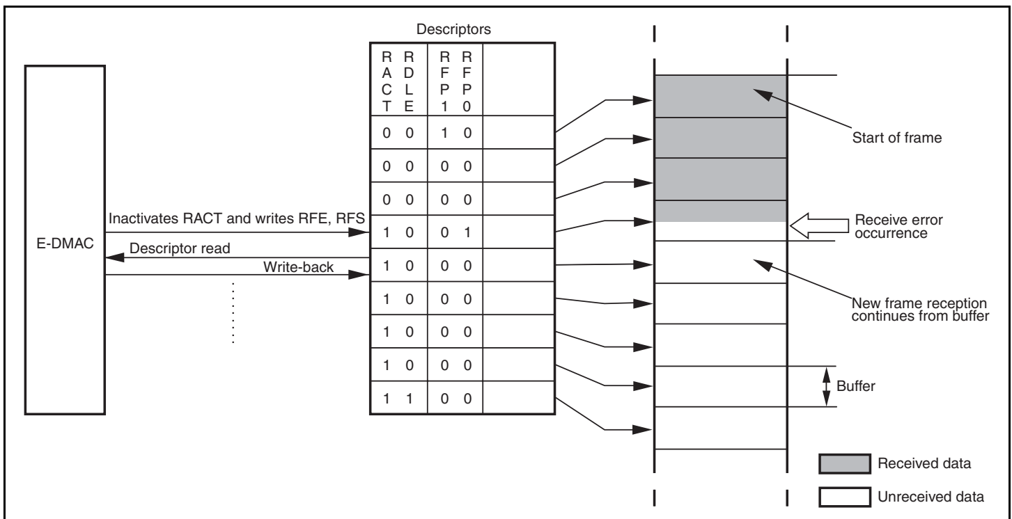
Figure 12.7 E-DMAC Operation after Receive Error
