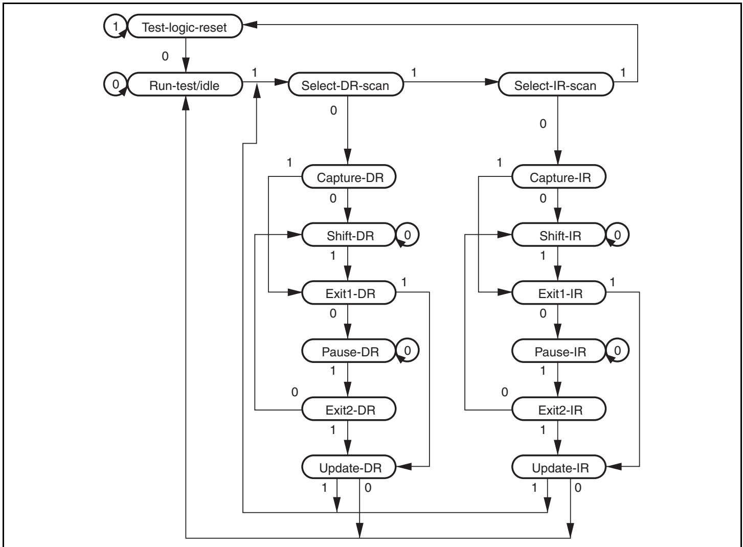
Figure 19.2 TAP Controller State Transitions
