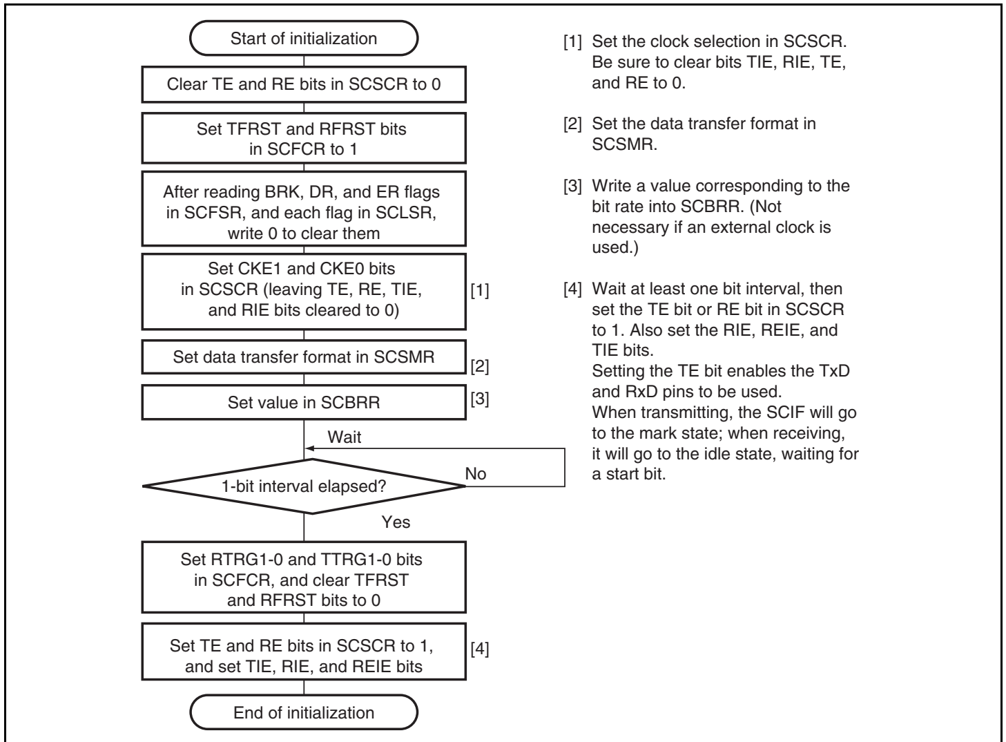
Figure 14.3 Sample Flowchart for SCIF Initialization
