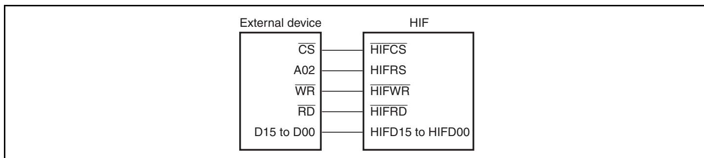
Figure 15.2 HIF Connection Example
