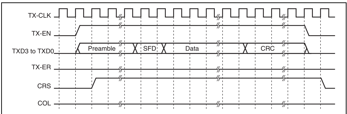
Figure 11.4 (1) MII Frame Transmit Timing (Normal Transmission)
