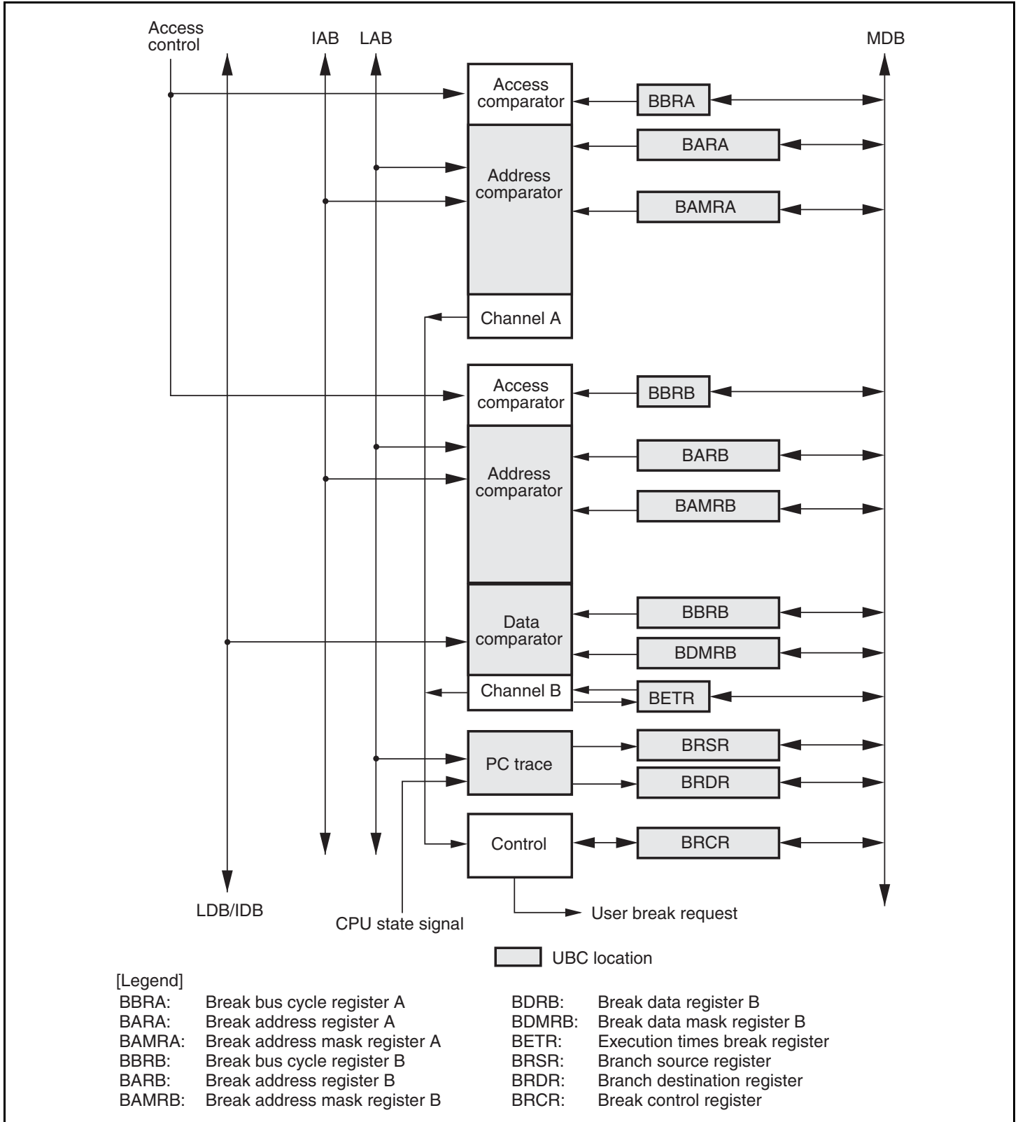
Figure 18.1 Block Diagram of UBC
