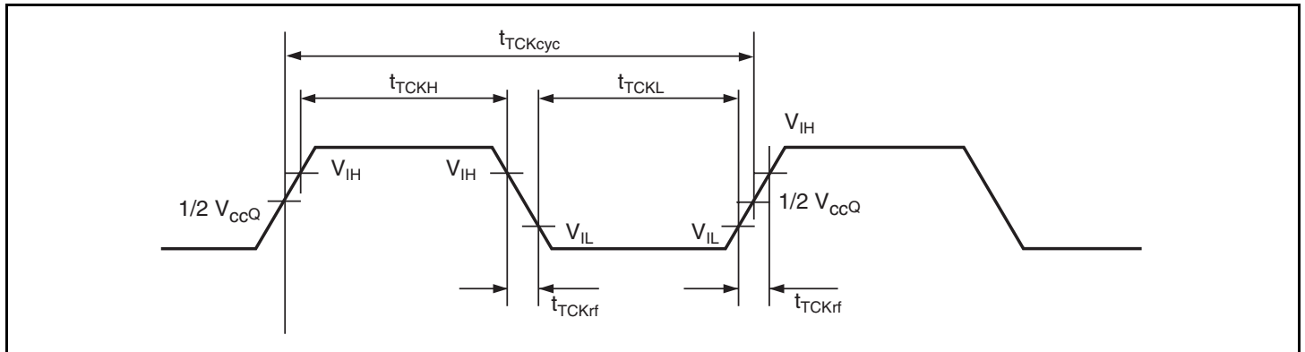
Figure 21.51 TCK Input Timing
