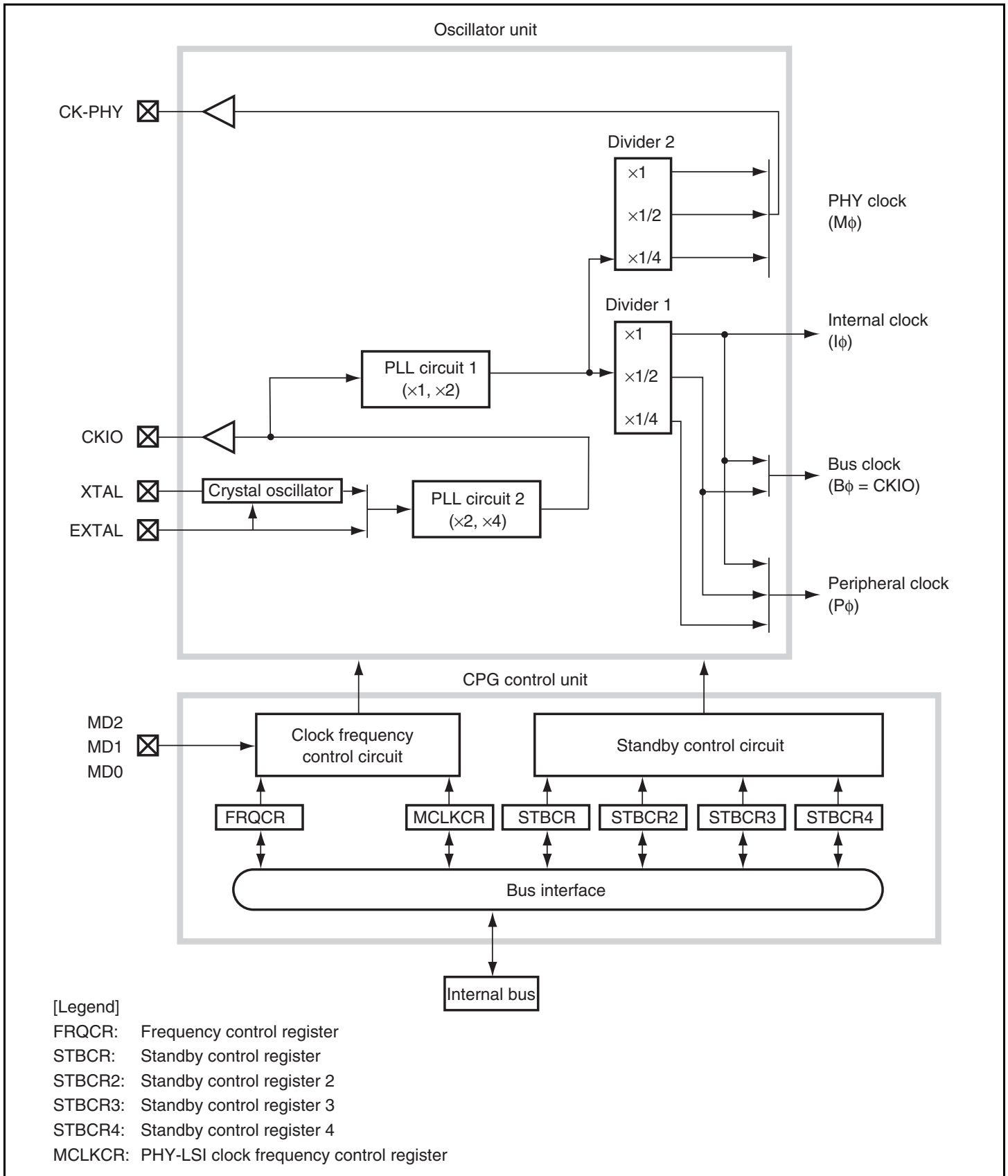
Figure 8.1 Block Diagram of CPG
