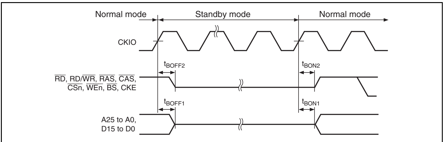
Figure 21.9 Pin Drive Timing in Standby Mode
