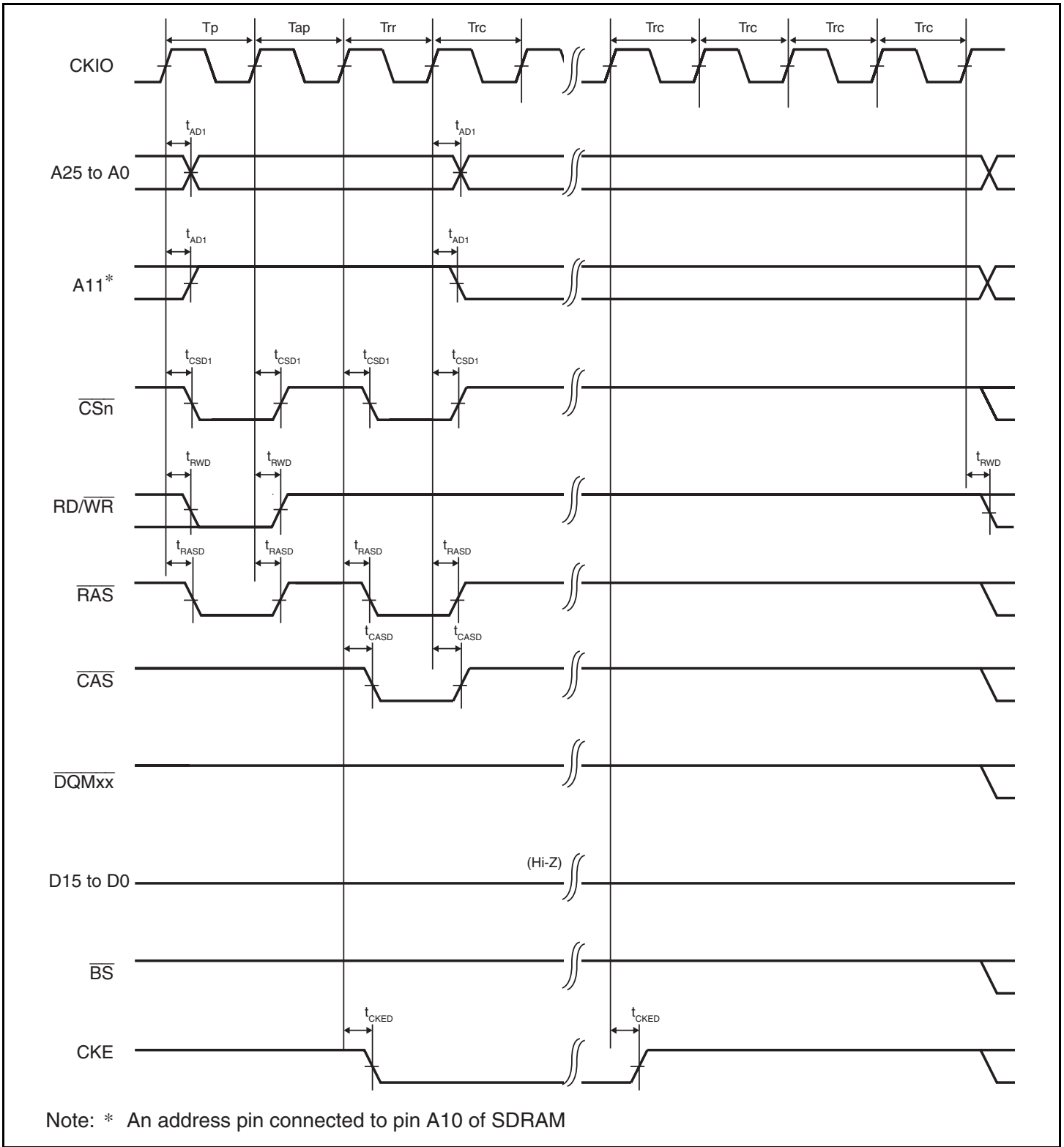
Figure 21.31 Synchronous DRAM Self-Refreshing Timing (WTRP = 1 Cycle)
