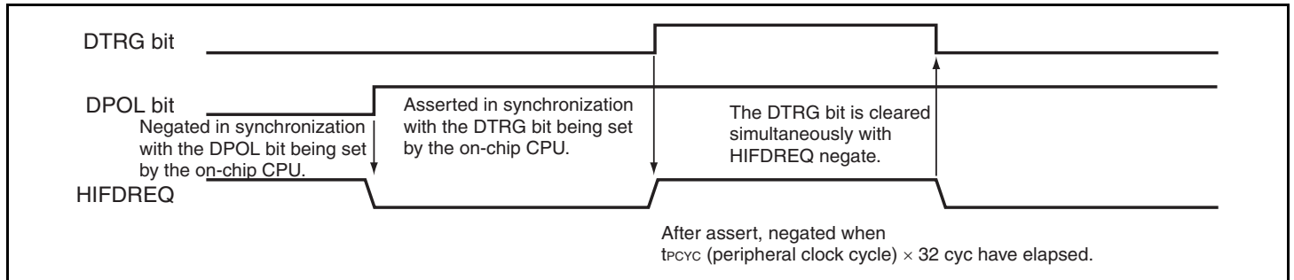
Figure 15.11 HIFDREQ Timing (When DMD = 1 and DPOL = 1 )
