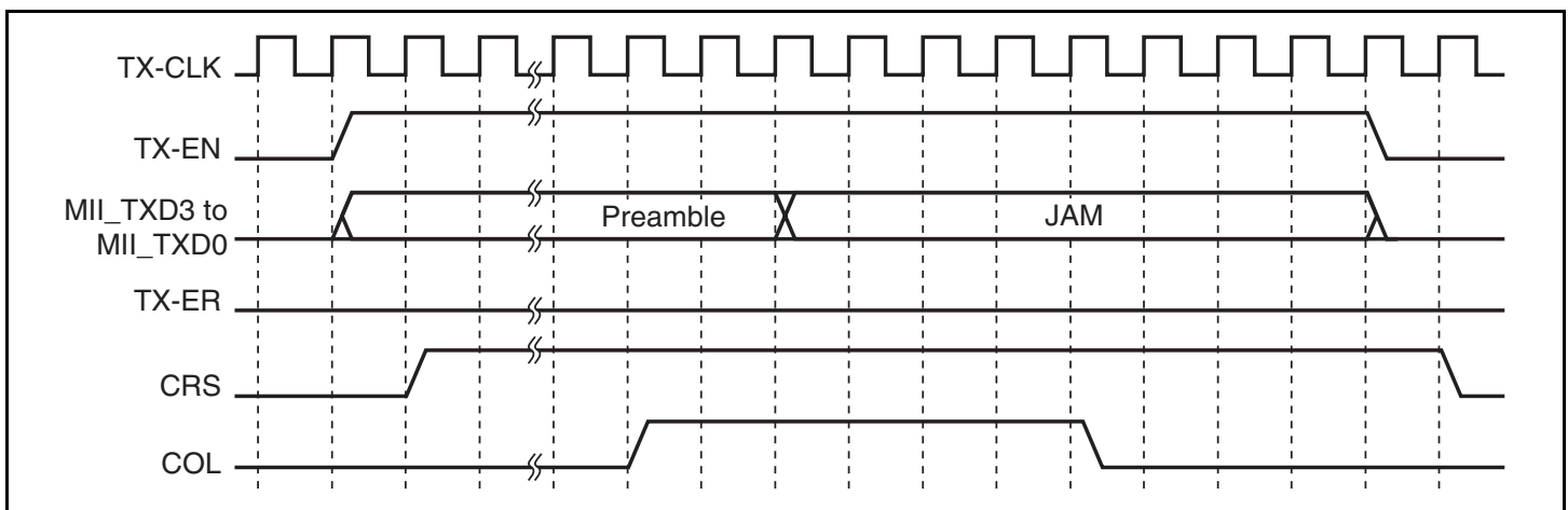
Figure 11.4 (2) MII Frame Transmit Timing (Collision)
