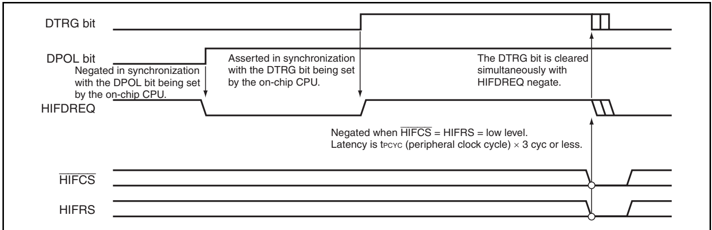
Figure 15.9 HIFDREQ Timing (When DMD = 0 and DPOL = 1 )
