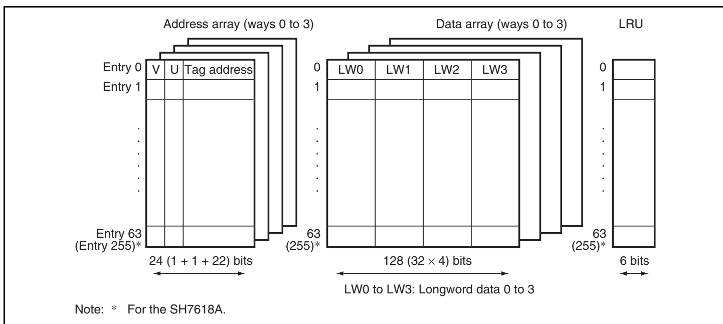
Figure 3.1 Cache Structure
