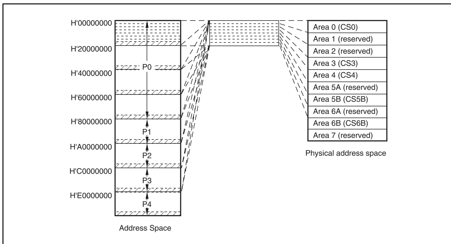
Figure 7.2 Address Space
