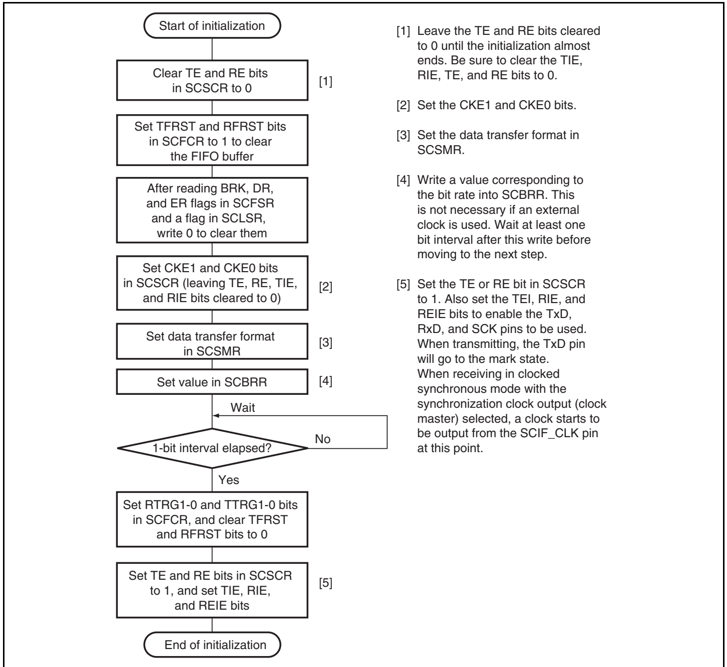
Figure 14.12 Sample Flowchart for SCIF Initialization
