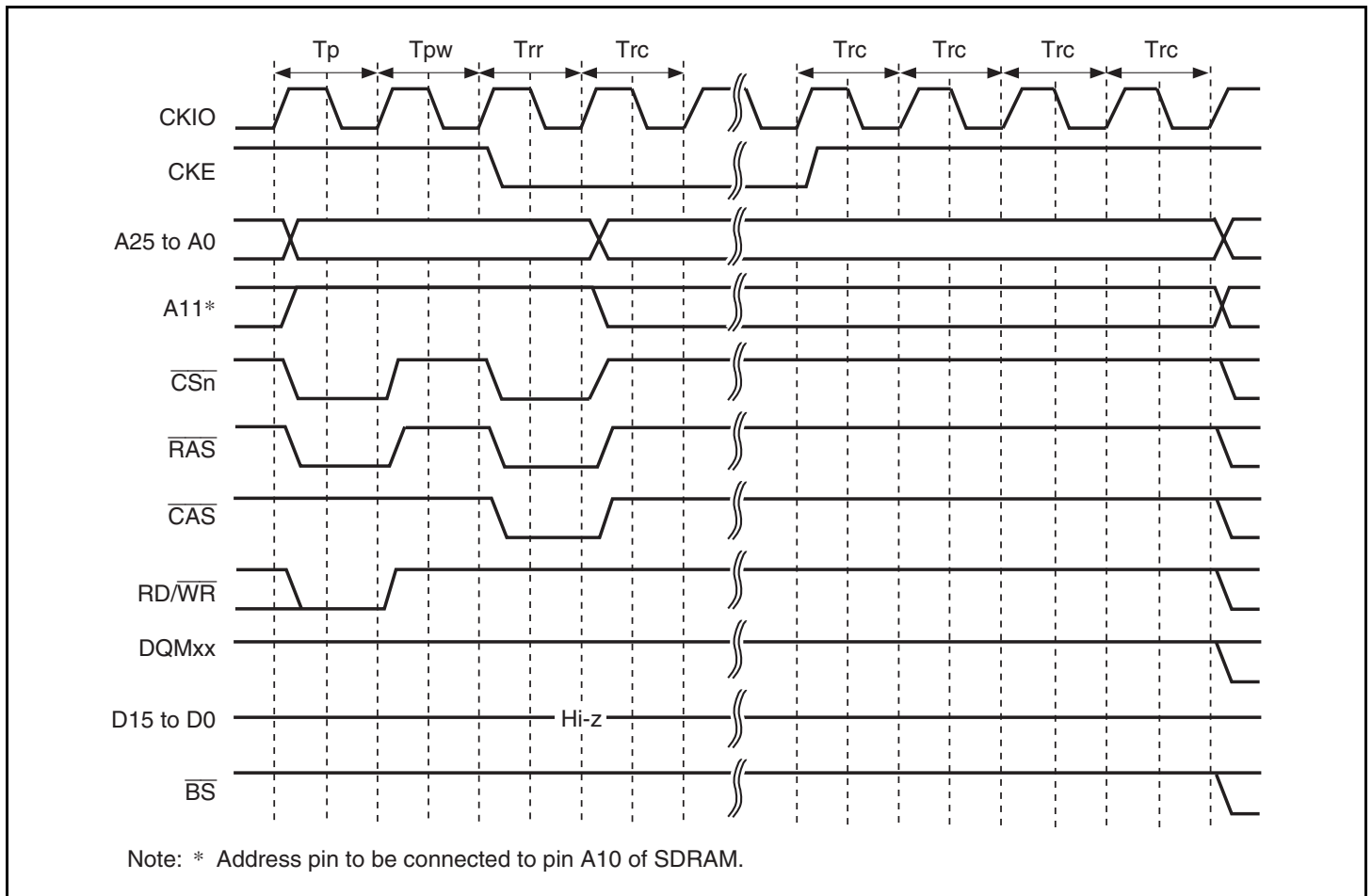
Figure 7.24 Self-Refreshing Timing
