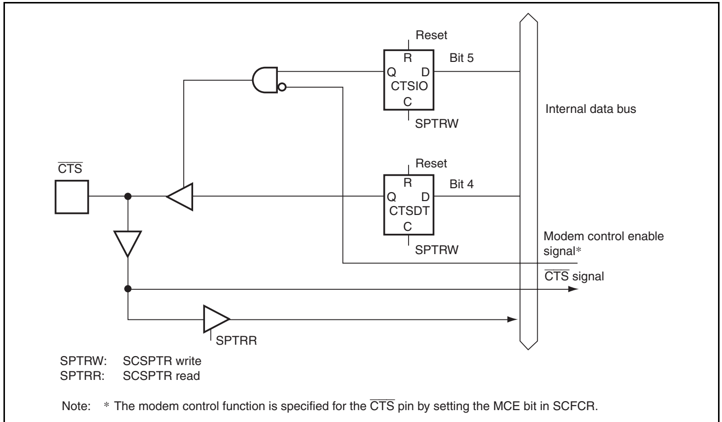
Figure 14.20 CTSIO Bit, CTSDT bit, and \overline{\text{CTS}} Pin
