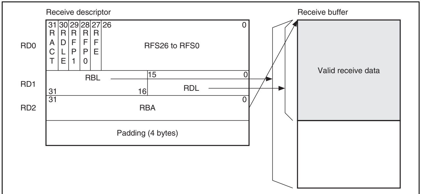
Figure 12.3 Relationship between Receive Descriptor and Receive Buffer
