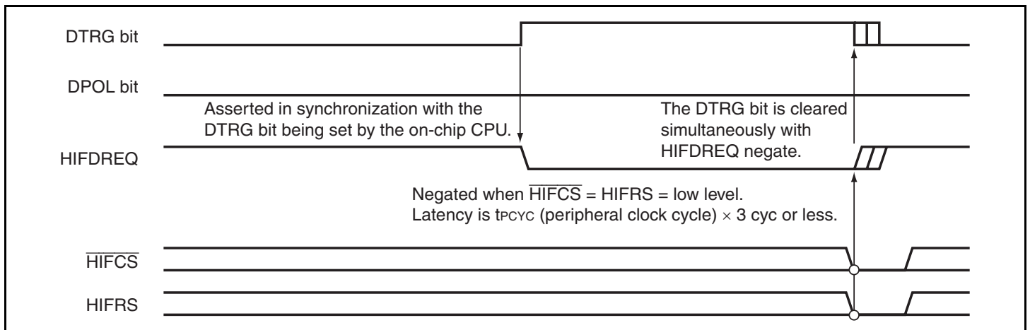
Figure 15.8 HIFDREQ Timing (When DMD = 0 and DPOL = 0 )
