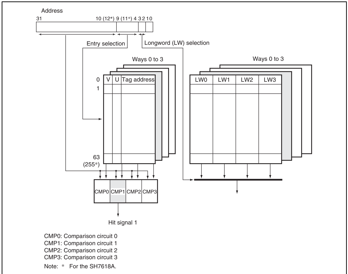
Figure 3.2 Cache Search Scheme
