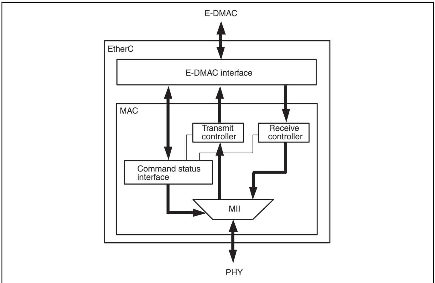
Figure 11.1 Configuration of EtherC
