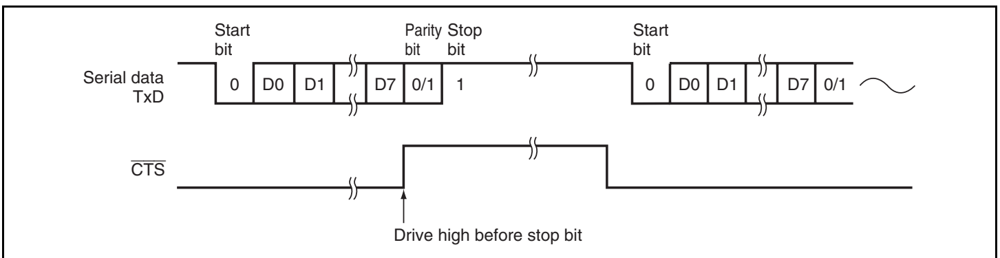
Figure 14.6 Example of Operation Using Modem Control ( \overline{\text{CTS}} )
