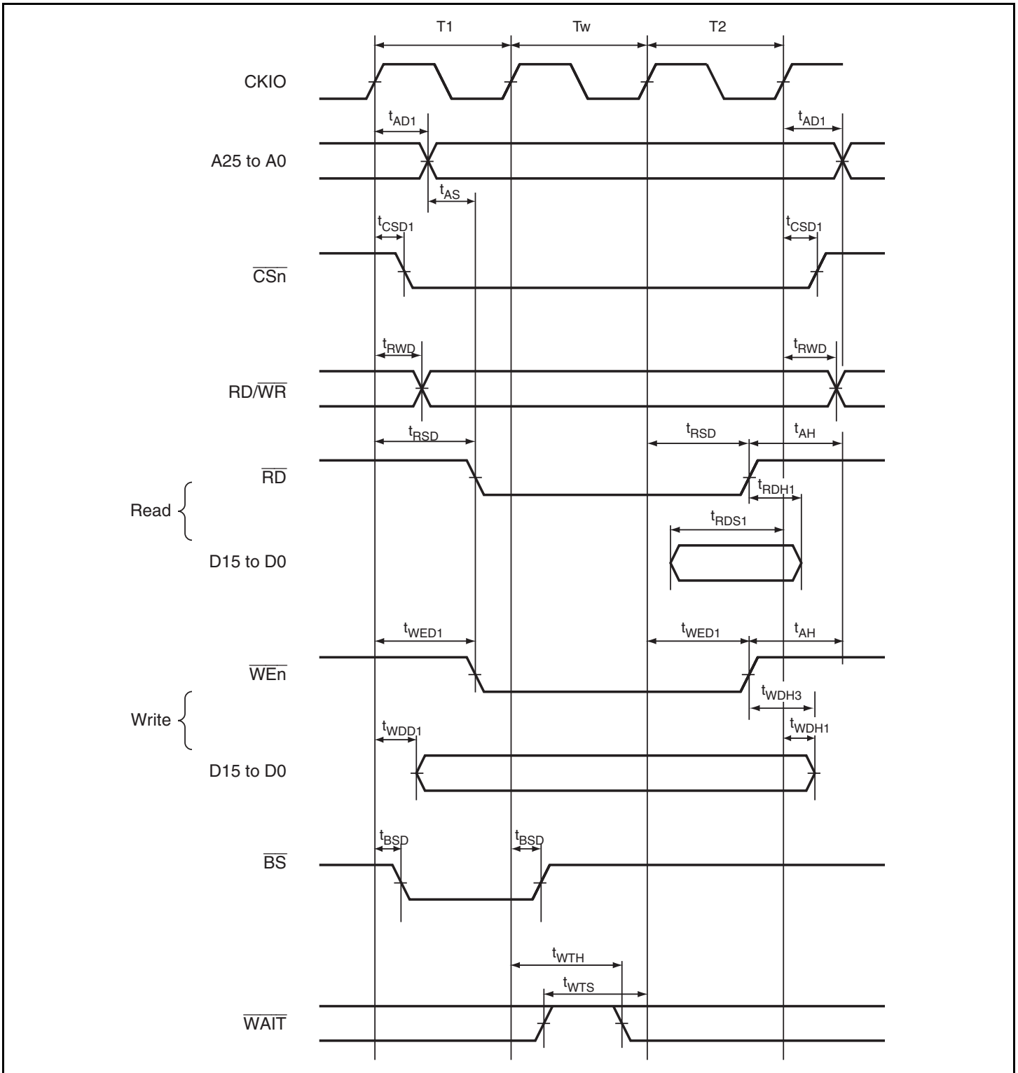
Figure 21.11 Basic Bus Timing: One Software Wait Cycle
