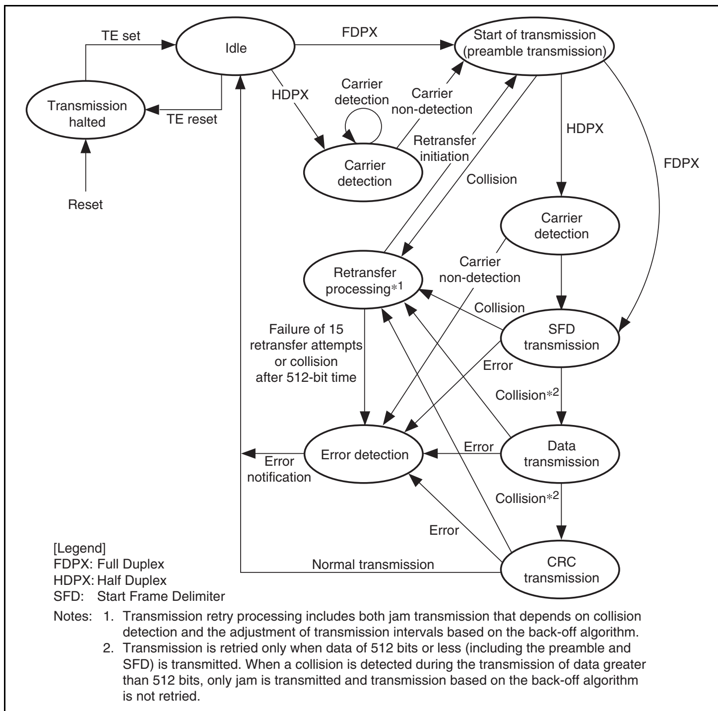
Figure 11.2 EtherC Transmitter State Transitions
