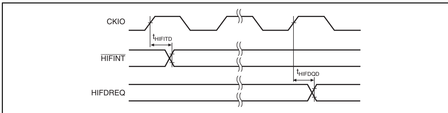
Figure 21.41 \overline{\text{HIFINT}} and HIFDREQ Timing
