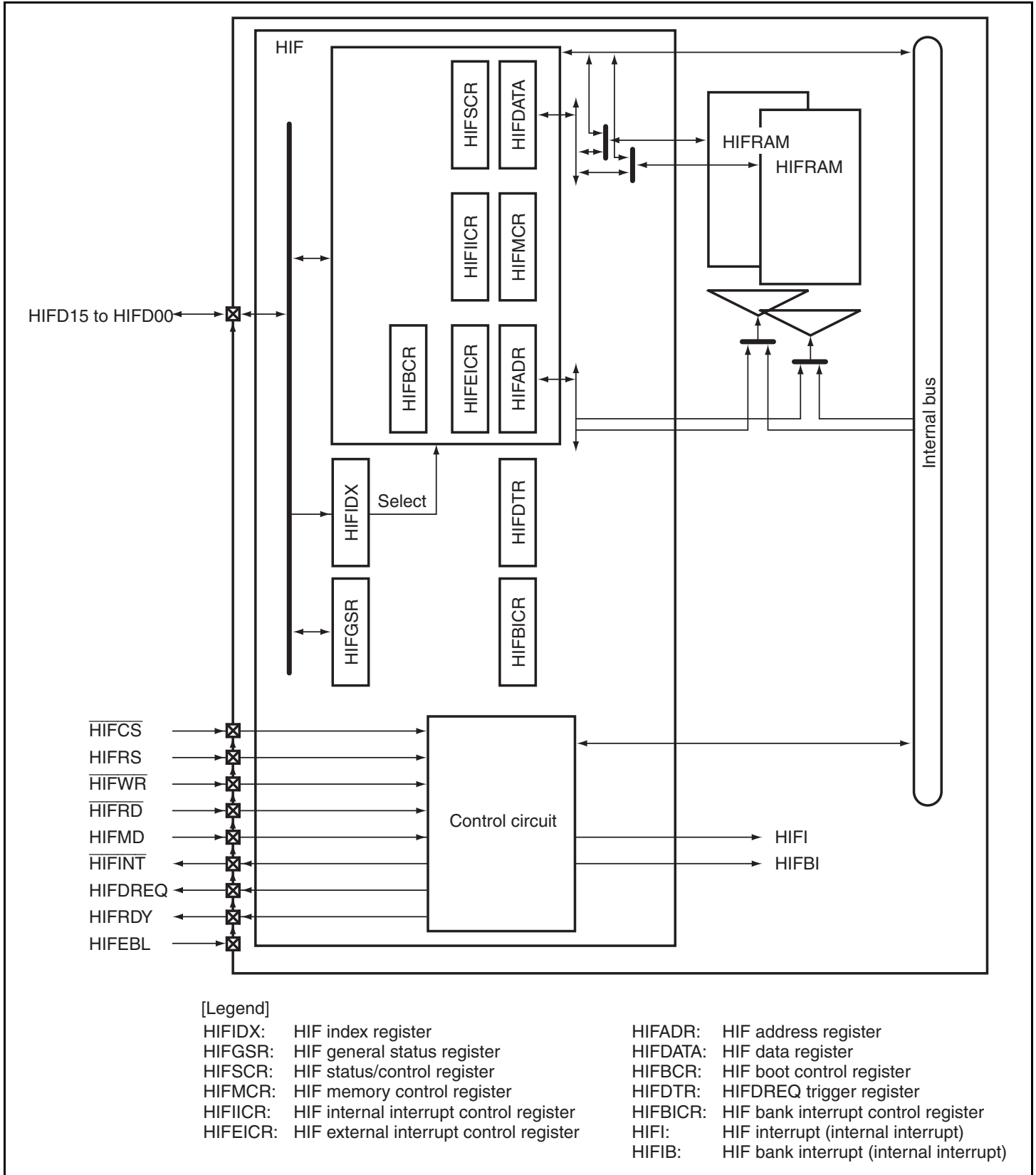
Figure 15.1 Block Diagram of HIF
