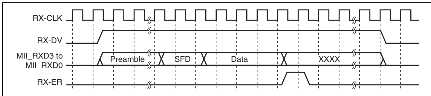
Figure 11.4 (5) MII Frame Receive Timing (Reception Error (1))
