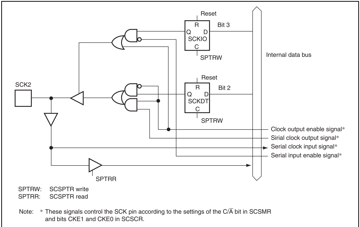
Figure 14.21 SCKIO Bit, SCKDT bit, and SCK Pin
