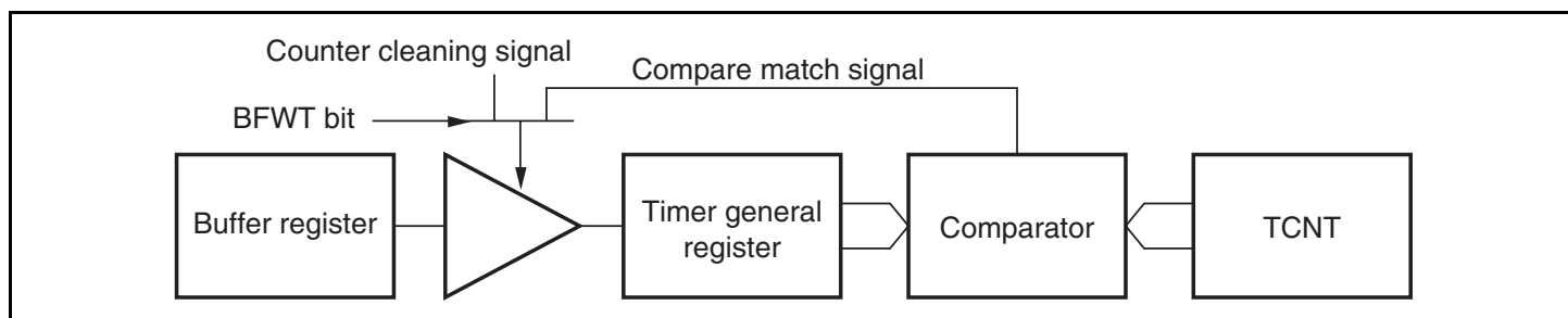
Figure 15.8 Compare Match Buffer Operation
