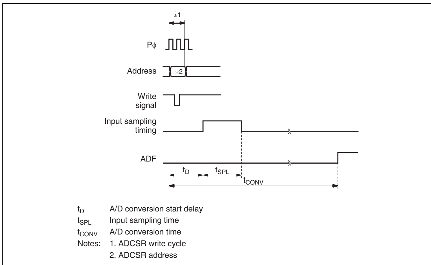
Figure 27.5 A/D Conversion Timing
