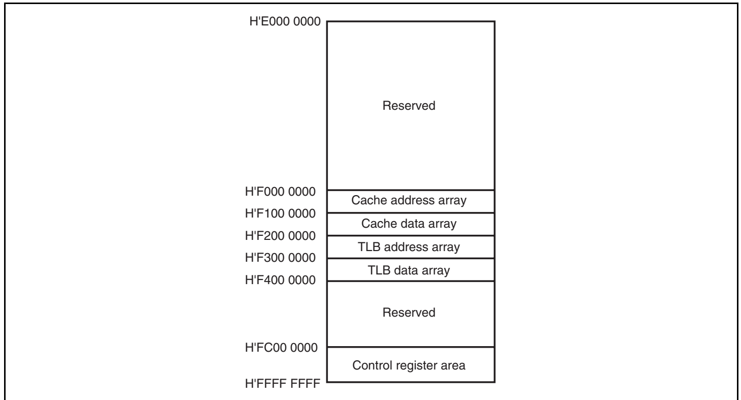
Figure 4.4 P4 Area
