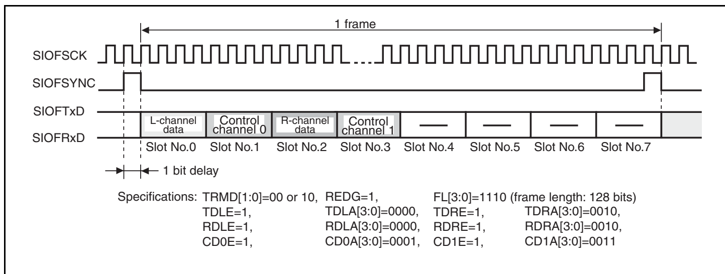
Figure 21.19 Transmit and Receive Timing (16-Bit Stereo Data (4))
