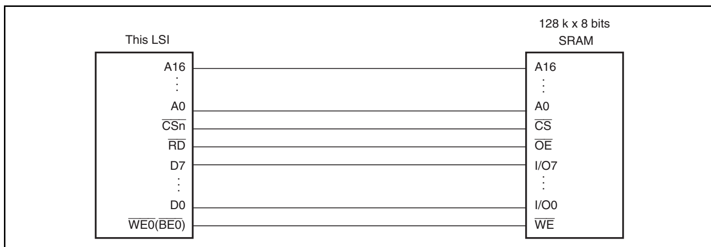
Figure 9.8 Example of 8-Bit Data-Width SRAM Connection
