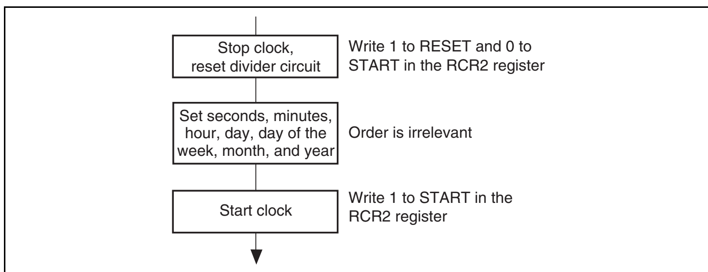
Figure 17.2 Setting Time
