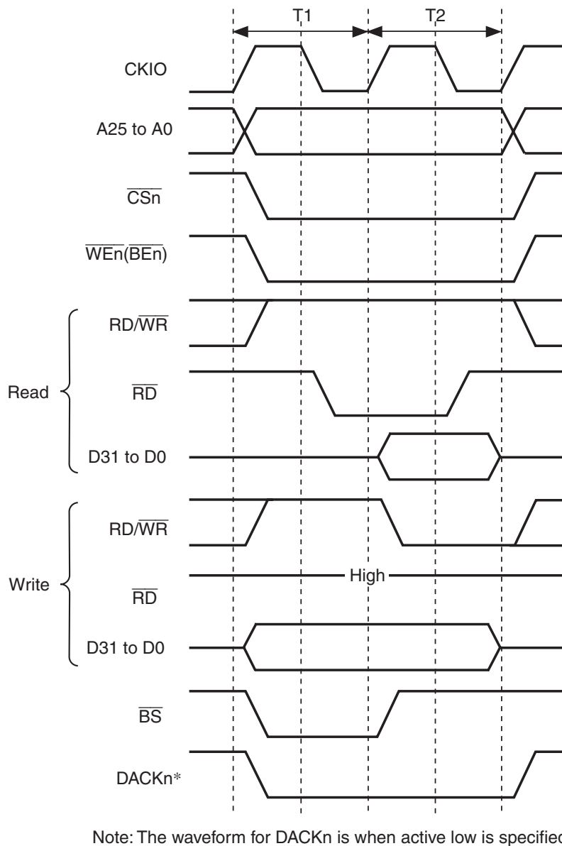
Figure 9.33 Basic Access Timing for Byte-Selection SRAM (BAS = 1)
