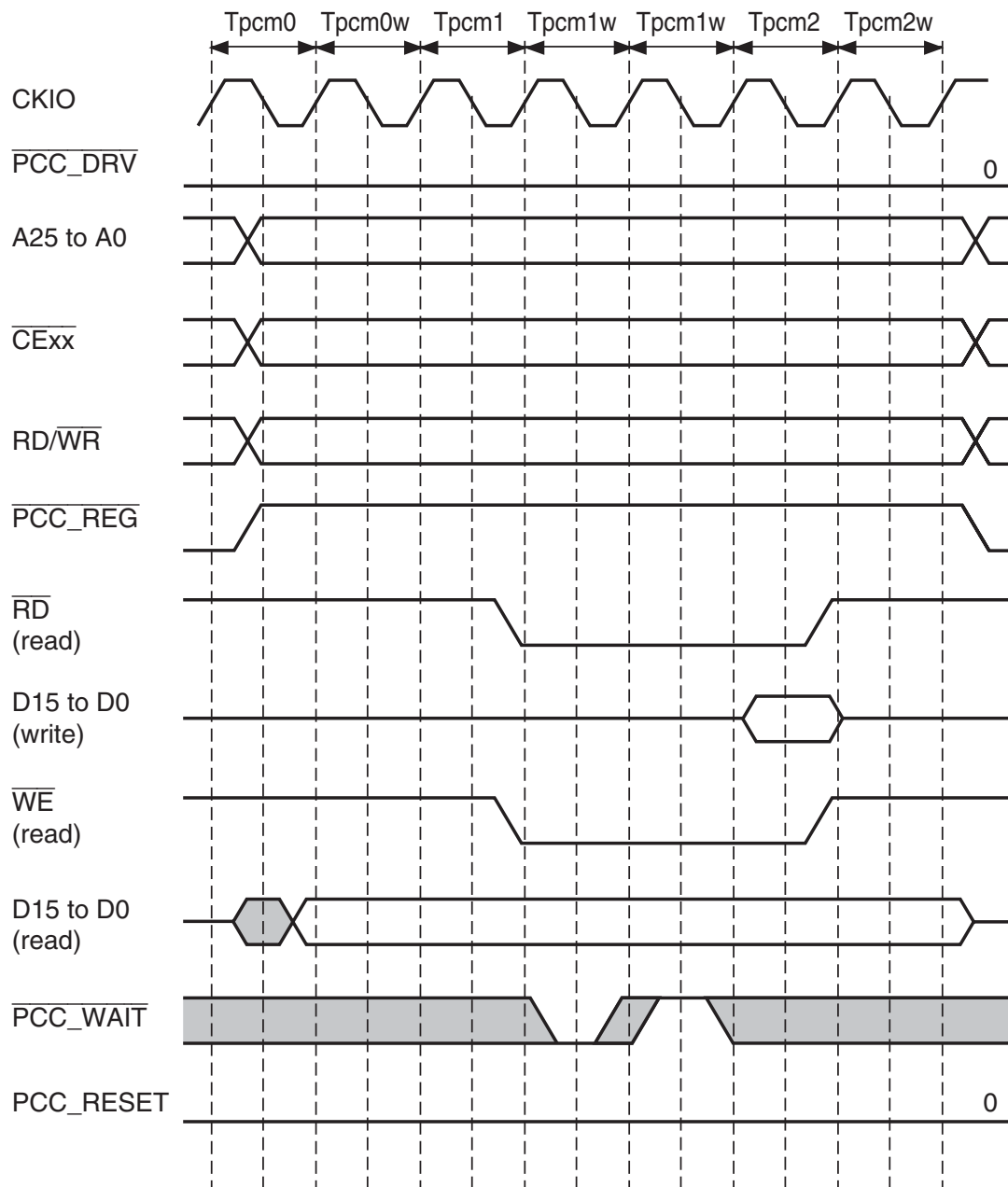
Figure 29.6 PCMCIA Memory Card Interface Wait Timing
