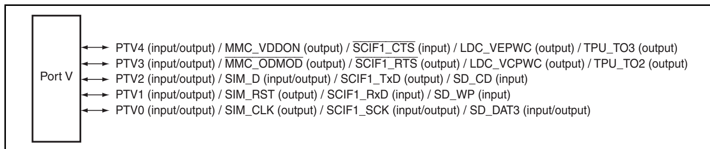
Figure 35.18 Port V
