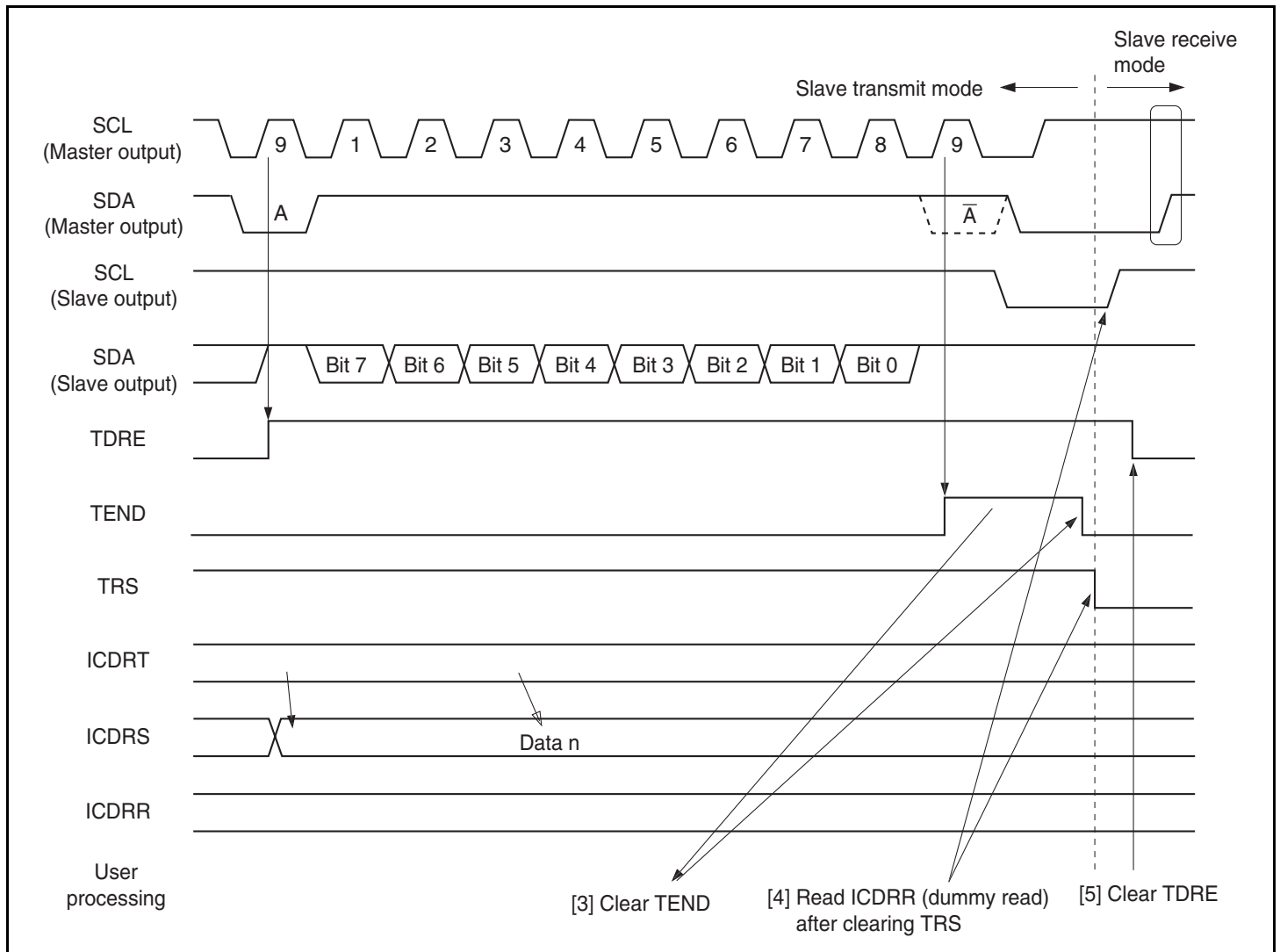
Figure 20.10 Slave Transmit Mode Operation Timing (2)
