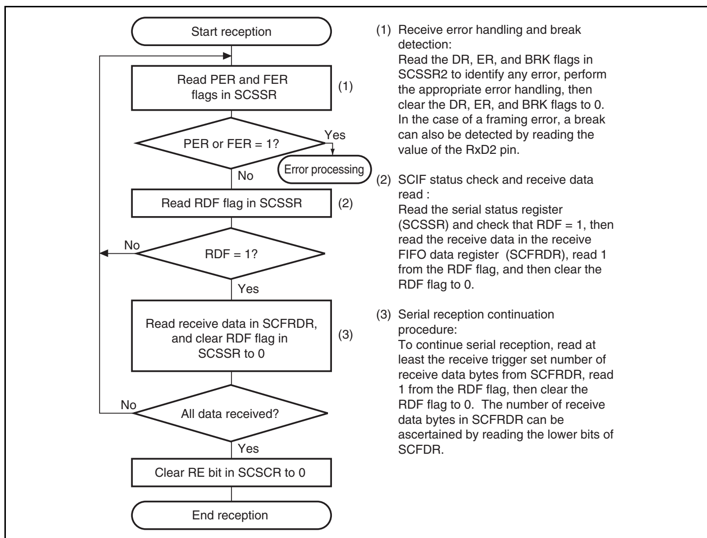
Figure 18.7 Sample Serial Reception Flowchart (1)
