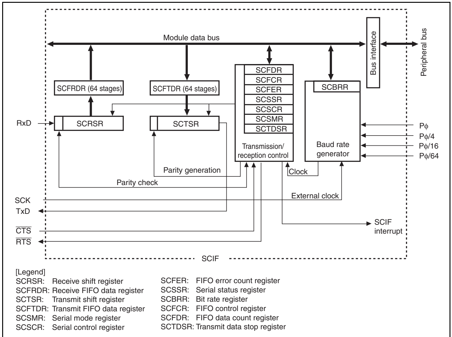
Figure 18.1 Block Diagram of SCIF
