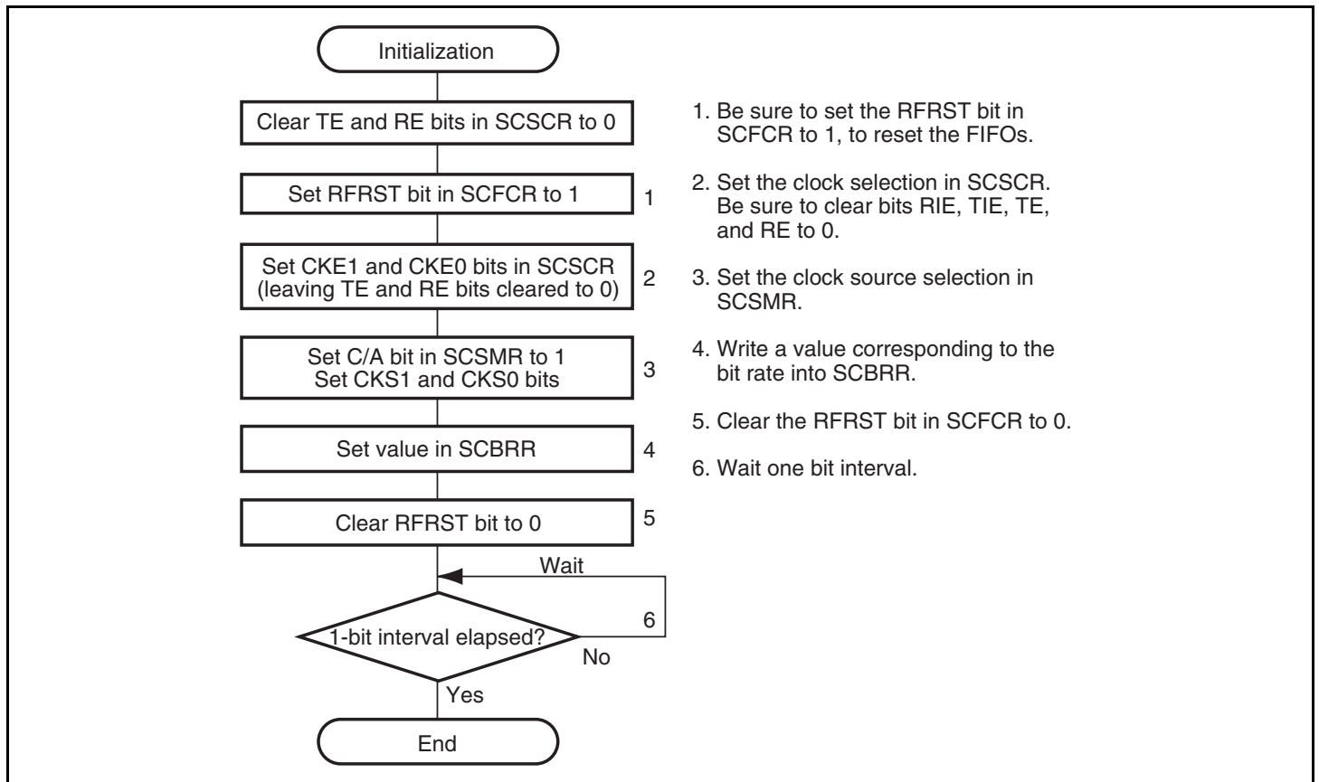
Figure 18.13 Sample SCIF Initialization Flowchart (2) (Reception)
