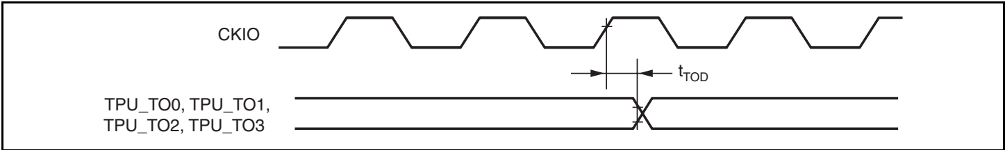
Figure 38.47 TPU Output Timing
