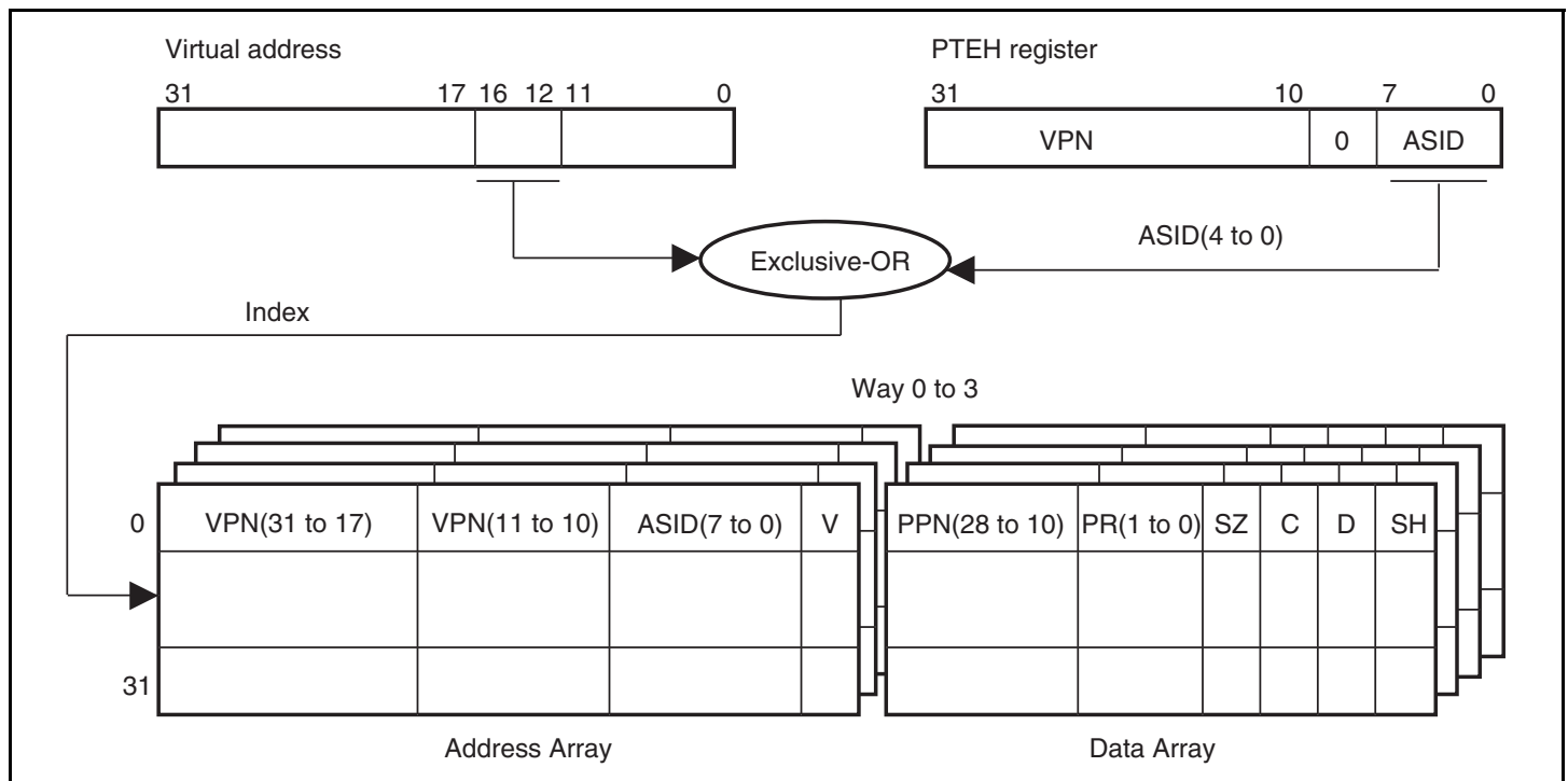
Figure 4.8 TLB Indexing (IX = 1)
