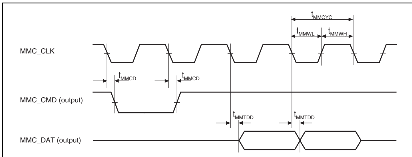
Figure 38.63 MMCIF Transmit Timing
