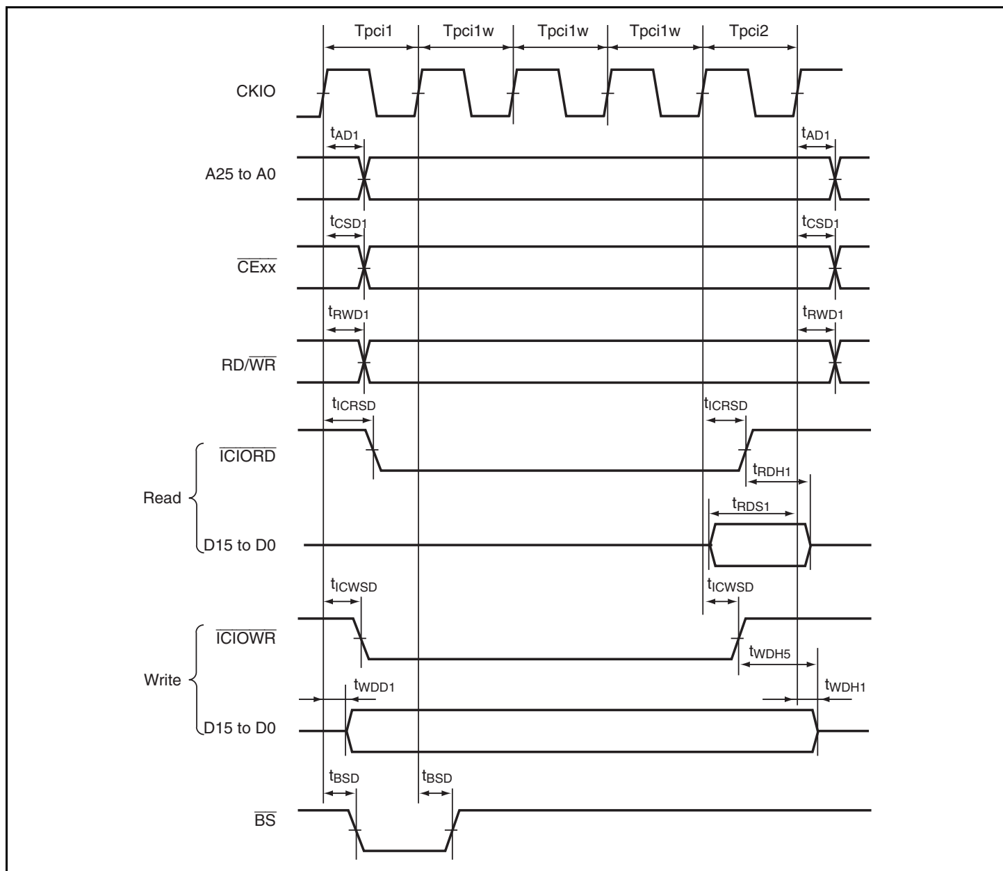
Figure 38.41 PCMCIA I/O Card Interface Bus Timing
