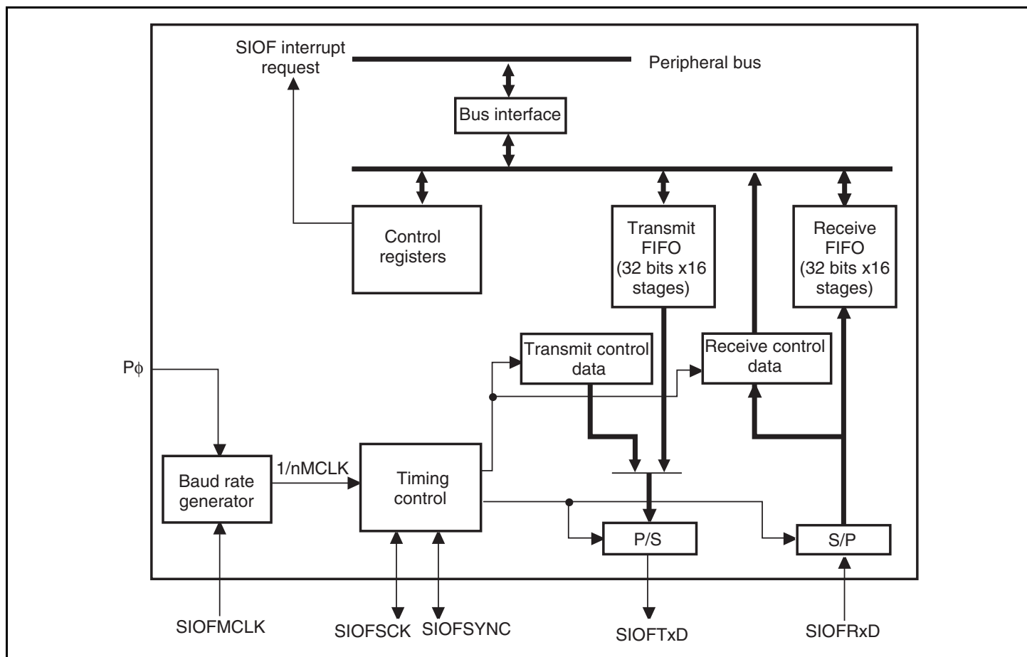
Figure 21.1 Block Diagram of SIOF
