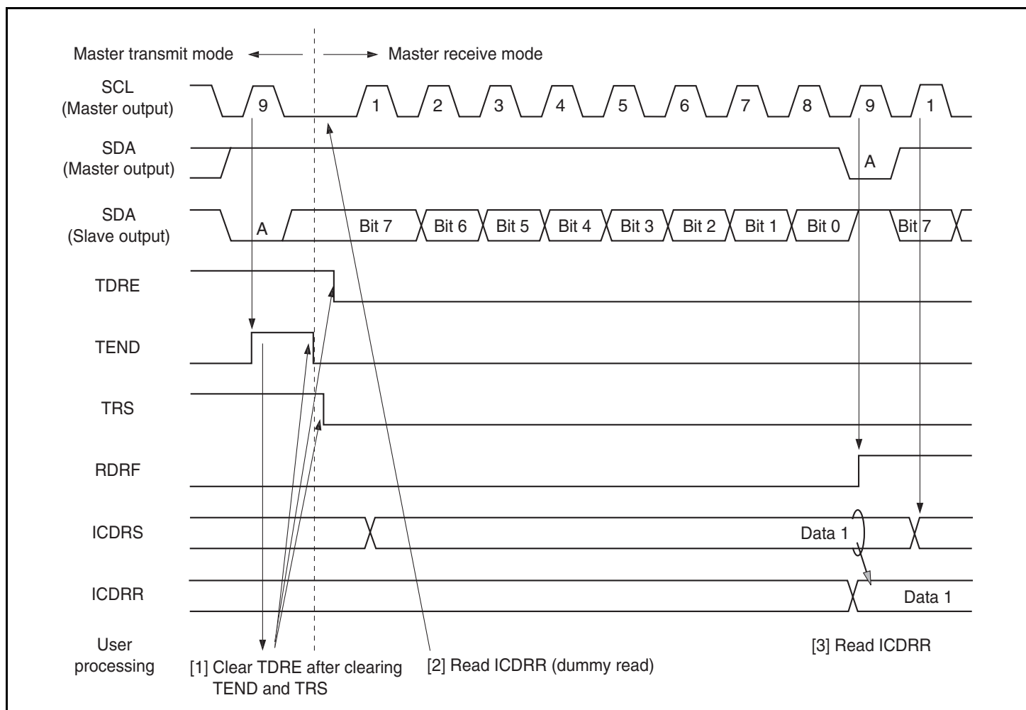
Figure 20.7 Master Receive Mode Operation Timing (1)
