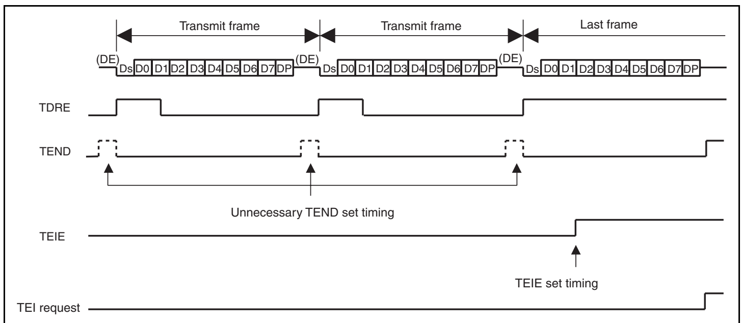
Figure 30.12 TEIE Set Timing
