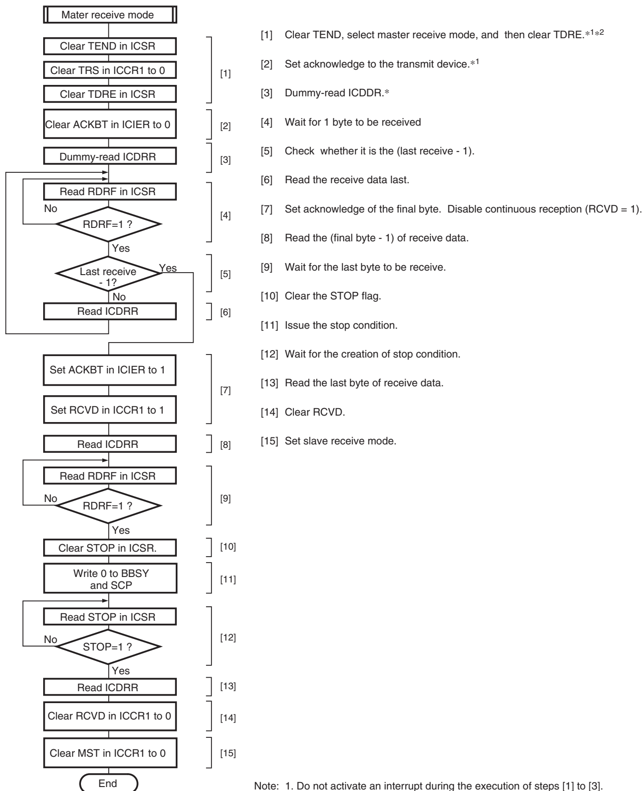
Figure 20.15 Sample Flowchart for Master Receive Mode
