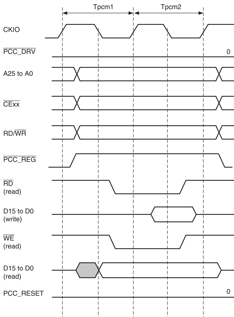
Figure 29.5 PCMCIA Memory Card Interface Basic Timing
