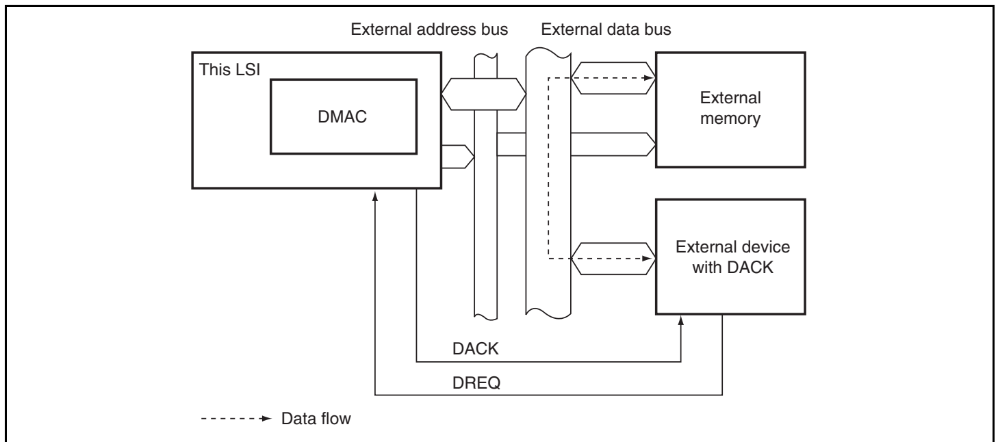
Figure 10.7 Data Flow in Single Address Mode
