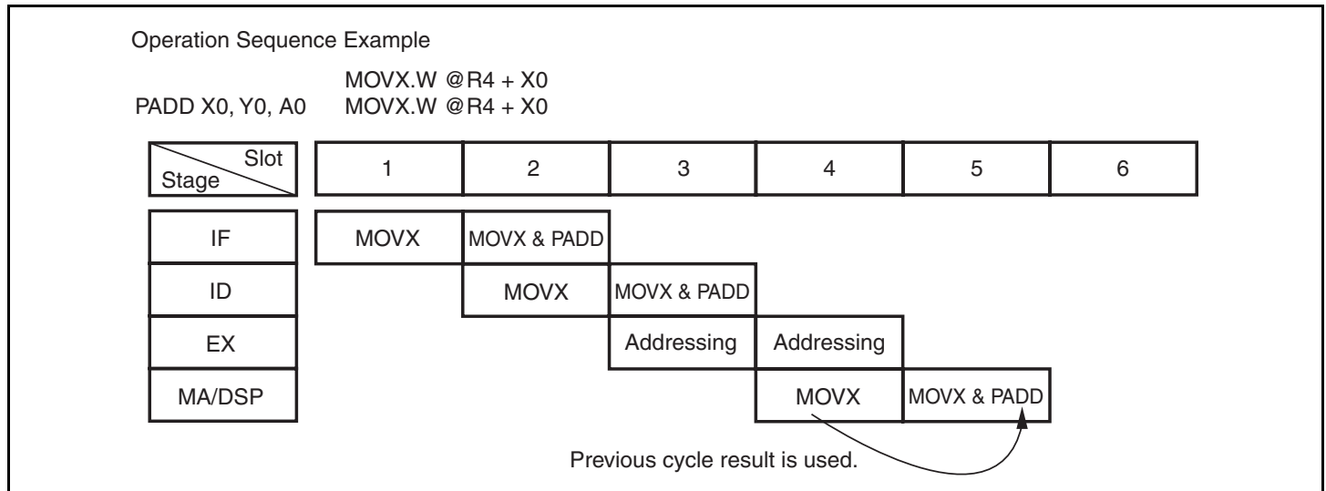
Figure 3.10 Operation Sequence Example
