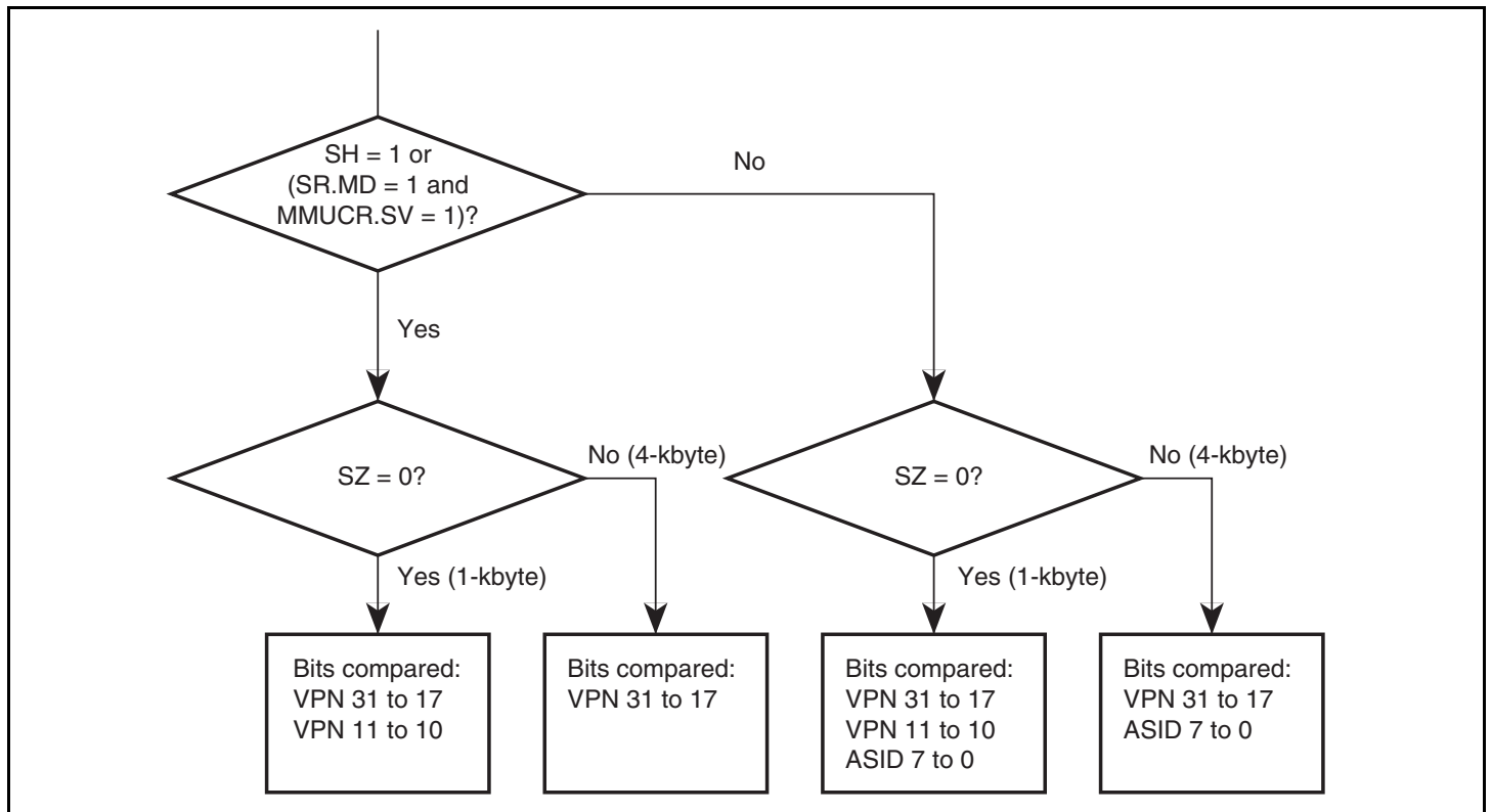
Figure 4.10 Objects of Address Comparison
