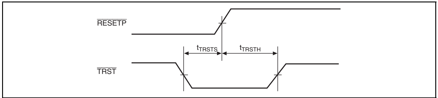
Figure 38.66 \overline{\text{TRST}} Input Timing (Reset Hold)
