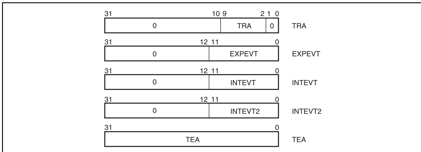
Figure 7.1 Register Bit Configuration
