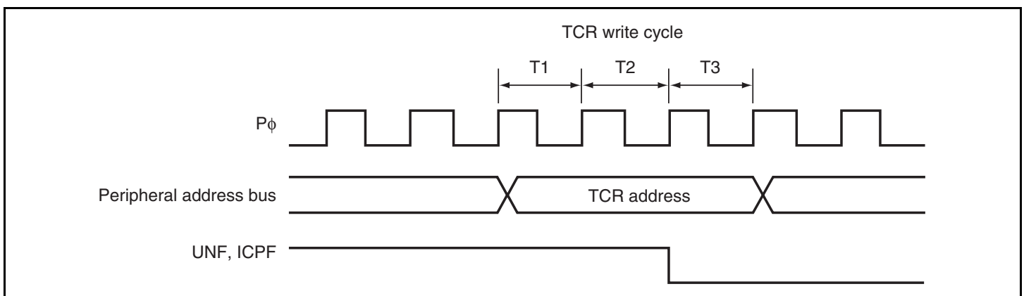
Figure 14.7 Status Flag Clear Timing
