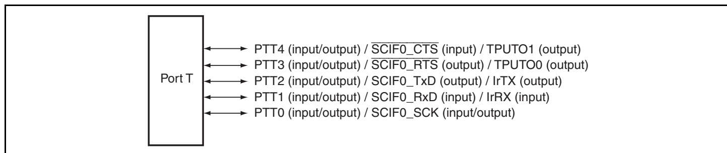
Figure 35.16 Port T
