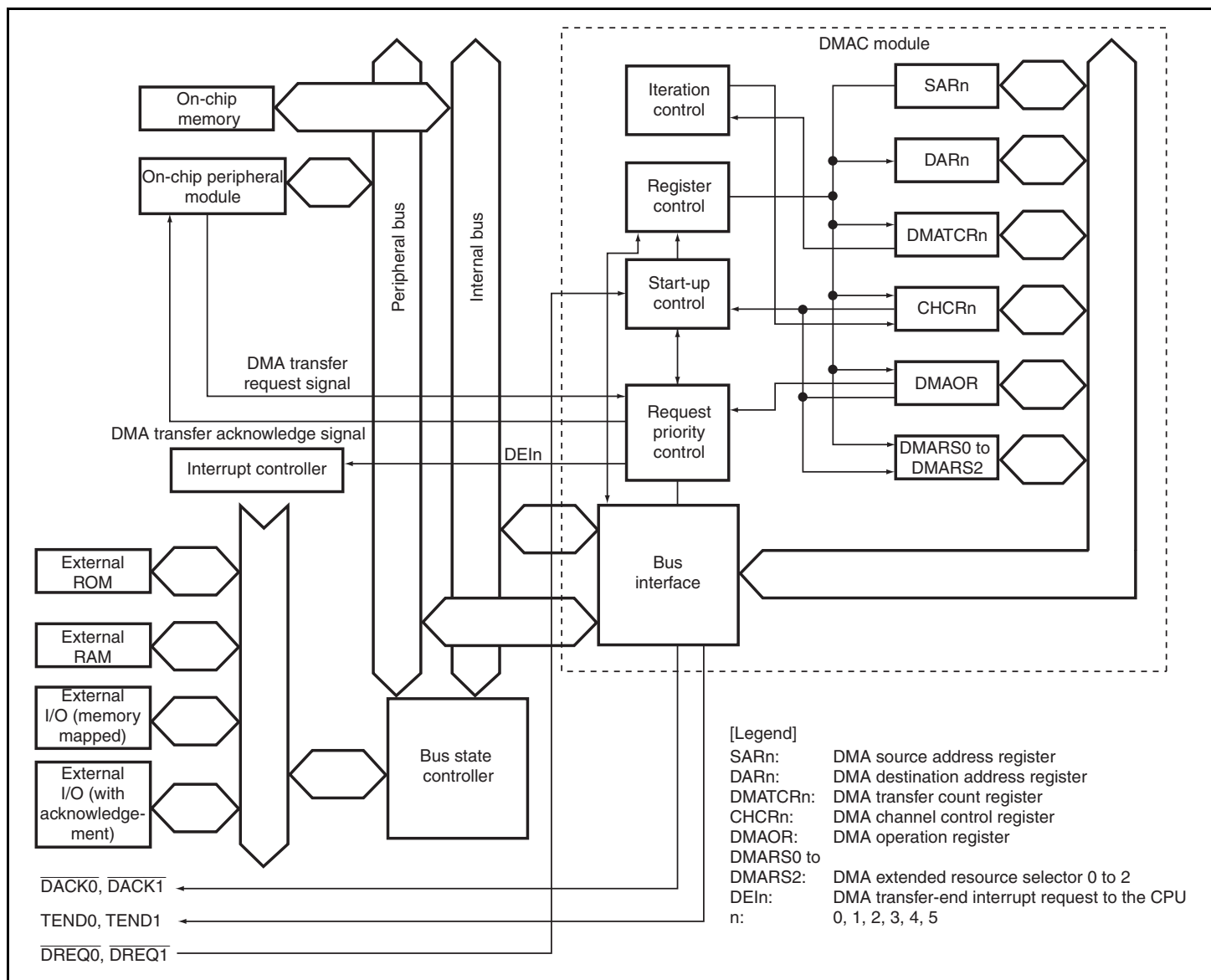
Figure 10.1 Block Diagram of DMAC
