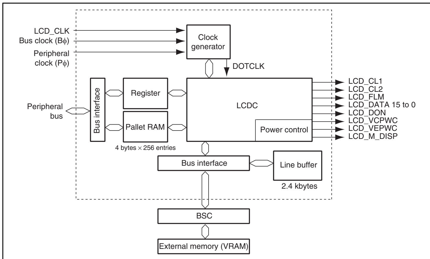
Figure 26.1 LCDC Block Diagram
