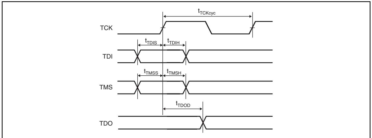
Figure 38.67 H-UDI Data Transfer Timing
