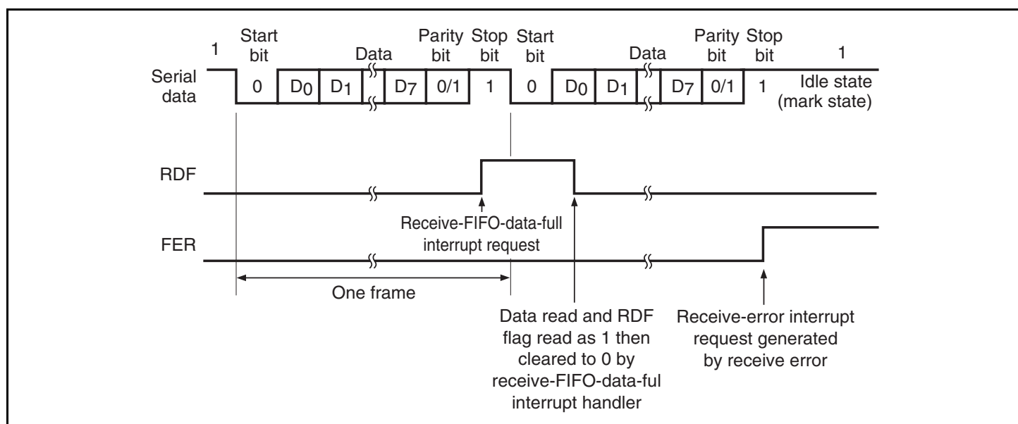
Figure 18.9 Example of SCIF Receive Operation (Example with 8-Bit Data, Parity, One Stop Bit)
