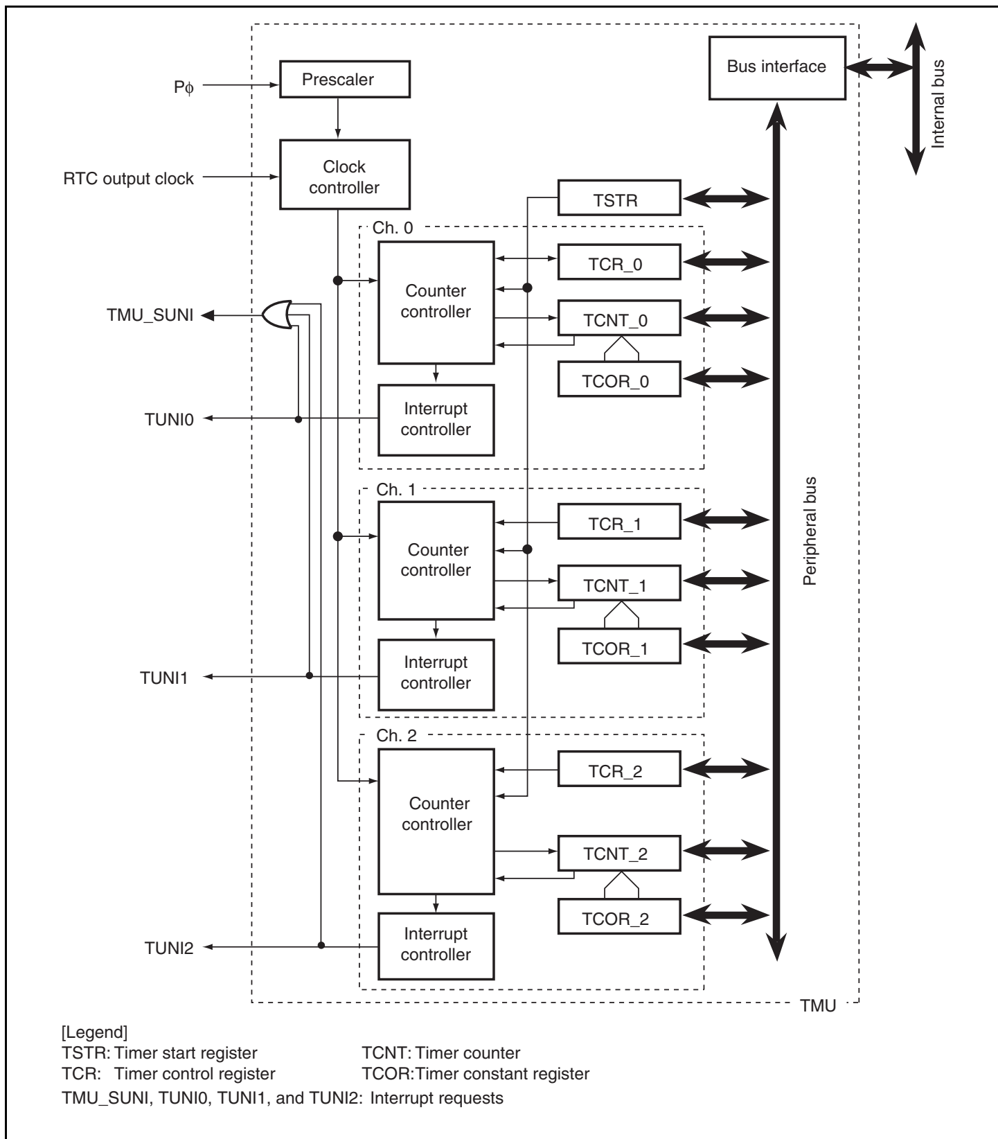
Figure 14.1 Block Diagram of TMU
