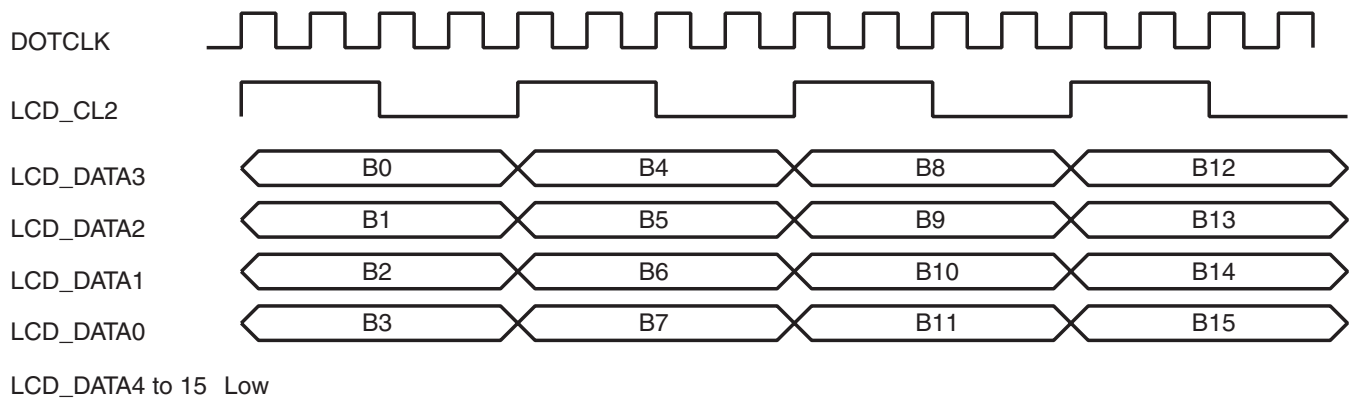
Figure 26.10 Clock and LCD Data Signal Example
