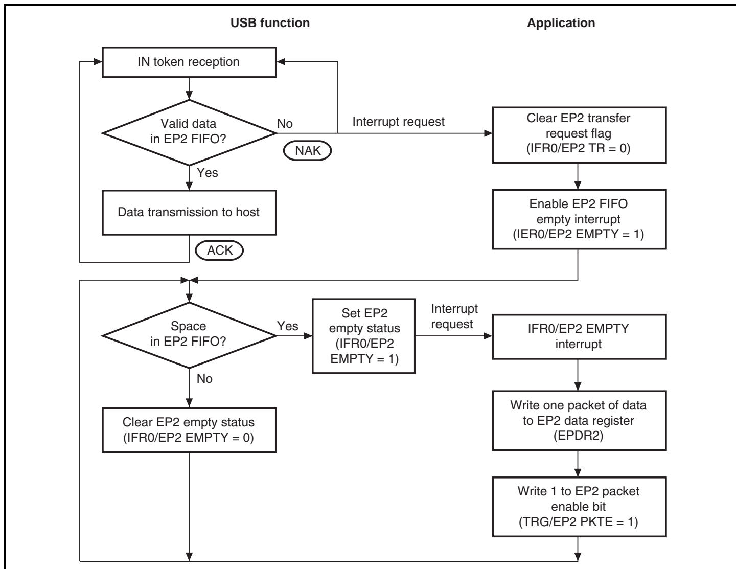
Figure 25.12 EP2 Bulk-In Transfer Operation
