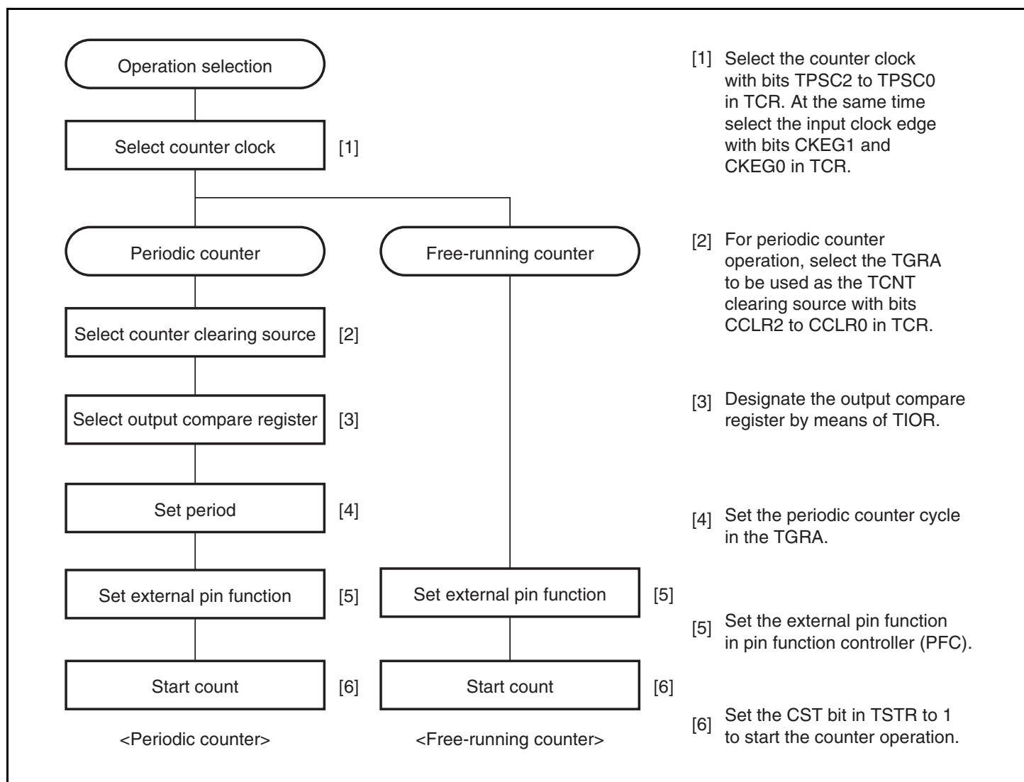
Figure 15.2 Example of Counter Operation Setting Procedure
