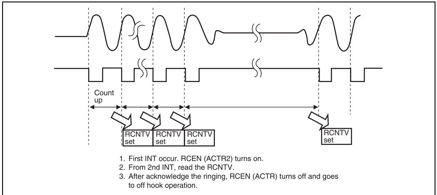
Figure 22.8 Ringing Detect Sequence
