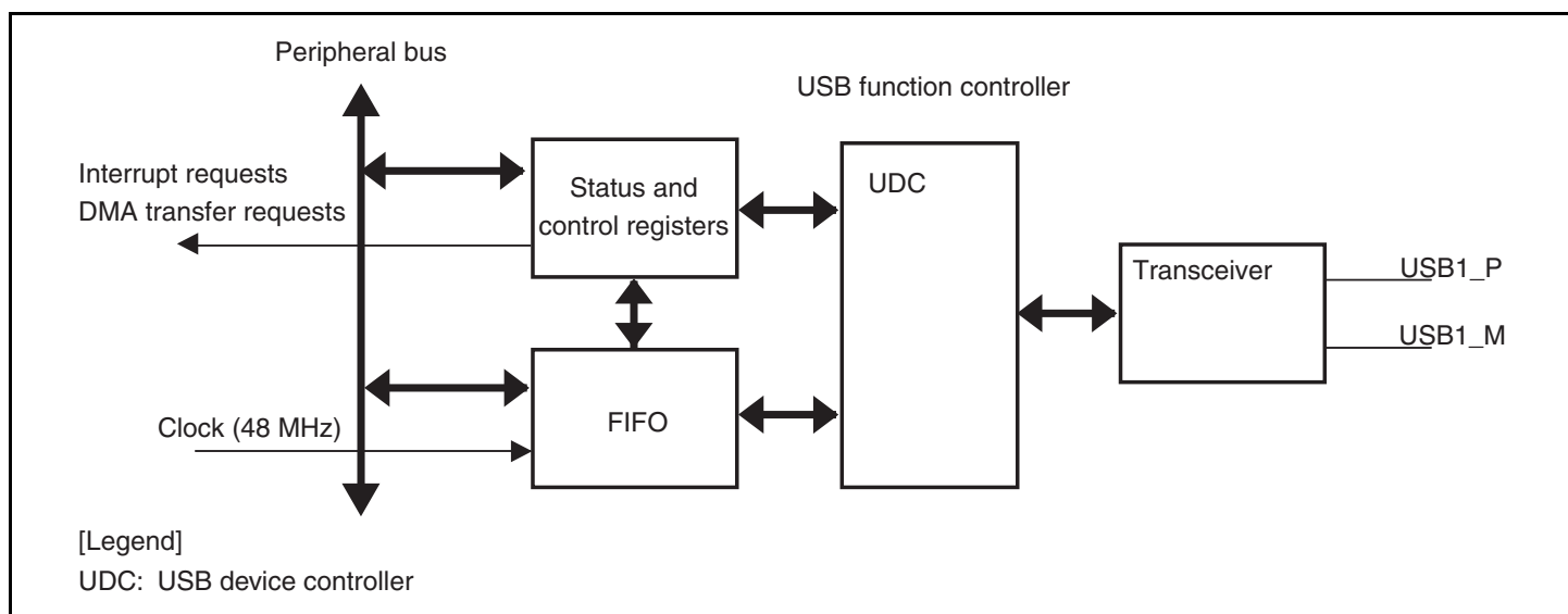
Figure 25.1 Block Diagram of USBF
