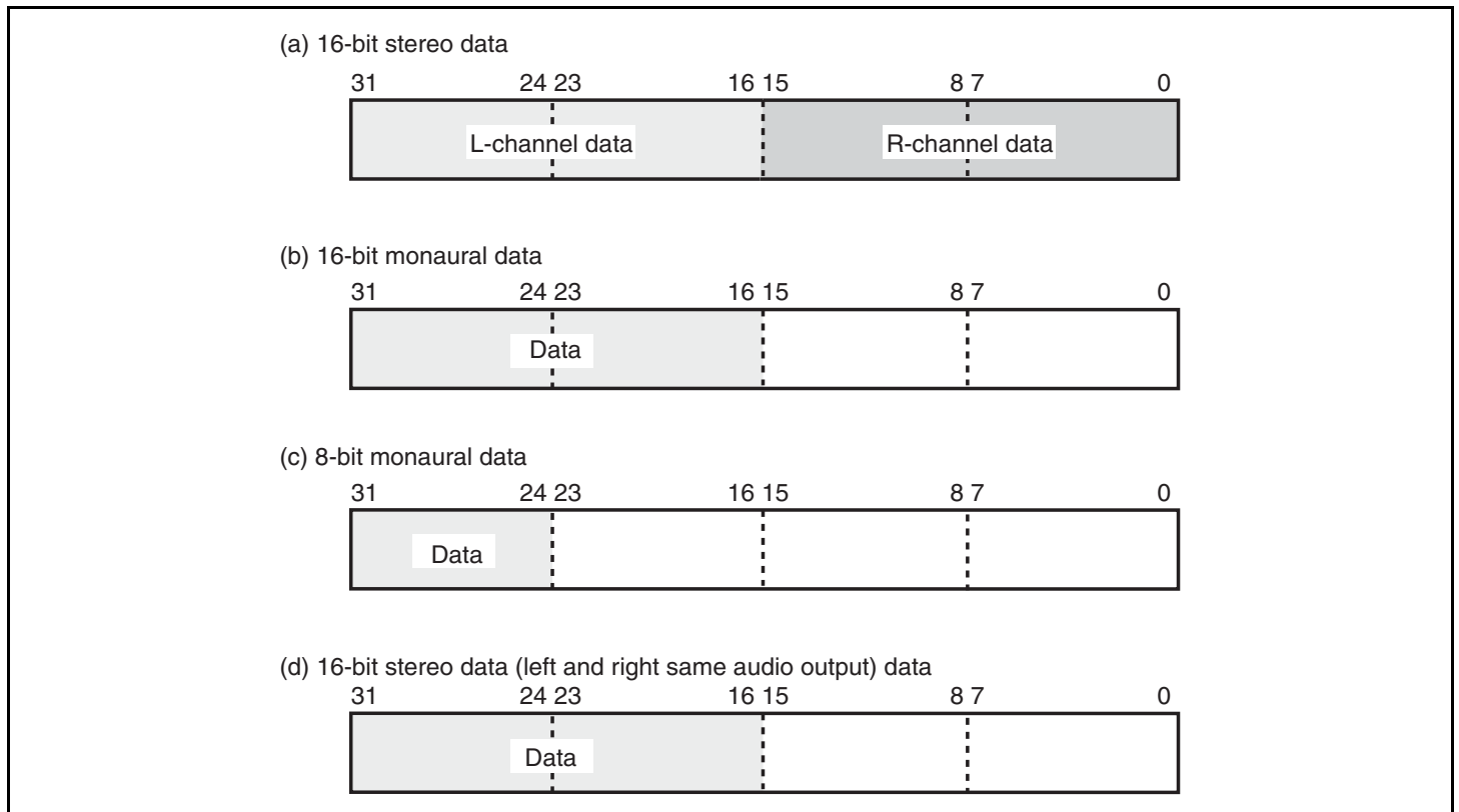
Figure 21.5 Transmit/Receive Data Bit Alignment
