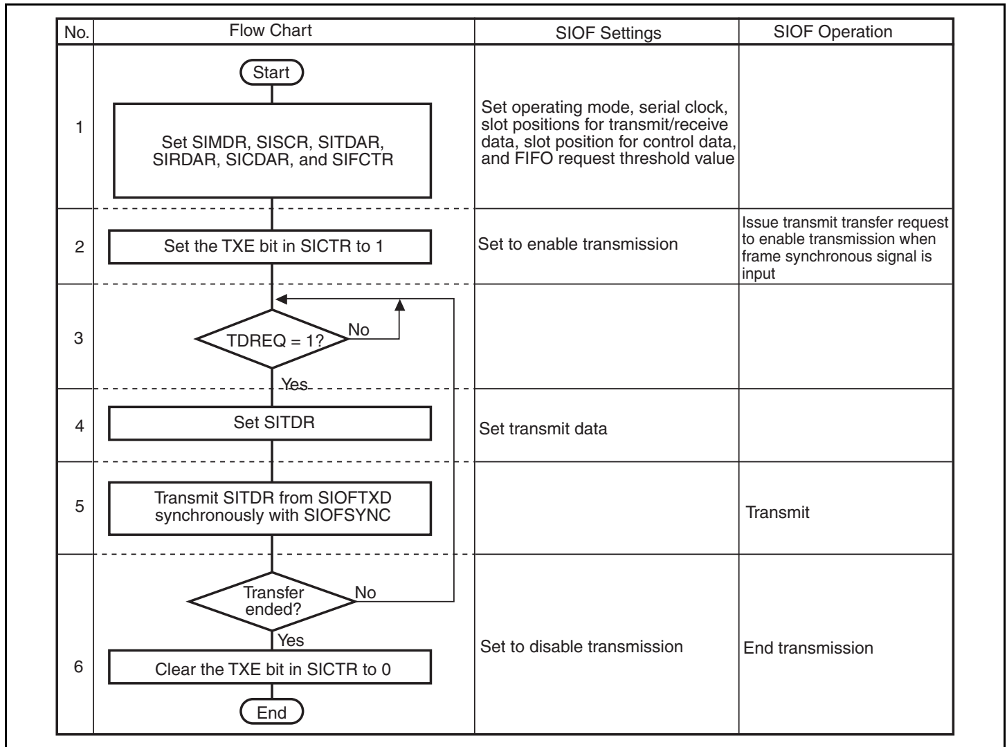
Figure 21.11 Example of Transmit Operation in Slave Mode
