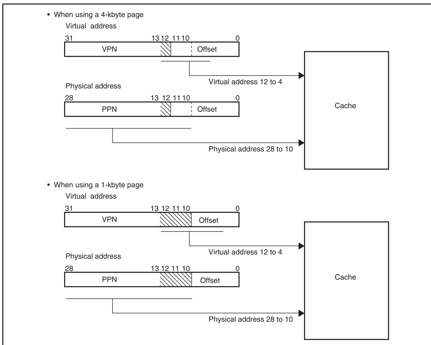
Figure 4.12 Synonym Problem (32-kbyte Cache)
