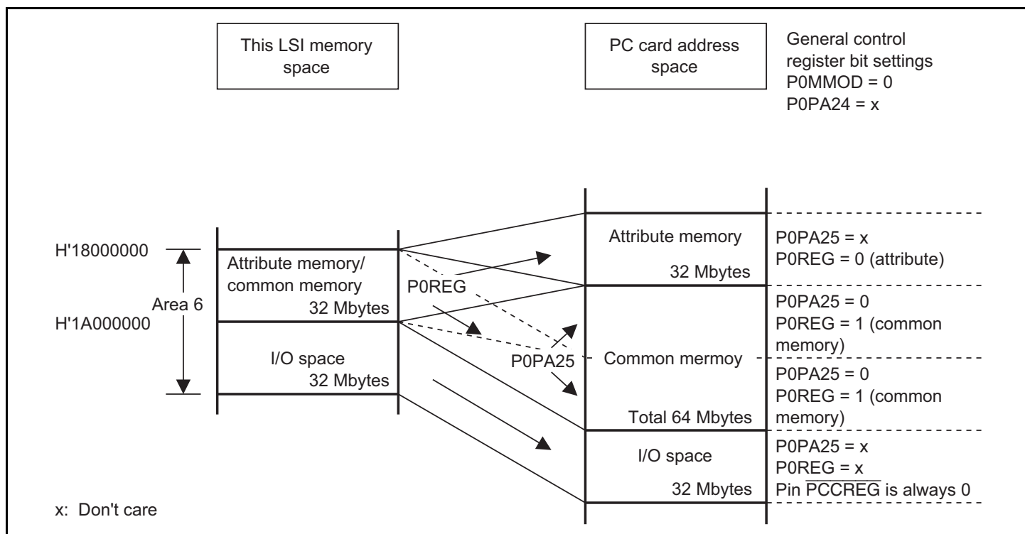
Figure 29.2 Continuous 32-Mbyte Area Mode
