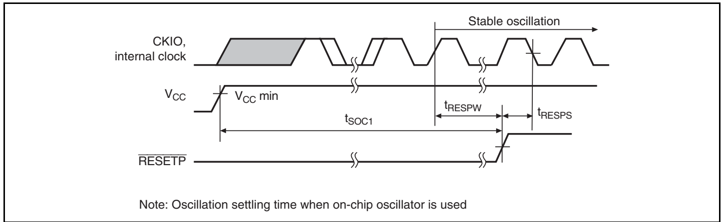
Figure 38.4 Power-On Oscillation Settling Time
