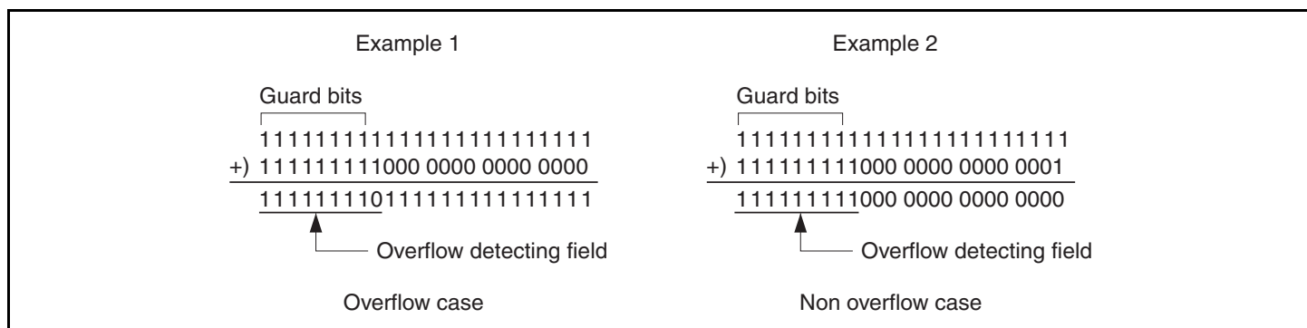
Figure 3.13 DC Bit Generation Examples in Overflow Mode
