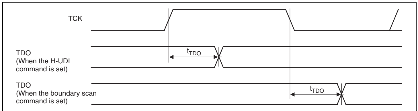
Figure 36.3 H-UDI Data Transfer Timing
