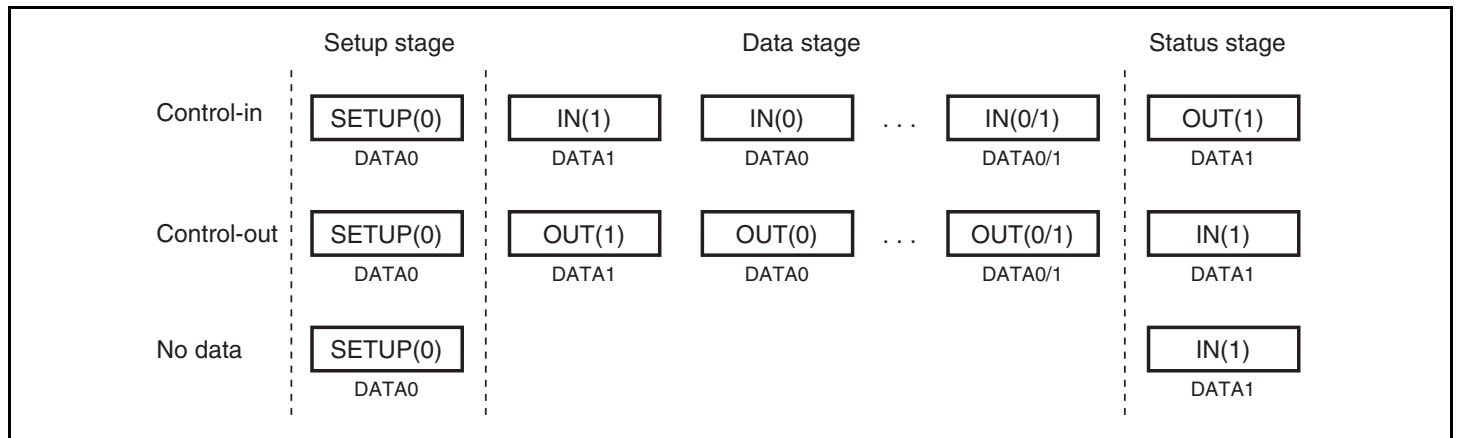
Figure 25.5 Transfer Stages in Control Transfer
