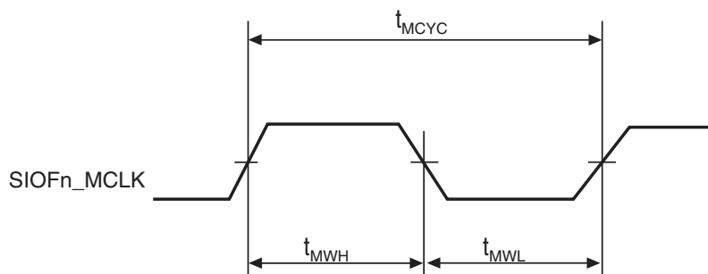
Figure 38.53 SIOF_MCLK Input Timing
