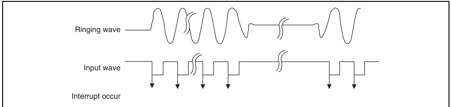
Figure 22.3 Ringing Interrupt Occurrence Timing
