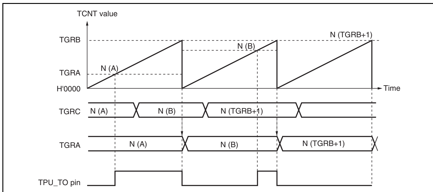
Figure 15.10 Example of Buffer Operation
