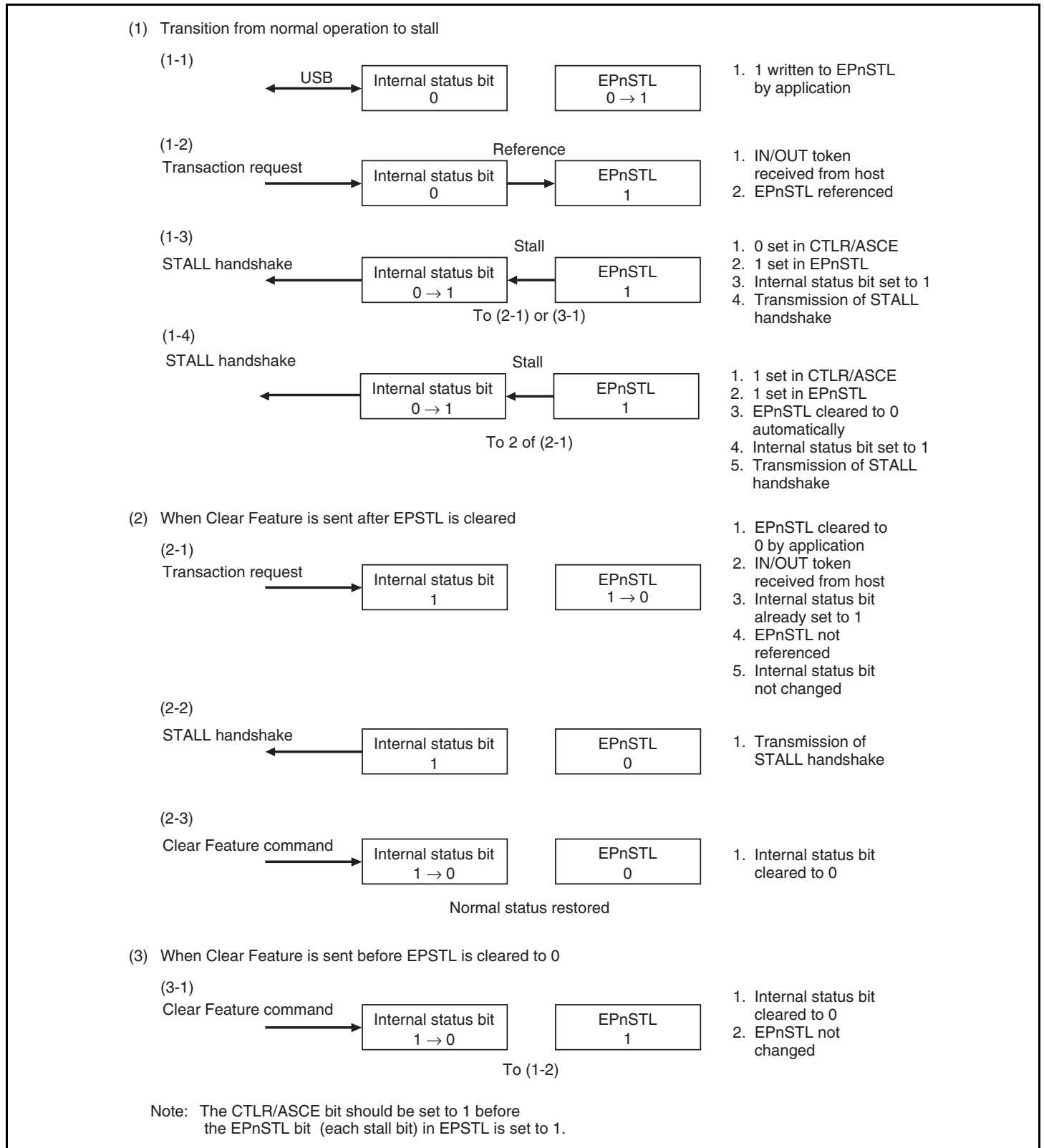
Figure 25.18 Forcible Stall by Application
