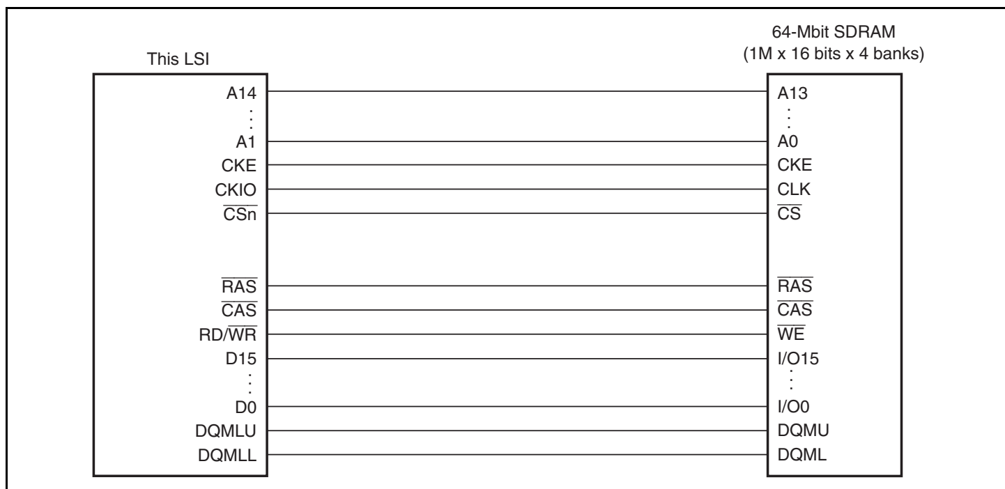
Figure 9.13 Example of 16-Bit Data-Width SDRAM Connection
