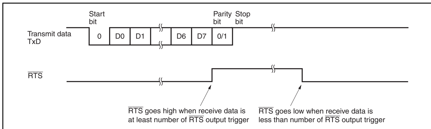
Figure 18.11 Example of \overline{\text{RTS}} Control Operation
