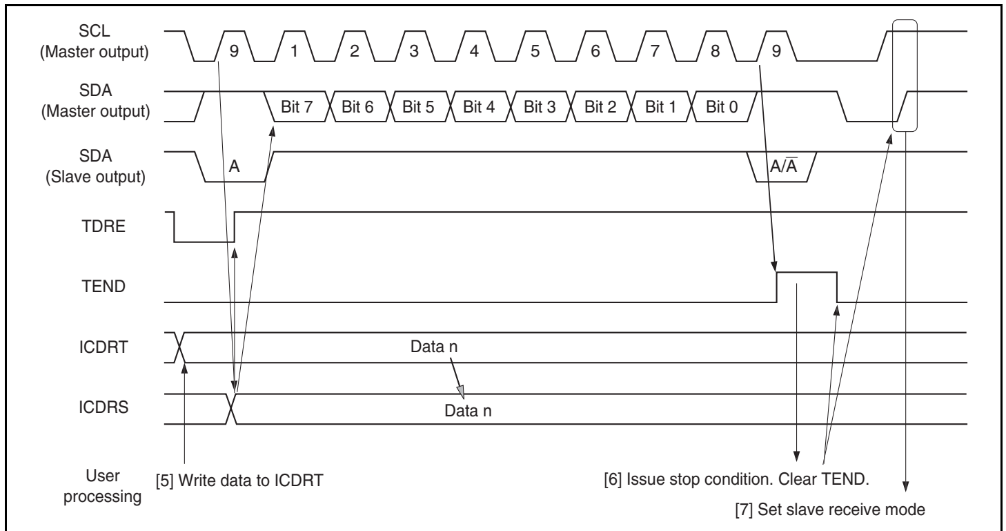
Figure 20.6 Master Transmit Mode Operation Timing (2)
