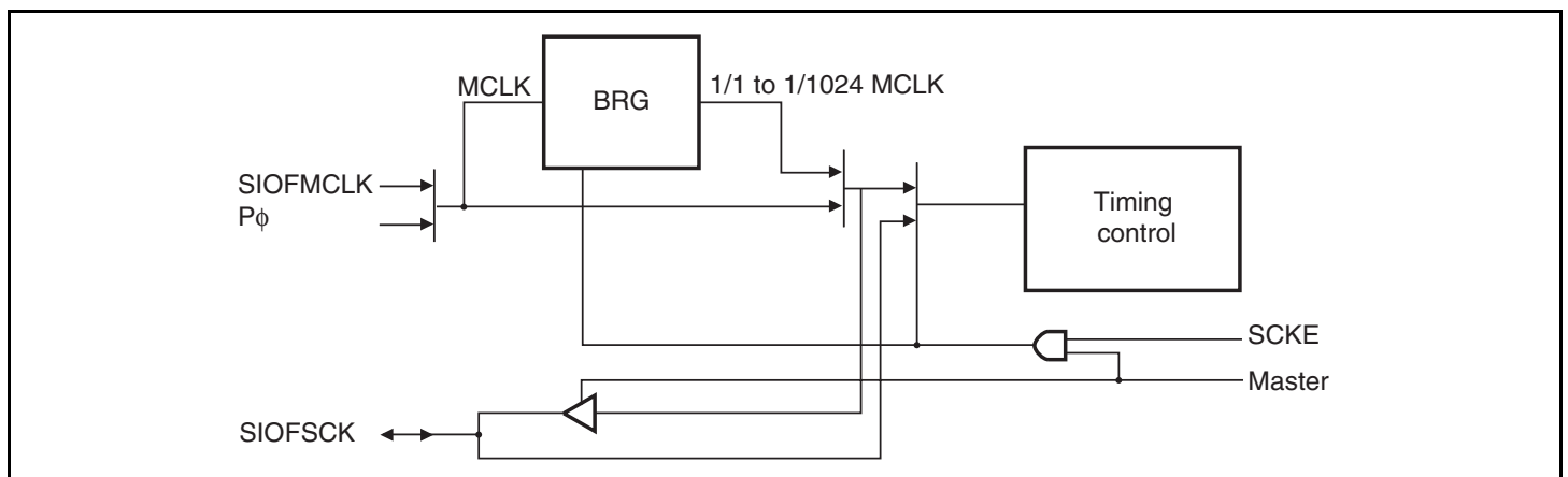
Figure 21.2 Serial Clock Supply
