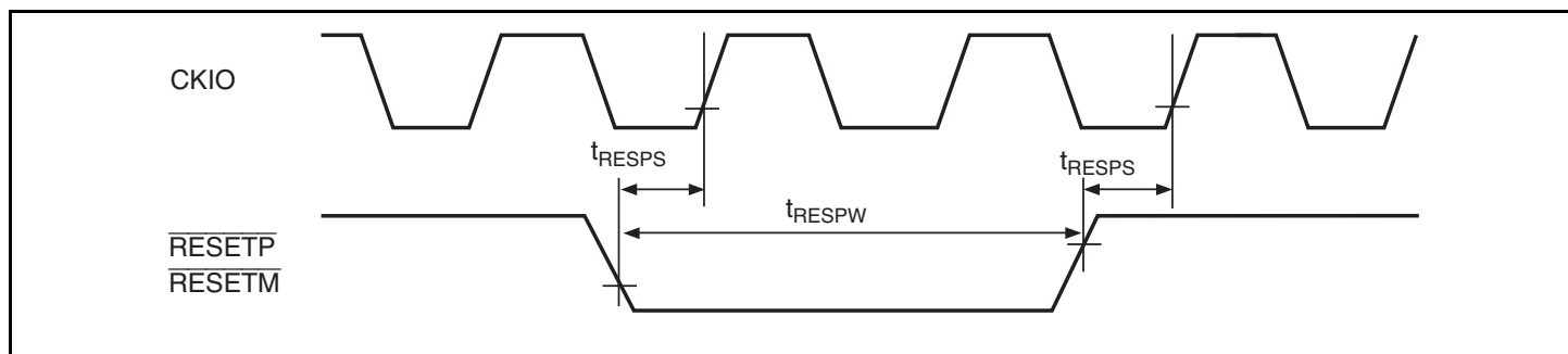
Figure 38.8 Reset Input Timing
