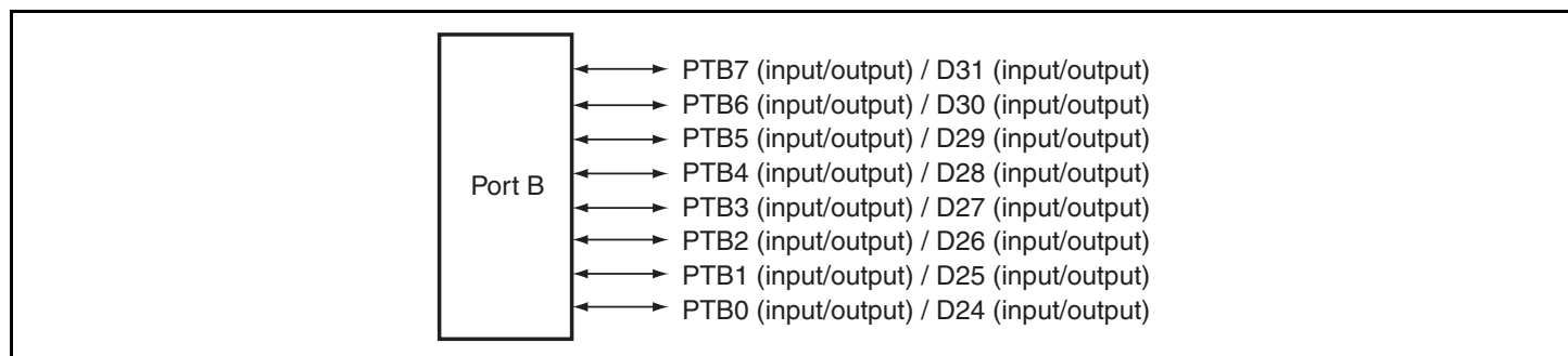
Figure 35.2 Port B
