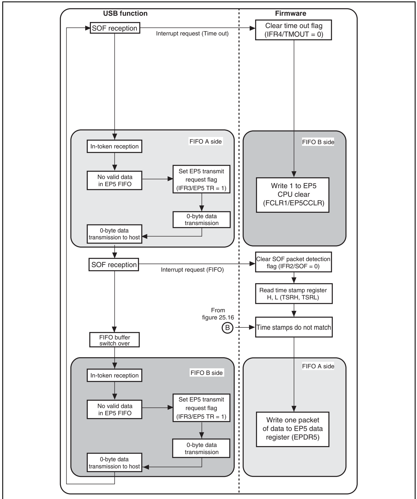
Figure 25.17 EP5 Isochronous-In Transfer Operation (SOF in Broken)
