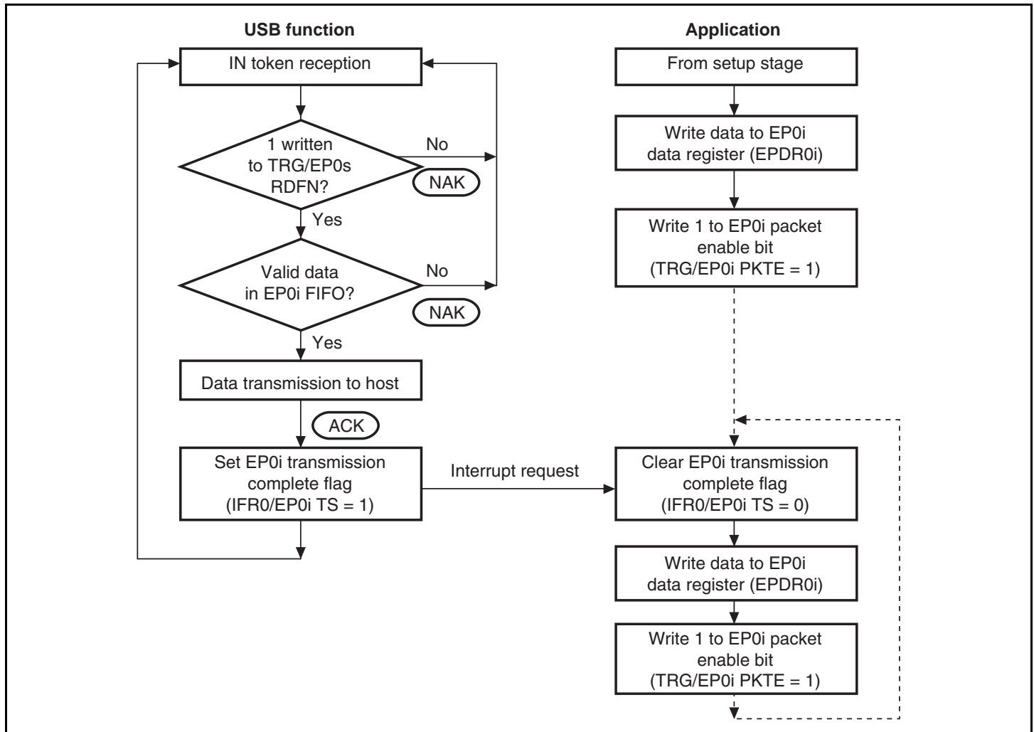
Figure 25.7 Data Stage (Control-In) Operation
