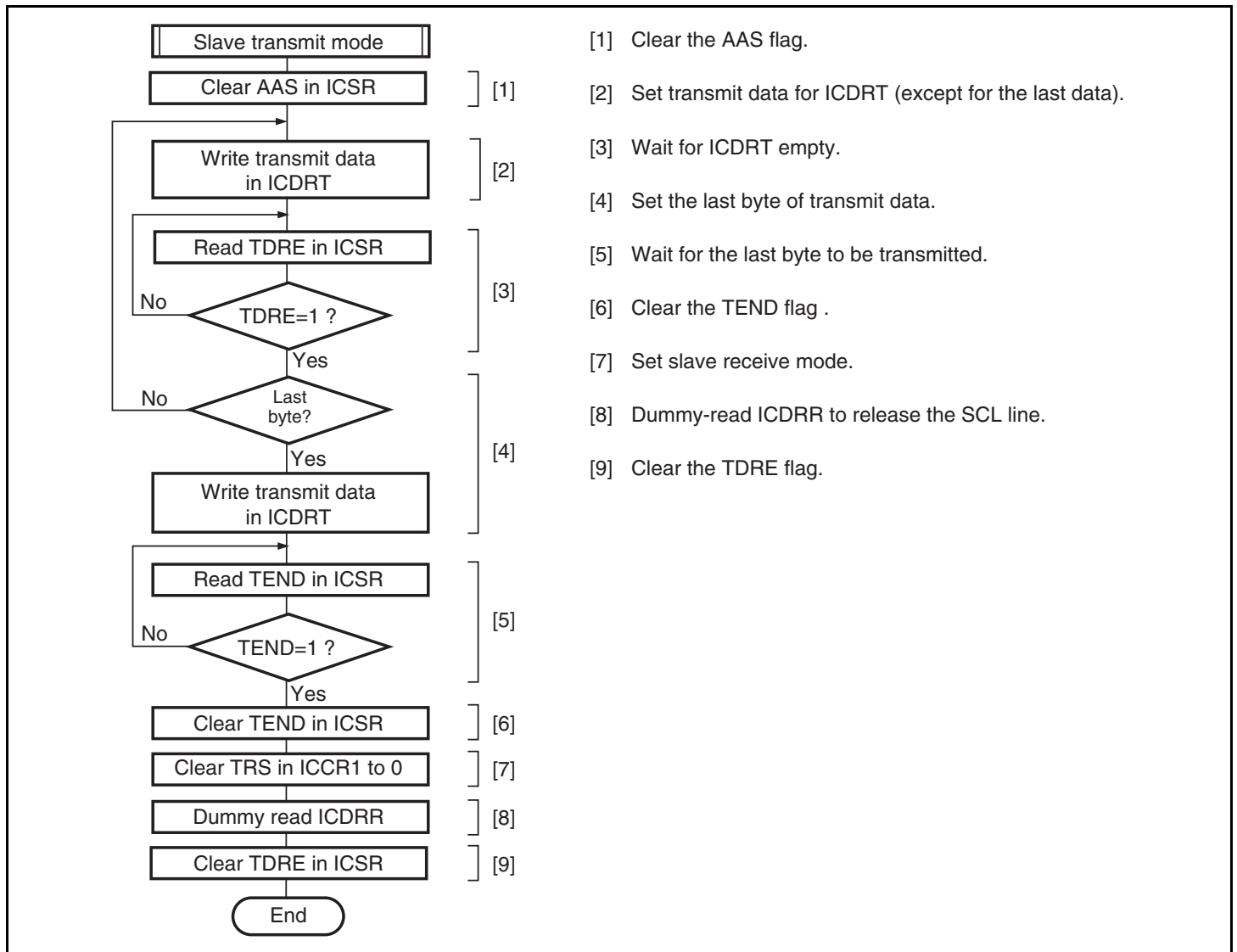
Figure 20.16 Sample Flowchart for Slave Transmit Mode
