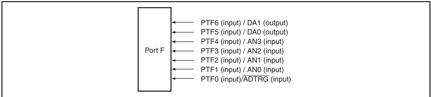
Figure 35.6 Port F
