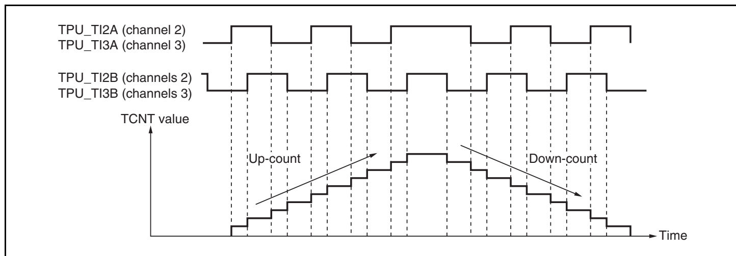
Figure 15.15 Example of Phase Counting Mode 1 Operation
