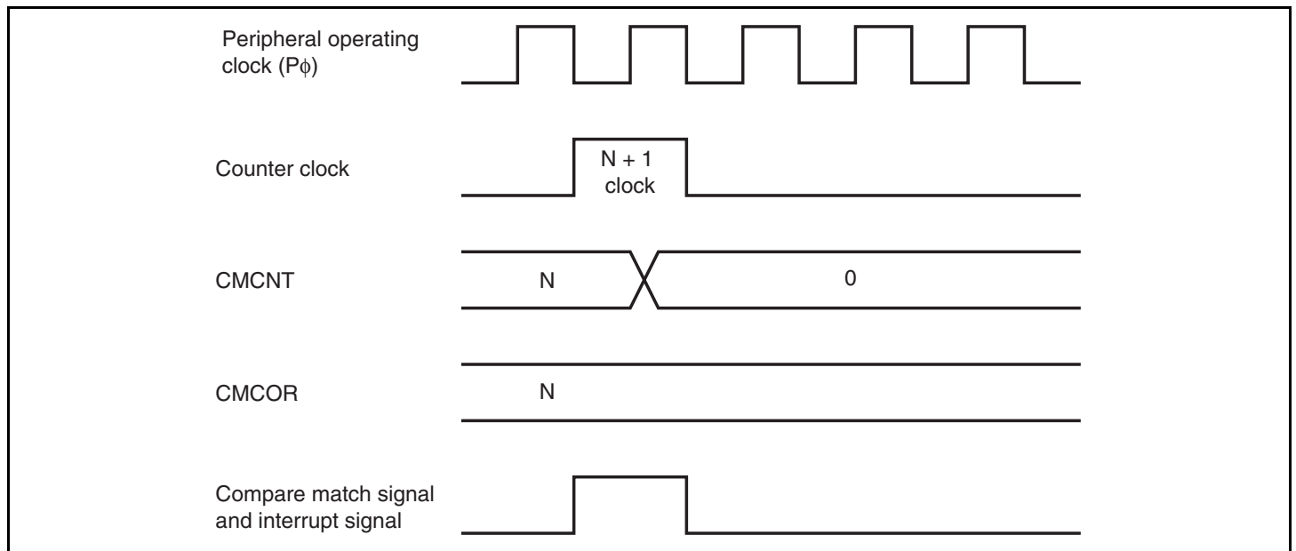
Figure 16.4 CMF Set Timing
