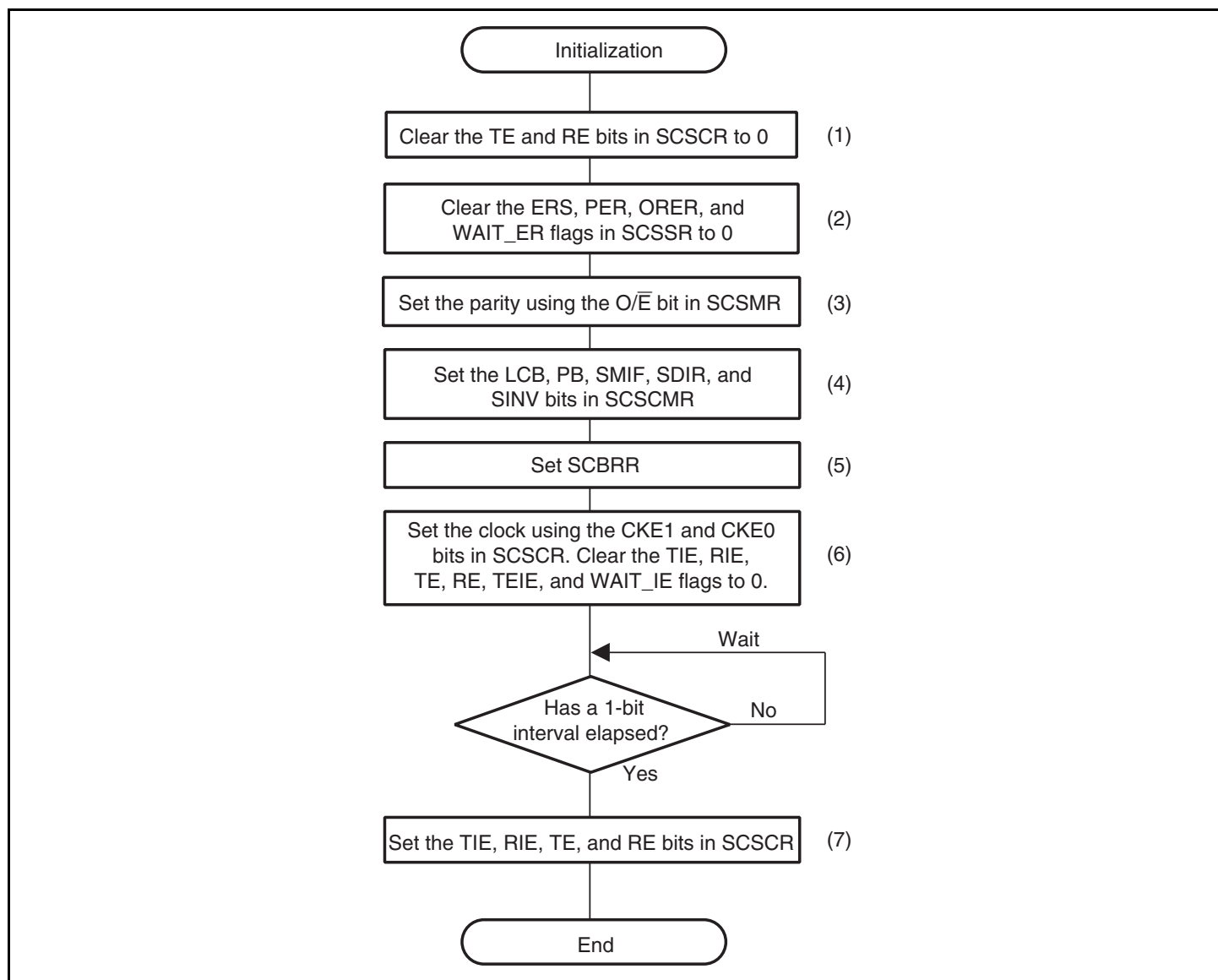
Figure 30.4 Example of Initialization Flow
