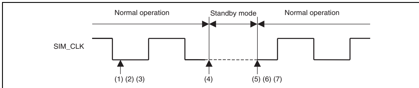
Figure 30.10 Procedure for Stopping Clock and Restarting
