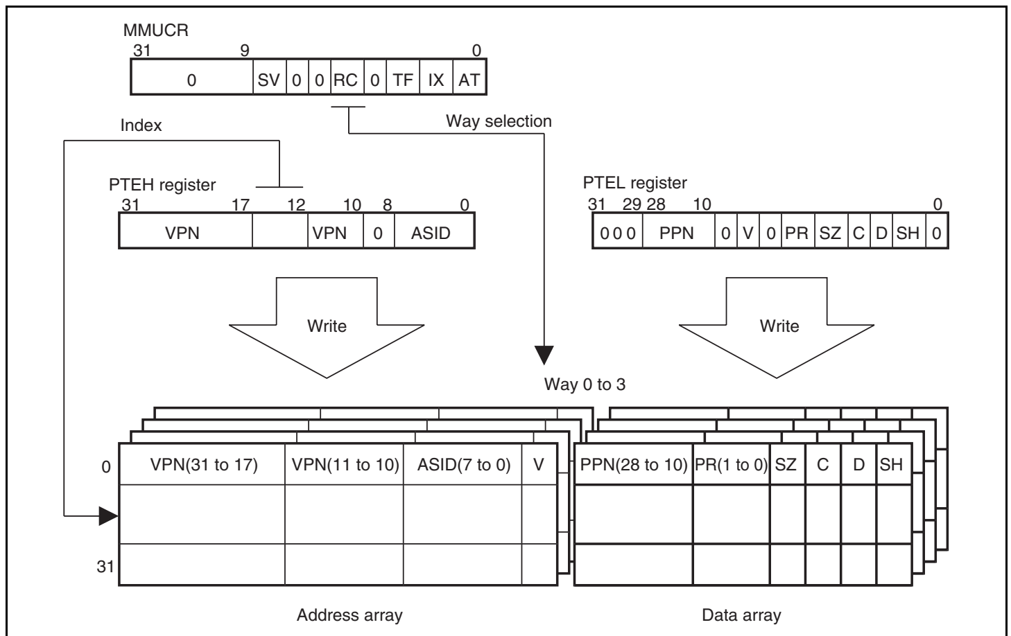
Figure 4.11 Operation of LDTLB Instruction
