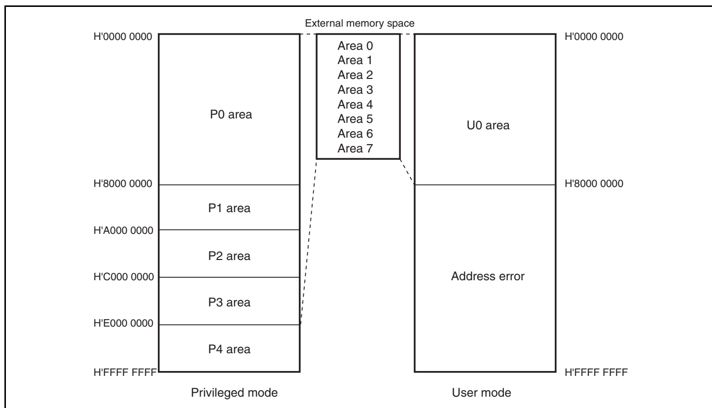
Figure 2.2 Virtual Address to External Memory Space Mapping
