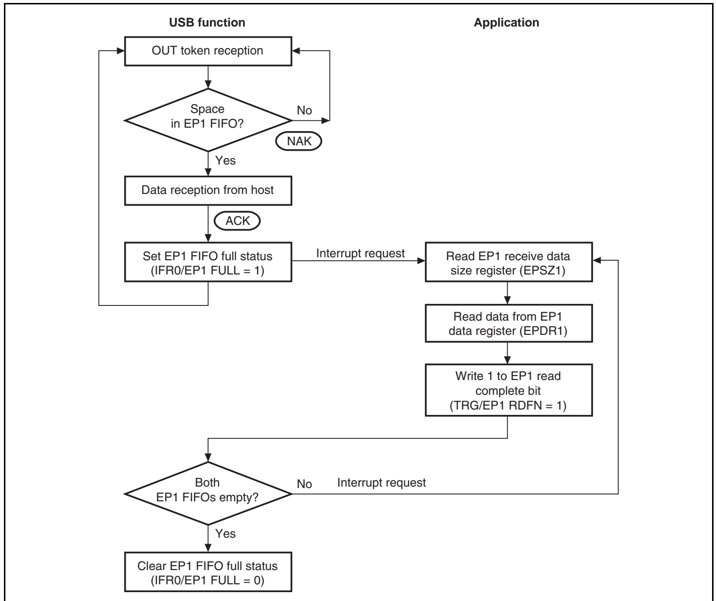
Figure 25.11 EP1 Bulk-Out Transfer Operation
