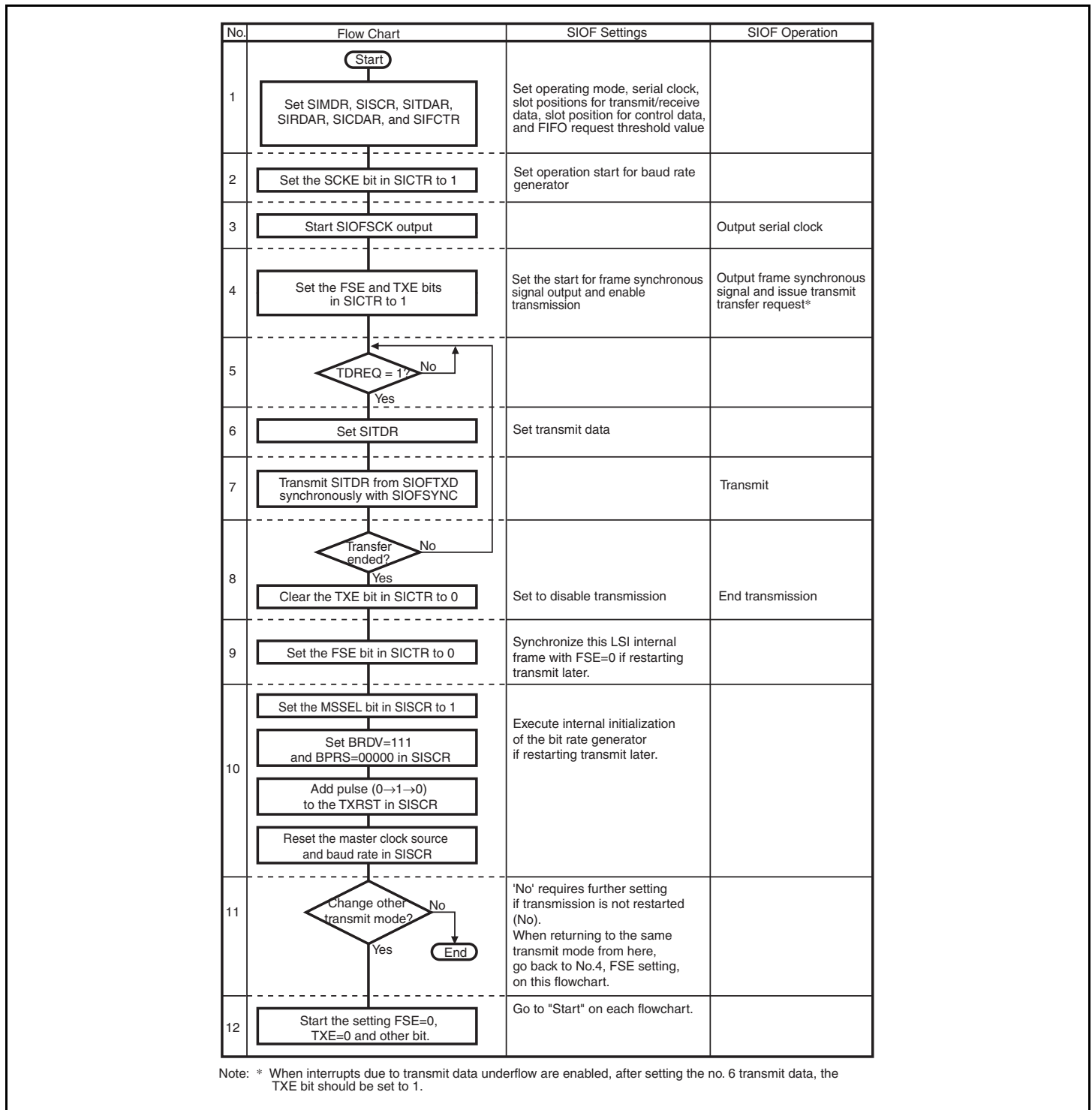
Figure 21.9 Example of Transmit Operation in Master Mode
