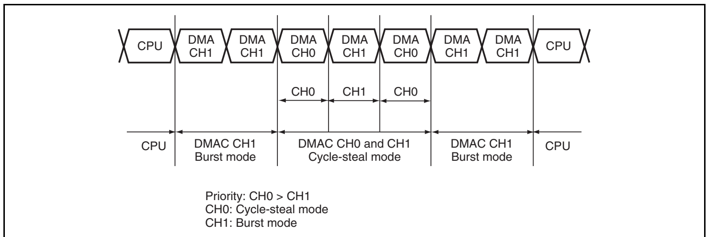
Figure 10.12 Bus State when Multiple Channels are Operating
