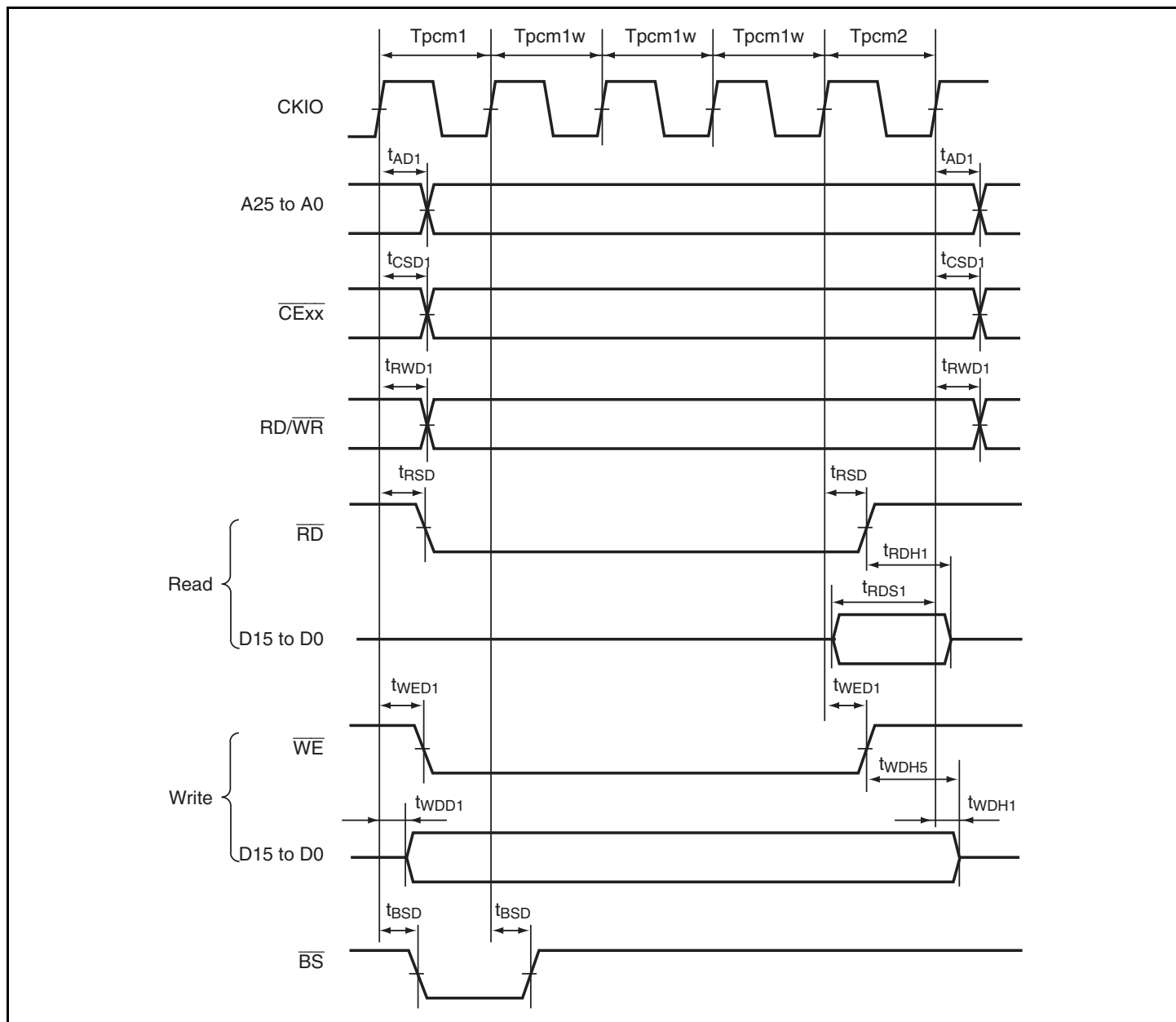
Figure 38.39 PCMCIA Memory Card Interface Bus Timing
