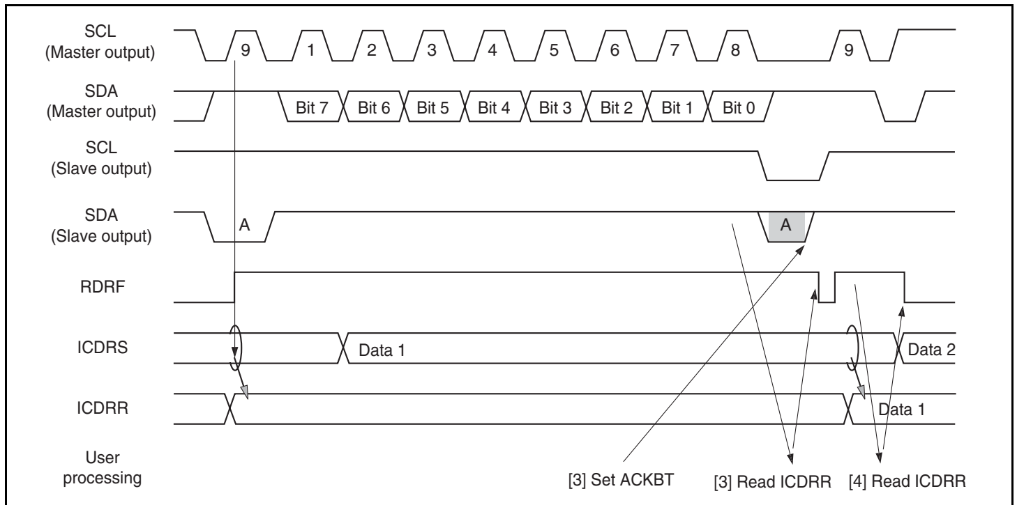
Figure 20.12 Slave Receive Mode Operation Timing (2)
