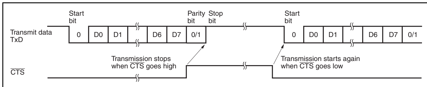
Figure 18.10 Example of \overline{\text{CTS}} Control Operation
