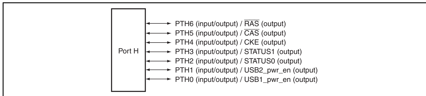
Figure 35.8 Port H
