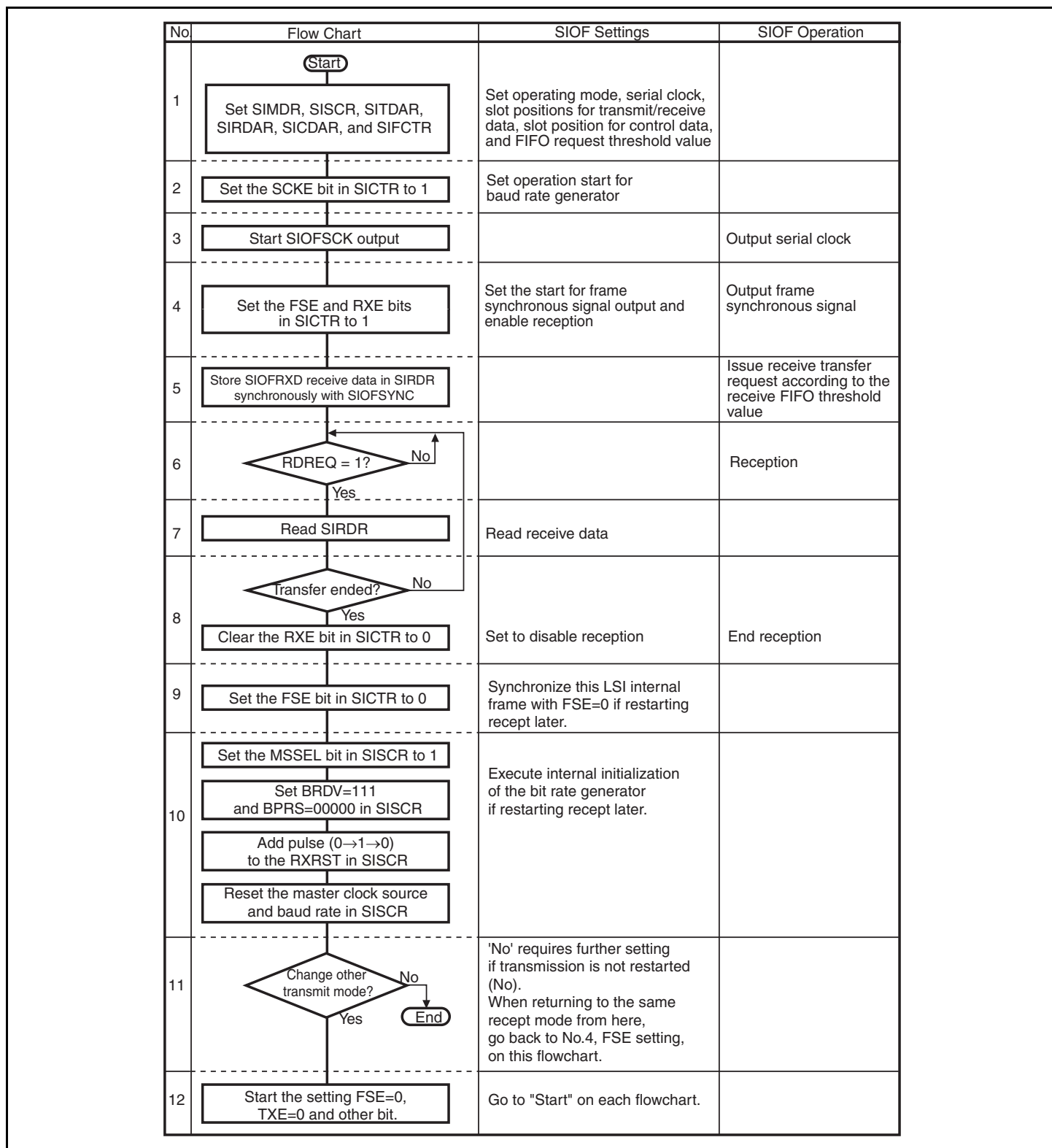
Figure 21.10 Example of Receive Operation in Master Mode
