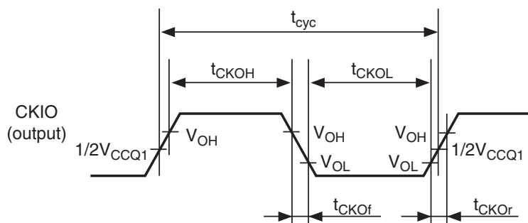
Figure 38.2 CKIO Clock Output Timing
