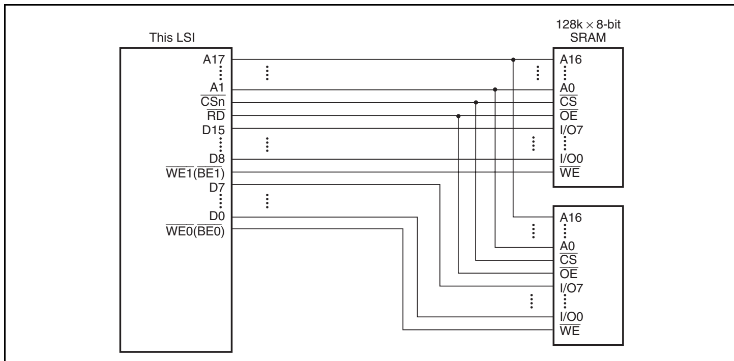
Figure 9.7 Example of 16-Bit Data-Width SRAM Connection
