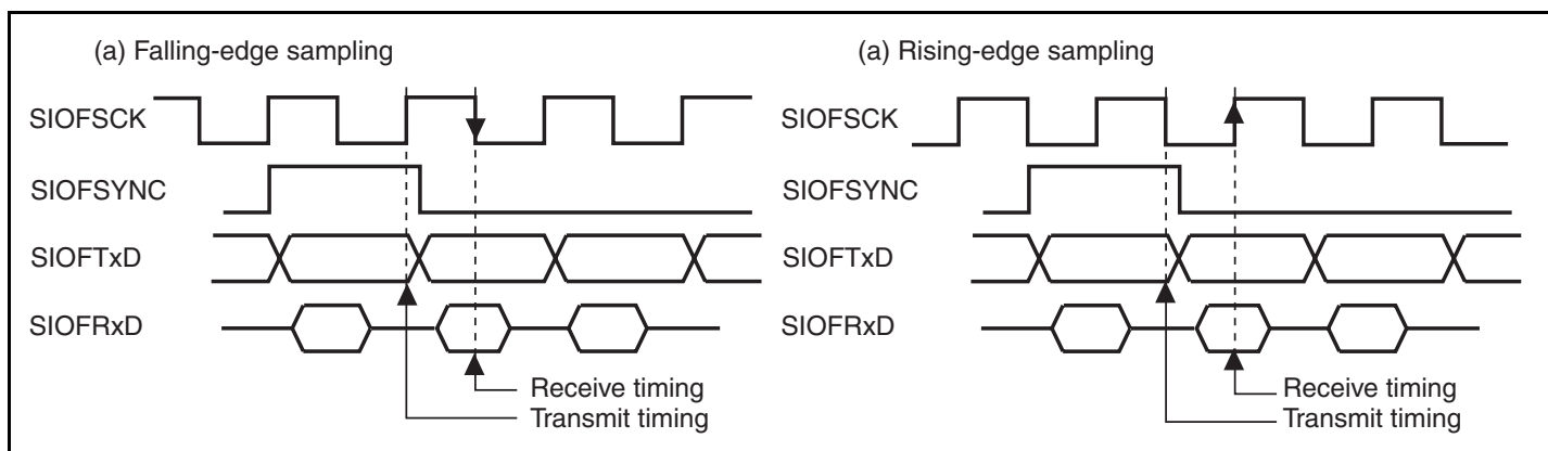
Figure 21.4 SIOF Transmit/Receive Timing
