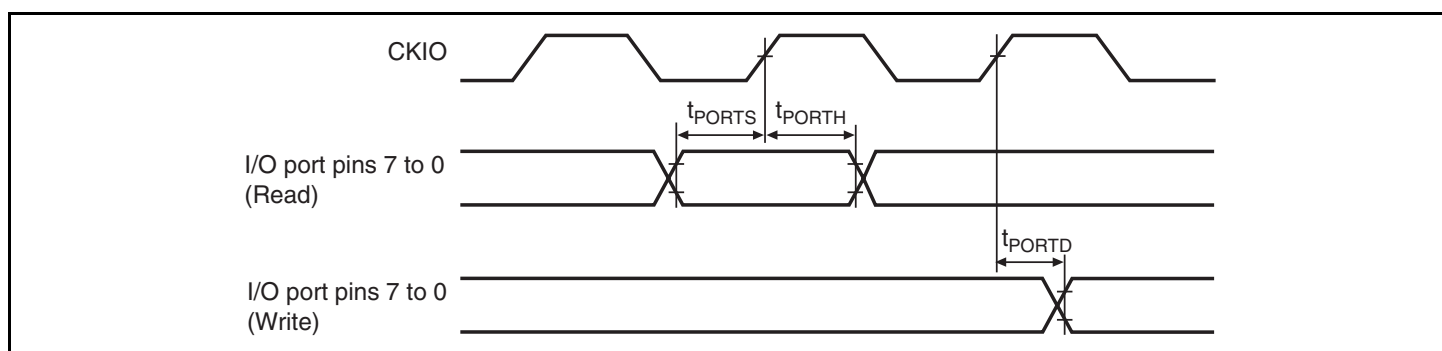
Figure 38.44 I/O Port Timing
