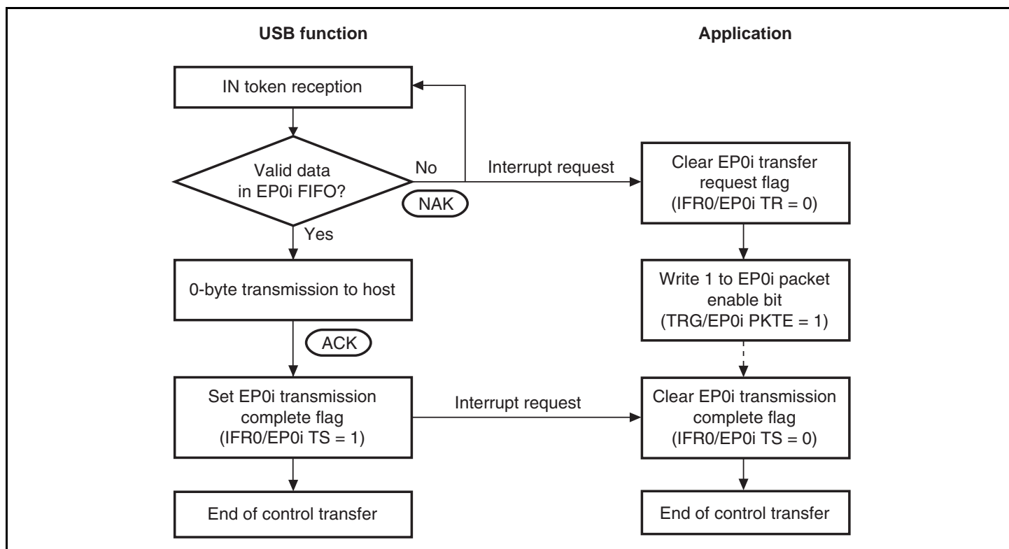
Figure 25.10 Status Stage (Control-Out) Operation
