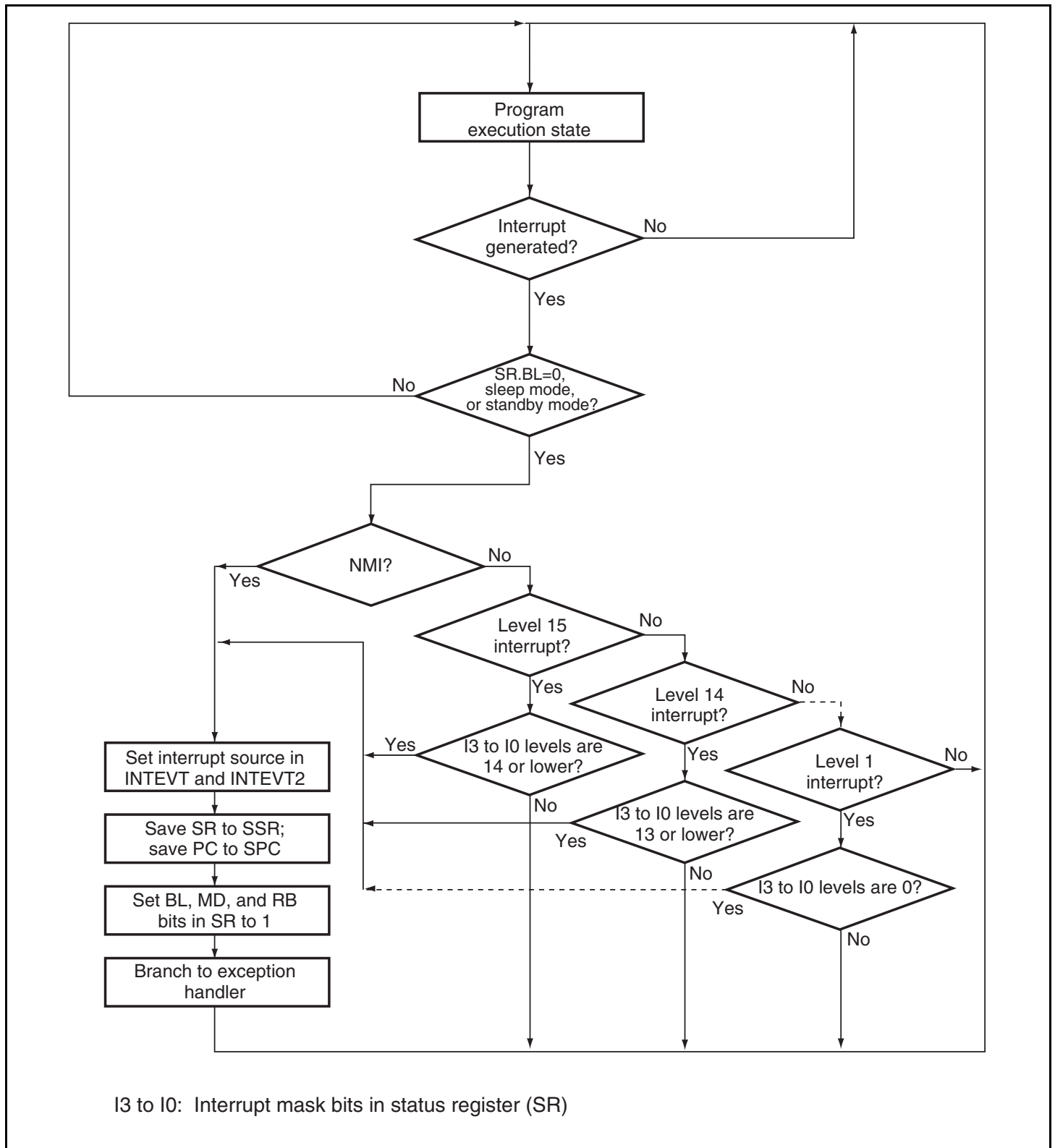
Figure 8.3 Interrupt Operation Flowchart
