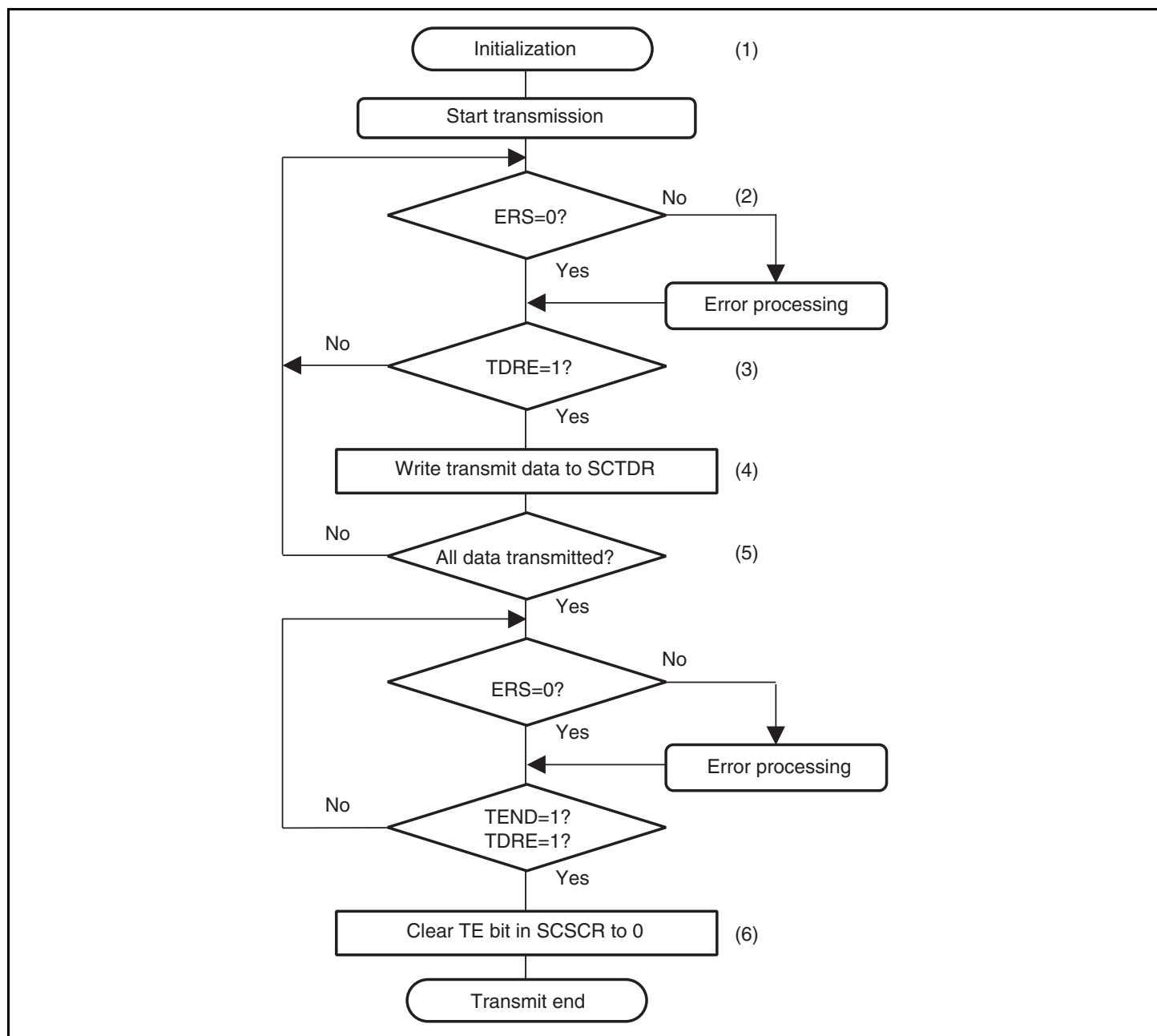
Figure 30.5 Example of Transmit Processing
