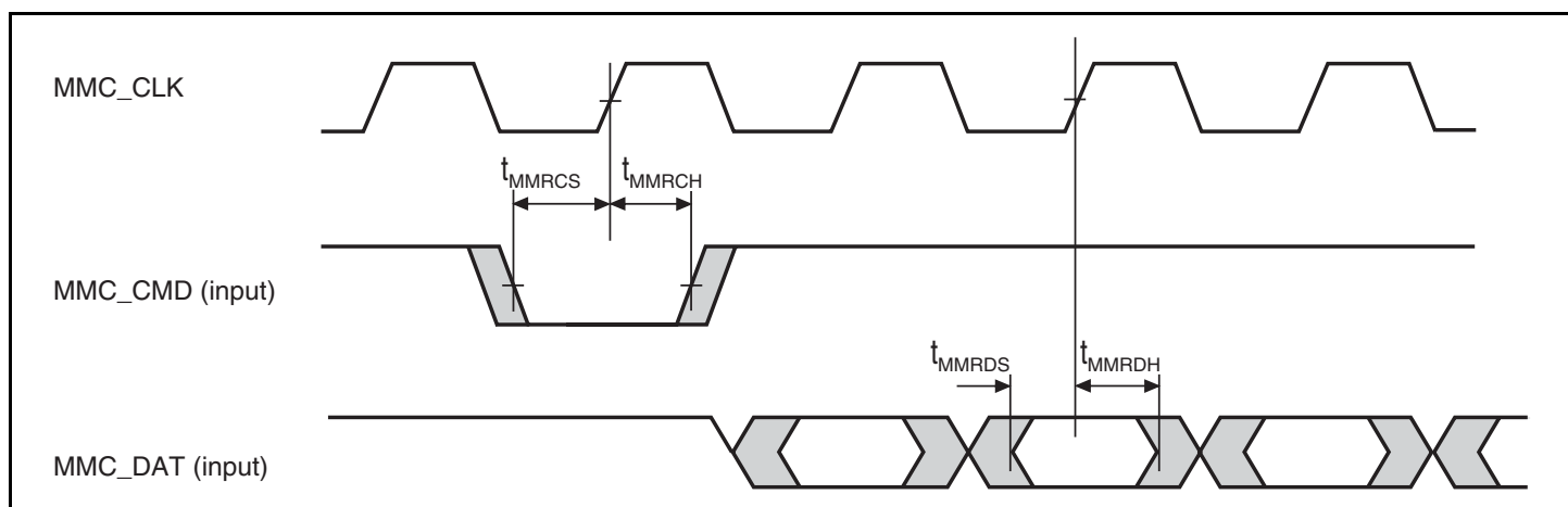
Figure 38.64 MMCIF Receive Timing (Rise Sampling)
