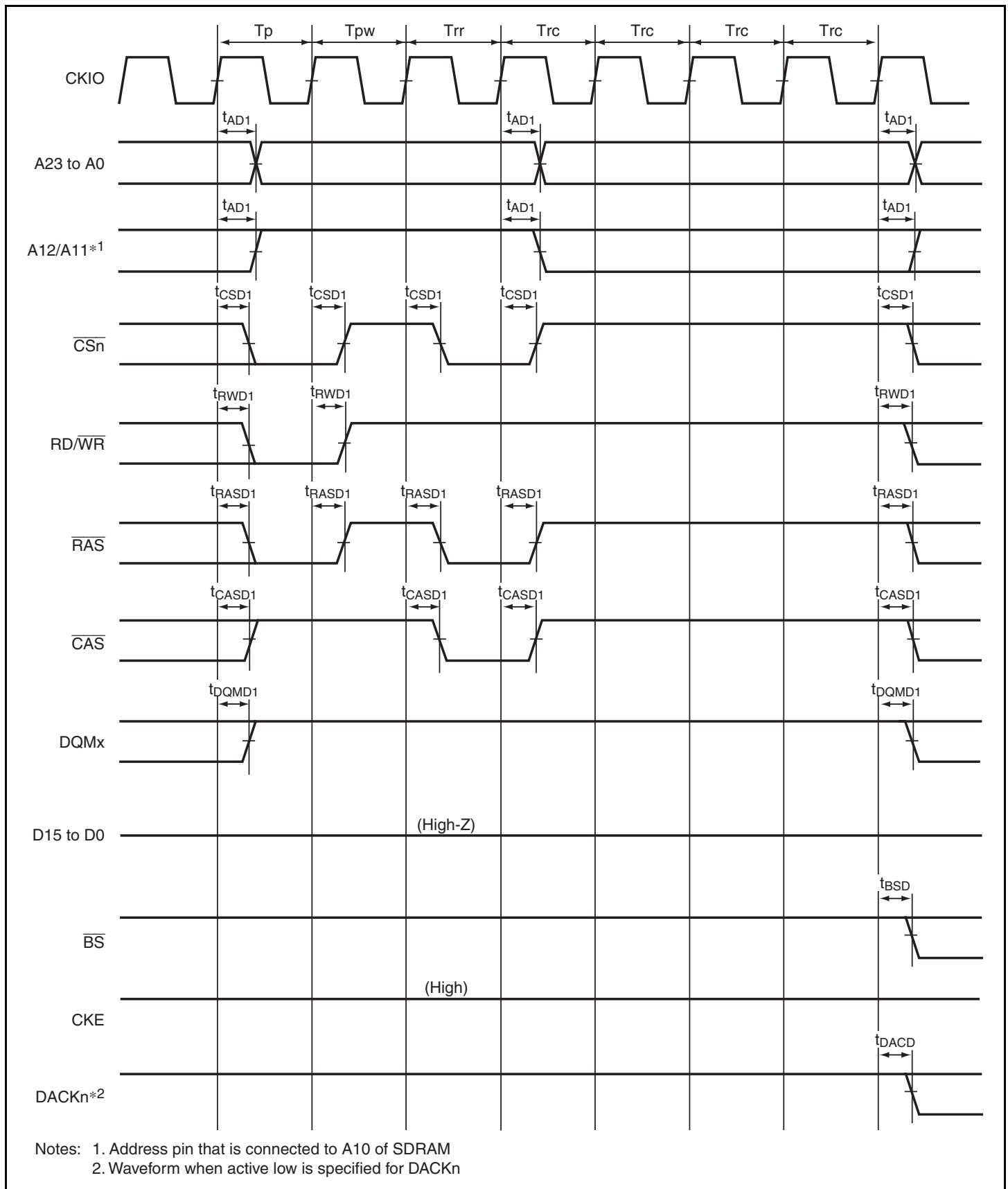
Figure 38.34 Auto Refresh Timing of SDRAM (TRP = 2 Cycles)
