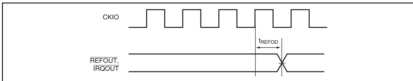
Figure 38.43 REFOUT, IRQOUT Delay Time
