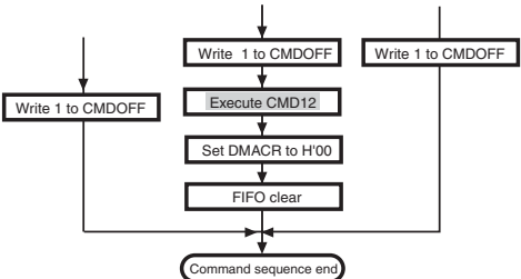
Figure 31.32 Operational Flowchart for Pre-defied Multiblock Write Transfer in Auto Mode (2)
