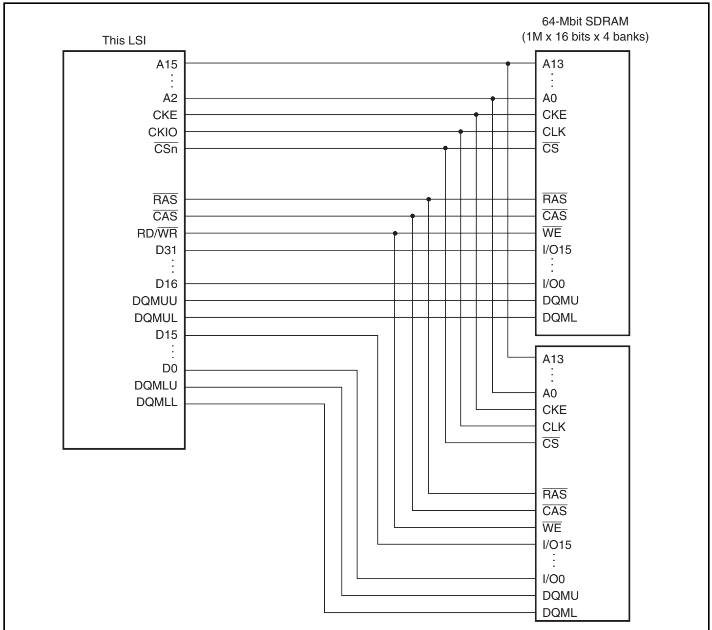
Figure 9.12 Example of 32-Bit Data-Width SDRAM Connection
