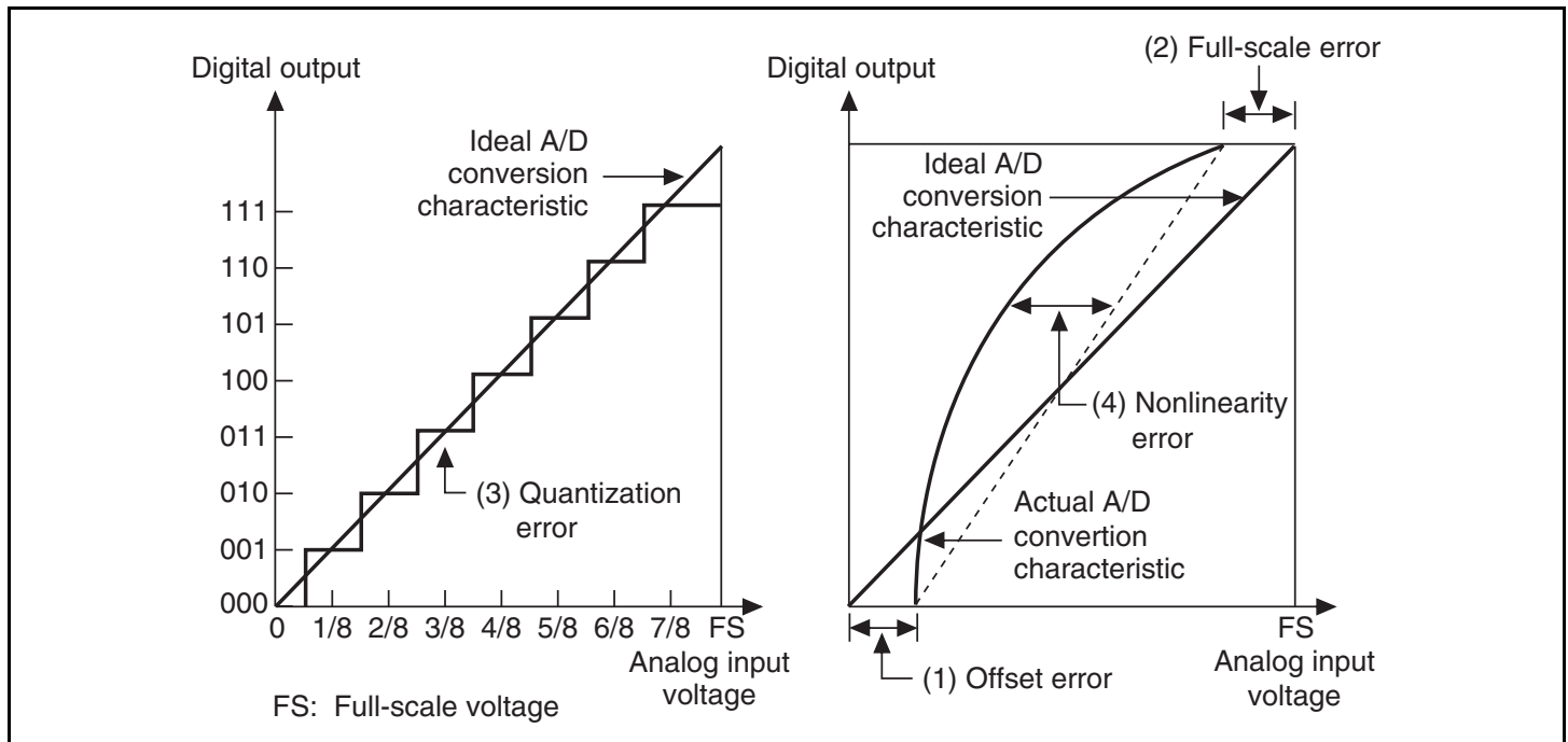
Figure 27.7 Definitions of A/D Conversion Accuracy
