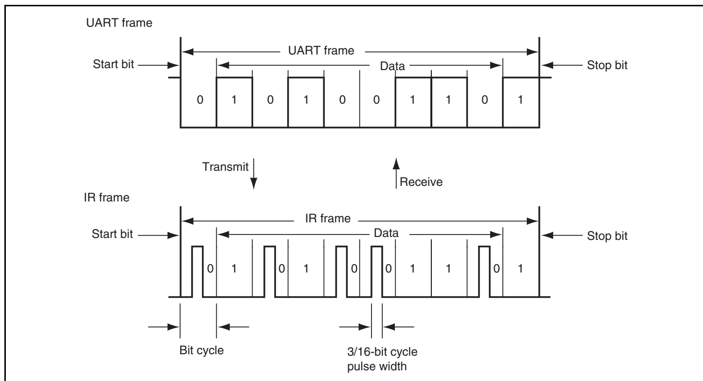
Figure 19.2 Transmit/Receive Operation
