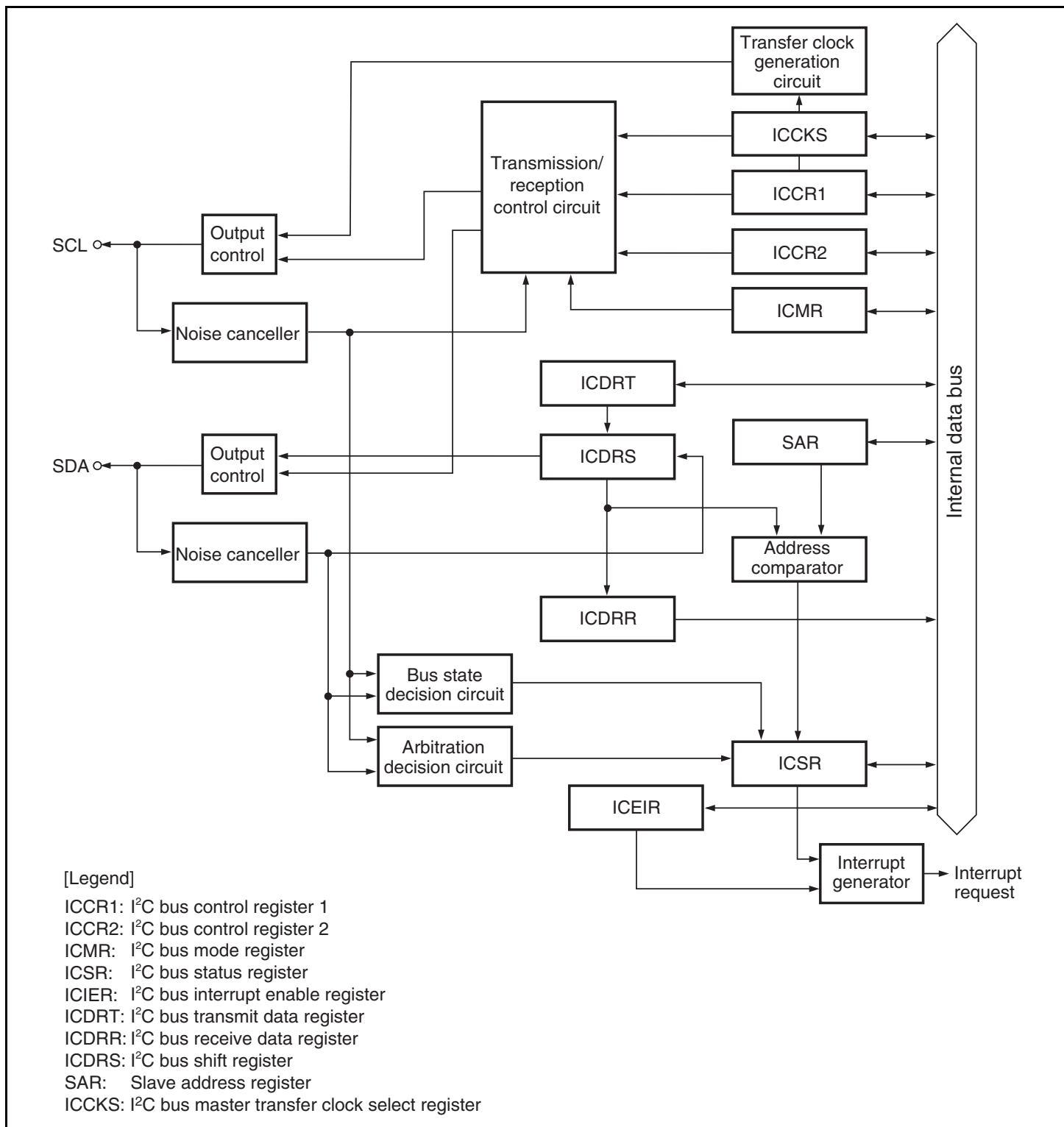
Figure 20.1 Block Diagram of I 2 C Bus Interface
