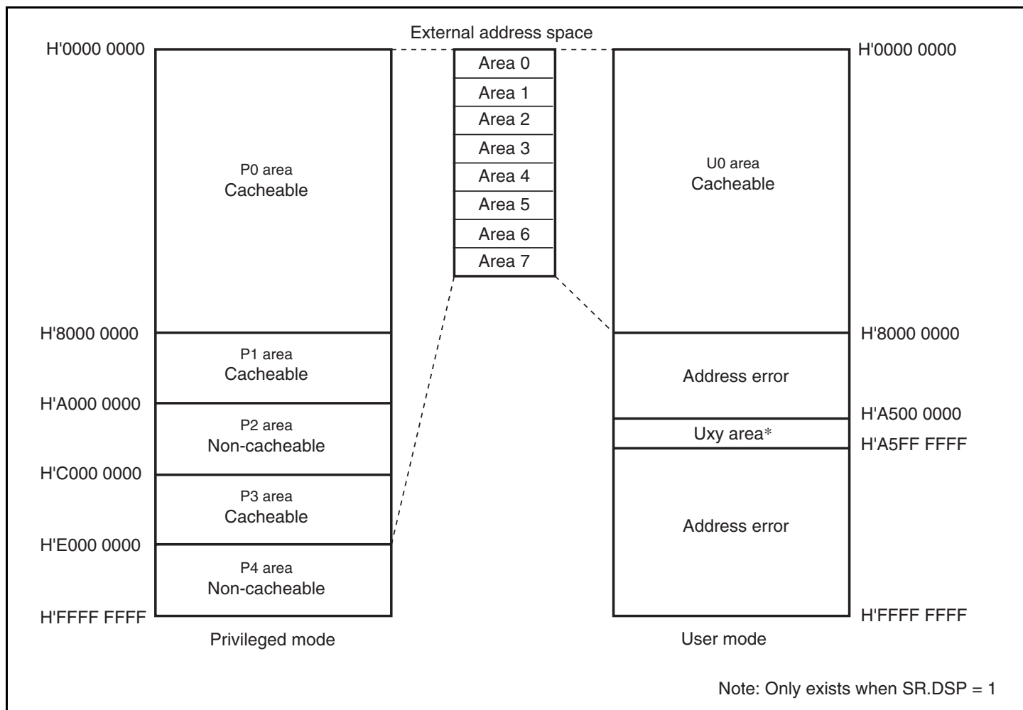
Figure 4.3 Virtual Address Space (MMUCR.AT = 0)
