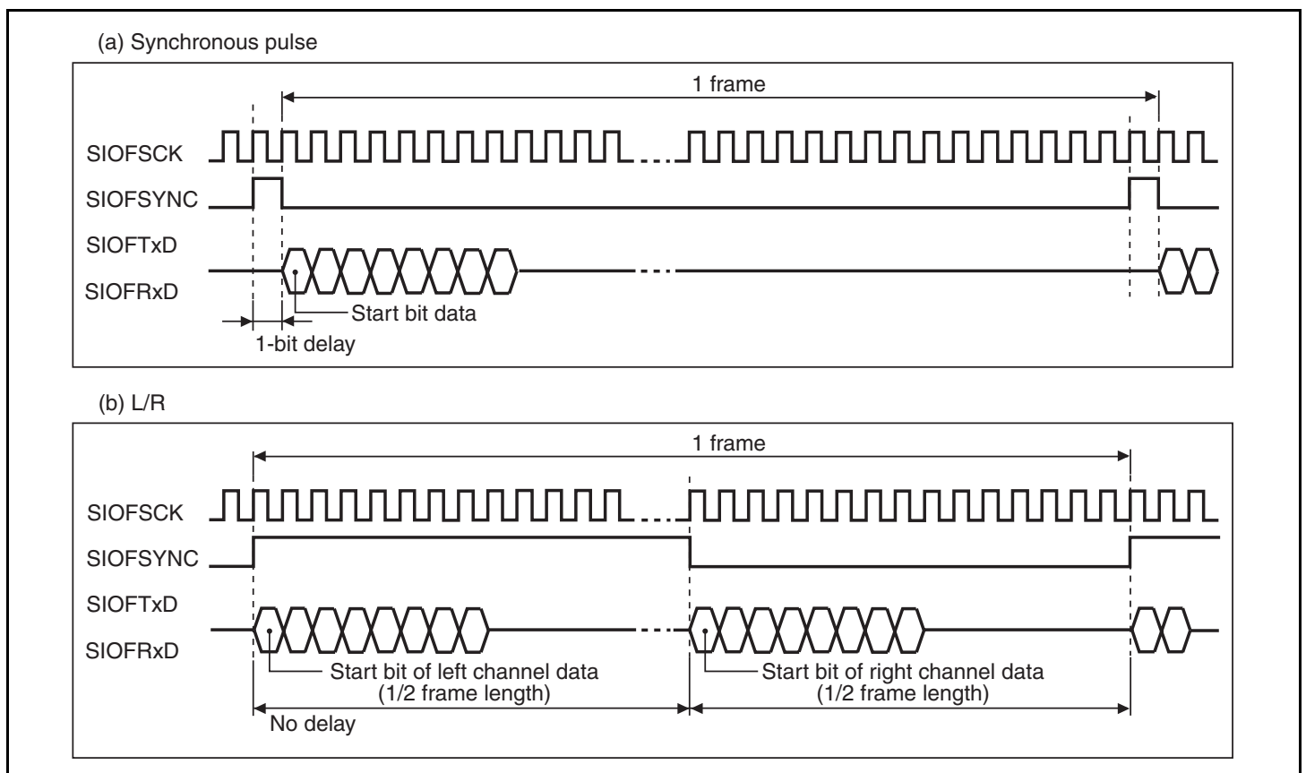
Figure 21.3 Serial Data Synchronization Timing
