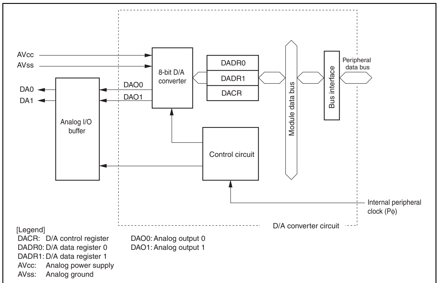
Figure 28.1 Block Diagram of D/A Converter
