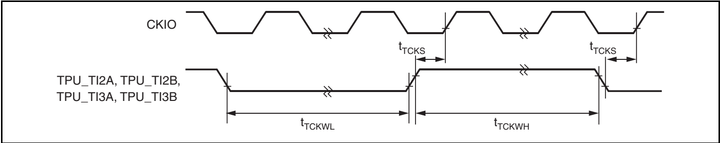
Figure 38.48 TPU Clock Input Timing
