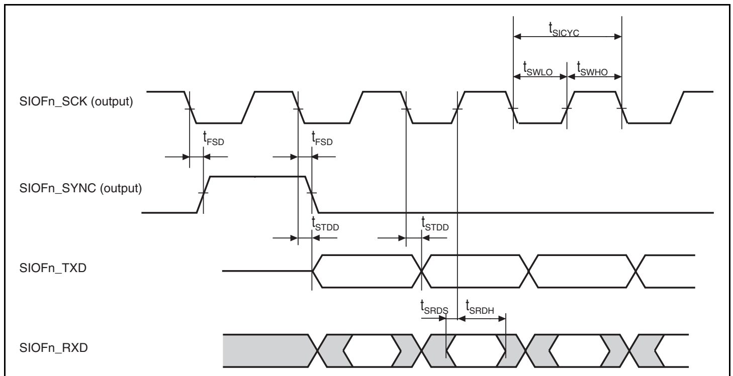
Figure 38.55 SIOF Transmission/Reception Timing (Master Mode 1, Rise Sampling)
