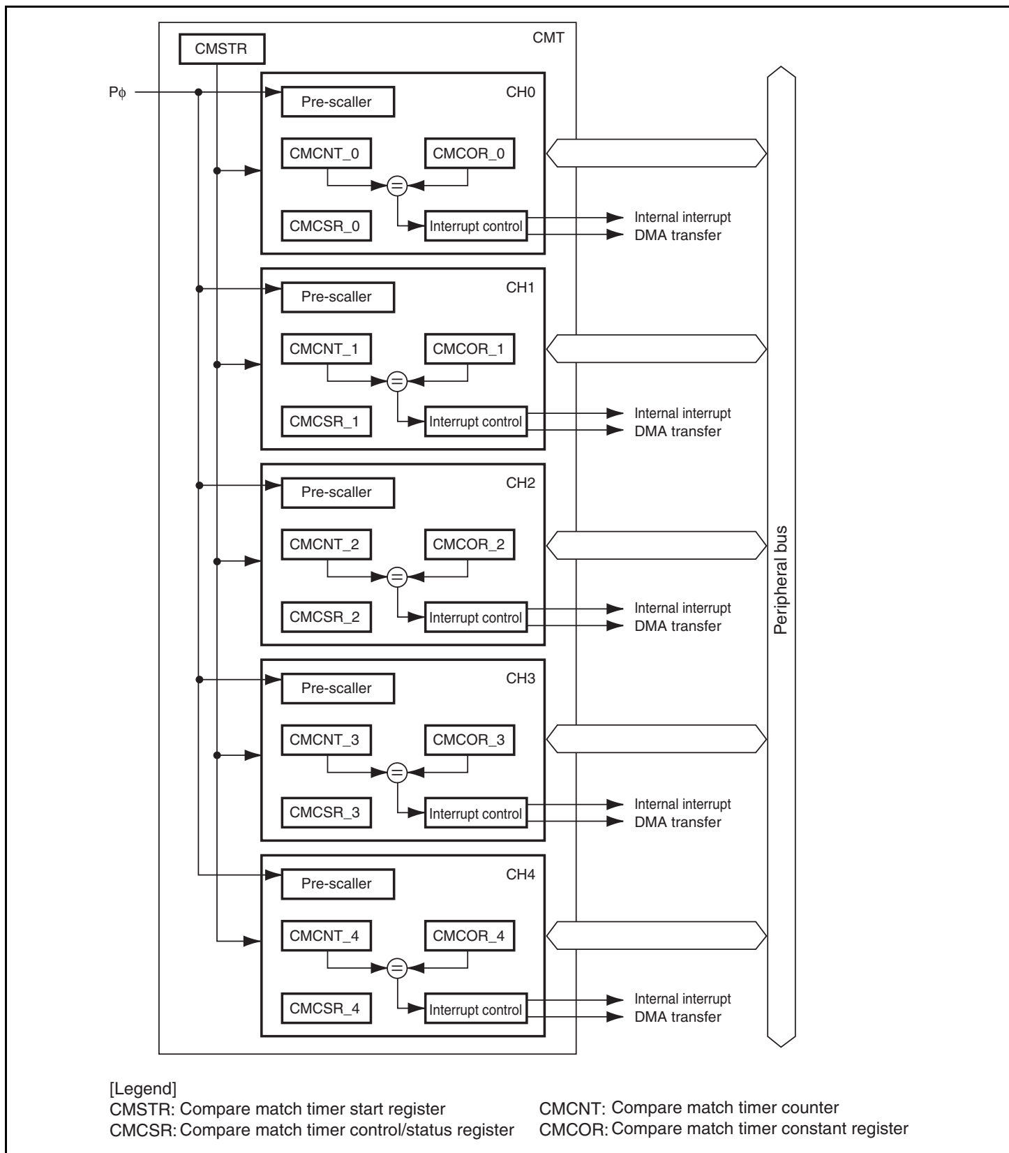
Figure 16.1 Block Diagram of CMT
