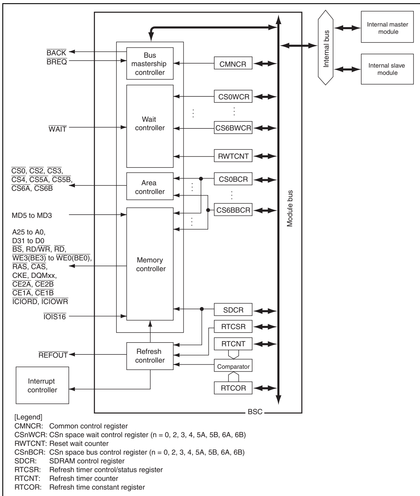
Figure 9.1 Block Diagram of BSC
