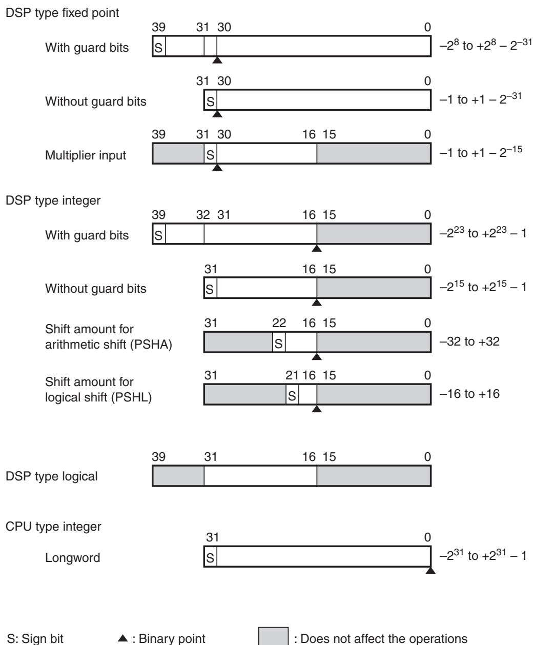
Figure 3.8 Data Formats
