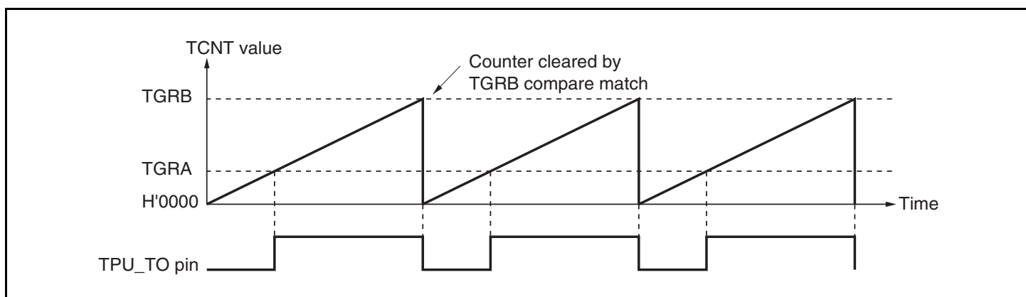
Figure 15.12 Example of PWM Mode Operation (1)
