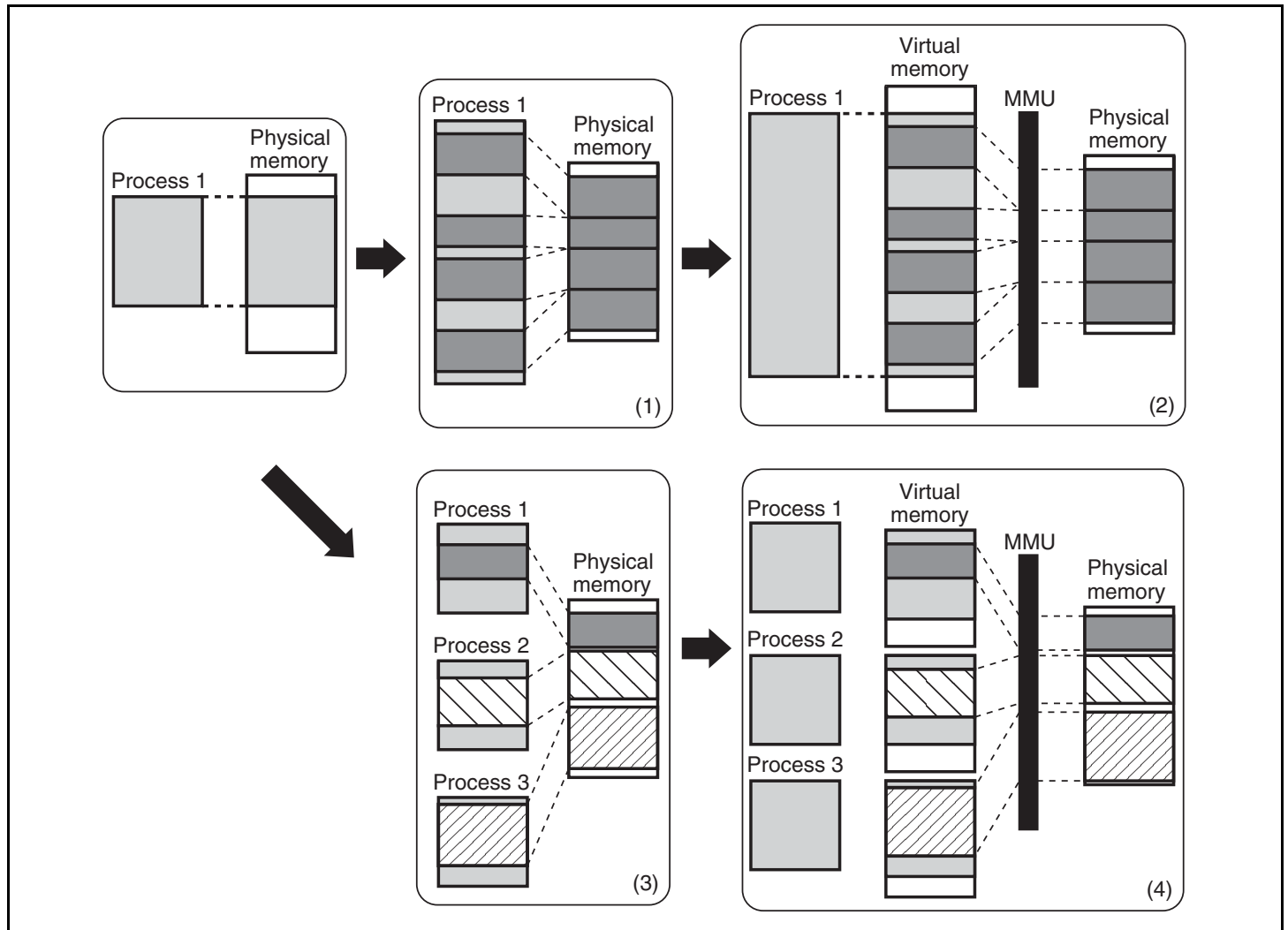
Figure 4.1 MMU Functions
