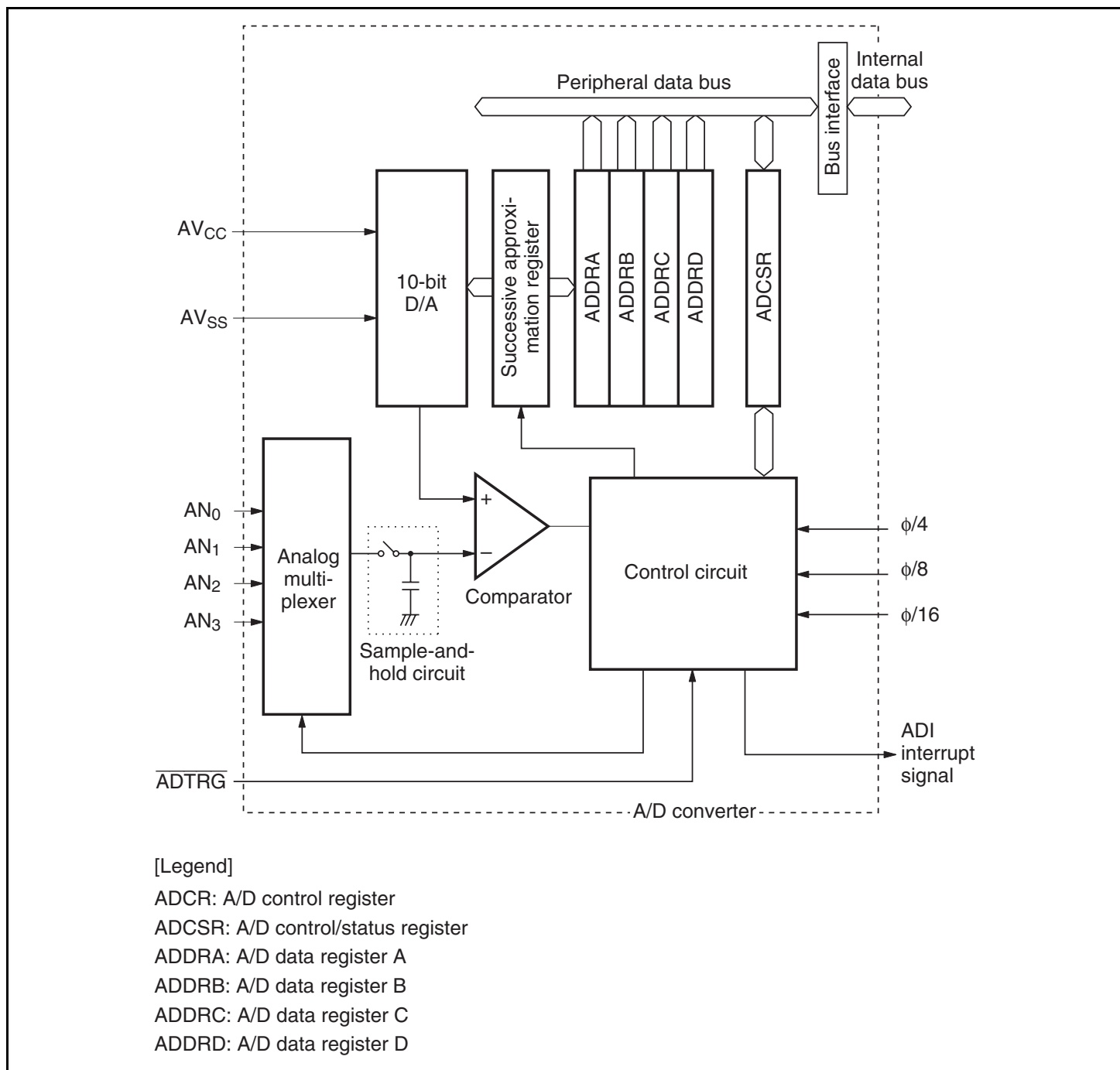
Figure 27.1 Block Diagram of A/D Converter
