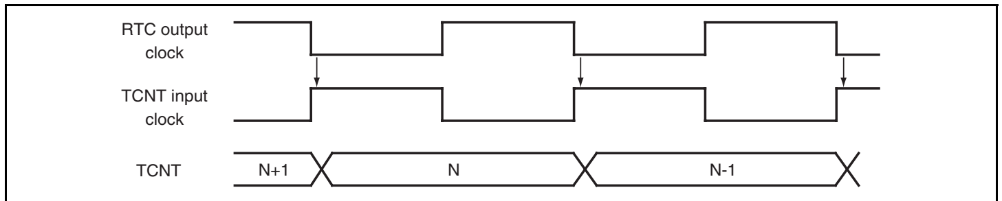
Figure 14.5 Count Timing when RTC Clock is Operating
