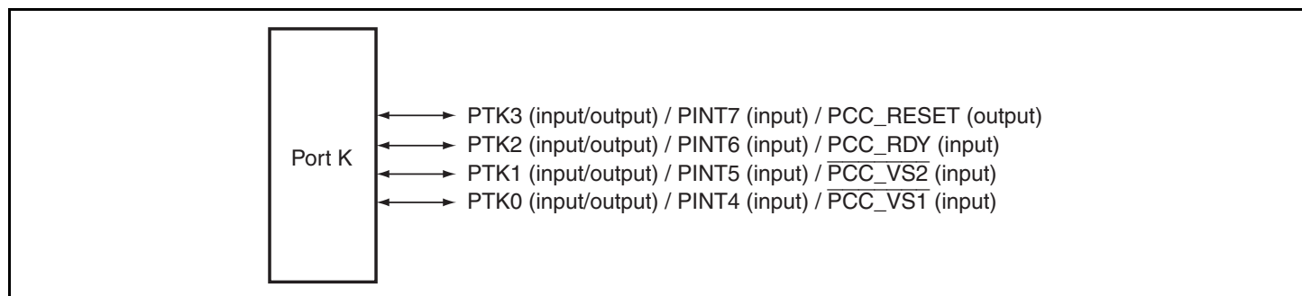
Figure 35.10 Port K
