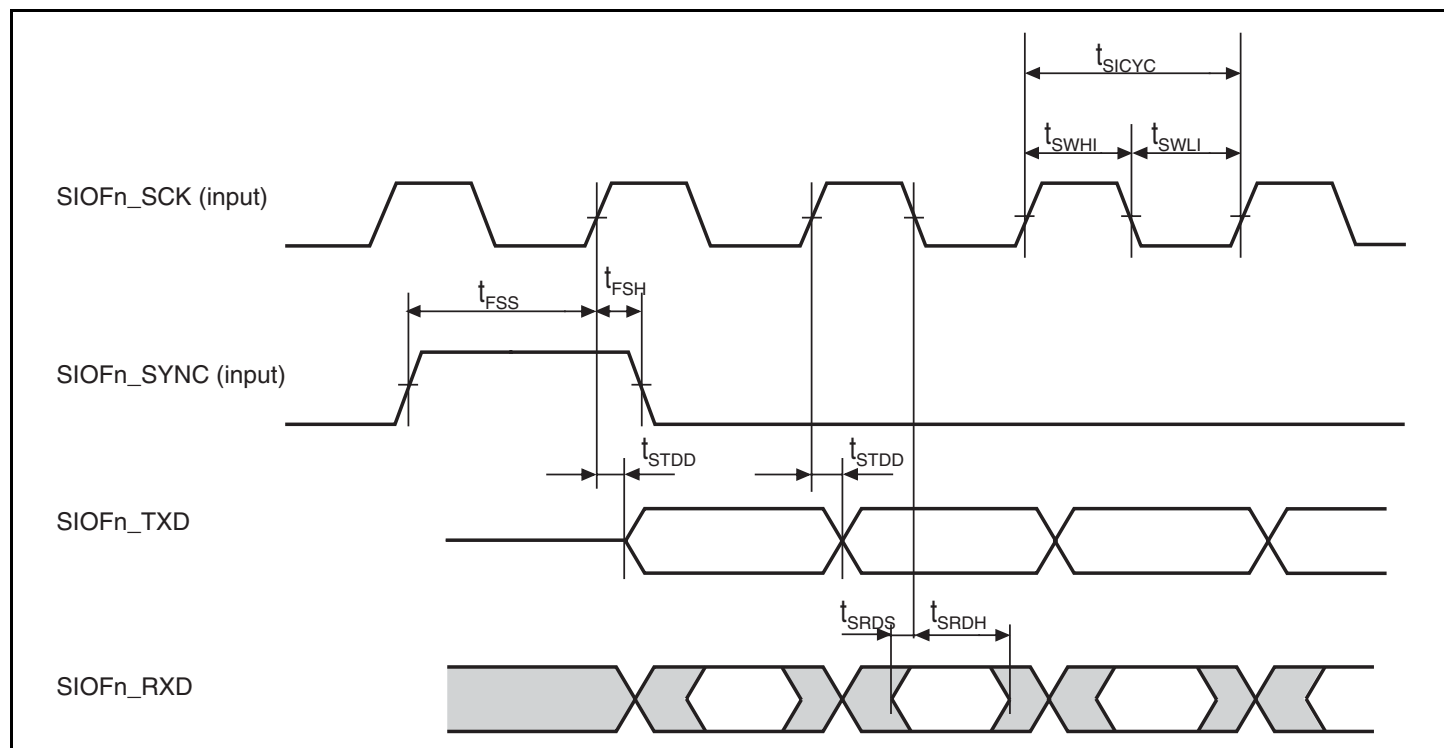
Figure 38.58 SIOF Transmission/Reception Timing (Slave Mode 1, Slave Mode 2)
