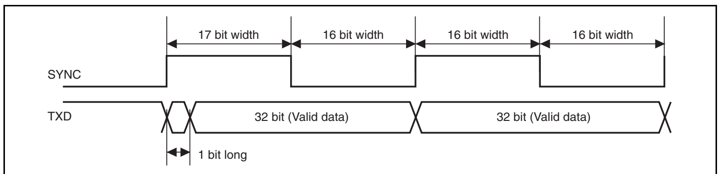
Figure 21.21 Frame Length (32-Bit)
