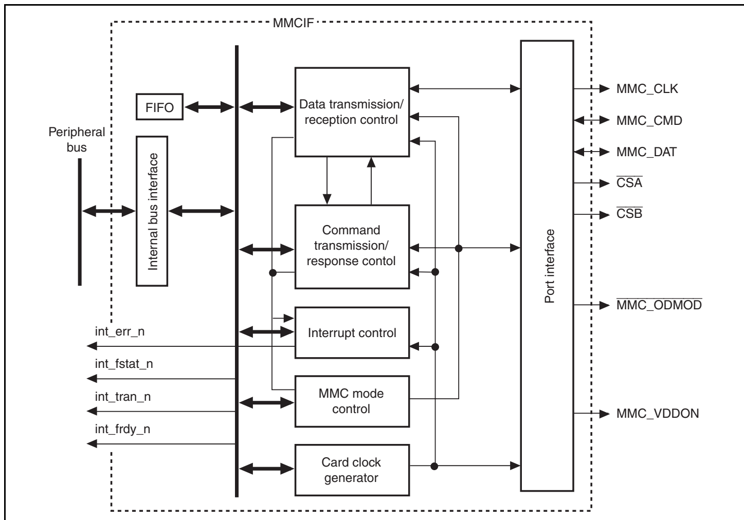
Figure 31.1 Block Diagram of MMCIF
