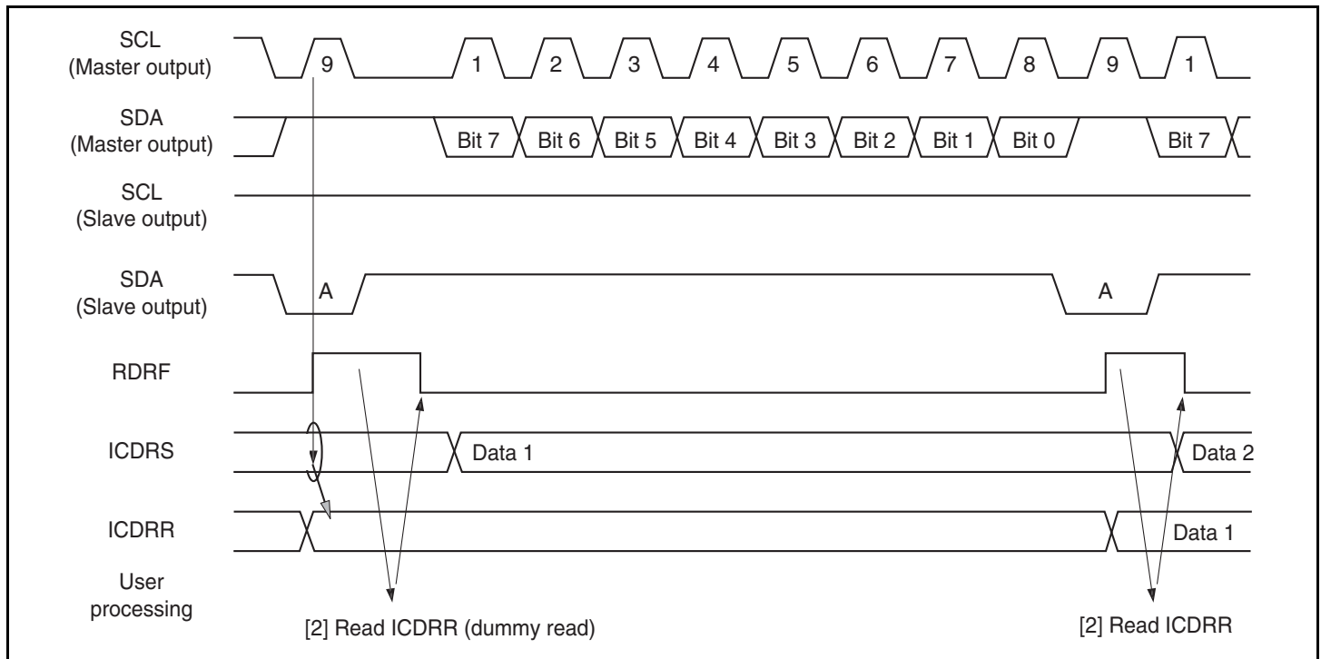
Figure 20.11 Slave Receive Mode Operation Timing (1)
