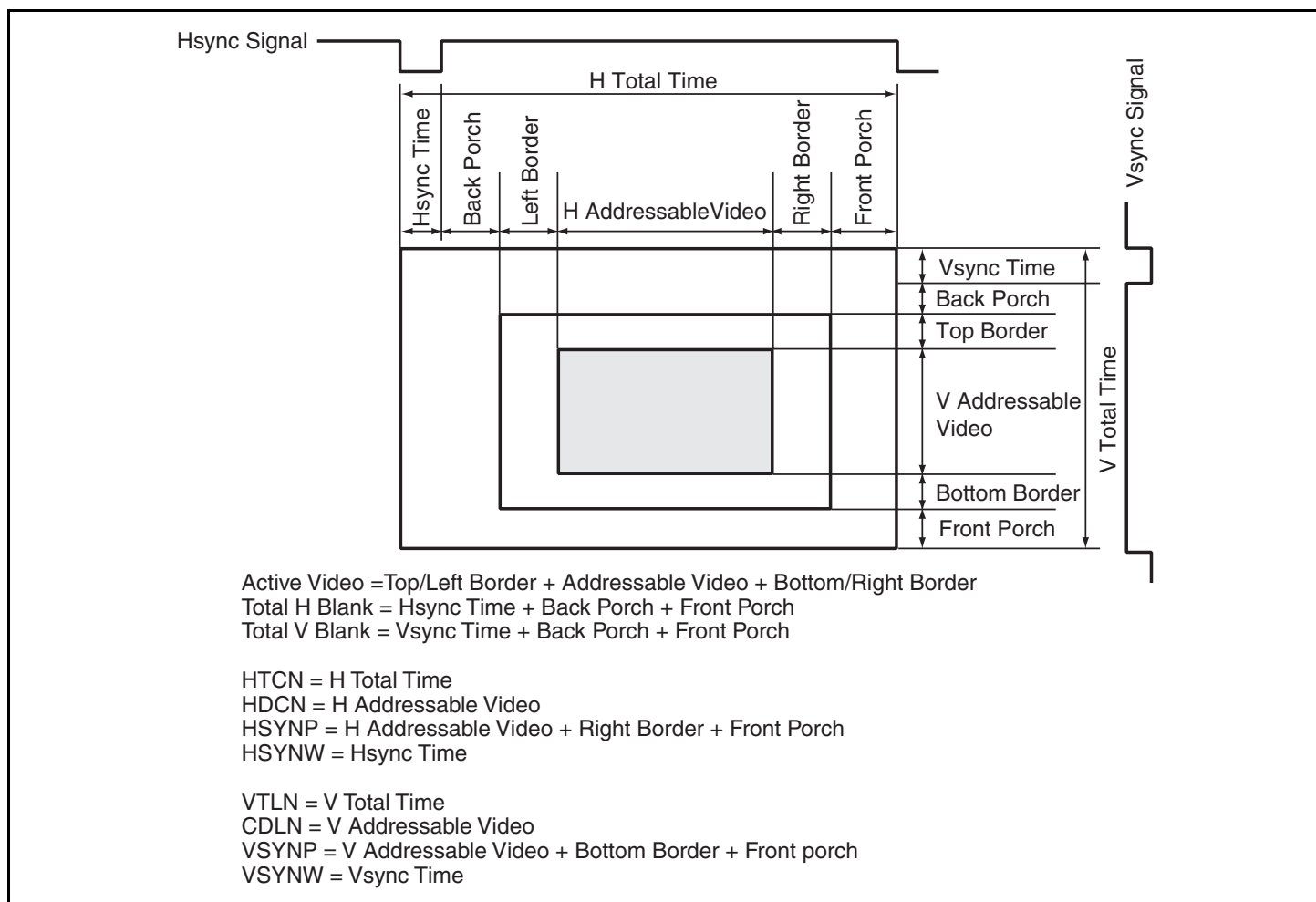
Figure 26.2 Valid Display and the Retrace Period
