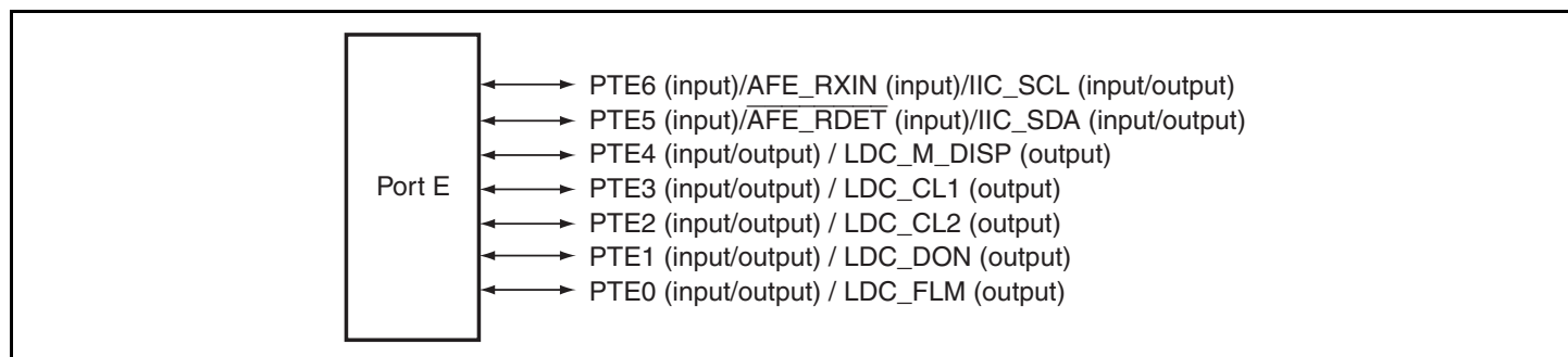
Figure 35.5 Port E
