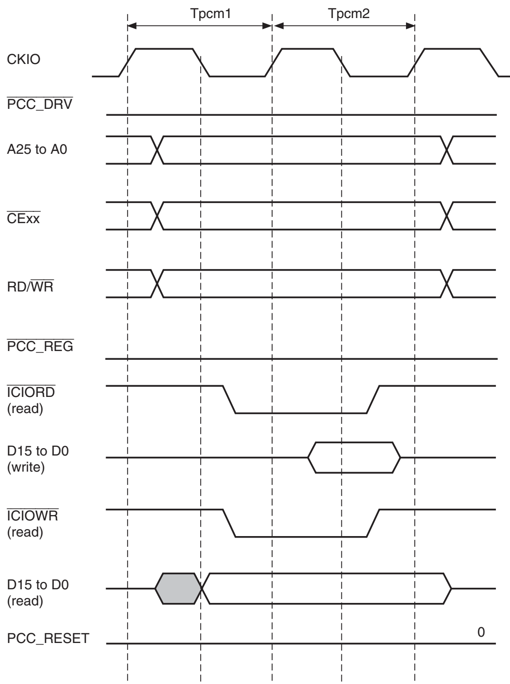
Figure 29.7 PCMCIA I/O Card Interface Basic Timing
