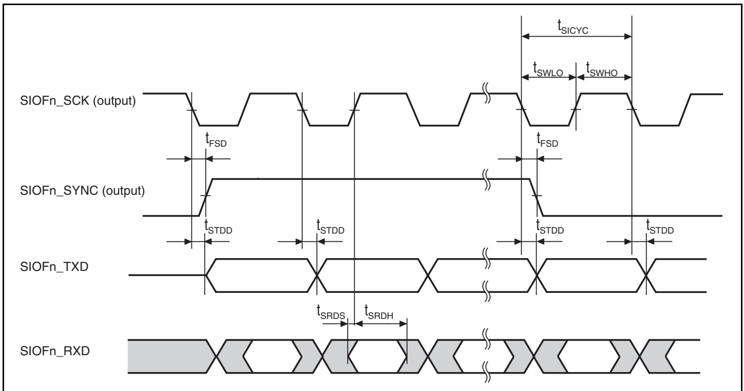
Figure 38.57 SIOF Transmission/Reception Timing (Master Mode 2, Rise Sampling)
