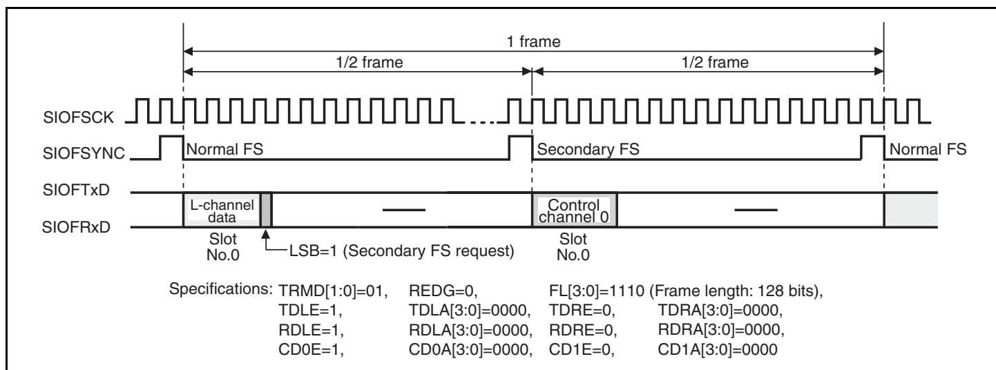
Figure 21.8 Control Data Interface (Secondary FS)
