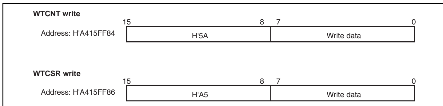
Figure 12.2 Writing to WTCNT and WTCSR
