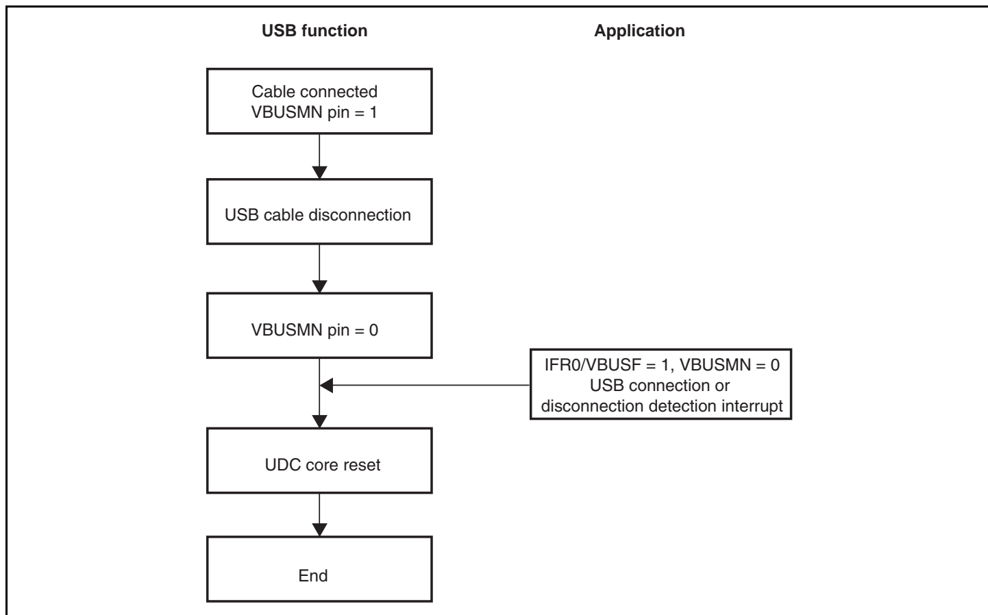
Figure 25.4 Cable Disconnection Operation
