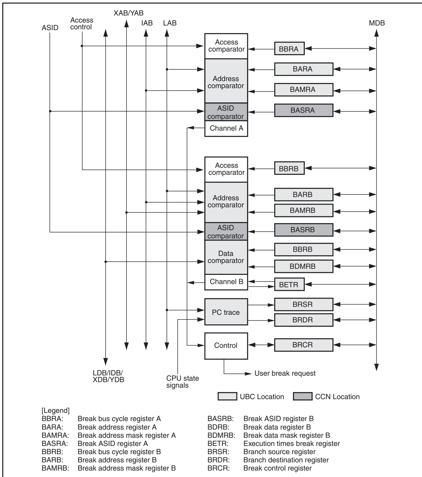
Figure 33.1 Block Diagram of UBC
