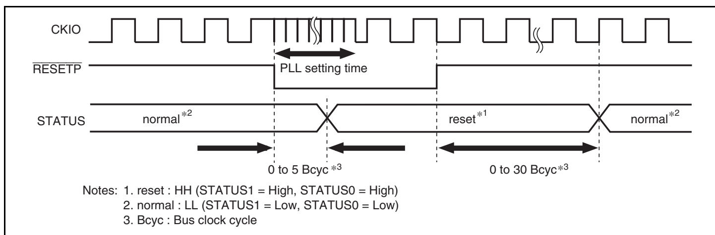
Figure 13.2 STATUS Output at Power-on Reset
