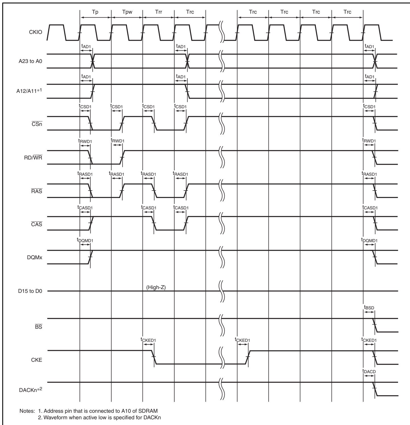
Figure 38.35 Self Refresh Timing of SDRAM (TRP = 2 Cycles)
