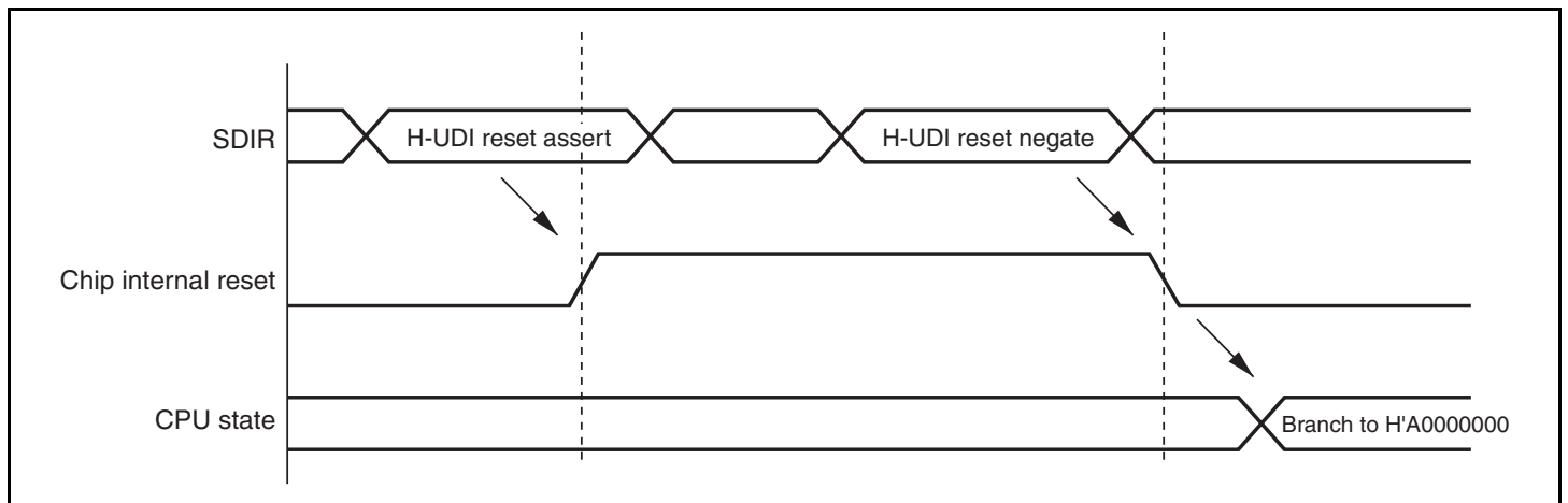
Figure 36.4 H-UDI Reset
