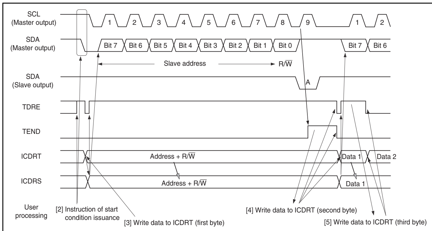
Figure 20.5 Master Transmit Mode Operation Timing (1)
