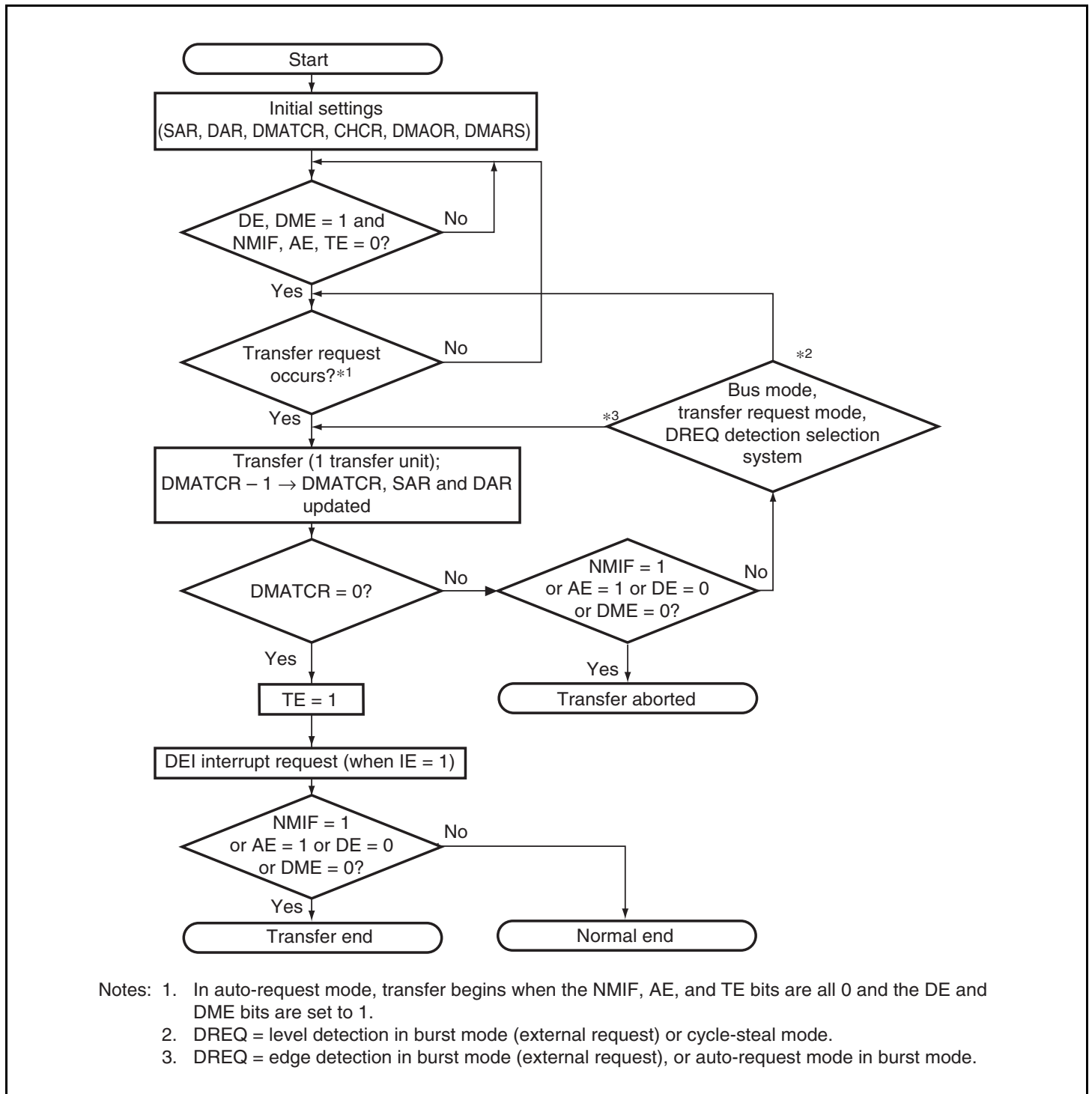
Figure 10.2 DMA Transfer Flowchart
