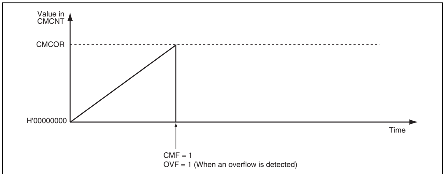
Figure 16.2 Counter Operation (One-Shot Operation)
