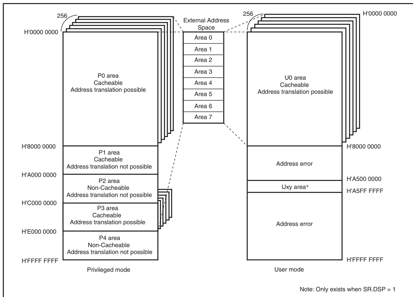
Figure 4.2 Virtual Address Space (MMUCR.AT = 1)
