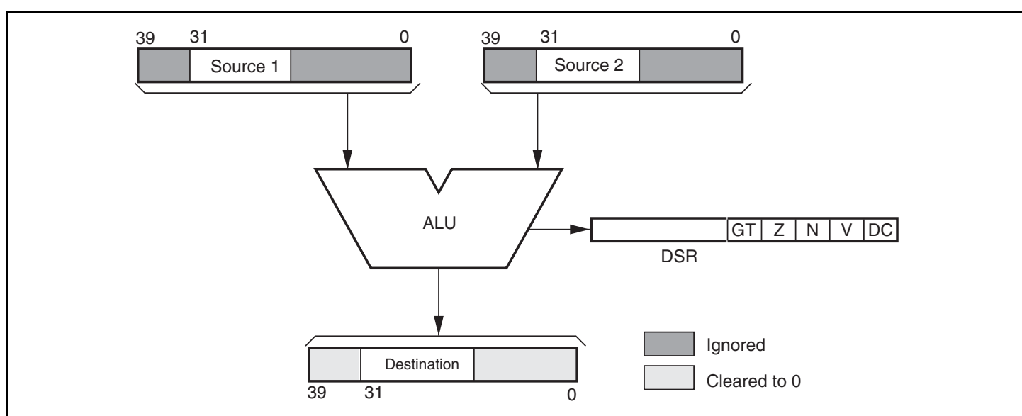
Figure 3.15 ALU Logical Operation Flow
