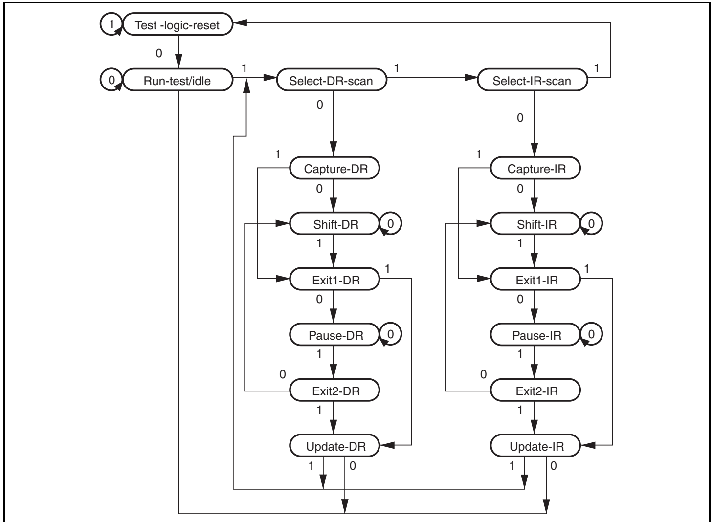
Figure 36.2 TAP Controller State Transitions
