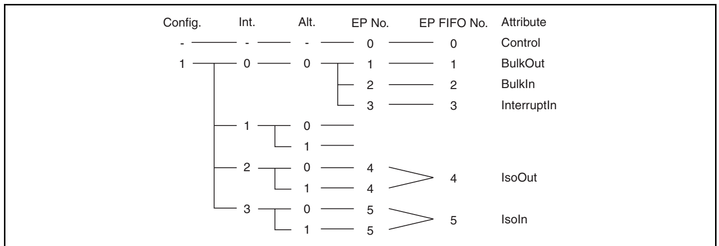
Figure 25.2 Example of Endpoint Configuration
