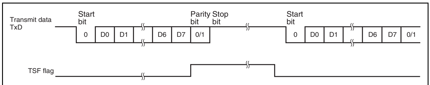
Figure 18.5 Example of Transmit Data Stop Function
