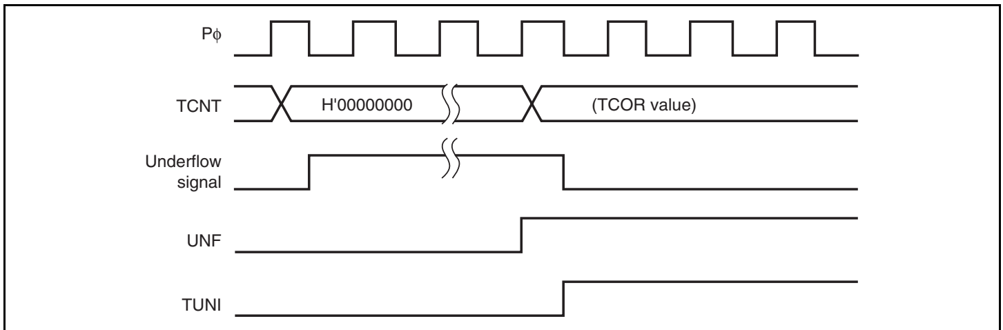
Figure 14.6 UNF Set Timing
