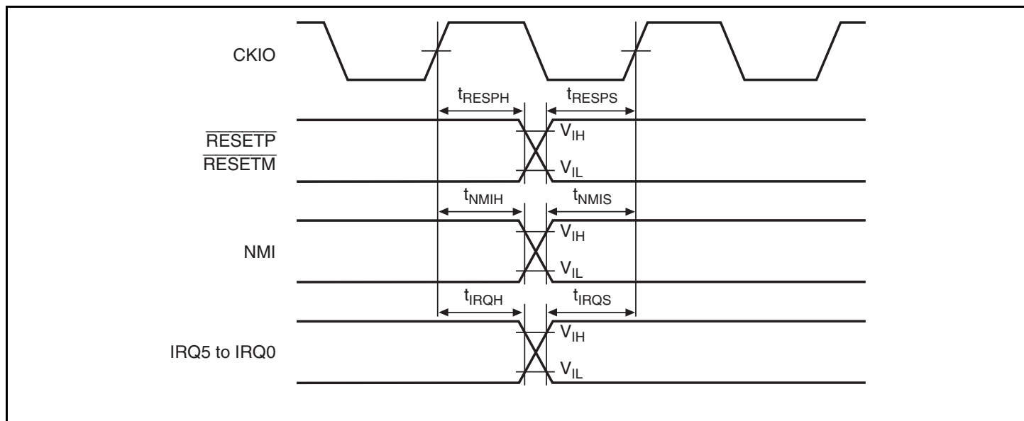
Figure 38.9 Interrupt Signal Input Timing
