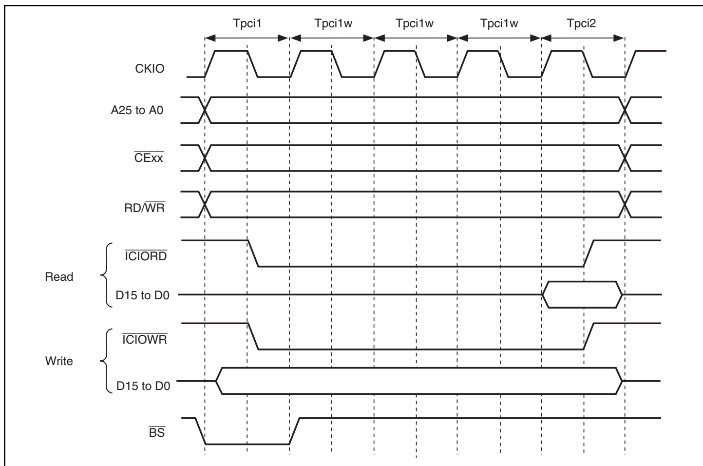
Figure 9.41 Basic Timing for PCMCIA I/O Card Interface
