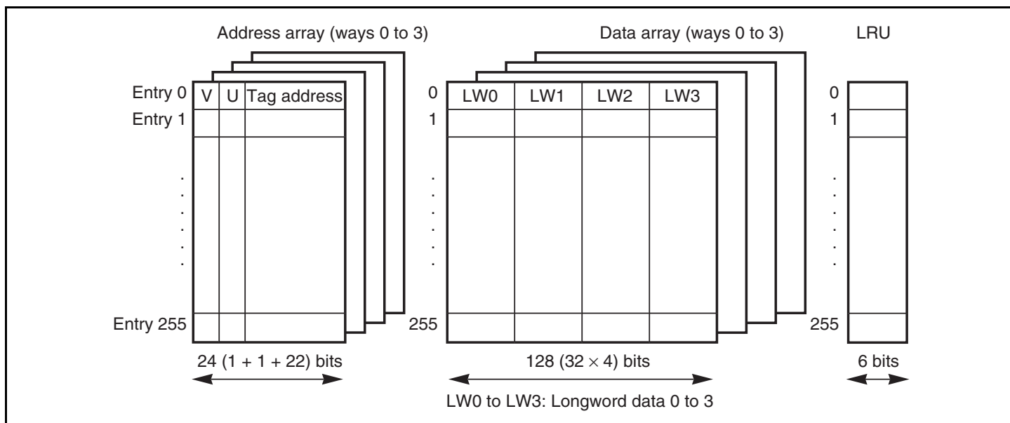
Figure 5.1 Cache Structure
