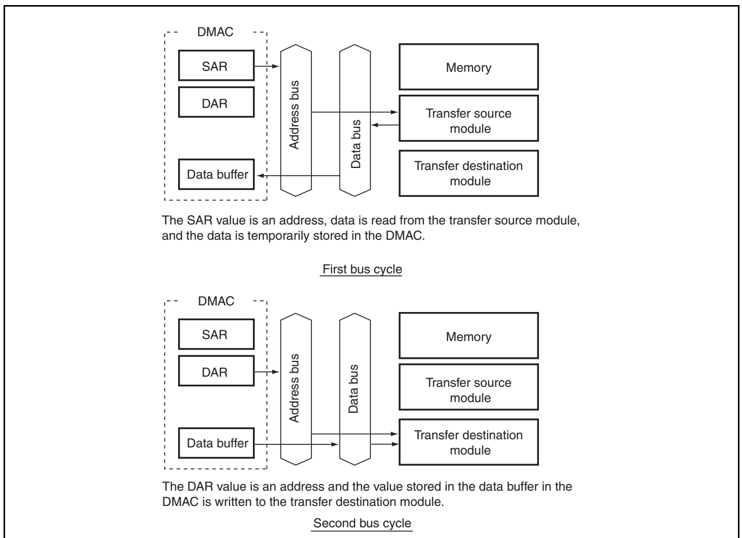
Figure 10.5 Data Flow of Dual Address Mode
