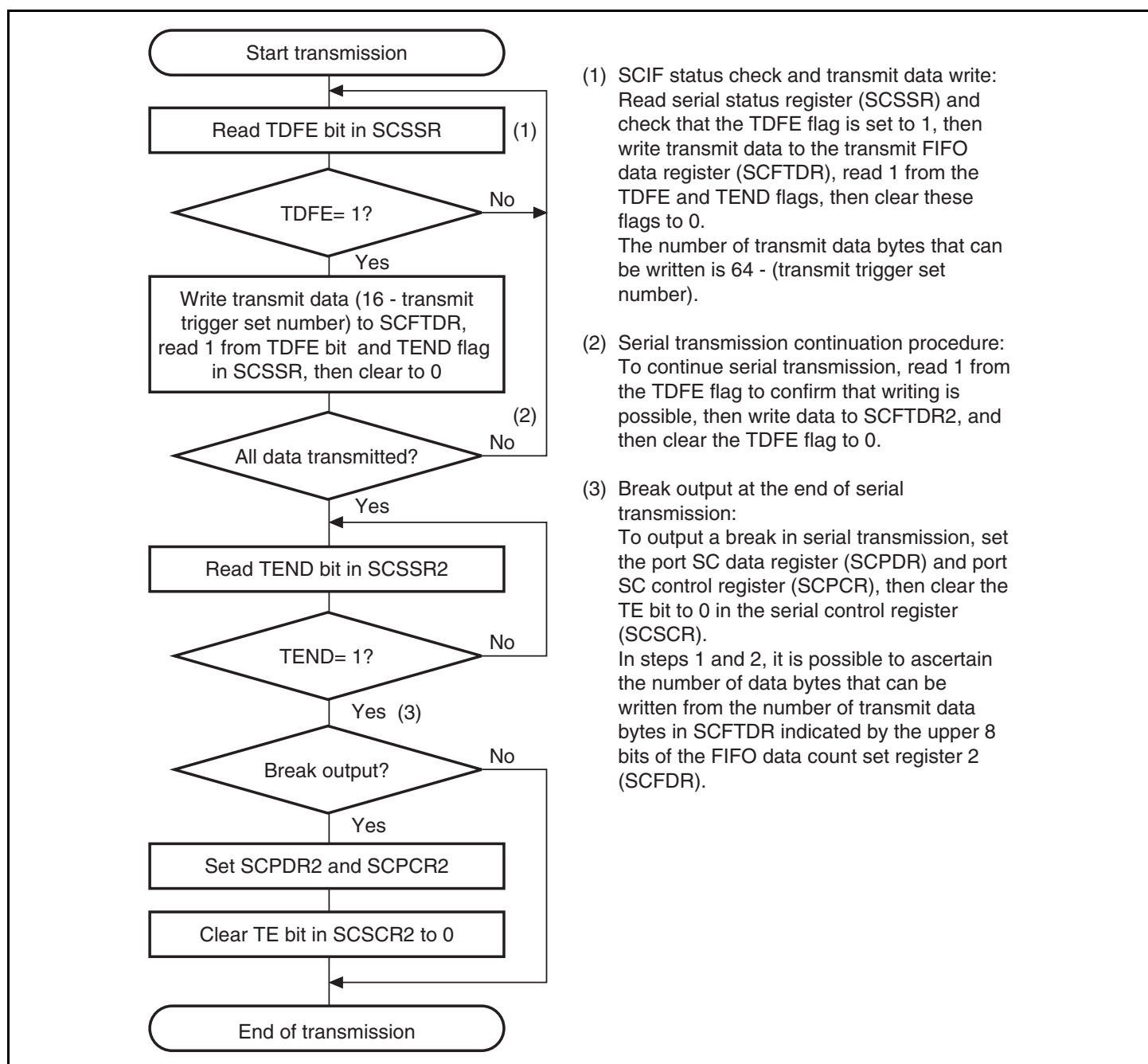
Figure 18.3 Sample Serial Transmission Flowchart
