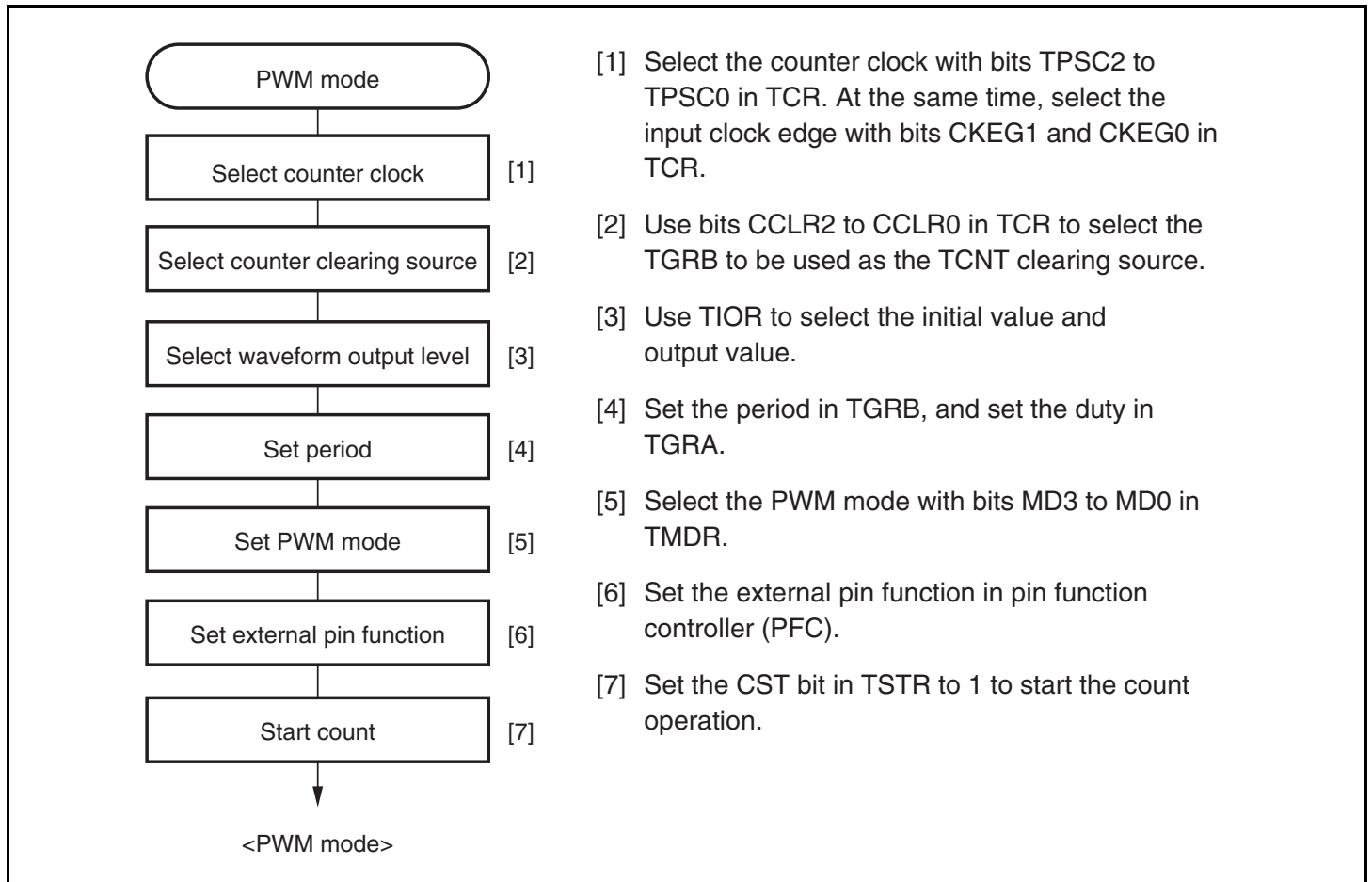
Figure 15.11 Example of PWM Mode Setting Procedure
