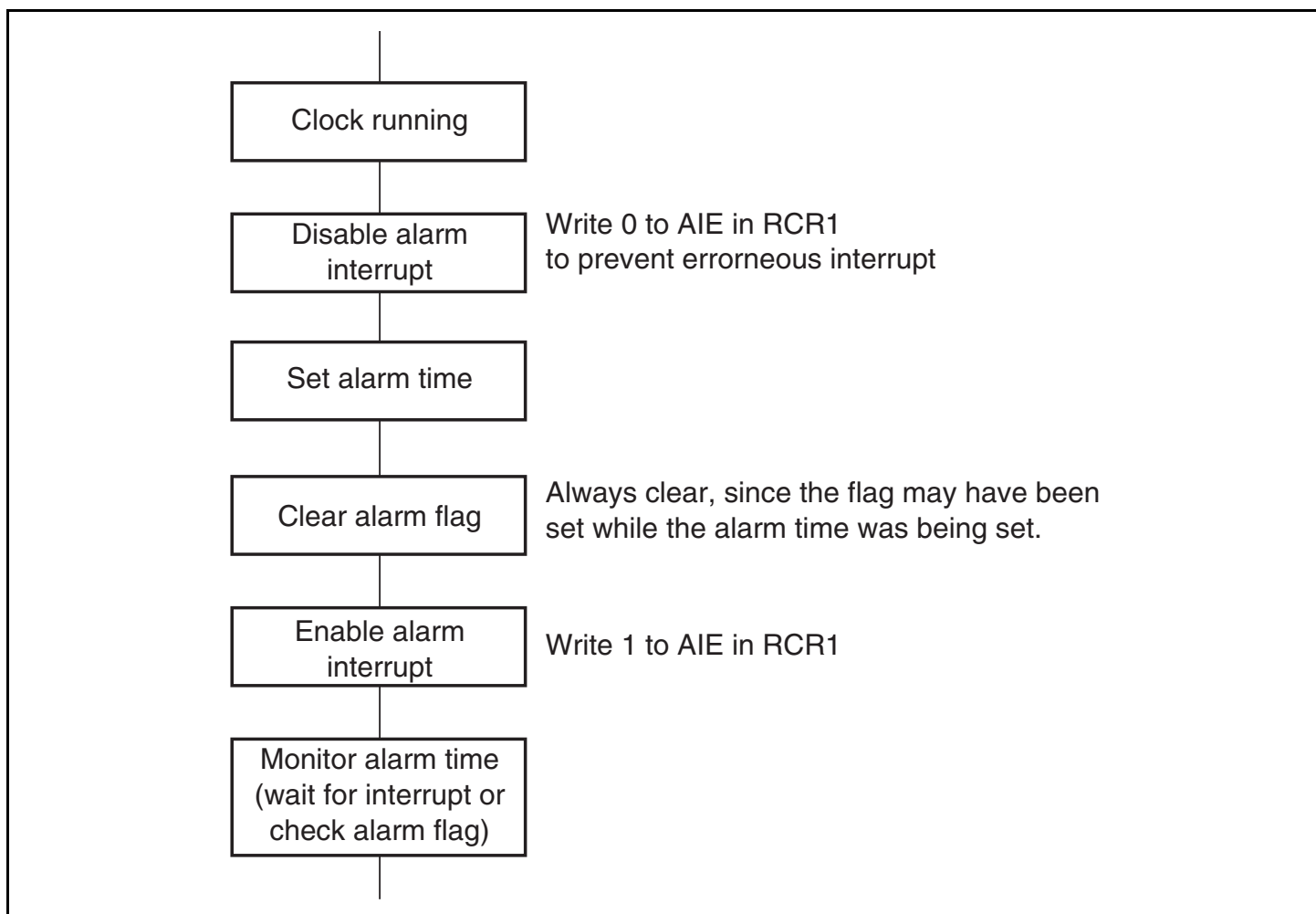
Figure 17.4 Using Alarm Function
