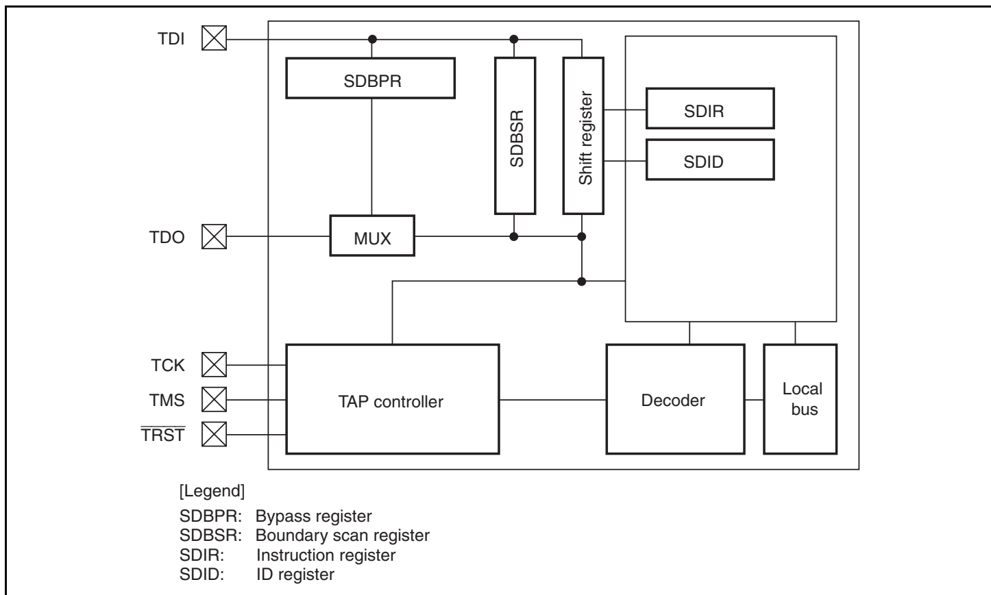
Figure 36.1 Block Diagram of H-UDI
