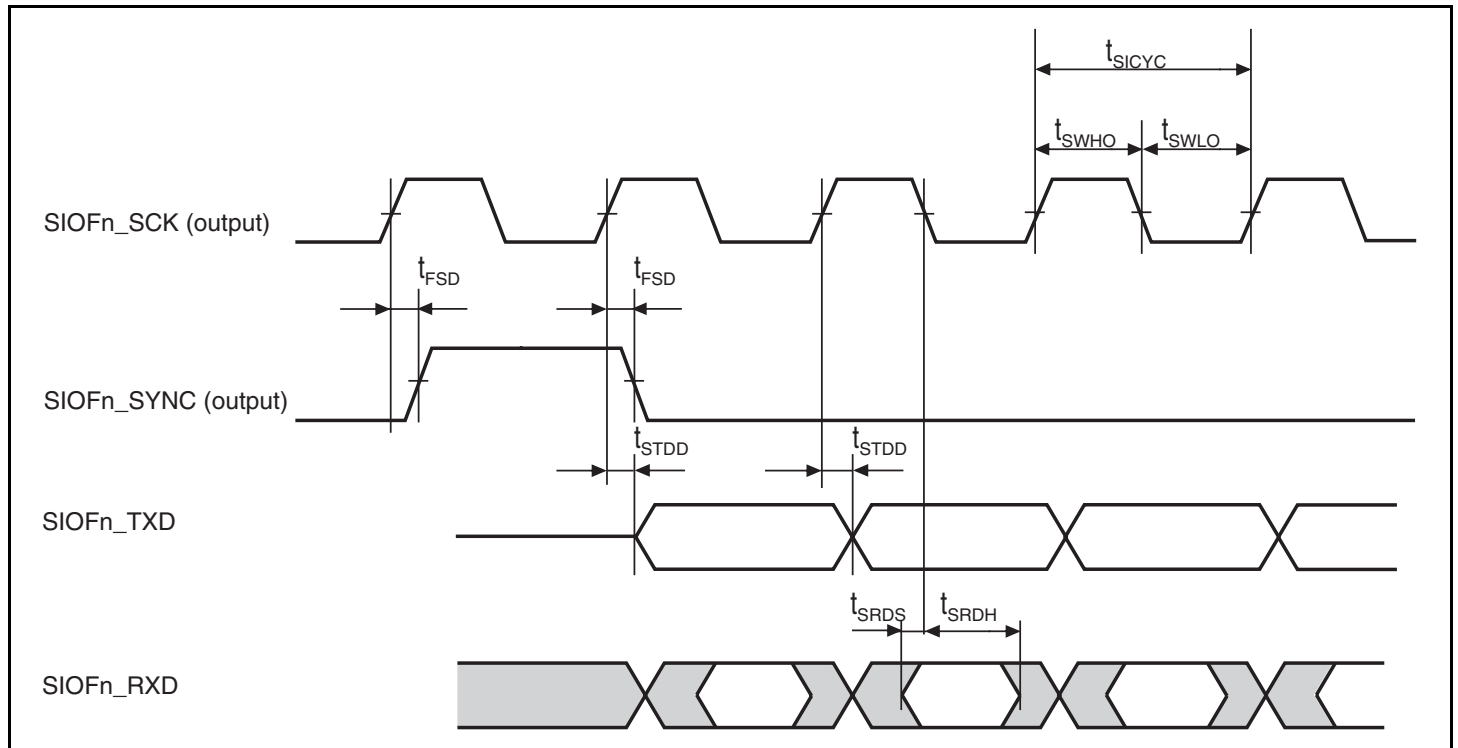
Figure 38.54 SIOF Transmission/Reception Timing (Master Mode 1, Fall Sampling)
