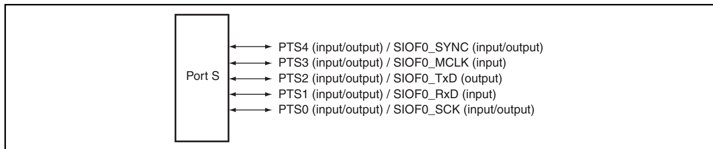
Figure 35.15 Port S
