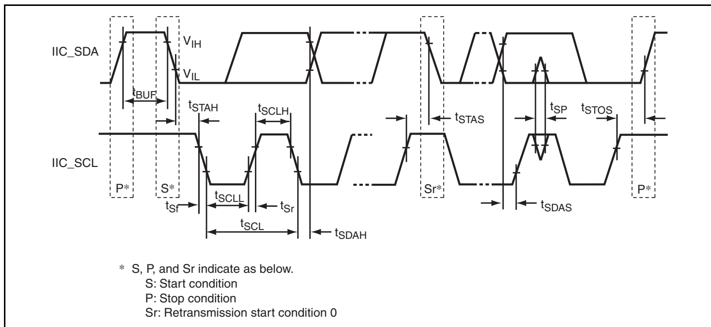
Figure 38.52 I 2 C Bus Interface Input/Output Timing
