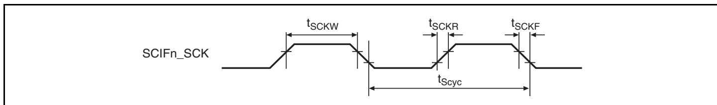
Figure 38.50 SCK Input Clock Timing
