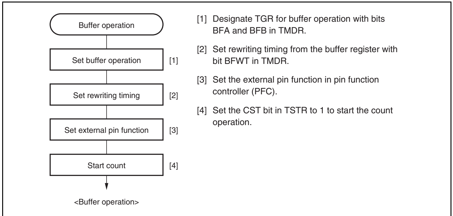
Figure 15.9 Example of Buffer Operation Setting Procedure
