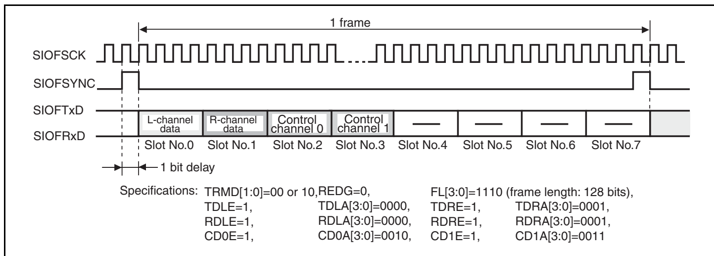
Figure 21.18 Transmit and Receive Timing (16-Bit Stereo Data (3))
