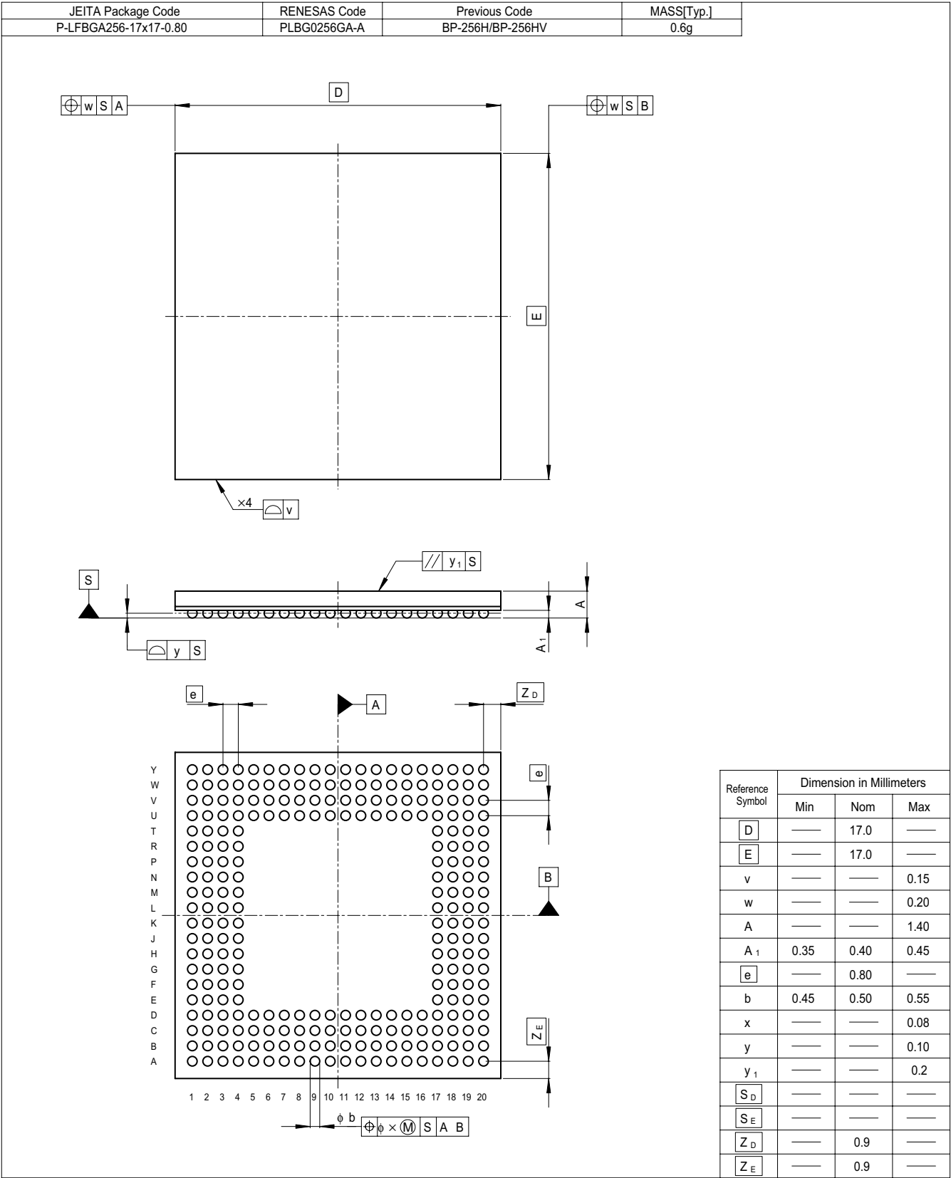
Figure C.1 Package Dimensions (PLBG0256GA-A (BP-256H/HV))
