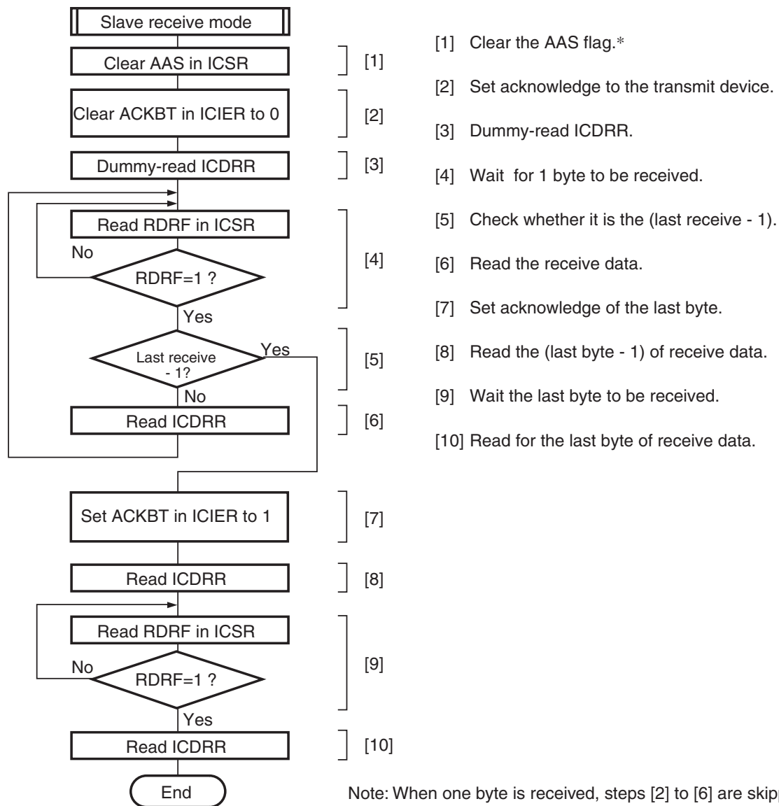
Figure 20.17 Sample Flowchart for Slave Receive Mode
