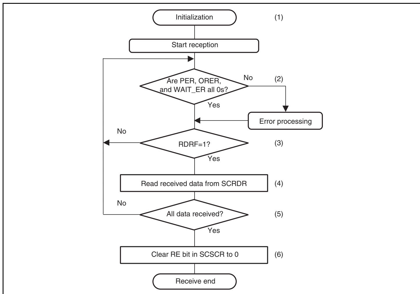
Figure 30.6 Example of Receive Processing
