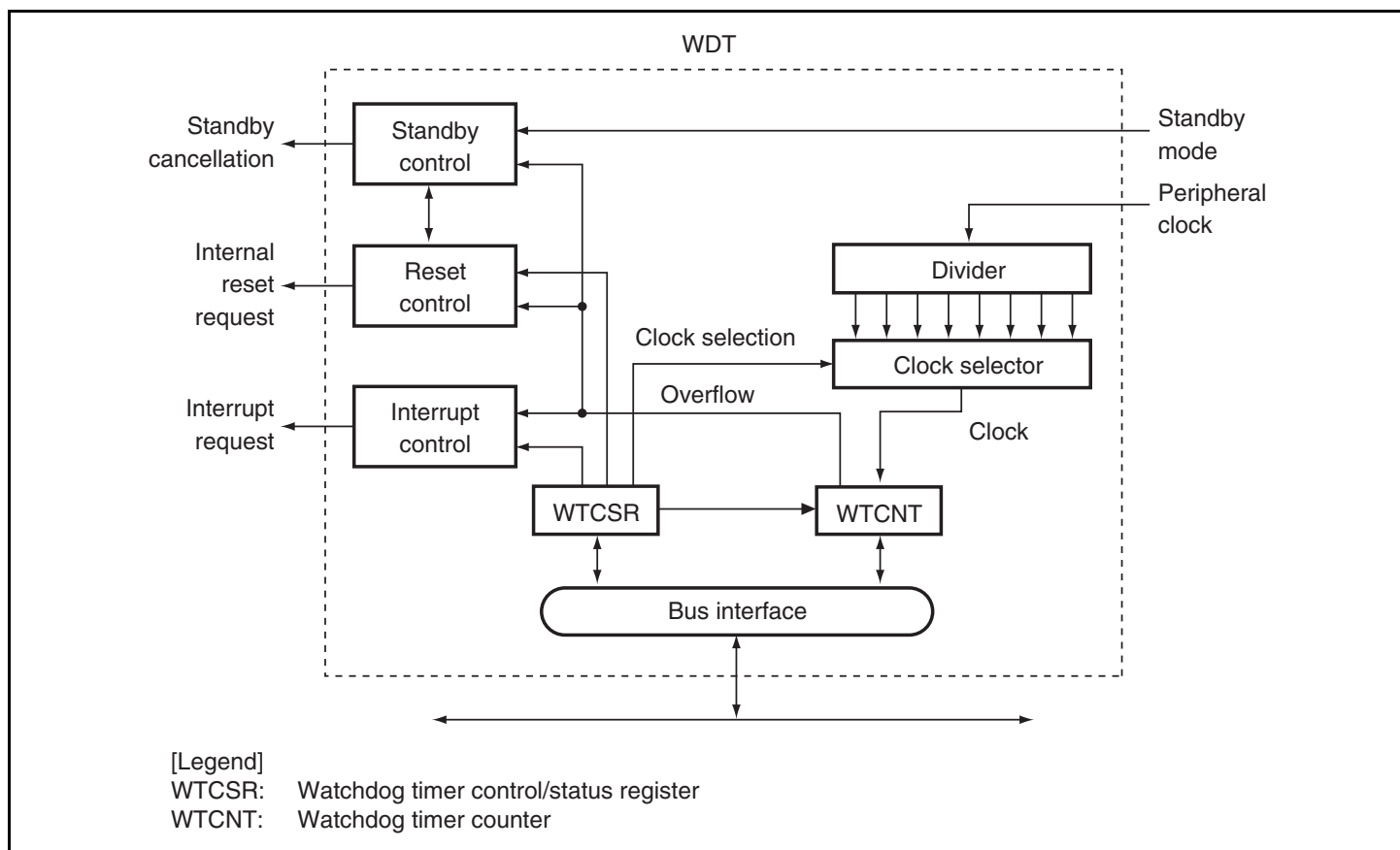
Figure 12.1 Block Diagram of WDT
