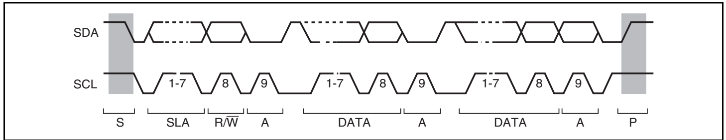
Figure 20.4 I 2 C Bus Timing
