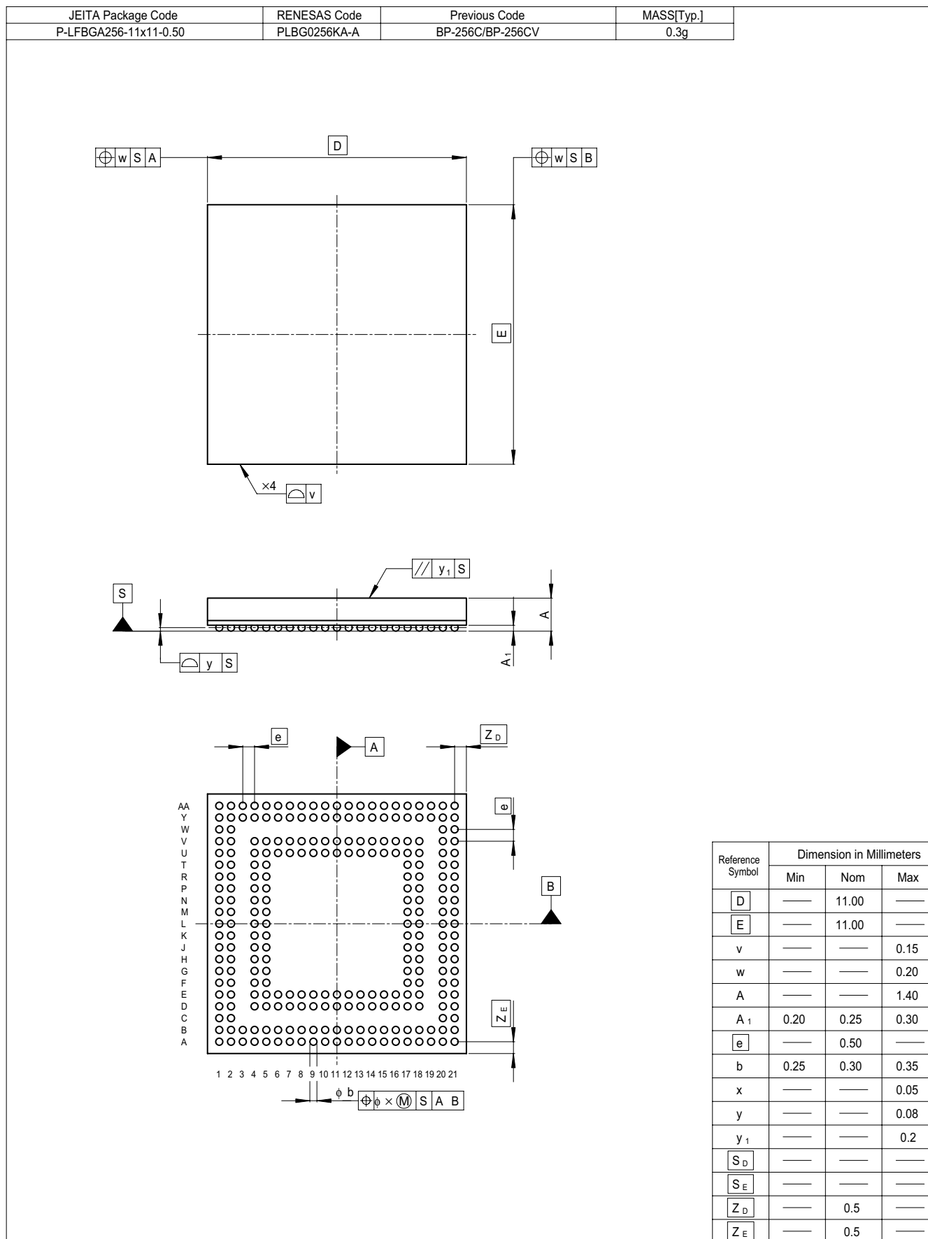
Figure C.2 Package Dimensions (PLBG0256KA-A (BP-256C/CV))
