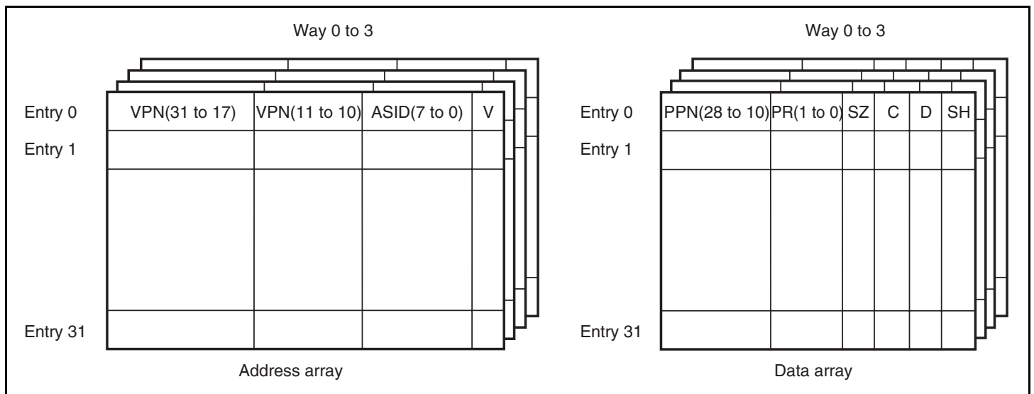
Figure 4.6 Overall Configuration of the TLB
