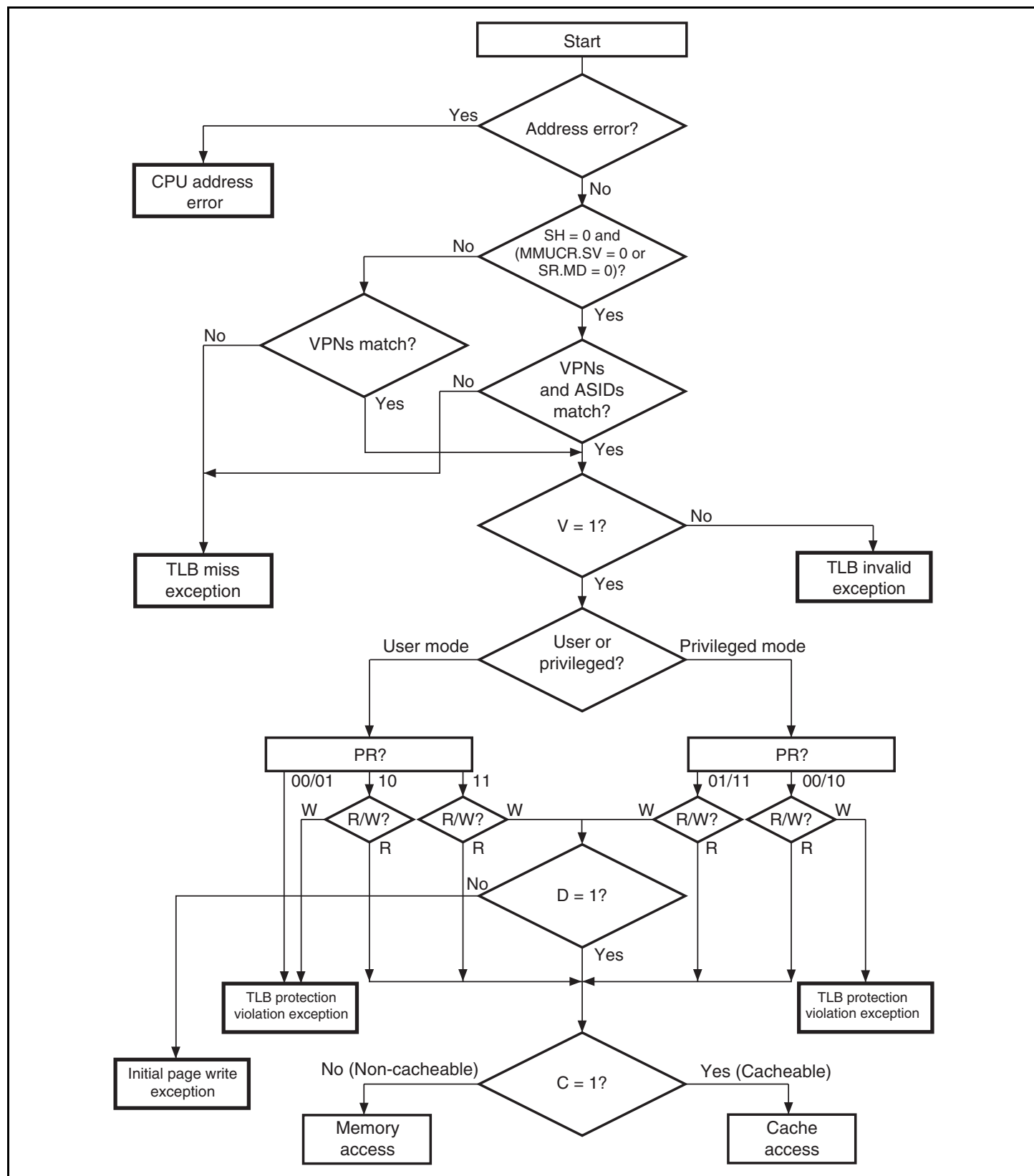
Figure 4.13 MMU Exception Generation Flowchart
