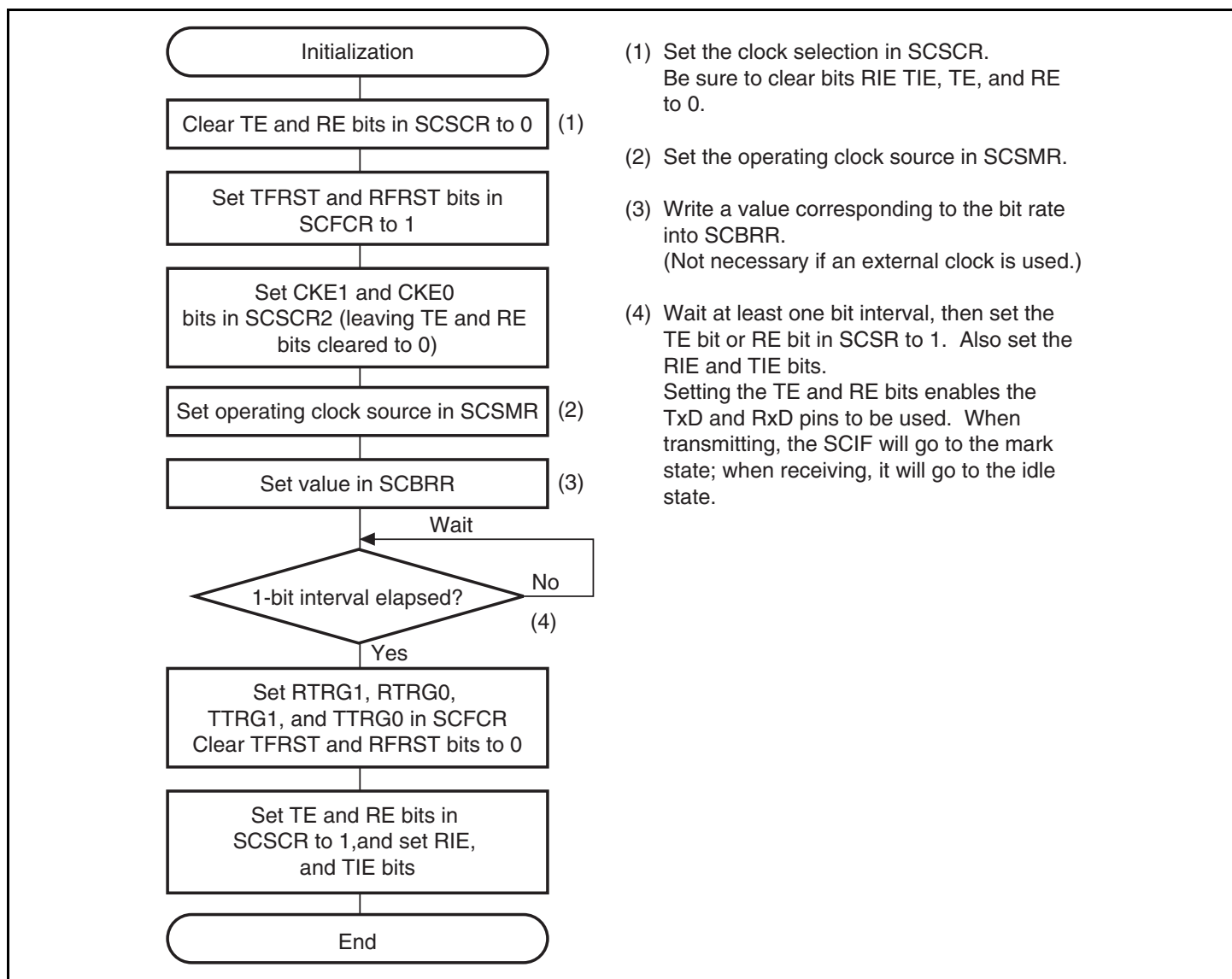
Figure 18.2 Sample SCIF Initialization Flowchart
