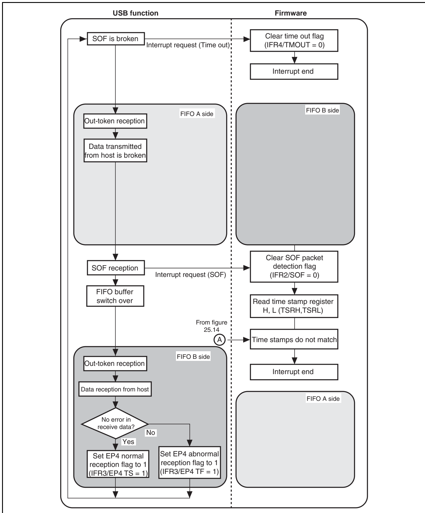
Figure 25.15 EP4 Isochronous-Out Transfer Operation (SOF is Broken)
