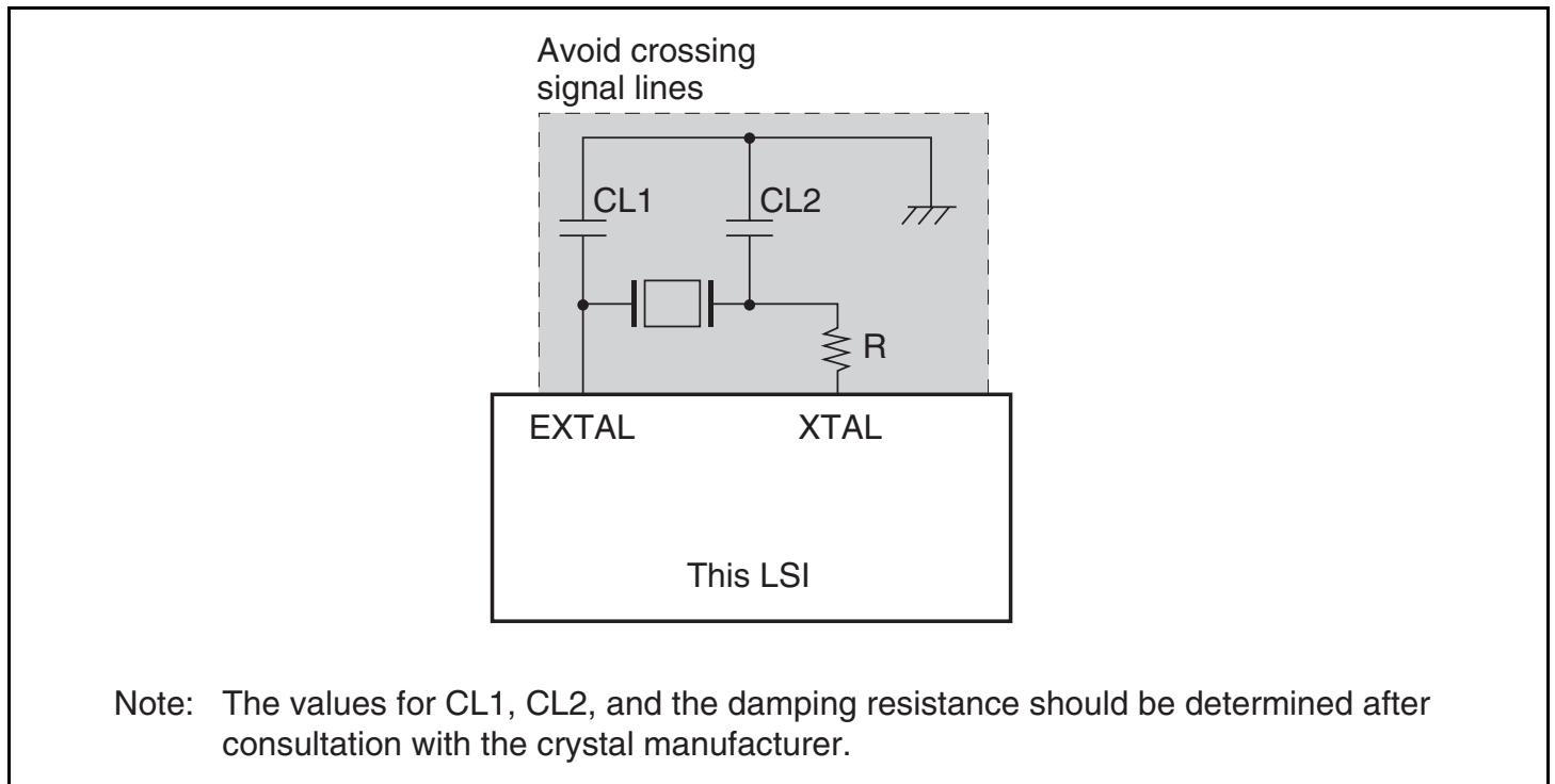
Figure 11.2 Points for Attention when Using Crystal Resonator
