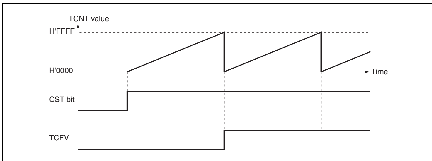
Figure 15.3 Free-Running Counter Operation
