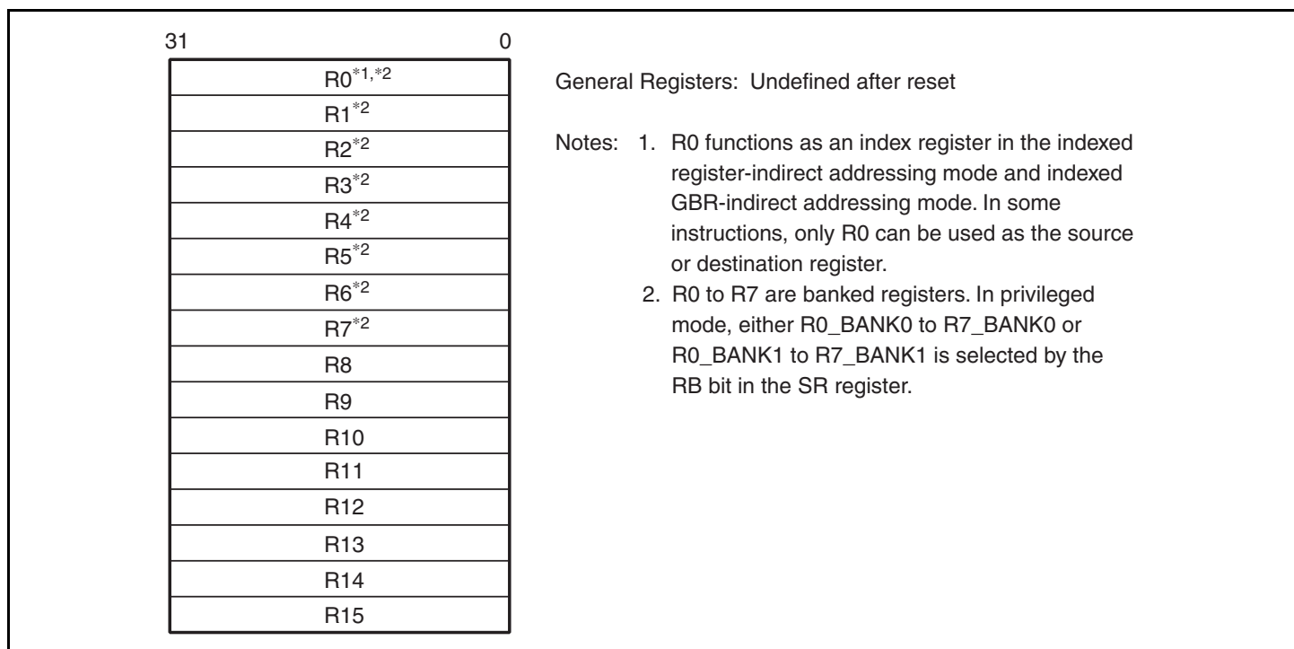
Figure 2.4 General Registers
