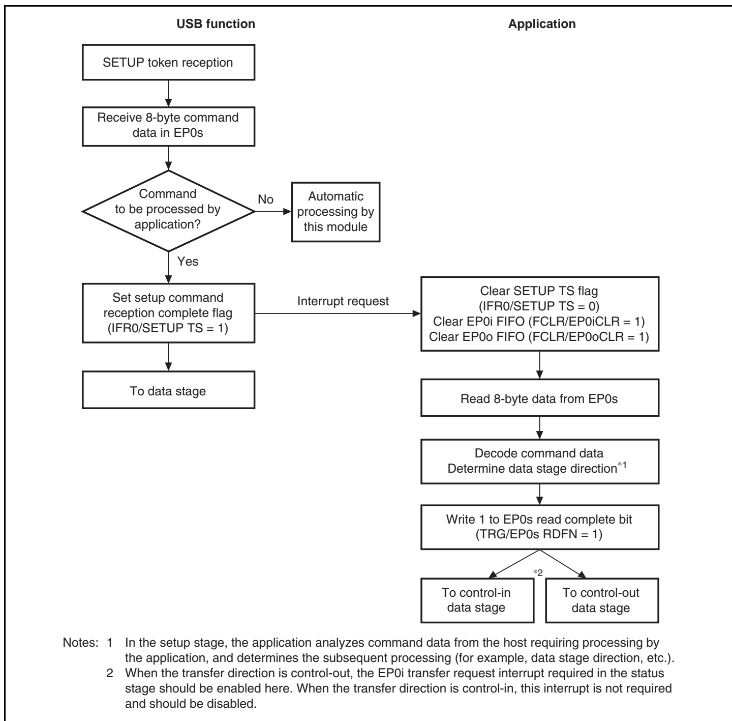
Figure 25.6 Setup Stage Operation
