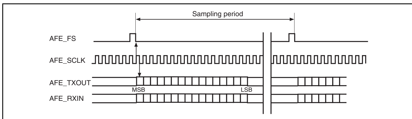
Figure 22.5 AFE Serial Interface
