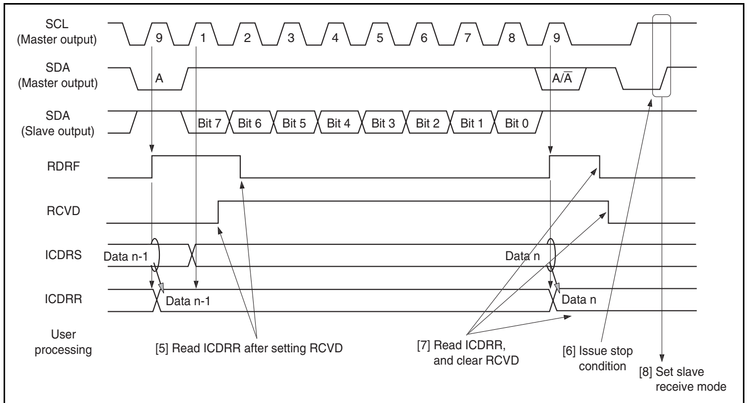
Figure 20.8 Master Receive Mode Operation Timing (2)
