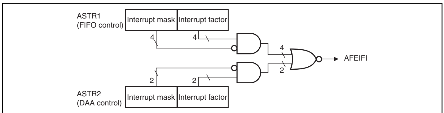
Figure 22.4 Interrupt Generator
