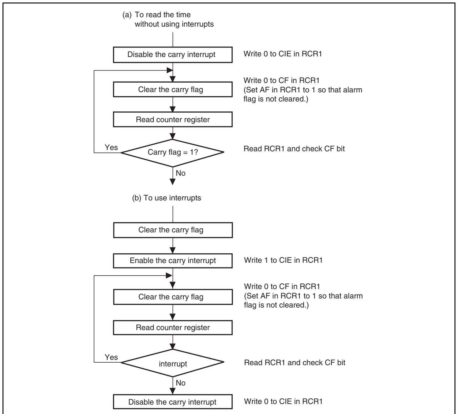
Figure 17.3 Reading Time
