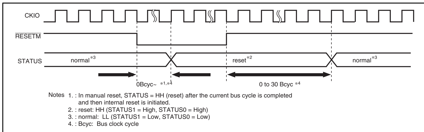
Figure 13.3 STATUS Output at Manual Reset
