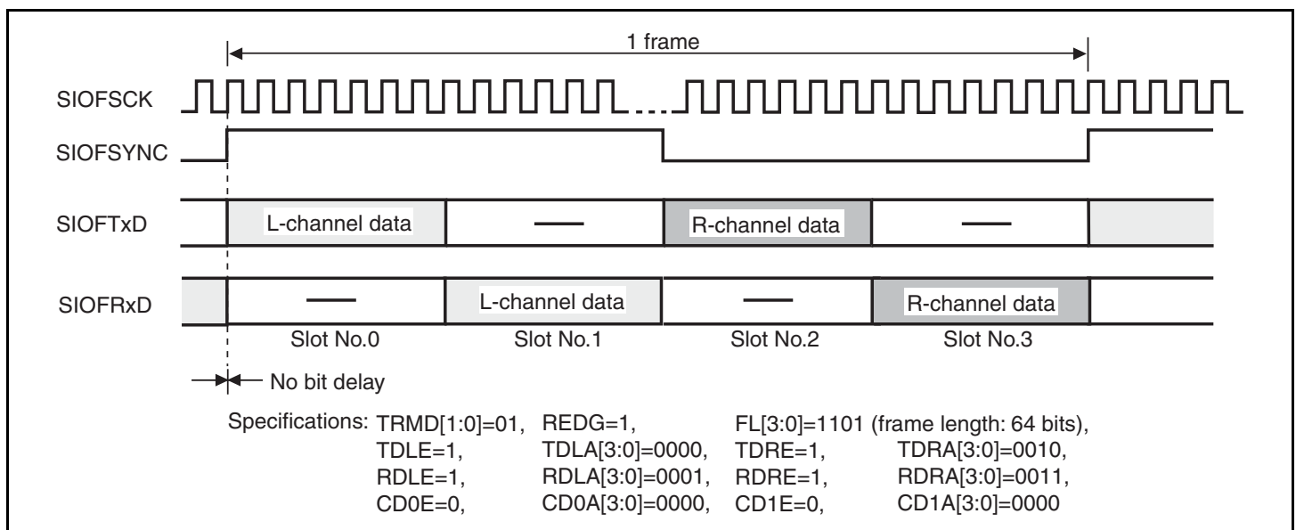
Figure 21.17 Transmit and Receive Timing (16-Bit Stereo Data (2))
