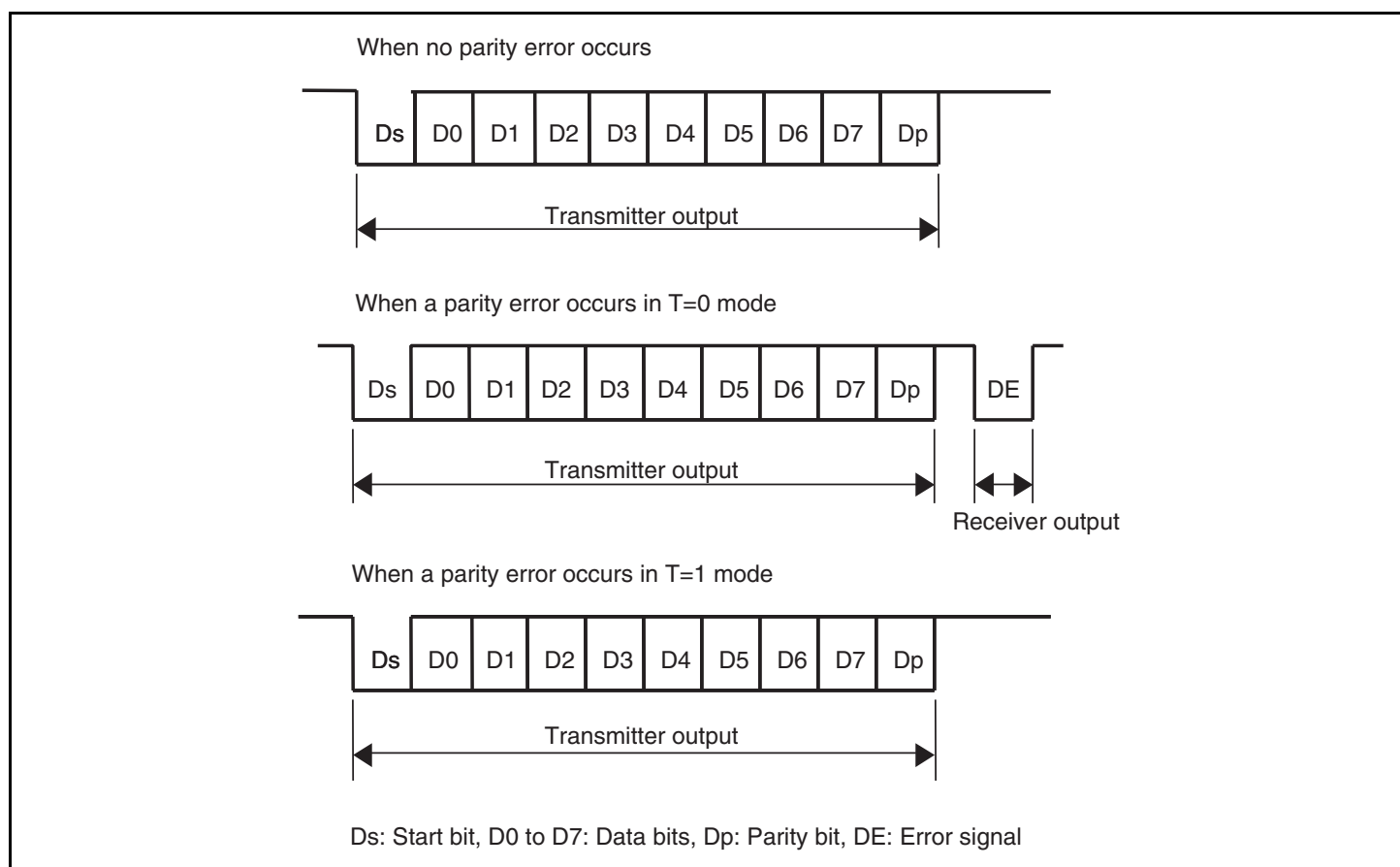
Figure 30.2 Data Format Used by Smart Card Interface
