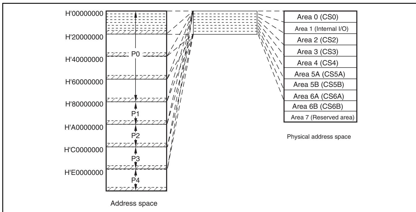
Figure 9.2 Address Space
