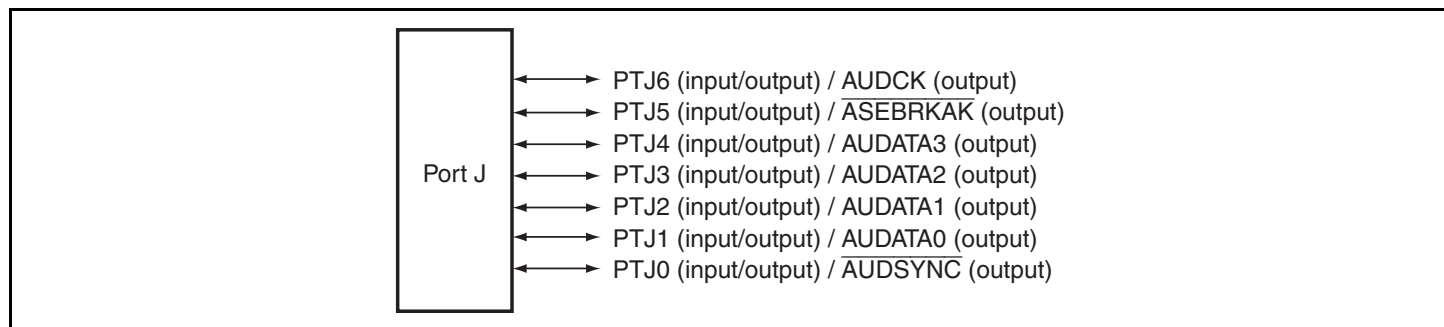
Figure 35.9 Port J
