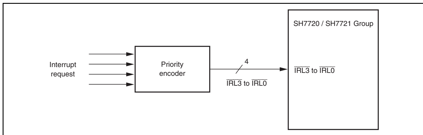
Figure 8.2 Example of IRL Interrupt Connection
