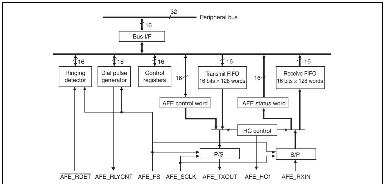
Figure 22.1 Block Diagram of AFE Interface
