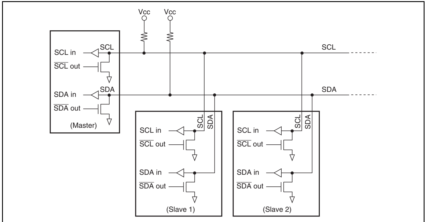
Figure 20.2 External Circuit Connections of I/O Pins
