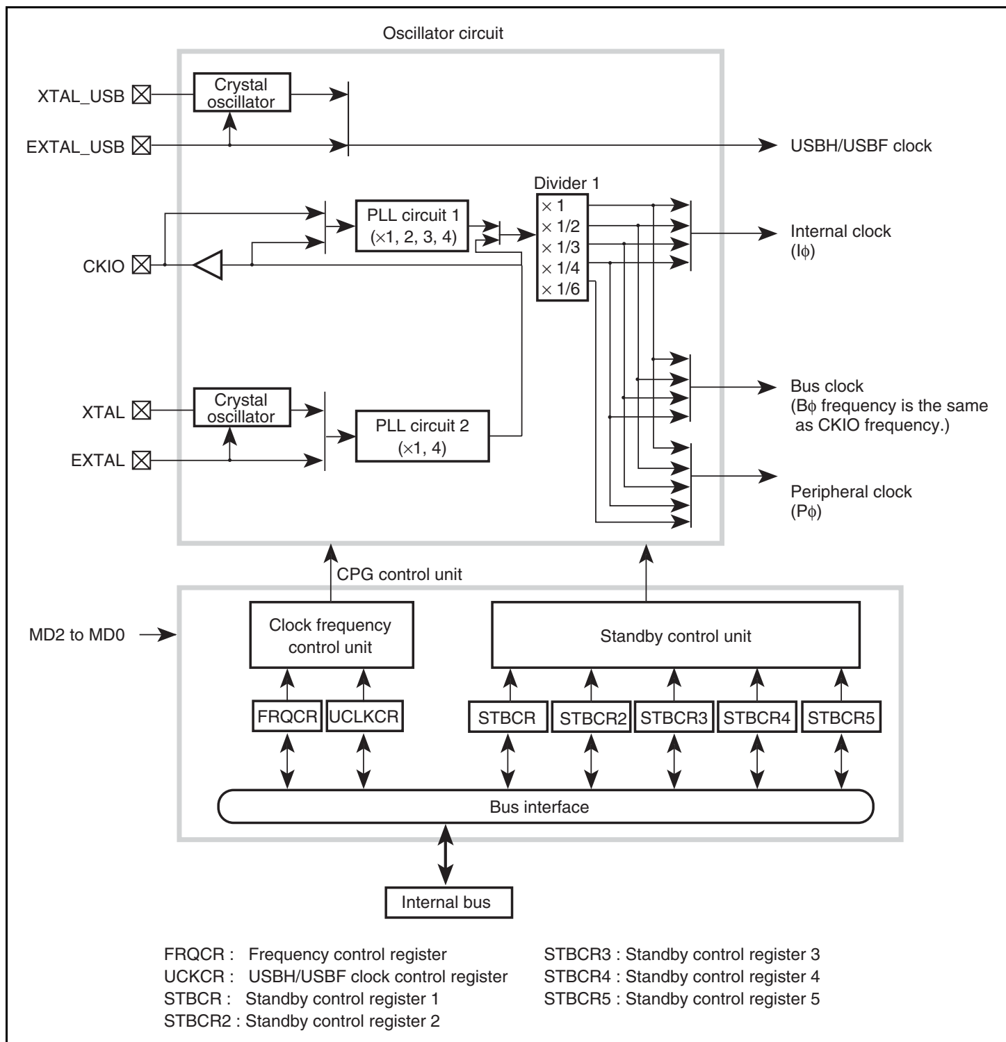
Figure 11.1 Block Diagram of CPG
