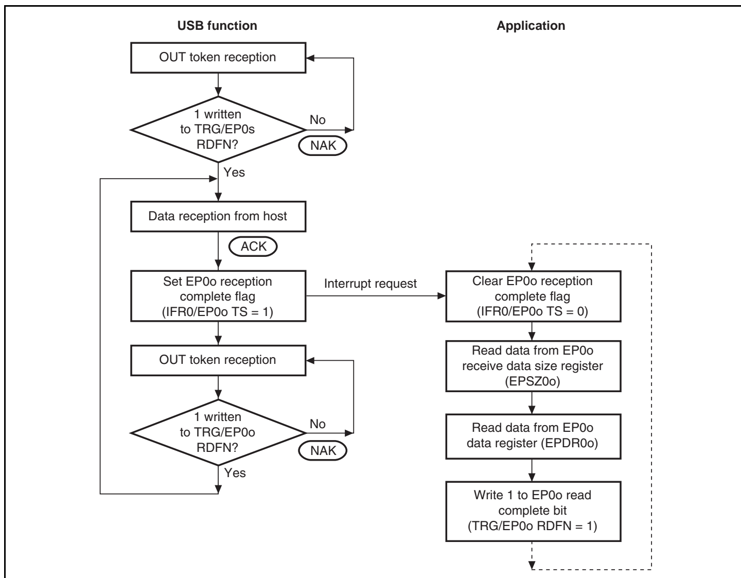
Figure 25.8 Data Stage (Control-Out) Operation
