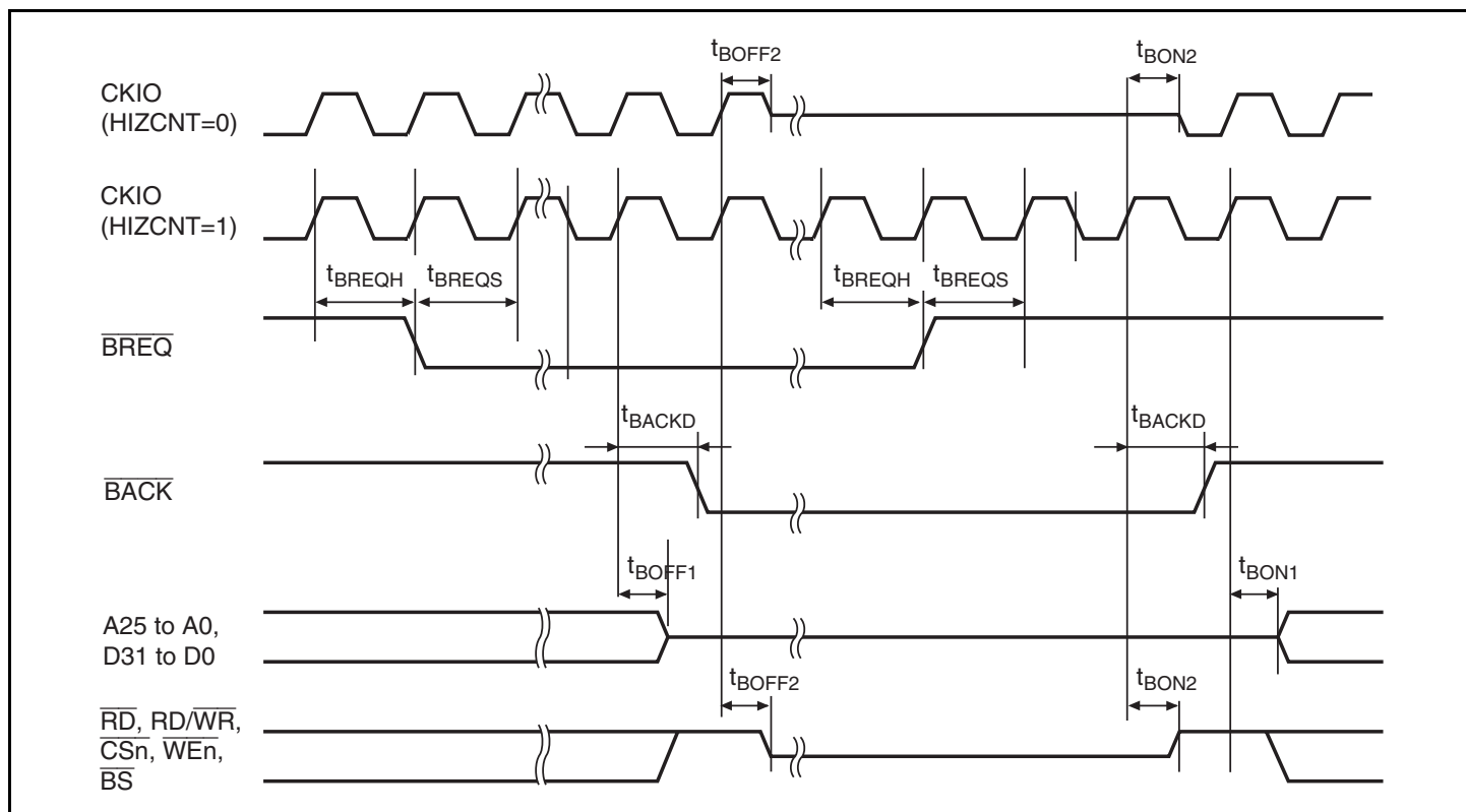
Figure 38.10 Bus Release Timing
