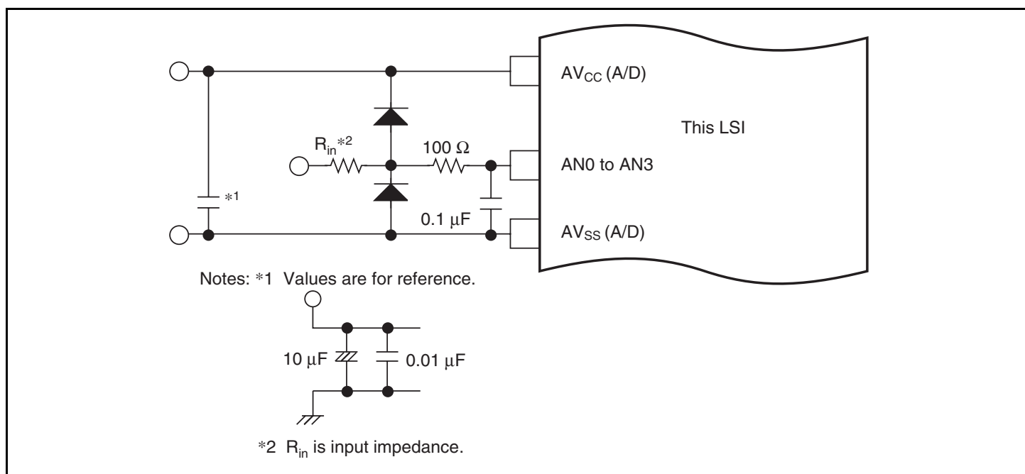
Figure 27.9 Example of Analog Input Protection Circuit
