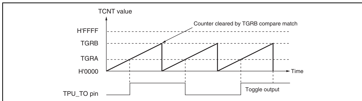
Figure 15.7 Example of Toggle Output Operation
