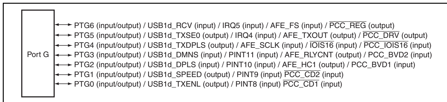
Figure 35.7 Port G
