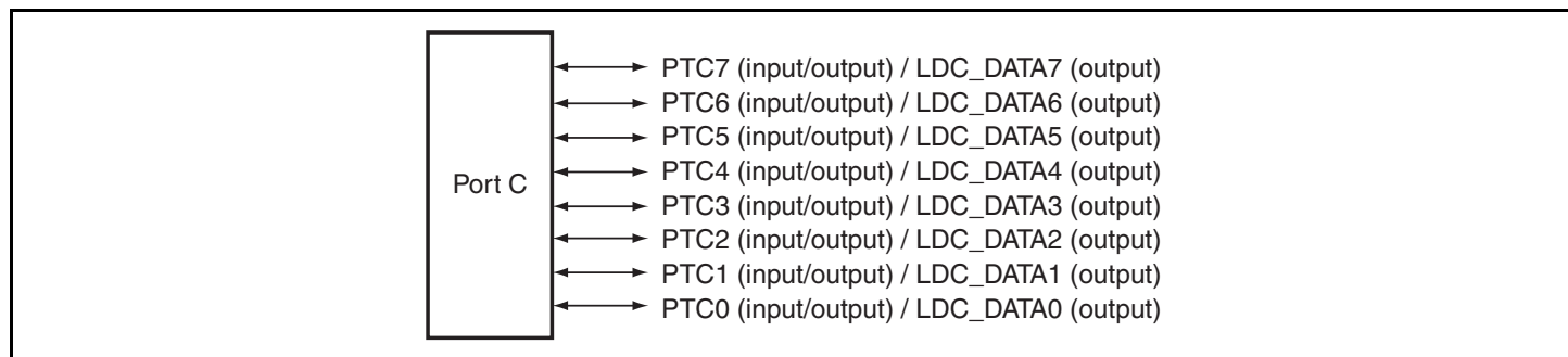
Figure 35.3 Port C
