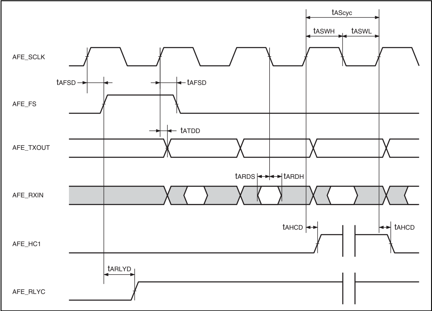
Figure 38.59 AFEIF Module AC Timing
