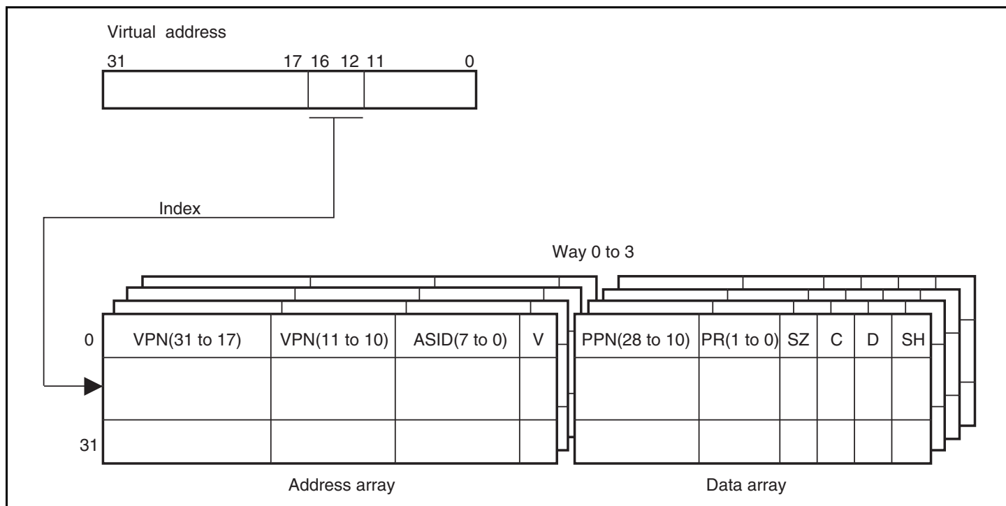
Figure 4.9 TLB Indexing (IX = 0)
