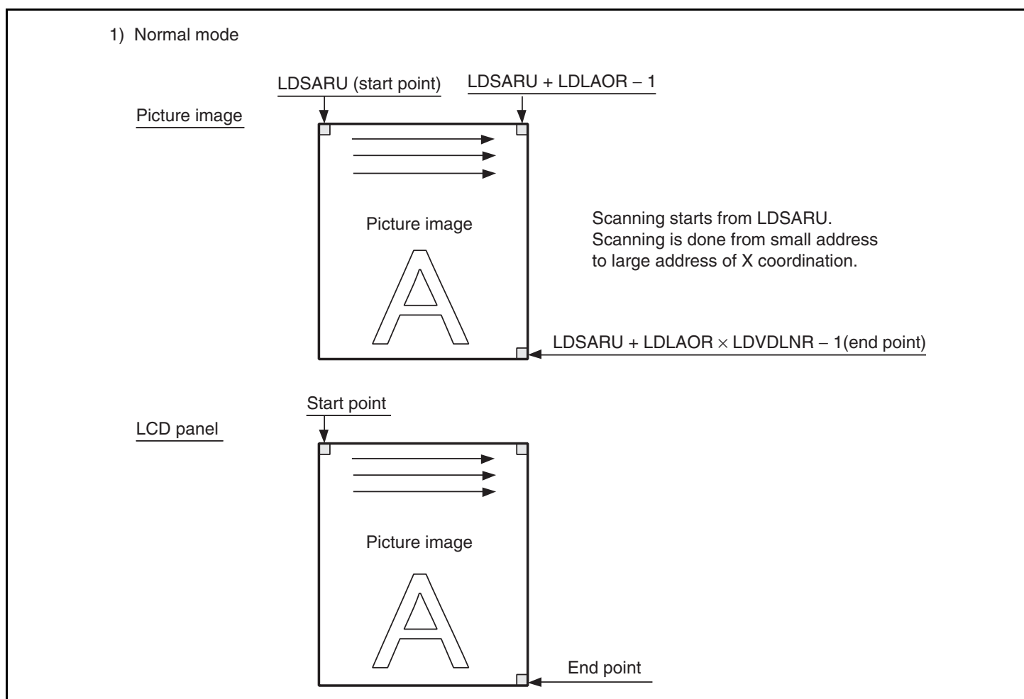
Figure 26.8 Operation for Hardware Rotation (Normal Mode)
