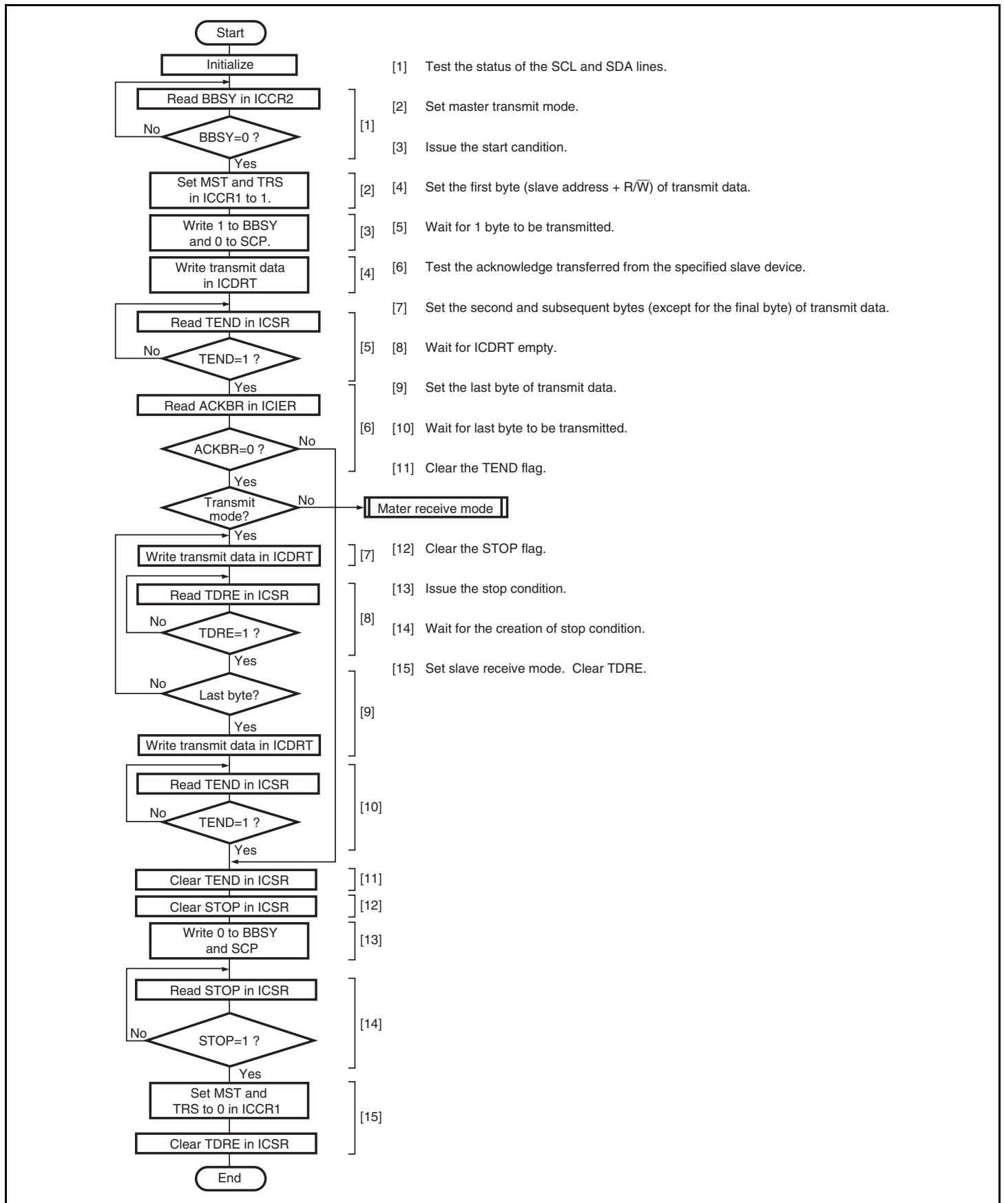
Figure 20.14 Sample Flowchart for Master Transmit Mode
