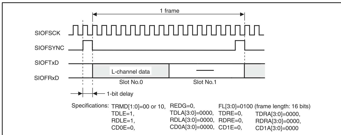
Figure 21.14 Transmit and Receive Timing (8-Bit Monaural Data (2))
