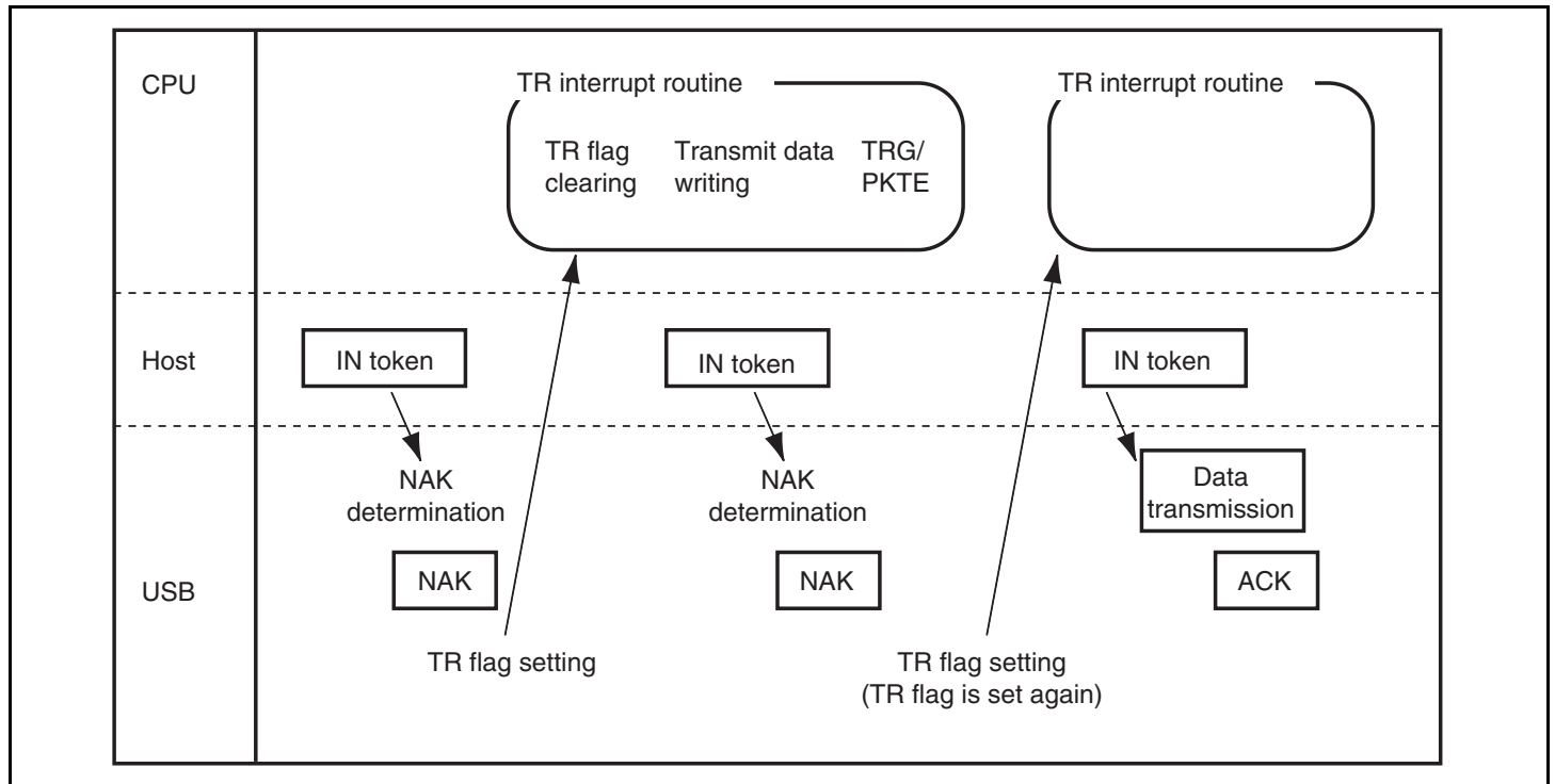
Figure 25.20 Set Timing of TR Interrupt Flag
