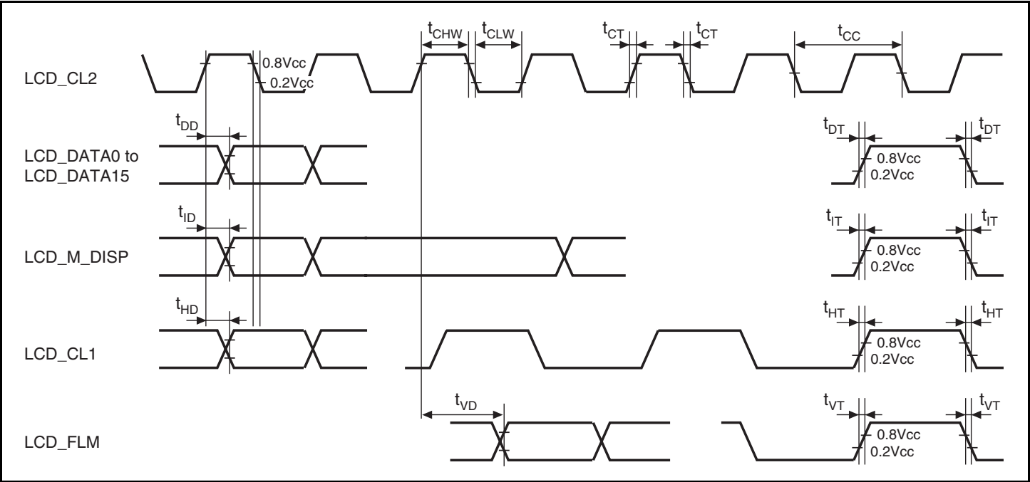
Figure 38.61 LCDC Module Signal Timing
