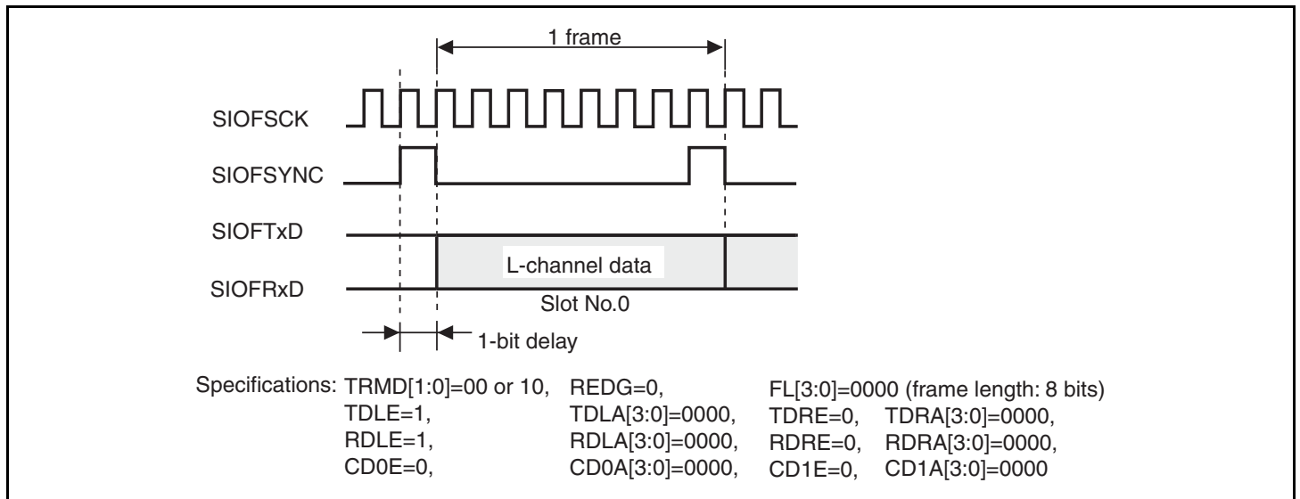
Figure 21.13 Transmit and Receive Timing (8-Bit Monaural Data (1))
