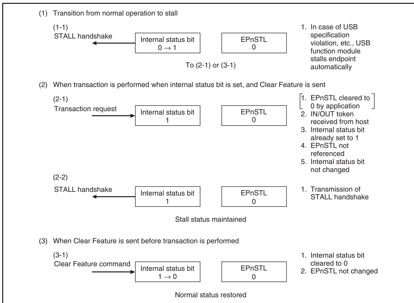
Figure 25.19 Automatic Stall by USB Function Controller
