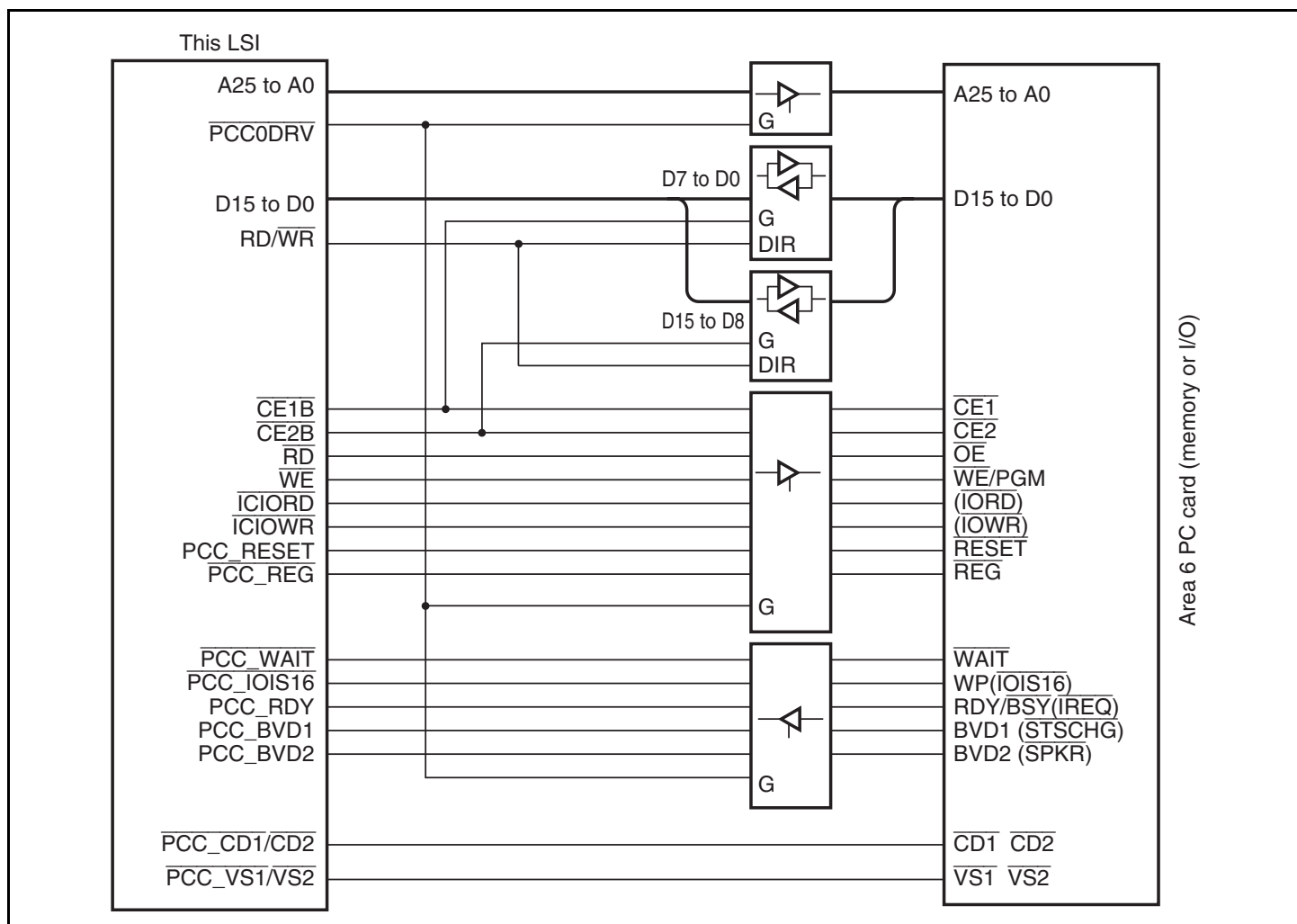
Figure 29.4 Interface
