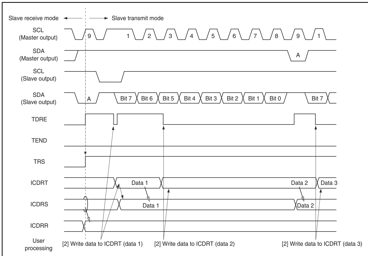
Figure 20.9 Slave Transmit Mode Operation Timing (1)
