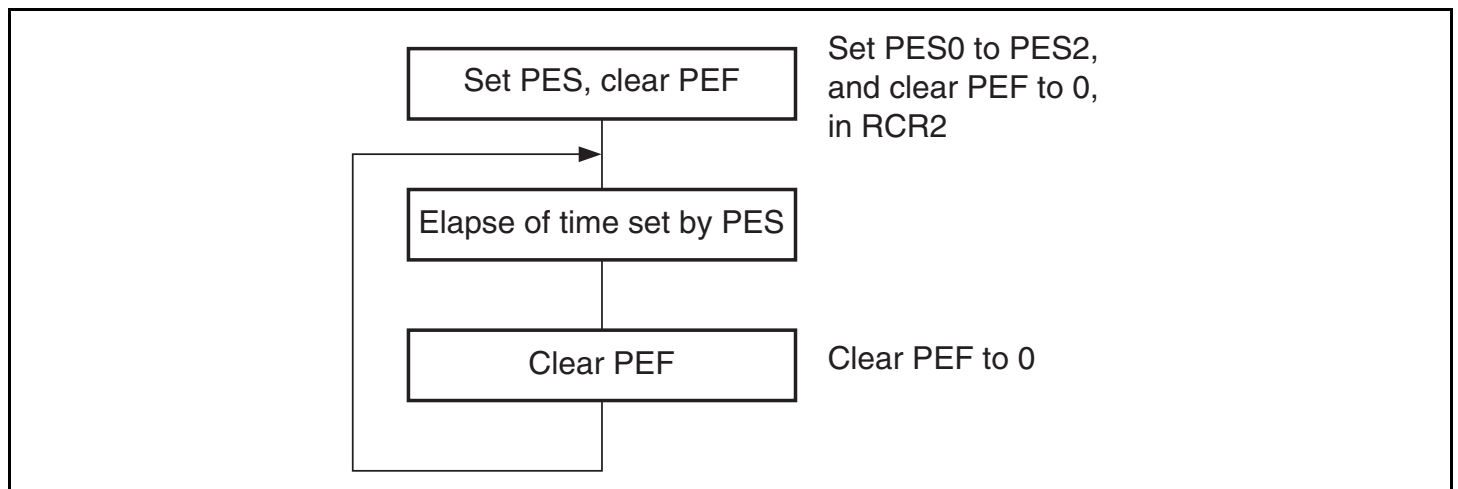
Figure 17.5 Using Periodic Interrupt Function
