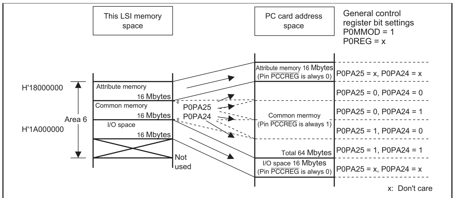
Figure 29.3 Continuous 16-Mbyte Area Mode (Area 6)
