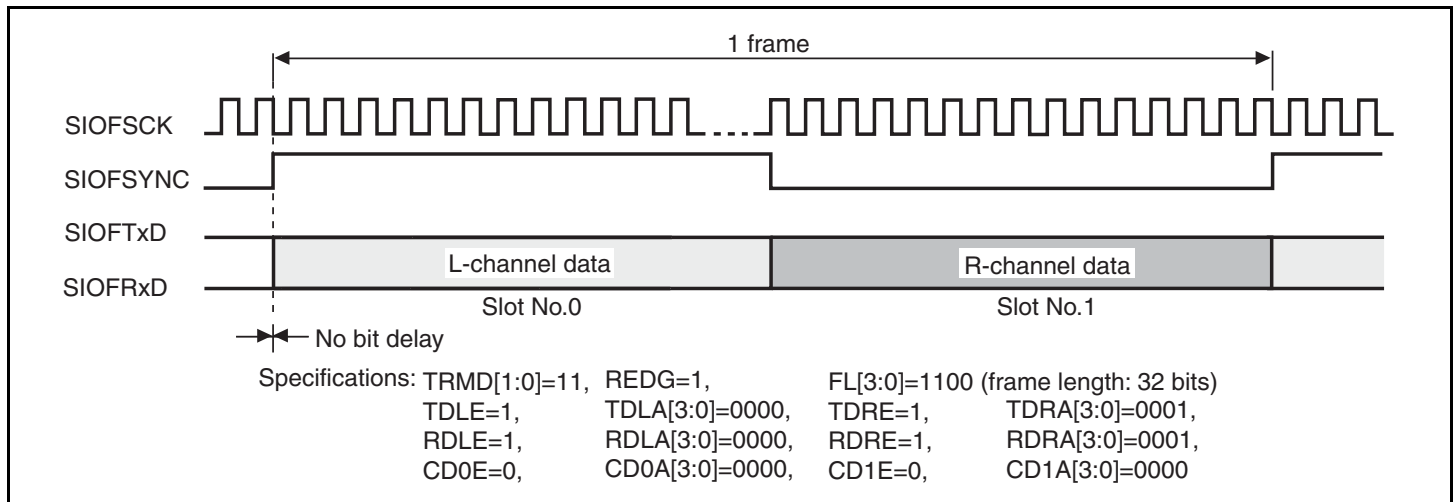
Figure 21.16 Transmit and Receive Timing (16-Bit Stereo Data (1))
