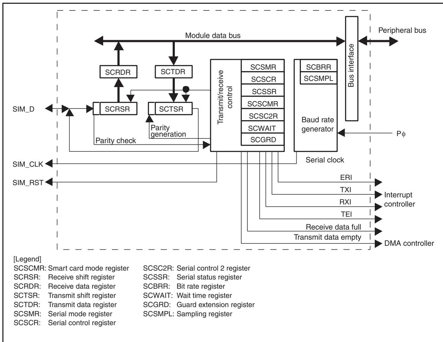
Figure 30.1 Smart Card Interface
