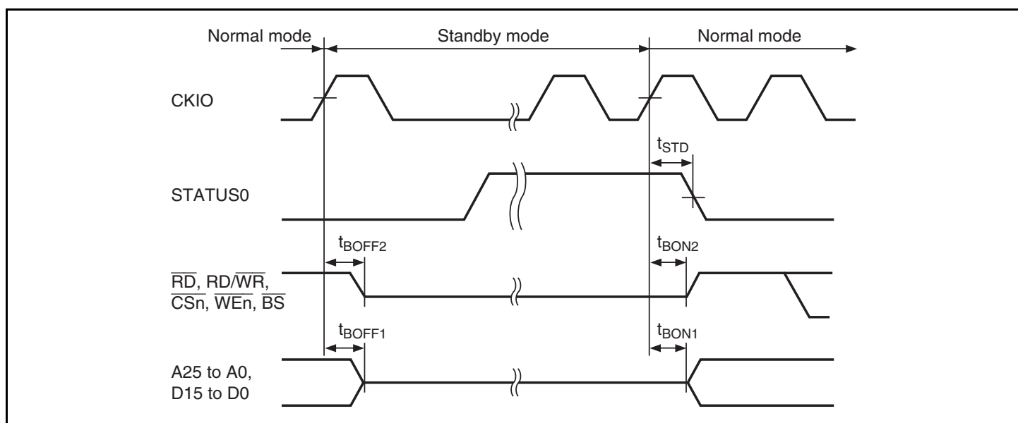
Figure 38.11 Pin Drive Timing at Standby
