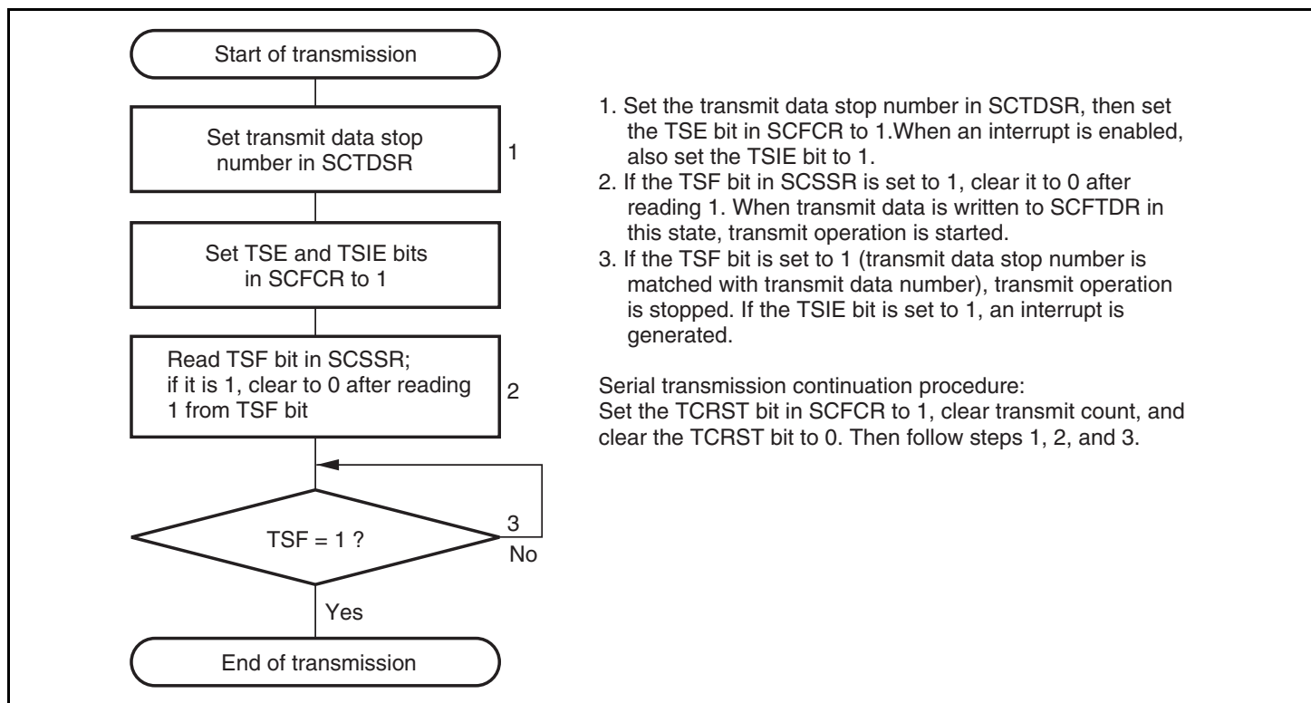
Figure 18.6 Transmit Data Stop Function Flowchart
