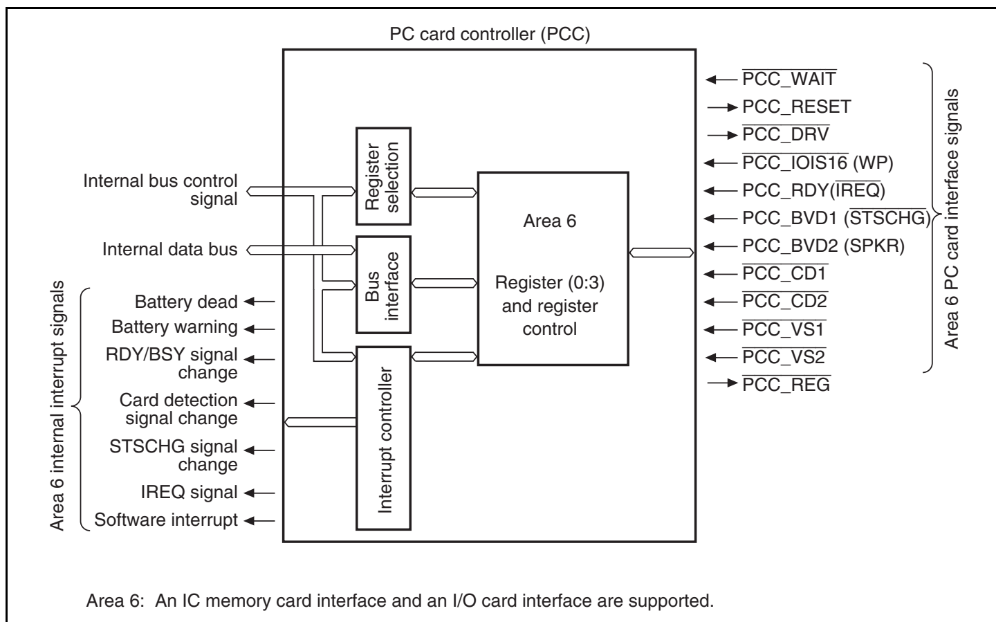
Figure 29.1 PC Card Controller Block Diagram
