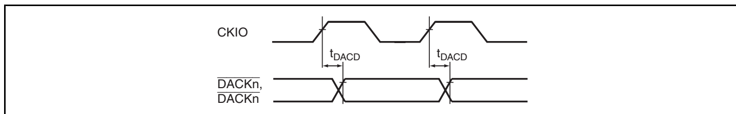
Figure 38.46 DACK Output Timing
