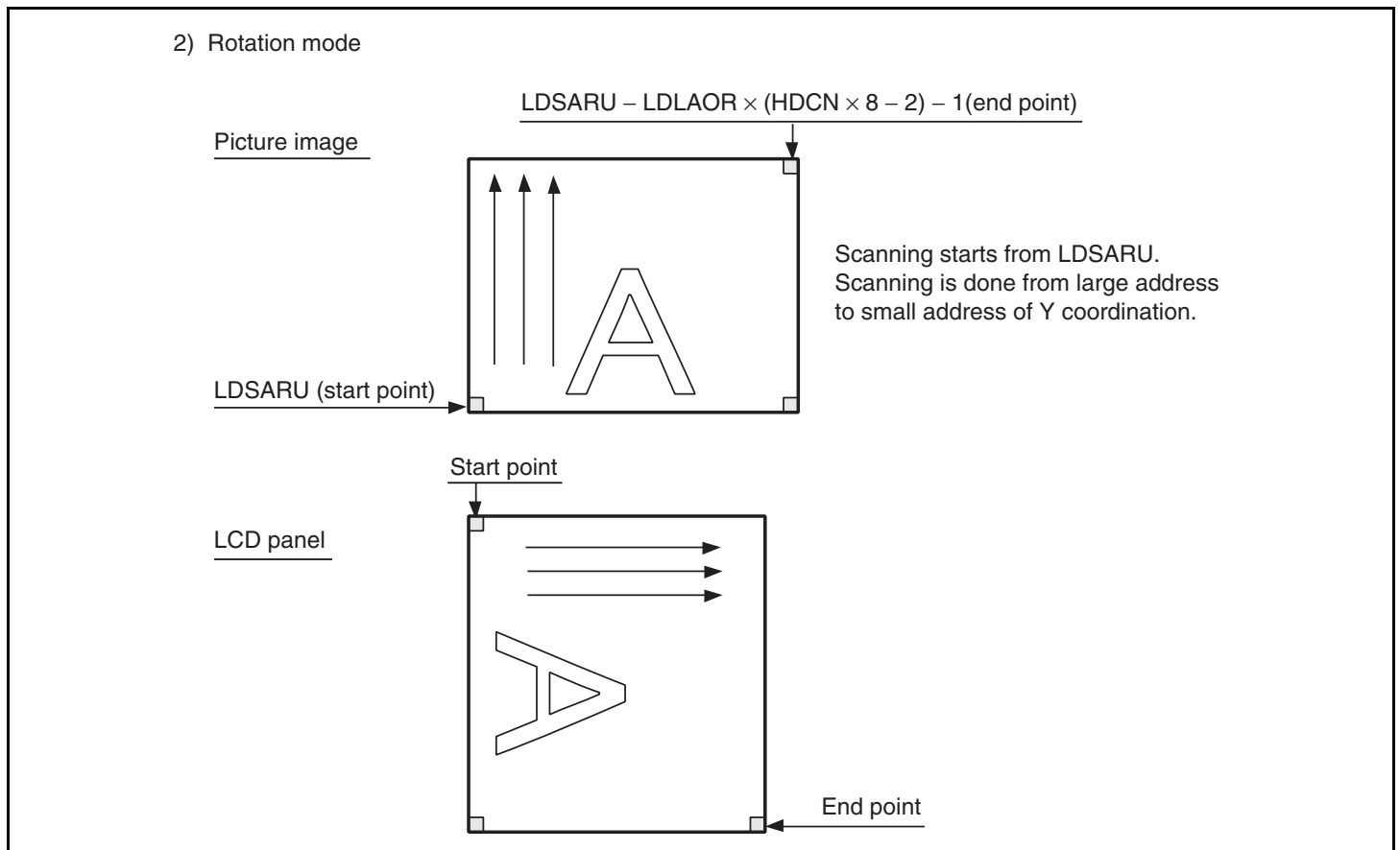
Figure 26.9 Operation for Hardware Rotation (Rotation Mode)
