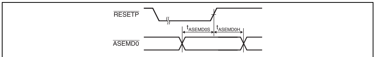
Figure 38.68 \overline{\text{ASEMD0}} Input Timing
