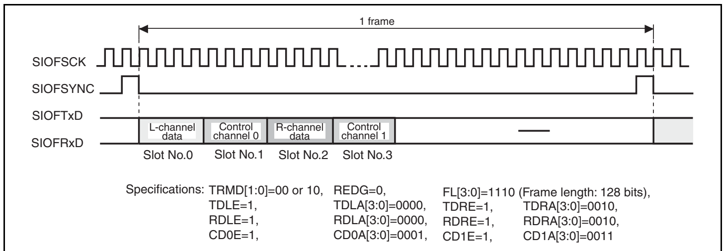
Figure 21.7 Control Data Interface (Slot Position)
