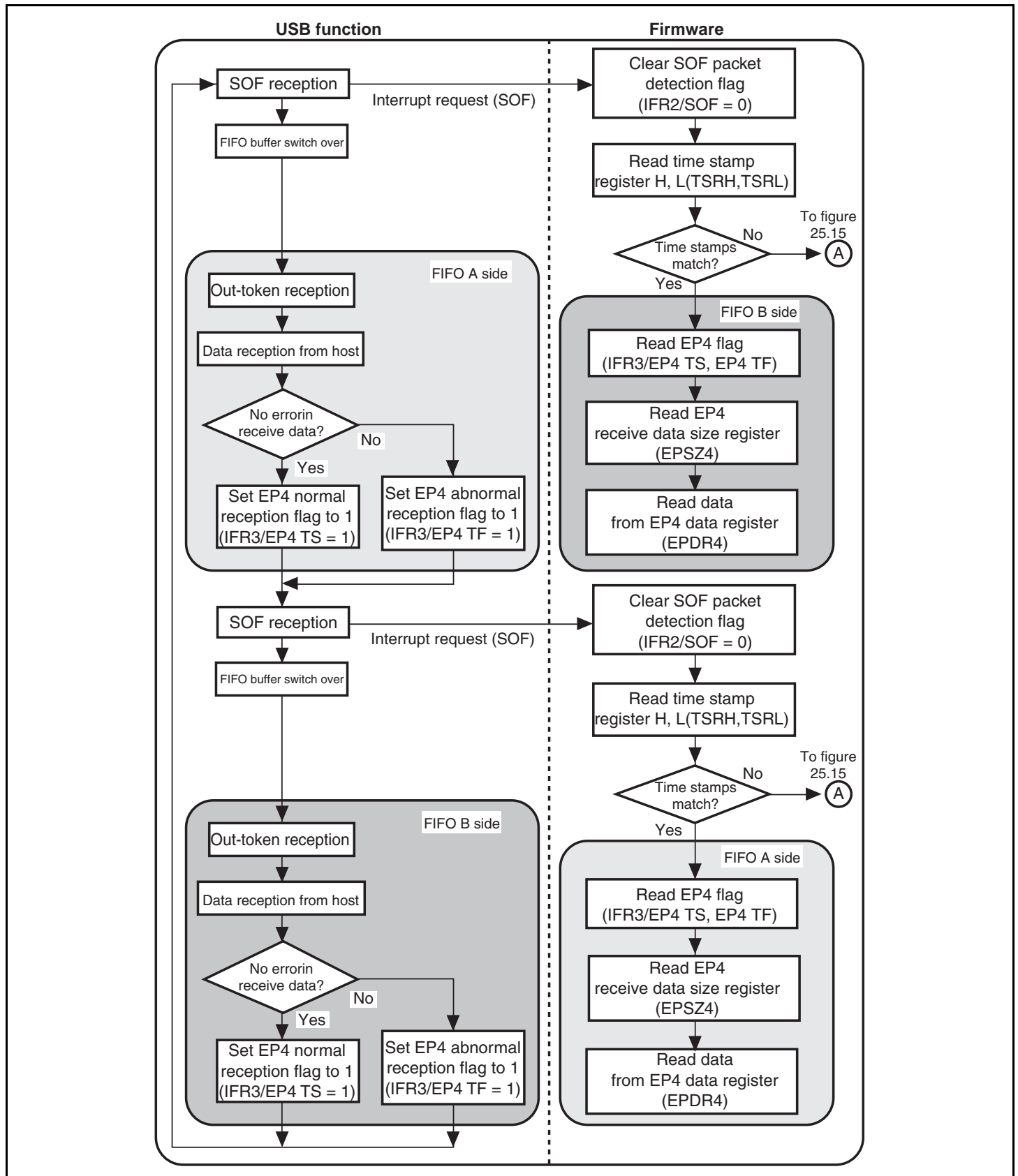
Figure 25.14 EP4 Isochronous-Out Transfer Operation (SOF is Normal)
