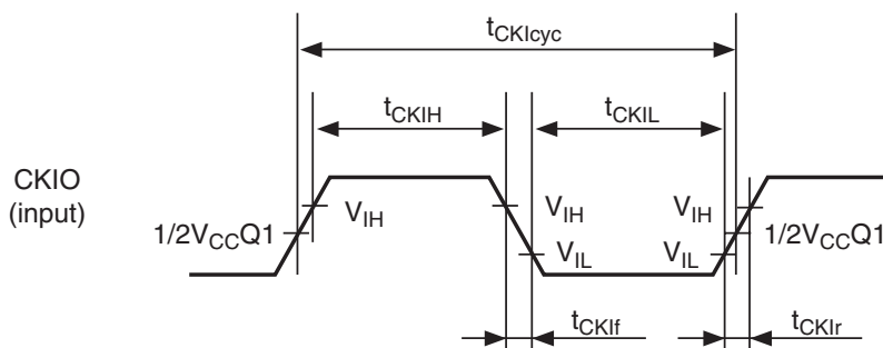
Figure 38.3 CKIO Clock Input Timing
