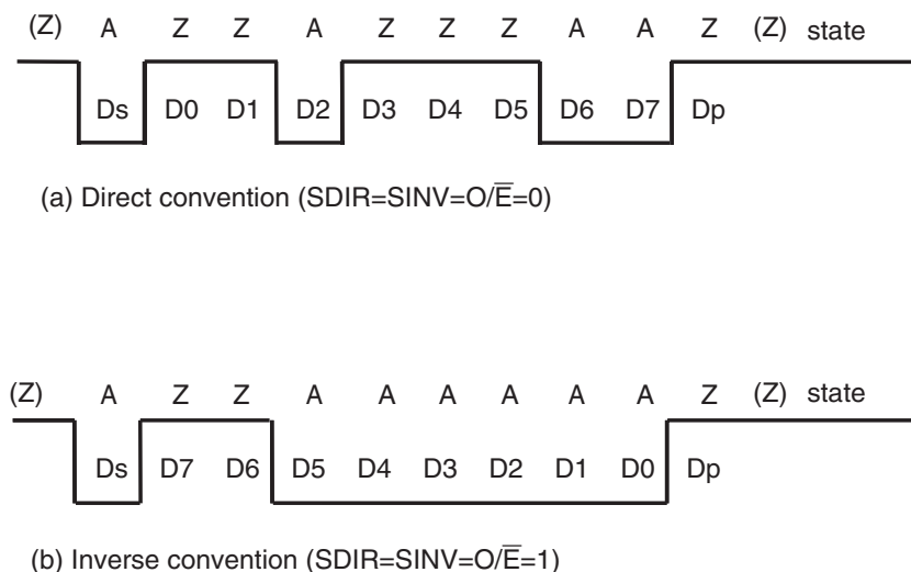
Figure 30.3 Examples of Start Character Waveforms
