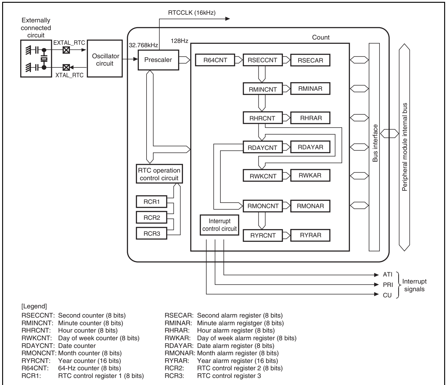
Figure 17.1 RTC Block Diagram
