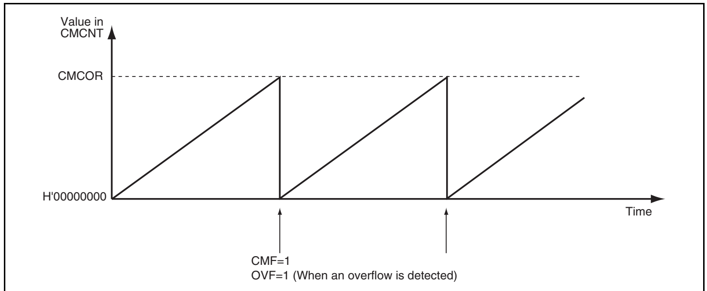
Figure 16.3 Counter Operation (Free-Running Operation)
