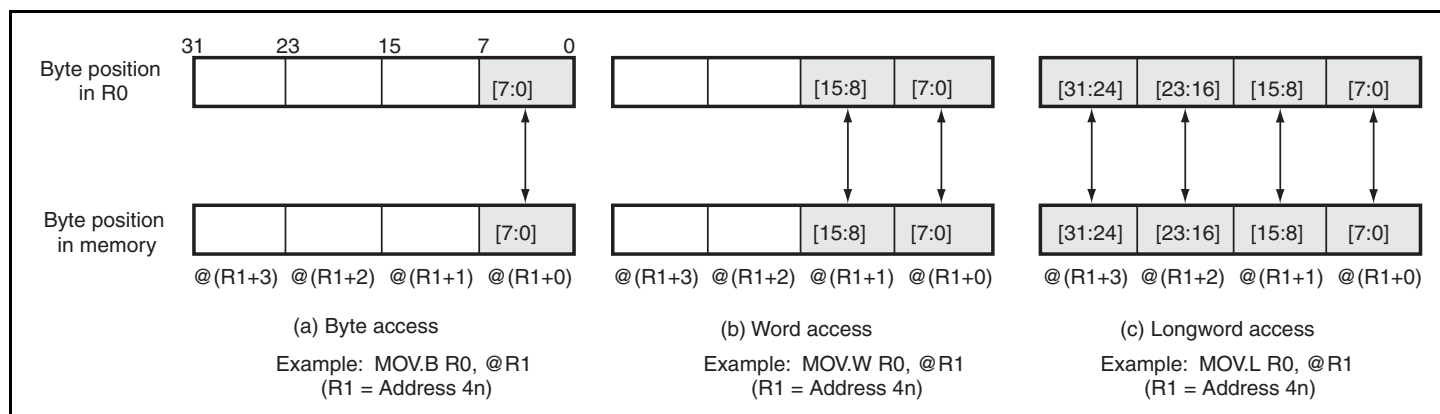
Figure 2.8 Data Format on Memory (Little Endian Mode)
