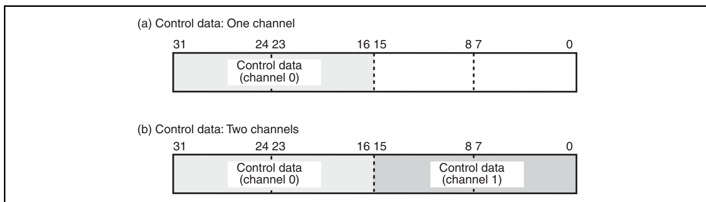
Figure 21.6 Control Data Bit Alignment
