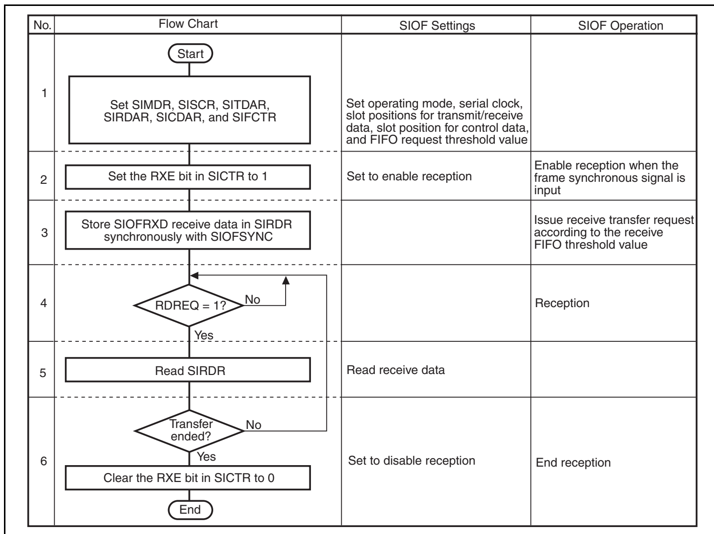
Figure 21.12 Example of Receive Operation in Slave Mode
