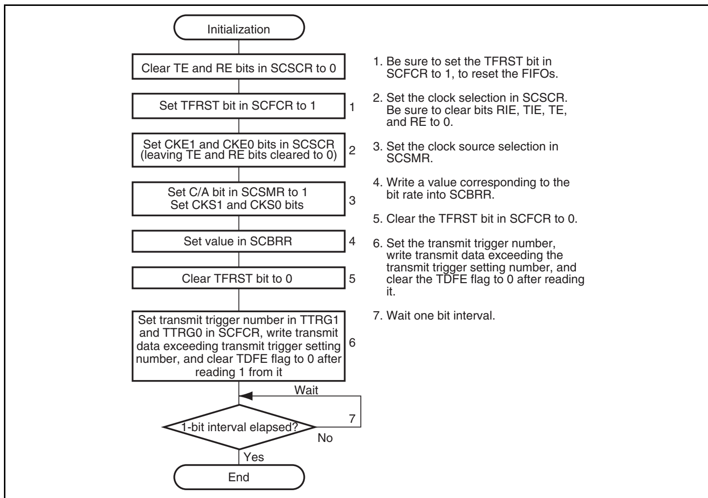
Figure 18.13 Sample SCIF Initialization Flowchart (1) (Transmission)
