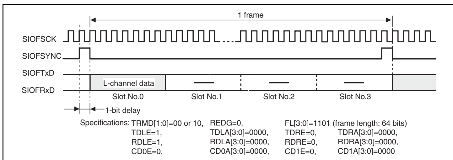
Figure 21.15 Transmit and Receive Timing (16-Bit Monaural Data (1))
