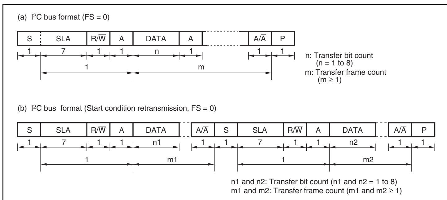
Figure 20.3 I 2 C Bus Formats
