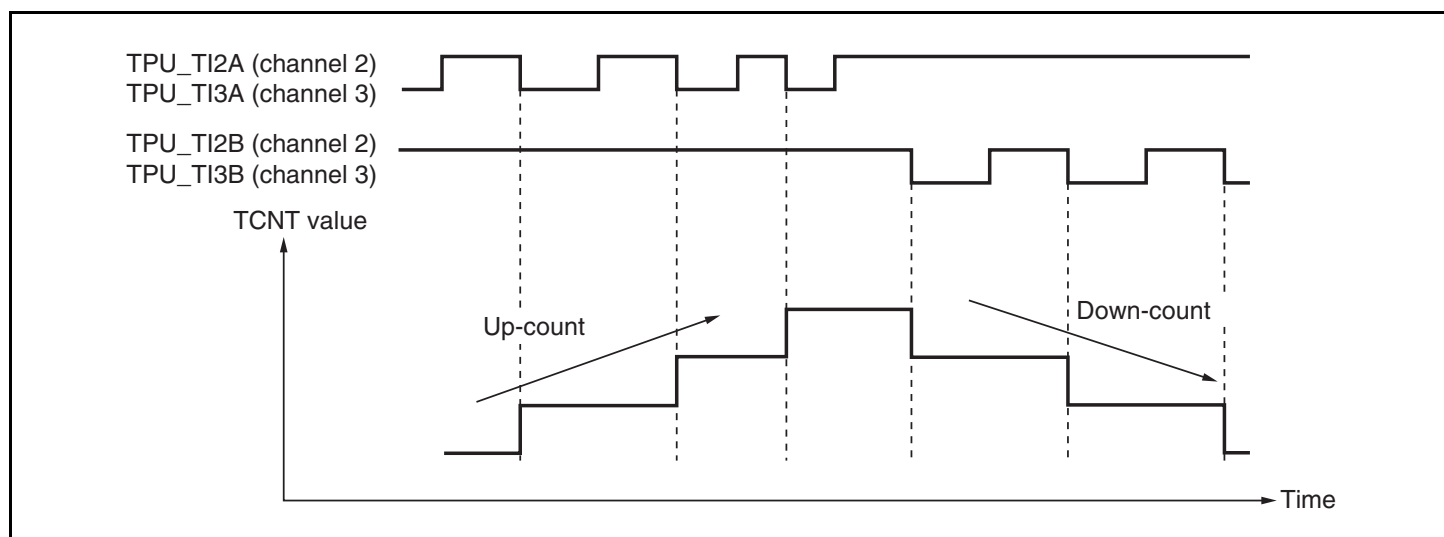
Figure 15.17 Example of Phase Counting Mode 3 Operation
