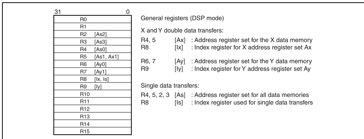
Figure 3.5 General Registers (DSP Mode)
