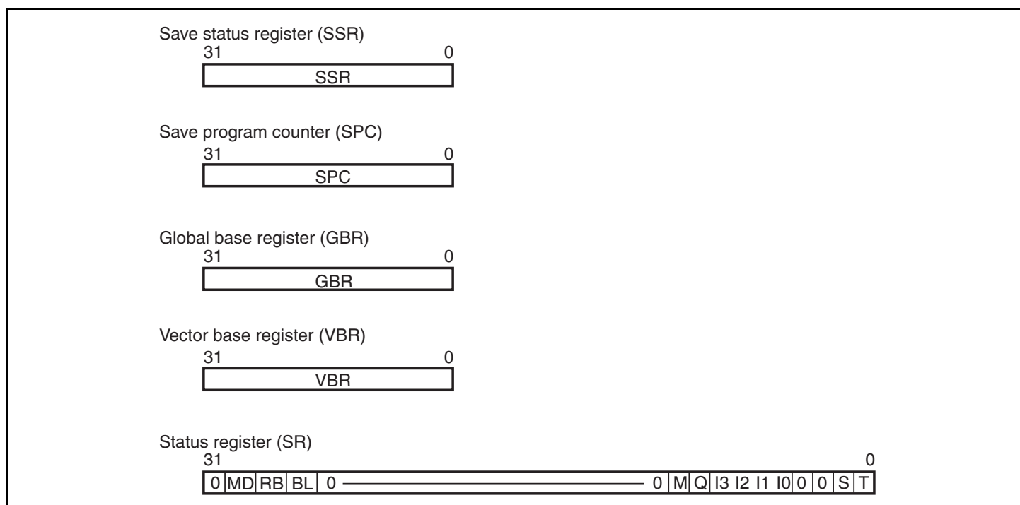
Figure 2.6 Control Register Configuration
