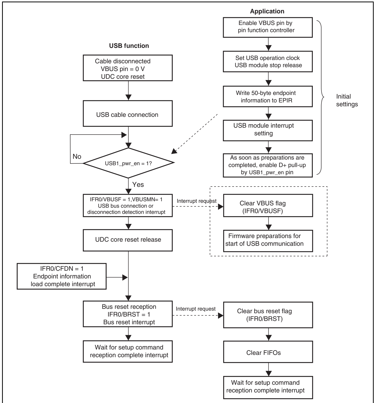
Figure 25.3 Cable Connection Operation
