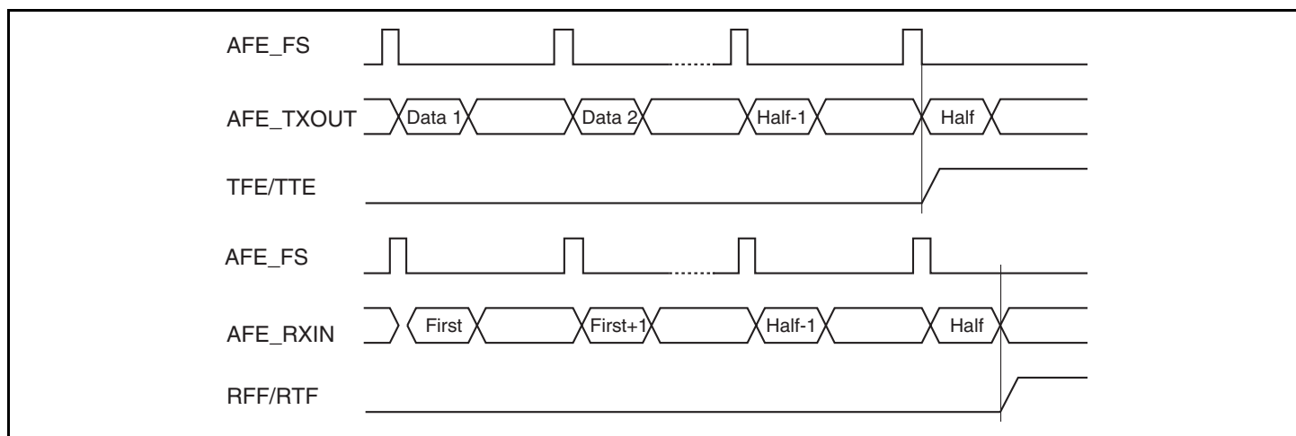
Figure 22.2 FIFO Interrupt Timing
