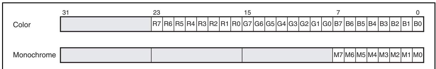
Figure 26.3 Color-Palette Data Format
