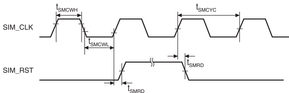
Figure 38.62 SIM Module Signal Timing
