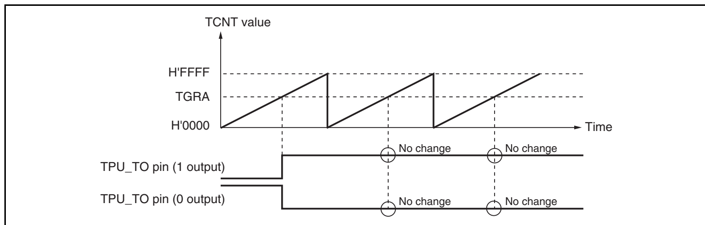
Figure 15.6 Example of 0 Output/1 Output Operation
