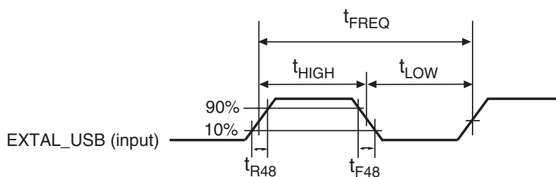
Figure 38.60 USB Clock Timing
