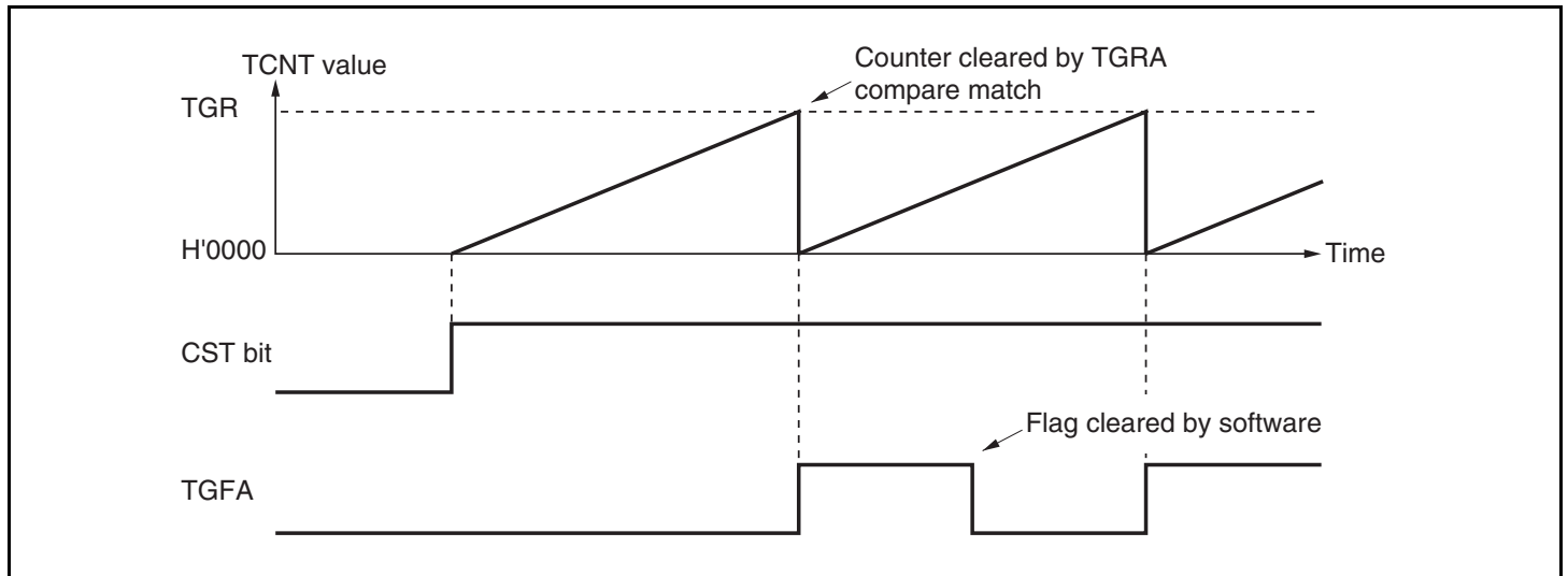
Figure 15.4 Periodic Counter Operation
