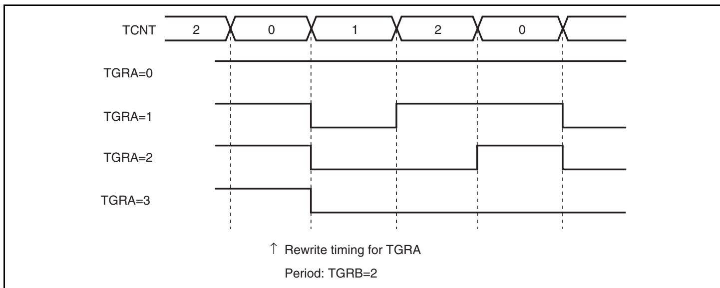
Figure 15.13 Examples of PWM Mode Operation (2)
