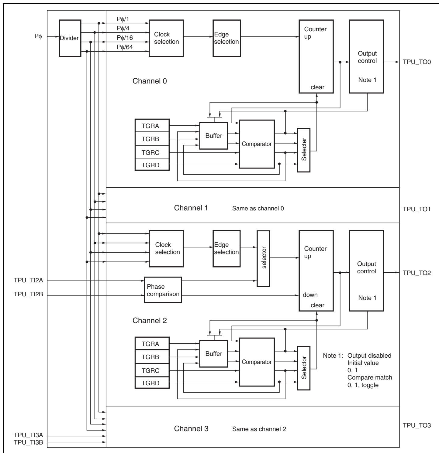
Figure 15.1 Block Diagram of TPU
