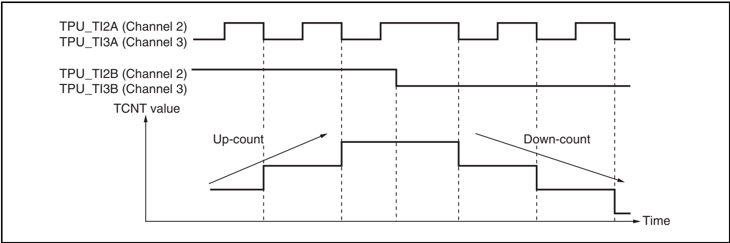
Figure 15.16 Example of Phase Counting Mode 2 Operation
