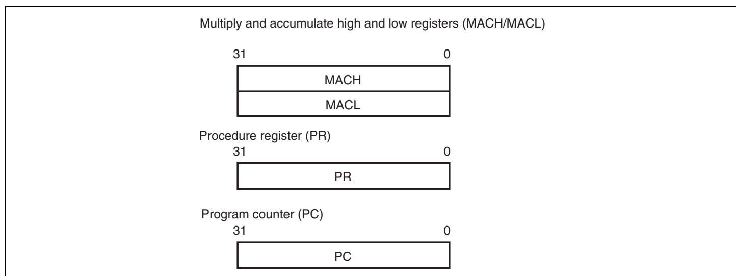
Figure 2.5 System Registers and Program Counter
