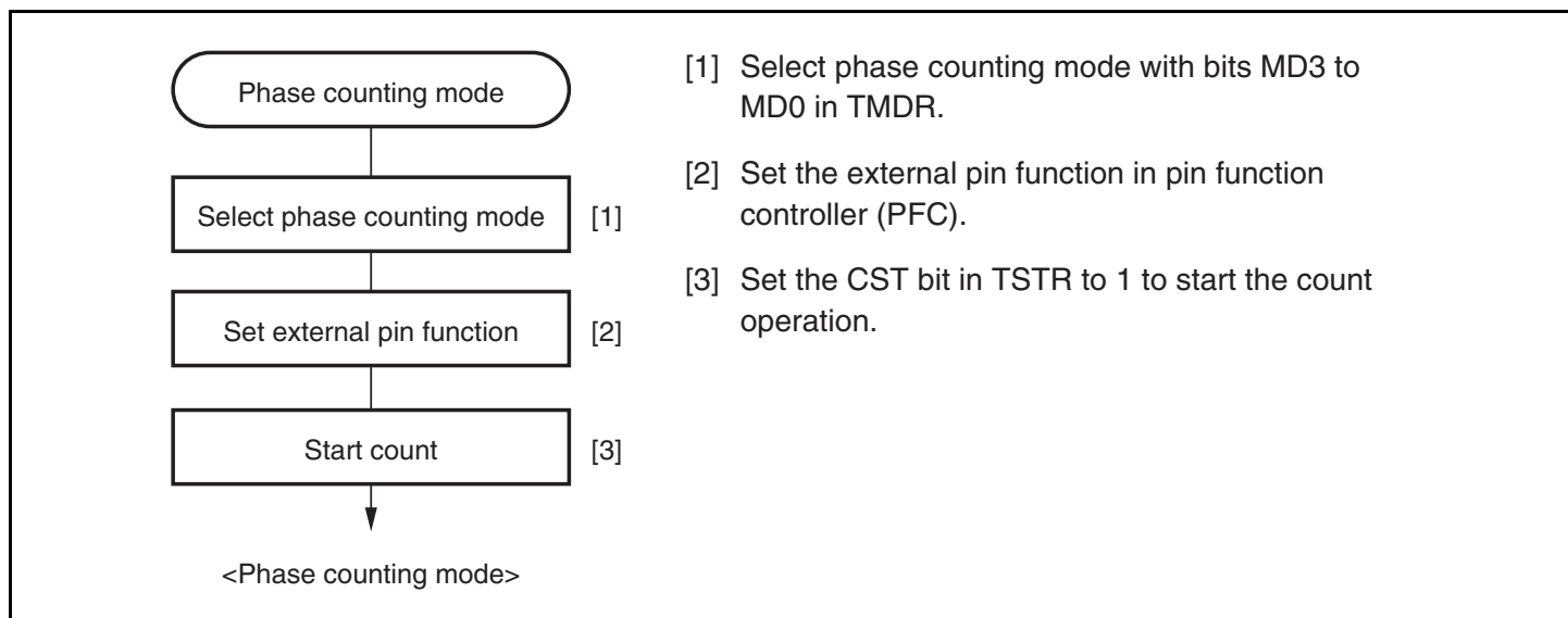
Figure 15.14 Example of Phase Counting Mode Setting Procedure
