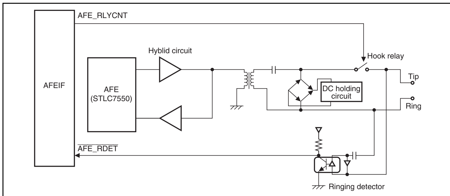
Figure 22.7 DAA Block Diagram
