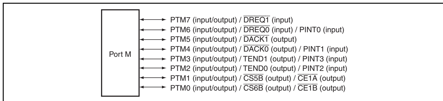
Figure 35.12 Port M
