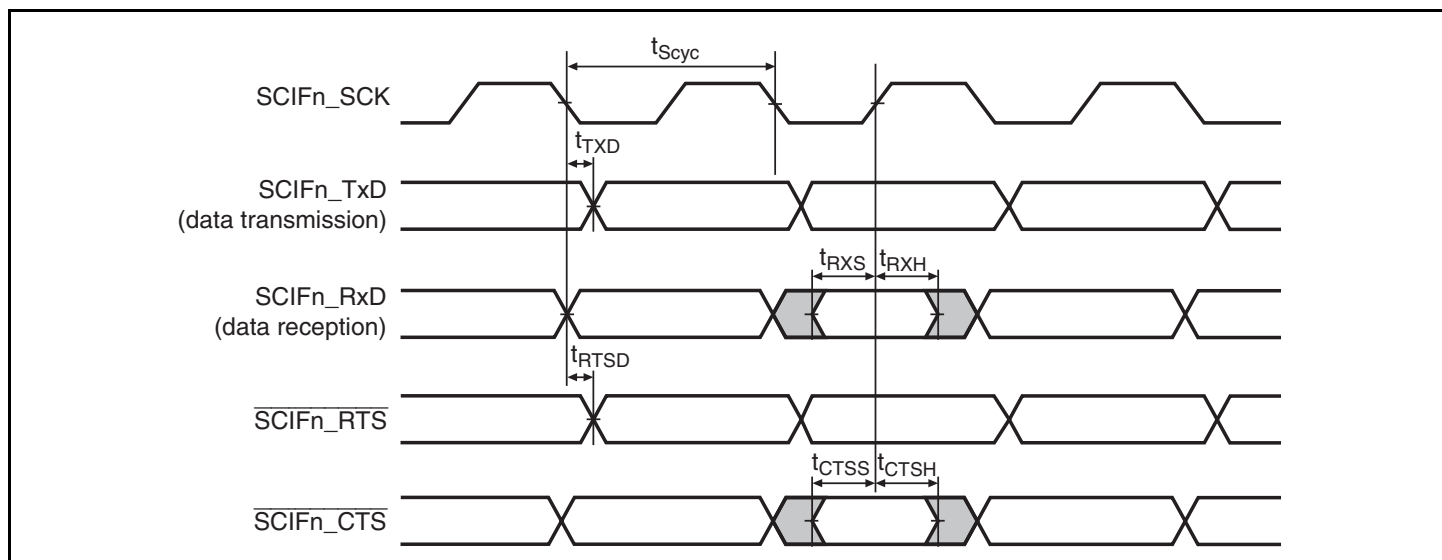
Figure 38.51 SCIF Input/Output Timing in Synchronous Mode
