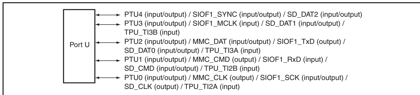
Figure 35.17 Port U
