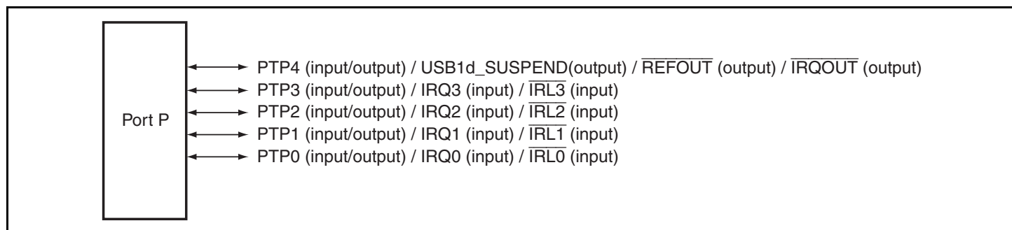
Figure 35.13 Port P
