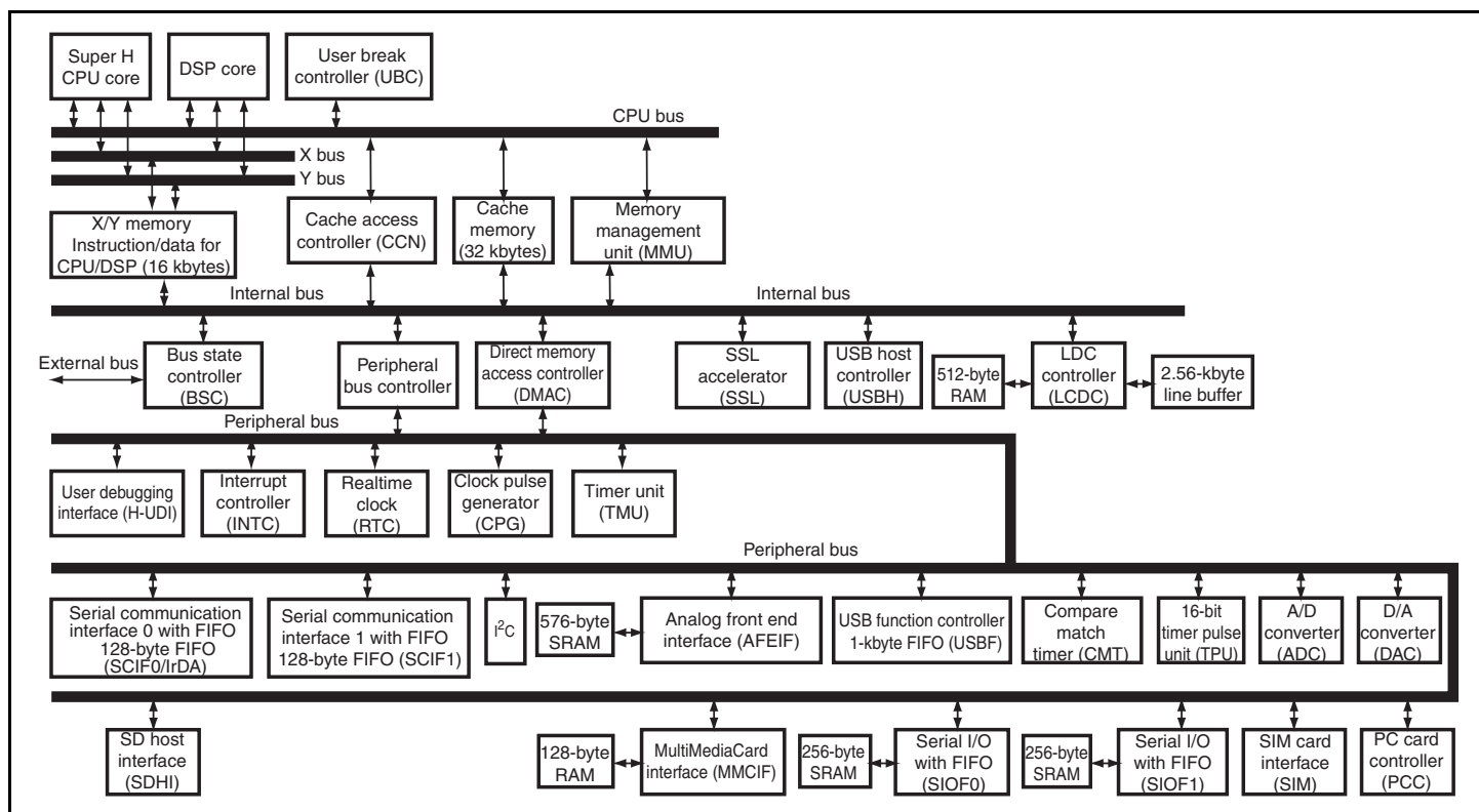
Figure 1.1 Block Diagram
