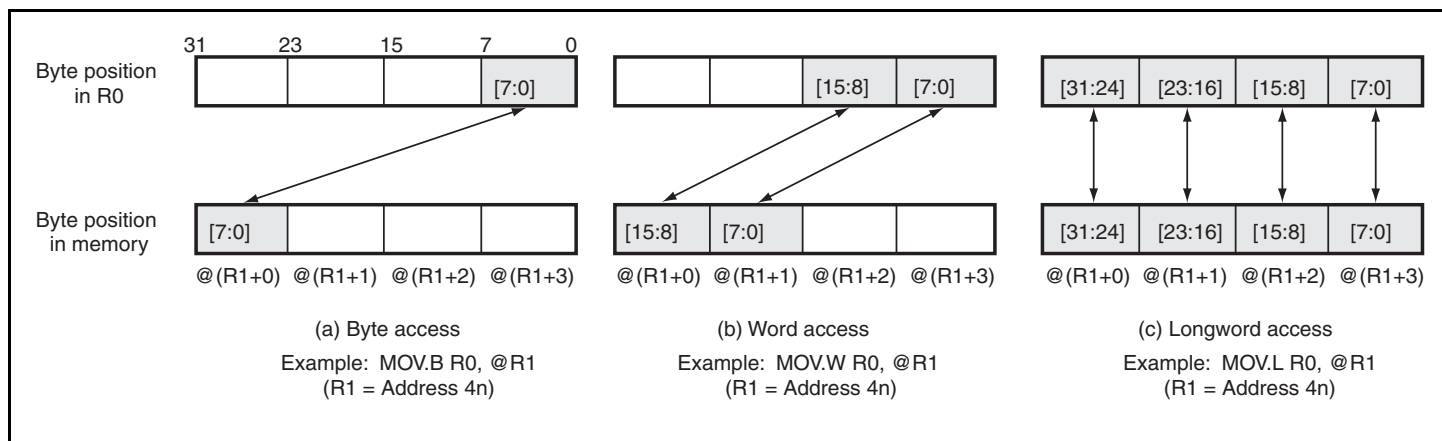
Figure 2.7 Data Format on Memory (Big Endian Mode)
