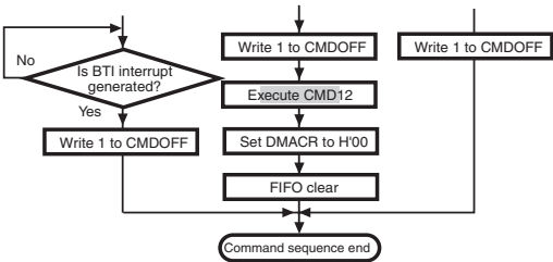
Figure 31.30 Operational Flowchart for Write Sequence (Pre-defined Multiblock Transfer) (2)
