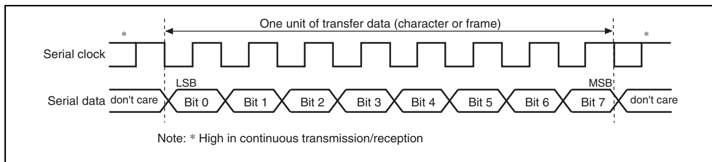
Figure 18.12 Data Format in Synchronous Communication
