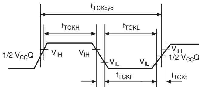
Figure 38.65 TCK Input Timing
