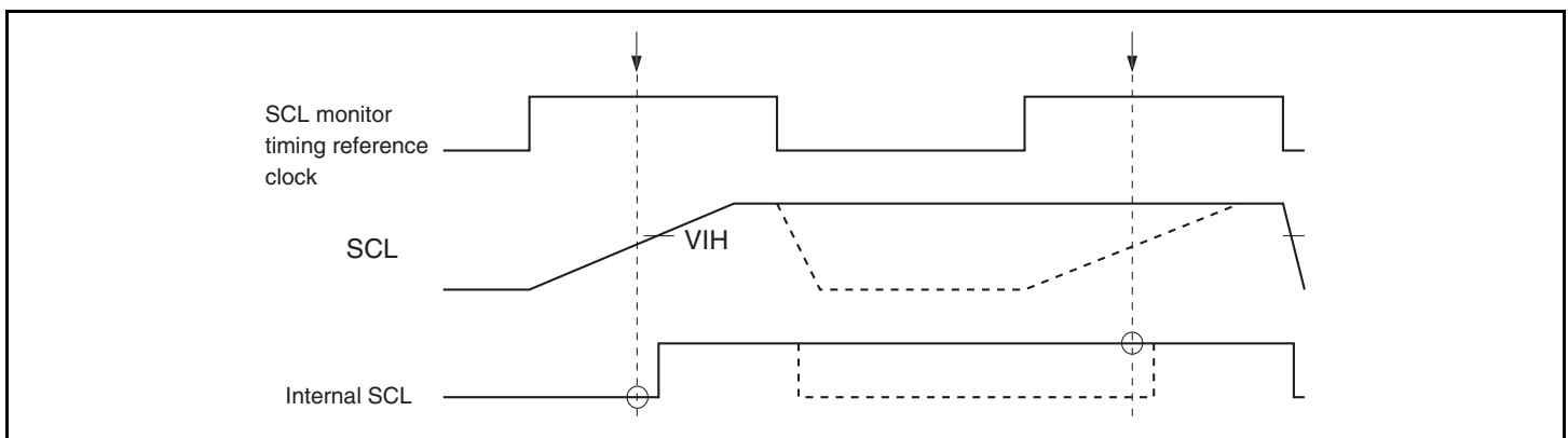
Figure 20.18 The Timing of the Bit Synchronous Circuit
