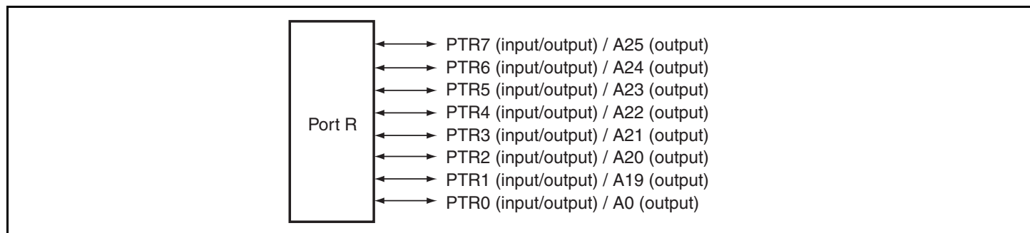
Figure 35.14 Port R
