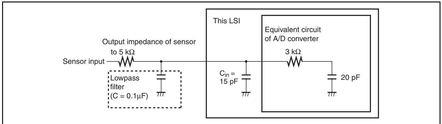
Figure 27.8 Analog Input Circuit Example
