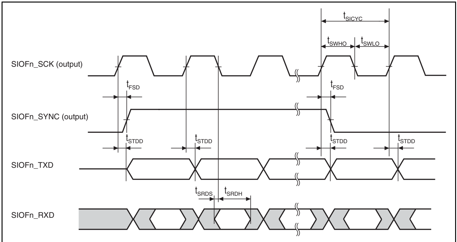
Figure 38.56 SIOF Transmission/Reception Timing (Master Mode 2, Fall Sampling)
