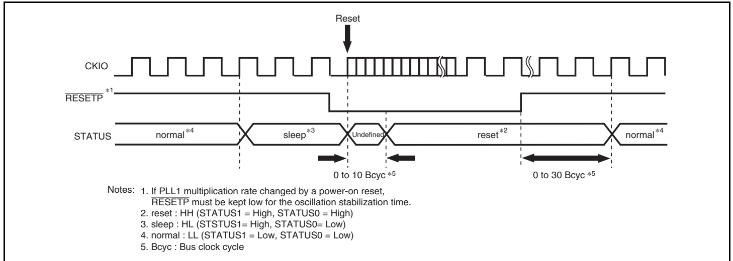
Figure 13.8 STATUS Output When Sleep Mode is Canceled by a Power-on Reset
