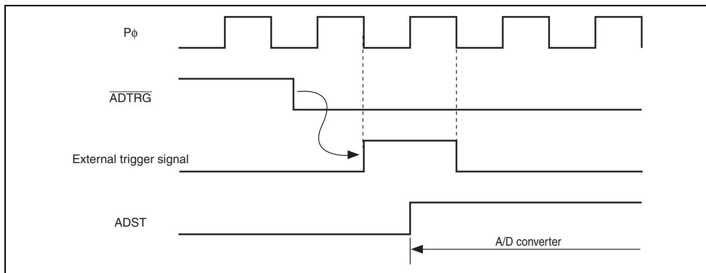
Figure 27.6 External Trigger Input Timing
