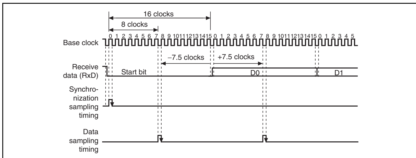
Figure 18.17 Receive Data Sampling Timing in Asynchronous Mode
