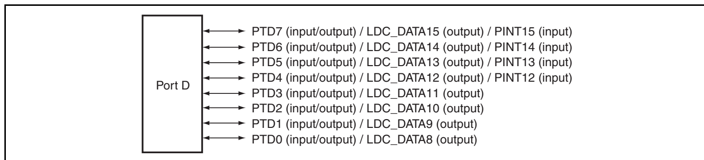
Figure 35.4 Port D
