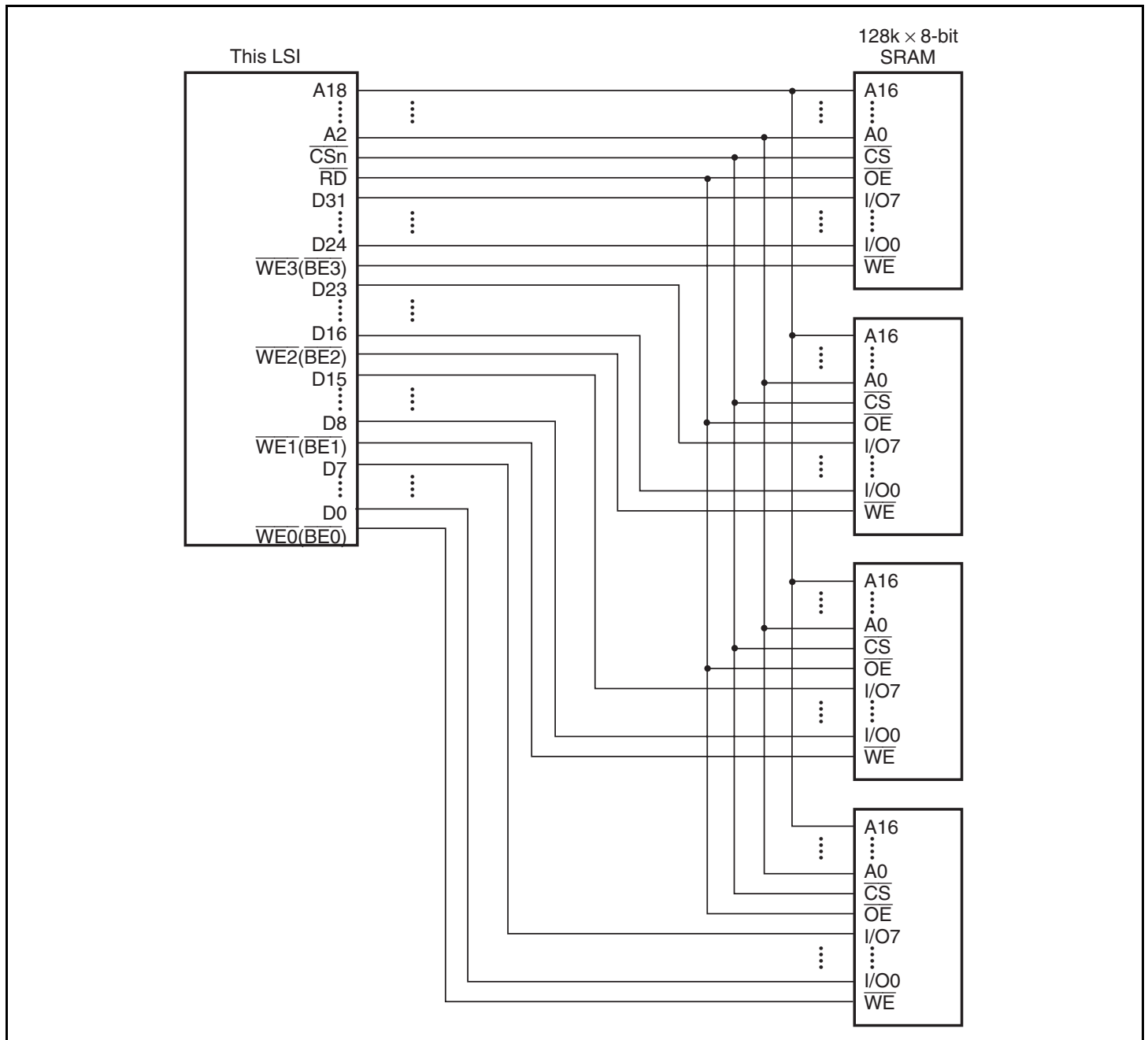
Figure 9.6 Example of 32-Bit Data-Width SRAM Connection
