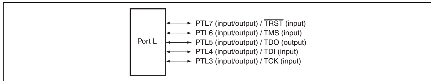
Figure 35.11 Port L
