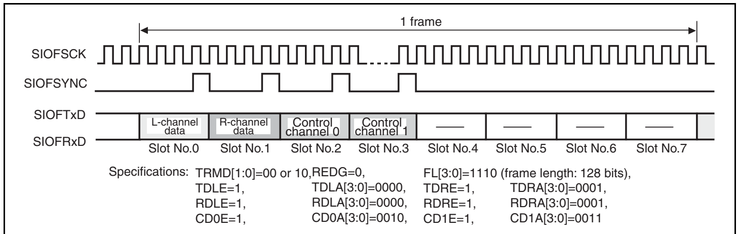
Figure 21.20 Transmit and Receive Timing (16-Bit Stereo Data)
