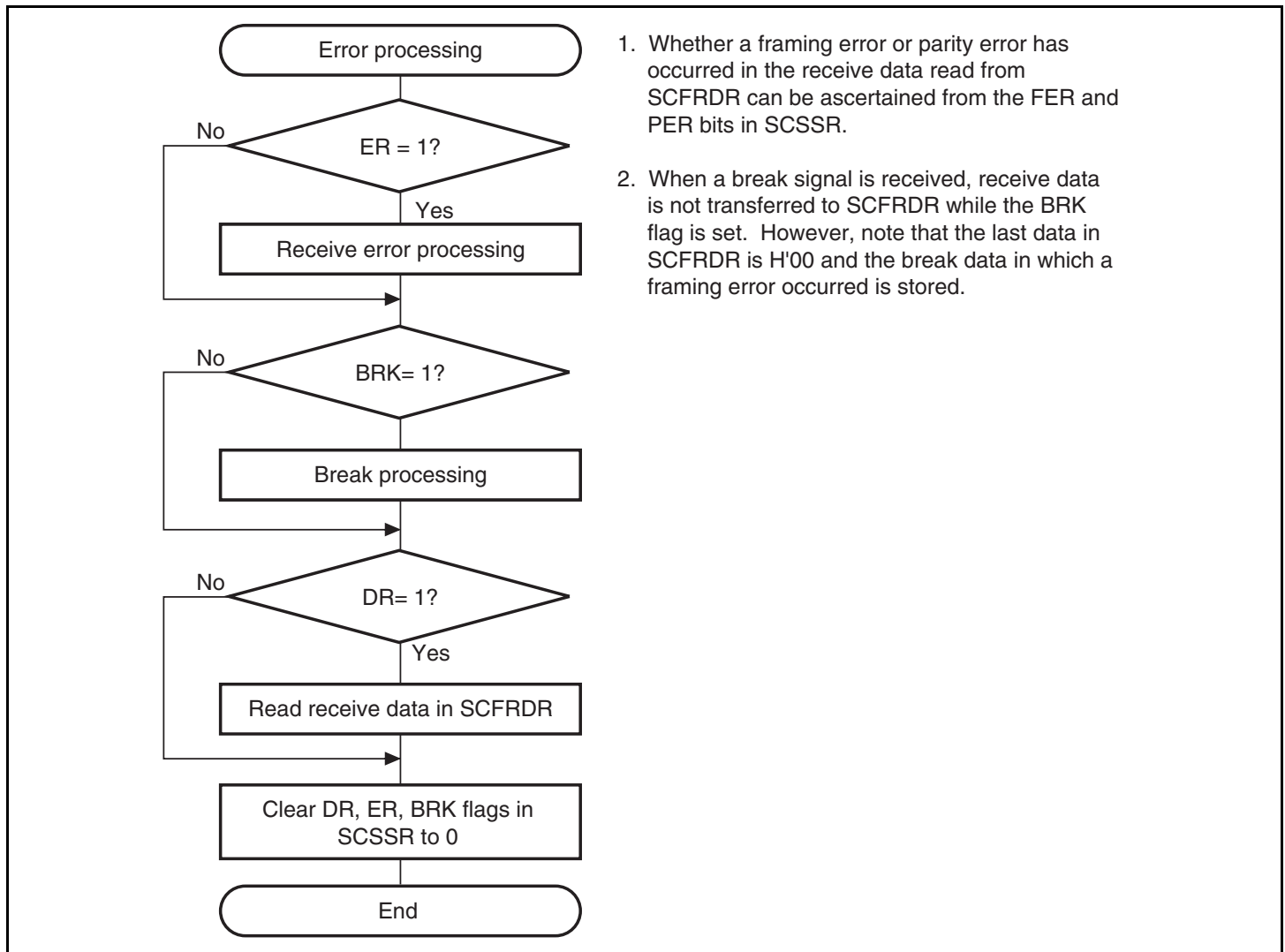
Figure 18.8 Sample Serial Reception Flowchart (2)
