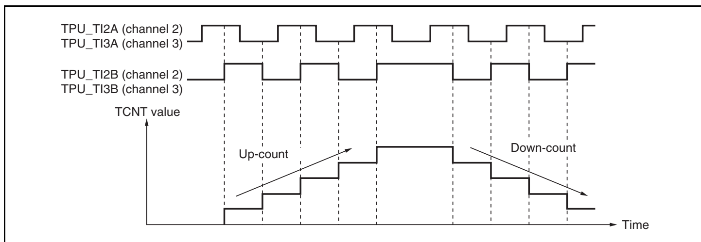
Figure 15.18 Example of Phase Counting Mode 4 Operation
