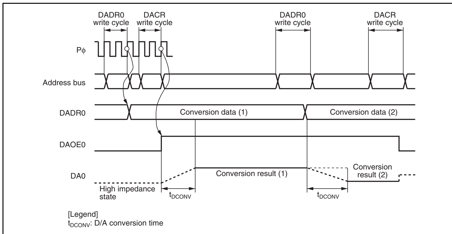
Figure 28.2 D/A Converter Operation Example
