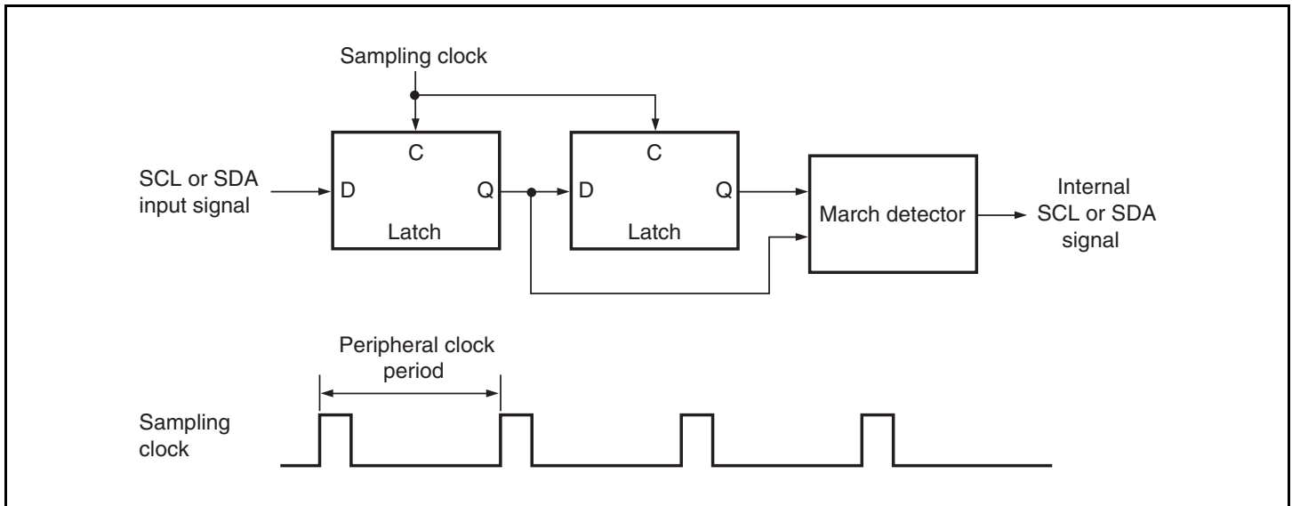
Figure 20.13 Block Diagram of Noise Canceller
