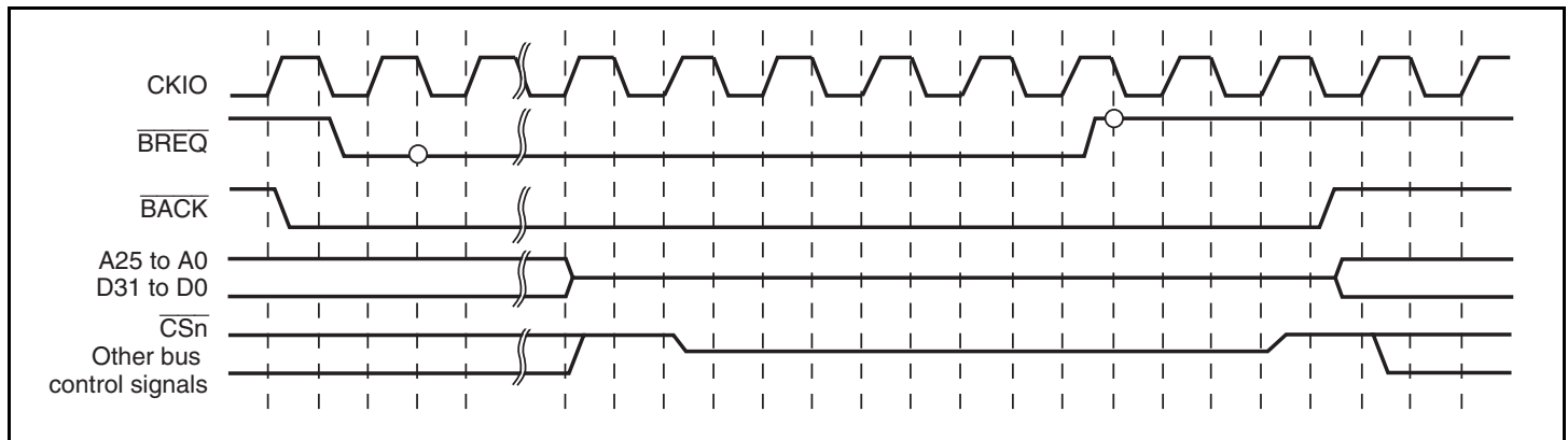
Figure 9.45 Bus Arbitration Timing
