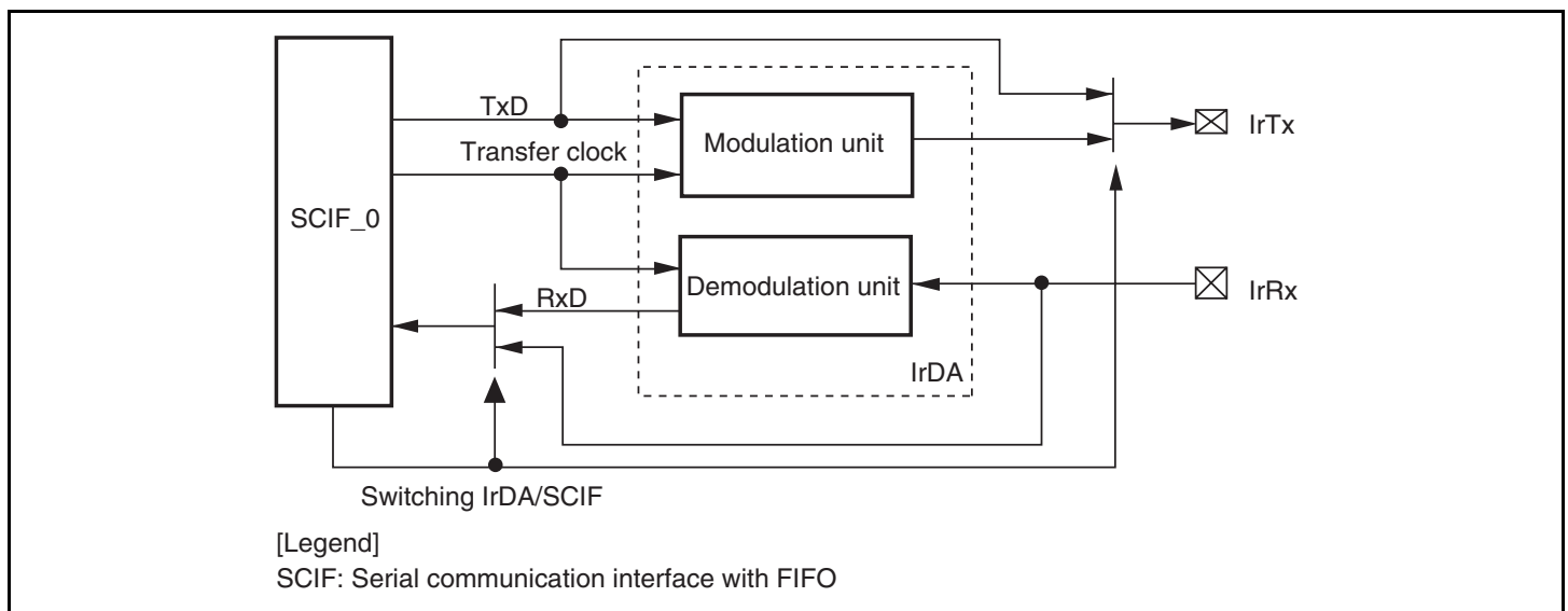
Figure 19.1 Block Diagram of IrDA
