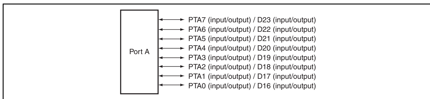
Figure 35.1 Port A
