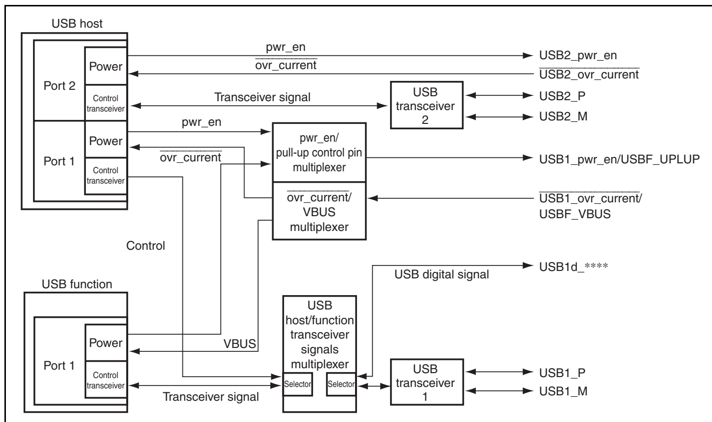
Figure 23.1 Block Diagram of USB PIN Multiplexer
