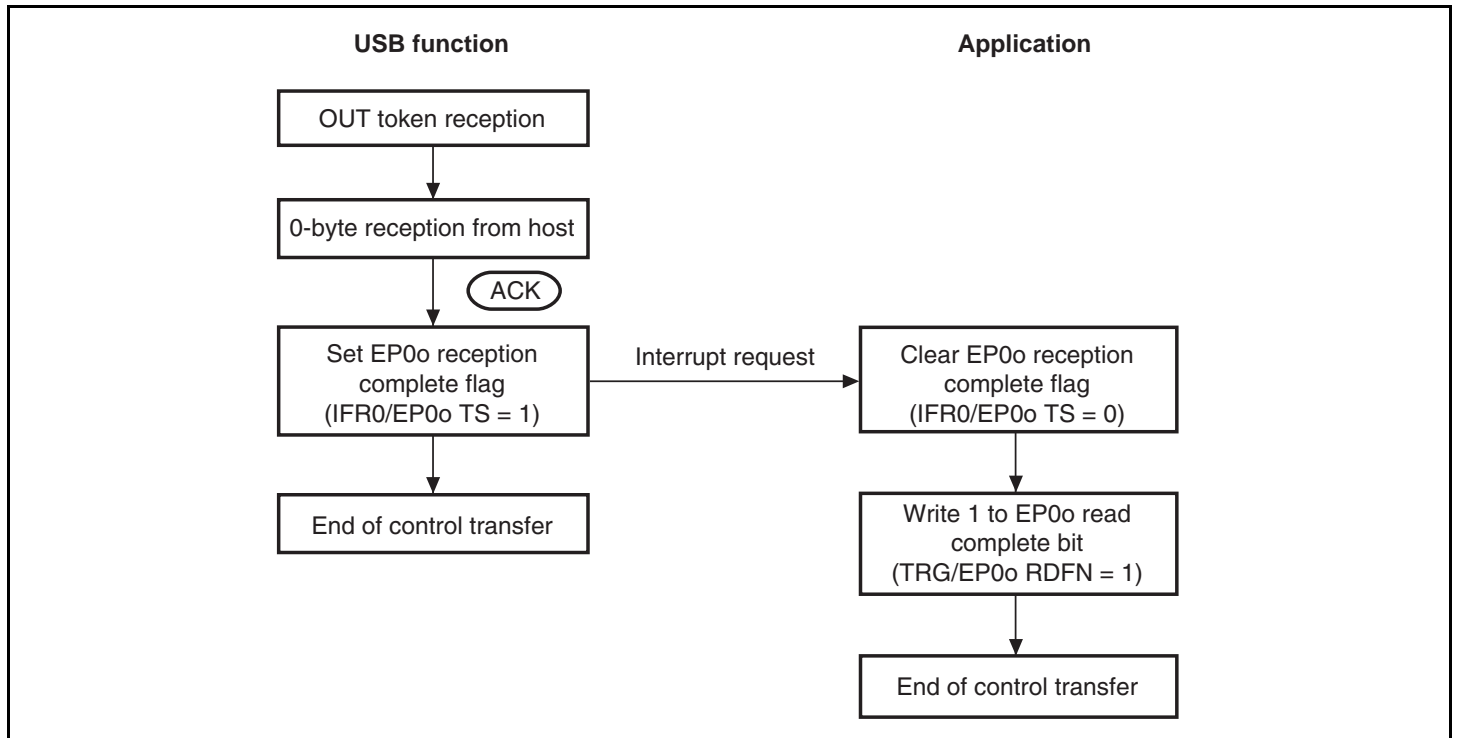
Figure 25.9 Status Stage (Control-In) Operation
