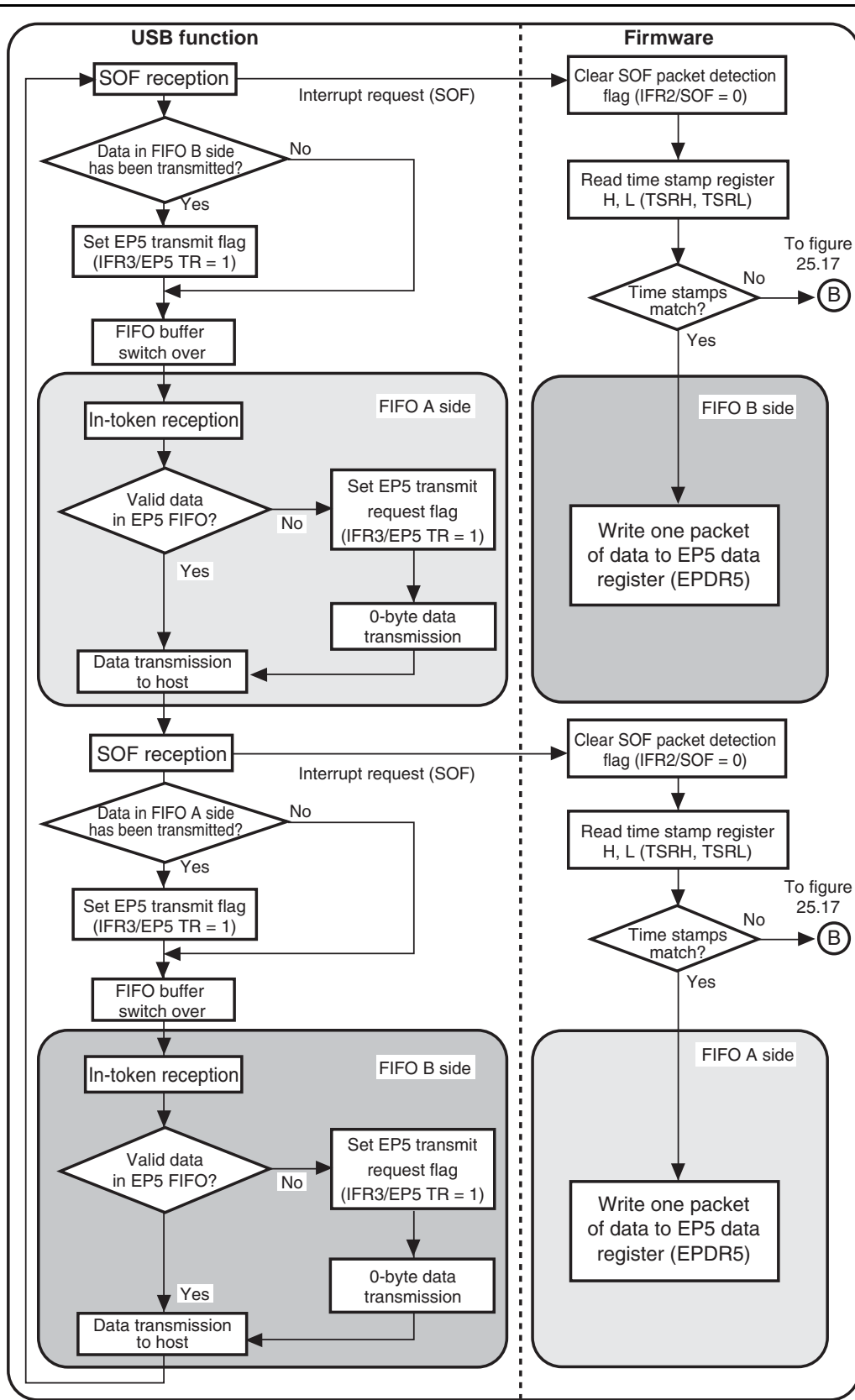
Figure 25.16 EP5 Isochronous-In Transfer Operation (SOF is Normal)
