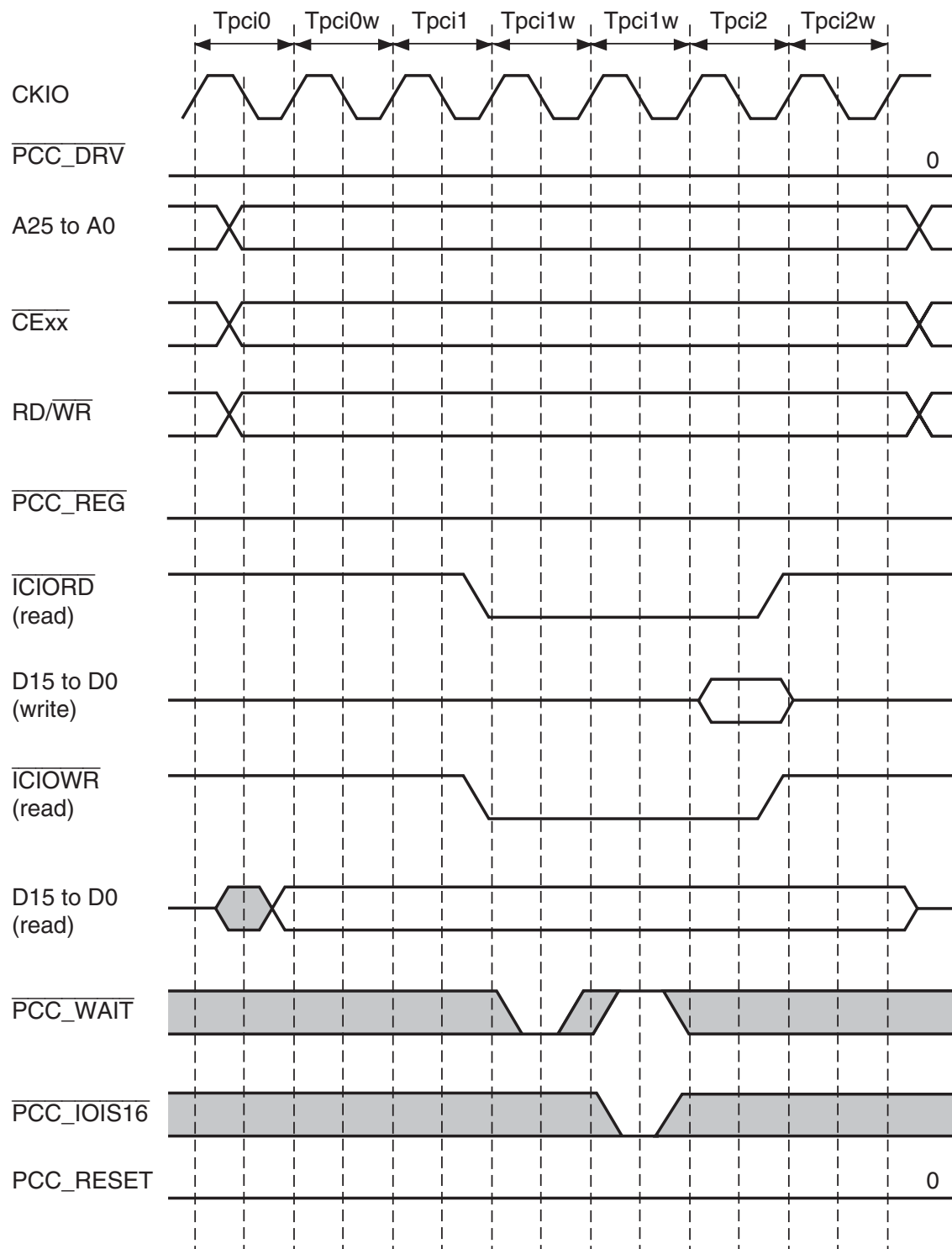
Figure 29.8 PCMCIA I/O Card Interface Wait Timing
