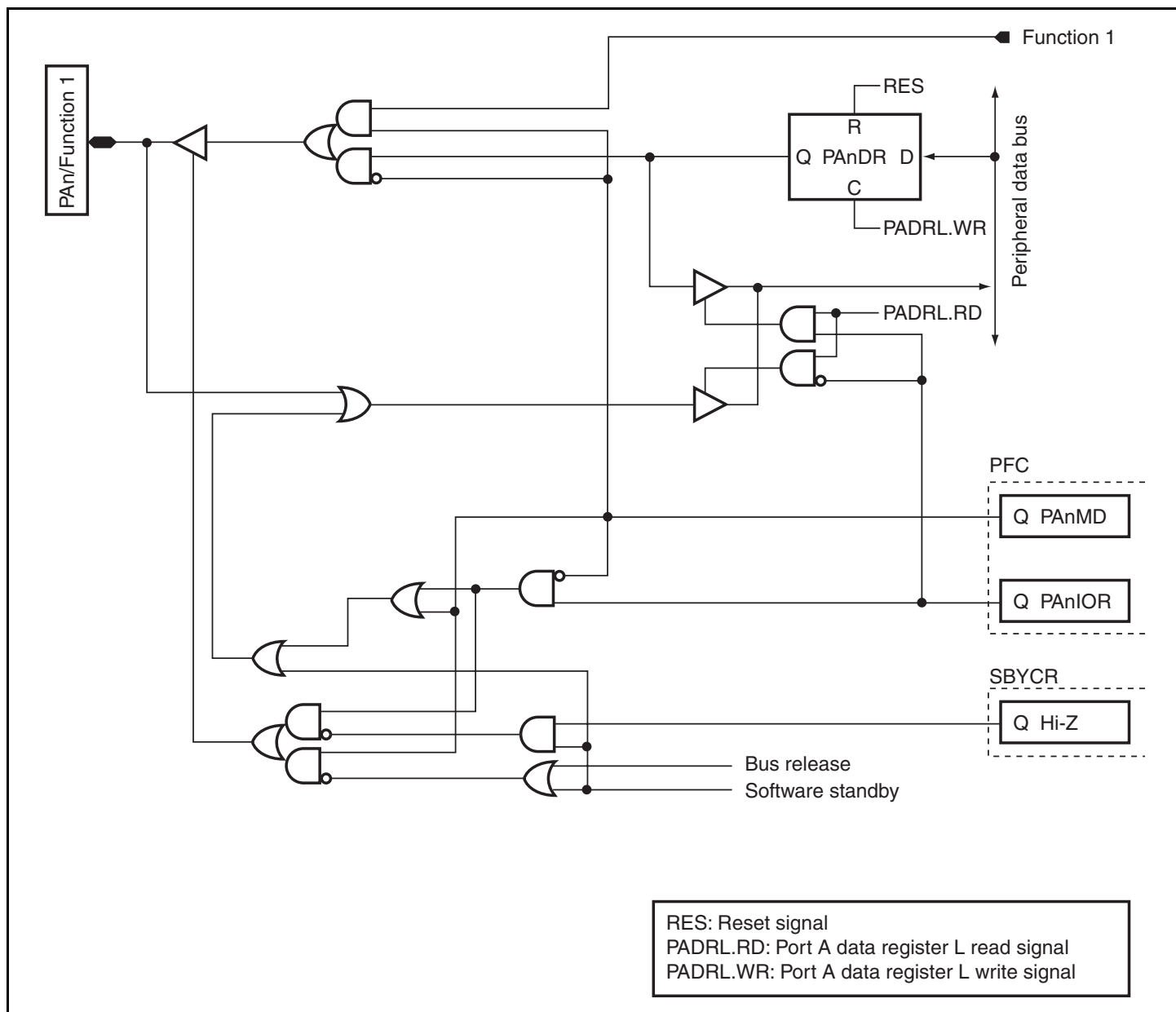
Figure D.6 PA n/Function 1
