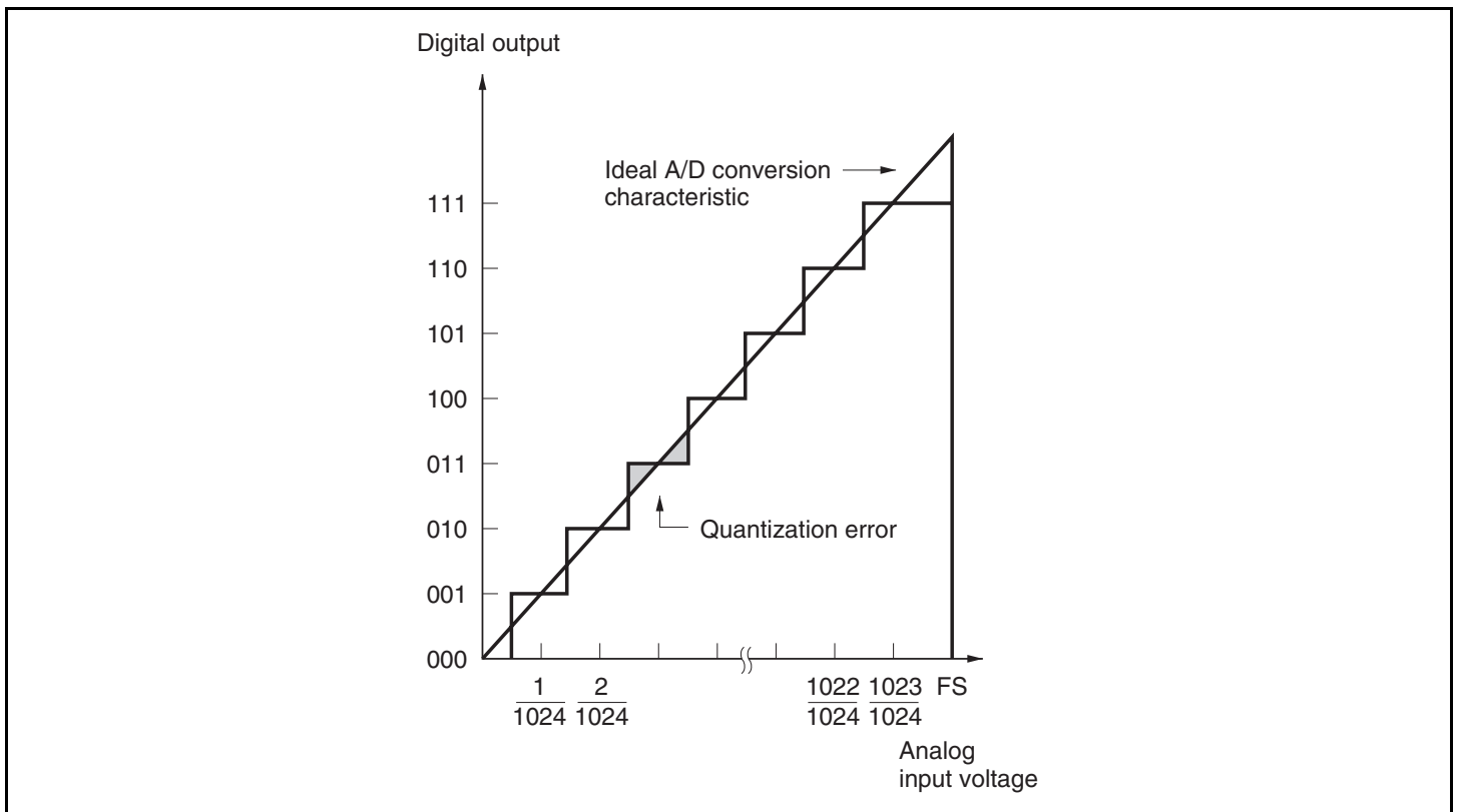
Figure 15.4 Definitions of A/D Conversion Accuracy
