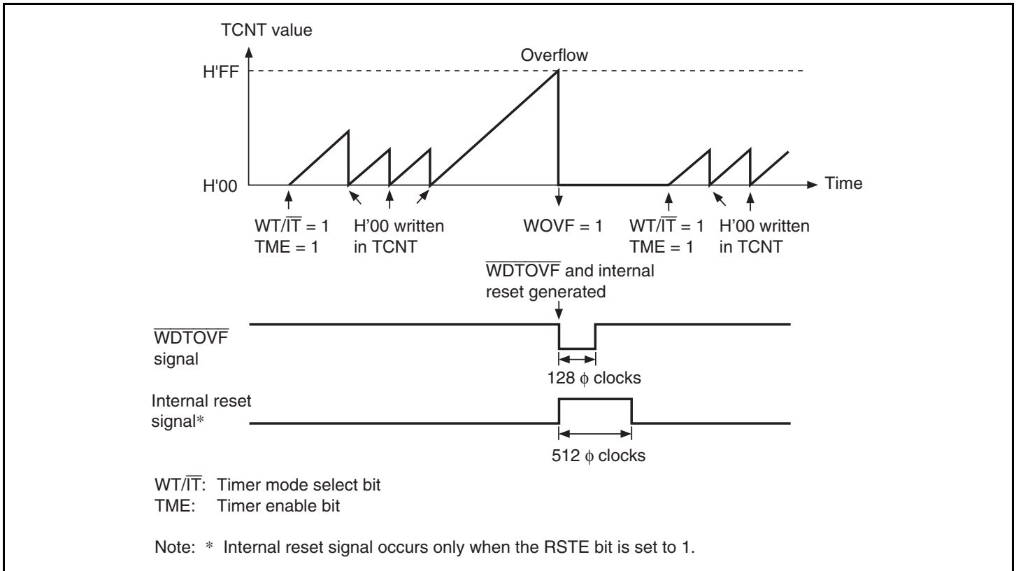
Figure 12.2 Operation in Watchdog Timer Mode
