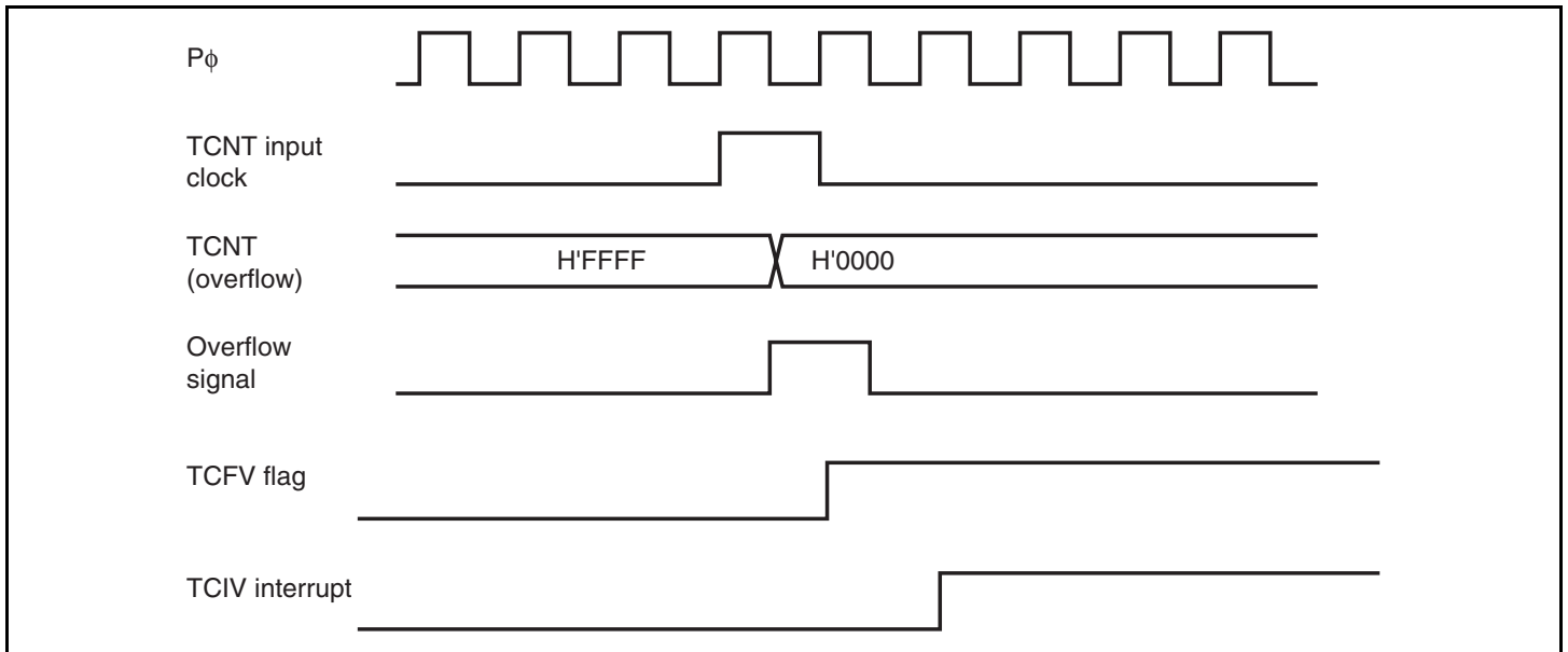
Figure 11.66 TCIV Interrupt Setting Timing
