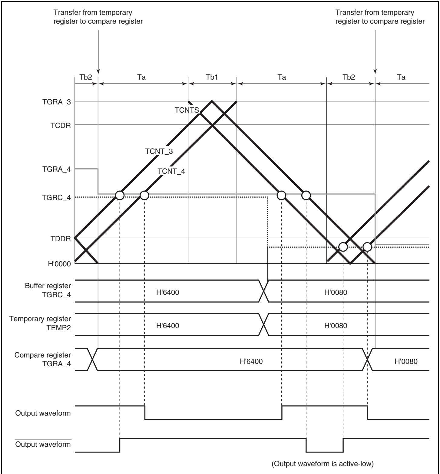
Figure 11.35 Example of Complementary PWM Mode Operation
