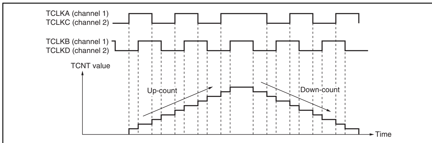
Figure 11.25 Example of Phase Counting Mode 1 Operation
