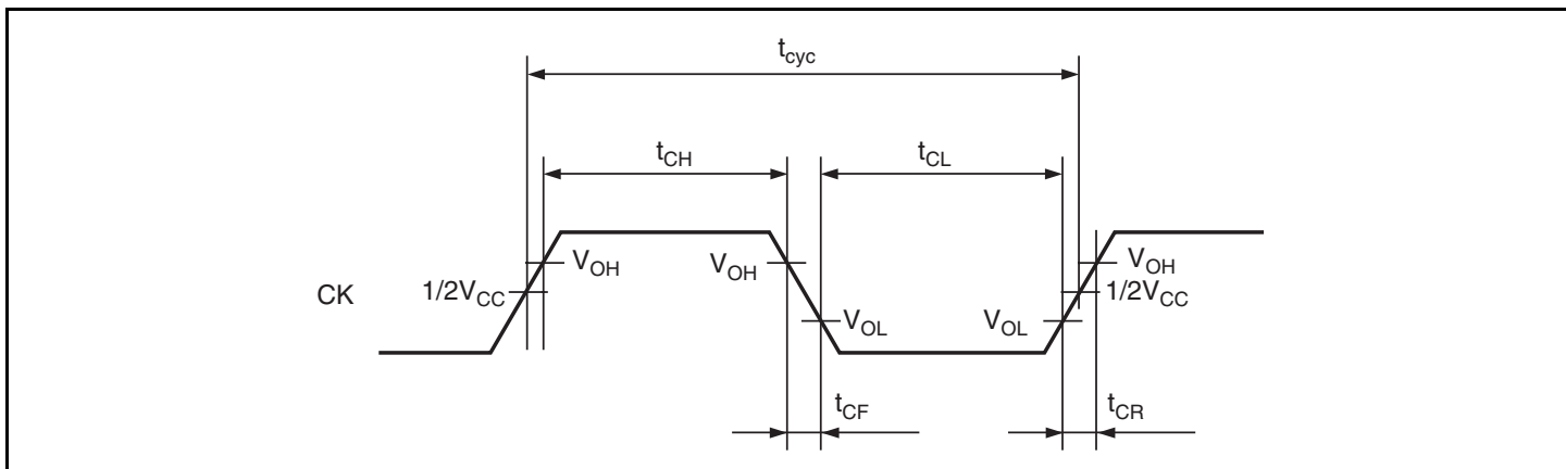
Figure 26.2 System Clock Timing
