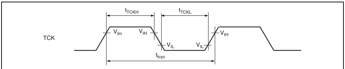
Figure 26.24 H-UDI Clock Timing
