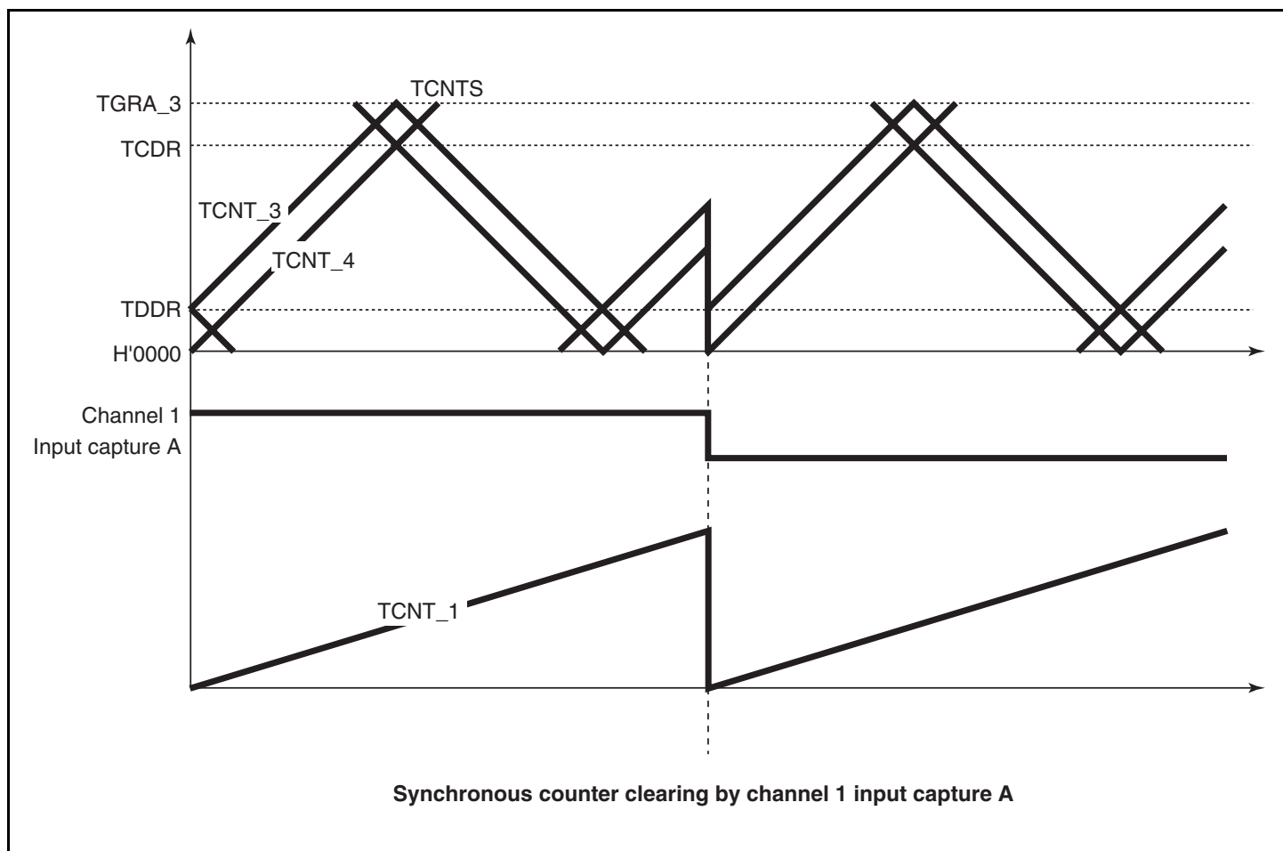
Figure 11.49 Counter Clearing Synchronized with Another Channel
