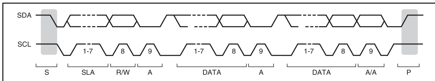
Figure 14.5 I 2 C Bus Timing
