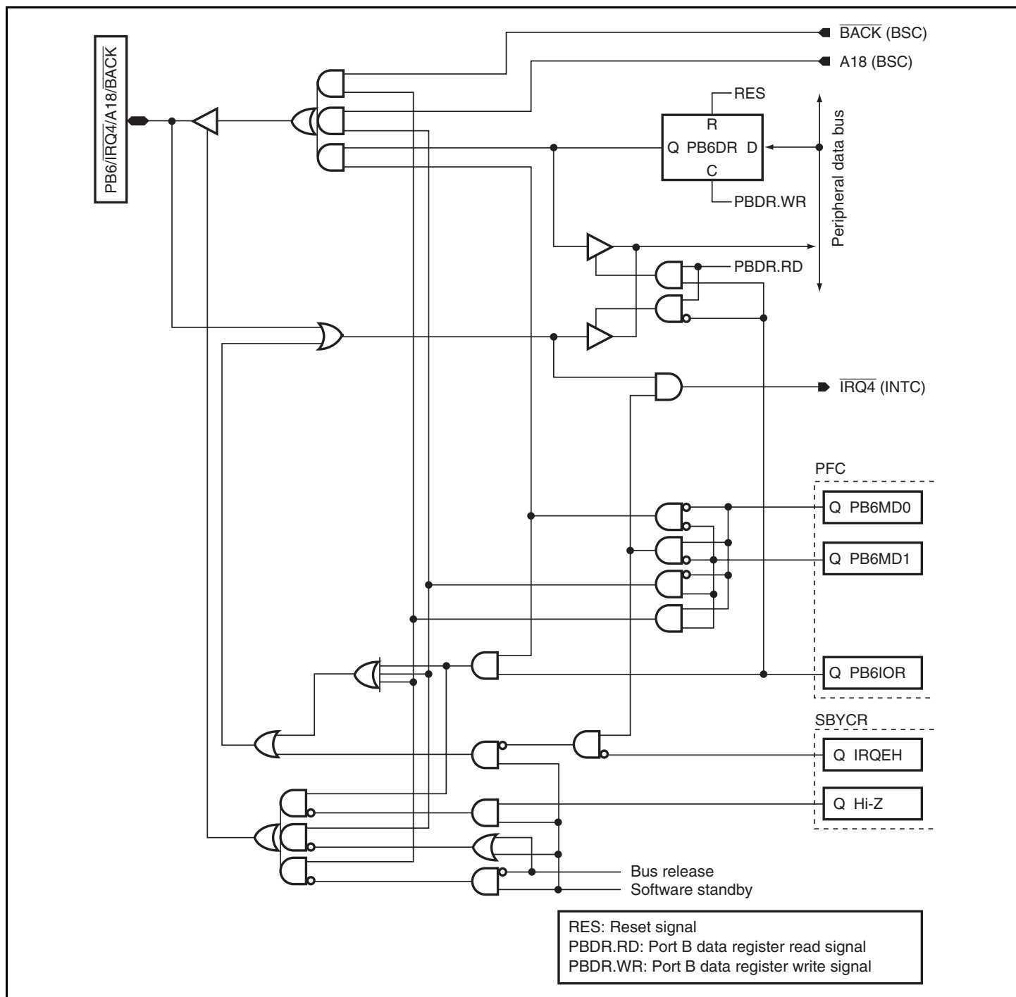
Figure D.18 PB6/IRQ4/A18/BACK
