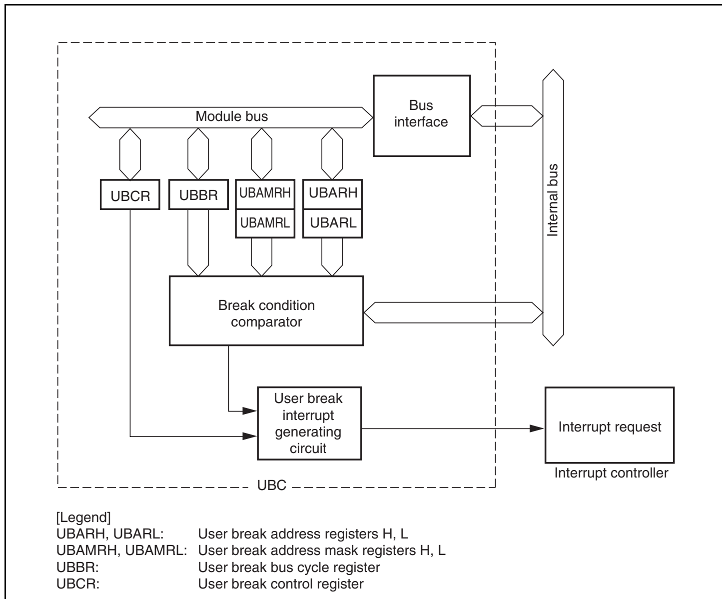
Figure 7.1 User Break Controller Block Diagram
