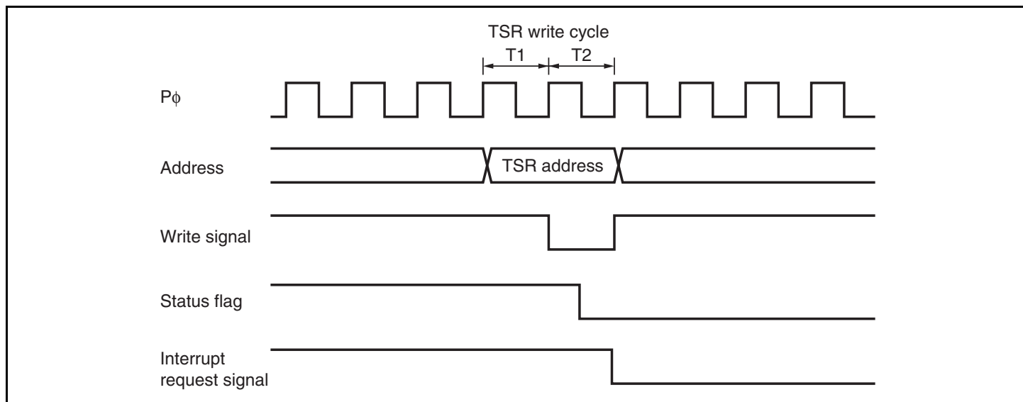
Figure 11.68 Timing for Status Flag Clearing by CPU
