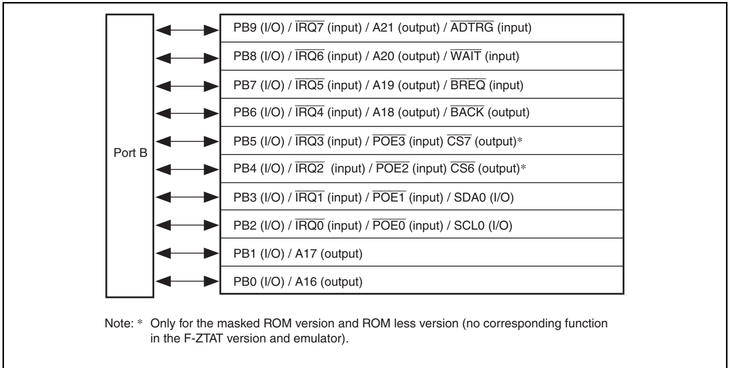
Figure 18.3 Port B
