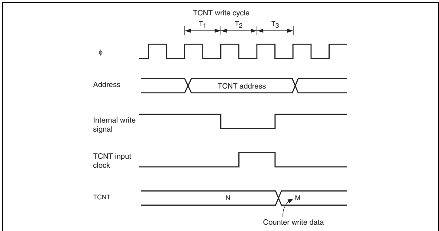
Figure 12.8 Contention between TCNT Write and Increment
