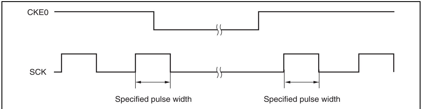
Figure 13.29 Timing for Fixing Clock Output Level
