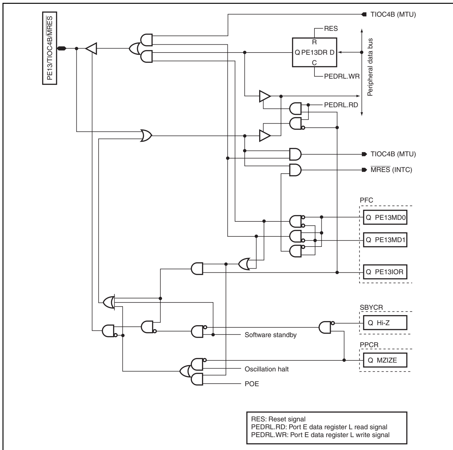
Figure D.40 PE13/TIOC4B/MRES
