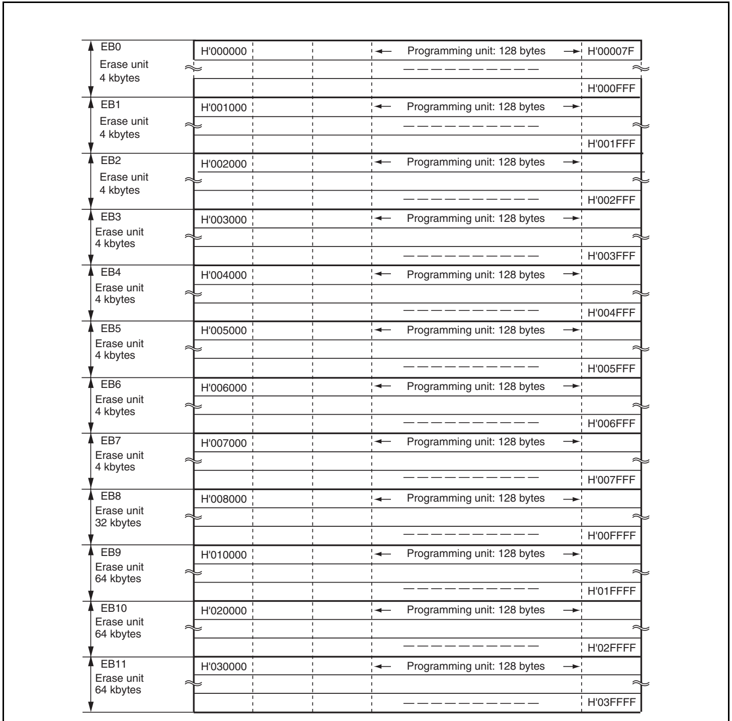
Figure 19.5 Flash Memory Block Configuration
