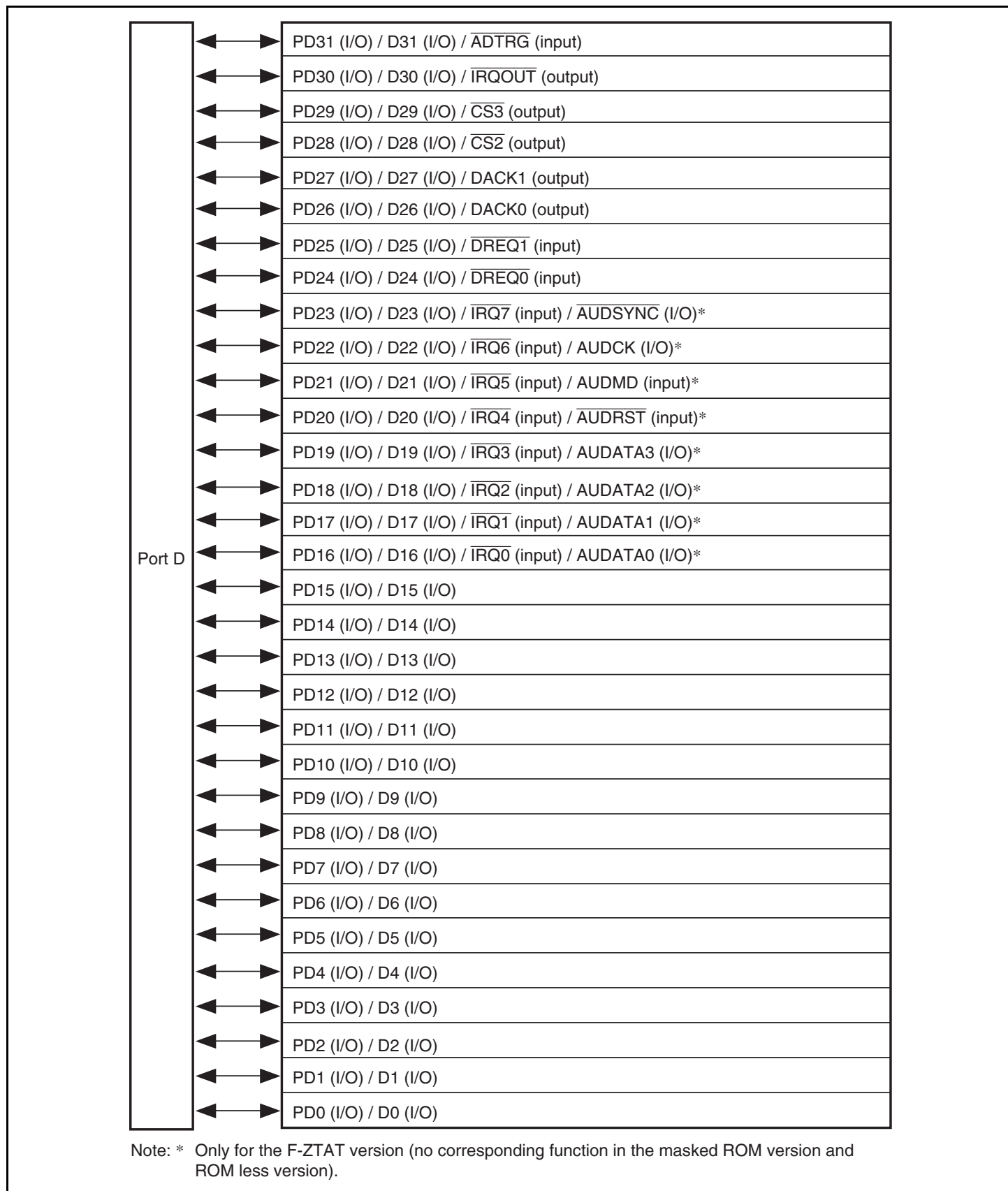
Figure 18.6 Port D (SH7145)
