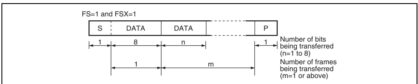
Figure 14.4 I 2 C Bus Data Format (Serial Format)
