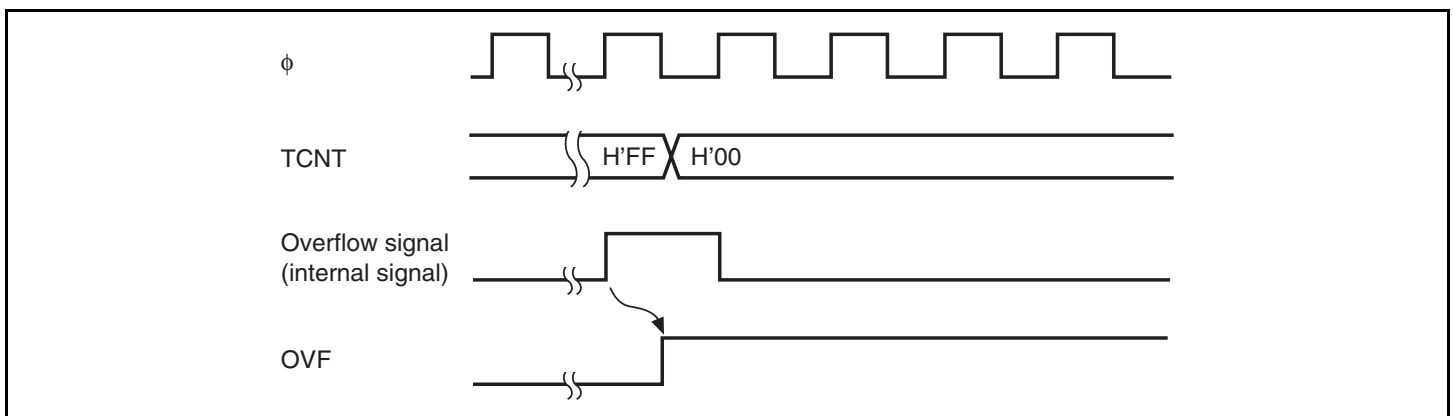
Figure 12.4 Timing of Setting OVF
