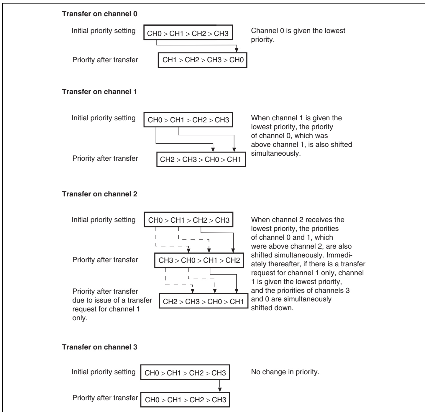
Figure 10.3 (1) Round Robin Mode
