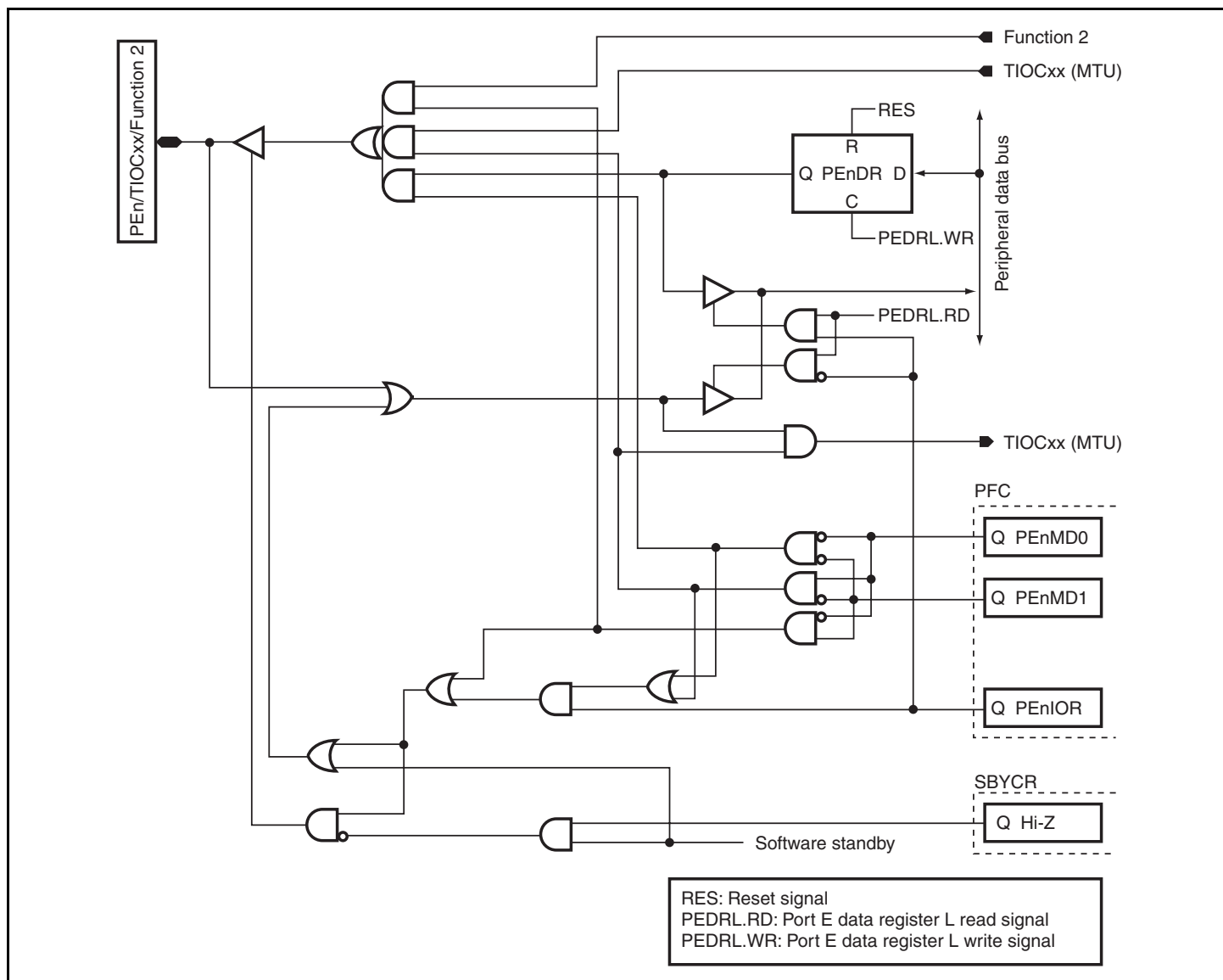
Figure D.35 PEn/TIOCxx/Function 2
