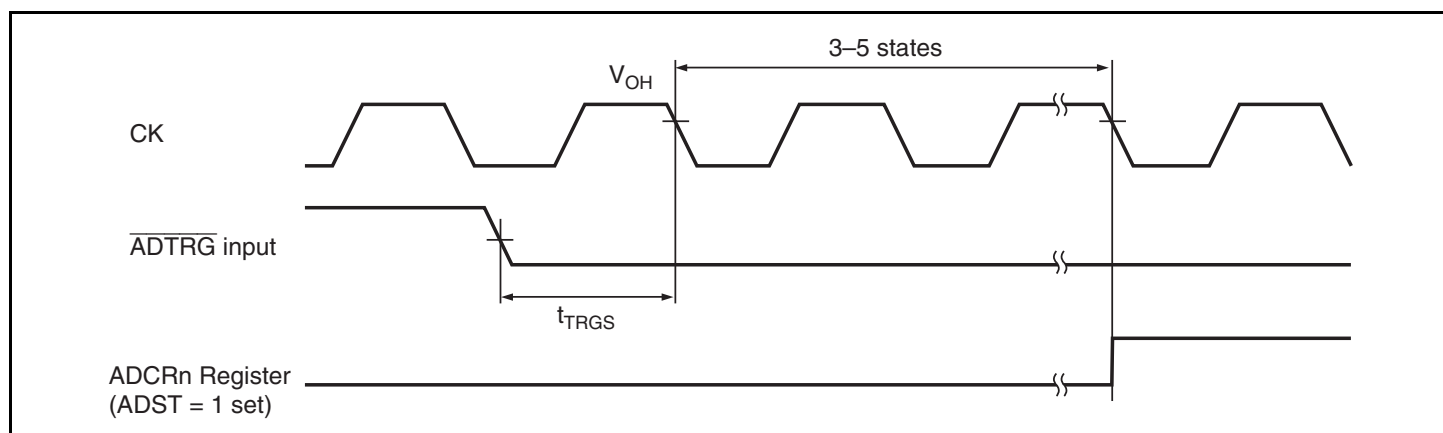
Figure 26.23 External Trigger Input Timing
