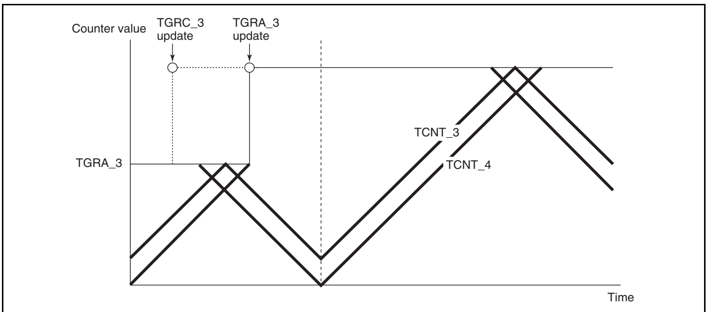
Figure 11.36 Example of PWM Cycle Updating
