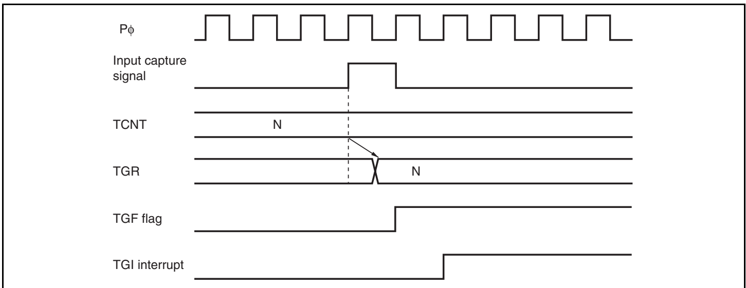
Figure 11.65 TGI Interrupt Timing (Input Capture)
