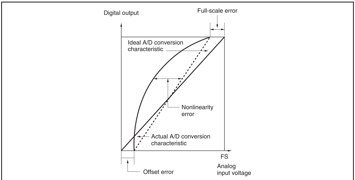
Figure 15.5 Definitions of A/D Conversion Accuracy
