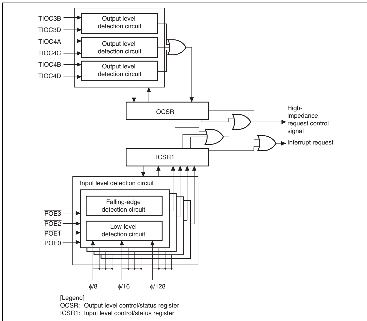
Figure 11.114 POE Block Diagram
