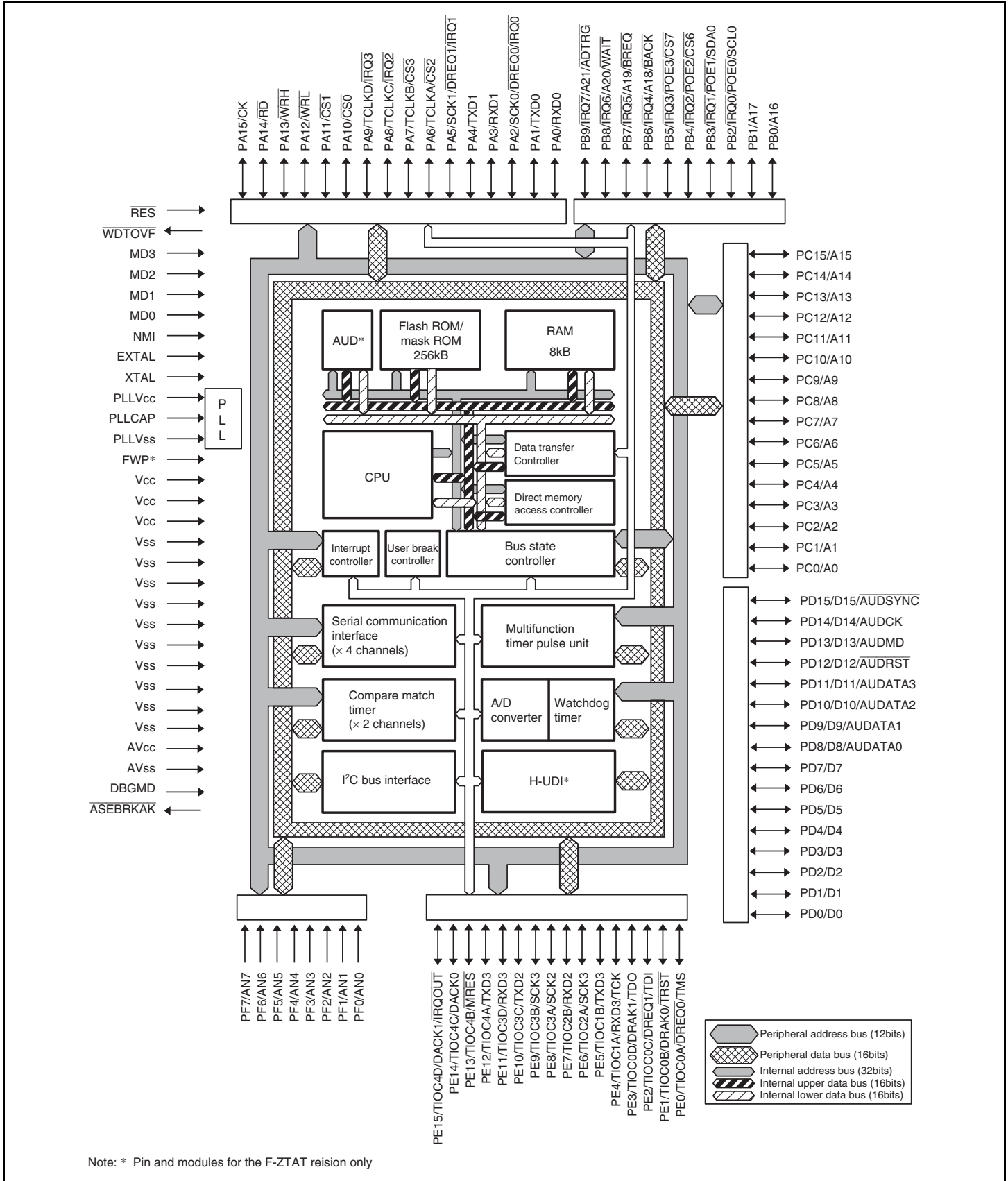
Figure 1.1 Internal Block Diagram of SH7144
