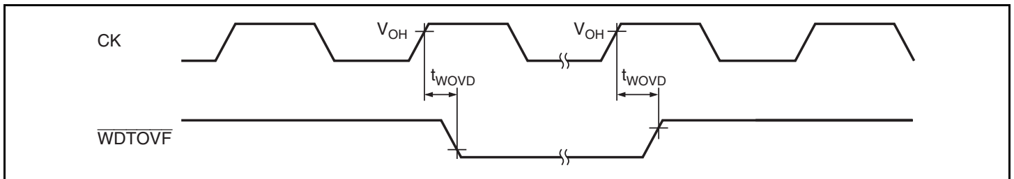
Figure 26.18 WDT Timing
