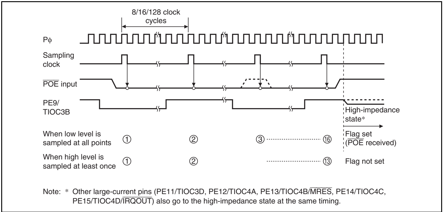
Figure 11.115 Low-Level Detection Operation
