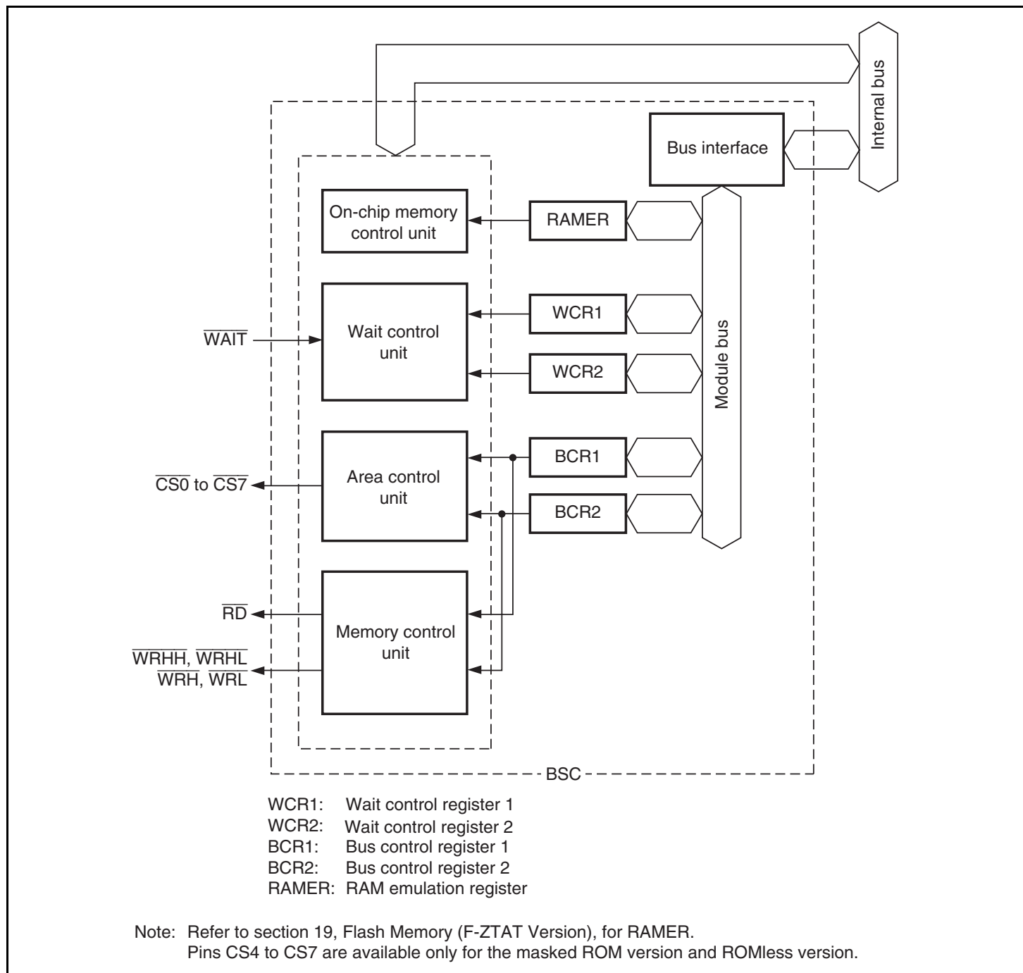
Figure 9.1 BSC Block Diagram
