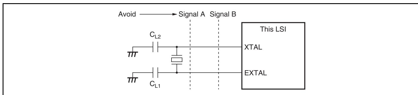
Figure 4.5 Cautions for Oscillator Circuit Board Design
