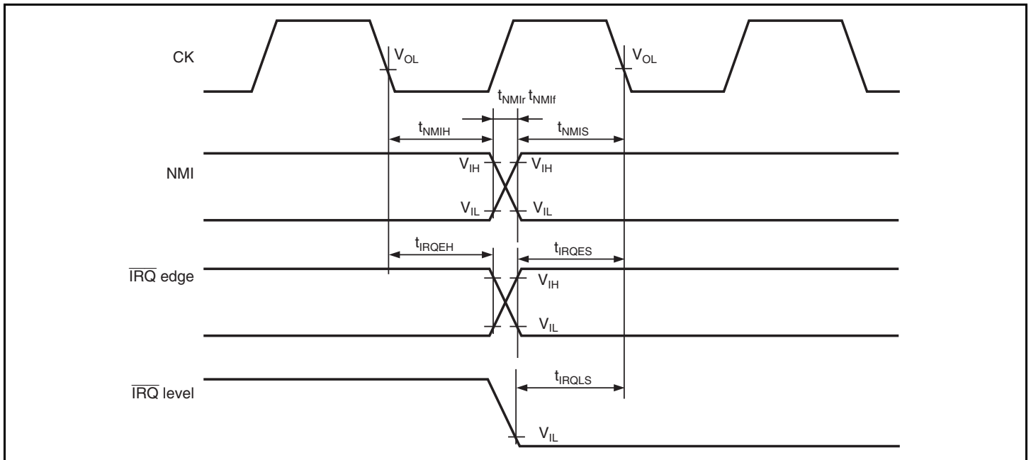
Figure 26.6 Interrupt Signal Input Timing
