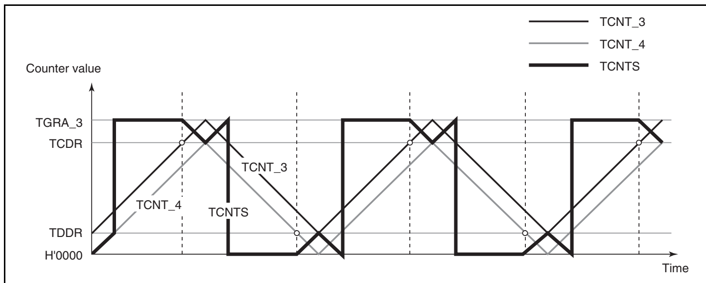
Figure 11.34 Complementary PWM Mode Counter Operation
