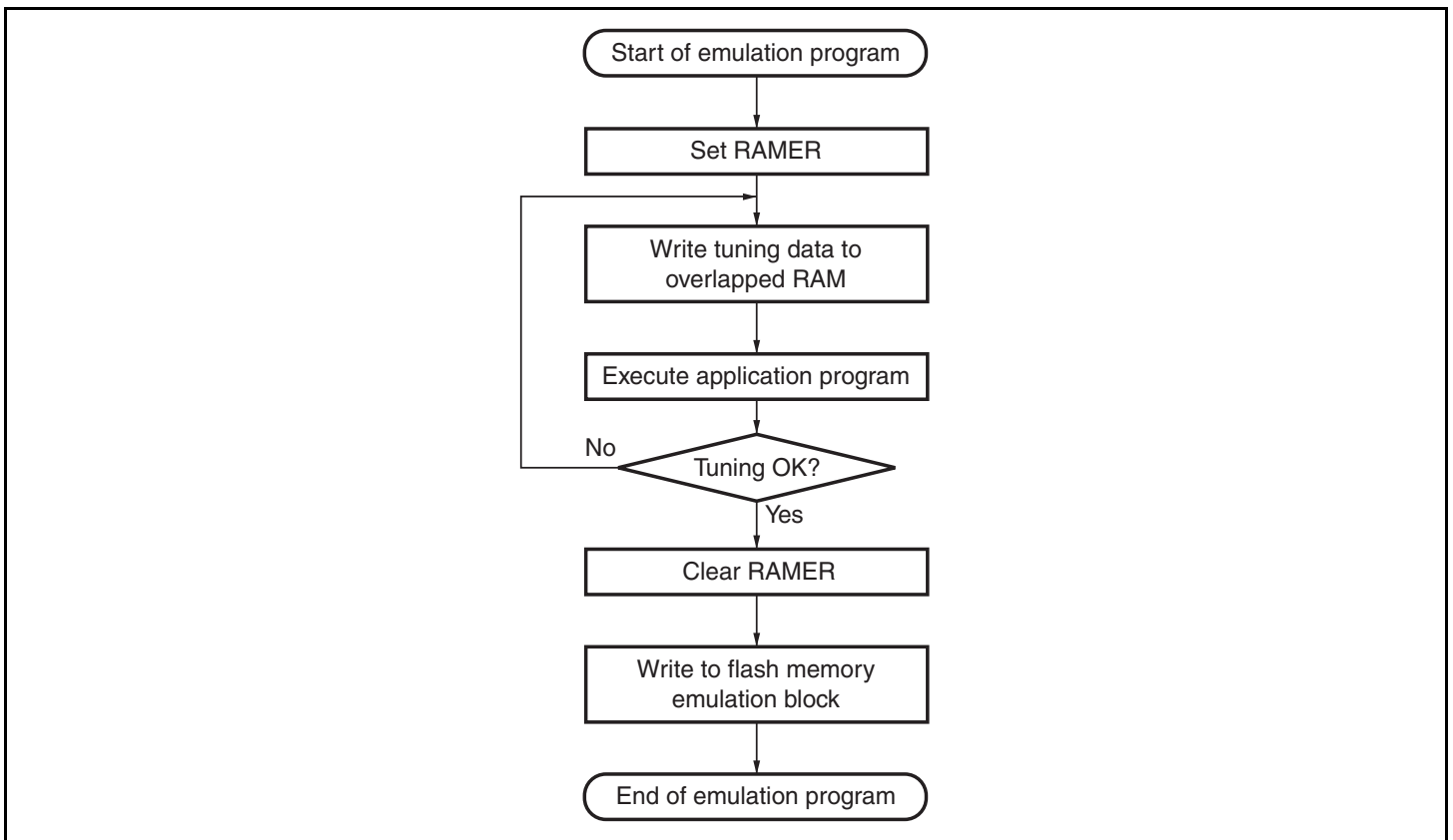
Figure 19.7 Flowchart for Flash Memory Emulation in RAM
