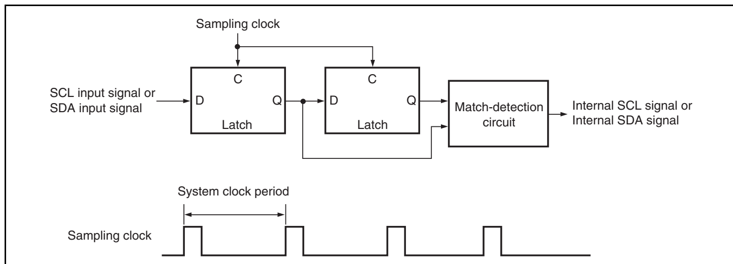
Figure 14.28 Block Diagram of the Noise Canceller
