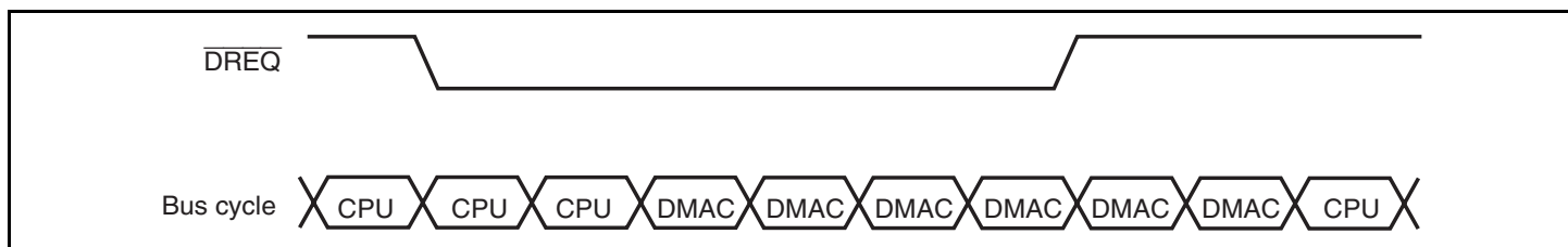
Figure 10.12 DMA Transfer Example in Burst Mode
