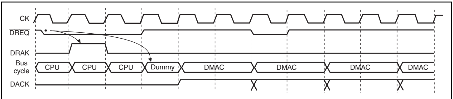
Figure 10.23 Burst Mode, Single Address and Edge Detection
