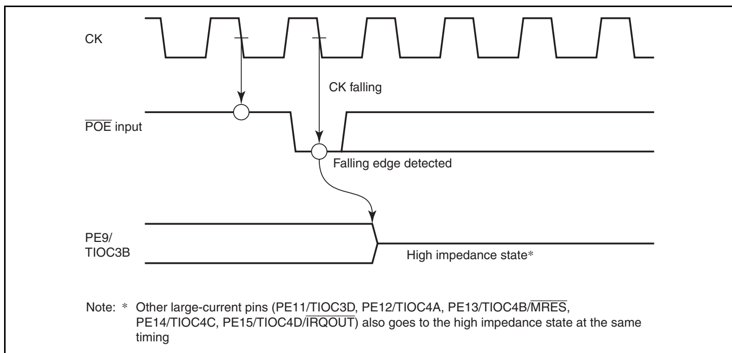
Figure 11.117 Falling Edge Detection Operation
