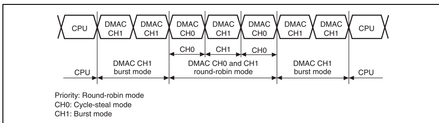
Figure 10.13 Bus Handling when Multiple Channels Are Operating
