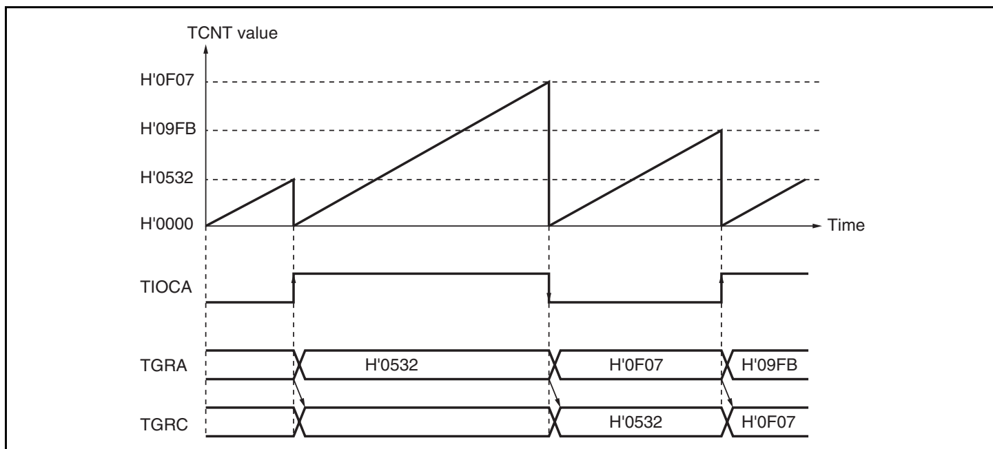
Figure 11.17 Example of Buffer Operation (2)
