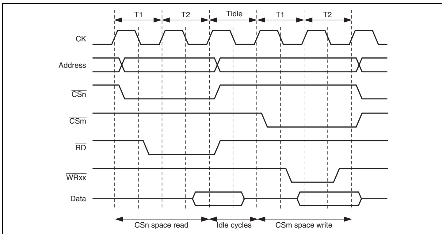
Figure 9.7 Example of Idle Cycle Insertion
