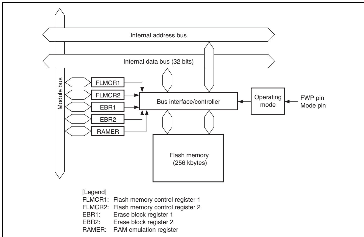
Figure 19.1 Block Diagram of Flash Memory
