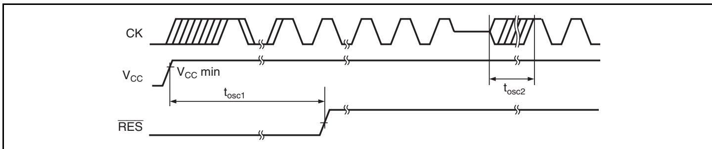
Figure 26.4 Oscillation Settling Time
