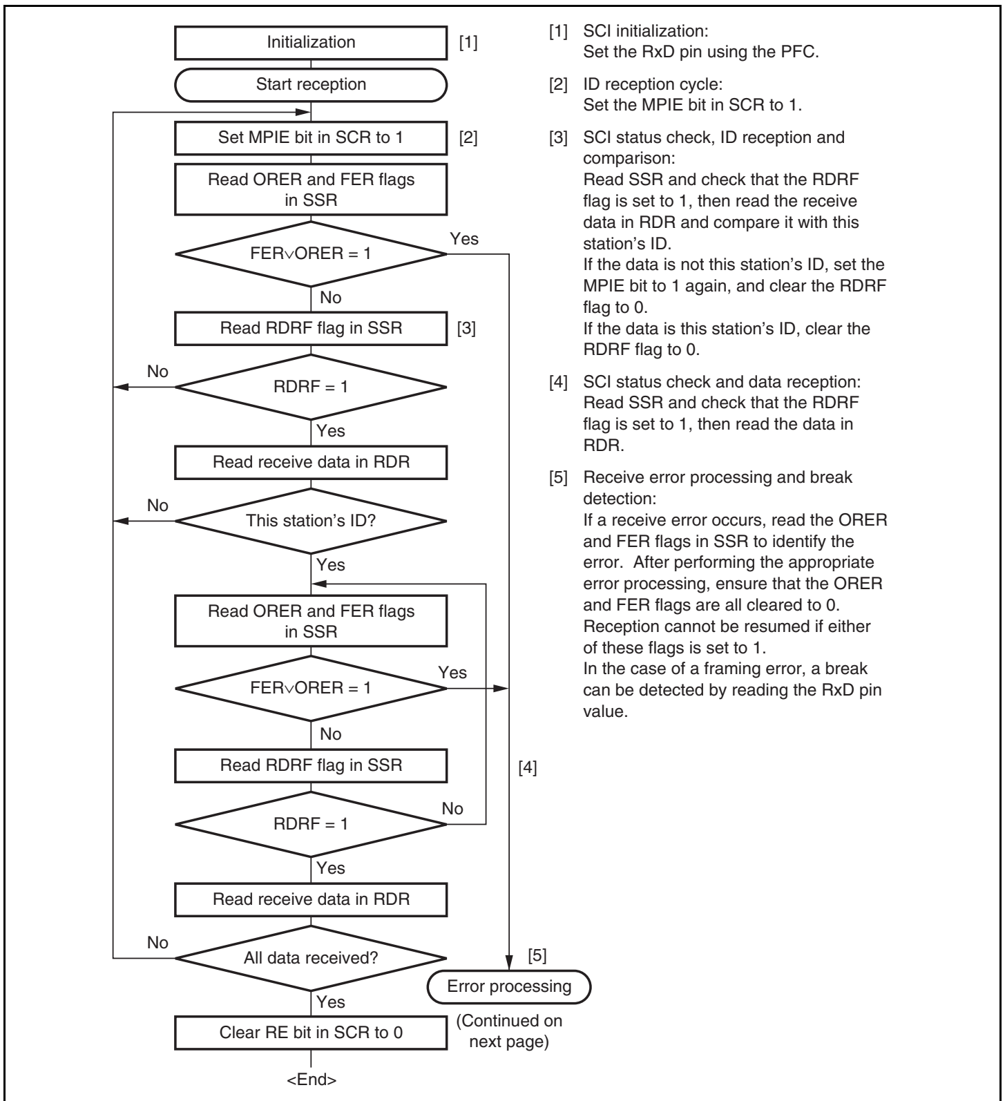
Figure 13.13 Sample Multiprocessor Serial Reception Flowchart (1)
