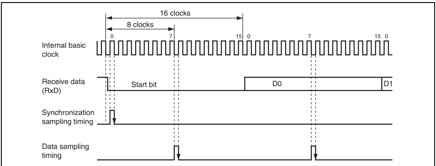
Figure 13.3 Receive Data Sampling Timing in Asynchronous Mode
