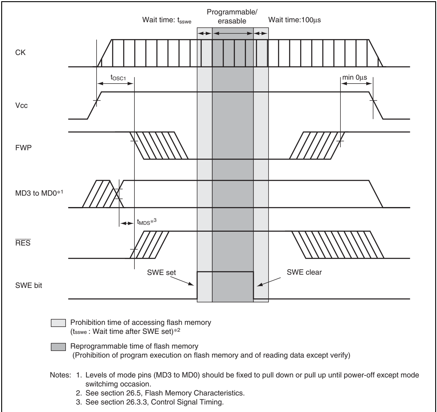
Figure 19.12 Power On/Off Timing (User Program Mode)
