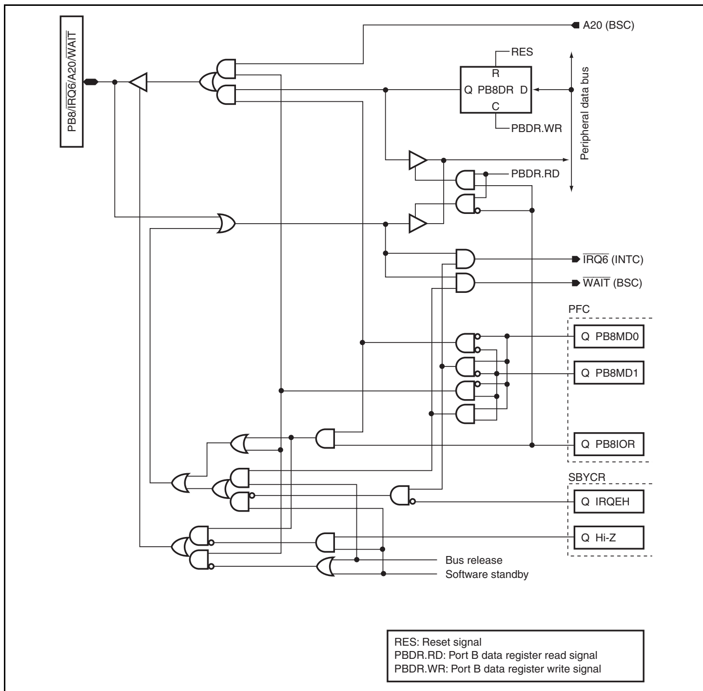
Figure D.20 PB8/ \overline{\text{IRQ6}} /A20/ \overline{\text{WAIT}}
