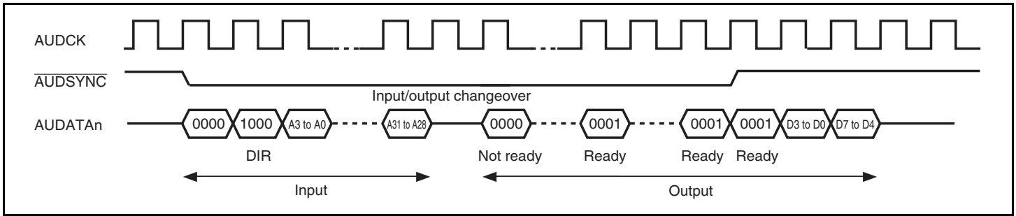
Figure 23.5 Example of Read Operation (Byte Read)
