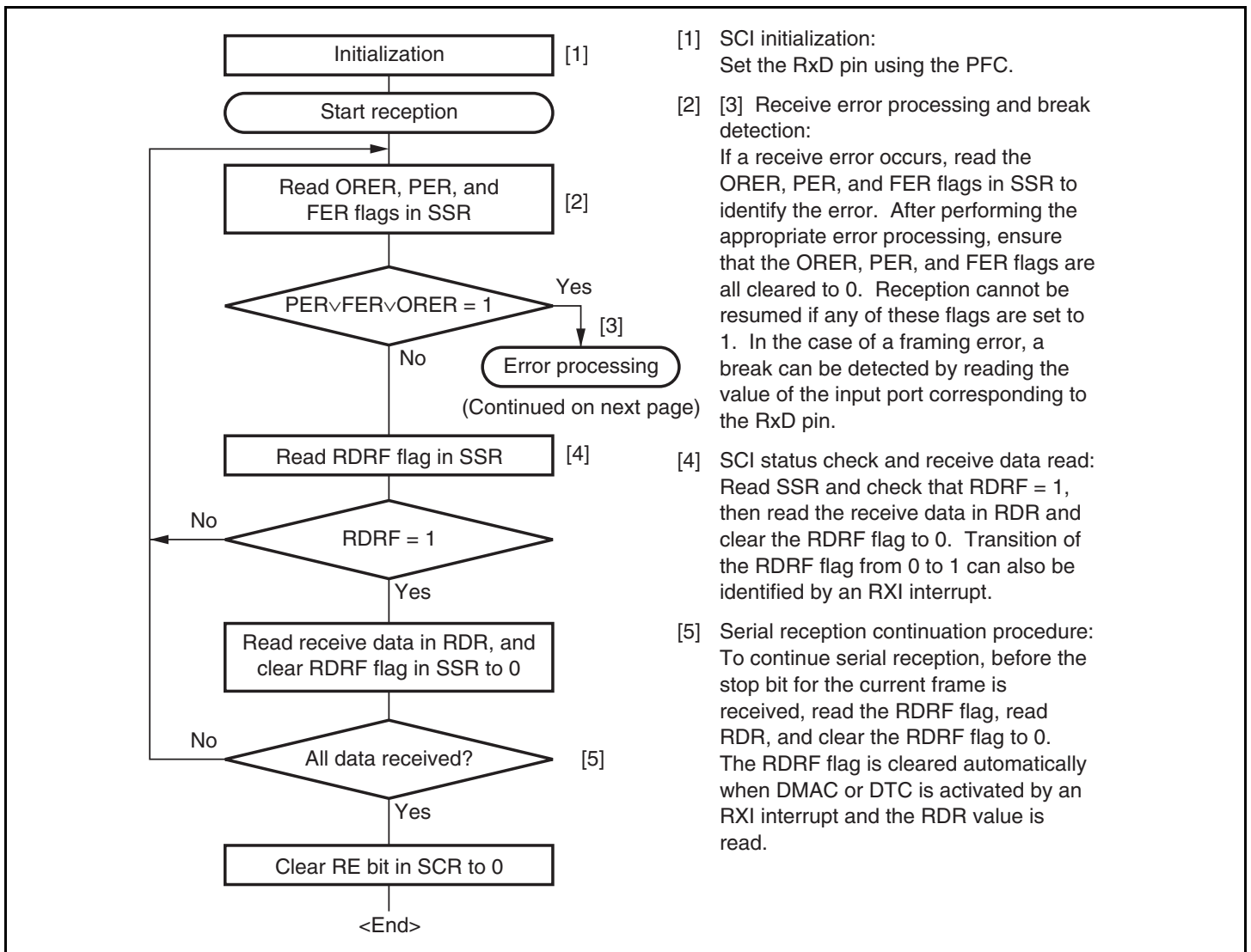
Figure 13.9 Sample Serial Reception Data Flowchart (1)
