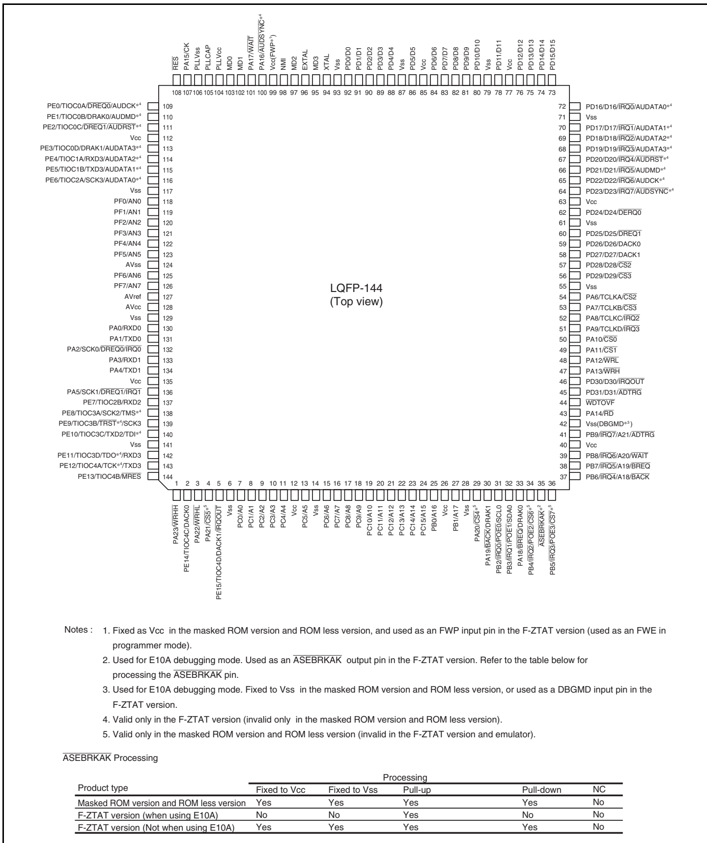
Figure 1.4 SH7145 Pin Arrangement
