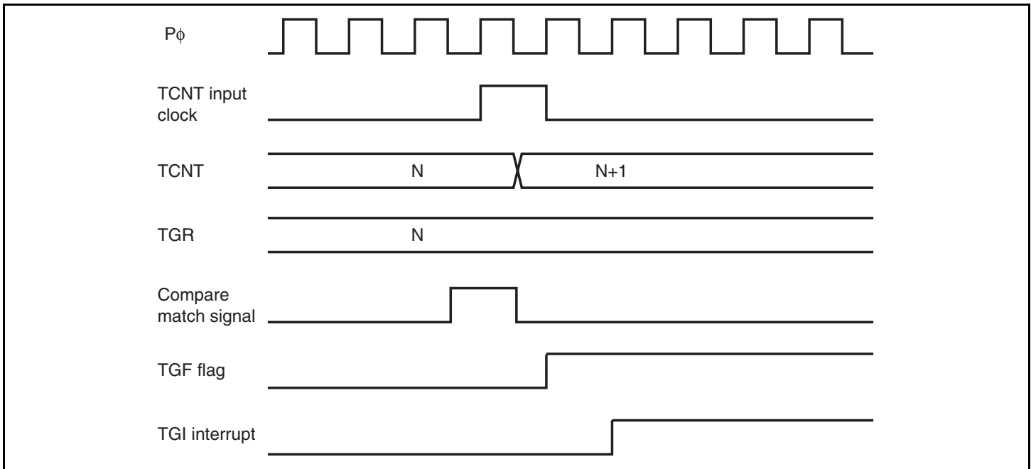
Figure 11.64 TGI Interrupt Timing (Compare Match)
