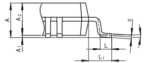
Detail F
