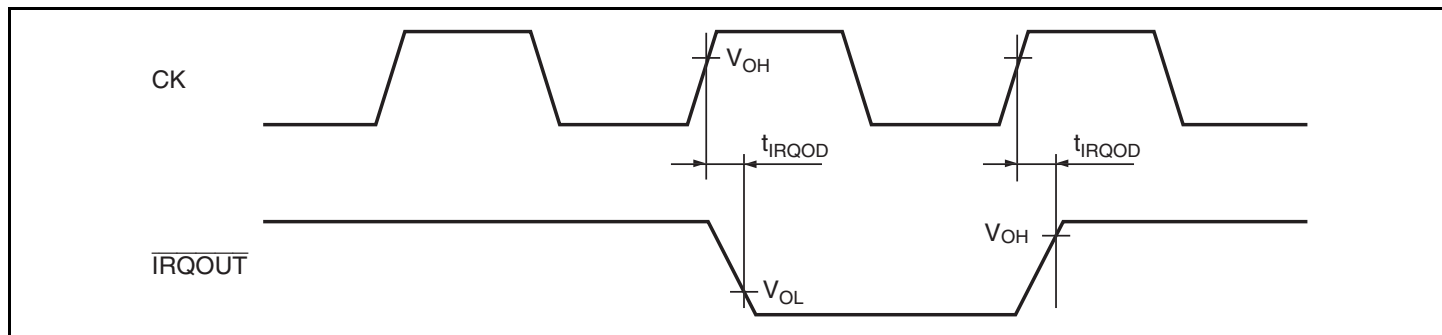
Figure 26.7 Interrupt Signal Output Timing
