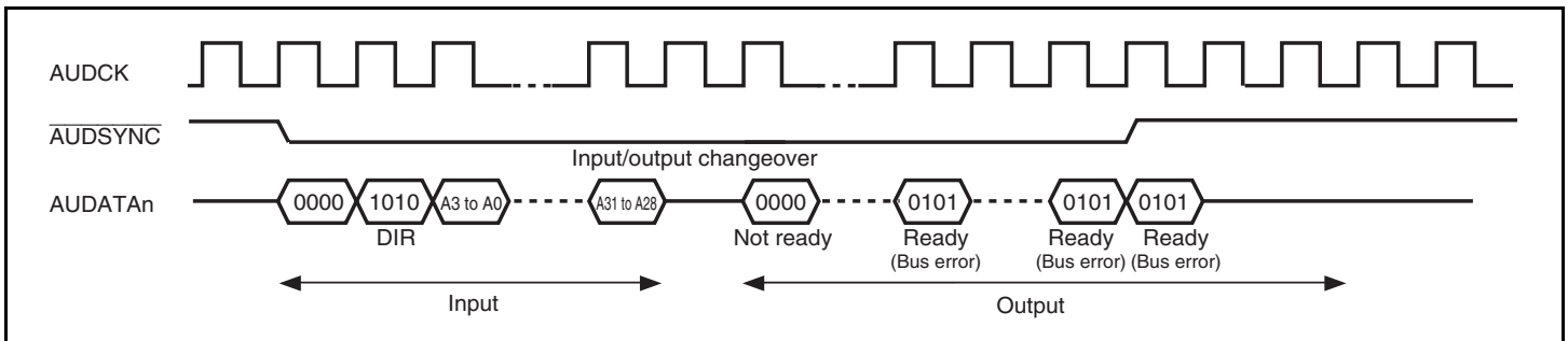
Figure 23.7 Example of Error Occurrence (Longword Read)
