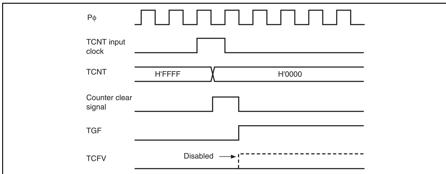
Figure 11.83 Contention between Overflow and Counter Clearing
