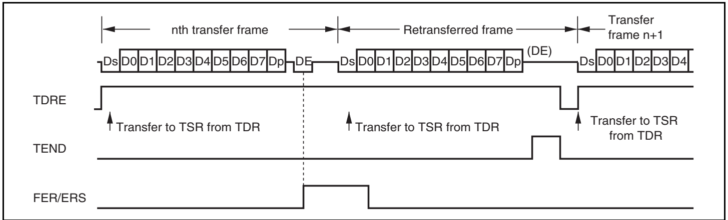
Figure 13.26 Retransfer Operation in SCI Transmit Mode
