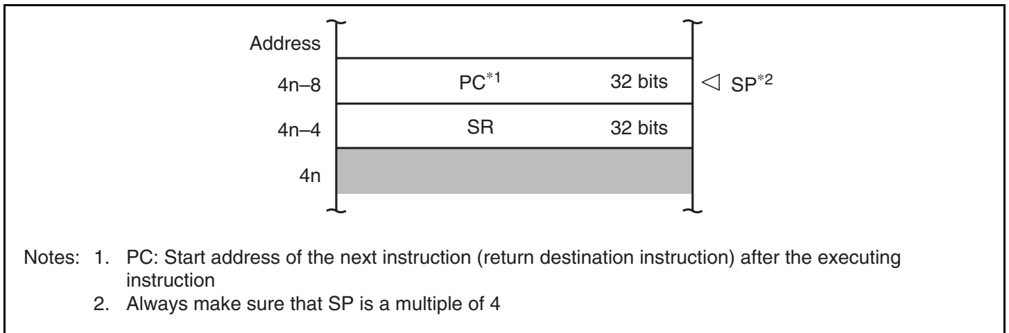
Figure 6.4 Stack after Interrupt Exception Processing
