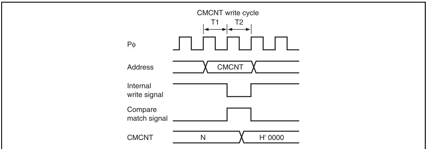
Figure 16.6 CMCNT Write and Compare Match Contention
