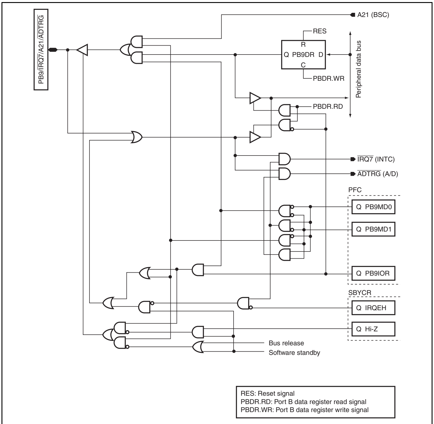
Figure D.21 \overline{\text{PB9}}/\overline{\text{IRQ7}}/\overline{\text{A21}}/\overline{\text{ADTRG}}
