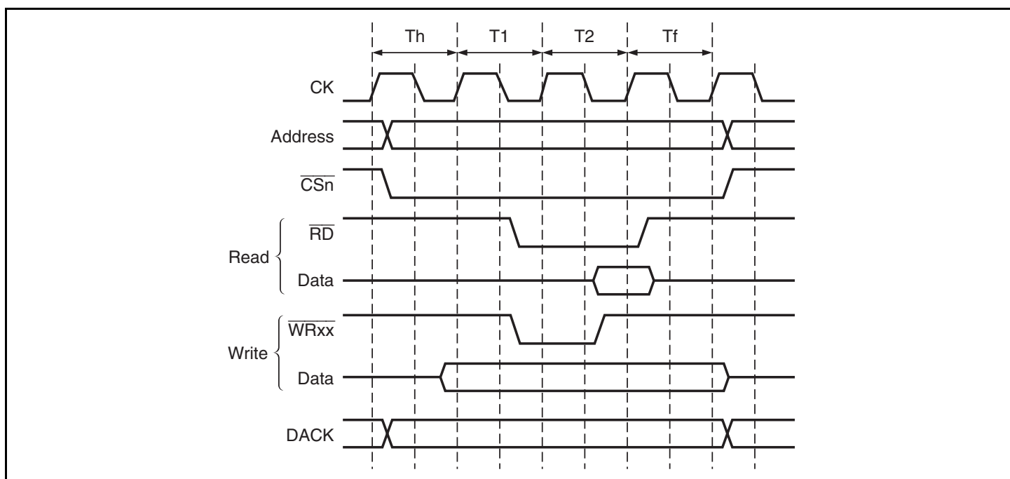
Figure 9.6 \overline{\text{CS}} Assert Period Extension Function
