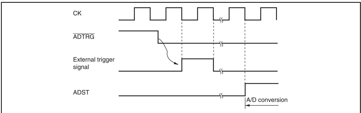
Figure 15.3 External Trigger Input Timing
