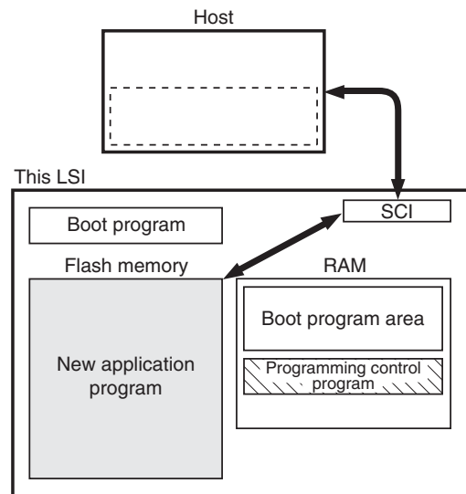
Figure 19.3 Boot Mode
