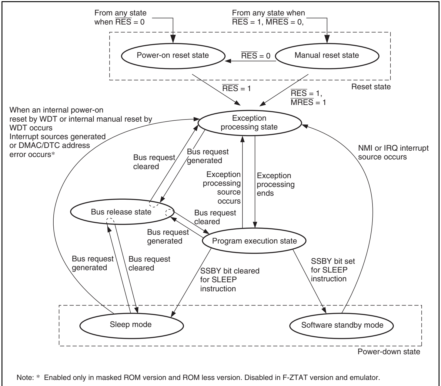
Figure 2.4 Transitions between Processing States
