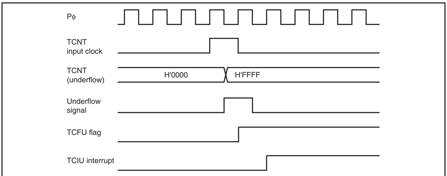
Figure 11.67 TCIU Interrupt Setting Timing
