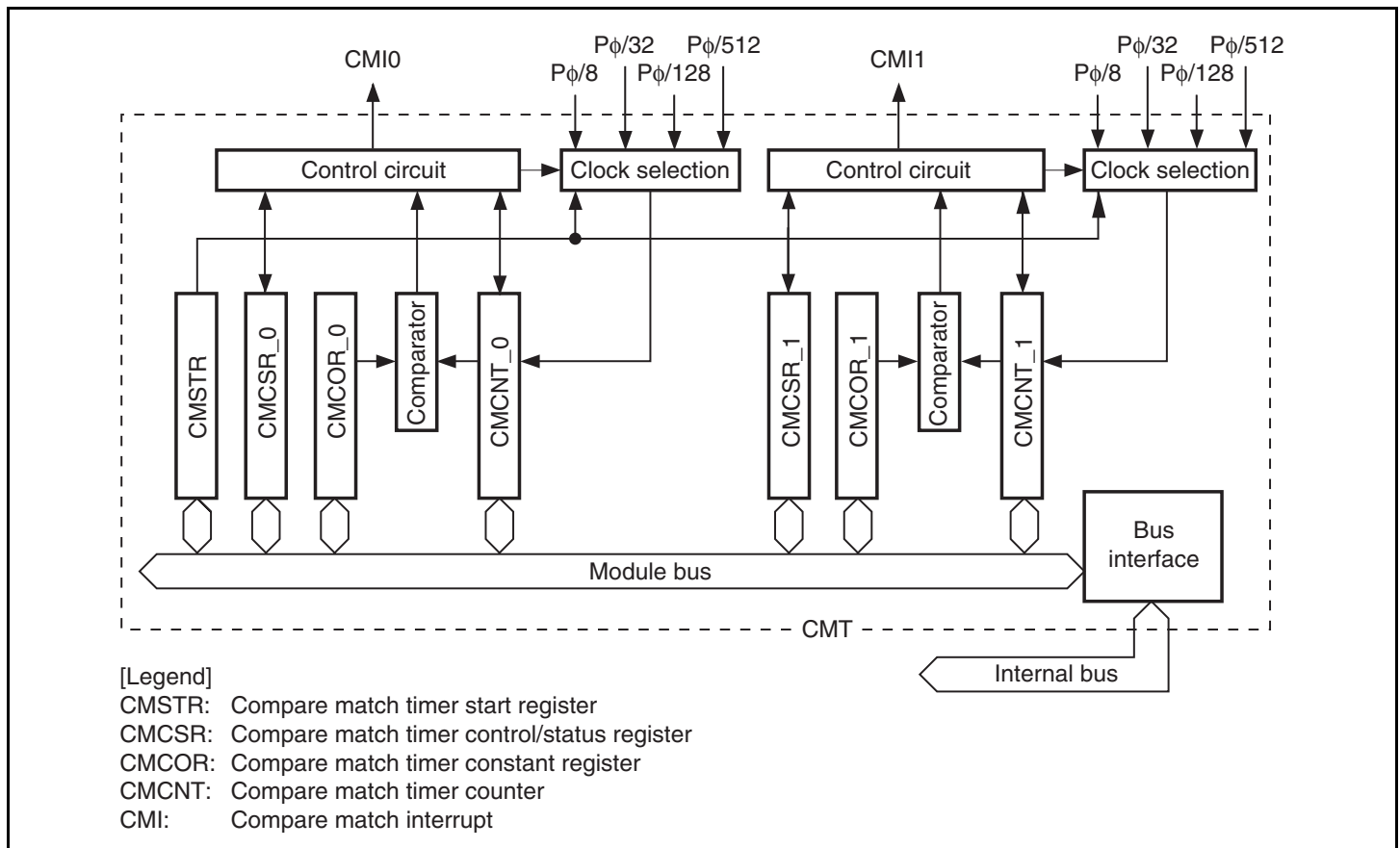
Figure 16.1 CMT Block Diagram
