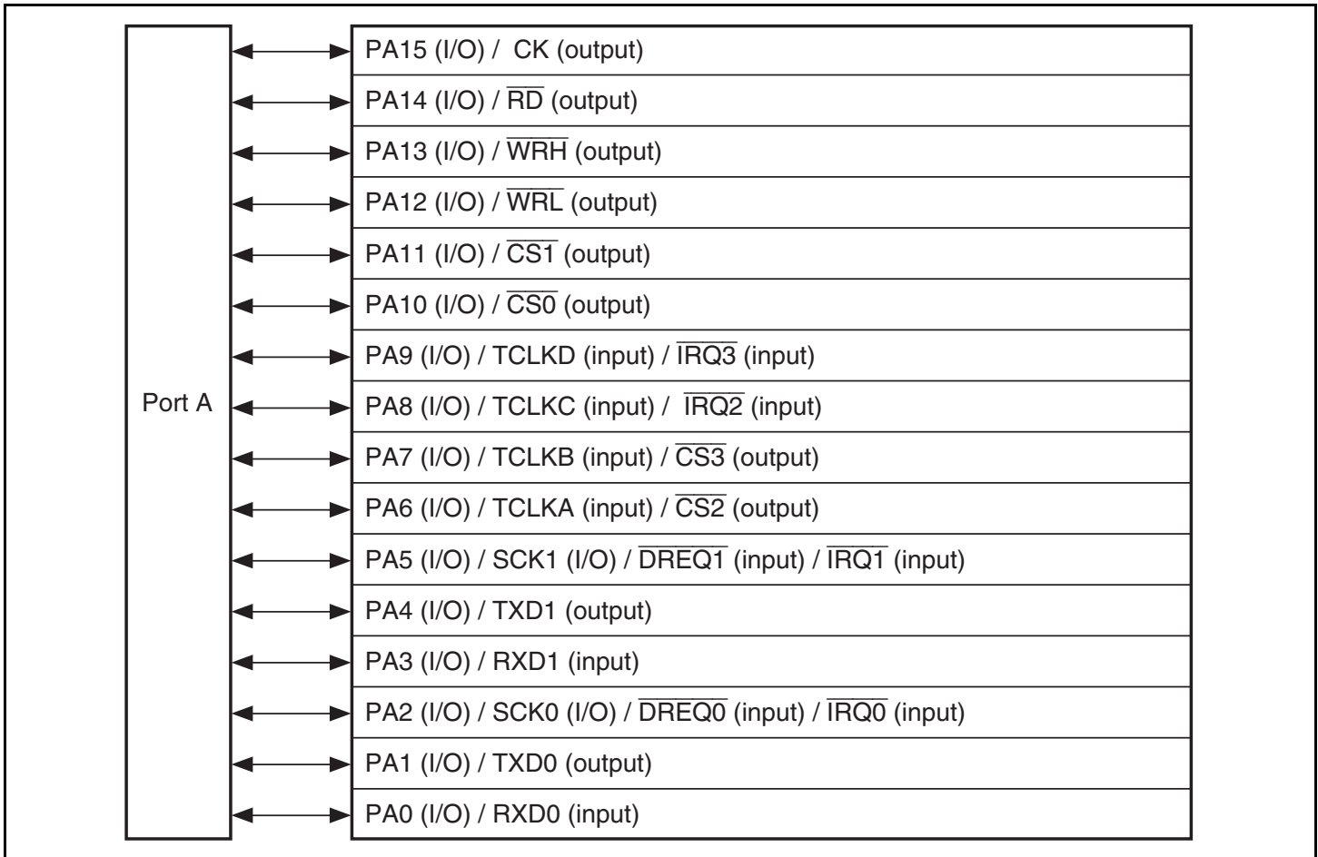
Figure 18.1 Port A (SH7144)
