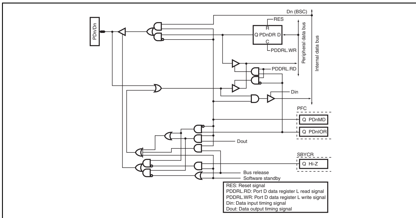
Figure D.23 PDn/Dn
