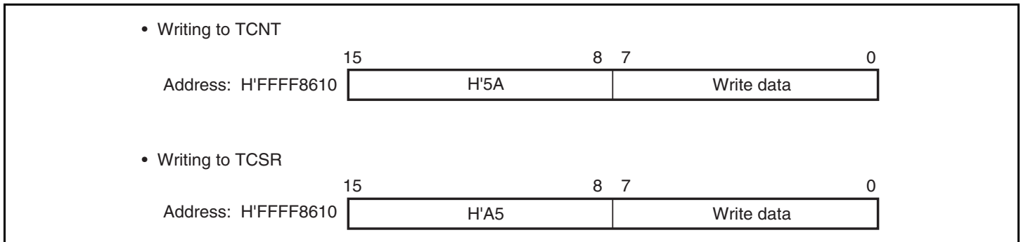
Figure 12.6 Writing to TCNT and TCSR
