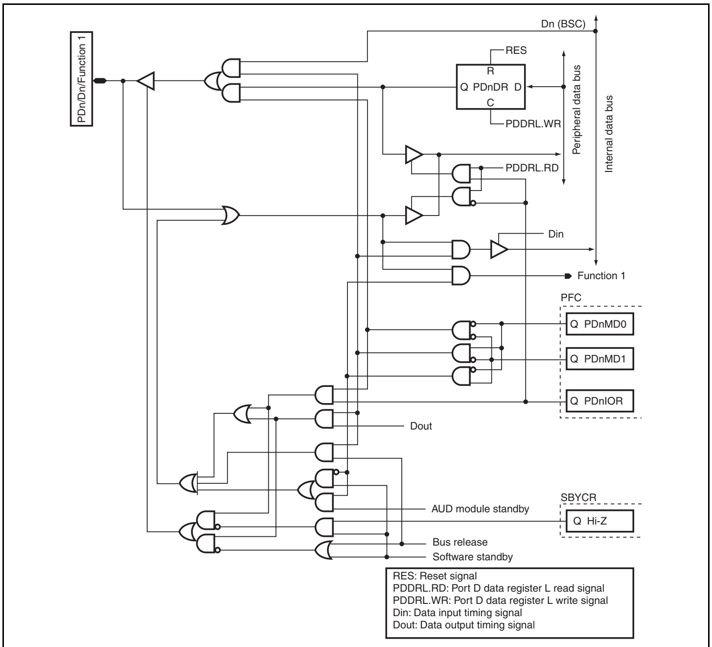
Figure D.25 PDn/Dn/Function 1
