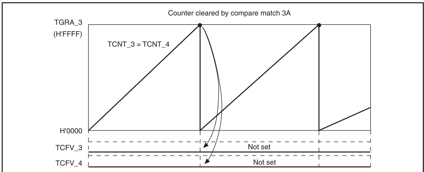
Figure 11.82 Reset Synchronous PWM Mode Overflow Flag
