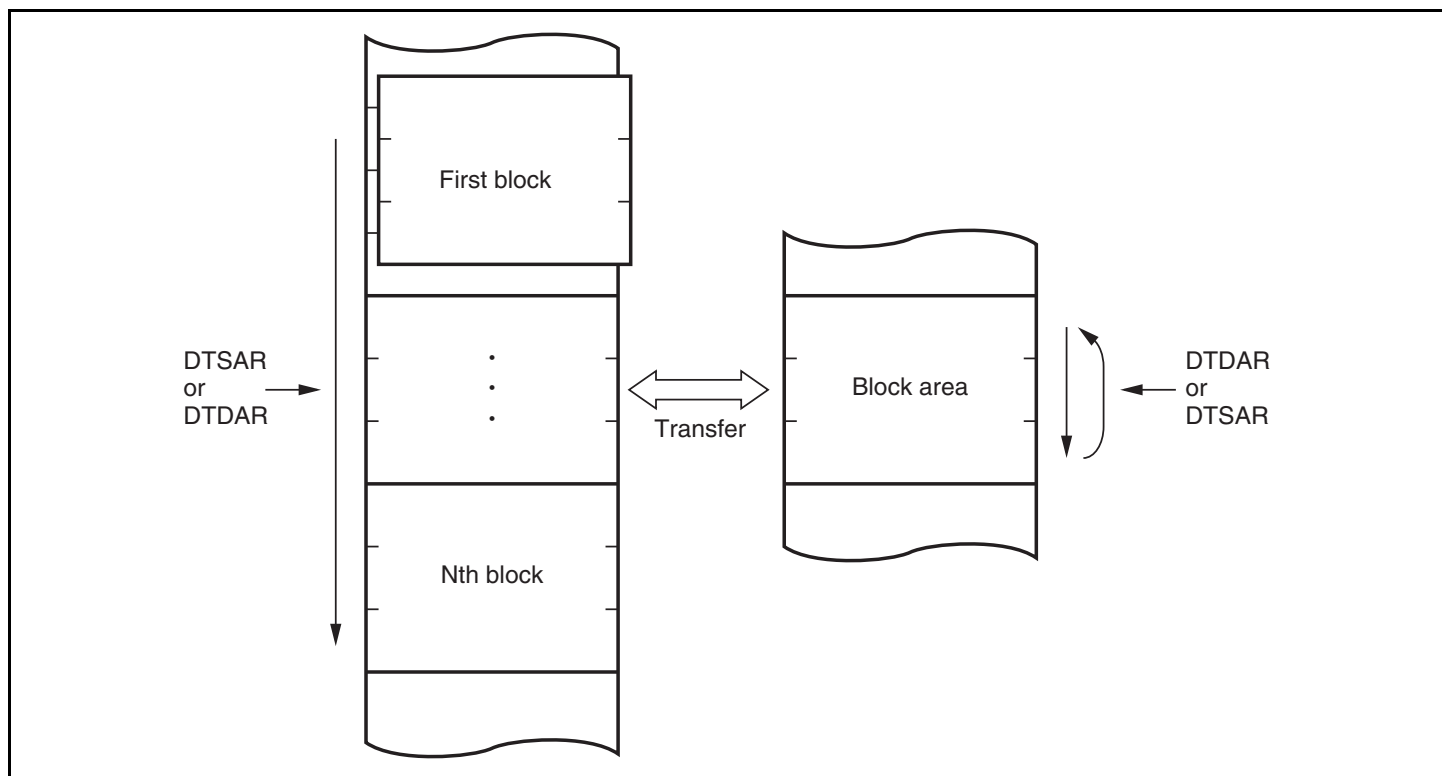
Figure 8.8 Memory Mapping in Block Transfer Mode
