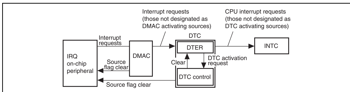
Figure 8.2 Activating Source Control Block Diagram
