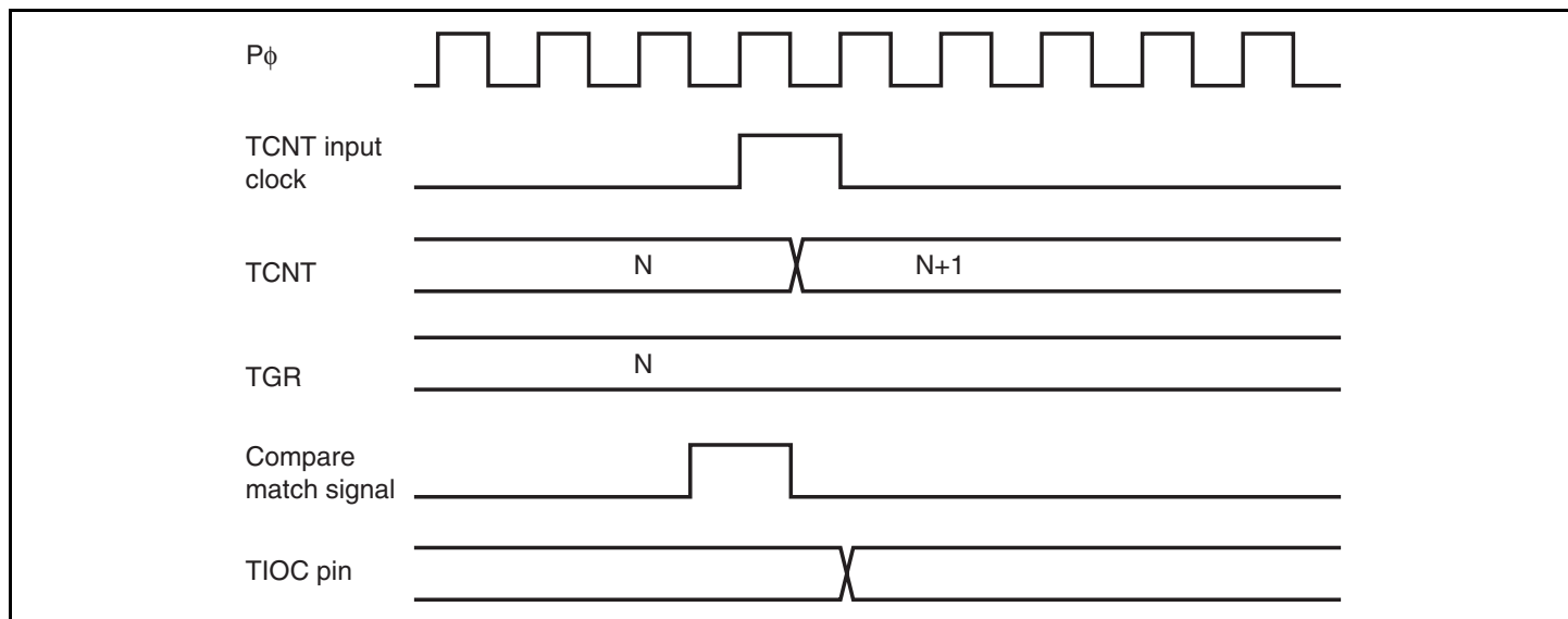
Figure 11.57 Output Compare Output Timing (Normal Mode/PWM Mode)
