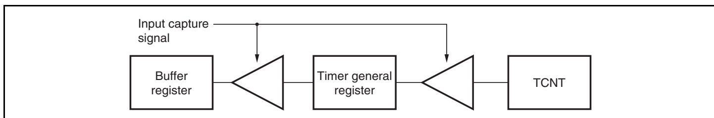
Figure 11.14 Input Capture Buffer Operation
