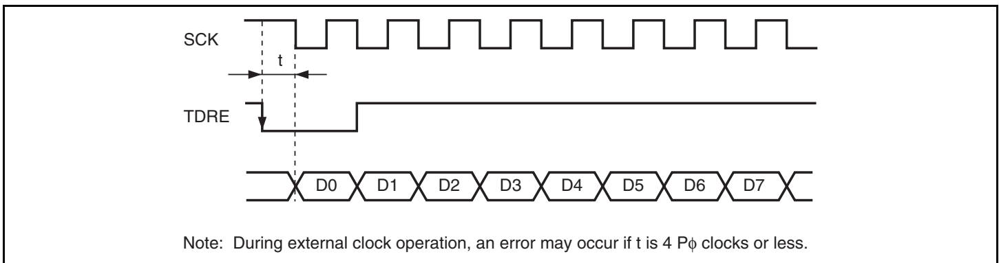
Figure 13.30 Example of Clocked Synchronous Transmission with DMAC/DTC
