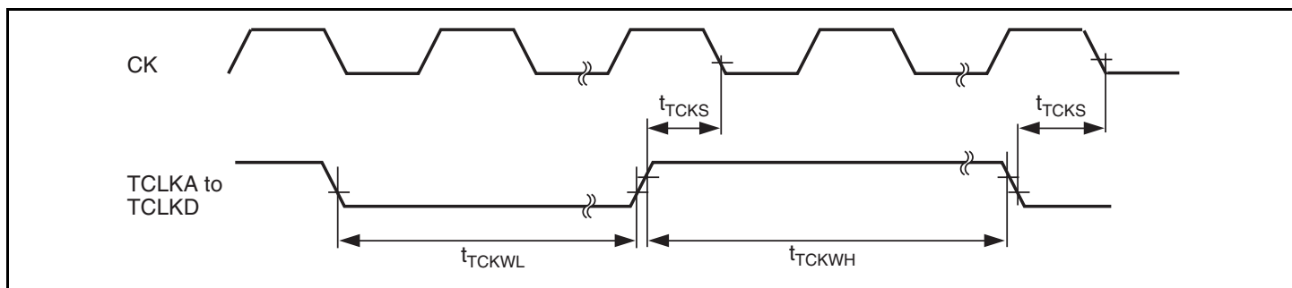
Figure 26.16 MTU Clock Input Timing
