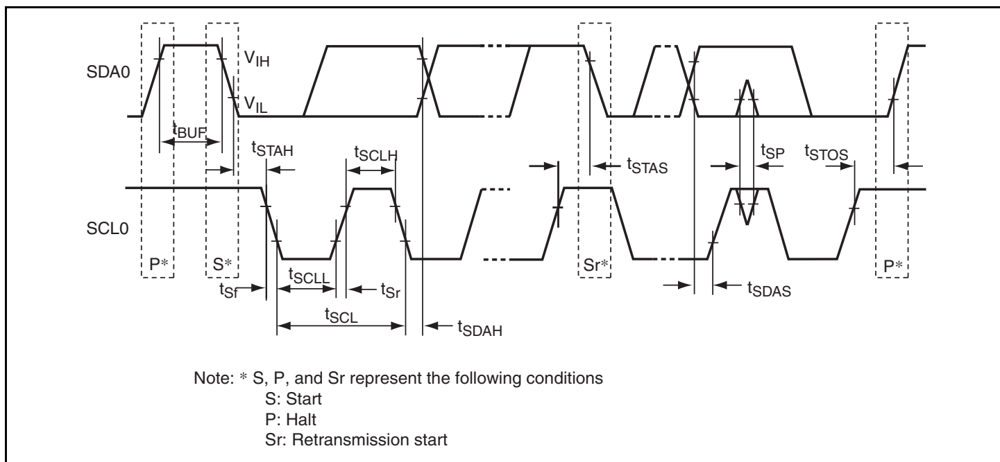
Figure 26.21 I 2 C Bus Interface Timing
