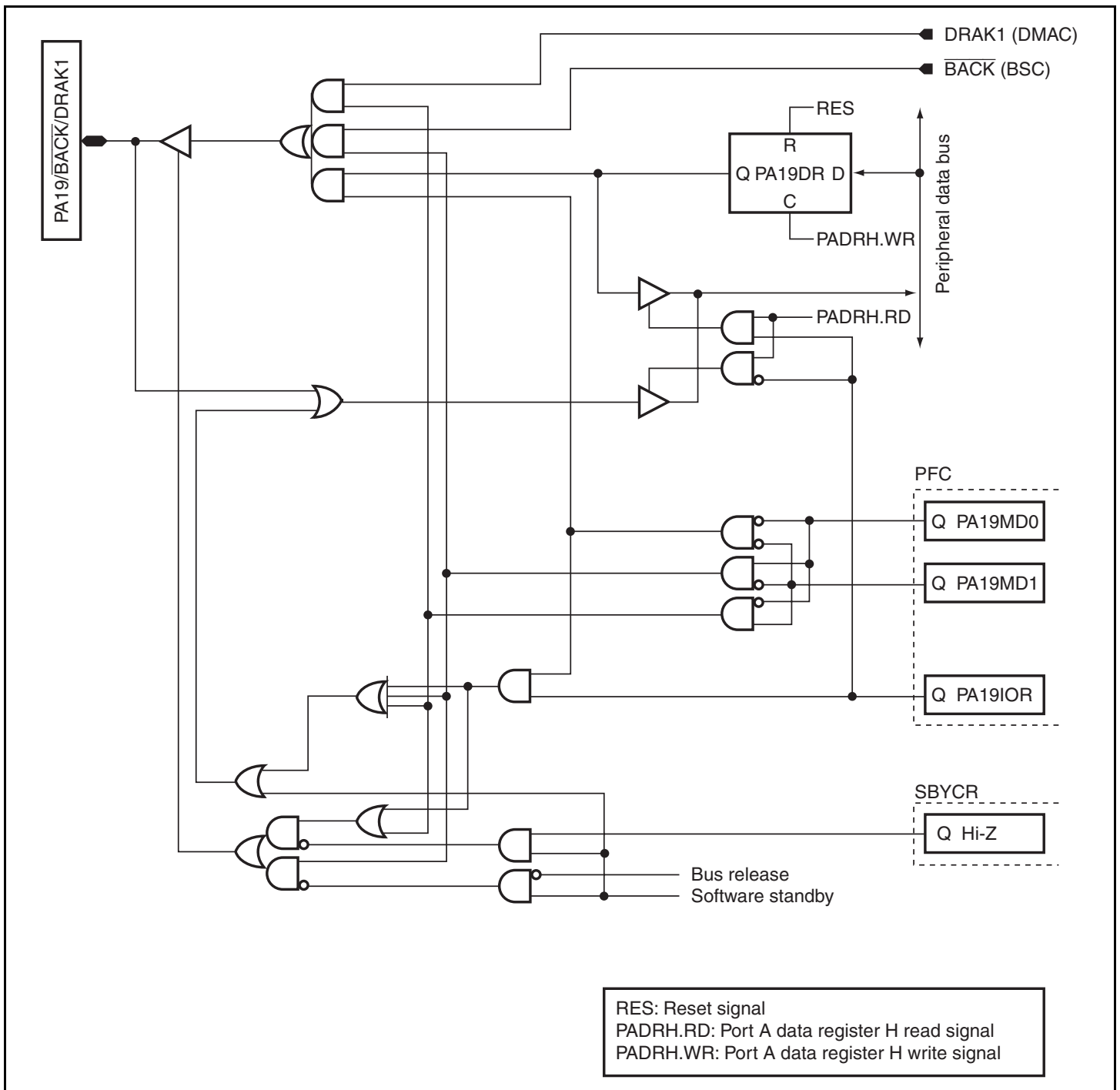
Figure D.11 PA19/ \overline{\text{BACK}} /DRAK1
