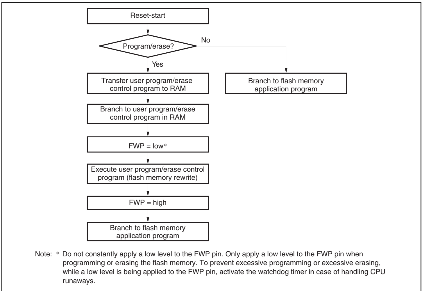
Figure 19.6 Programming/Erasing Flowchart Example in User Program Mode
