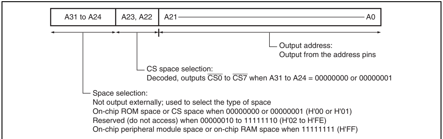
Figure 9.2 Address Format
