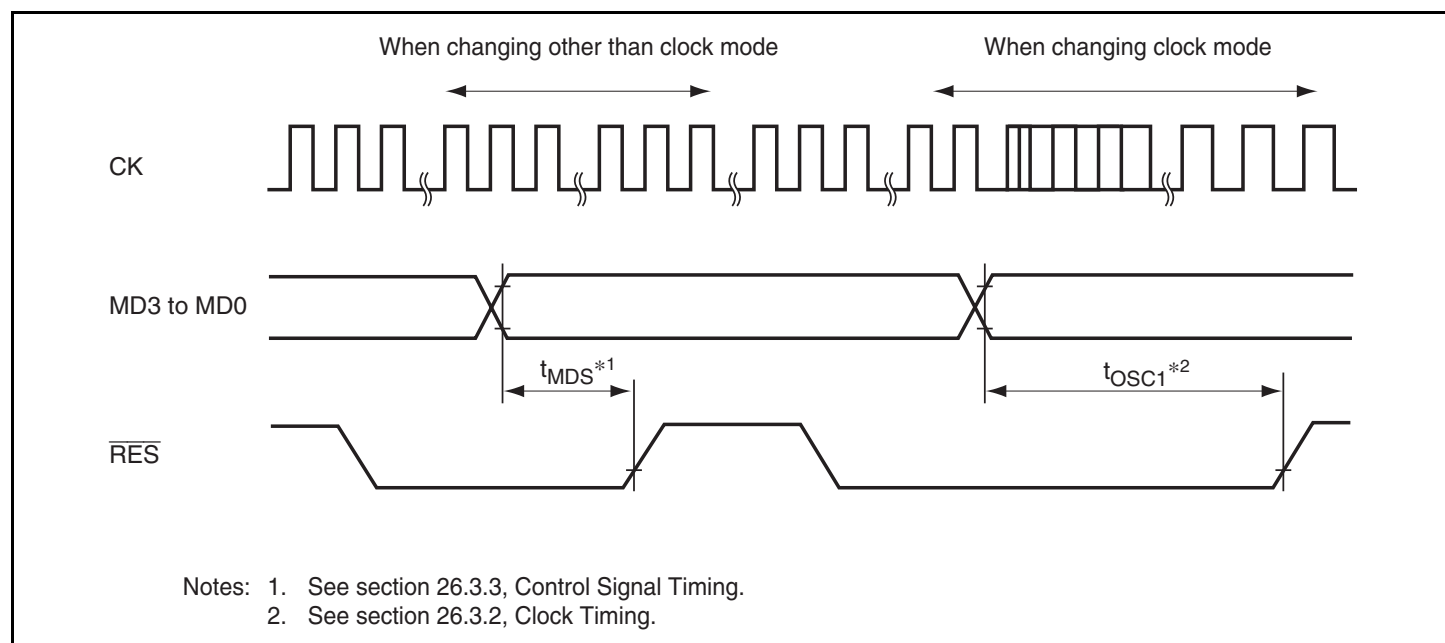
Figure 3.2 Reset Input Timing when Changing Operating Mode
