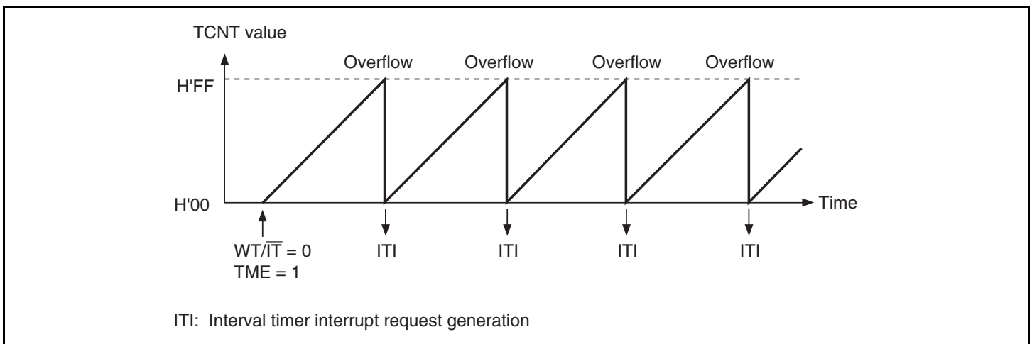
Figure 12.3 Operation in Interval Timer Mode
