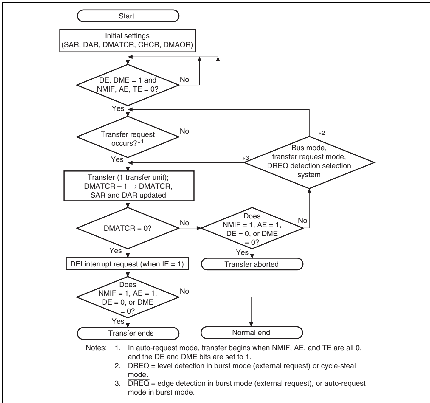
Figure 10.2 DMAC Transfer Flowchart
