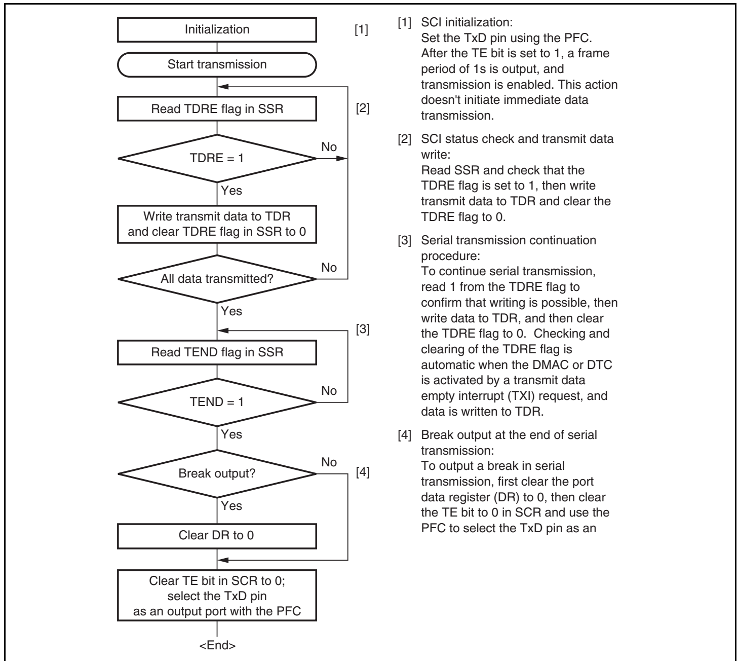
Figure 13.7 Sample Serial Transmission Flowchart
