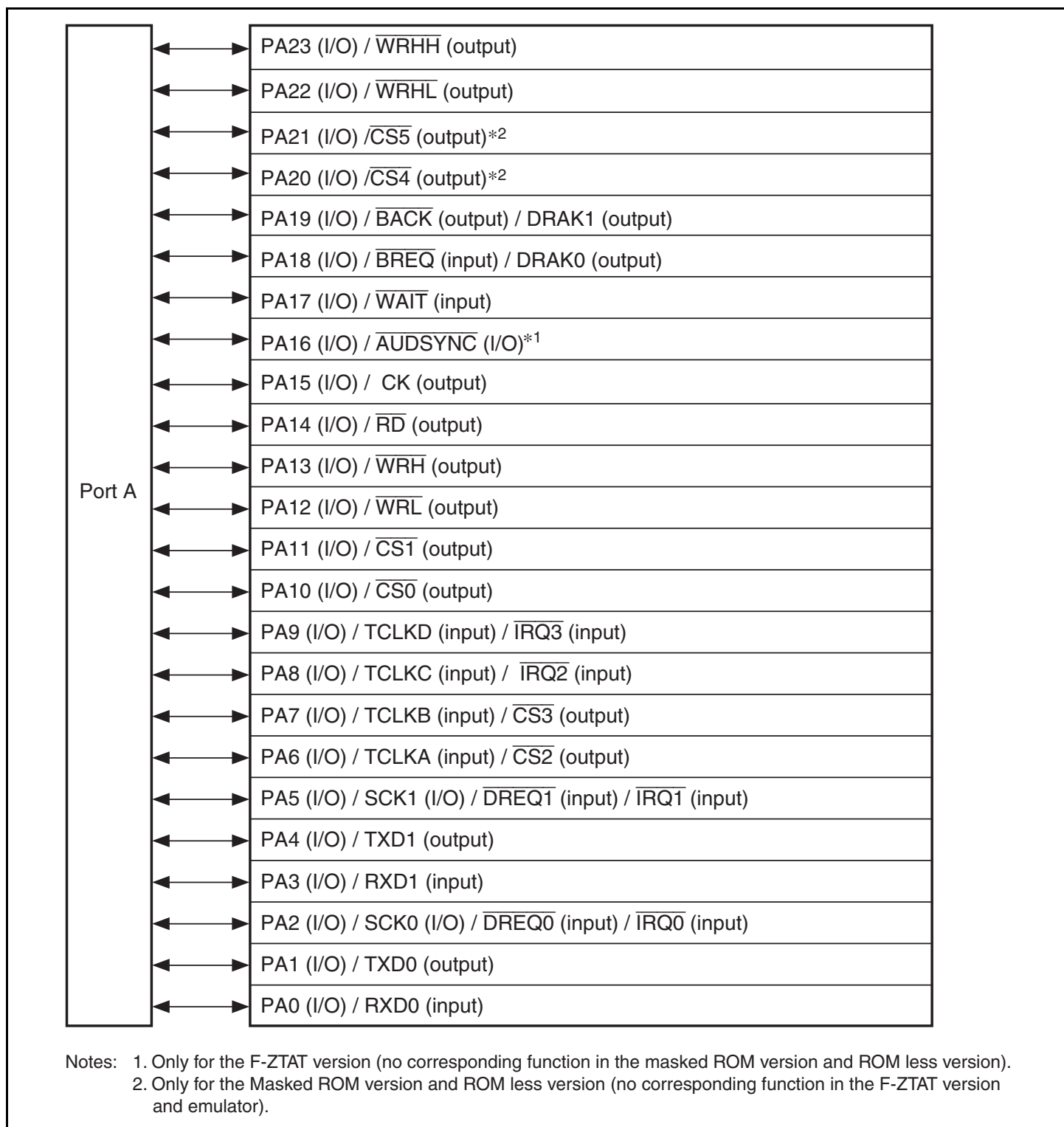
Figure 18.2 Port A (SH7145)
