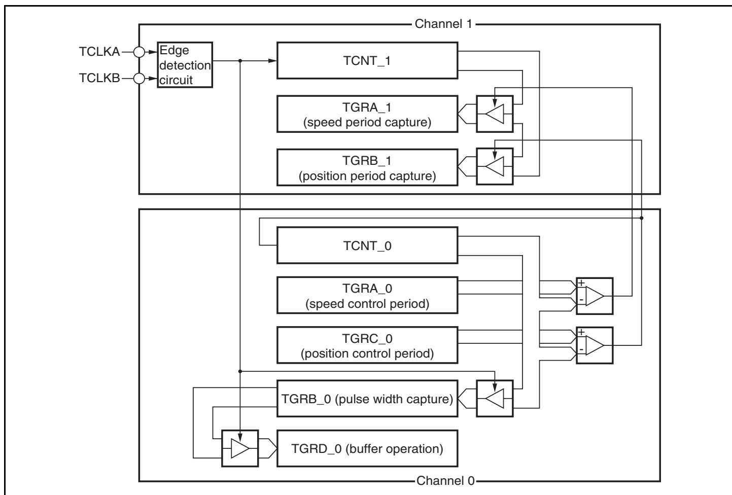
Figure 11.29 Phase Counting Mode Application Example
