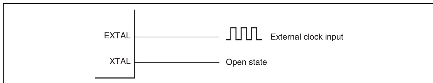
Figure 4.4 Example of External Clock Connection
