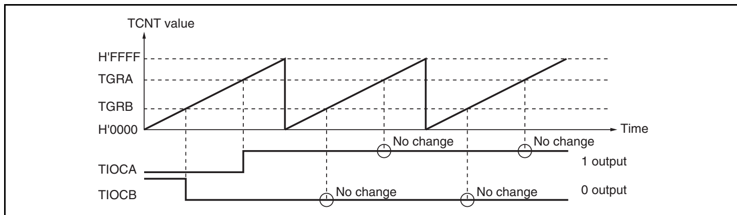
Figure 11.7 Example of 0 Output/1 Output Operation
