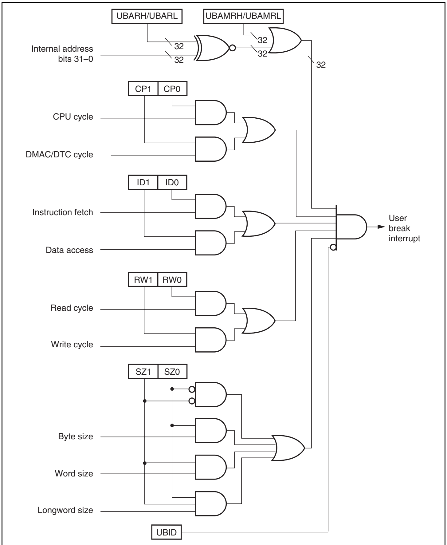
Figure 7.2 Break Condition Determination Method
