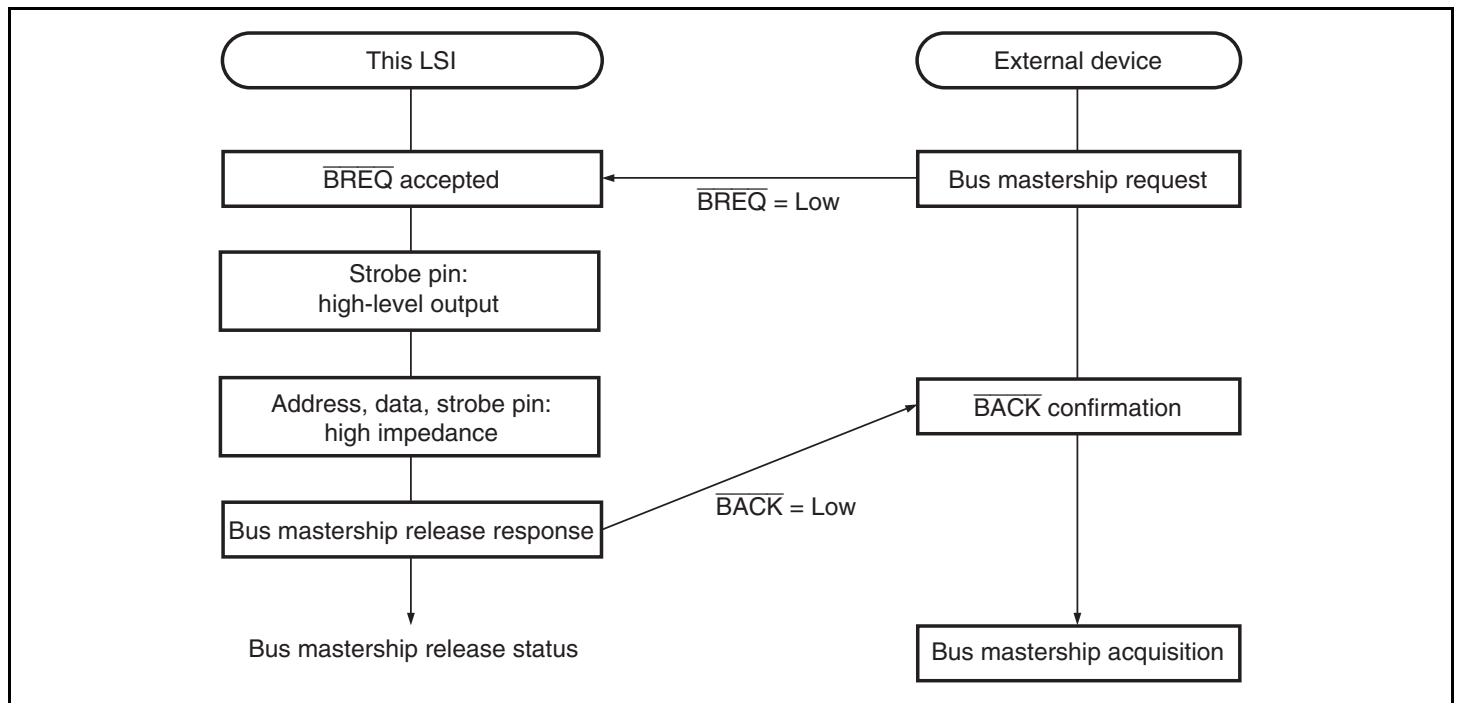
Figure 9.9 Bus Mastership Release Procedure
