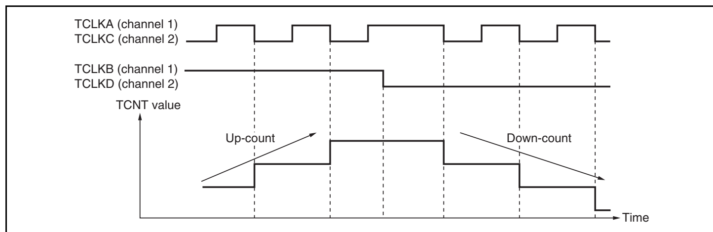
Figure 11.26 Example of Phase Counting Mode 2 Operation
