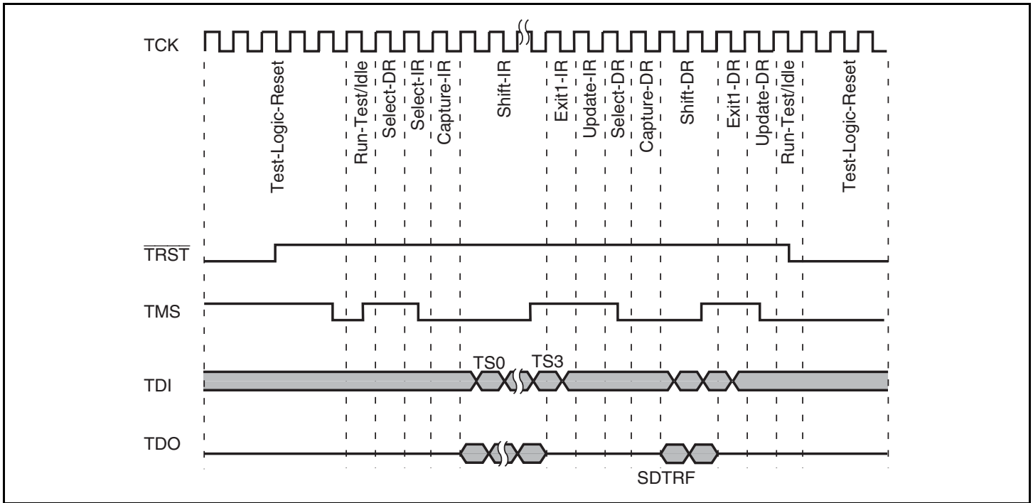
Figure 22.3 Data Input/Output Timing Chart (2)
