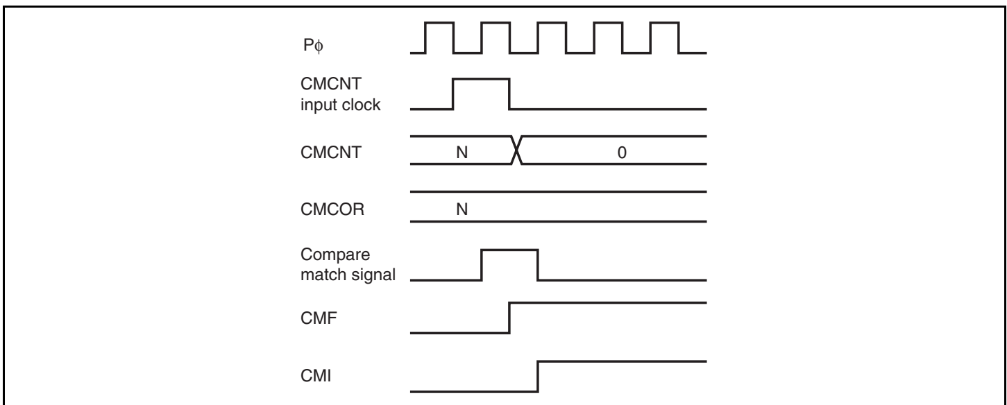
Figure 16.4 CMF Set Timing
