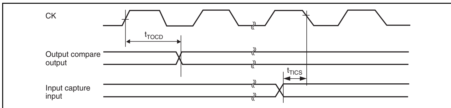
Figure 26.15 MTU Input/Output timing
