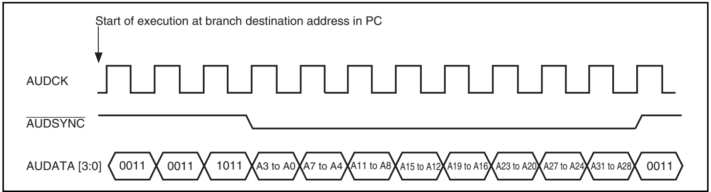
Figure 23.2 Example of Data Output (32-Bit Output)
