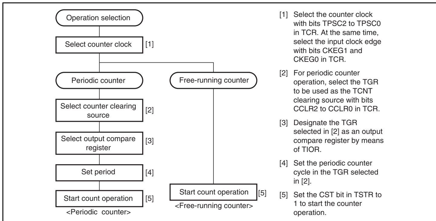
Figure 11.3 Example of Counter Operation Setting Procedure
