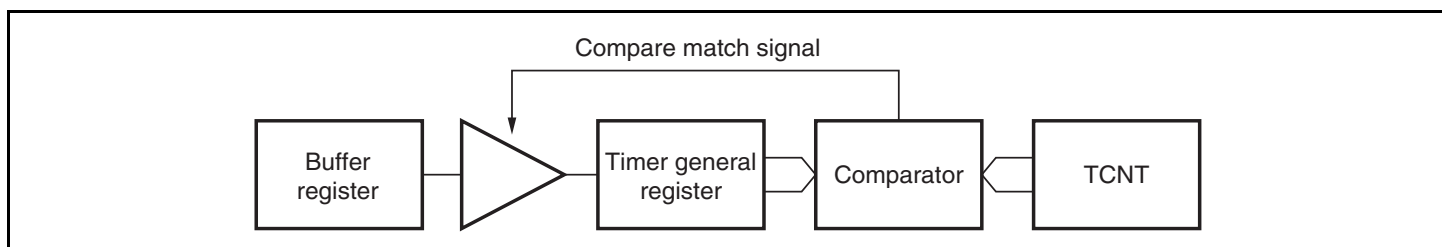
Figure 11.13 Compare Match Buffer Operation
