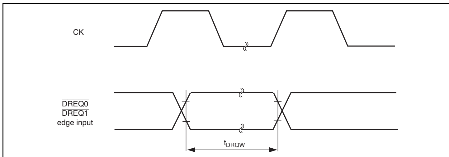
Figure 26.13 \overline{\text{DREQ0}} , \overline{\text{DREQ1}} Input Timing (2)
