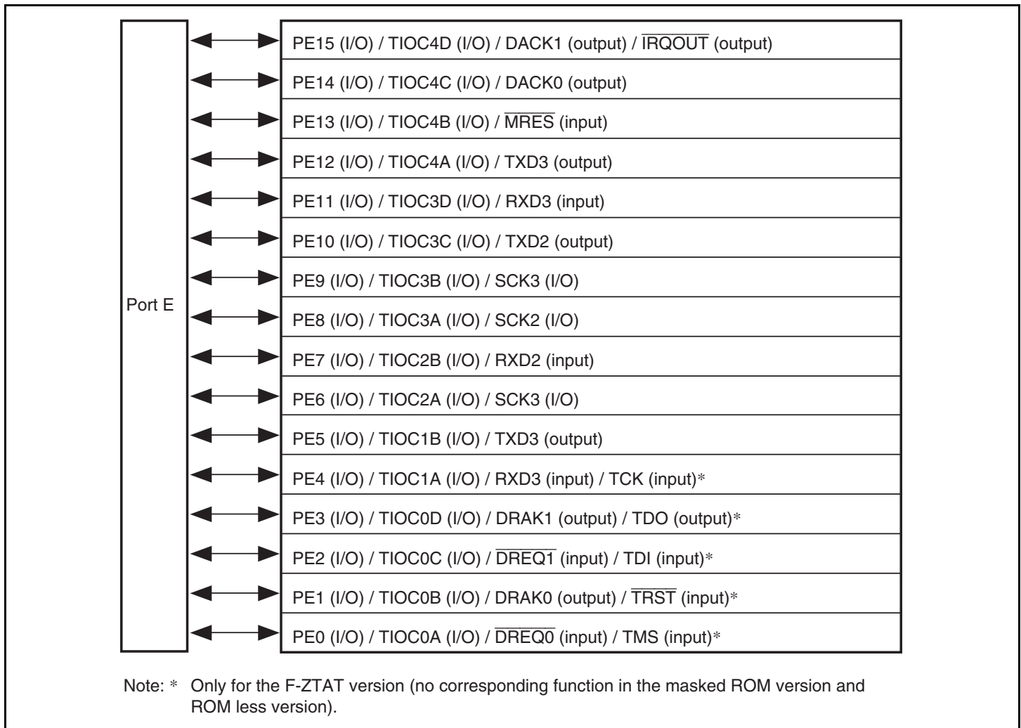
Figure 18.7 Port E (SH7144)
