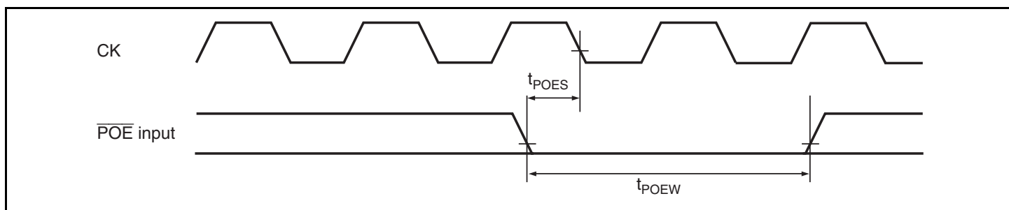
Figure 26.22 \overline{\text{POE}} Input/Output Timing
