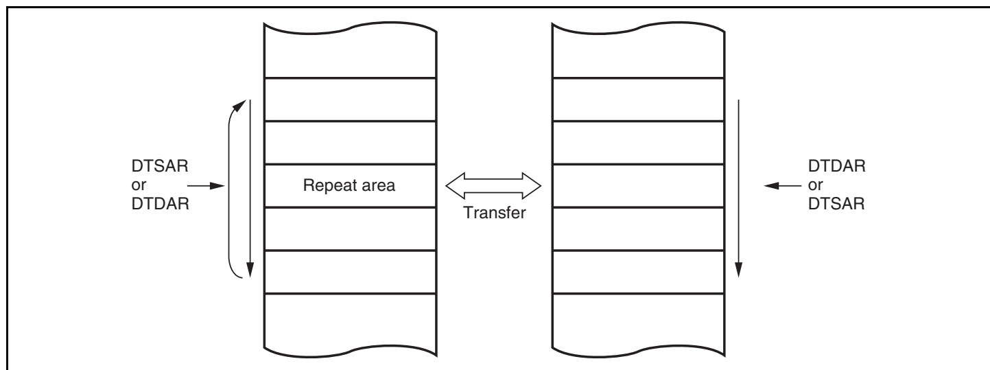
Figure 8.7 Memory Mapping in Repeat Mode
