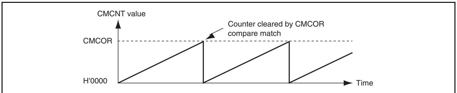
Figure 16.2 Counter Operation
