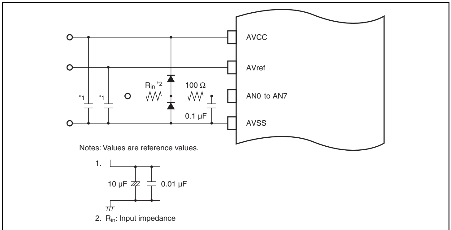
Figure 15.7 Example of Analog Input Protection Circuit
