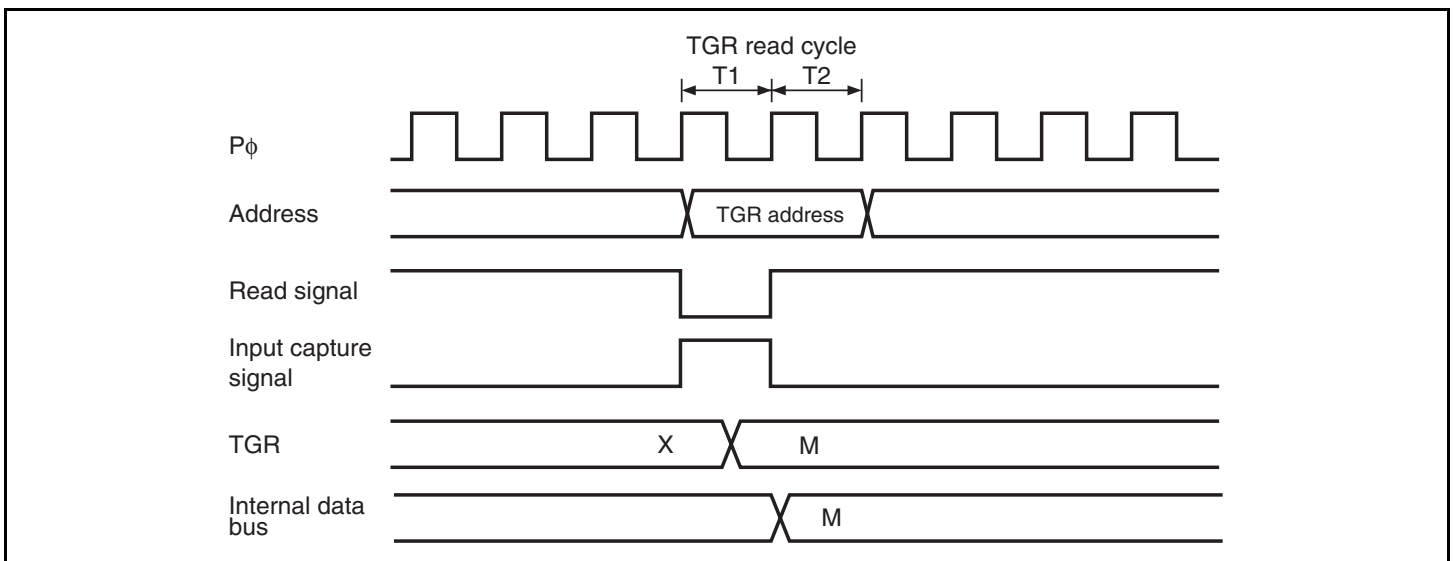
Figure 11.76 Contention between TGR Read and Input Capture
