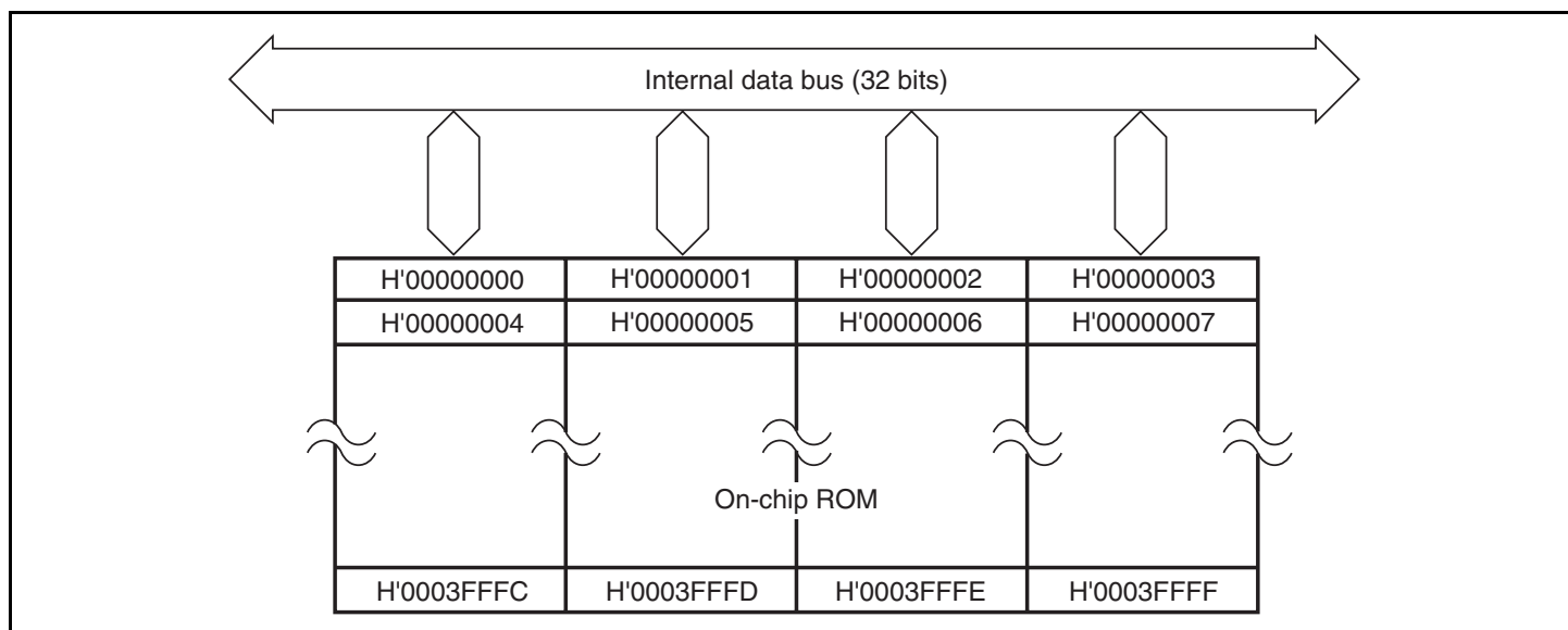
Figure 20.1 Mask ROM Block Diagram
