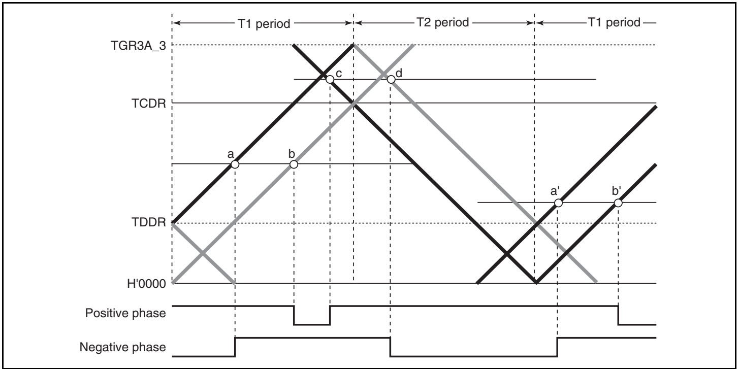
Figure 11.40 Example of Complementary PWM Mode Waveform Output (1)
