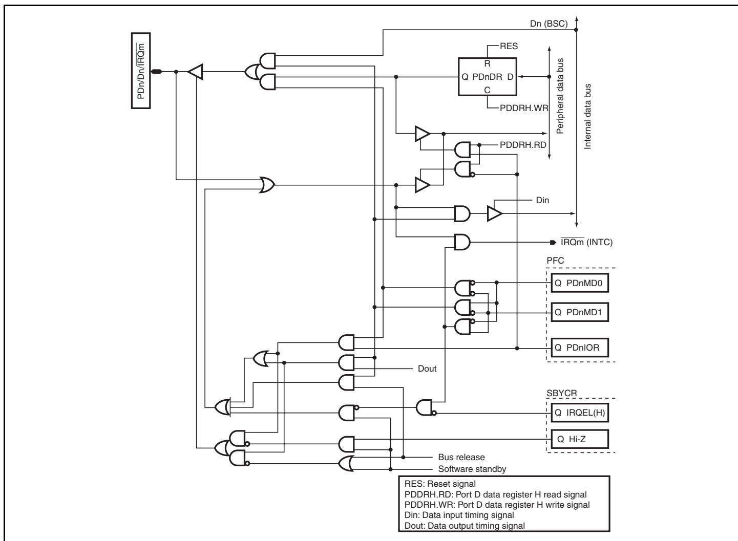
Figure D.27 PDn/Dn/ \overline{\text{IRQ}}_m
