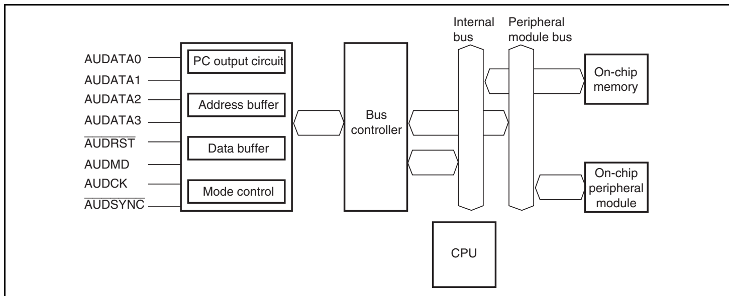
Figure 23.1 AUD Block Diagram
