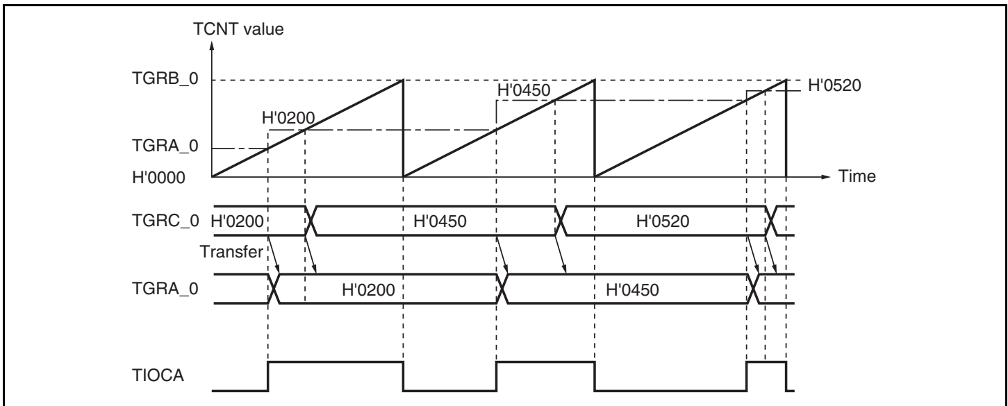
Figure 11.16 Example of Buffer Operation (1)
