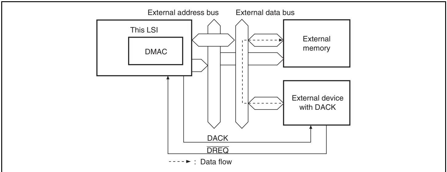
Figure 10.4 Data Flow in Single Address Mode
