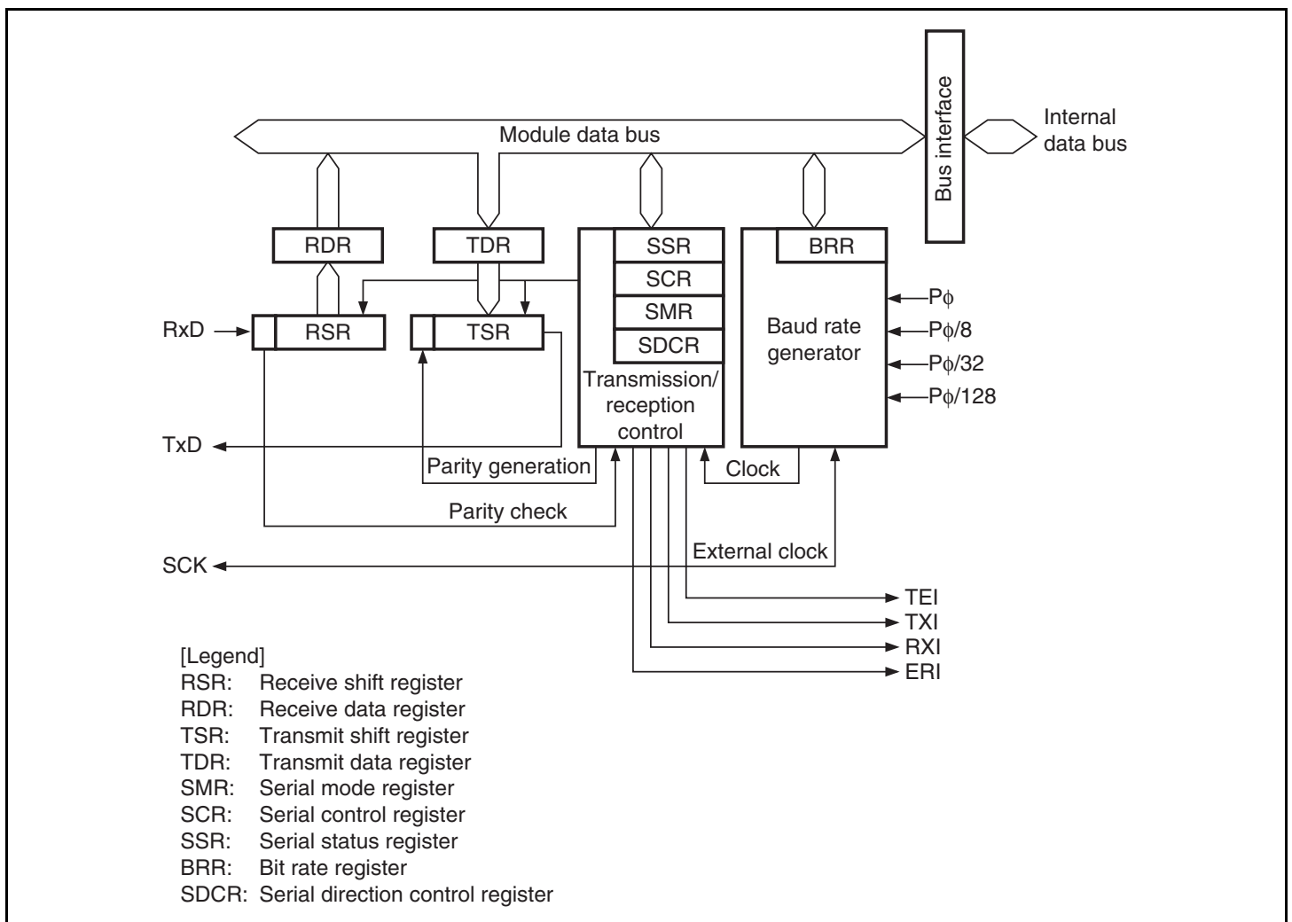
Figure 13.1 Block Diagram of SCI
