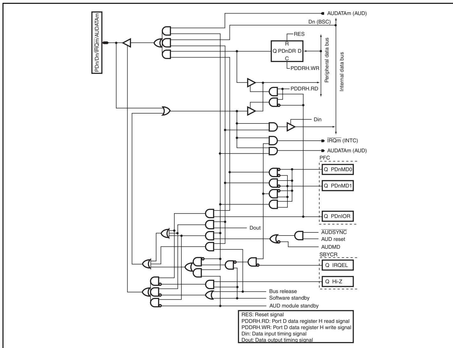
Figure D.28 PDn/Dn/IRQm/AUDATAm
