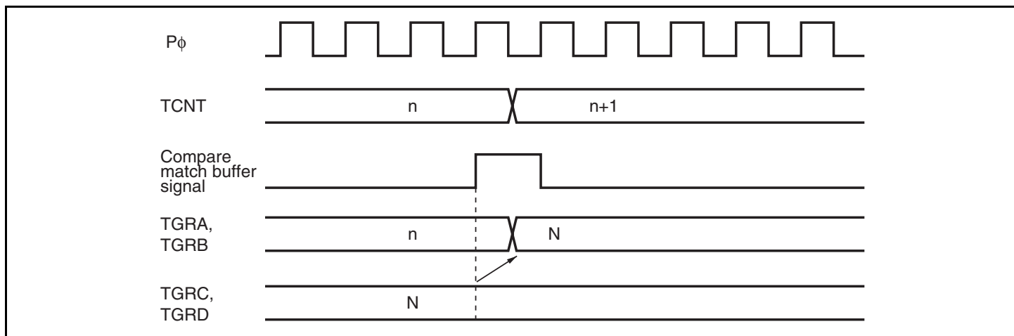
Figure 11.62 Buffer Operation Timing (Compare Match)
