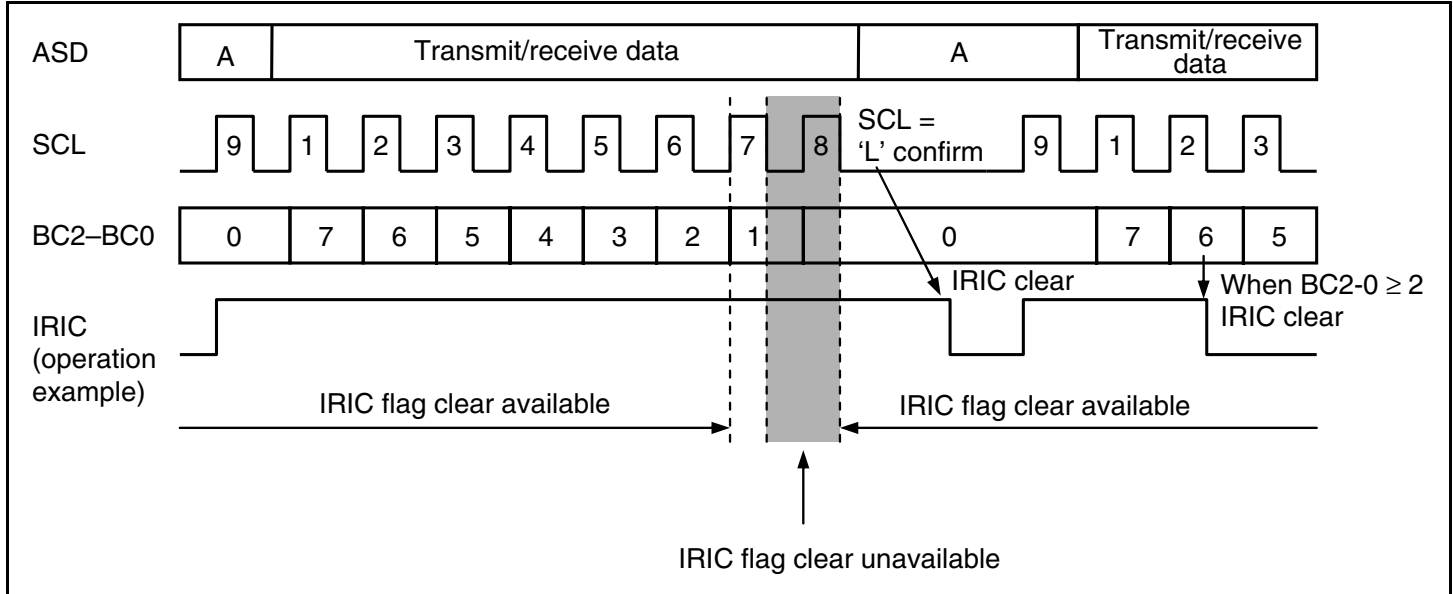
Figure 14.32 IRIC Flag Clear Timing on WAIT Operation
