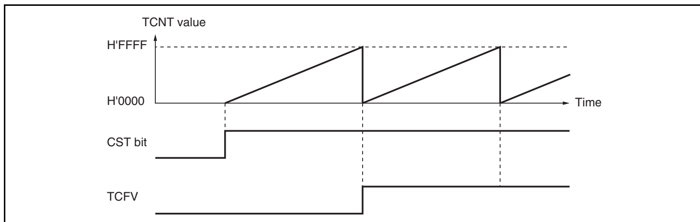
Figure 11.4 Free-Running Counter Operation
