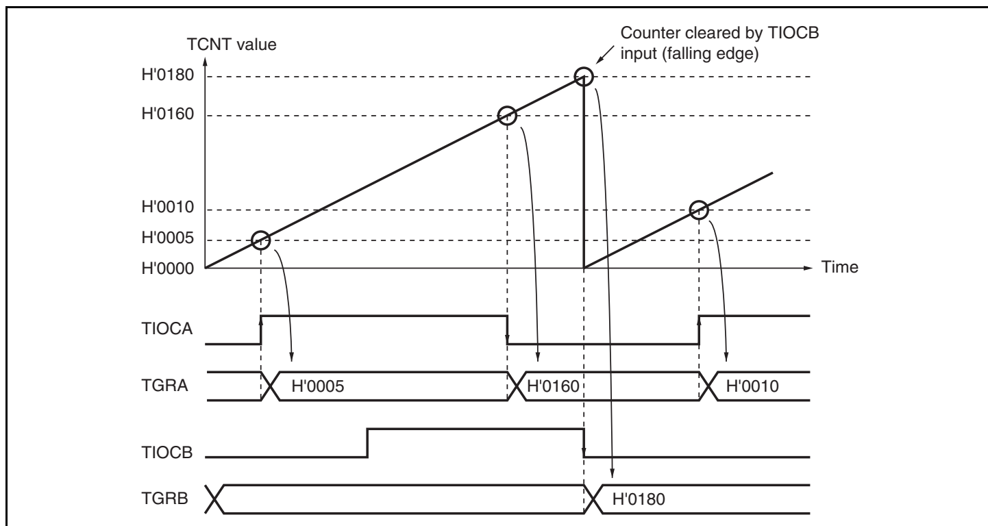
Figure 11.10 Example of Input Capture Operation
