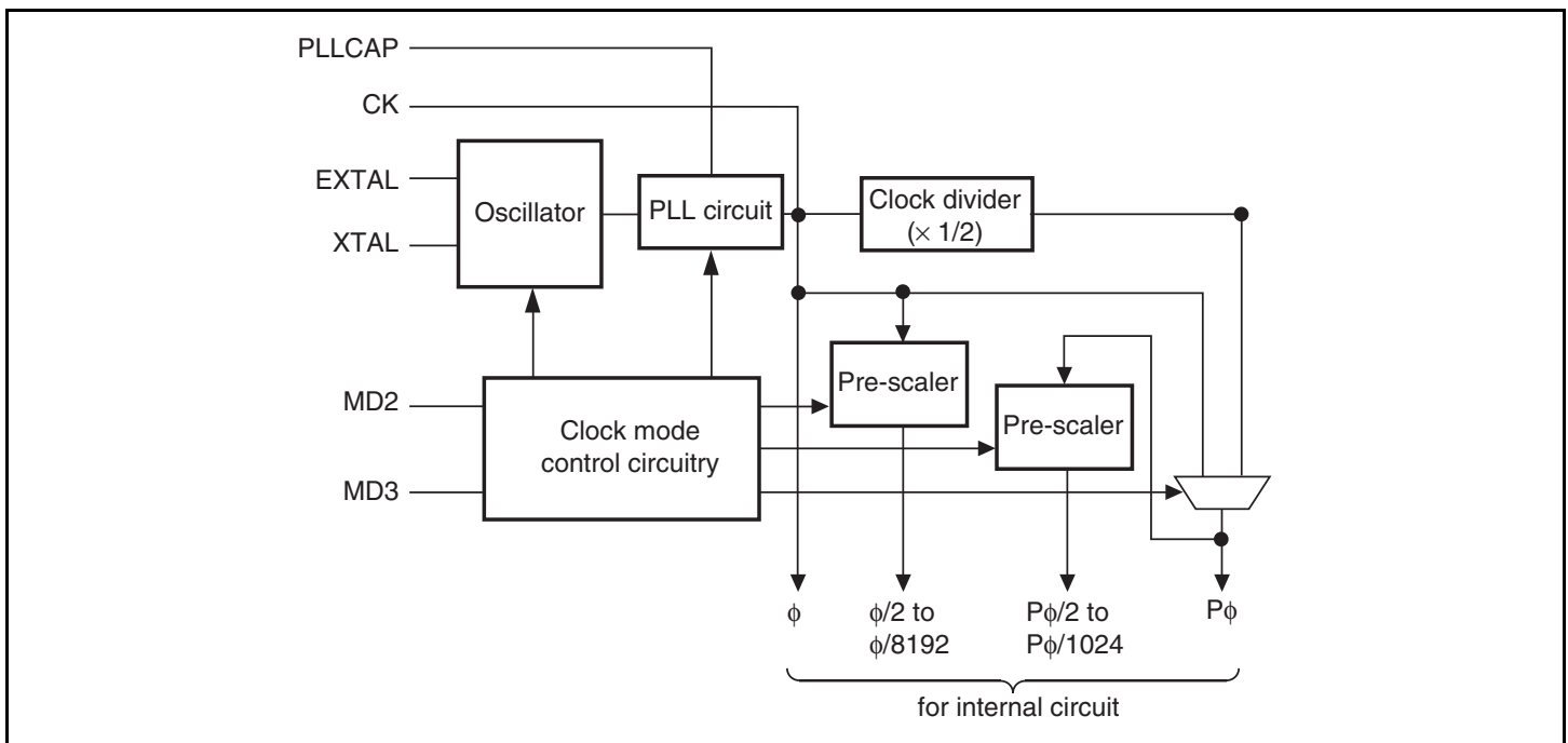
Figure 4.1 Block Diagram of Clock Pulse Generator
