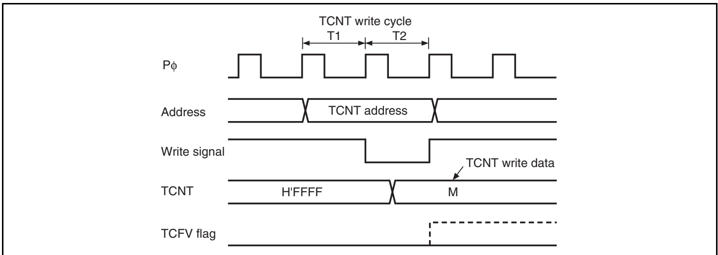
Figure 11.84 Contention between TCNT Write and Overflow
