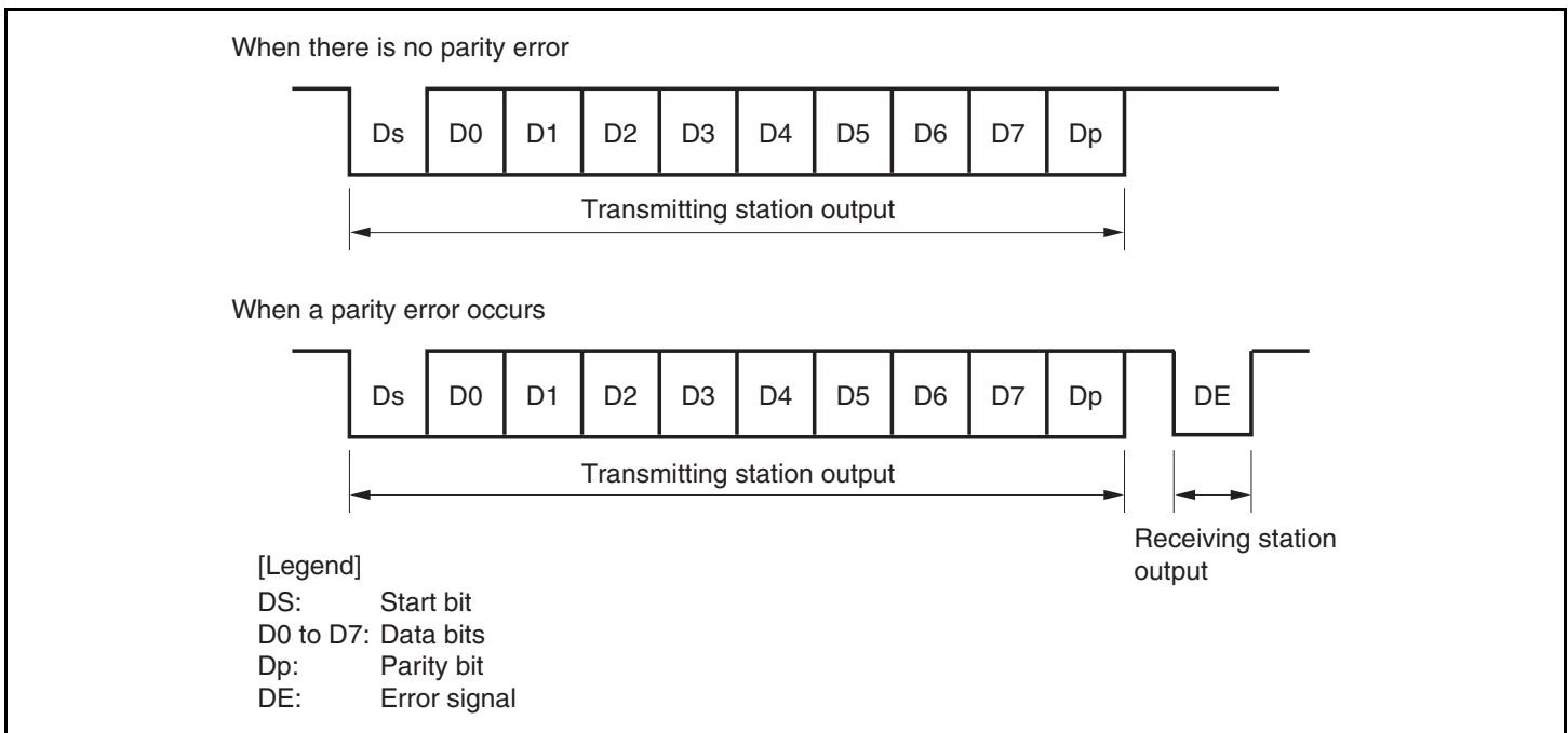
Figure 13.22 Normal Smart Card Interface Data Format
