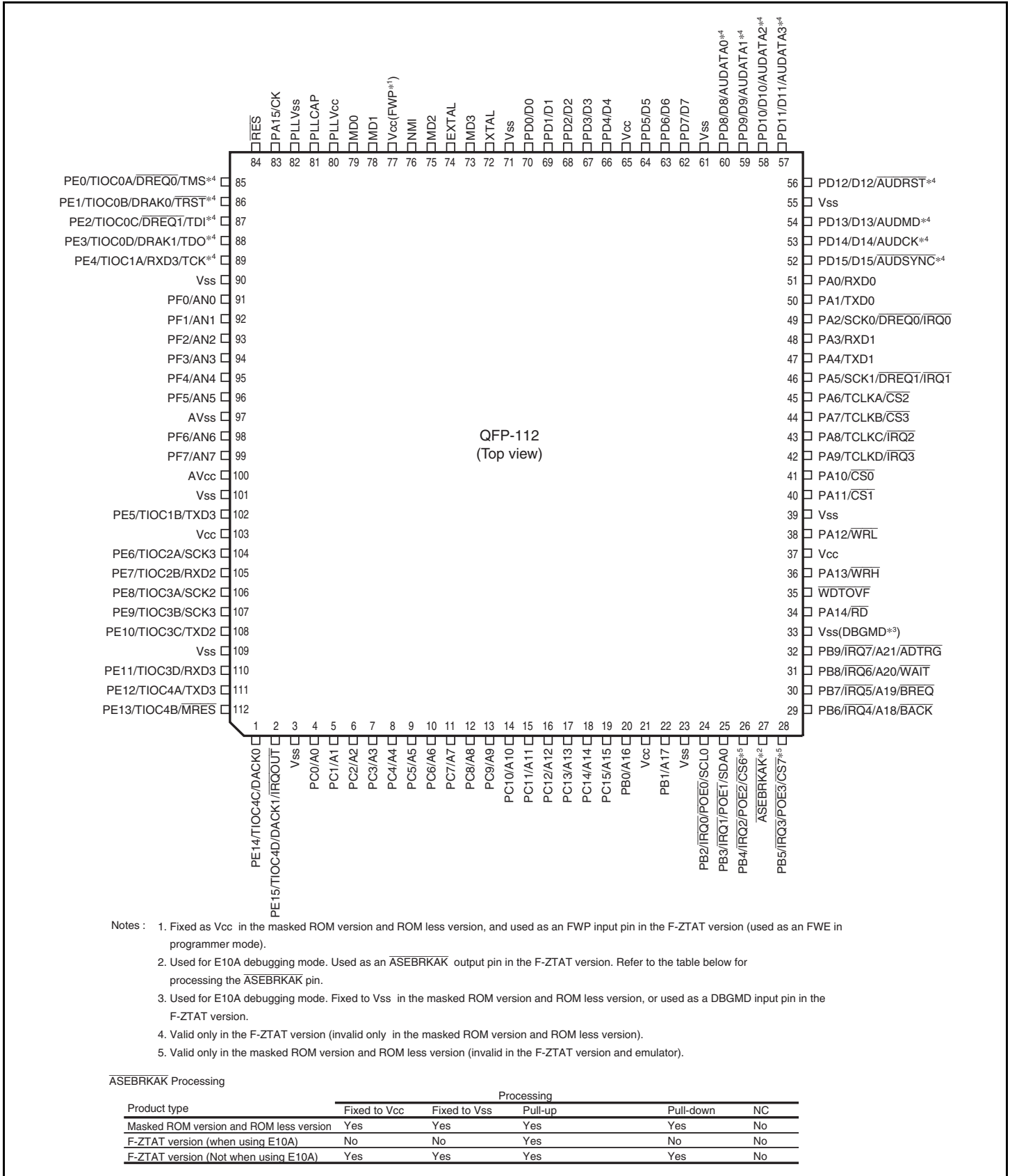
Figure 1.3 SH7144 Pin Arrangement
