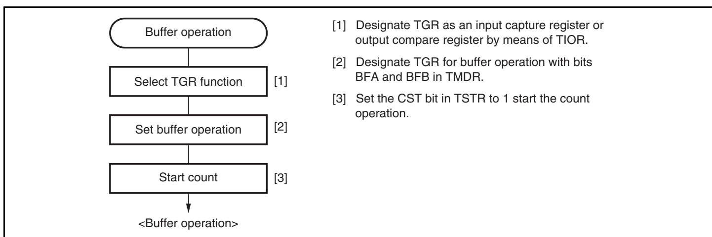
Figure 11.15 Example of Buffer Operation Setting Procedure
