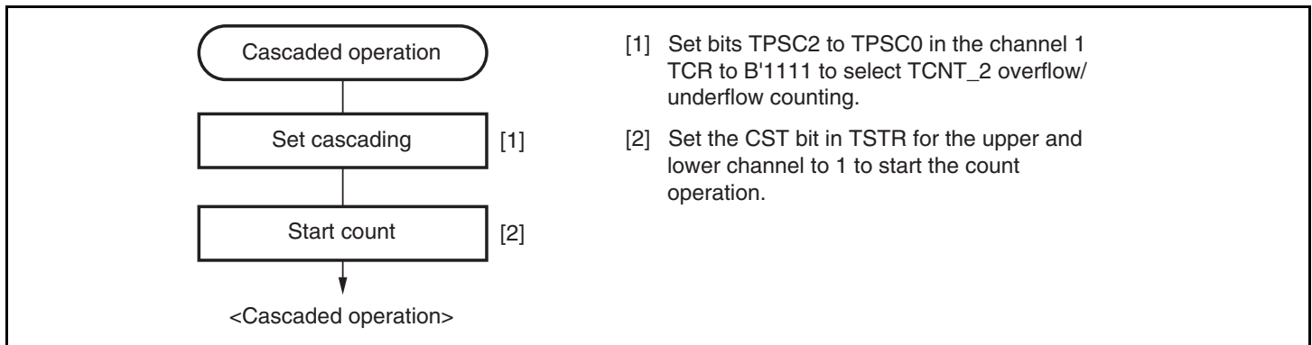
Figure 11.18 Cascaded Operation Setting Procedure
