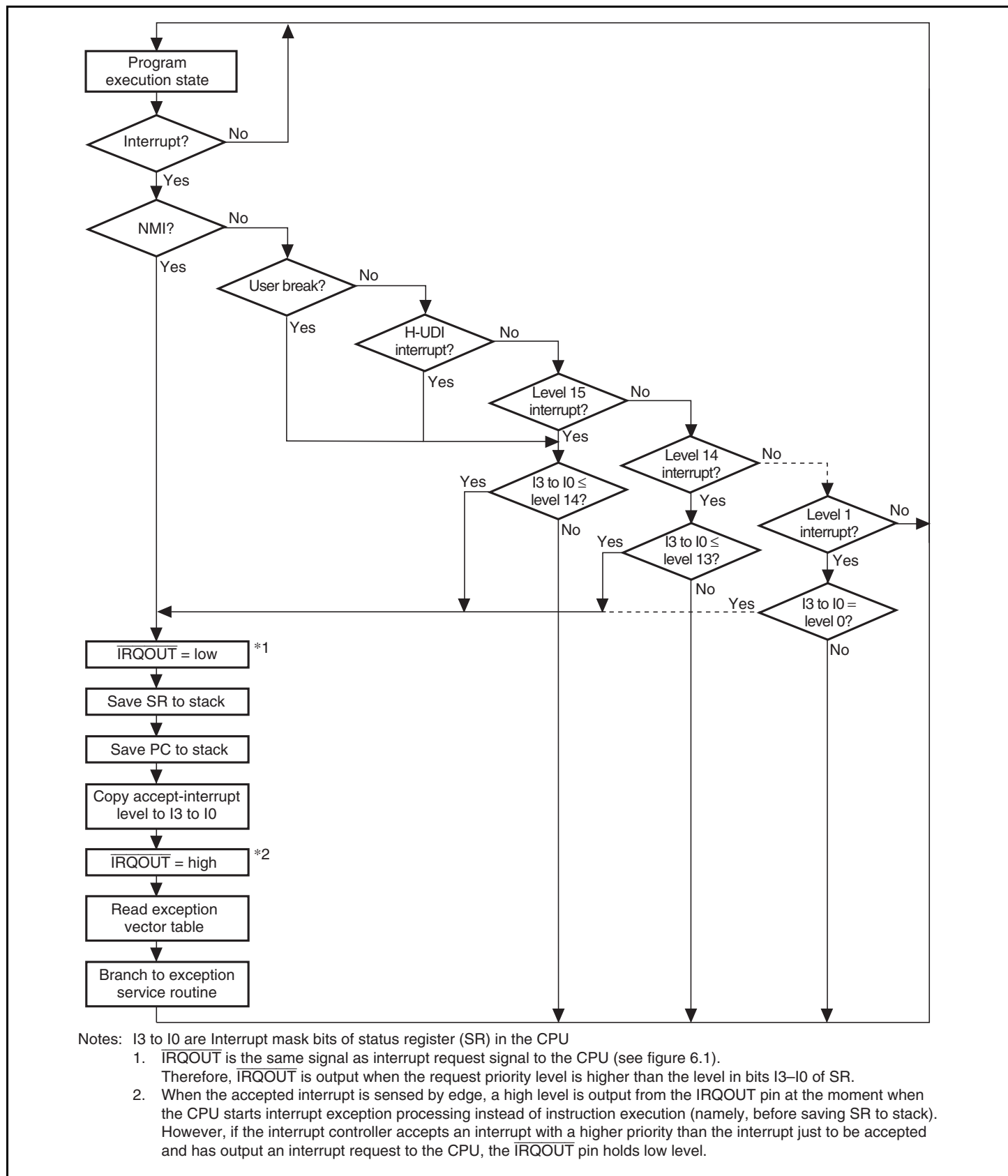
Figure 6.3 Interrupt Sequence Flowchart
