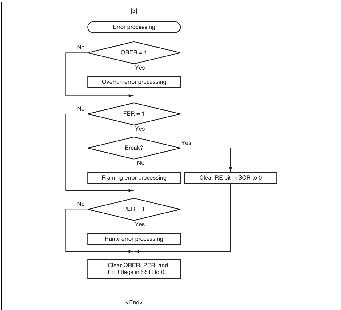
Figure 13.9 Sample Serial Reception Data Flowchart (2)
