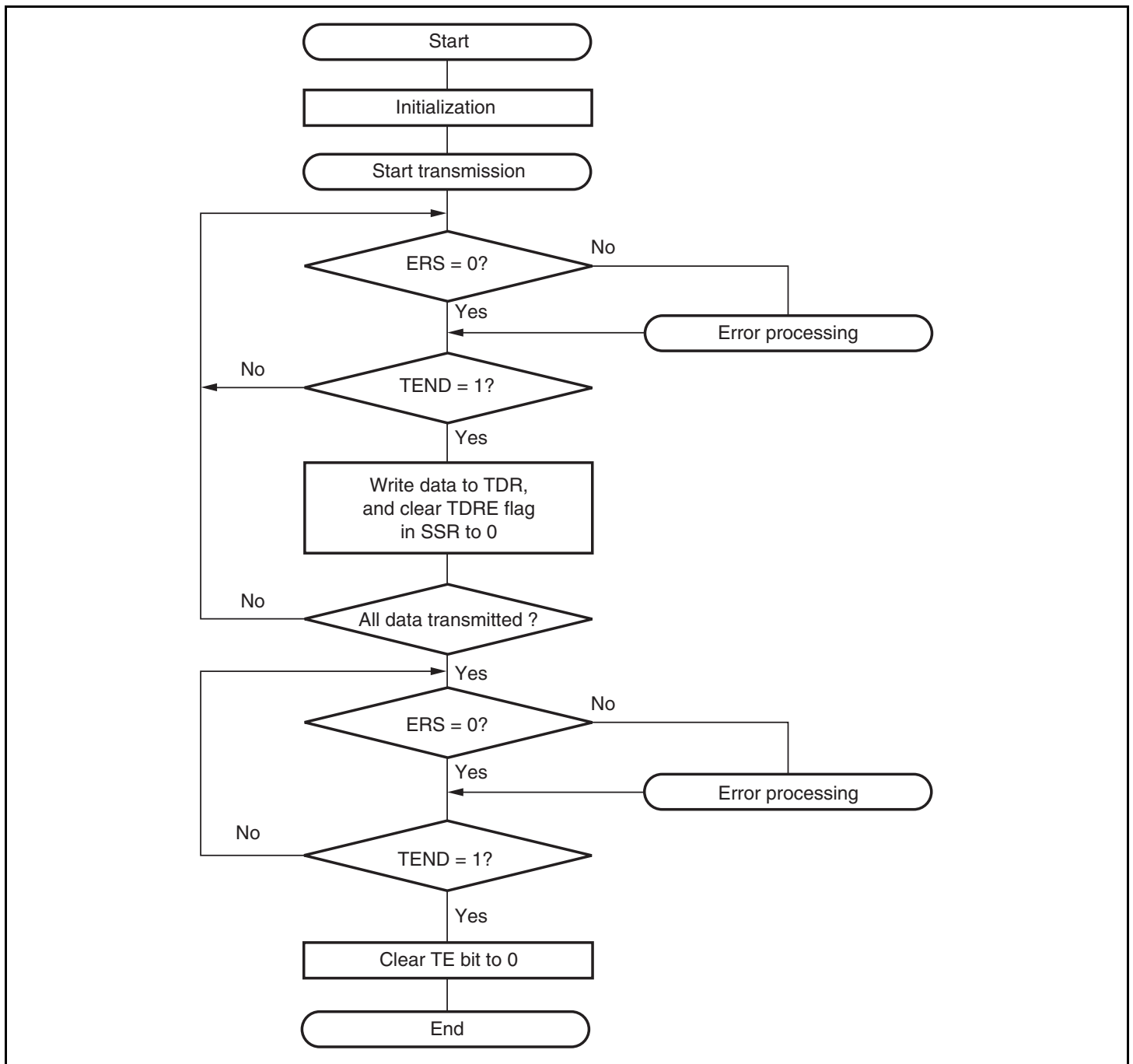
Figure 13.28 Example of Transmit Processing Flow
