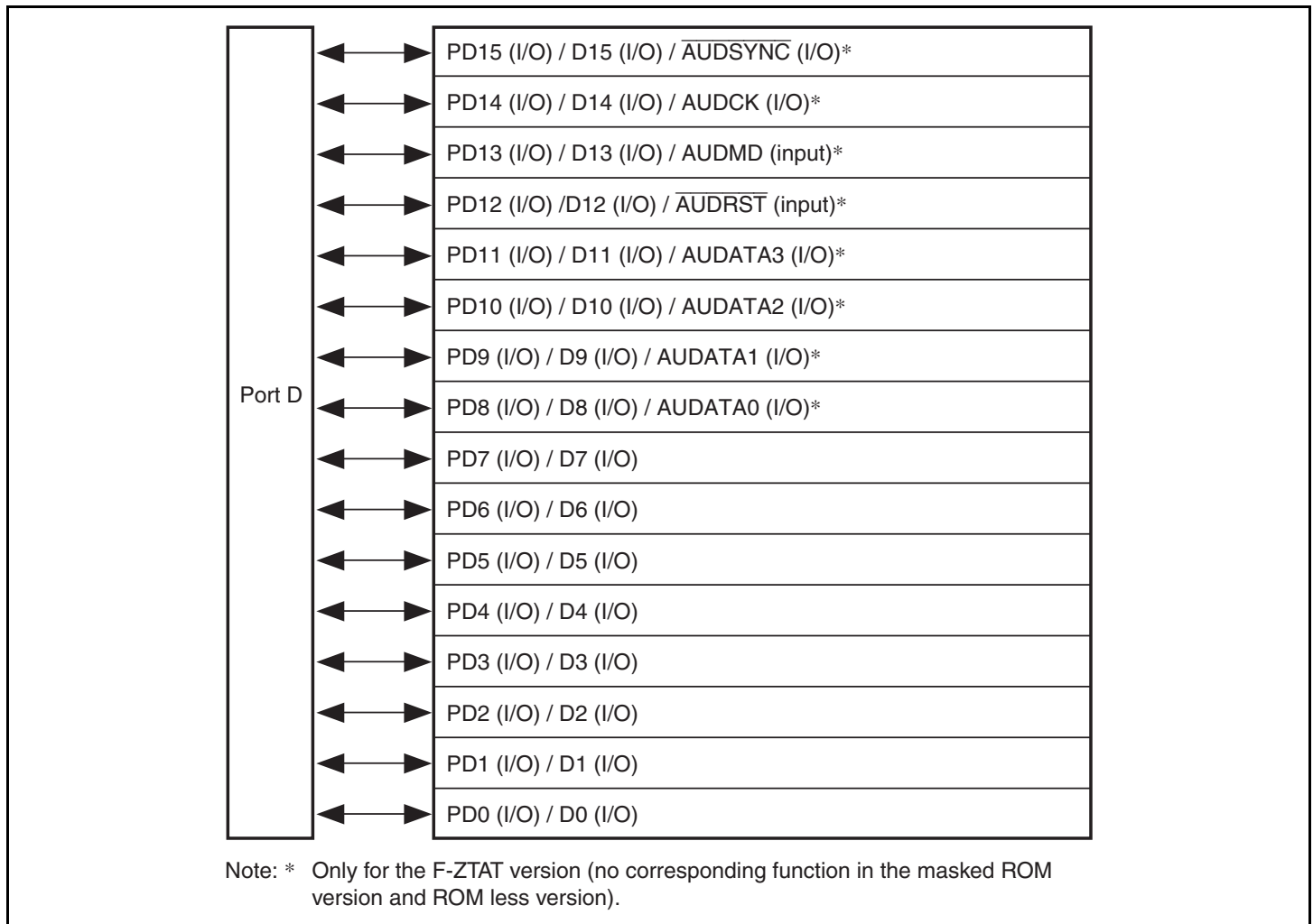
Figure 18.5 Port D (SH7144)
