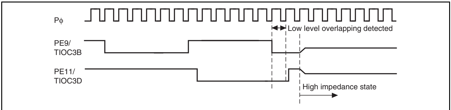
Figure 11.116 Output-Level Detection Operation
