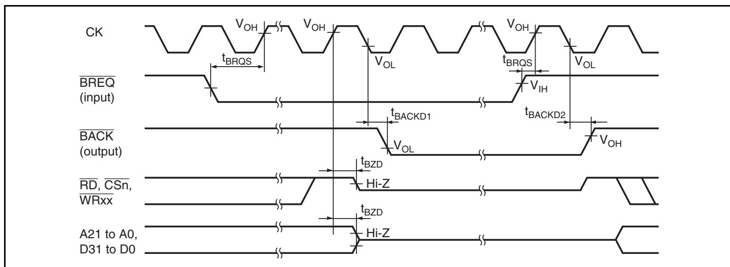
Figure 26.8 Bus Release Timing
