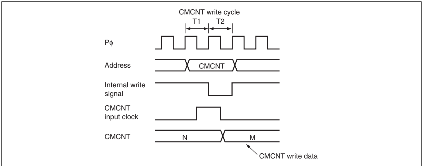
Figure 16.7 CMCNT Word Write and Increment Contention
