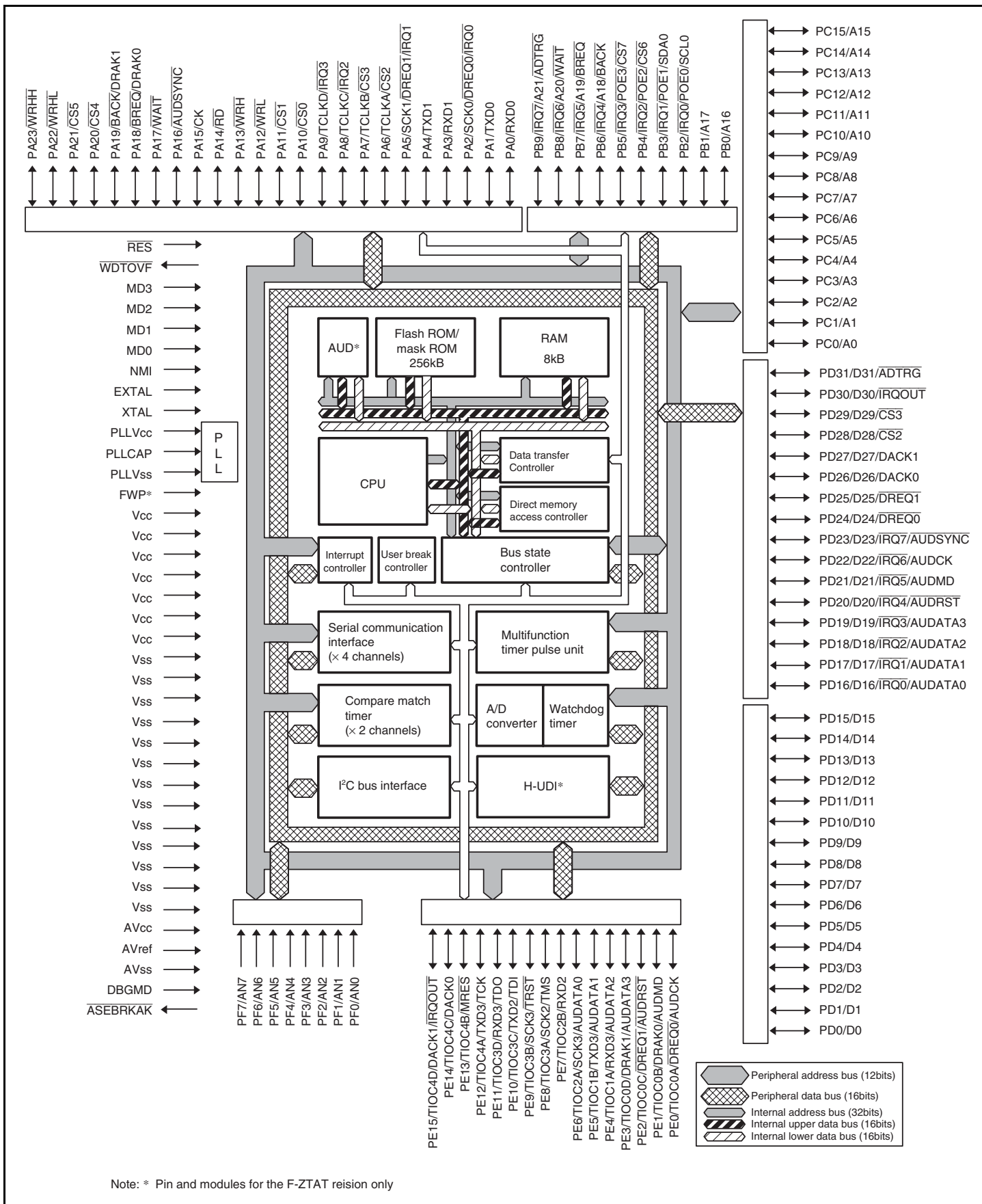
Figure 1.2 Block Diagram of SH7145
