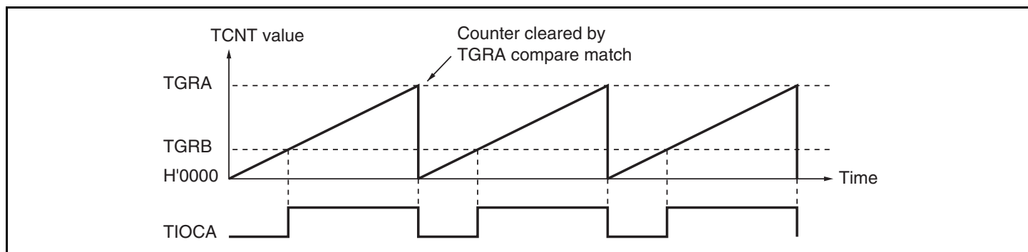
Figure 11.21 Example of PWM Mode Operation (1)
