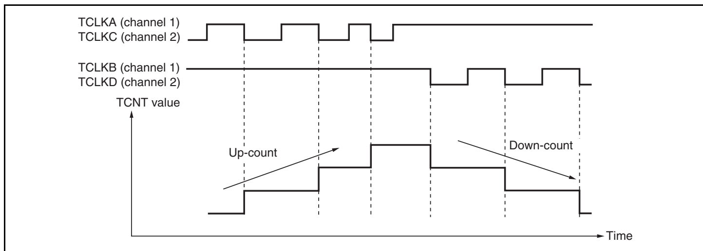
Figure 11.27 Example of Phase Counting Mode 3 Operation
