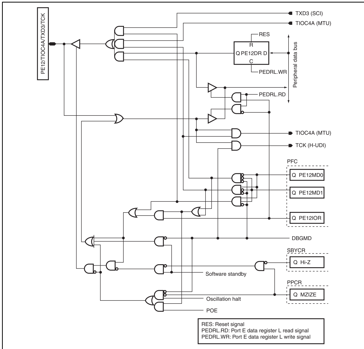
Figure D.56 PE12/TIOC4A/TXD3/TCK
