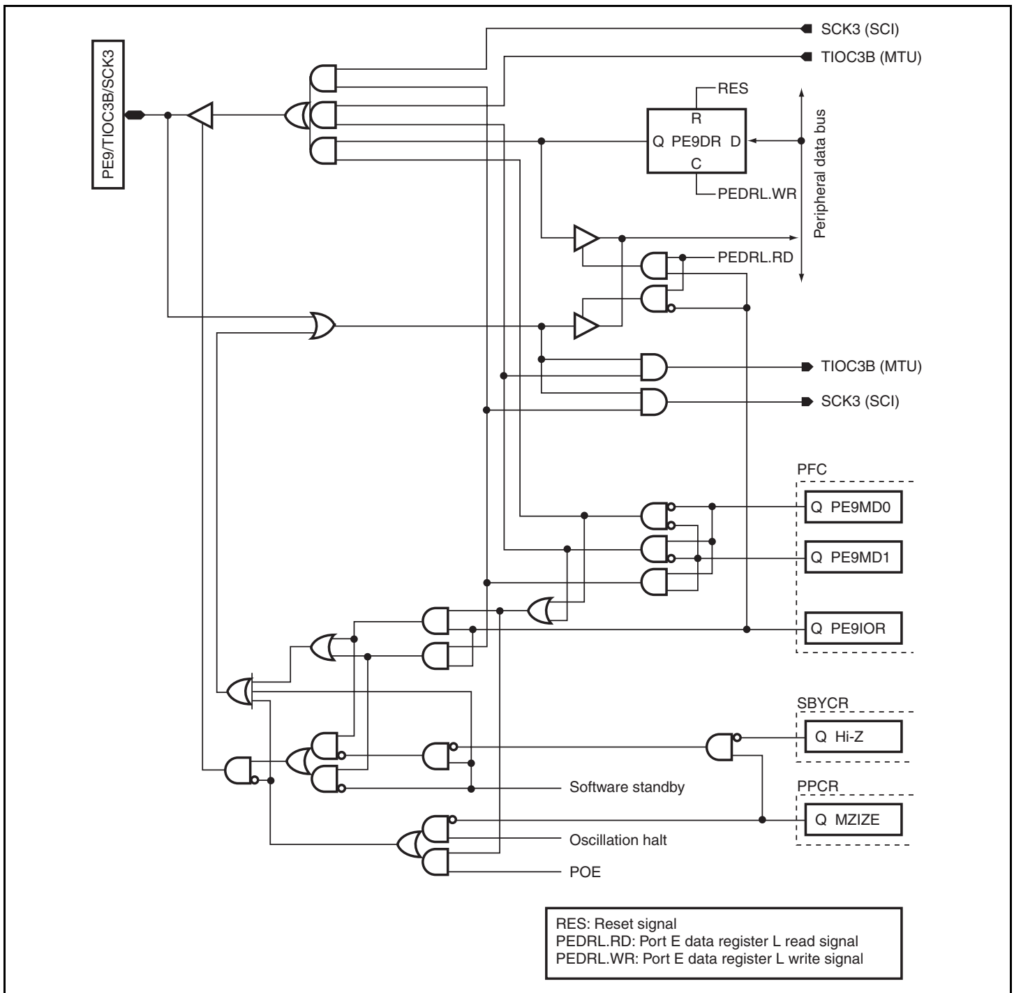
Figure D.37 PE9/TIOC3B/SCK3
