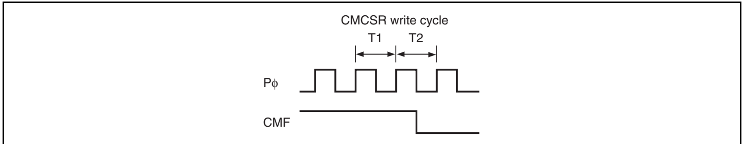
Figure 16.5 Timing of CMF Clear by CPU
