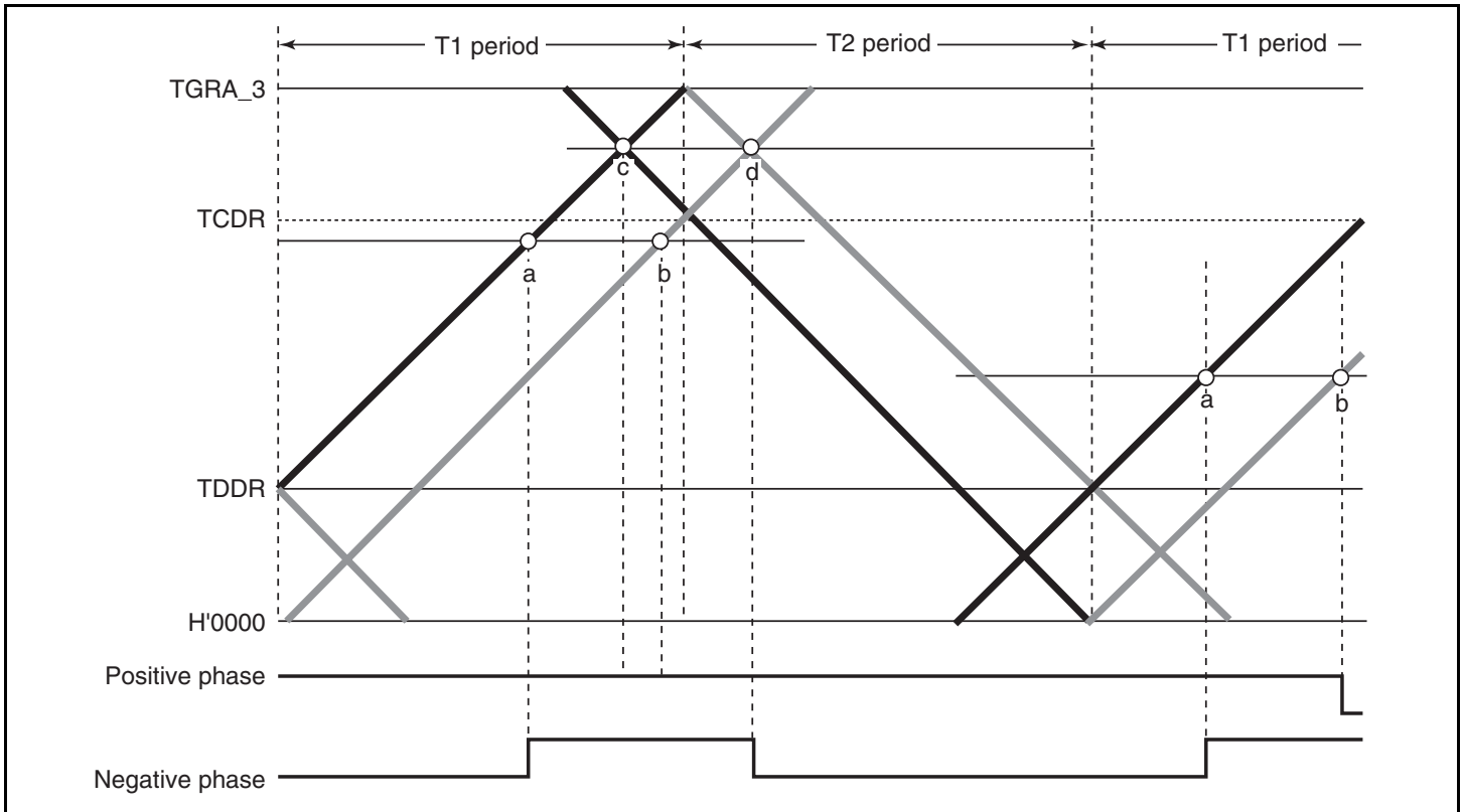
Figure 11.41 Example of Complementary PWM Mode Waveform Output (2)
