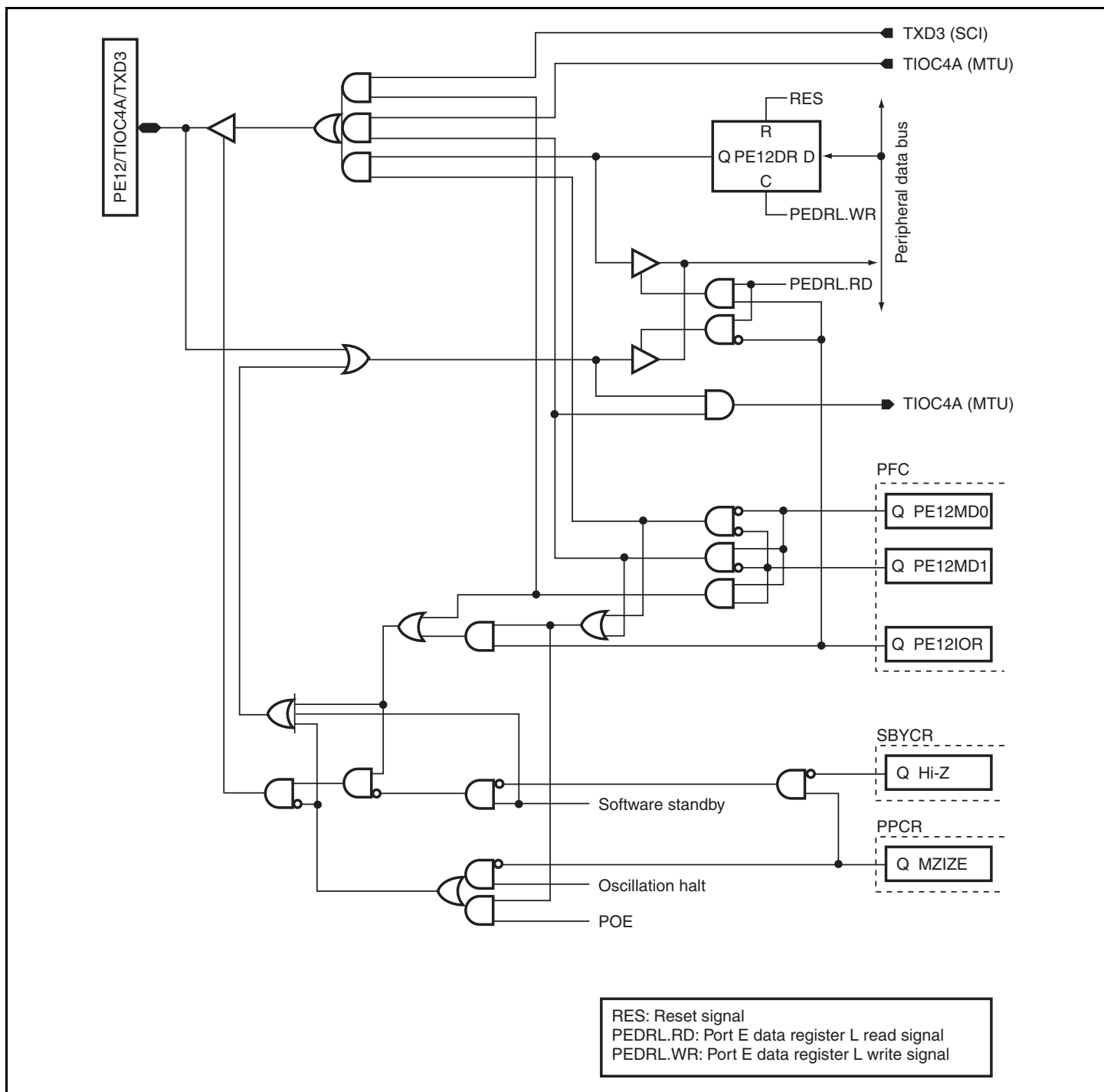
Figure D.39 PE12/TIOC4A/TXD3
