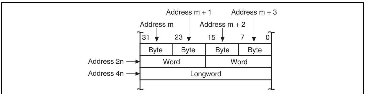
Figure 2.3 Data Formats in Memory
