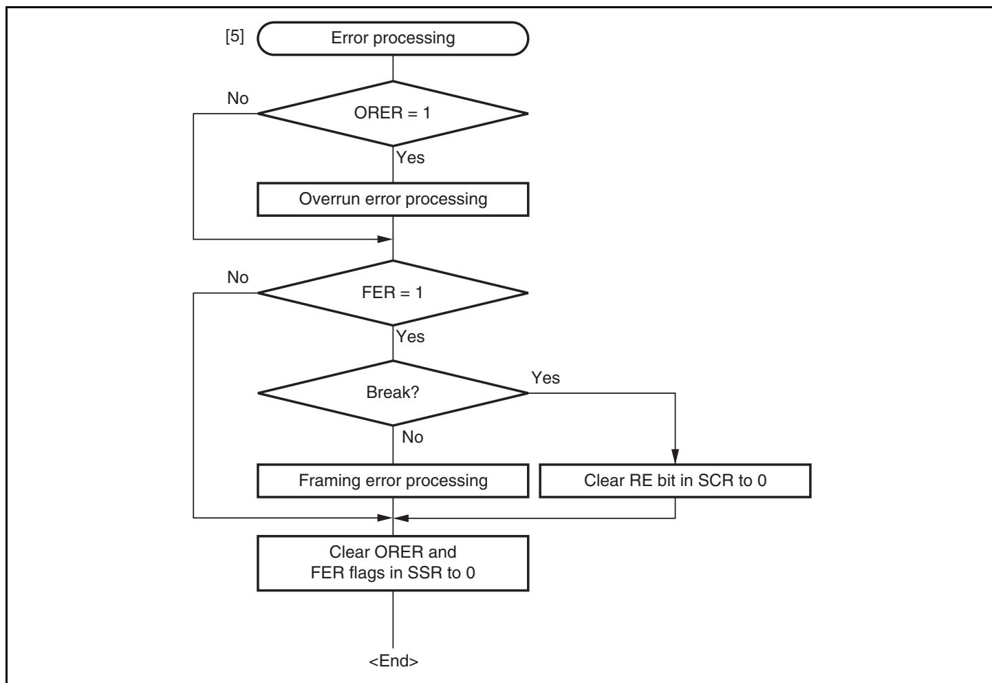
Figure 13.13 Sample Multiprocessor Serial Reception Flowchart (2)
