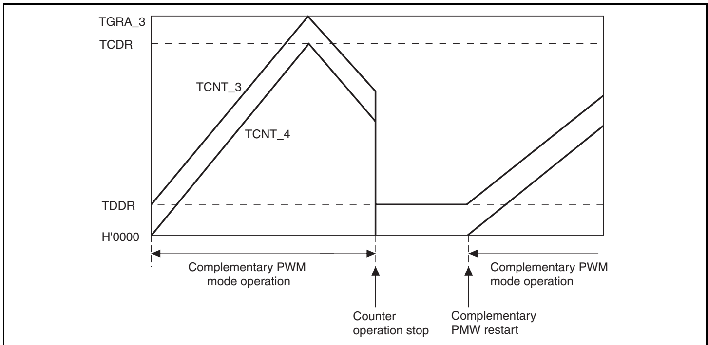
Figure 11.80 Counter Value during Complementary PWM Mode Stop
