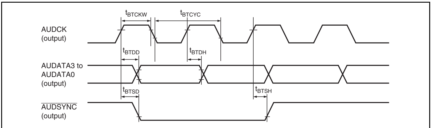
Figure 26.28 Branch Trace Timing
