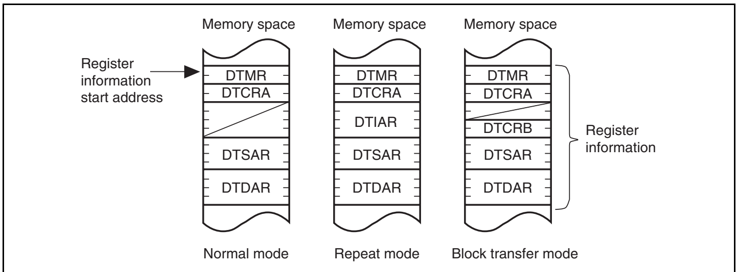
Figure 8.3 DTC Register Information Allocation in Memory Space
