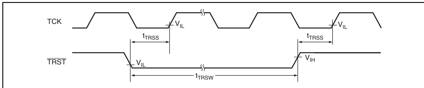
Figure 26.25 H-UDI \overline{\text{TRST}} Timing
