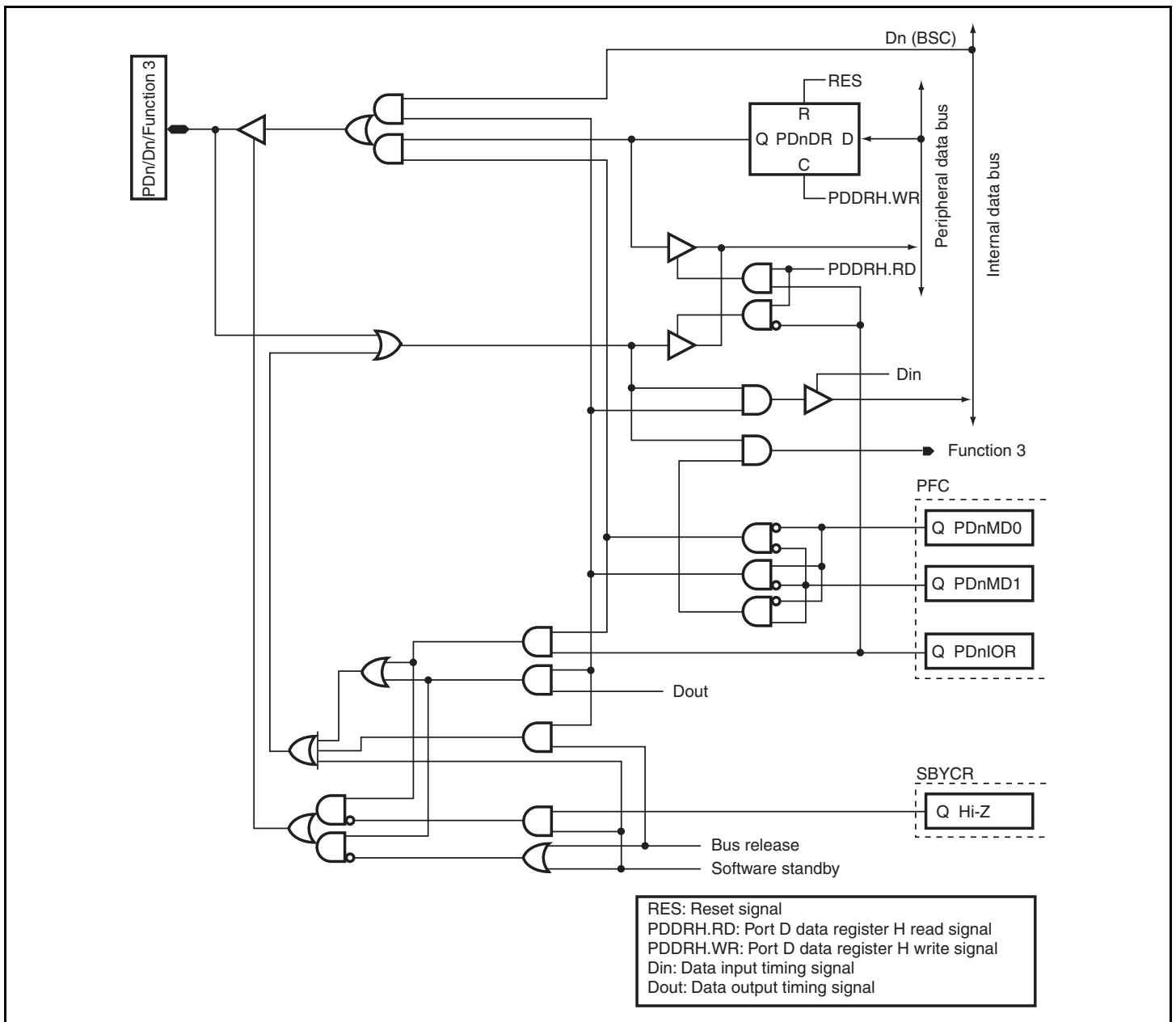
Figure D.31 PDn/Dn/Function 3
