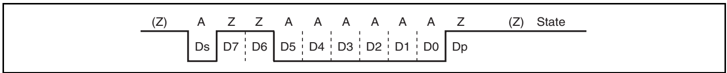
Figure 13.24 Inverse Convention ( DIR = SINV = O/\bar{E} = 1 )
