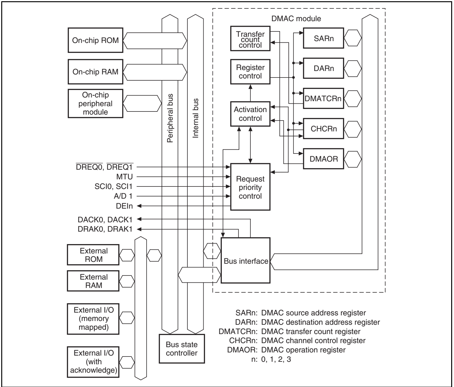
Figure 10.1 DMAC Block Diagram
