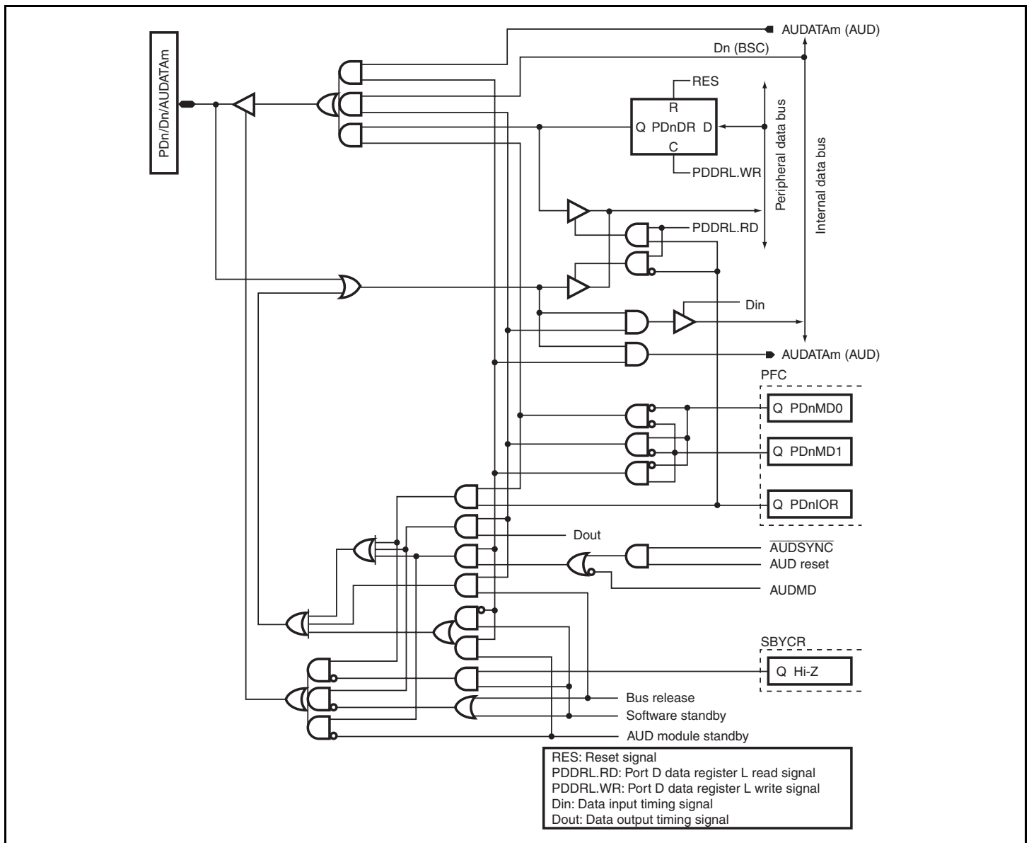
Figure D.24 PDn/Dn/AUDATAm
