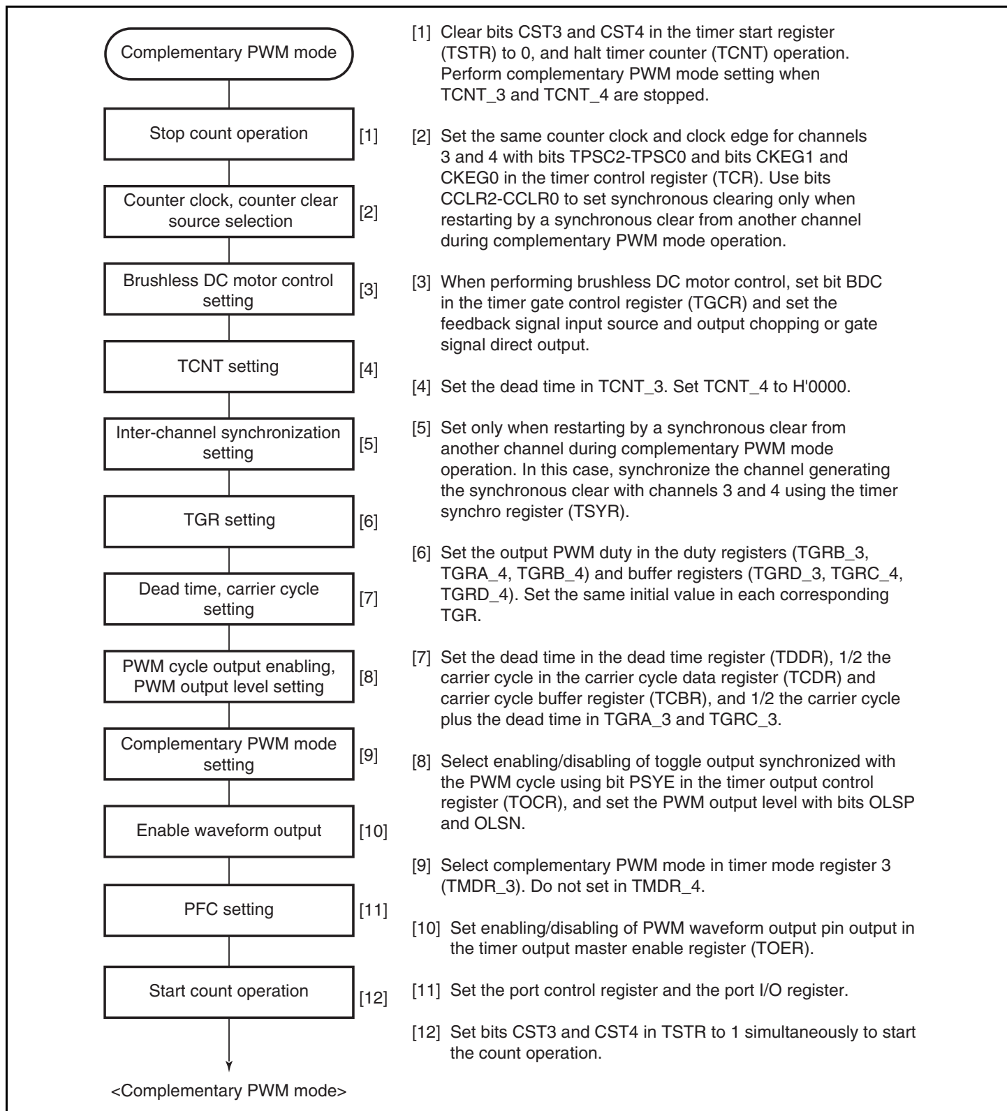
Figure 11.33 Example of Complementary PWM Mode Setting Procedure
