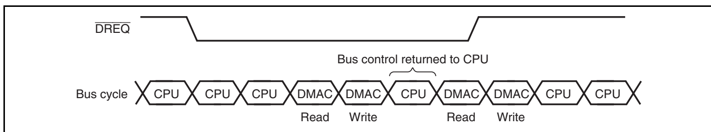
Figure 10.11 DMA Transfer Example in Cycle-Steal Mode
