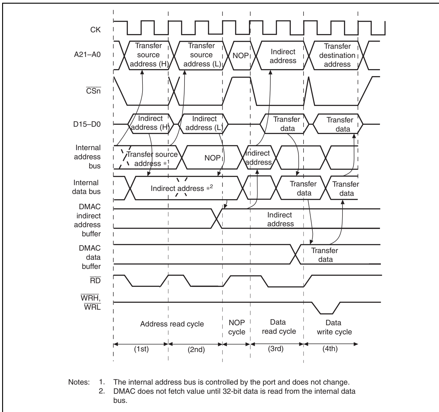
Figure 10.9 Dual Address Mode and Indirect Address Transfer Timing Example (External Memory Space to External Memory Space, 16-Bit Width)
