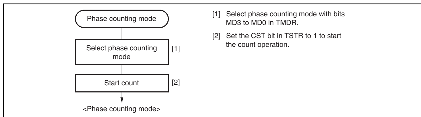
Figure 11.24 Example of Phase Counting Mode Setting Procedure
