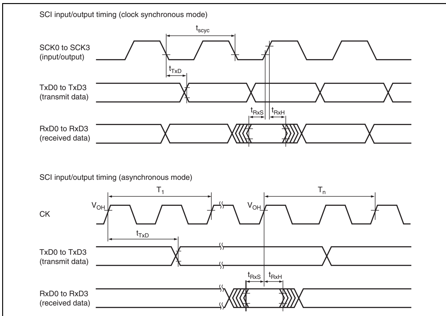
Figure 26.20 SCI Input/Output Timing
