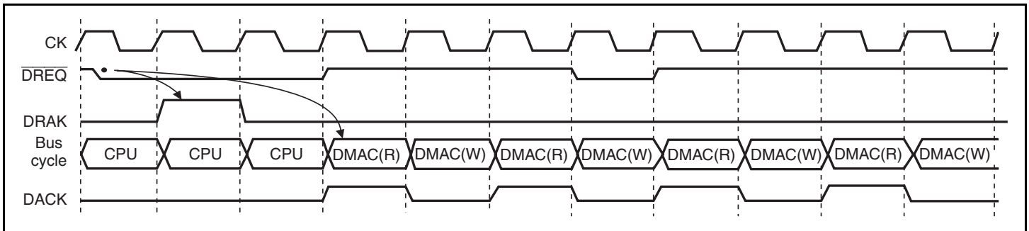
Figure 10.22 Burst Mode, Dual Address and Edge Detection
