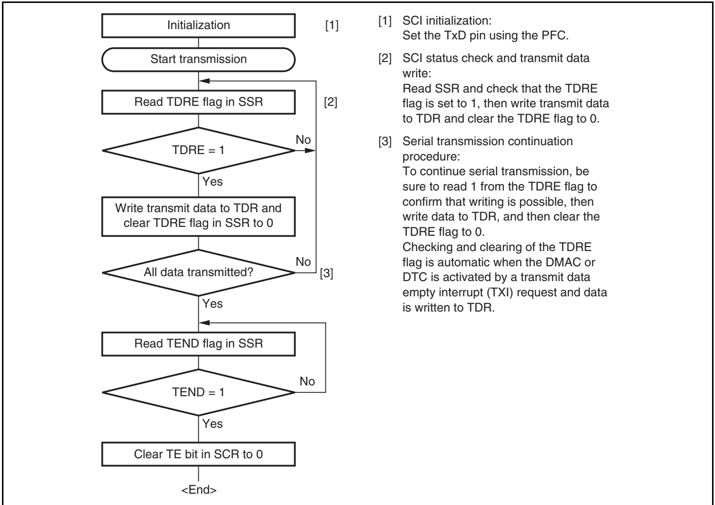
Figure 13.17 Sample Serial Transmission Flowchart
