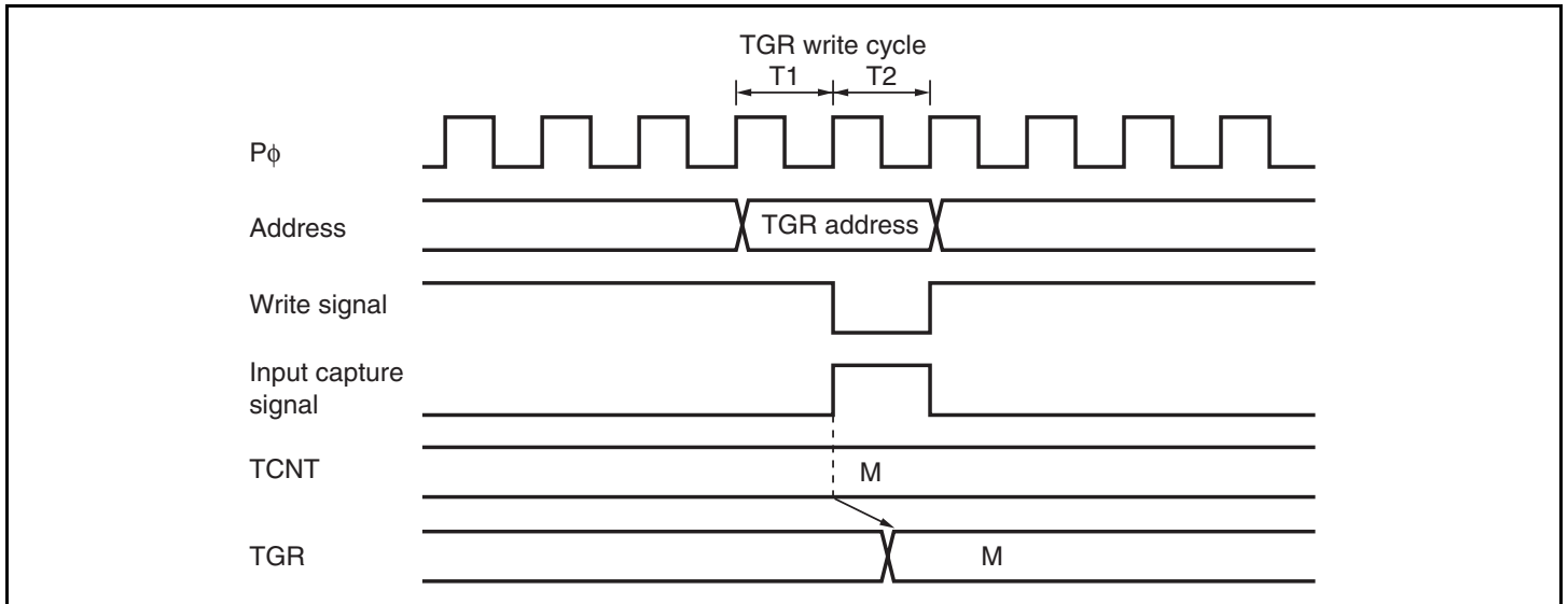
Figure 11.77 Contention between TGR Write and Input Capture
