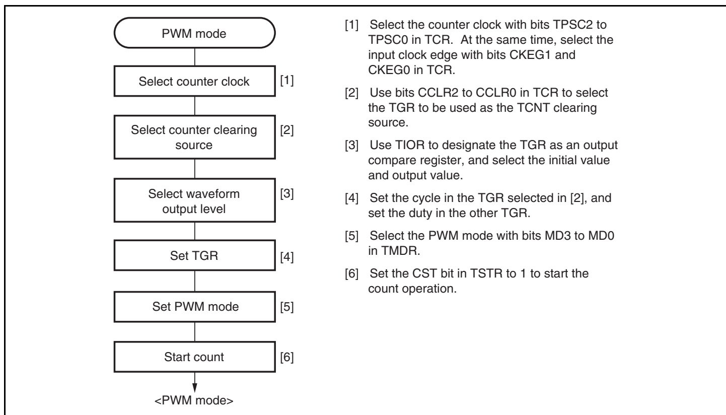
Figure 11.20 Example of PWM Mode Setting Procedure
