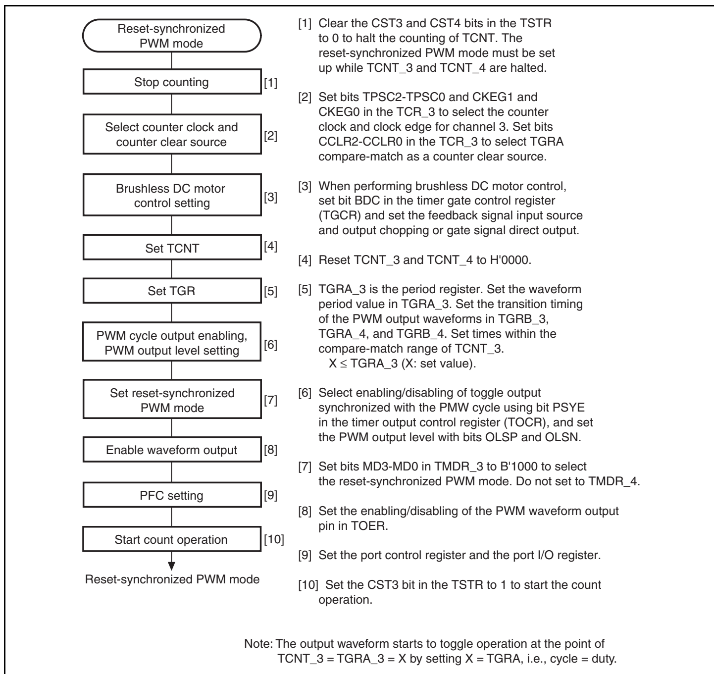
Figure 11.30 Procedure for Selecting Reset-Synchronized PWM Mode
