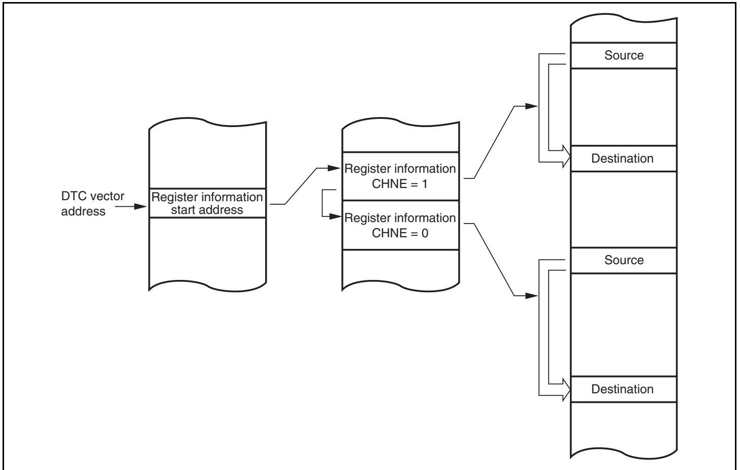
Figure 8.9 Chain Transfer
