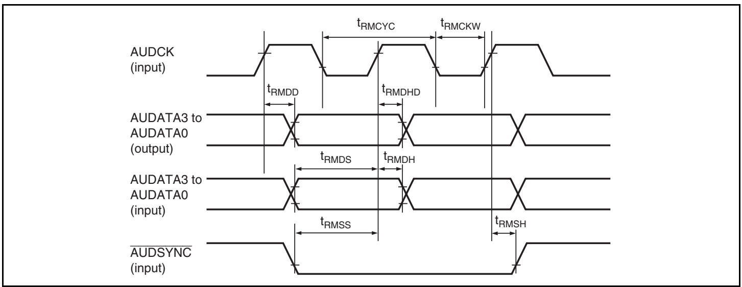
Figure 26.29 RAM Monitor Timing
