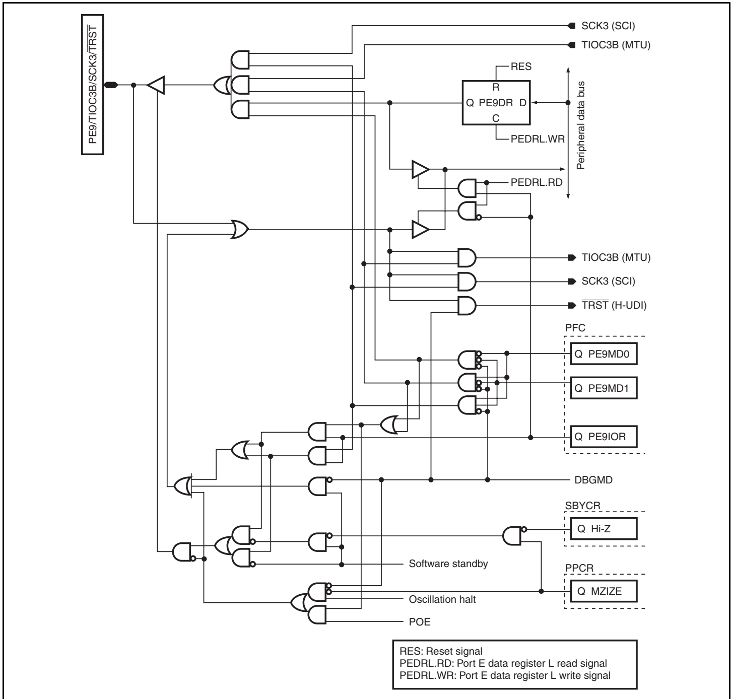
Figure D.53 PE9/TIOC3B/SCK3/TRST
