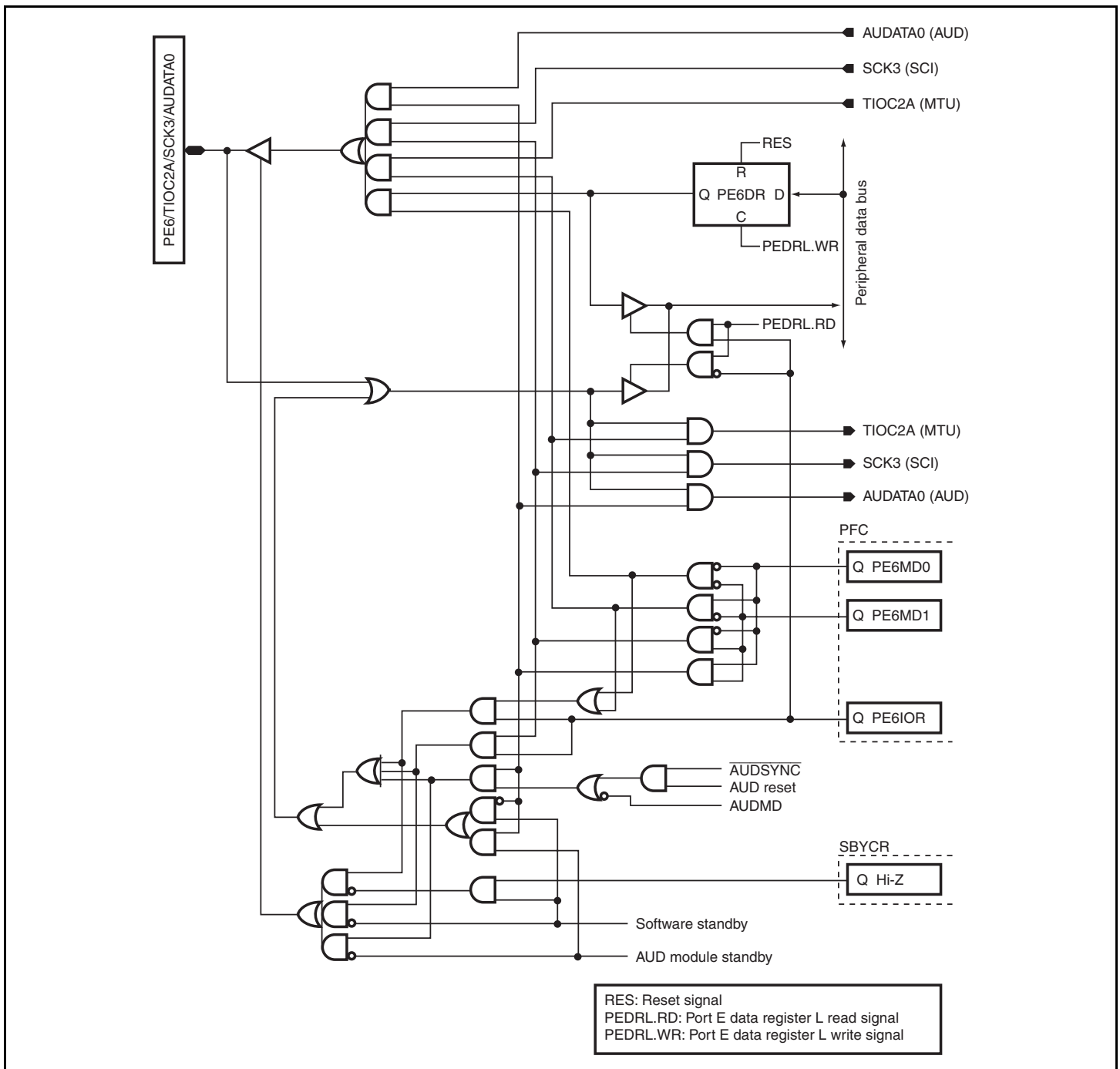
Figure D.51 PE6/TIOC2A/SCK3/AUDATA0
