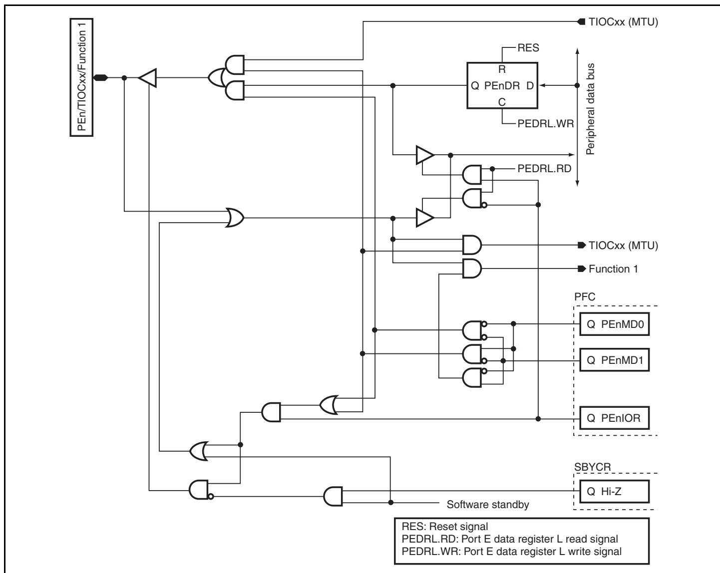
Figure D.34 PEn/TIOCxx/Function 1
