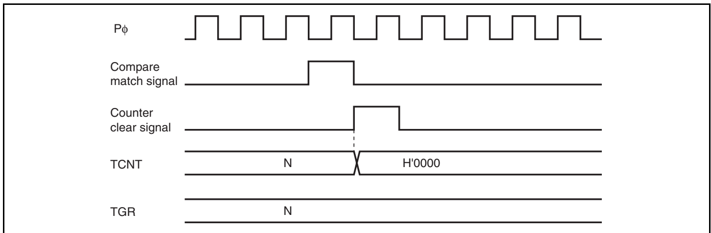
Figure 11.60 Counter Clear Timing (Compare Match)
