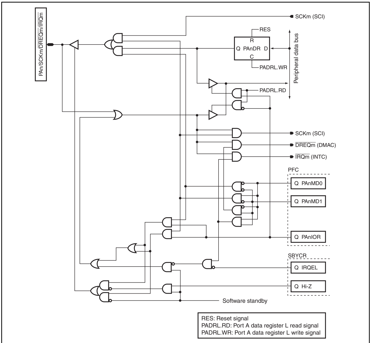
Figure D.3 PAn/SCKm/DREQm/IRQm
