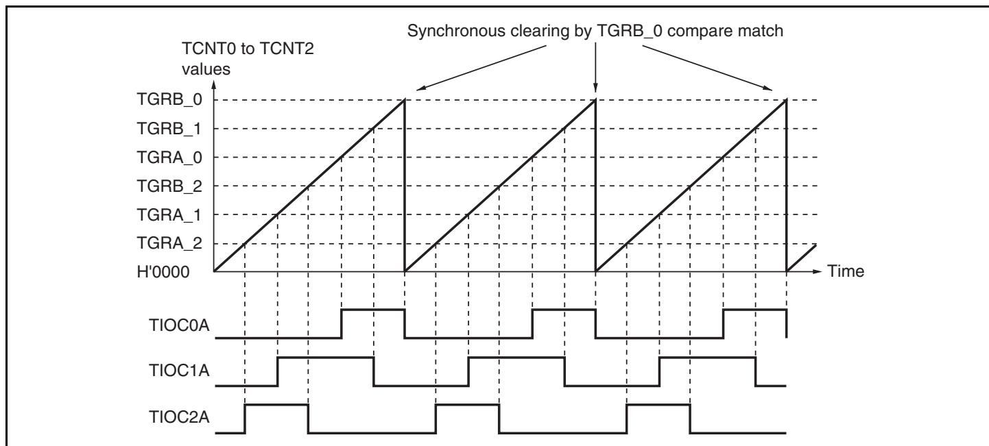
Figure 11.12 Example of Synchronous Operation
