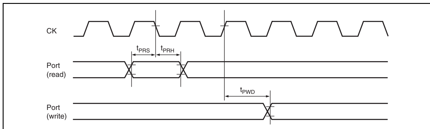
Figure 26.17 I/O Port Input/Output timing
