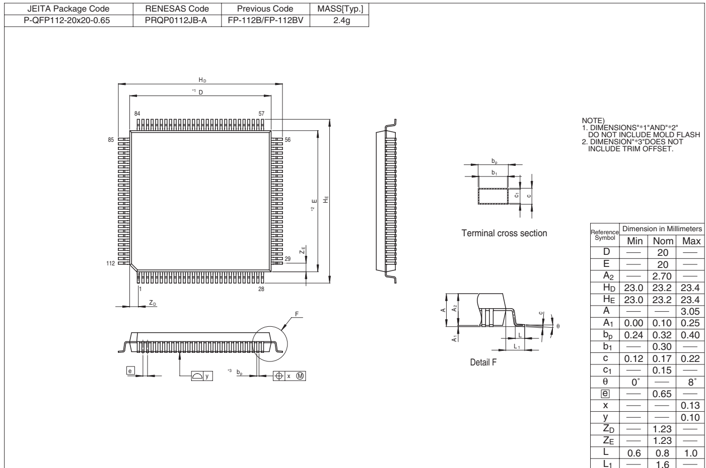
Figure E.1 FP-112B
