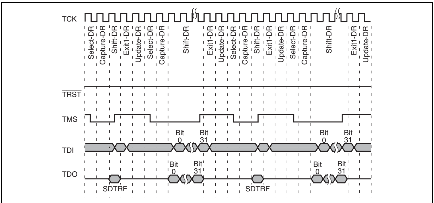
Figure 22.4 Data Input/Output Timing Chart (3)
