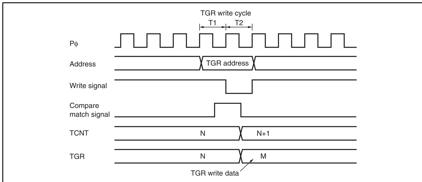
Figure 11.73 Contention between TGR Write and Compare Match
