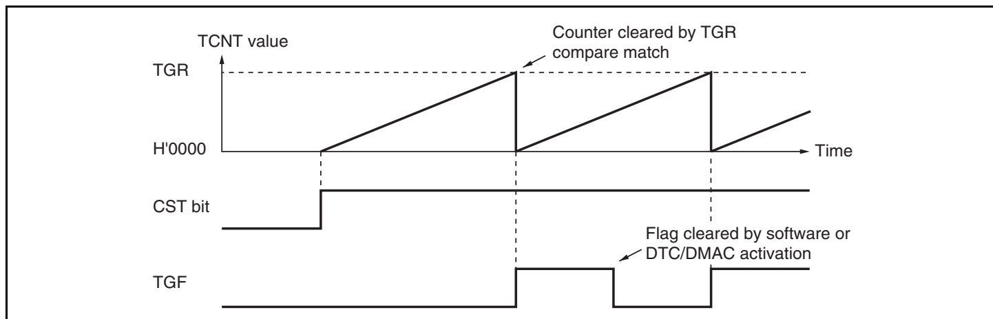
Figure 11.5 Periodic Counter Operation
