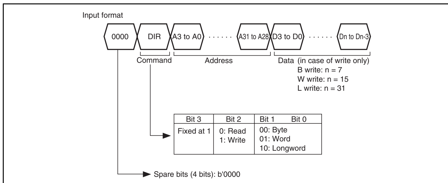
Figure 23.4 AUDATA Input Format
