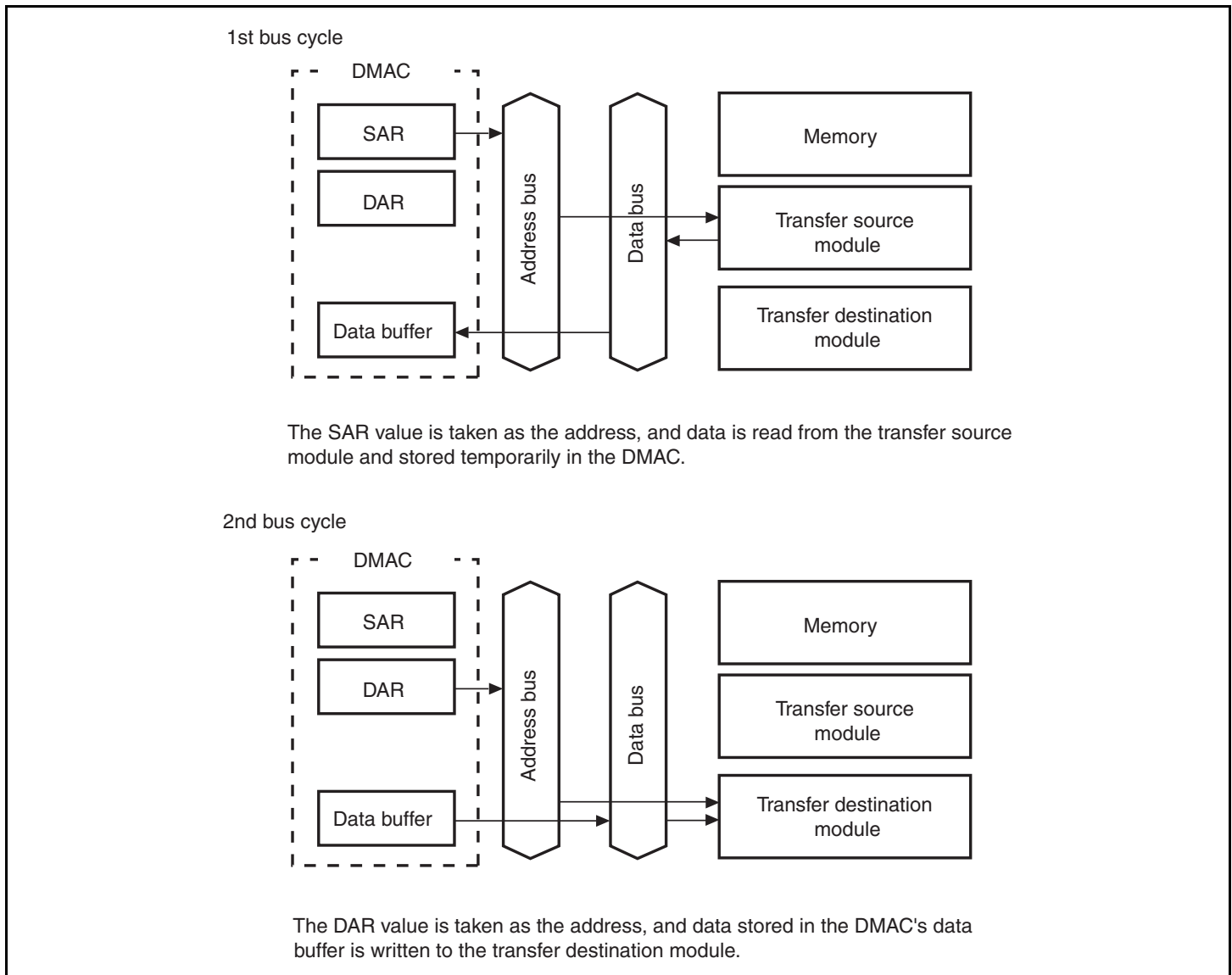
Figure 10.6 Direct Address Operation during Dual Address Mode
