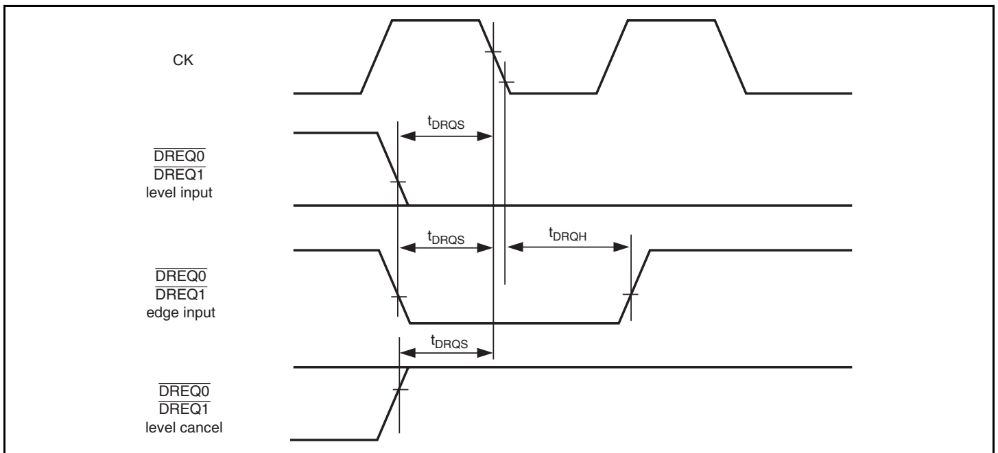
Figure 26.12 \overline{\text{DREQ0}} , \overline{\text{DREQ1}} Input Timing (1)
