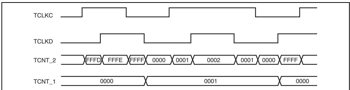
Figure 11.19 Example of Cascaded Operation
