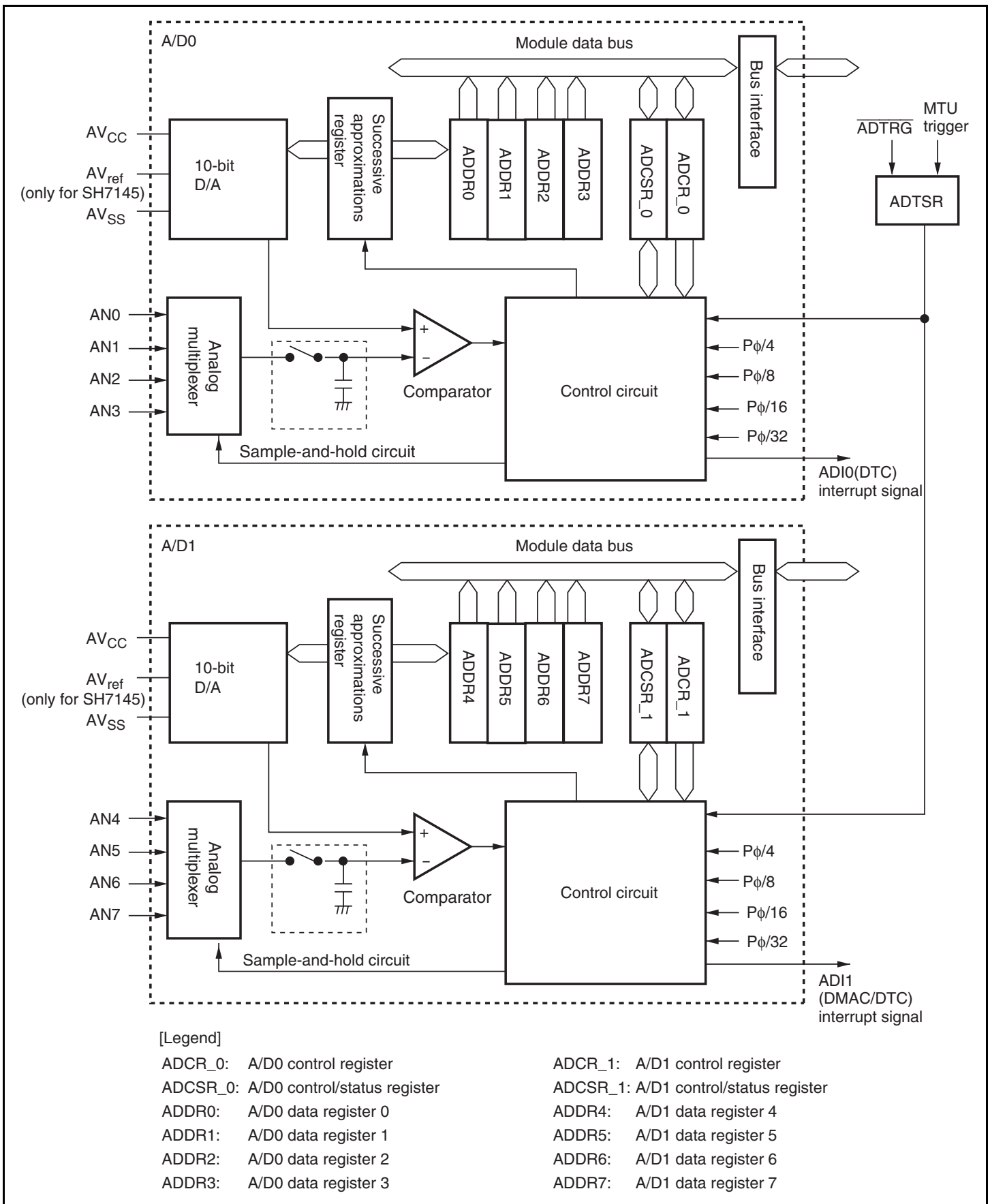
Figure 15.1 Block Diagram of A/D Converter
