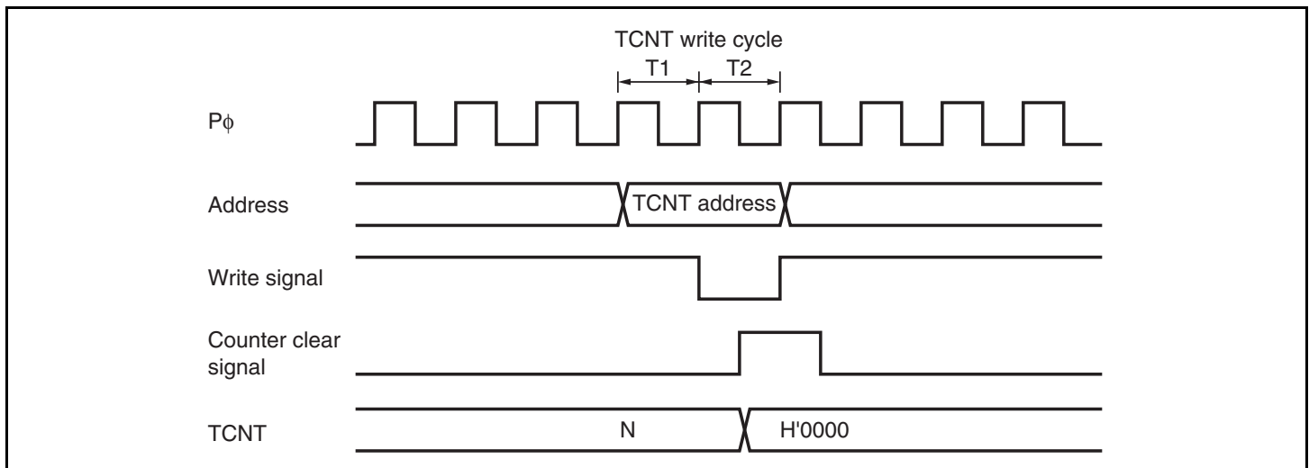
Figure 11.71 Contention between TCNT Write and Clear Operations
