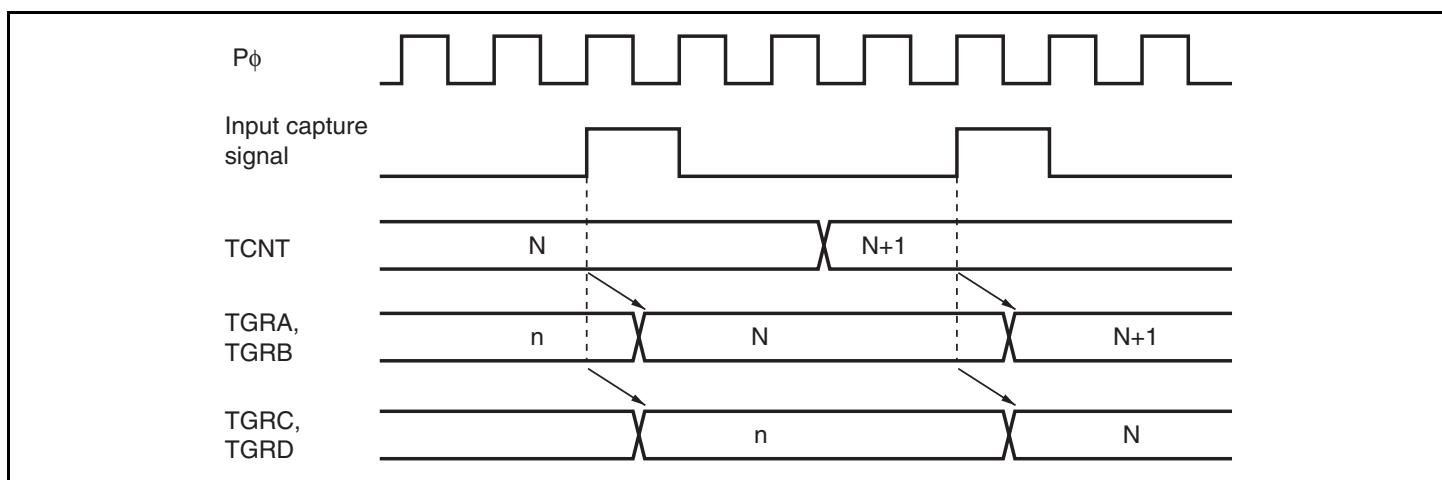
Figure 11.63 Buffer Operation Timing (Input Capture)
