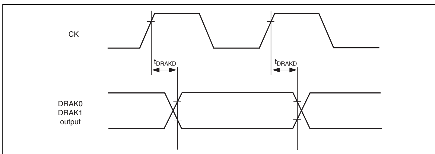
Figure 26.14 DRAK Output Delay Time
