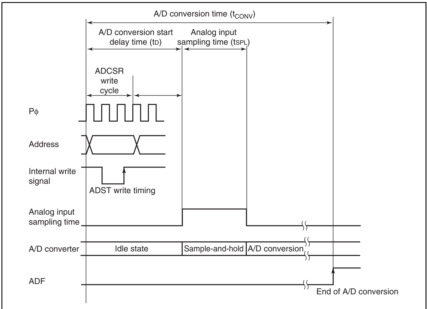
Figure 15.2 A/D Conversion Timing
