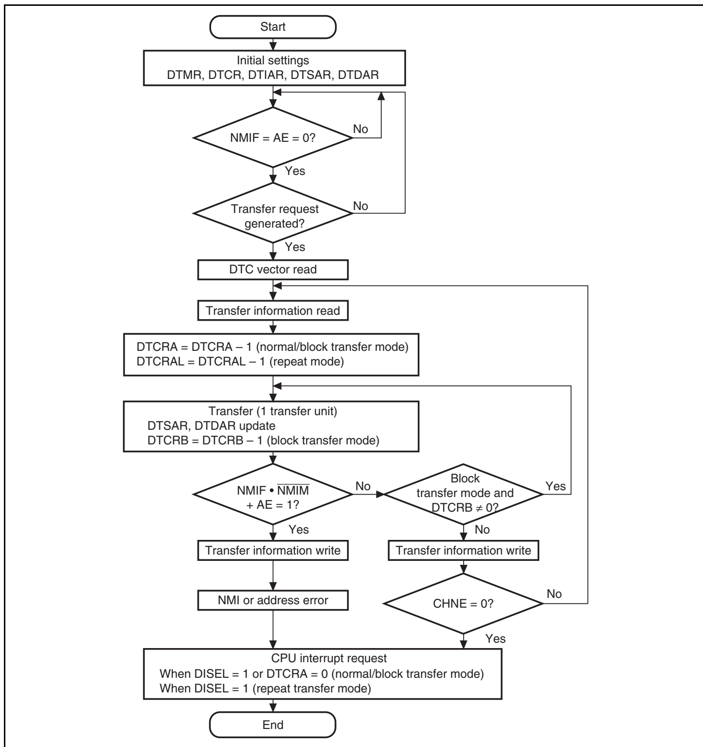
Figure 8.5 DTC Operation Flowchart
