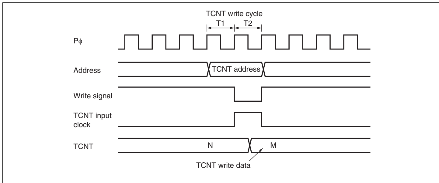
Figure 11.72 Contention between TCNT Write and Increment Operations
