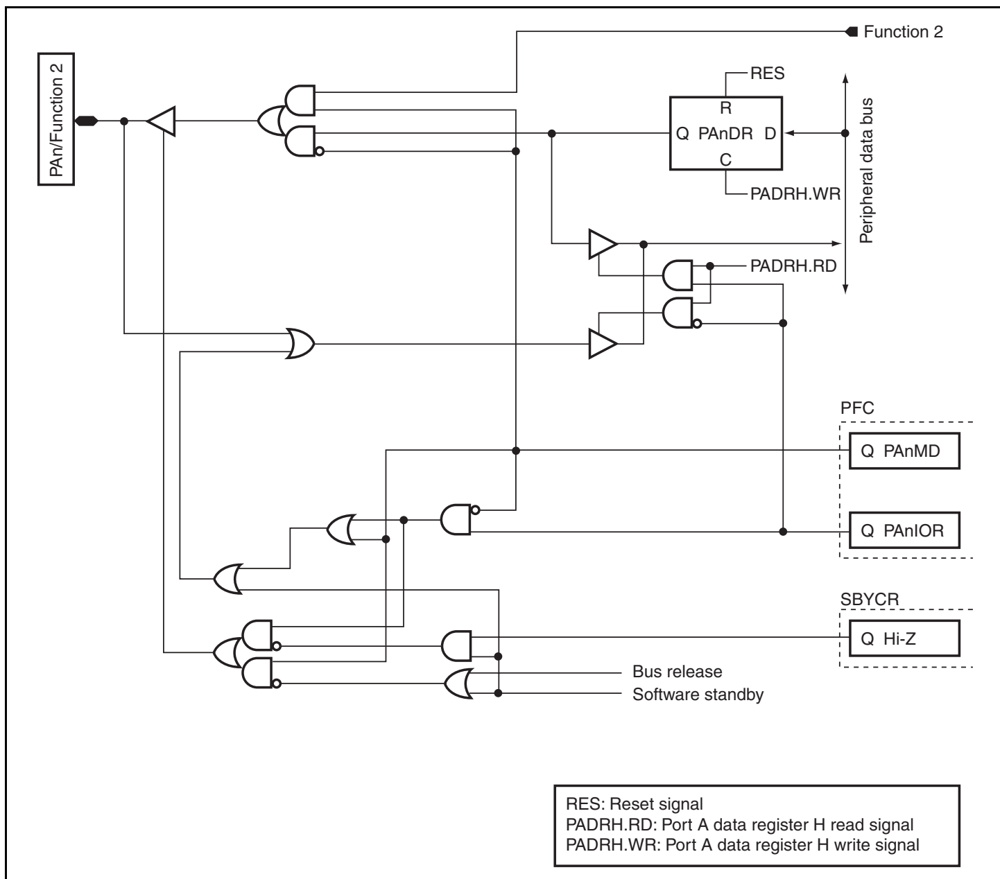
Figure D.13 PAn/Function 2
