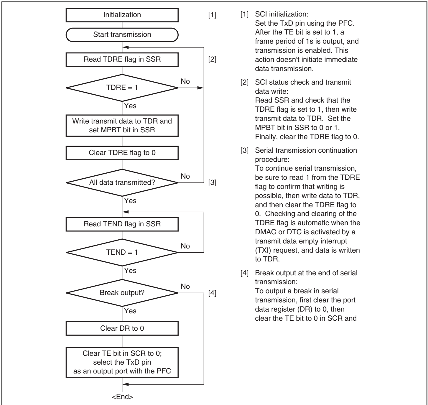
Figure 13.11 Sample Multiprocessor Serial Transmission Flowchart
