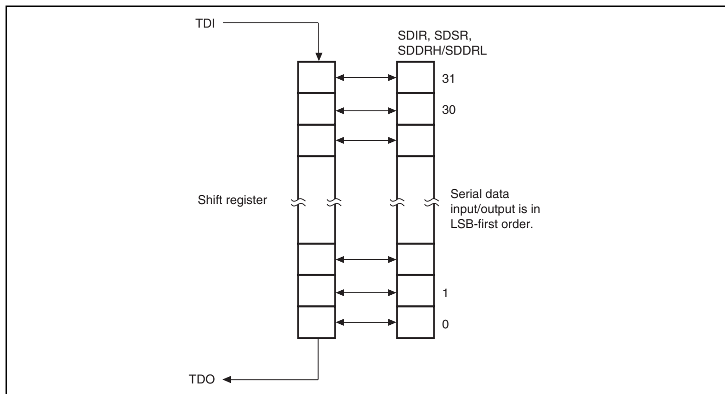
Figure 22.5 Serial Data Input/Output
