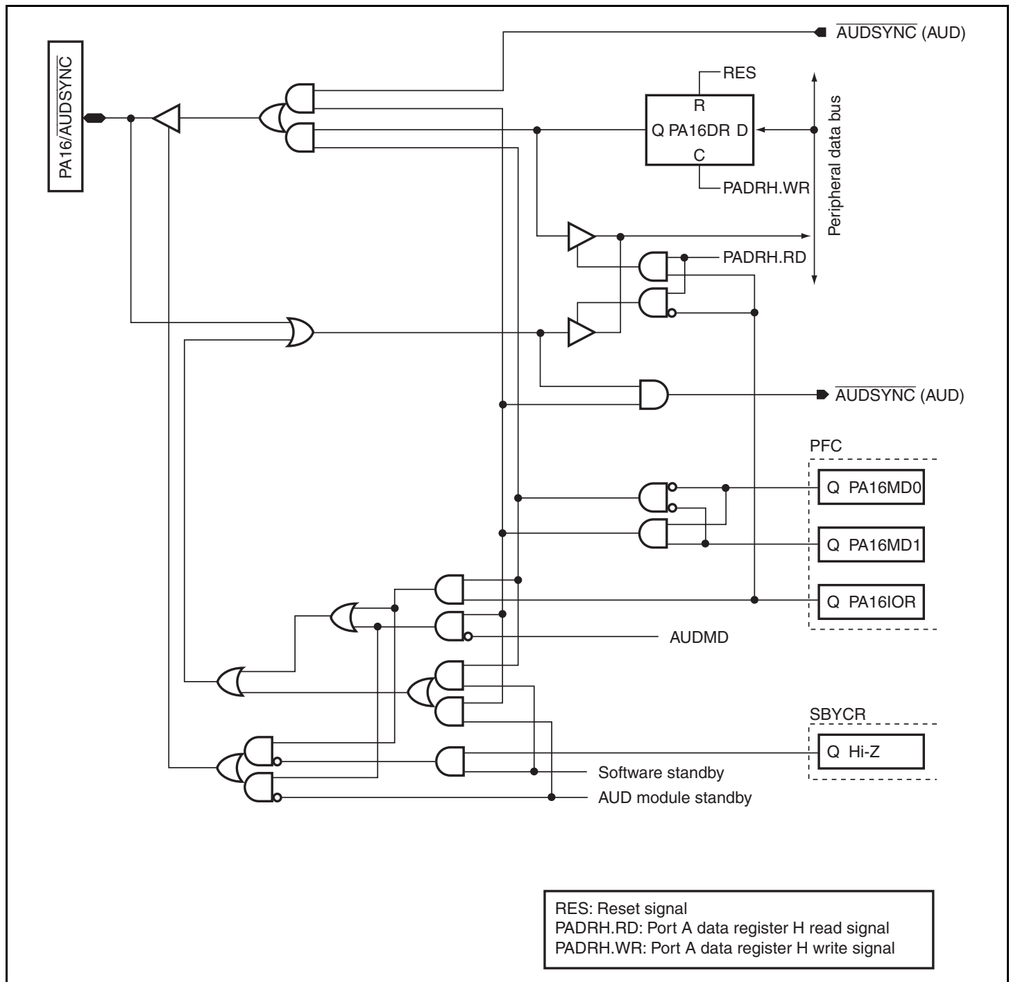
Figure D.8 PA16/AUDSYNC
