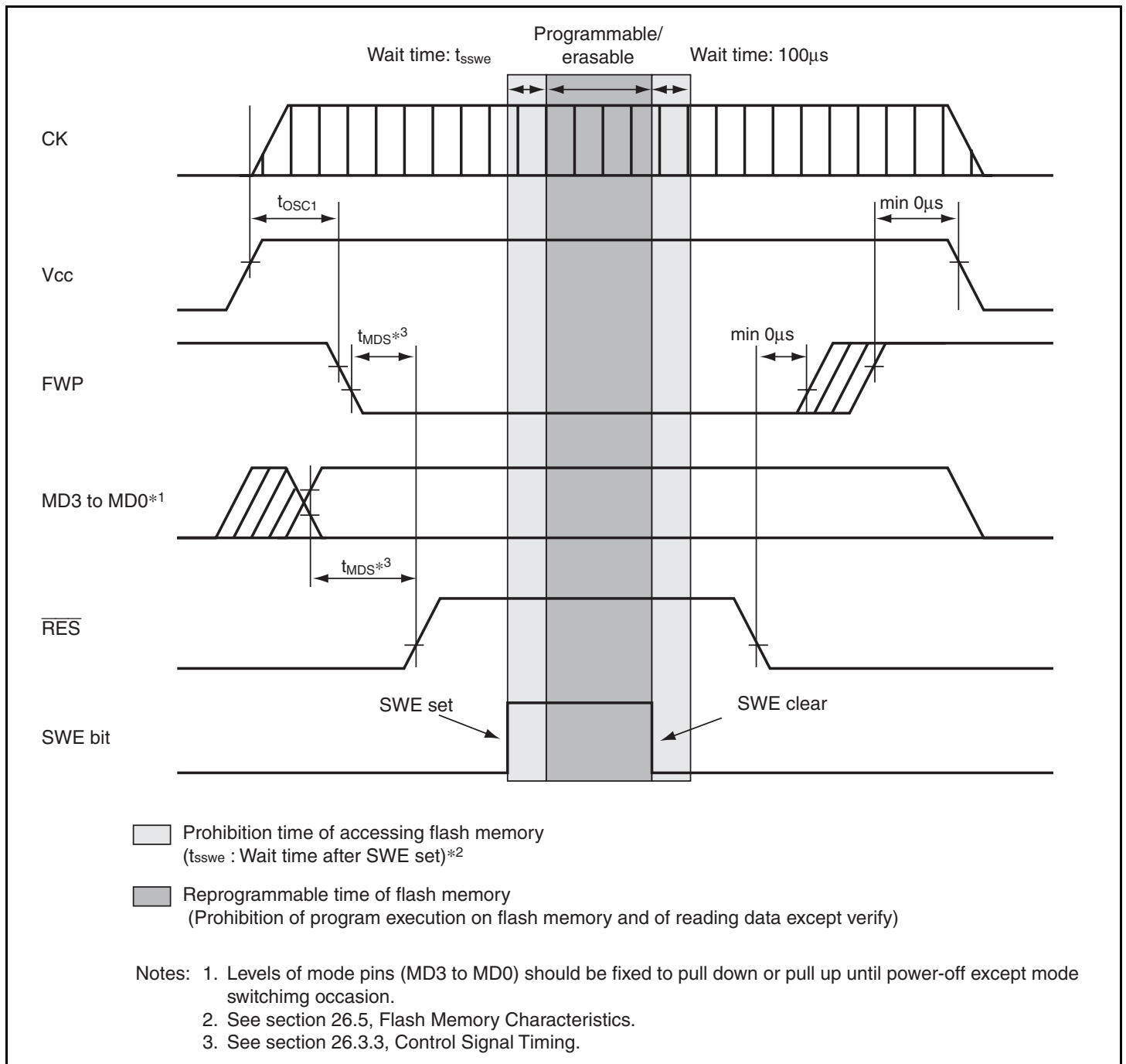
Figure 19.11 Power On/Off Timing (Boot Mode)
