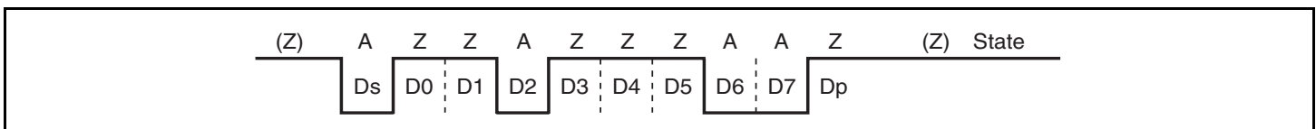
Figure 13.23 Direct Convention (DIR = SINV = \overline{O/E} = 0)
