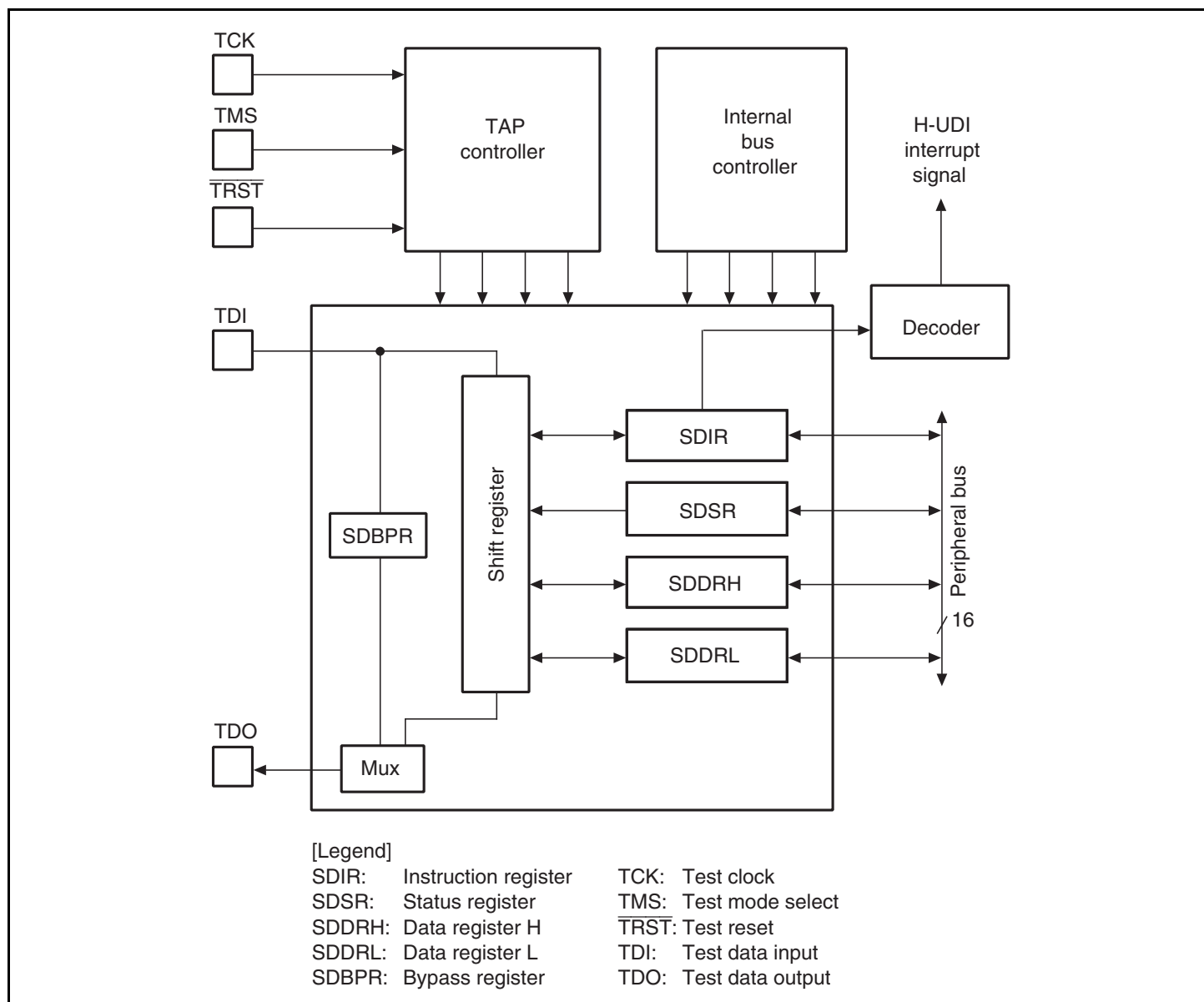
Figure 22.1 H-UDI Block Diagram
