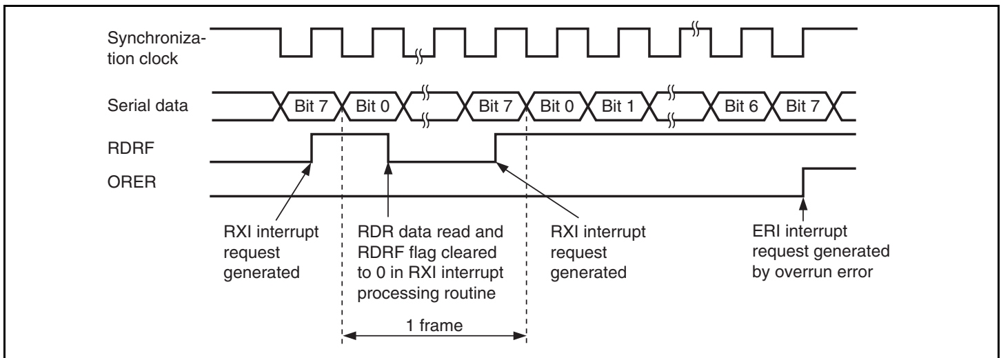
Figure 13.18 Example of SCI Operation in Reception
