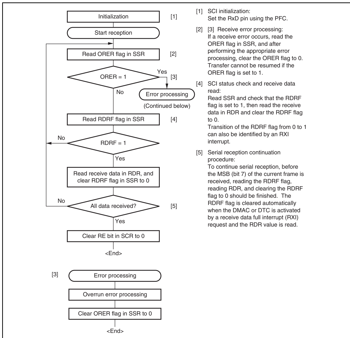
Figure 13.19 Sample Serial Reception Flowchart
