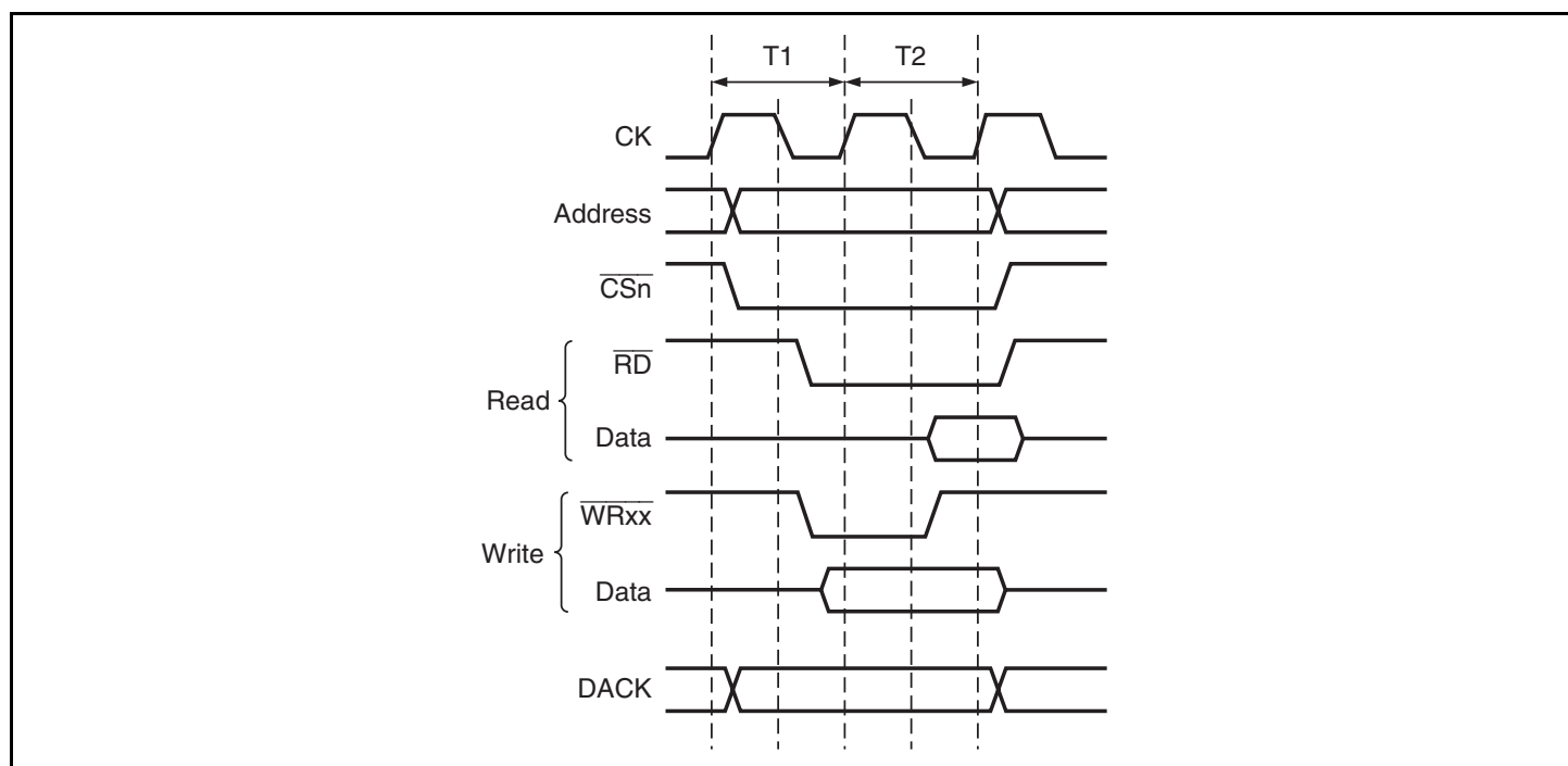
Figure 9.3 Basic Timing of External Space Access
