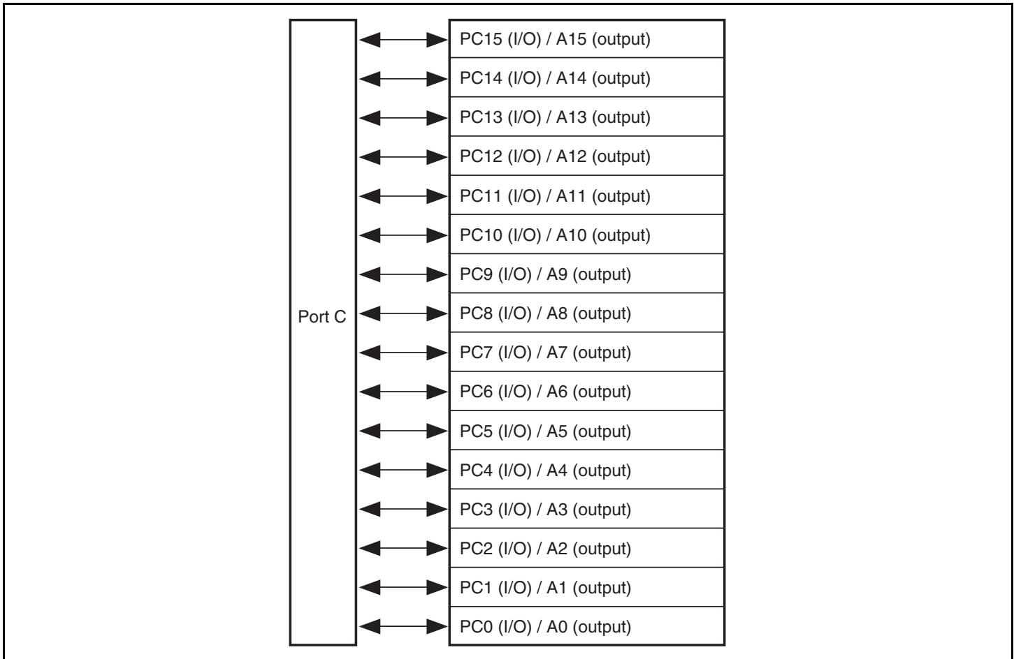
Figure 18.4 Port C
