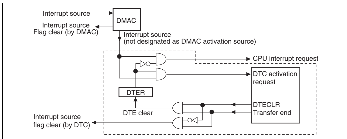
Figure 6.6 Interrupt Control Block Diagram
