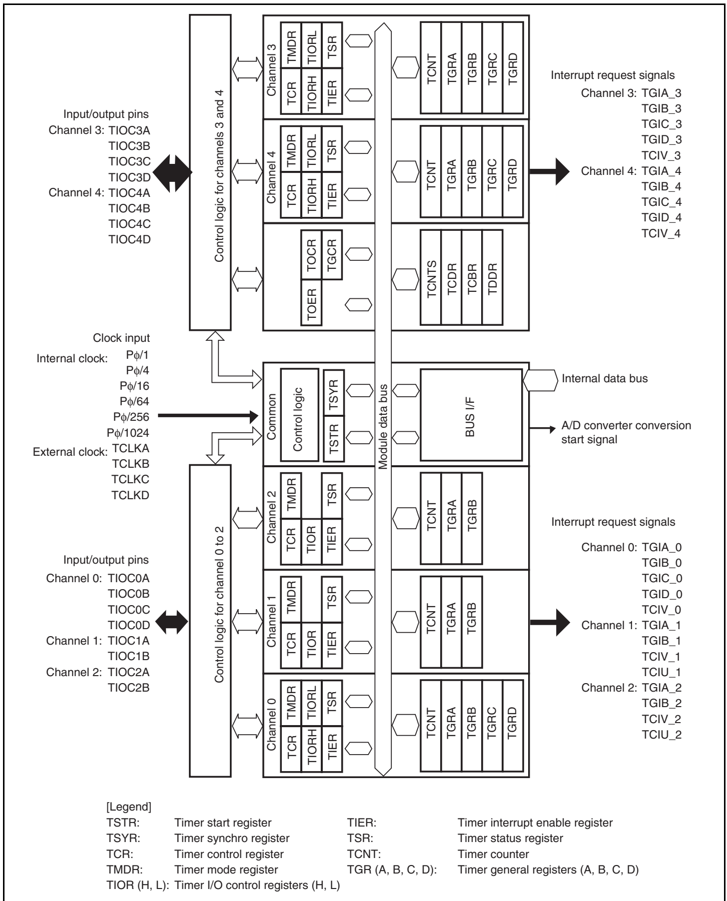
Figure 11.1 Block Diagram of MTU
