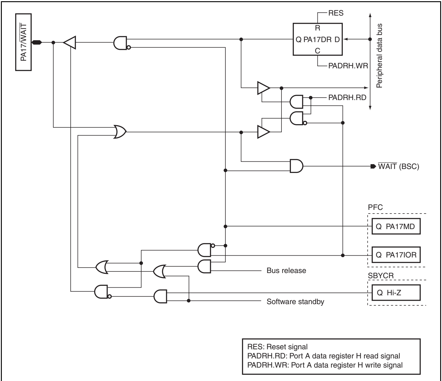
Figure D.9 PA17/ \overline{\text{WAIT}}
