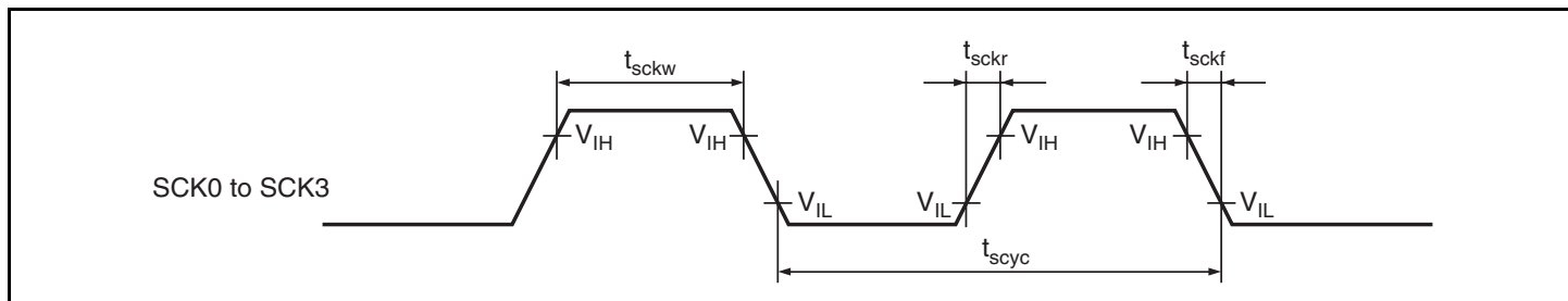
Figure 26.19 SCI Input Timing
