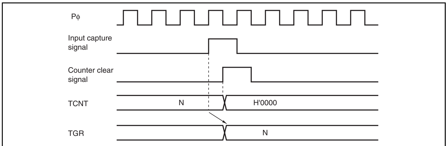
Figure 11.61 Counter Clear Timing (Input Capture)
