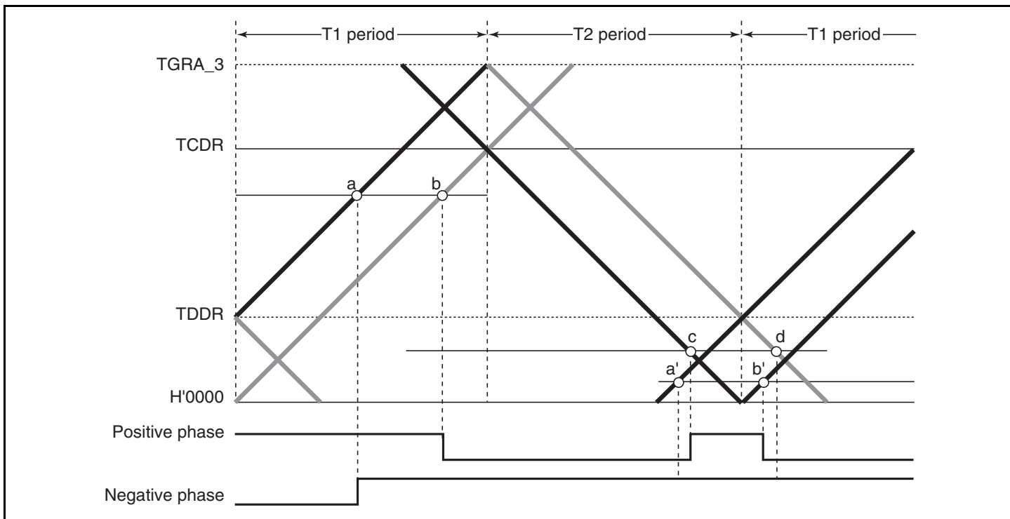
Figure 11.42 Example of Complementary PWM Mode Waveform Output (3)
