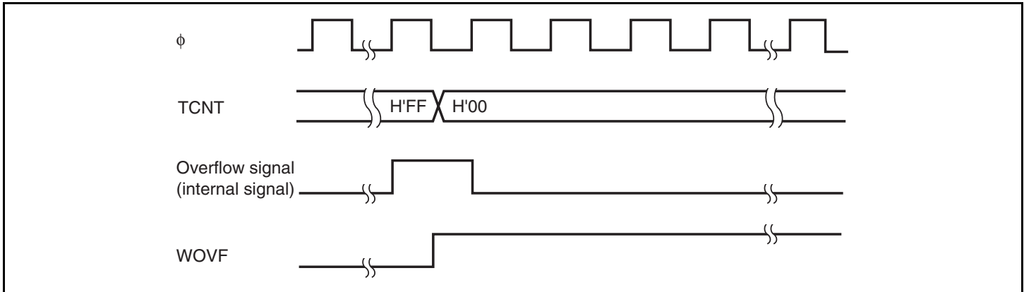
Figure 12.5 Timing of Setting WOVF
