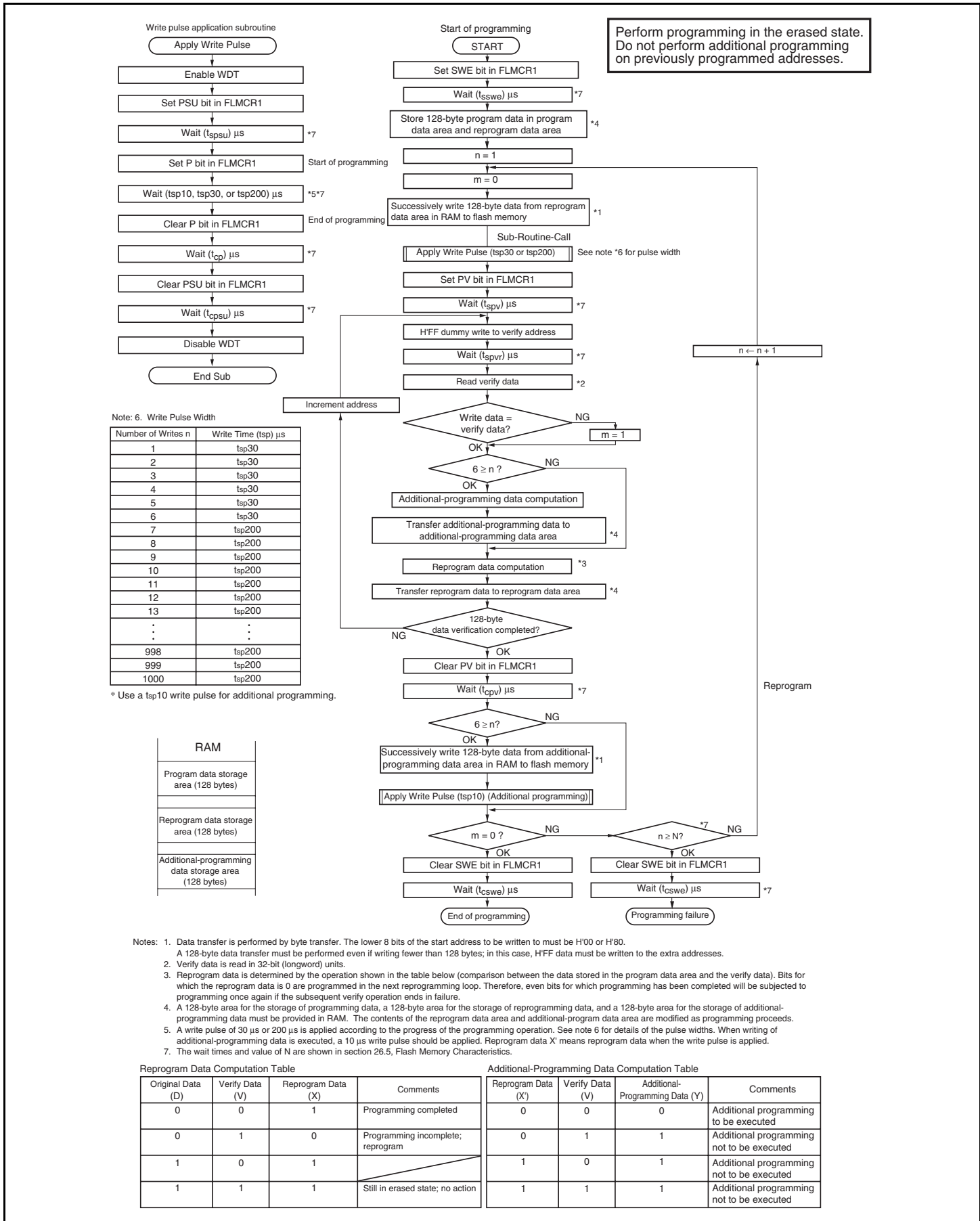
Figure 19.9 Program/Program-Verify Flowchart
