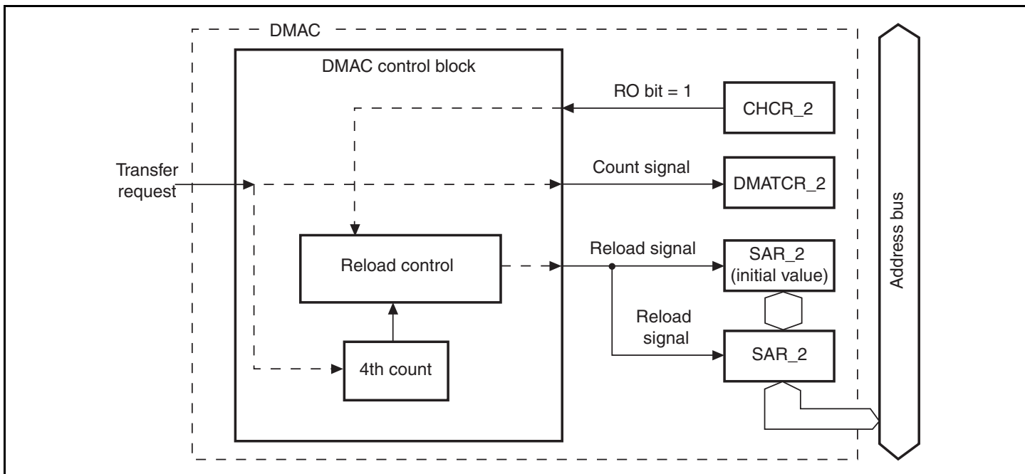
Figure 10.24 Source Address Reload Function
