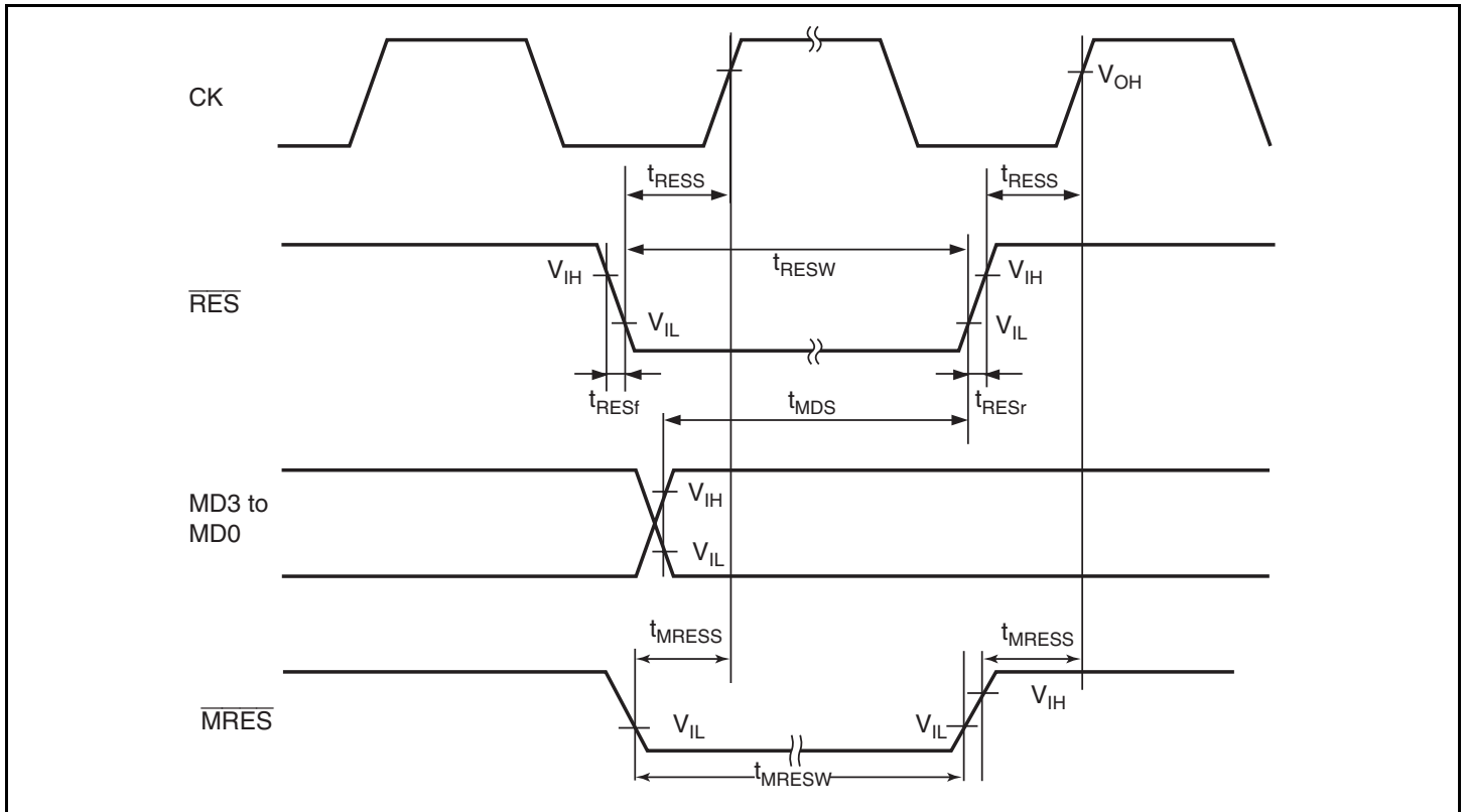
Figure 26.5 Reset Input Timing
