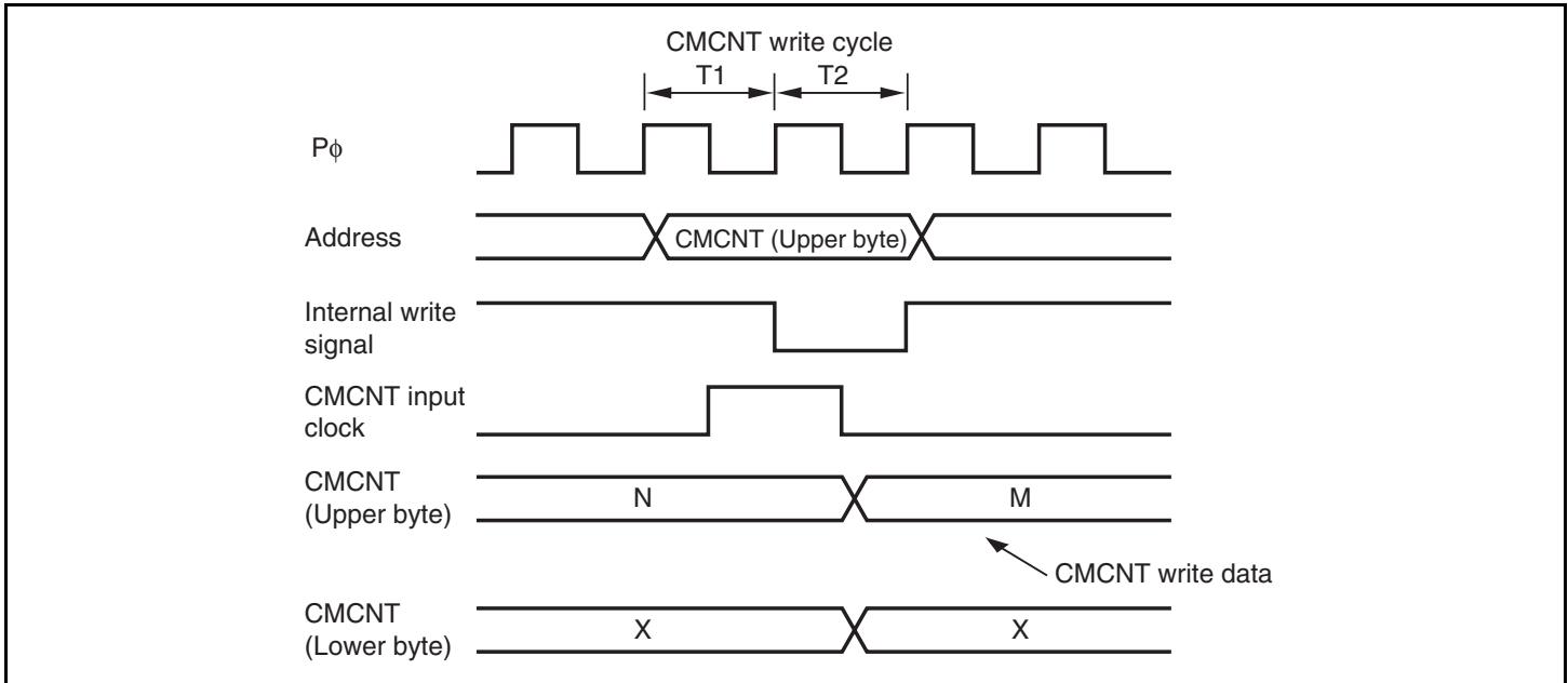
Figure 16.8 CMCNT Byte Write and Increment Contention
