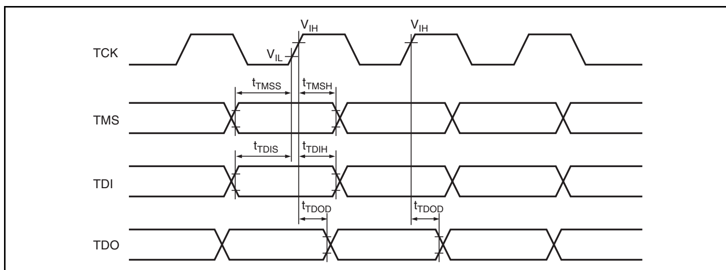
Figure 26.26 H-UDI Input/Output Timing
