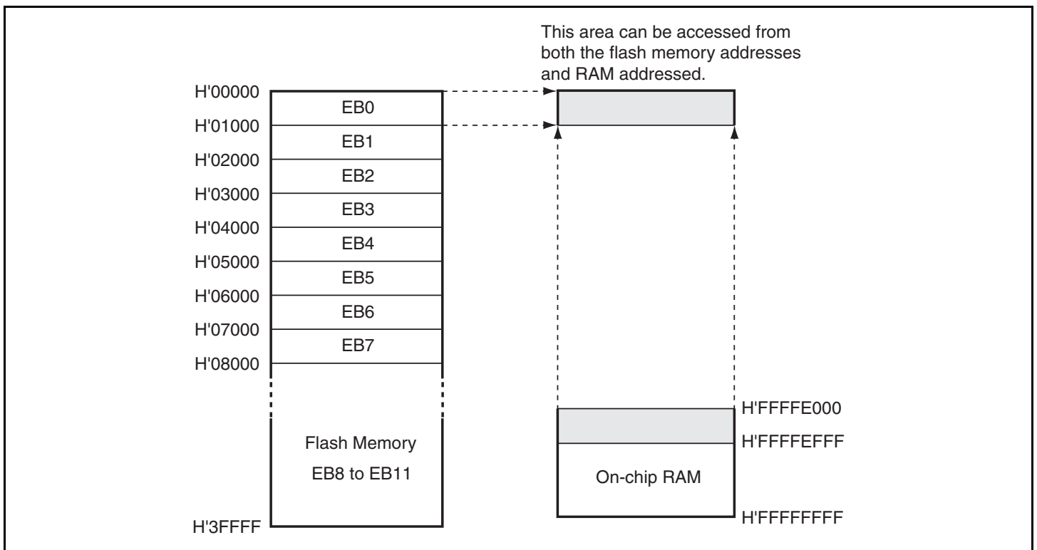
Figure 19.8 Example of RAM Overlap Operation (RAM[2:0] = B'000)
