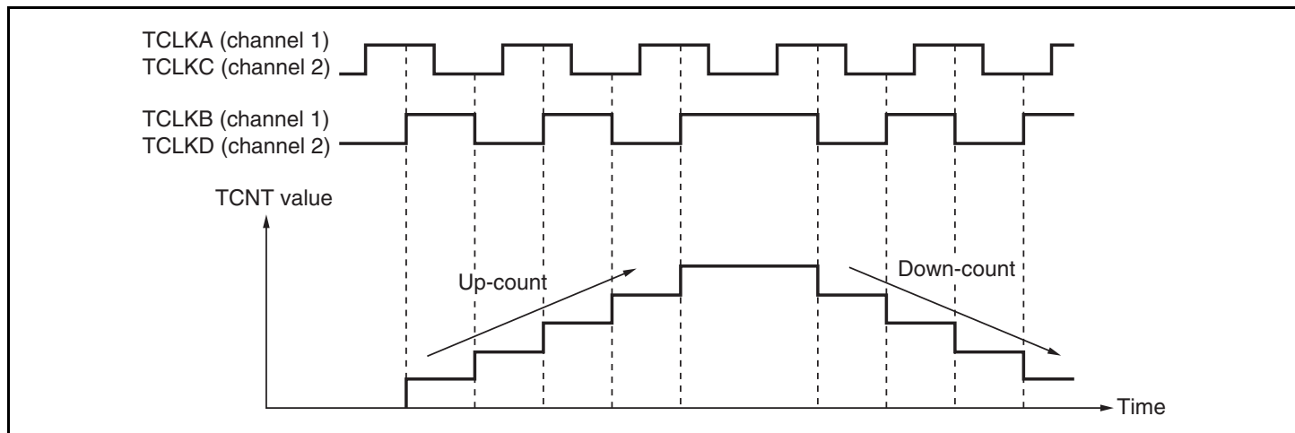
Figure 11.28 Example of Phase Counting Mode 4 Operation
