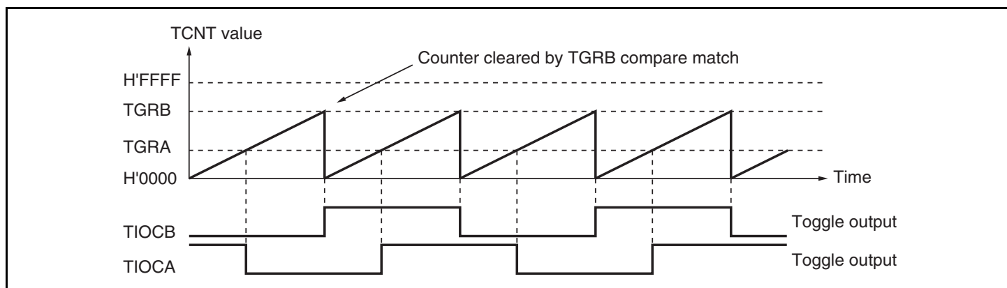
Figure 11.8 Example of Toggle Output Operation
