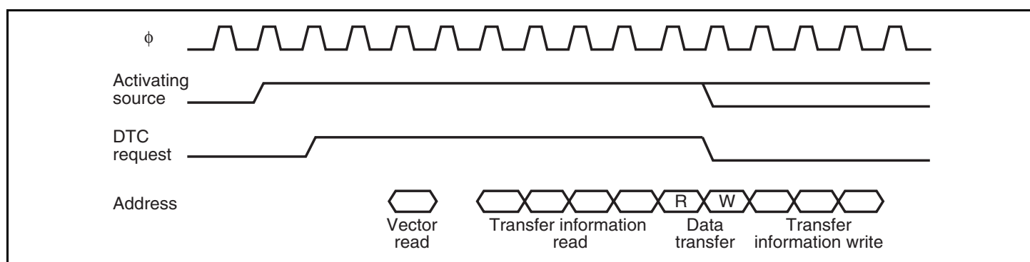
Figure 8.10 DTC Operation Timing Example (Normal Mode)
