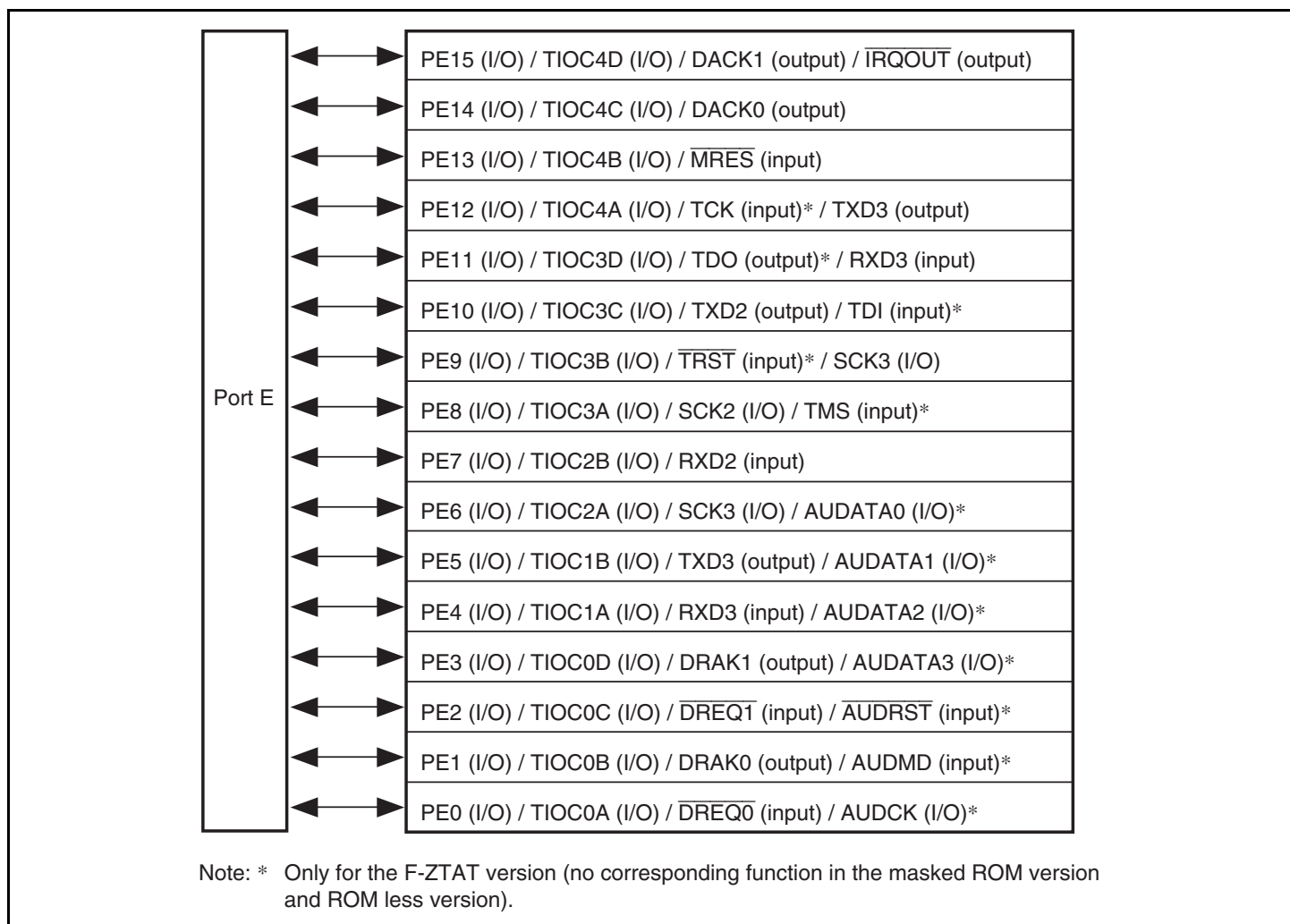
Figure 18.8 Port E (SH7145)
