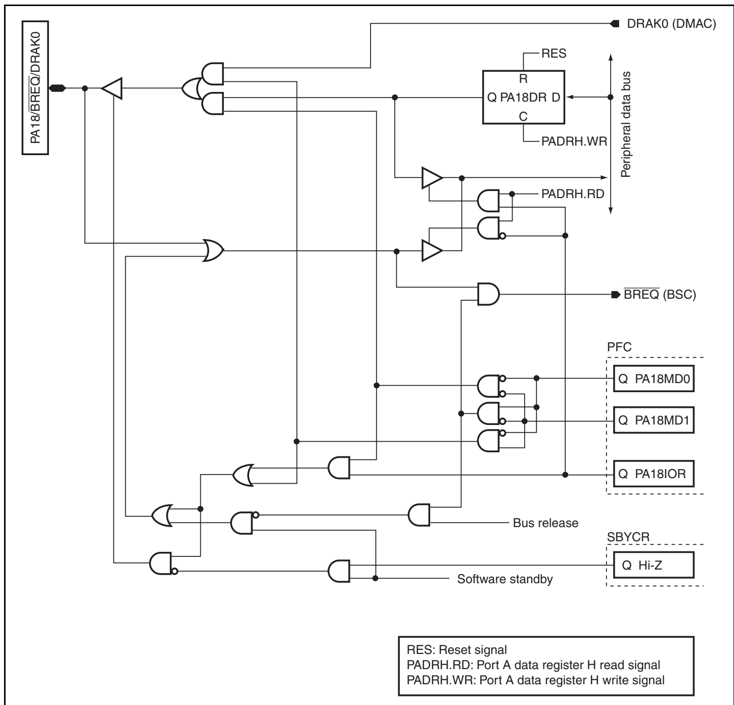
Figure D.10 PA18/ \overline{\text{BREQ}} /DRAK0
