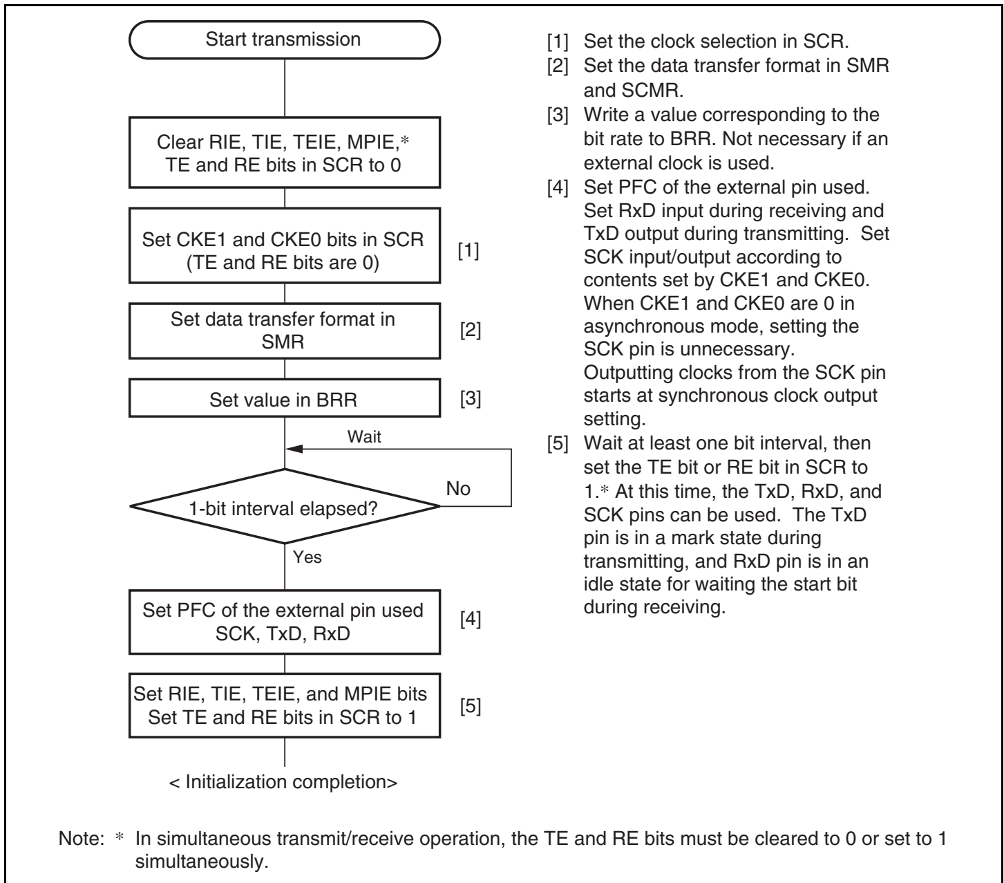
Figure 13.5 Sample SCI Initialization Flowchart
