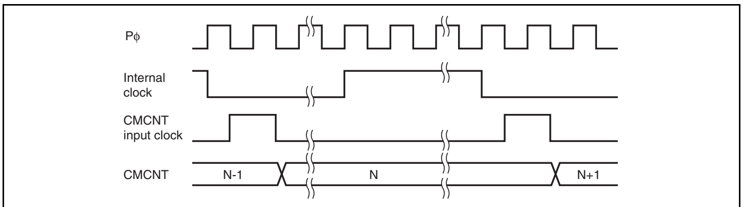
Figure 16.3 Count Timing
