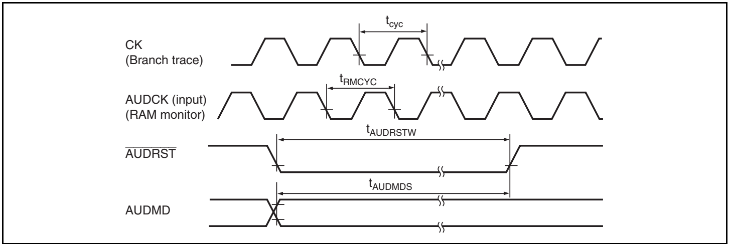
Figure 26.27 AUD Reset Timing
