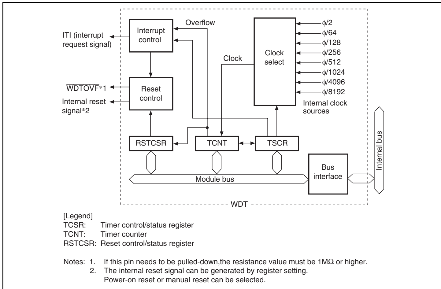
Figure 12.1 Block Diagram of WDT
