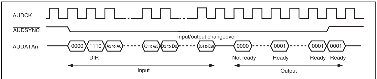
Figure 23.6 Example of Write Operation (Longword Write)
