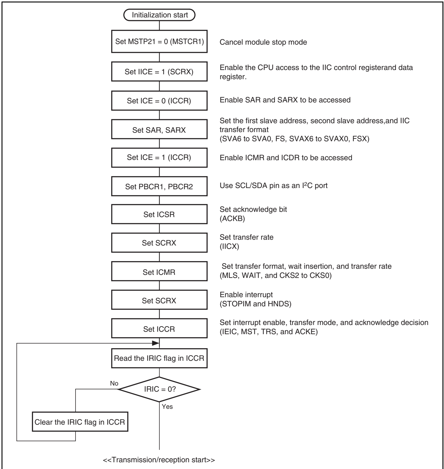
Figure 14.6 An Example of IIC Initialization Flowchart
