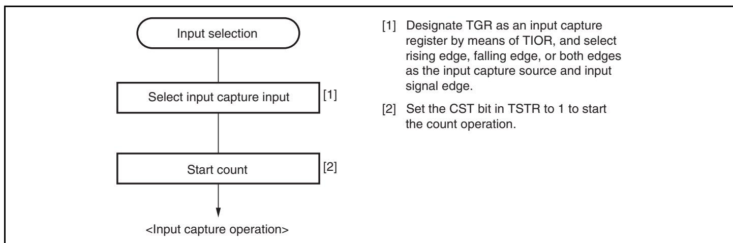
Figure 11.9 Example of Input Capture Operation Setting Procedure
