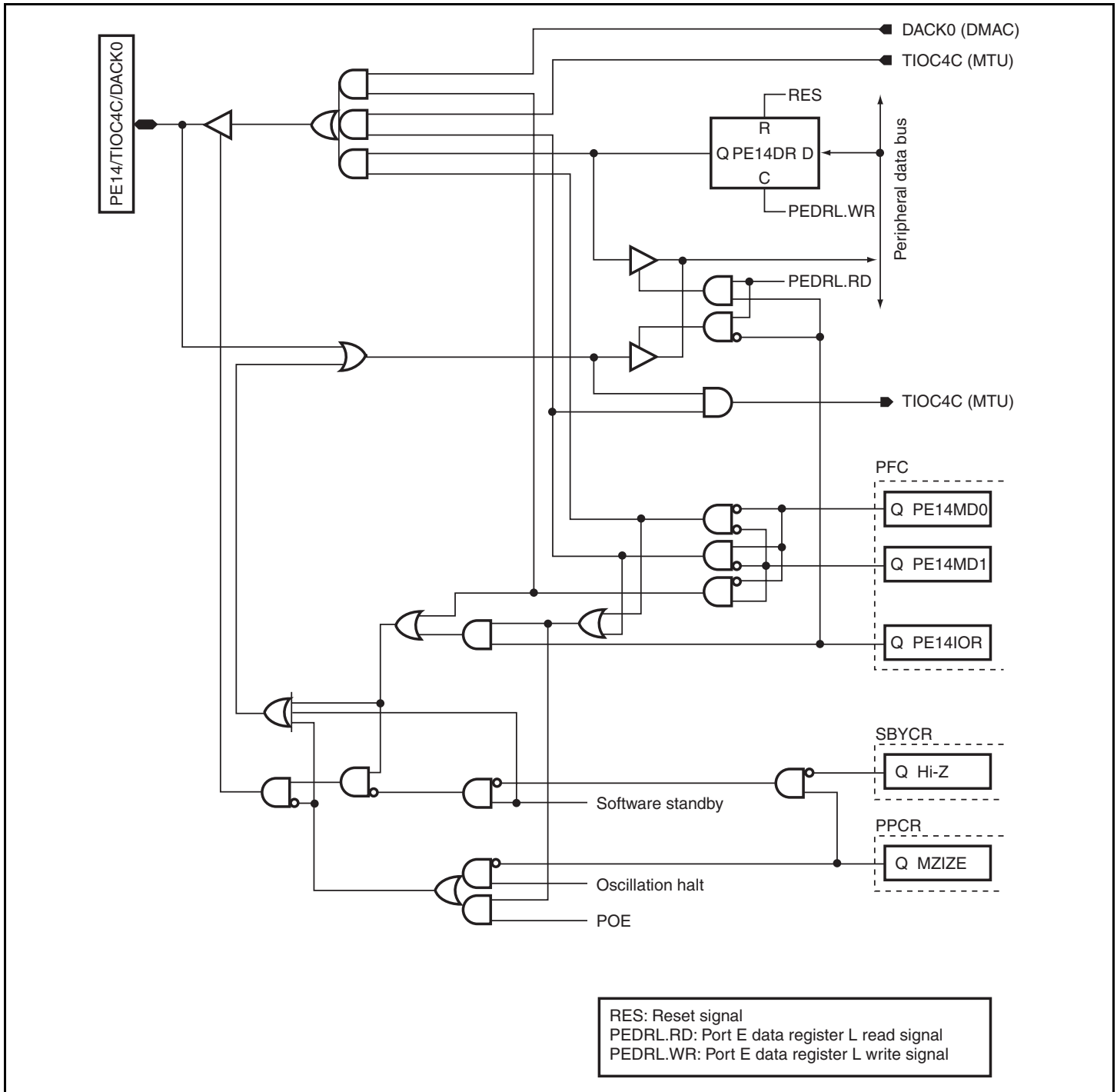
Figure D.41 PE14/TIOC4C/DACK0
