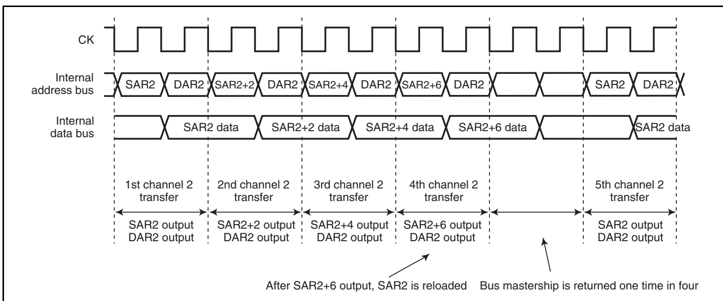
Figure 10.25 Source Address Reload Function Timing Chart
