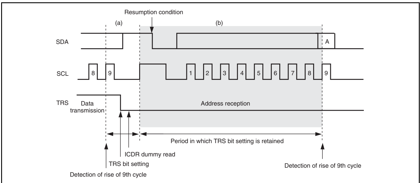
Figure 14.35 Timing for Setting TRS Bit in Slave Mode
