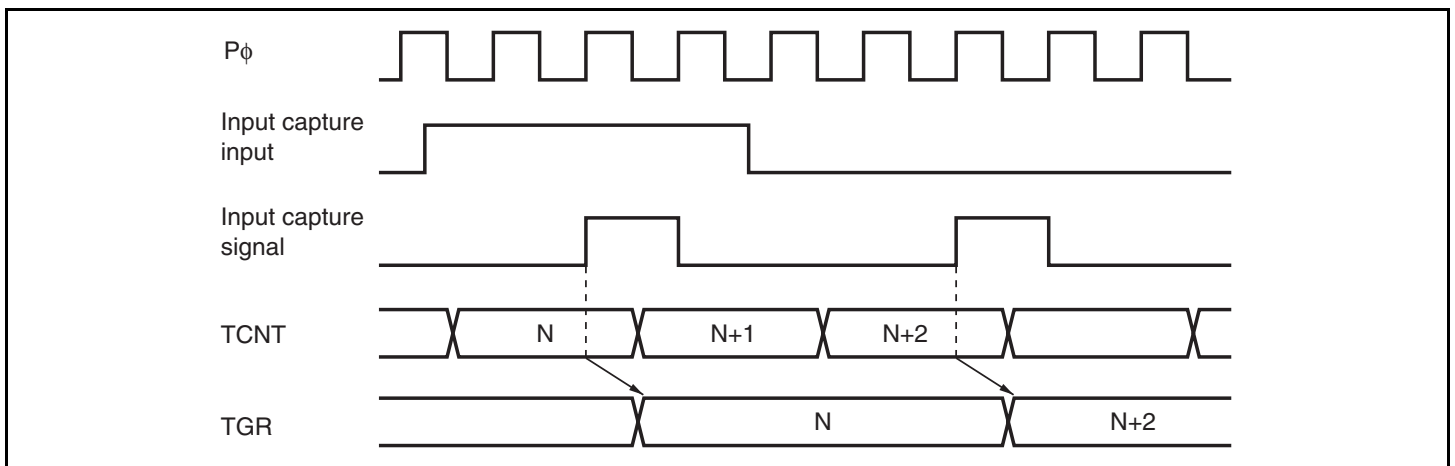
Figure 11.59 Input Capture Input Signal Timing
