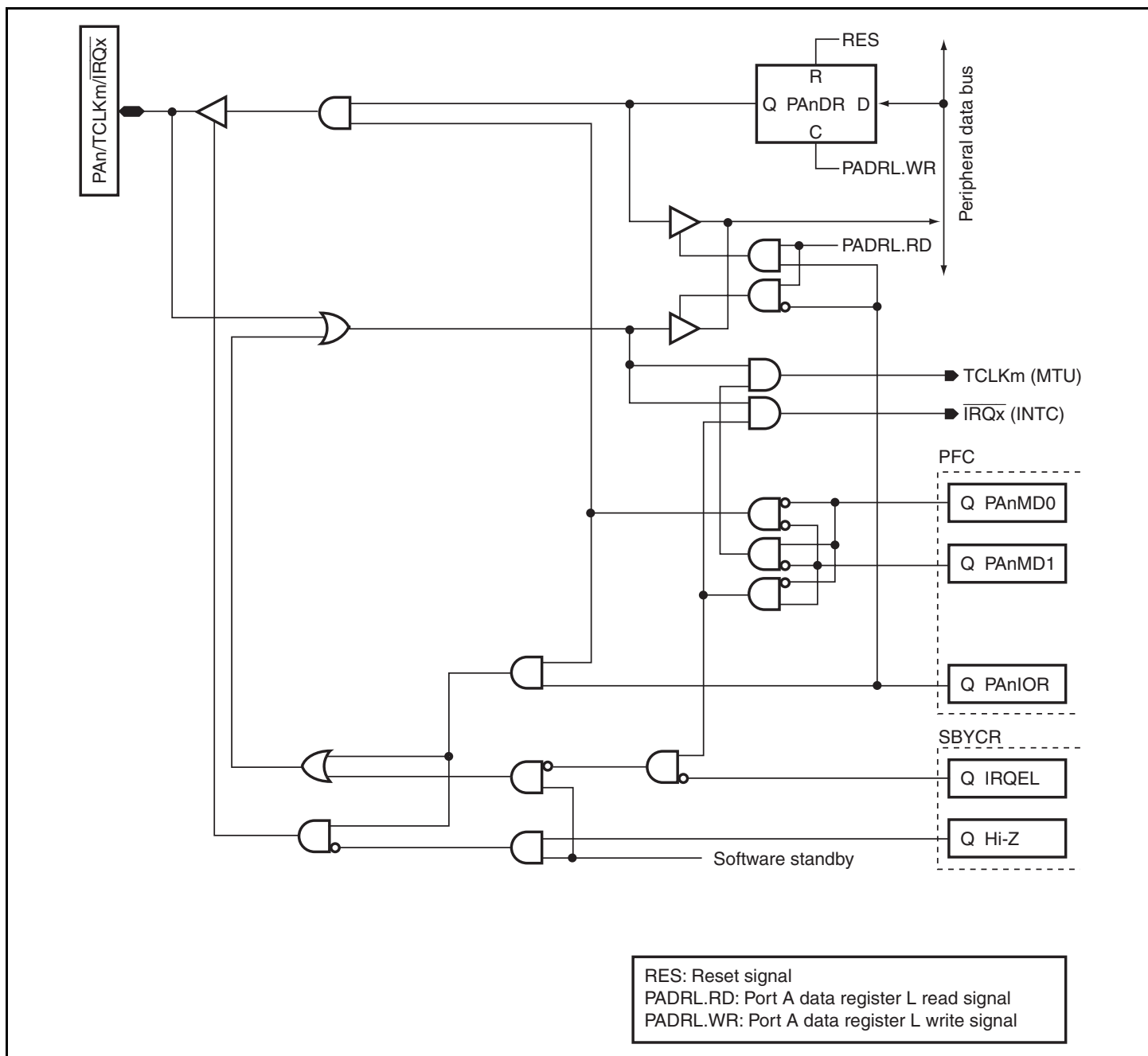
Figure D.5 PAn/TCLKm/IRQx
