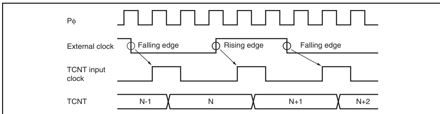
Figure 11.55 Count Timing in External Clock Operation
