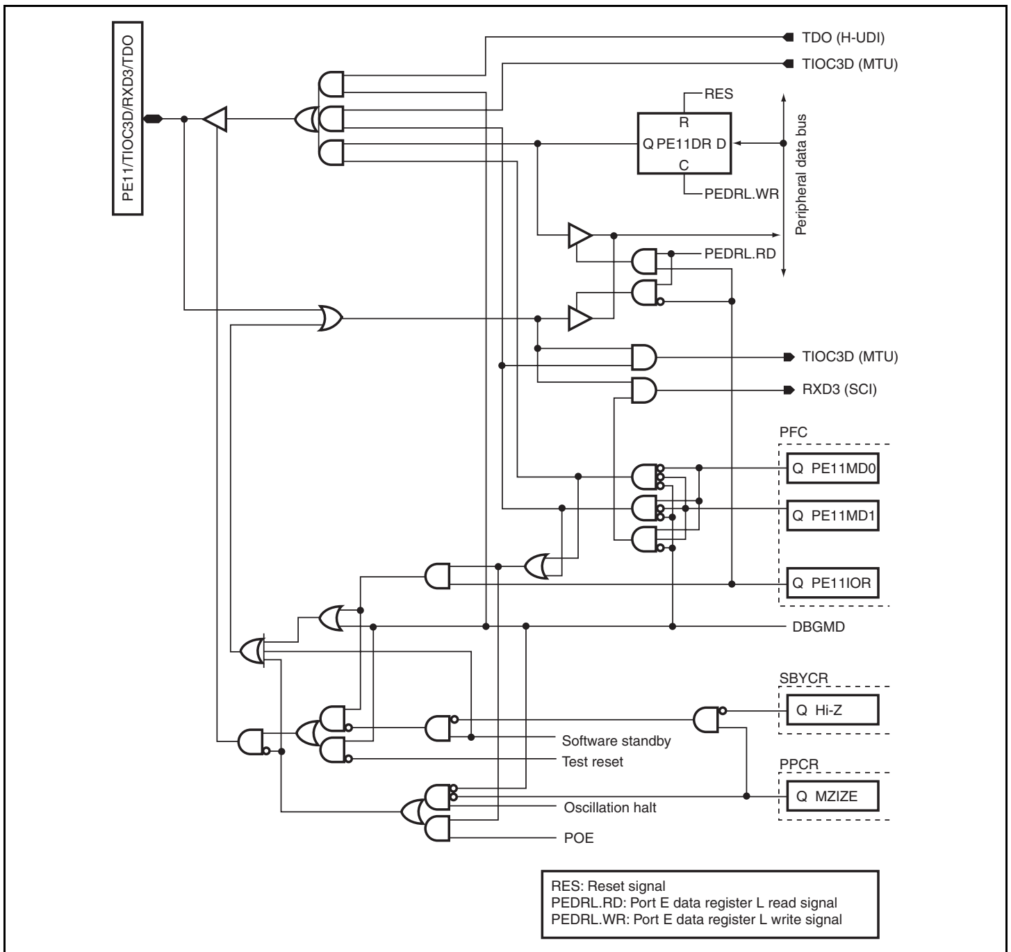
Figure D.55 PE11/TIOC3D/RXD3/TDO
