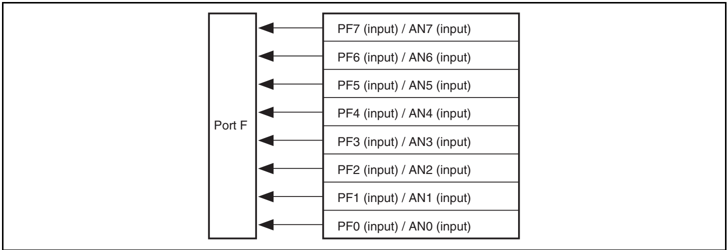
Figure 18.9 Port F
