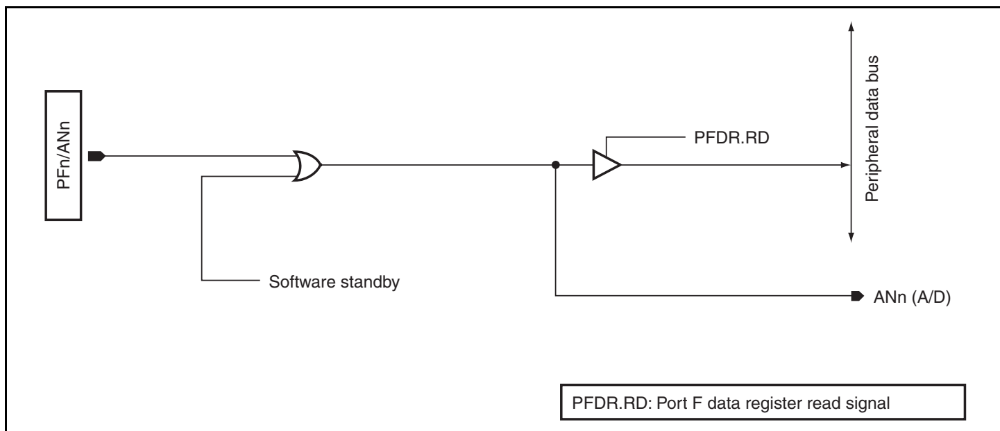
Figure D.57 PFn/ANn
