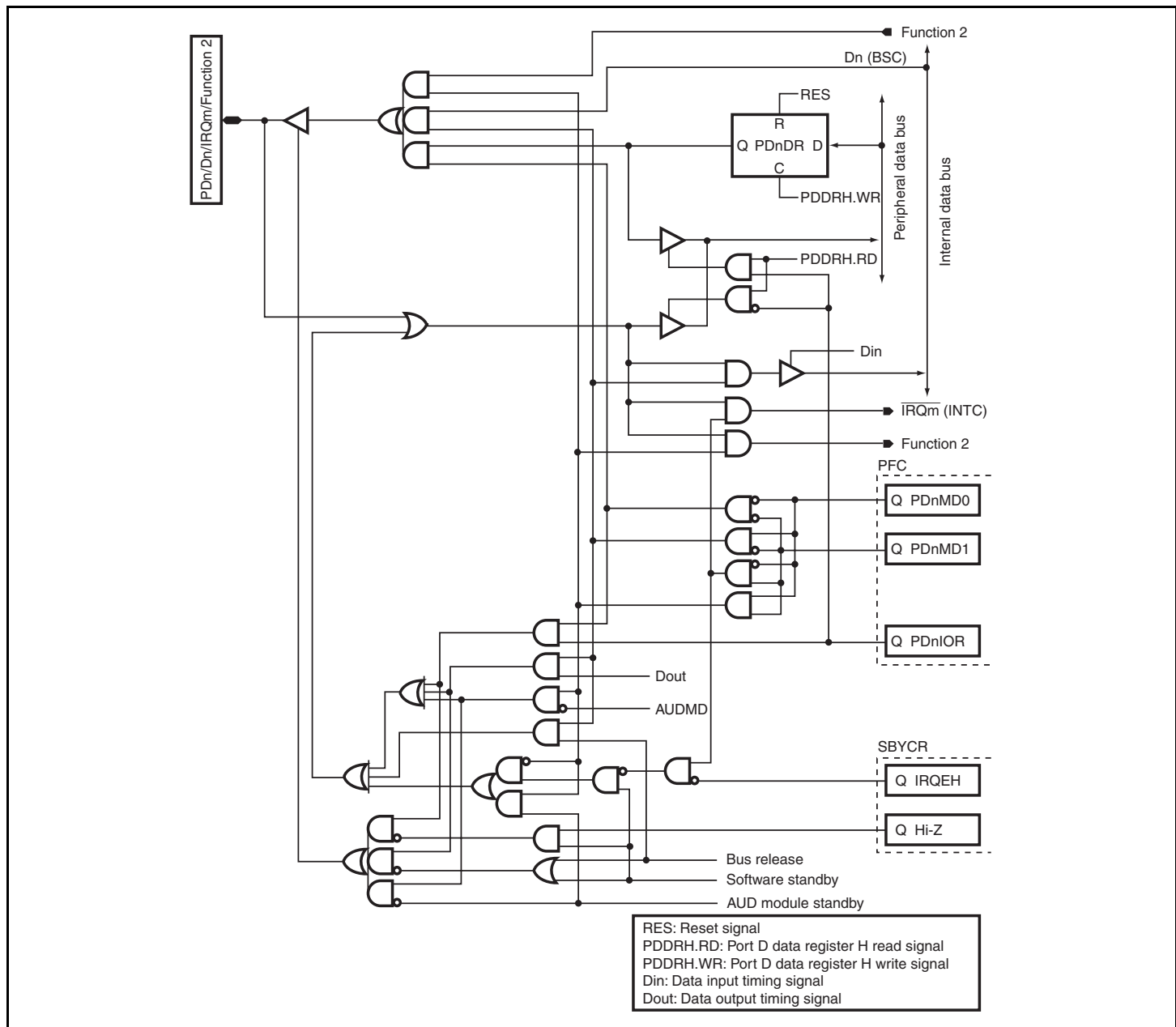
Figure D.30 PDn/Dn/ \overline{\text{IRQm}} /Function 2
