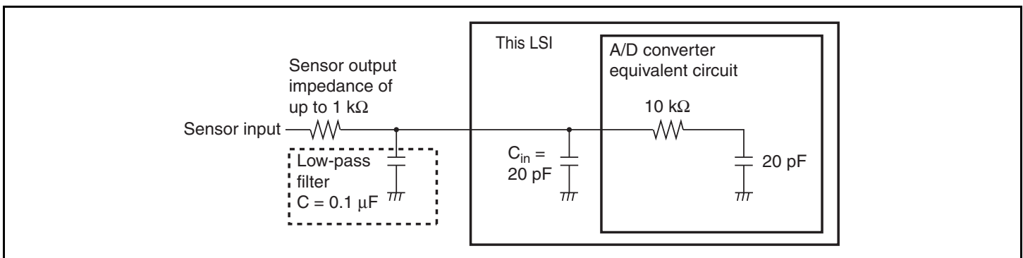
Figure 15.6 Example of Analog Input Circuit
