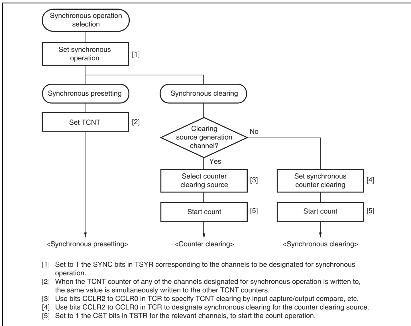
Figure 11.11 Example of Synchronous Operation Setting Procedure
