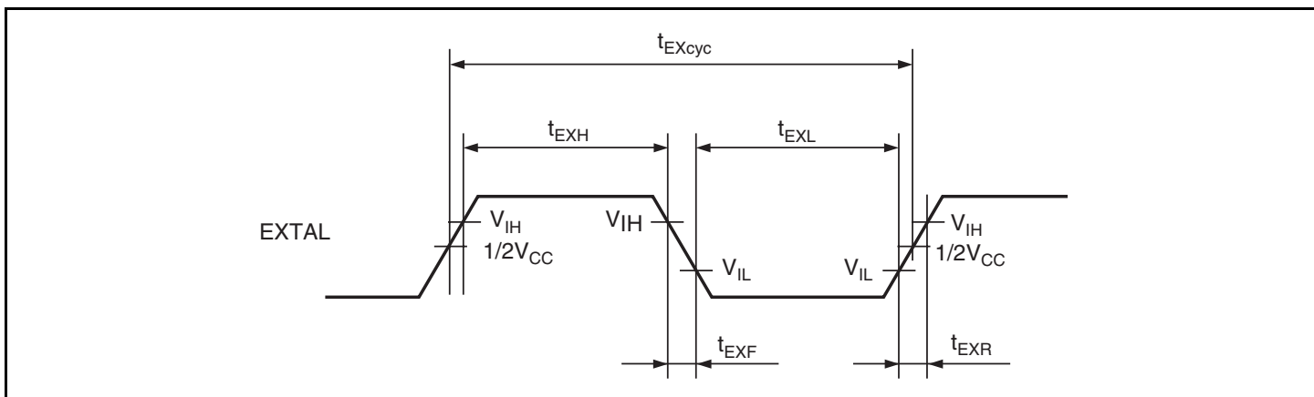
Figure 26.3 EXTAL Clock Input Timing
