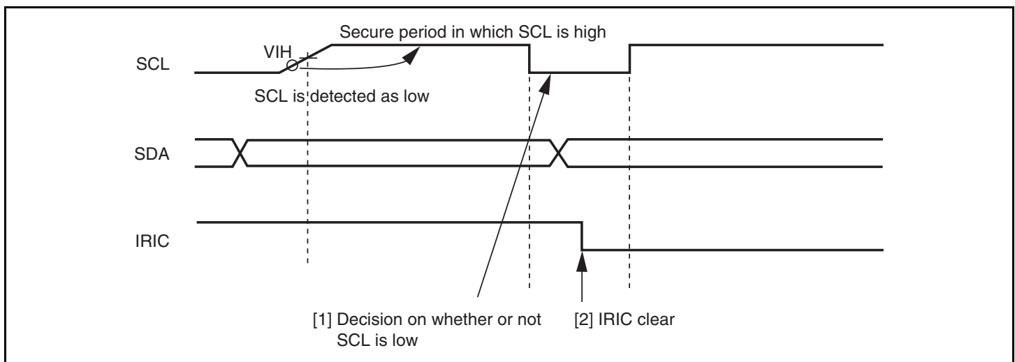
Figure 14.33 Timing for Clearing IRIC Flag When WAIT = 1
