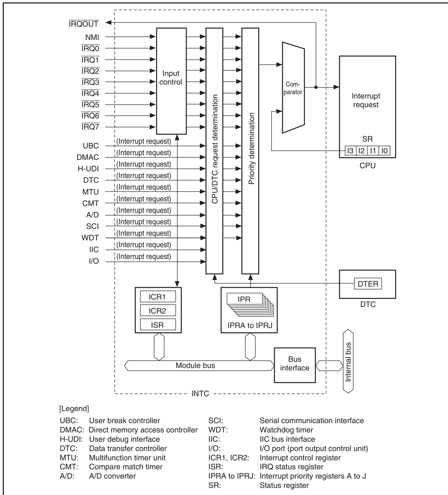
Figure 6.1 INTC Block Diagram
