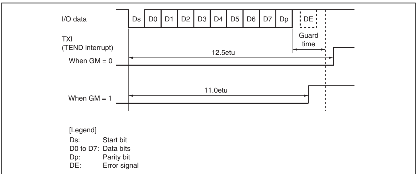
Figure 13.27 TEND Flag Generation Timing in Transmit Operation
