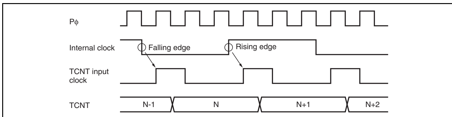
Figure 11.54 Count Timing in Internal Clock Operation
