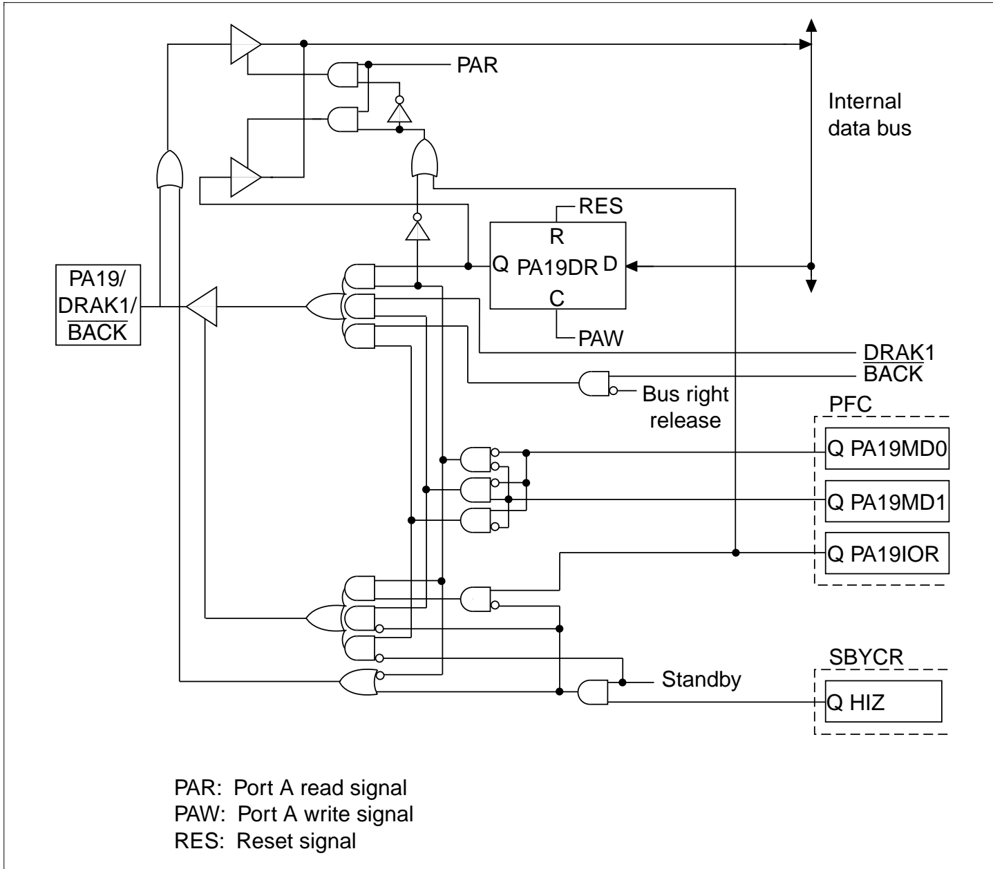
Figure B.10 PA19/DRAQ1/BACK Block Diagram
