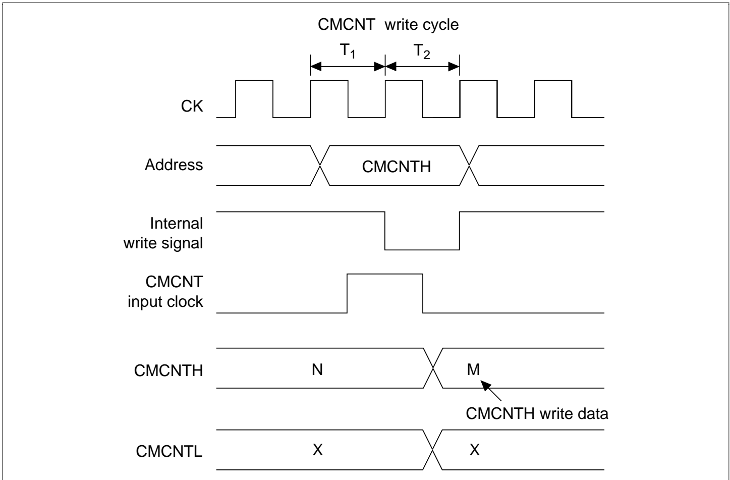
Figure 17.8 CMCNT Byte Write and Increment Contention
