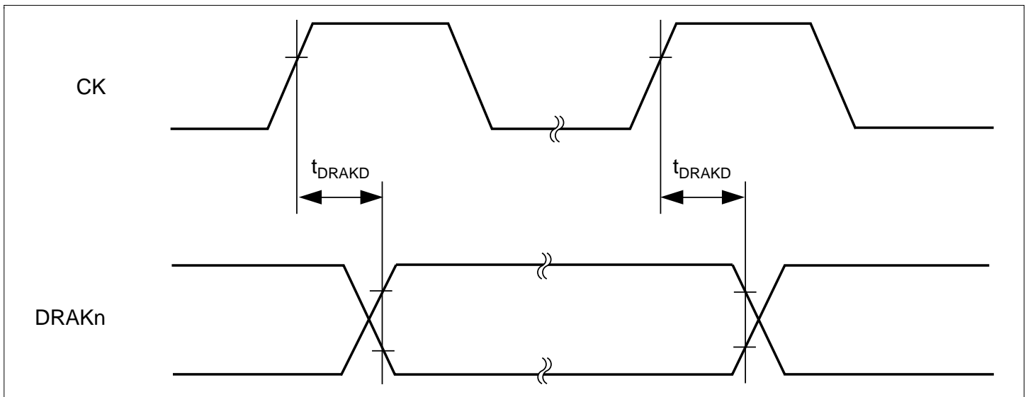
Figure 26.22 DRAK Output Delay Time
