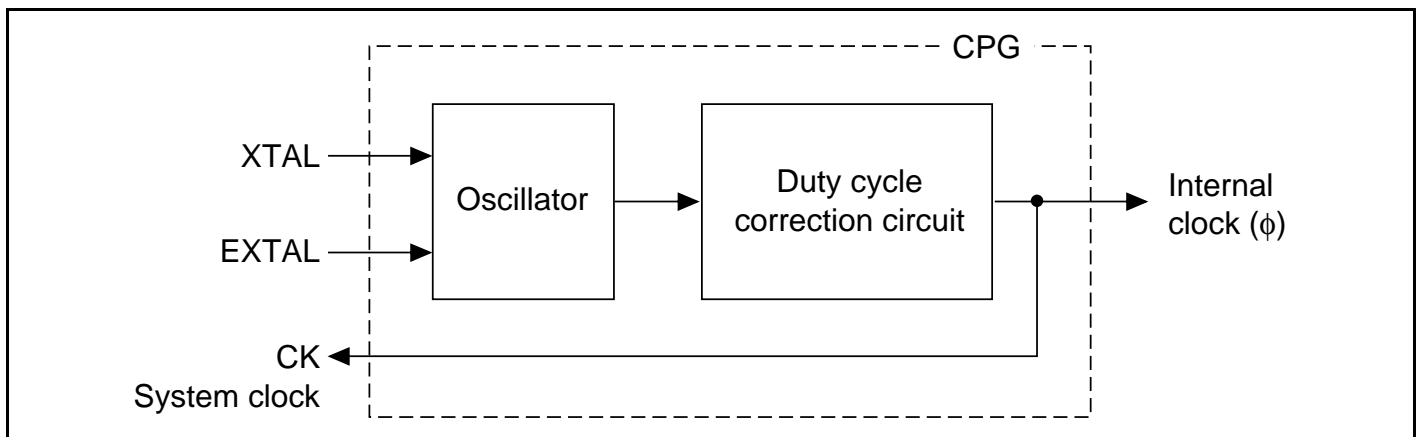
Figure 7.1 Block Diagram of Clock Pulse Generator
