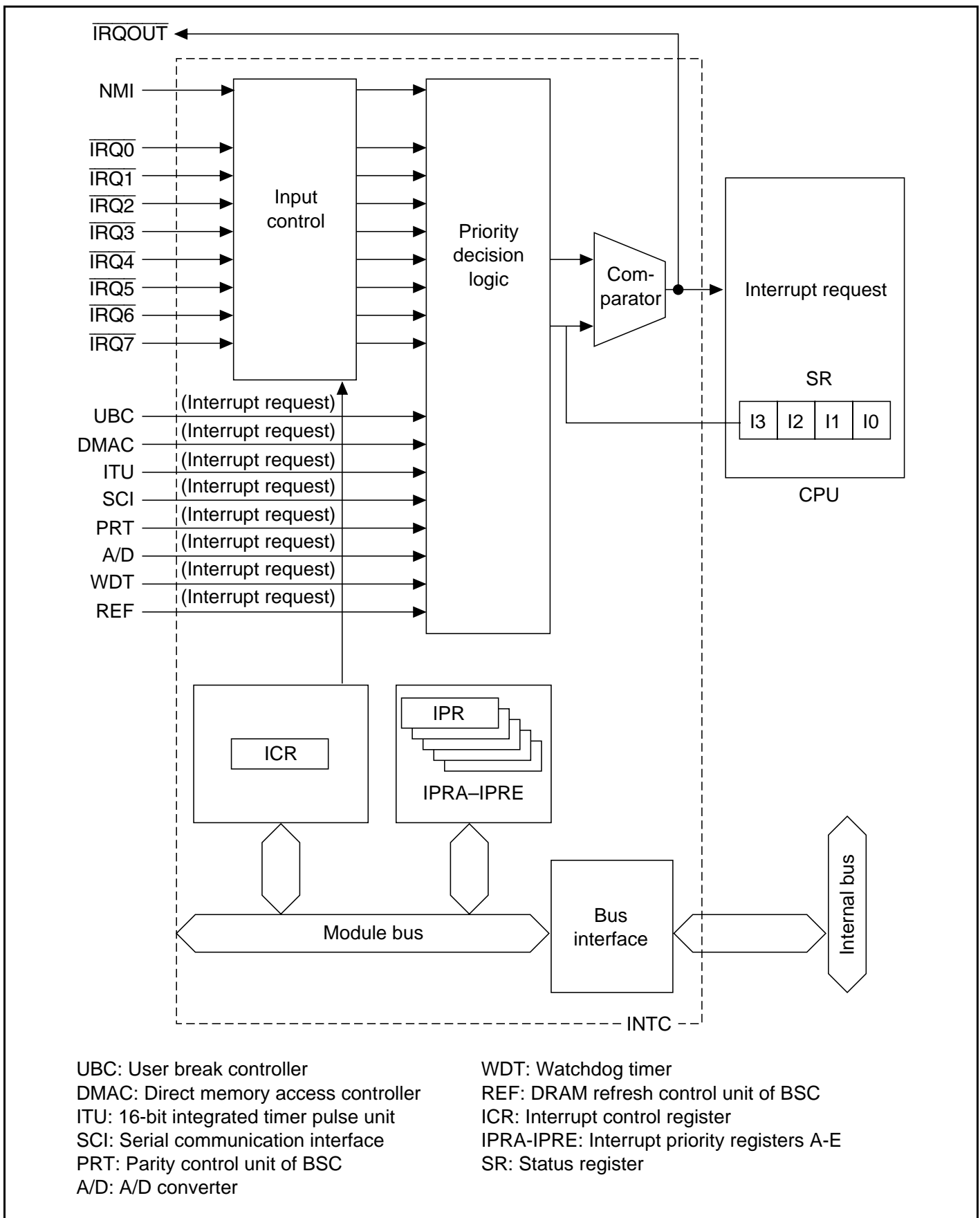
Figure 5.1 Block Diagram of Interrupt Controller
