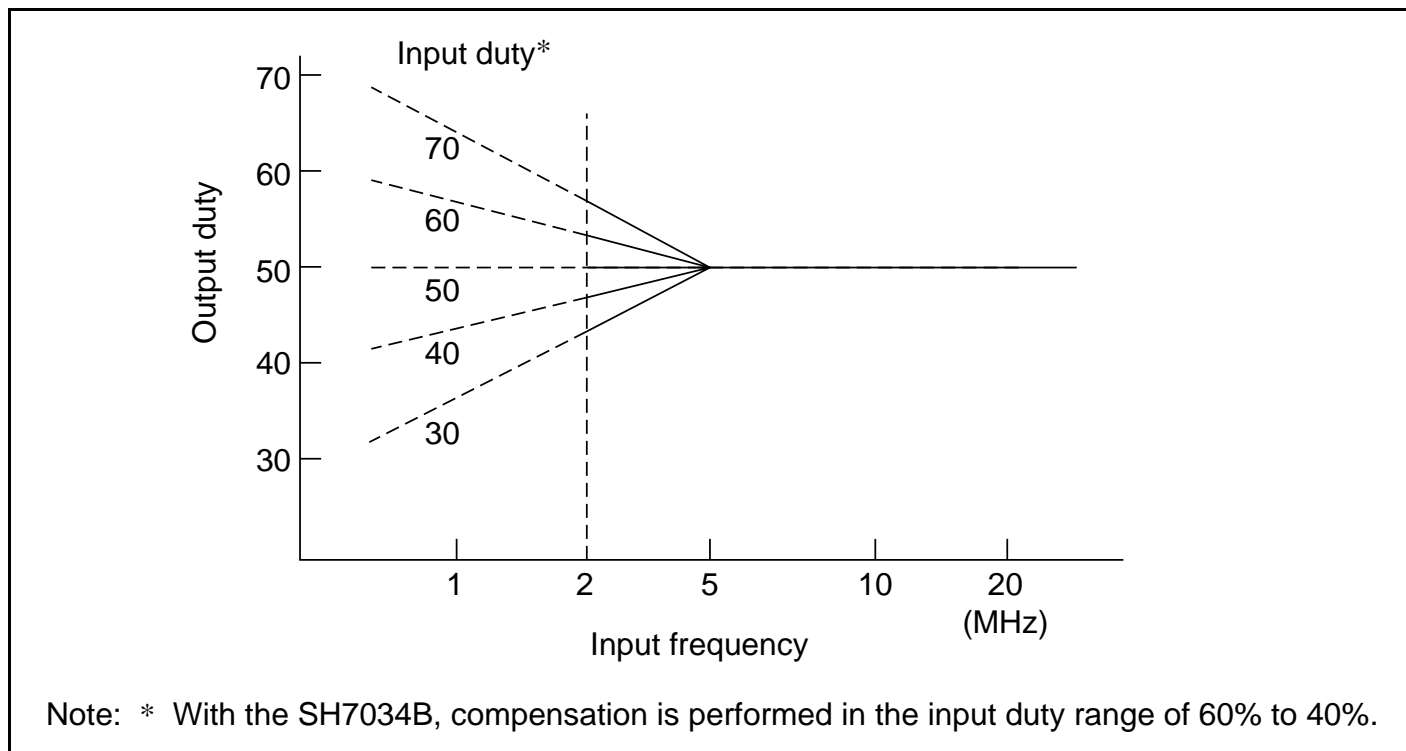
Figure 7.7 Duty Cycle Correction Circuit Standard Characteristics
