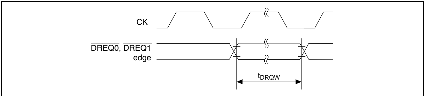
Figure 20.66 \overline{\text{DREQ0}} , \overline{\text{DREQ1}} Input Timing (2)
