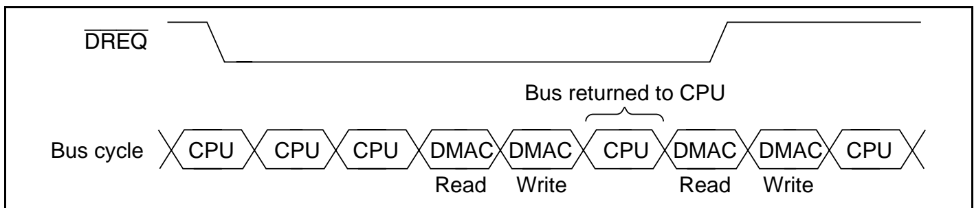
Figure 9.10 Transfer Example in Cycle-Steal Mode (Dual Address Mode, \overline{DREQ} Level Detection)
