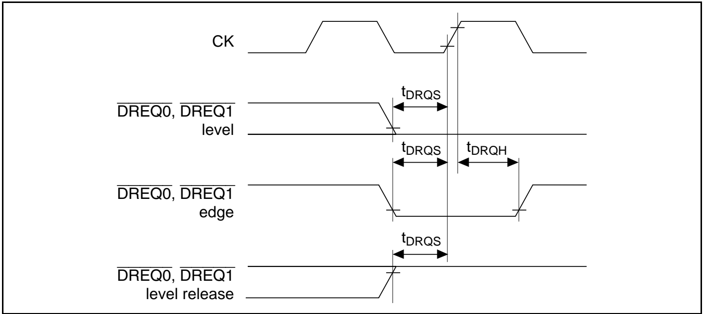
Figure 20.65 \overline{\text{DREQ0}} , \overline{\text{DREQ1}} Input Timing (1)
