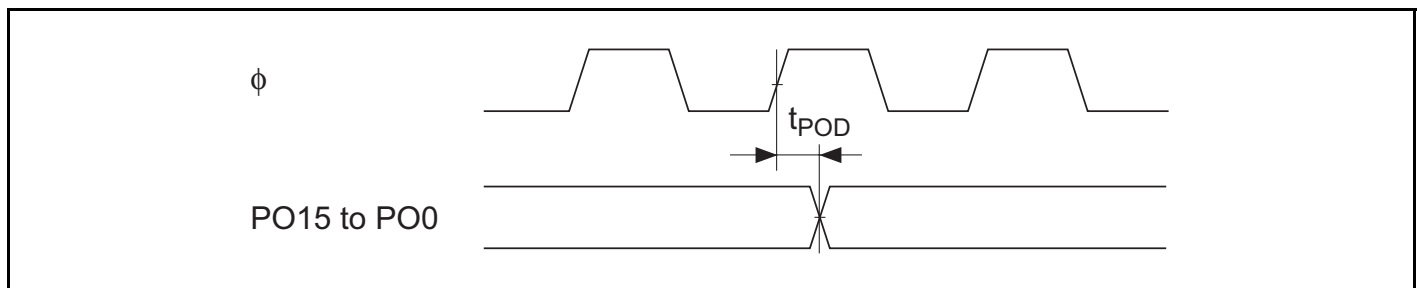
Figure 26.34 PPG Output Timing
