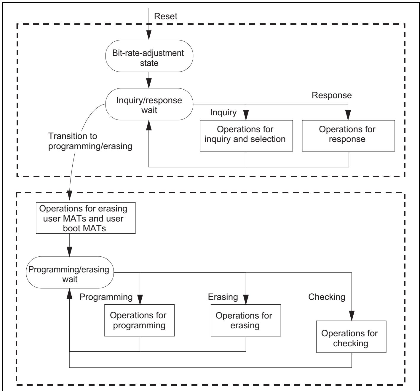
Figure 21.17 Boot Program States
