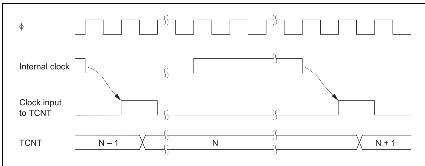
Figure 13.3 Count Timing for Internal Clock Input
