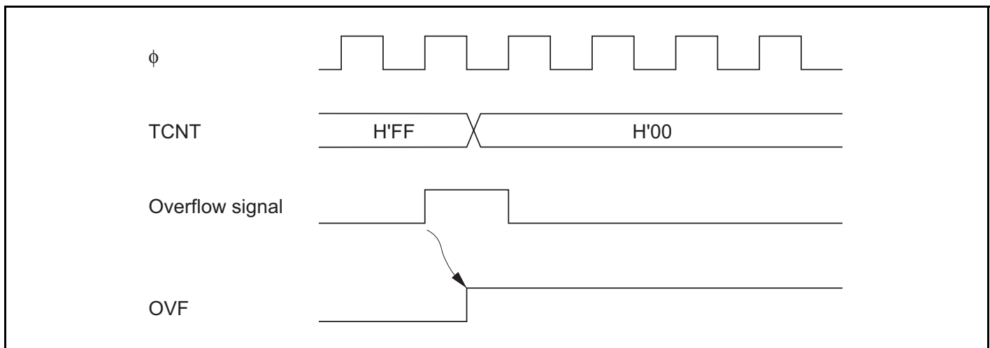
Figure 13.9 Timing of OVF Setting
