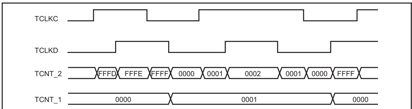
Figure 11.19 Example of Cascaded Operation (2)
