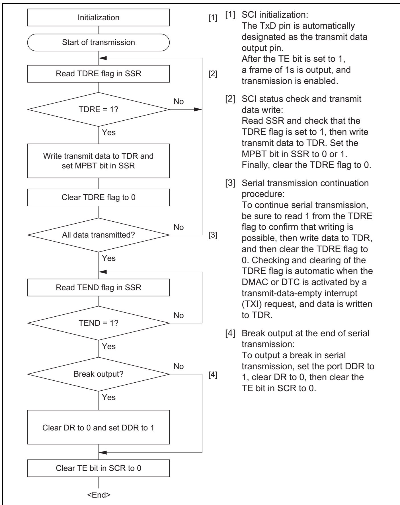
Figure 15.11 Sample Multiprocessor Serial Transmission Flowchart
