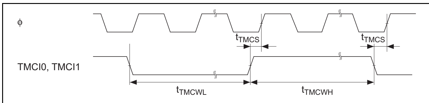
Figure 26.38 8-Bit Timer Clock Input Timing
