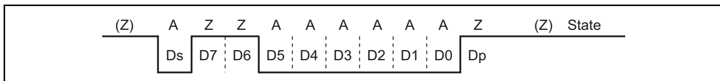
Figure 15.24 Inverse Convention ( SDIR = SINV = O/\bar{E} = 1 )
