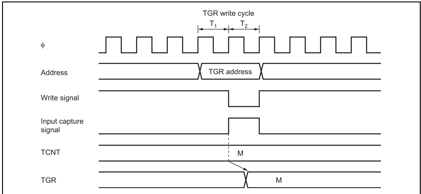
Figure 11.50 Contention between TGR Write and Input Capture
