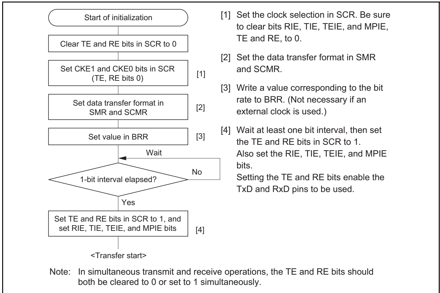
Figure 15.15 Sample SCI Initialization Flowchart
