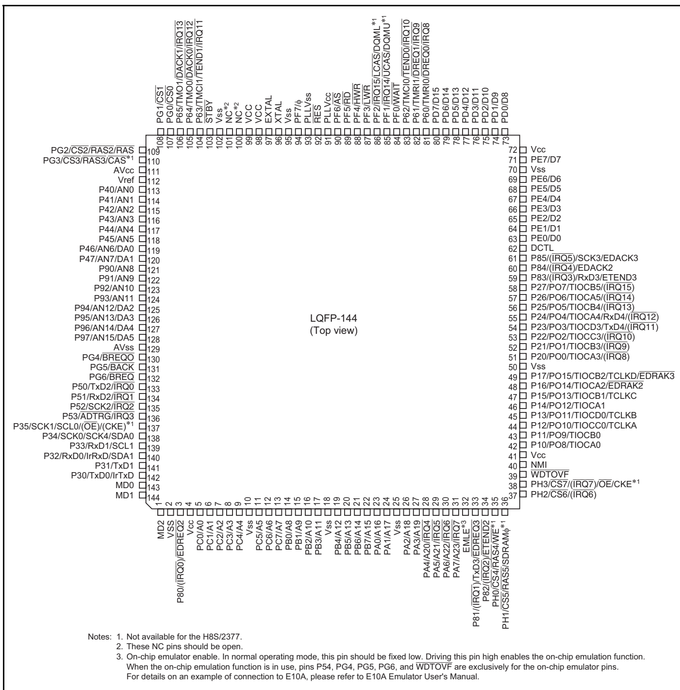
Figure 1.6 Pin Arrangement for H8S/2377 and H8S/2377R
