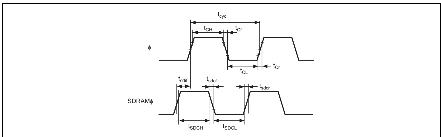
Figure 26.3 SDRAM \phi Timing
