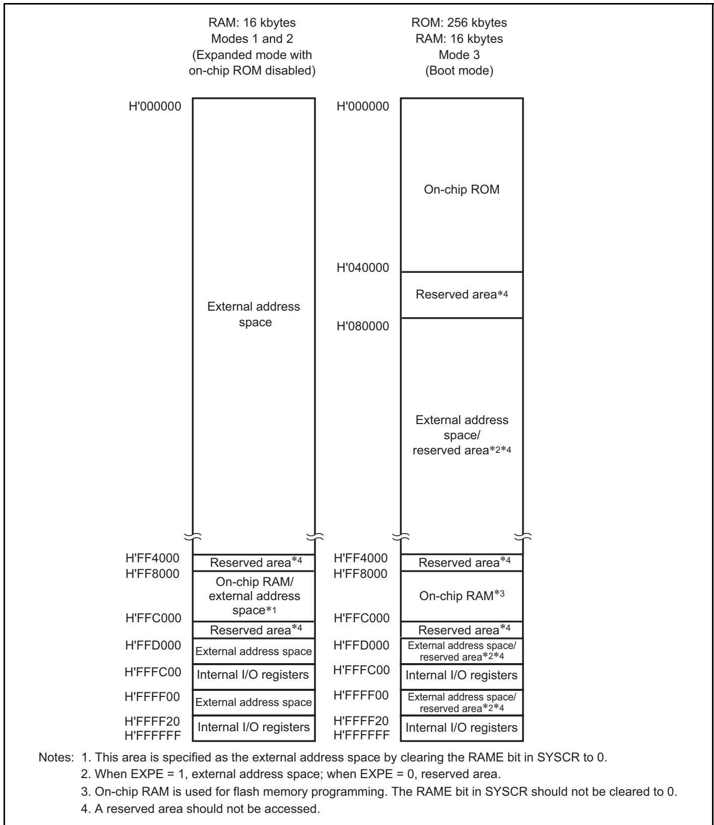
Figure 3.14 Memory Map for H8S/2370 and H8S/2370R (1)
