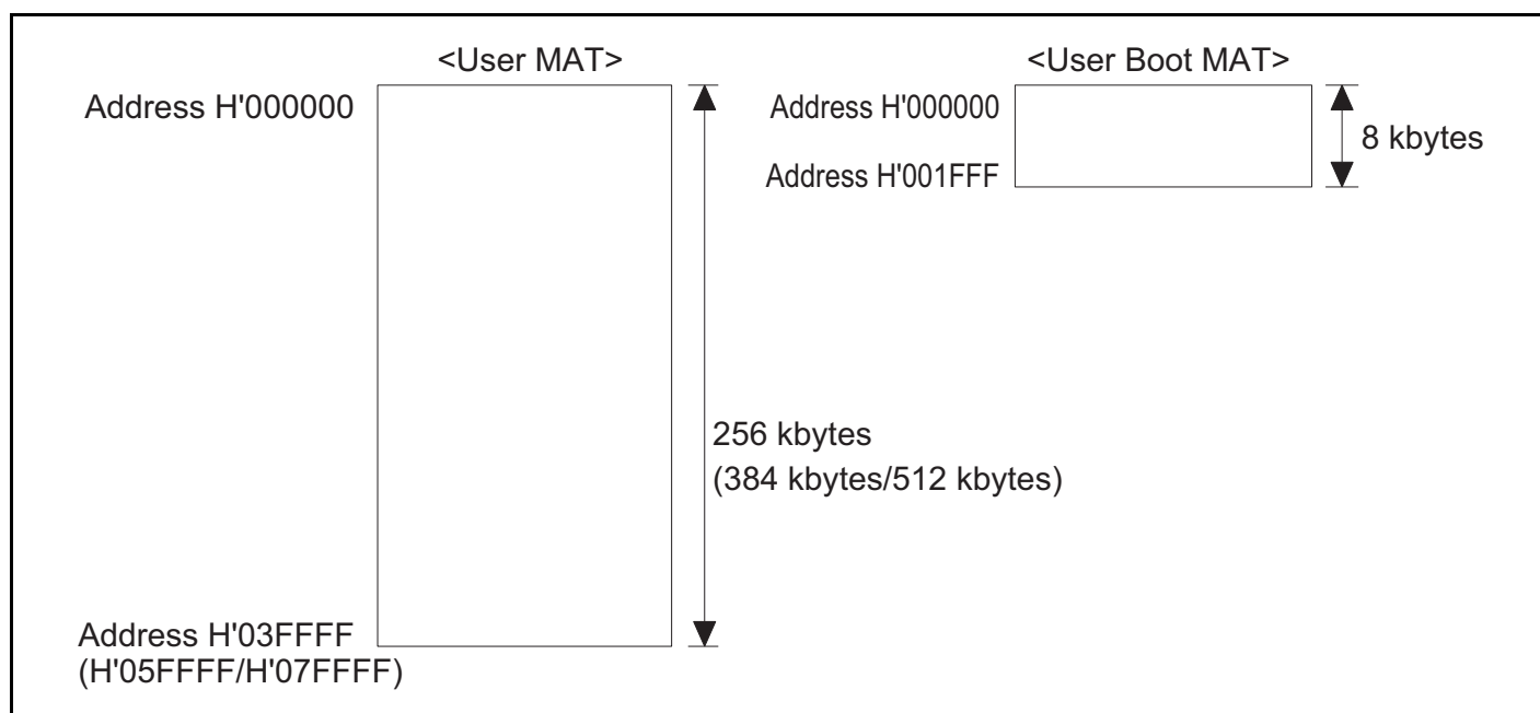
Figure 21.3 Flash Memory Configuration
