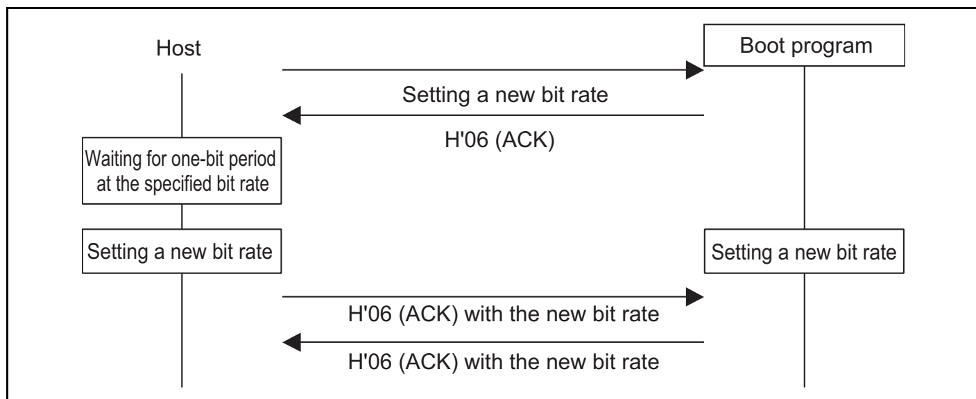
Figure 21.20 New Bit-Rate Selection Sequence
