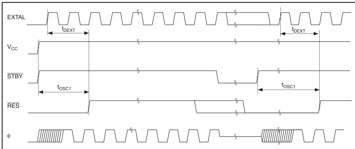
Figure 26.4 (1) Oscillation Settling Timing
