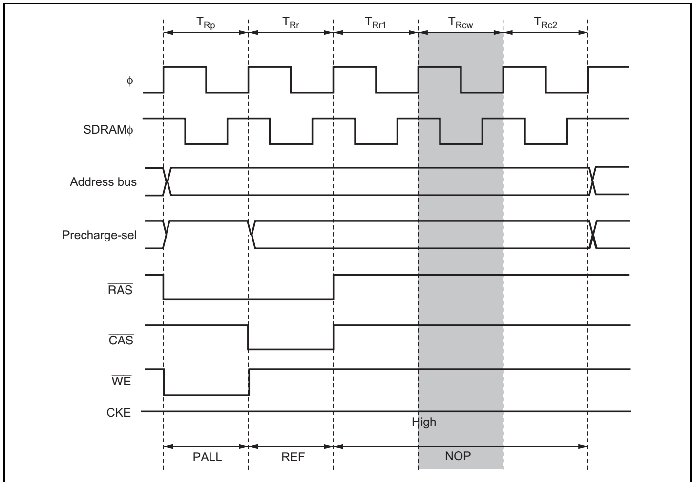
Figure 6.56 Auto Refresh Timing ( \text{TPC} = 0 , \text{TPC0} = 0 , \text{RLW1} = 0 , \text{RLW0} = 1 )
