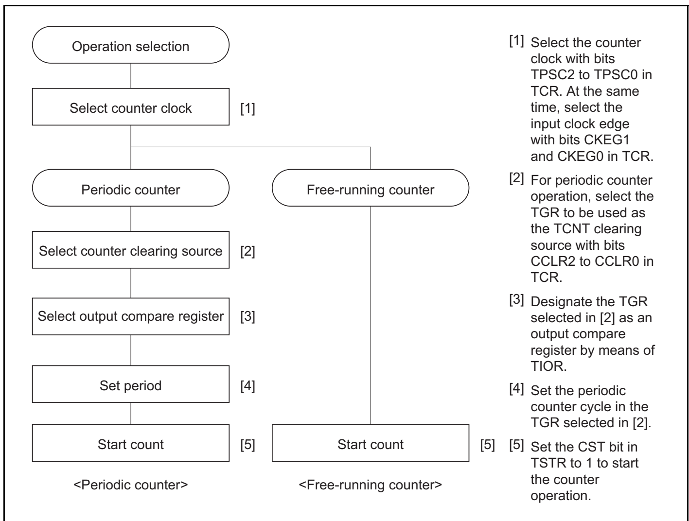
Figure 11.2 Example of Counter Operation Setting Procedure
