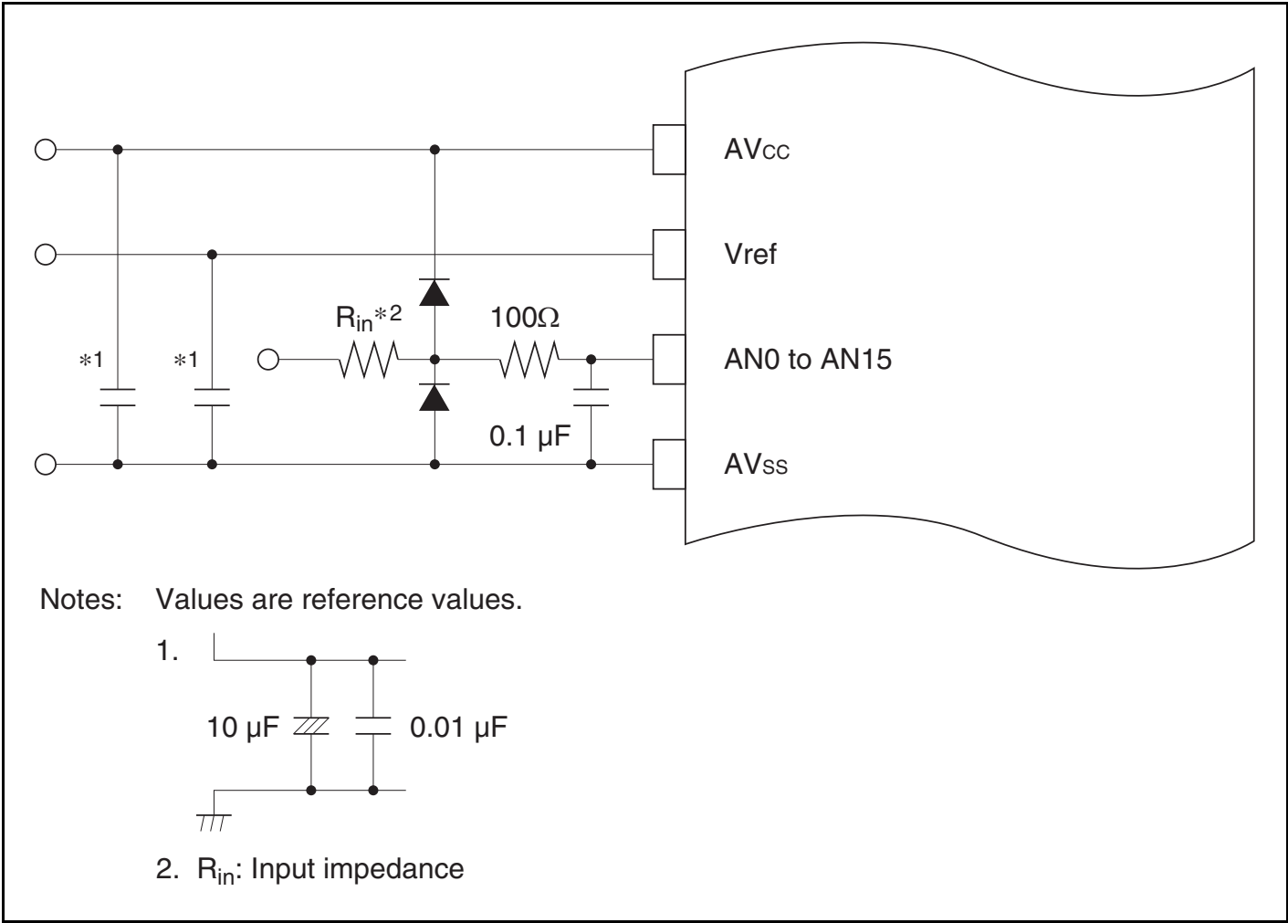
Figure 17.7 Example of Analog Input Protection Circuit
