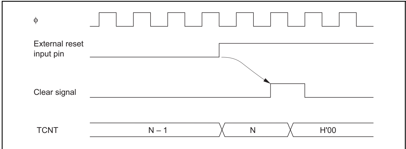
Figure 13.8 Timing of Clearance by External Reset
