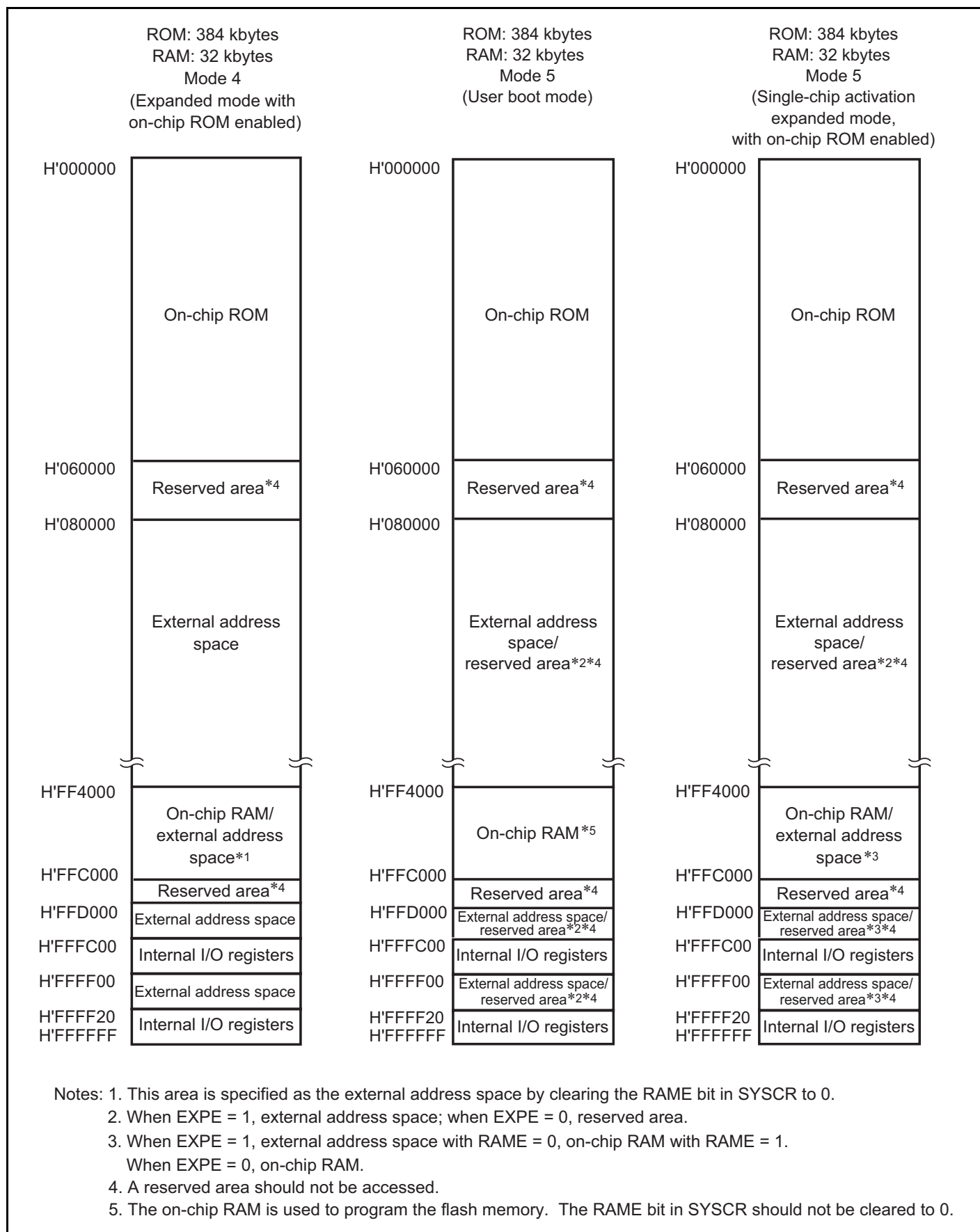
Figure 3.8 Memory Map for H8S/2374 and H8S/2374R (2)
