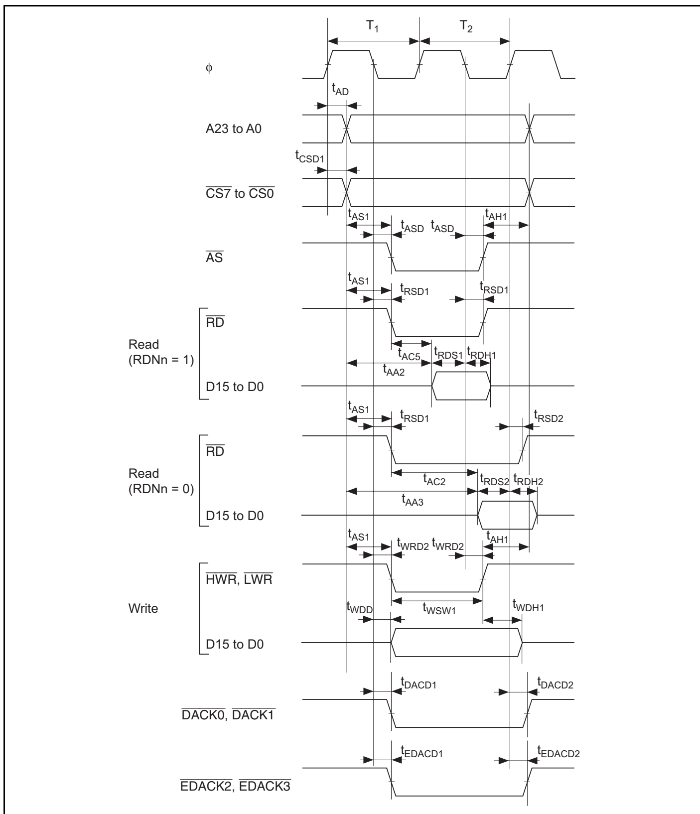
Figure 26.7 Basic Bus Timing: Two-State Access
