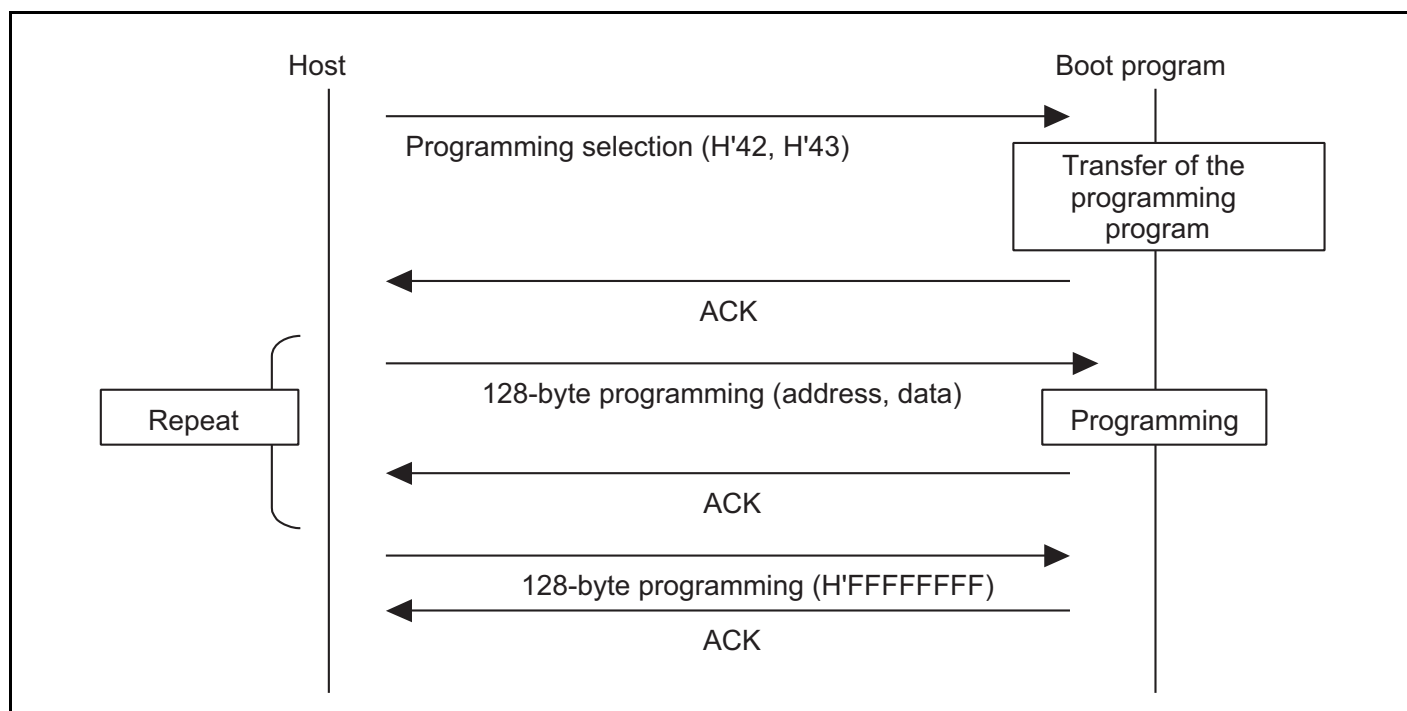
Figure 21.21 Programming Sequence
