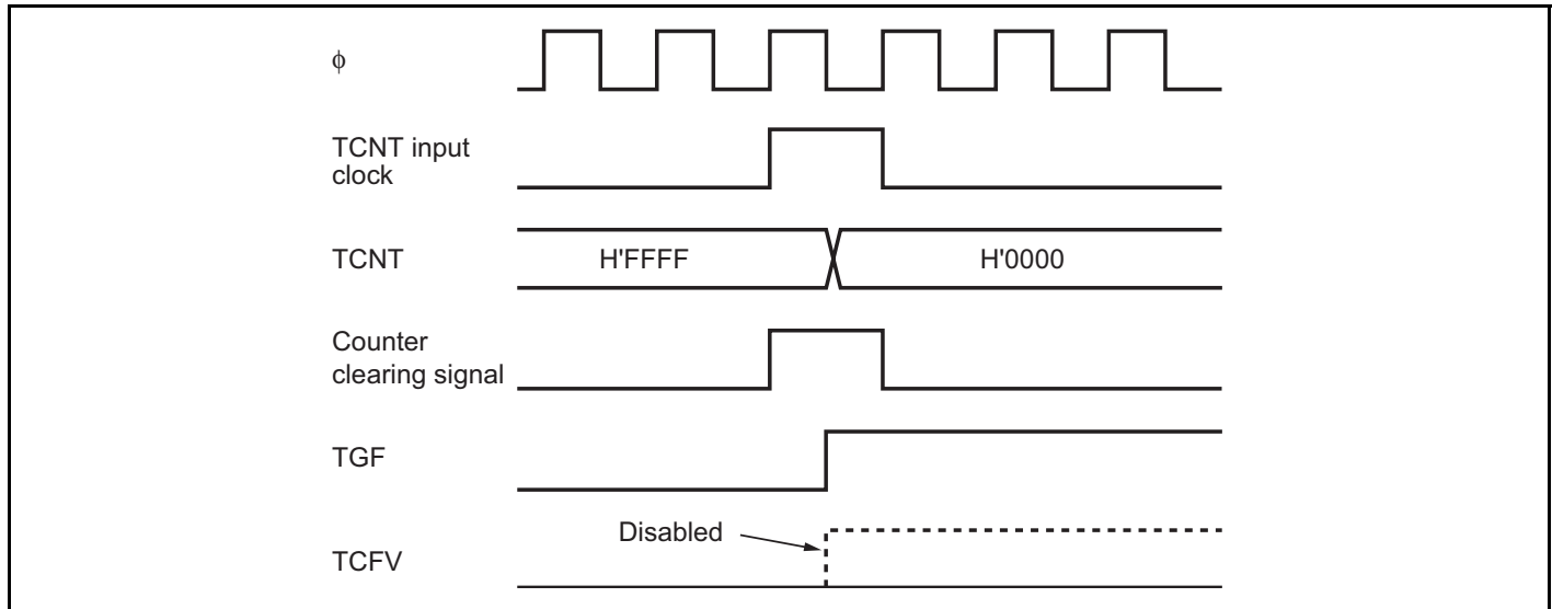
Figure 11.52 Contention between Overflow and Counter Clearing
