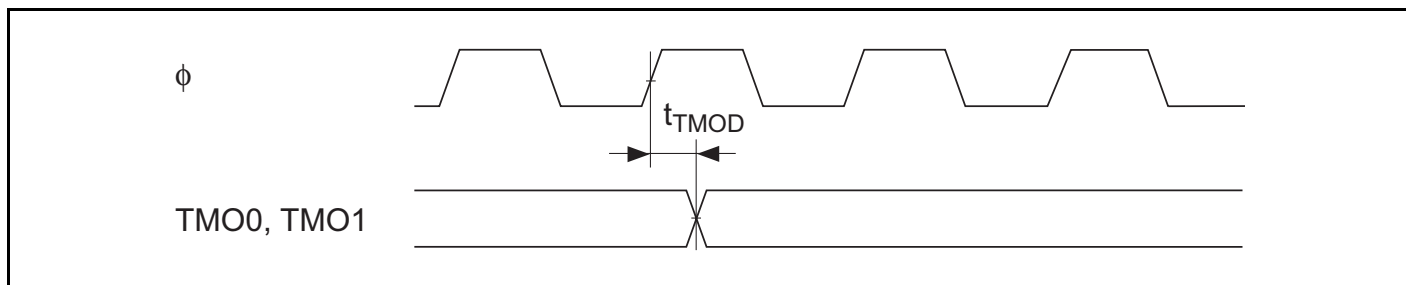
Figure 26.37 8-Bit Timer Output Timing
