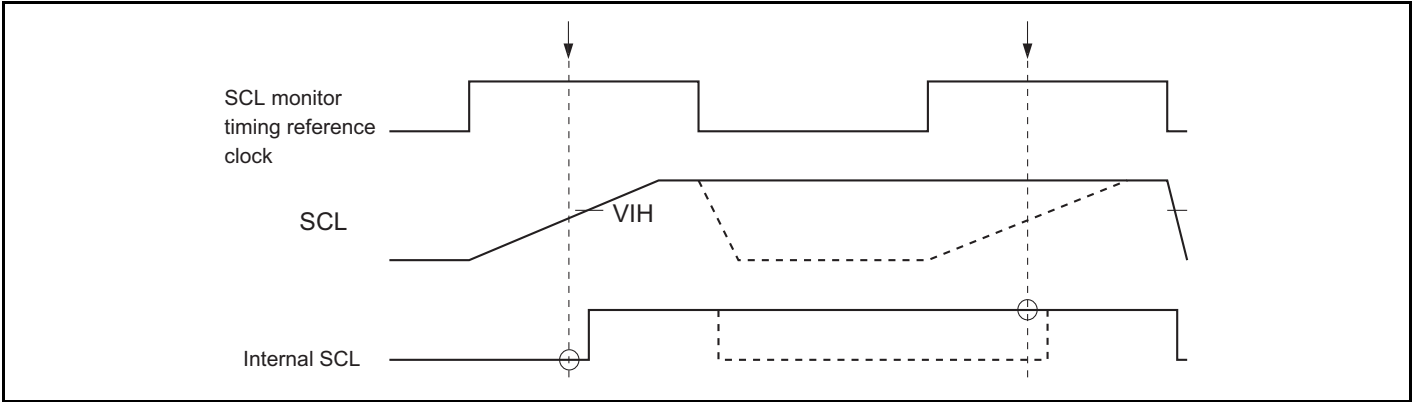
Figure 16.18 Timing of the Bit Synchronous Circuit
