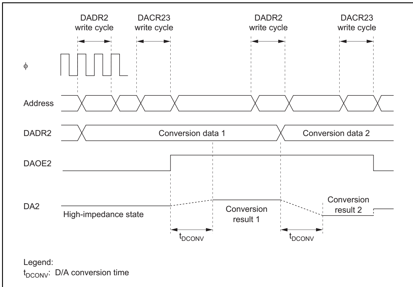
Figure 18.3 Example of D/A Converter Operation
