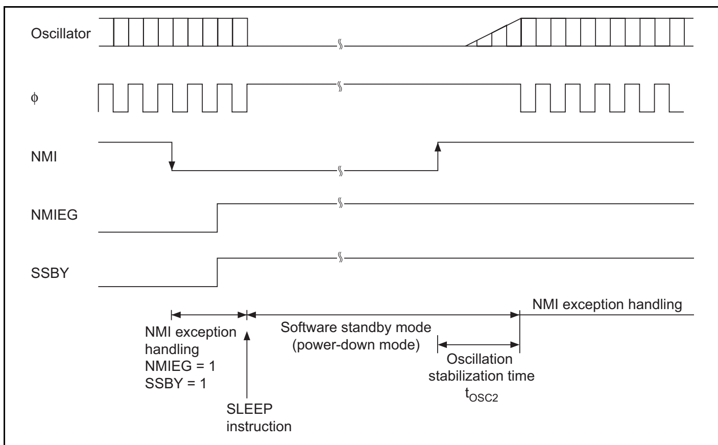
Figure 26.4 (2) Oscillation Settling Timing
