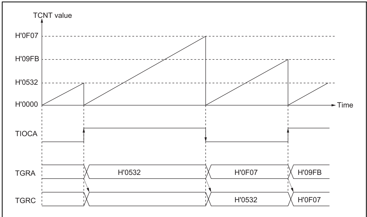
Figure 11.16 Example of Buffer Operation (2)
