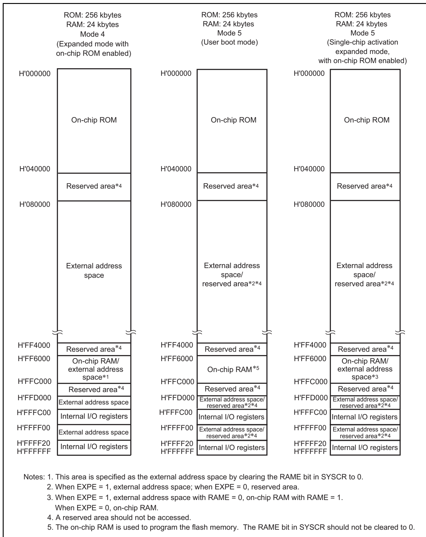
Figure 3.13 Memory Map for H8S/2371 and H8S/2371R (2)
