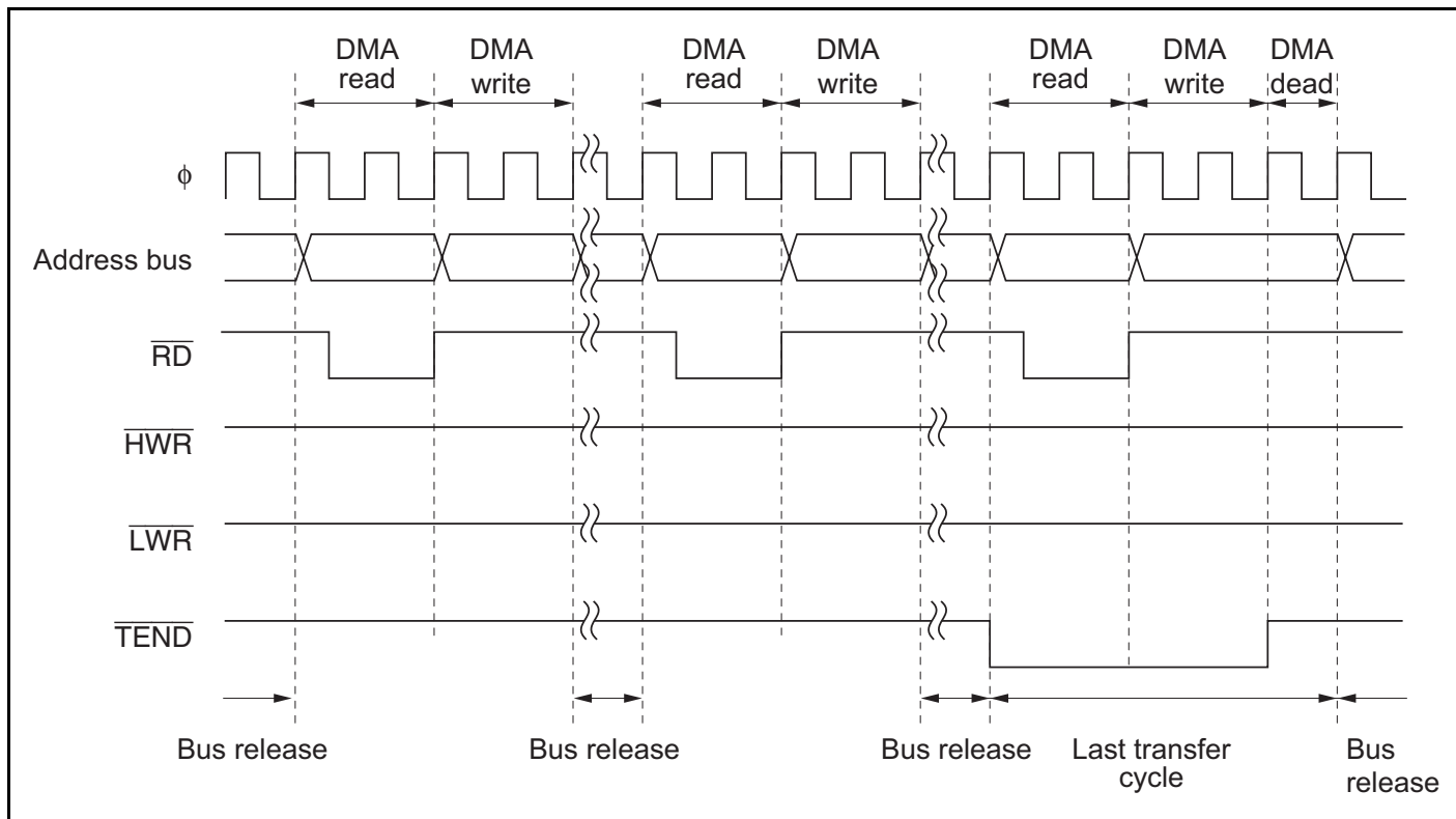
Figure 7.18 Example of Short Address Mode Transfer
