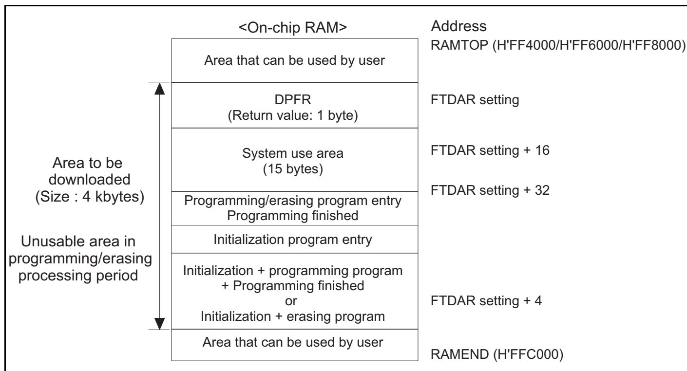
Figure 21.10 RAM Map when Programming/Erasing Is Executed
