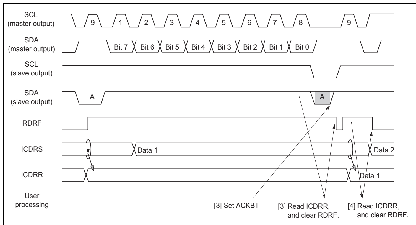
Figure 16.12 Slave Receive Mode Operation Timing 2
