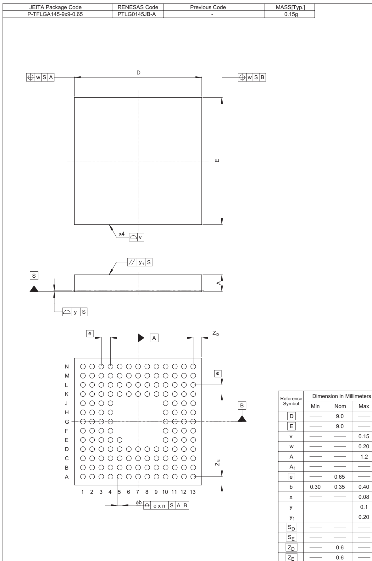
Figure C.2 Package Dimensions (TLP-145V)
