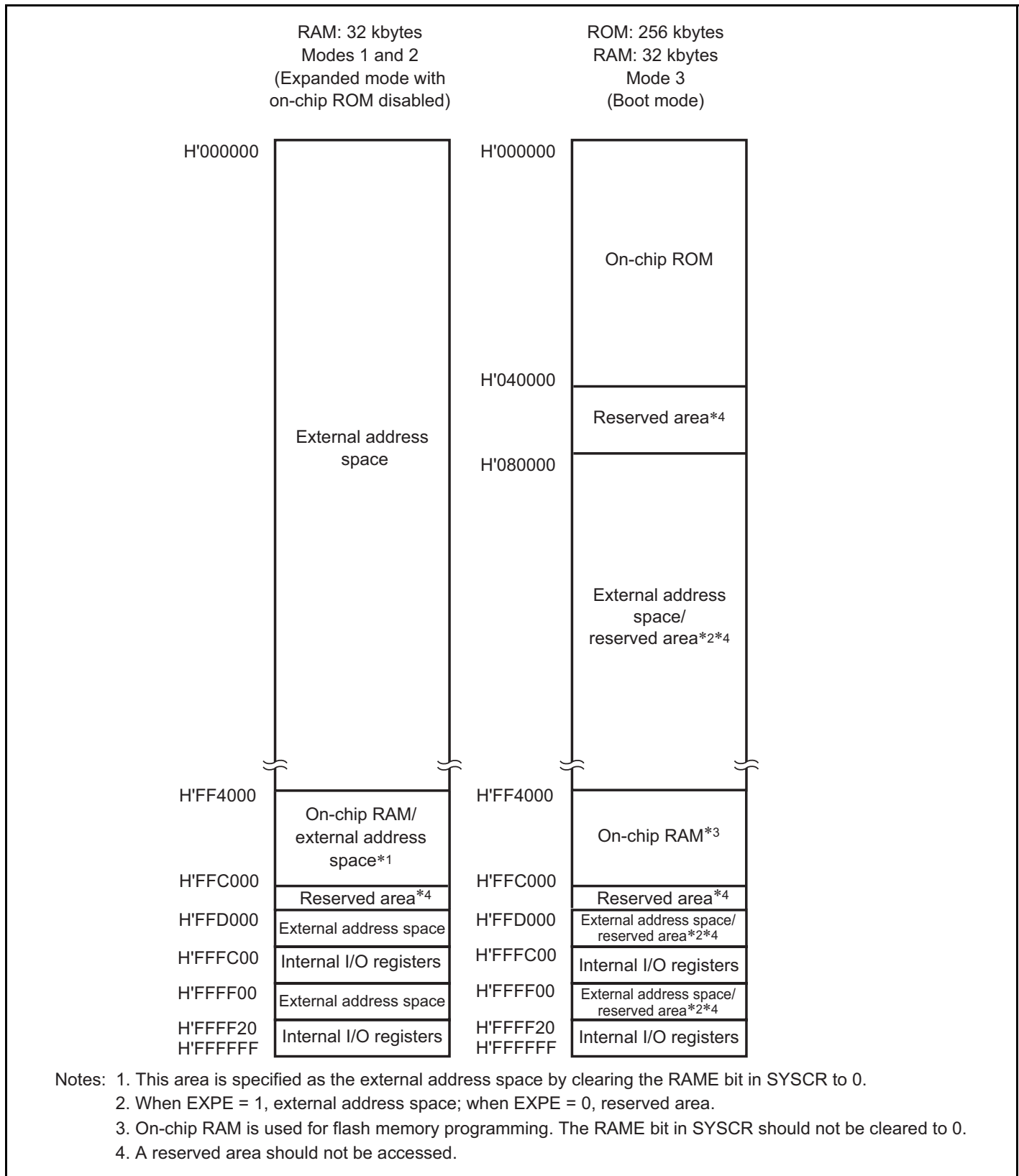
Figure 3.10 Memory Map for H8S/2372 and H8S/2372R (1)
