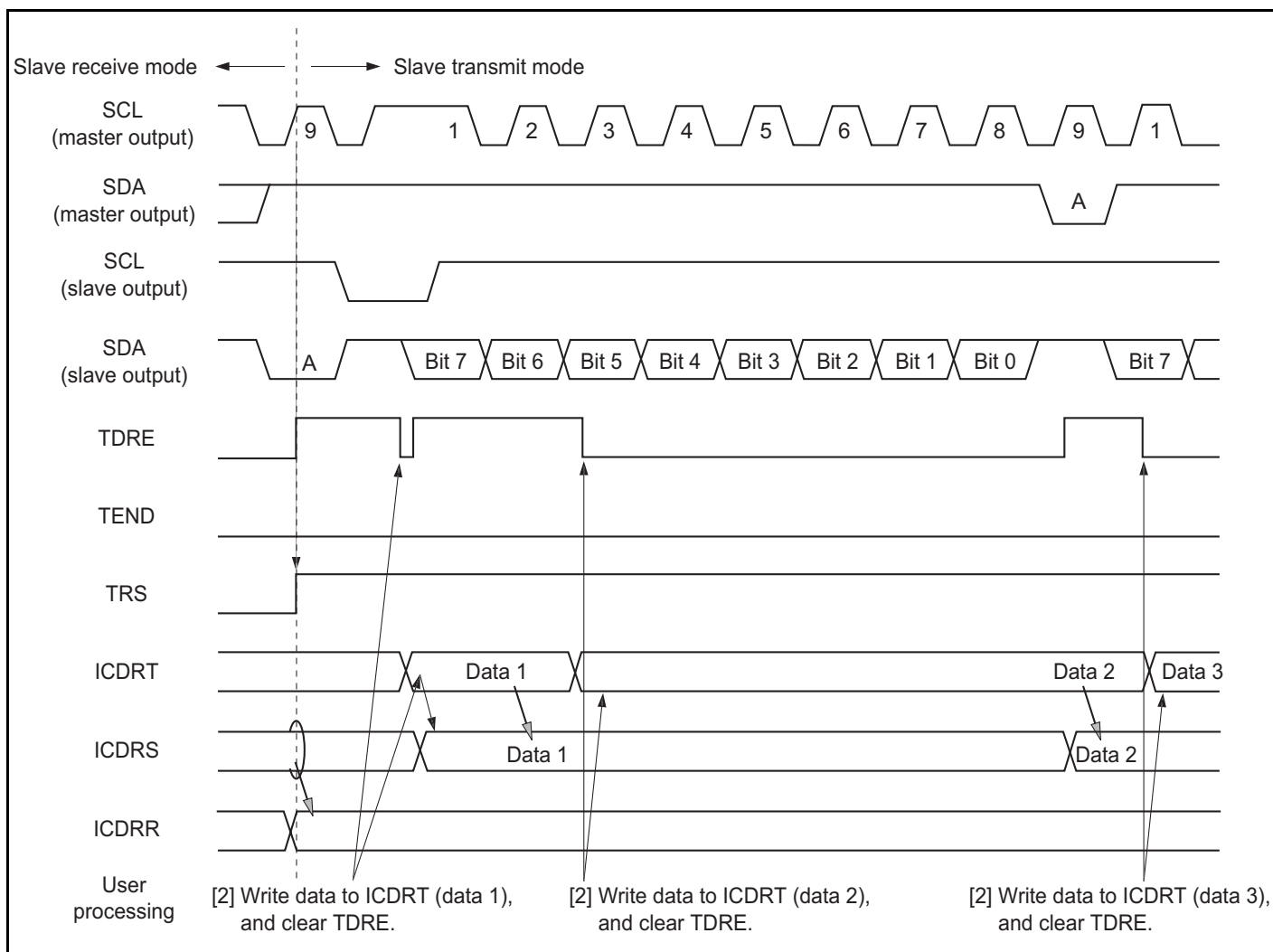
Figure 16.9 Slave Transmit Mode Operation Timing 1
