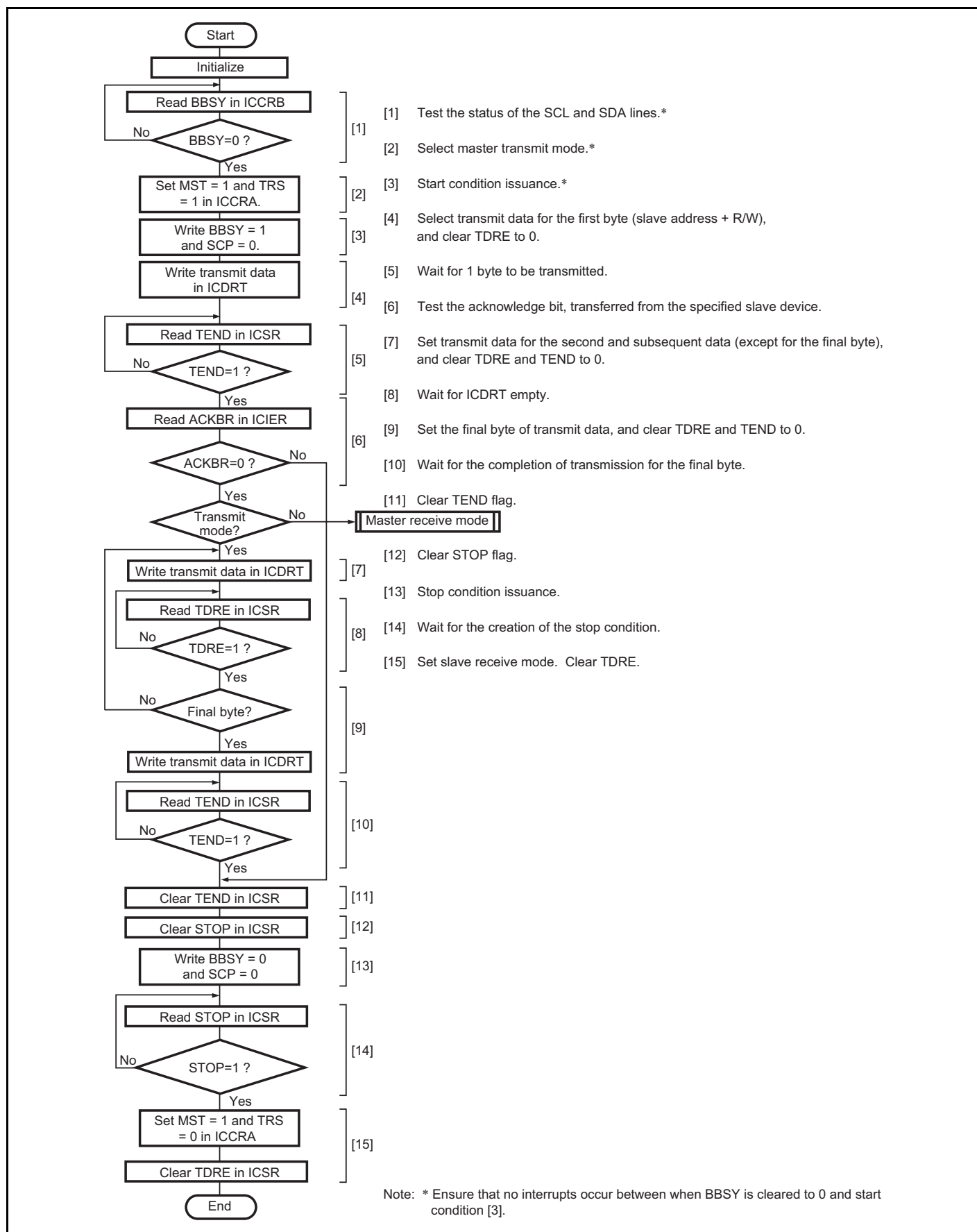
Figure 16.14 Sample Flowchart for Master Transmit Mode
