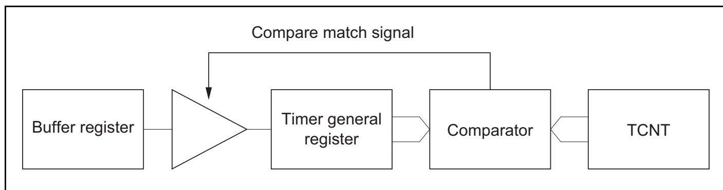
Figure 11.12 Compare Match Buffer Operation
