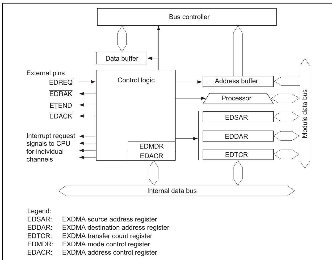
Figure 8.1 Block Diagram of EXDMAC
