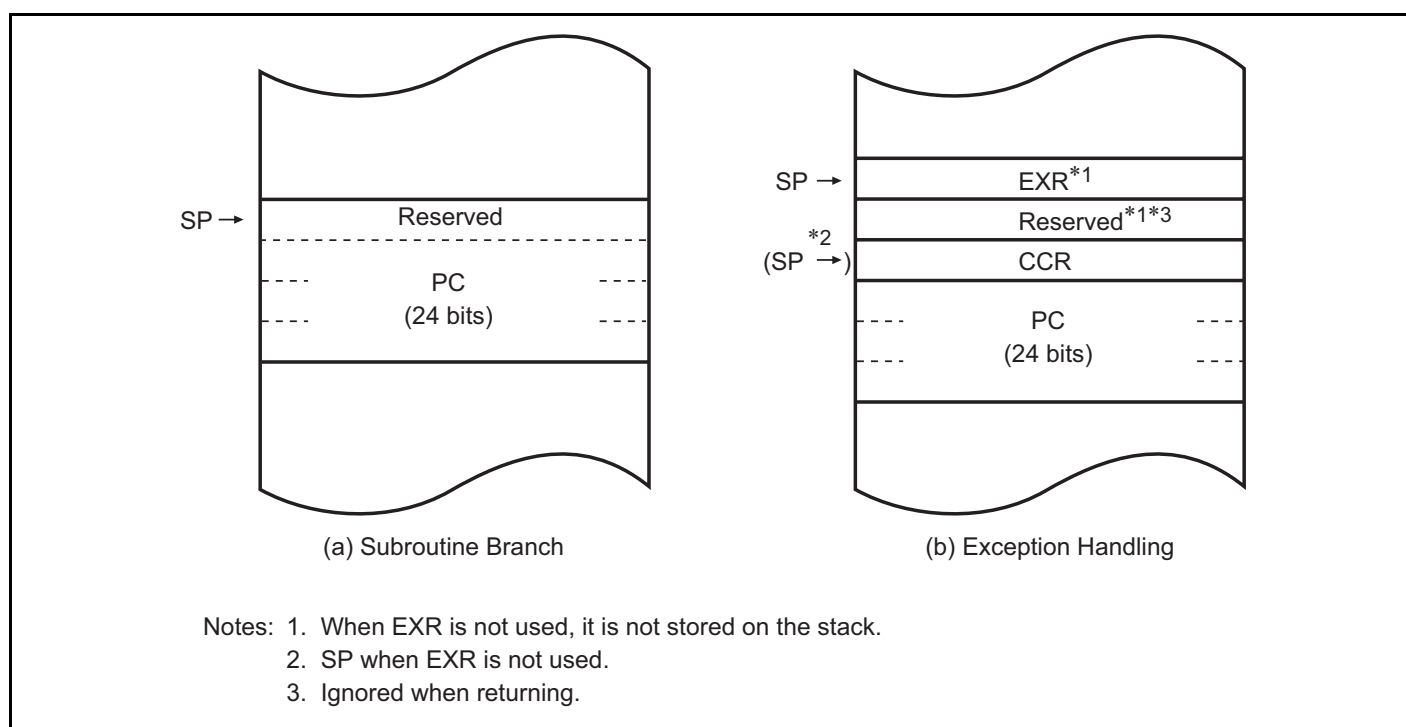
Figure 2.4 Stack Structure in Advanced Mode
