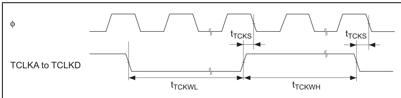
Figure 26.36 TPU Clock Input Timing
