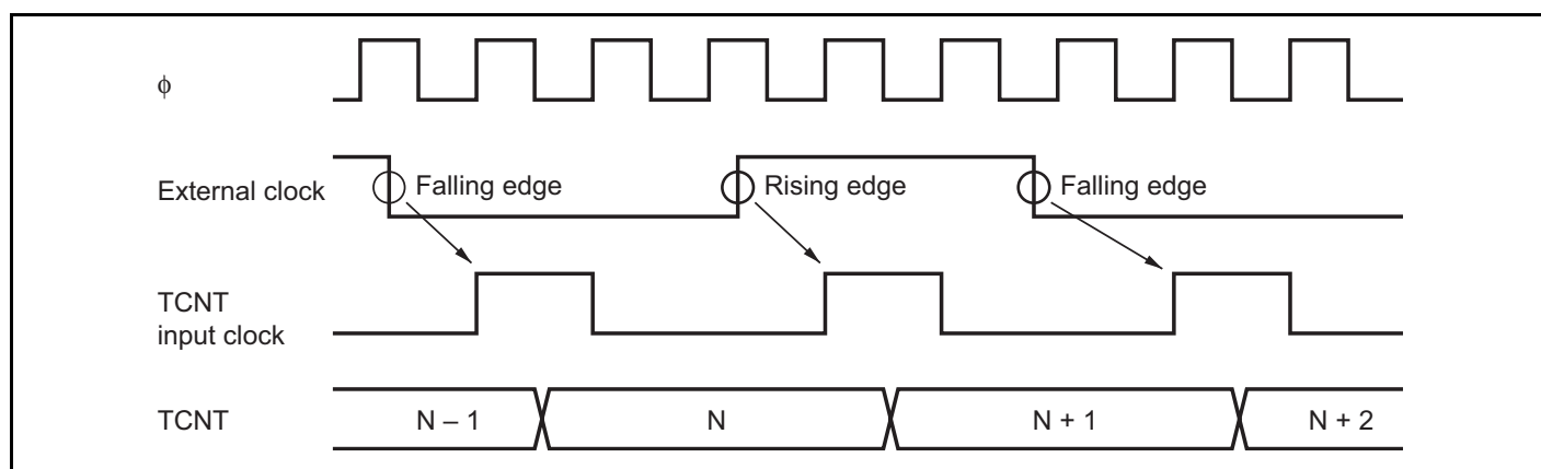
Figure 11.31 Count Timing in External Clock Operation
