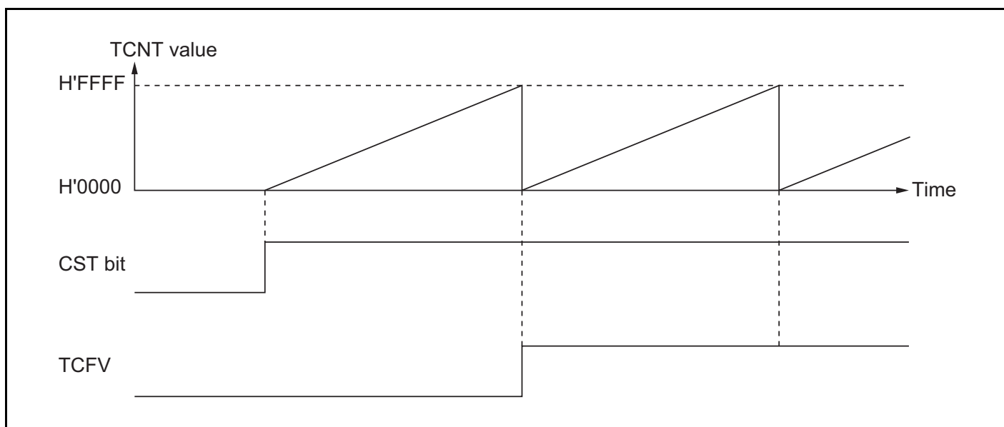
Figure 11.3 Free-Running Counter Operation
