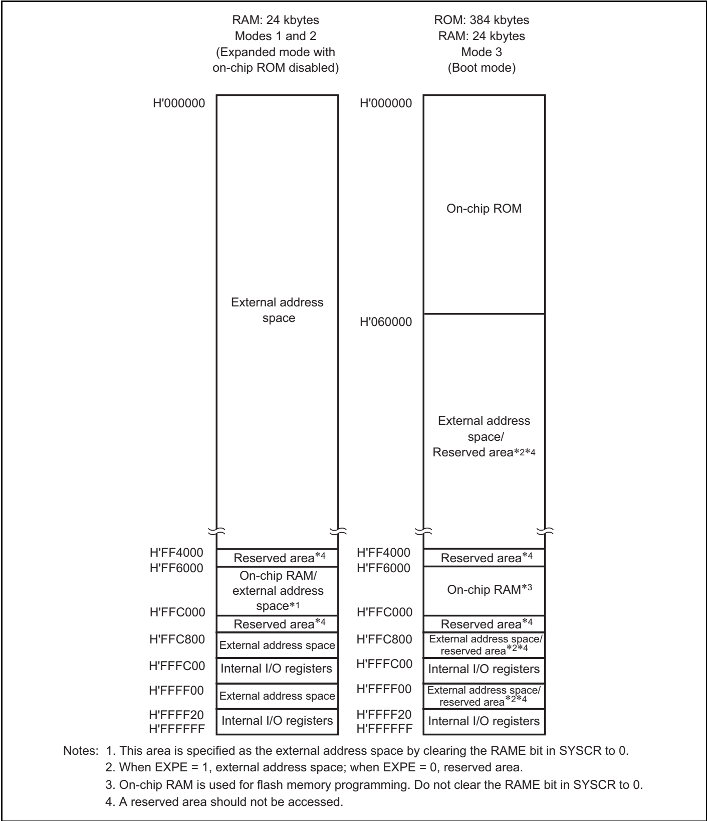
Figure 3.3 Memory Map for H8S/2377 and H8S/2377R (1)
