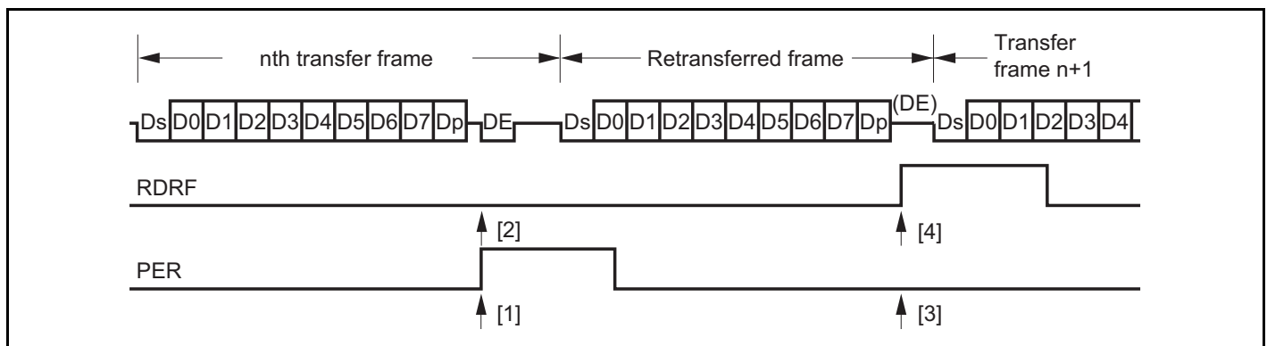
Figure 15.29 Retransfer Operation in SCI Receive Mode
