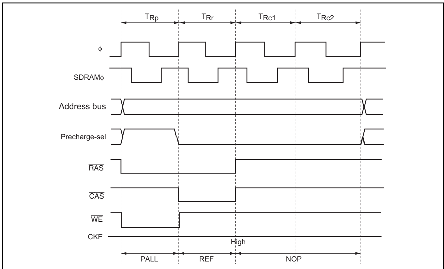
Figure 6.54 Auto Refresh Timing
