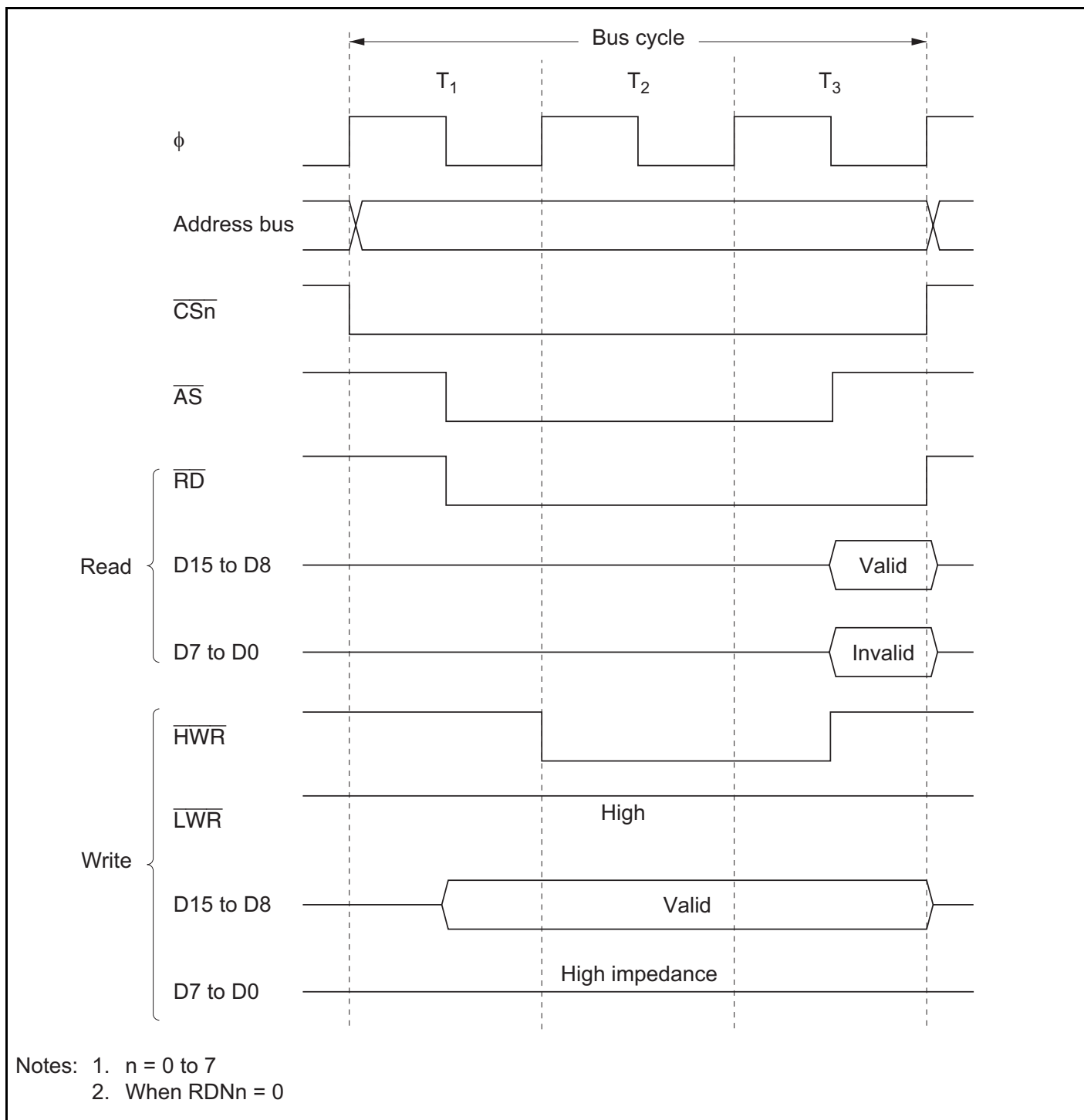
Figure 6.11 Bus Timing for 8-Bit, 3-State Access Space
