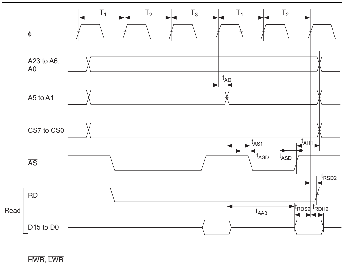
Figure 26.13 Burst ROM Access Timing: Two-State Burst Access
