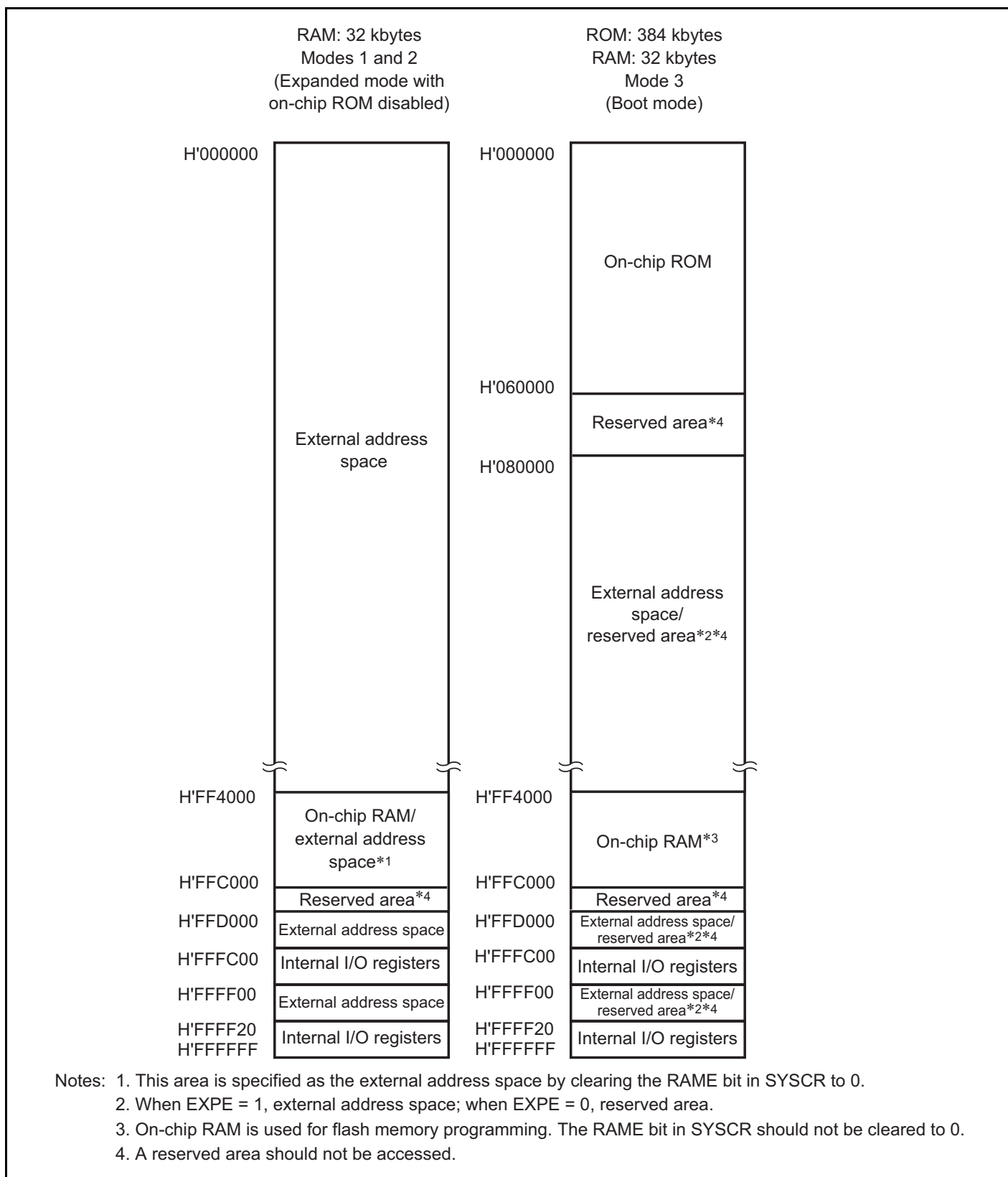
Figure 3.7 Memory Map for H8S/2374 and H8S/2374R (1)
