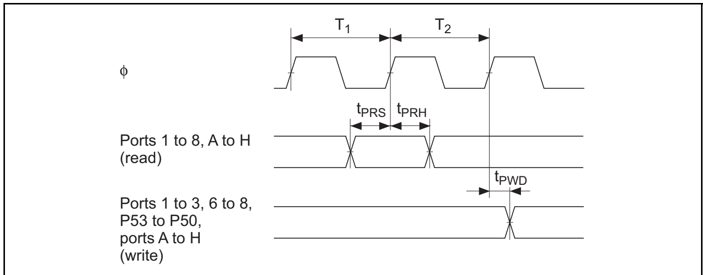
Figure 26.33 I/O Port Input/Output Timing
