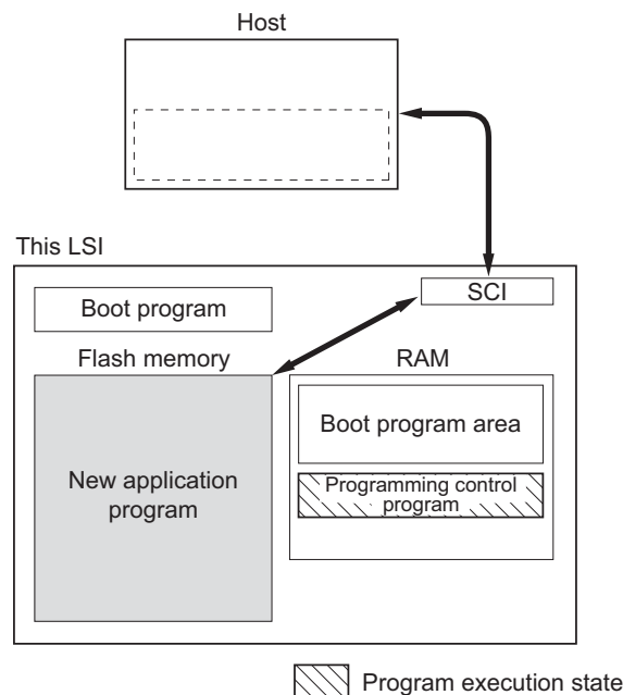
Figure 20.3 Boot Mode
