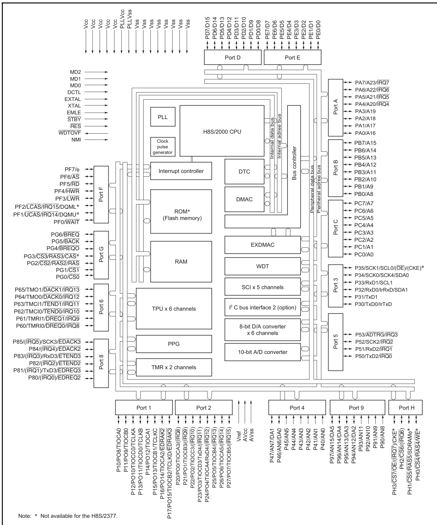
Figure 1.2 Internal Block Diagram for H8S/2377 and H8S/2377R
