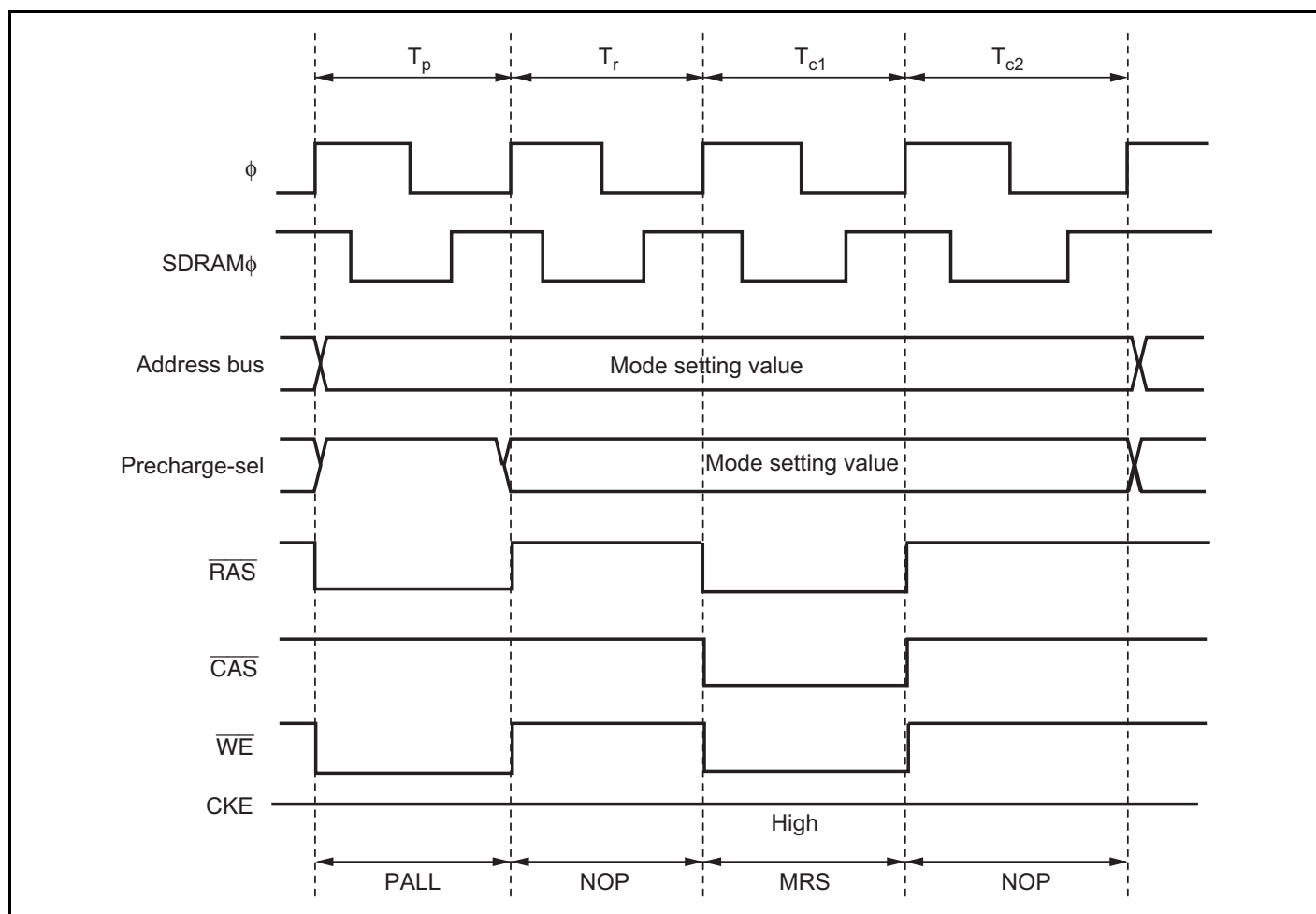
Figure 6.59 Synchronous DRAM Mode Setting Timing
