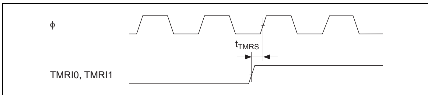
Figure 26.39 8-Bit Timer Reset Input Timing
