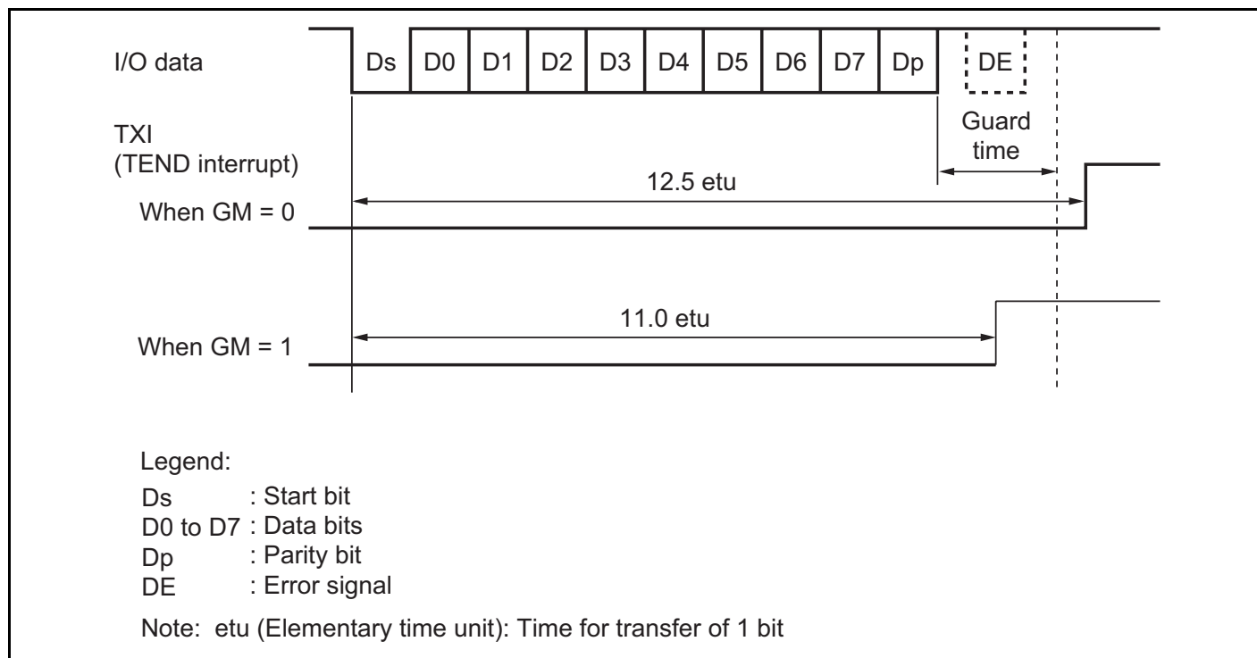
Figure 15.27 TEND Flag Generation Timing in Transmission Operation
