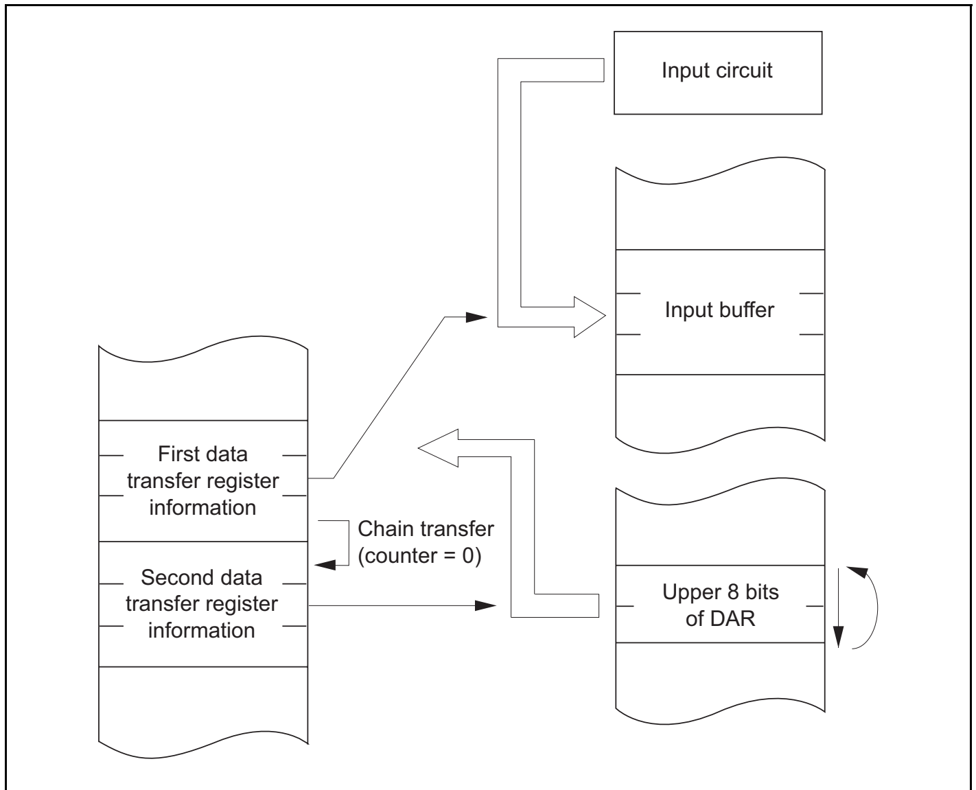
Figure 9.13 Chain Transfer when Counter = 0
