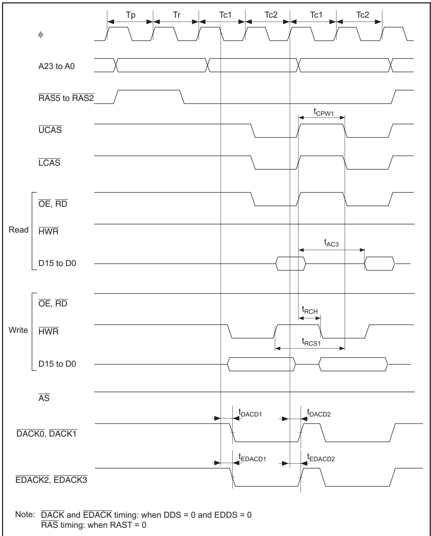
Figure 26.16 DRAM Access Timing: Two-State Burst Access
