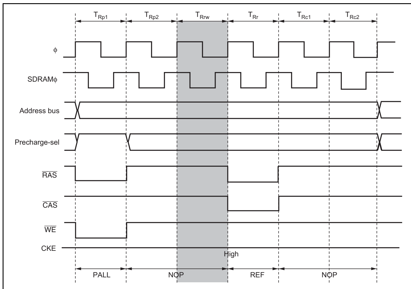
Figure 6.55 Auto Refresh Timing (TPC = 1, TPC0 = 1, RCW1 = 0, RCW0 = 1)
