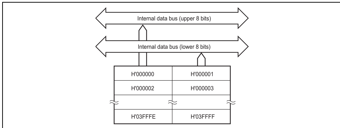
Figure 22.1 Block Diagram of 256-kbyte Masked ROM (HD6432375)
