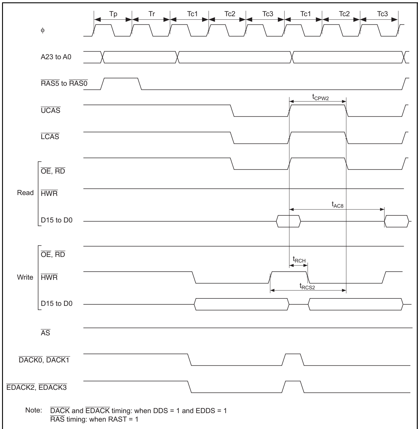
Figure 26.18 DRAM Access Timing: Three-State Burst Access
