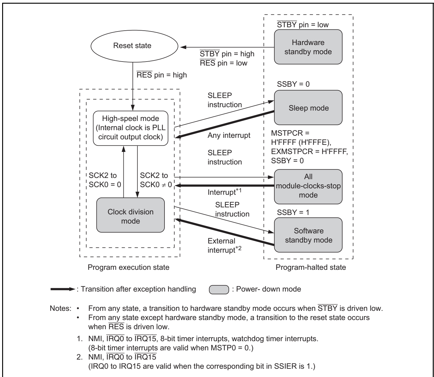
Figure 24.1 Mode Transitions
