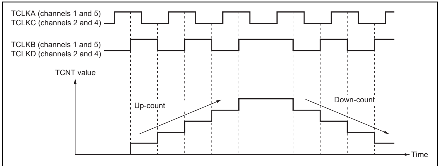
Figure 11.28 Example of Phase Counting Mode 4 Operation
