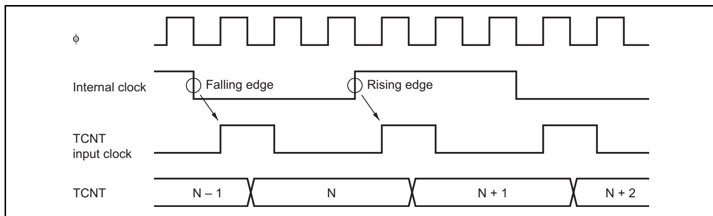
Figure 11.30 Count Timing in Internal Clock Operation
