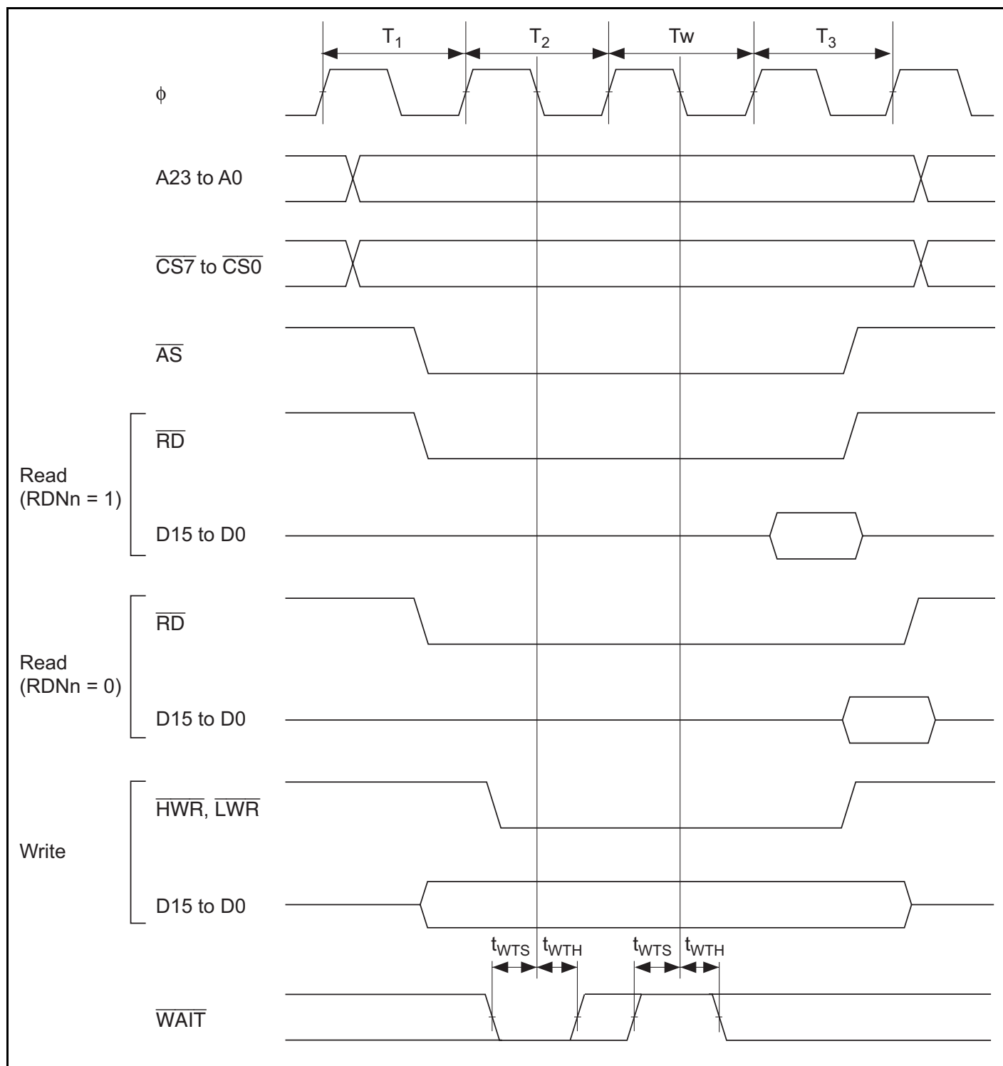
Figure 26.9 Basic Bus Timing: Three-State Access, One Wait
