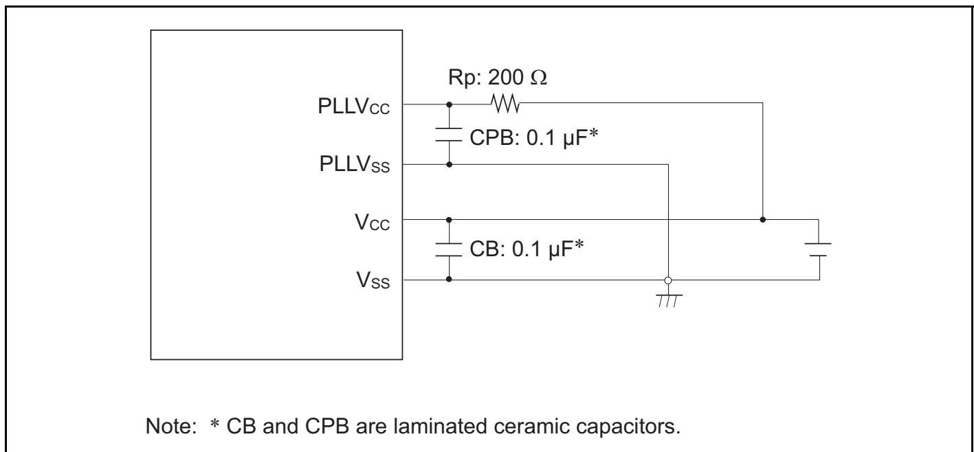
Figure 23.7 Recommended External Circuitry for PLL Circuit
