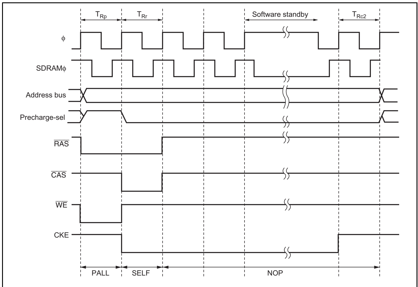
Figure 6.57 Self-Refresh Timing
