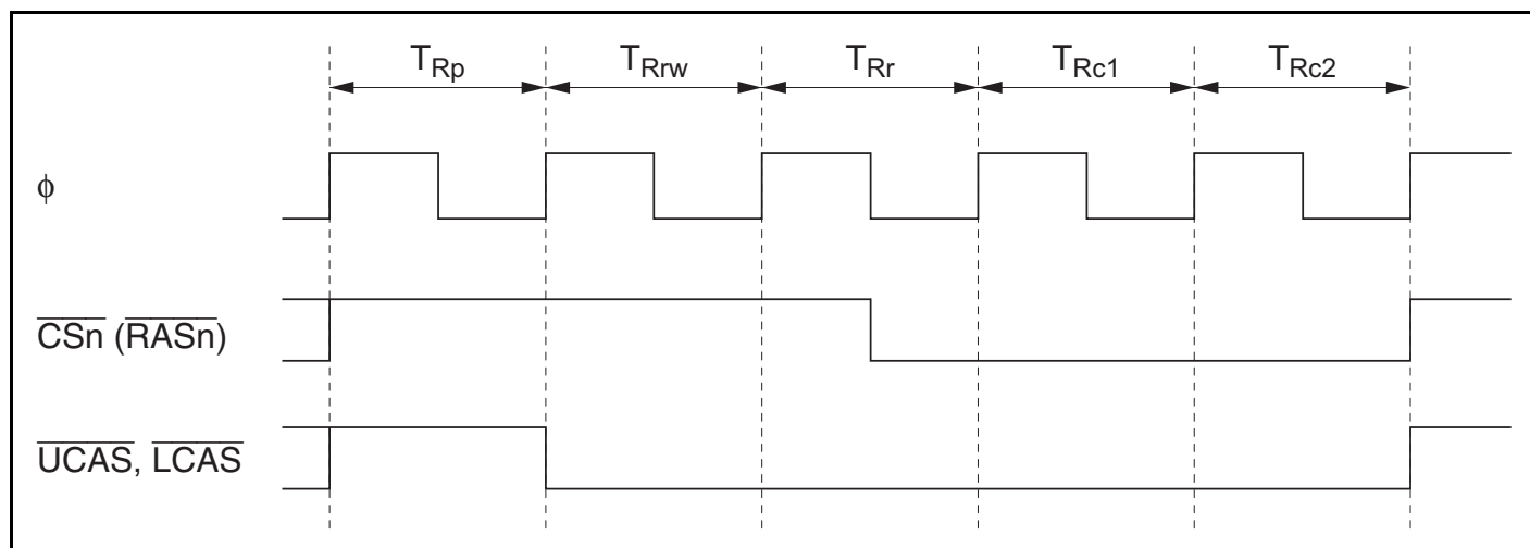
Figure 6.37 CBR Refresh Timing (RCW1 = 0, RCW0 = 1, RLW1 = 0, RLW0 = 0)
