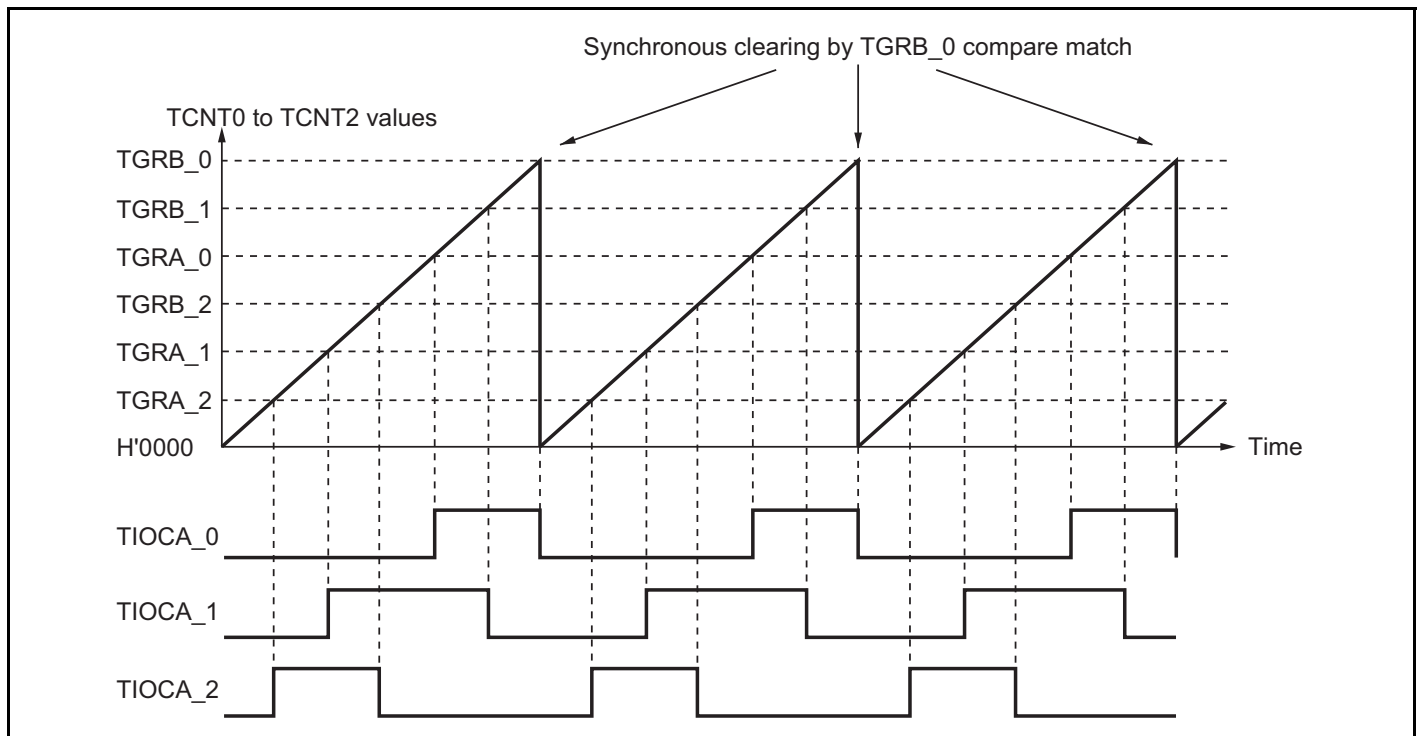
Figure 11.11 Example of Synchronous Operation
