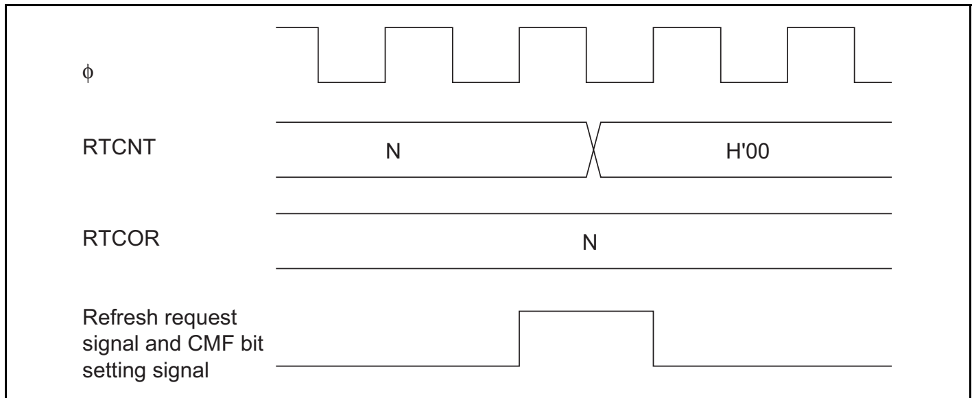
Figure 6.35 Compare Match Timing
