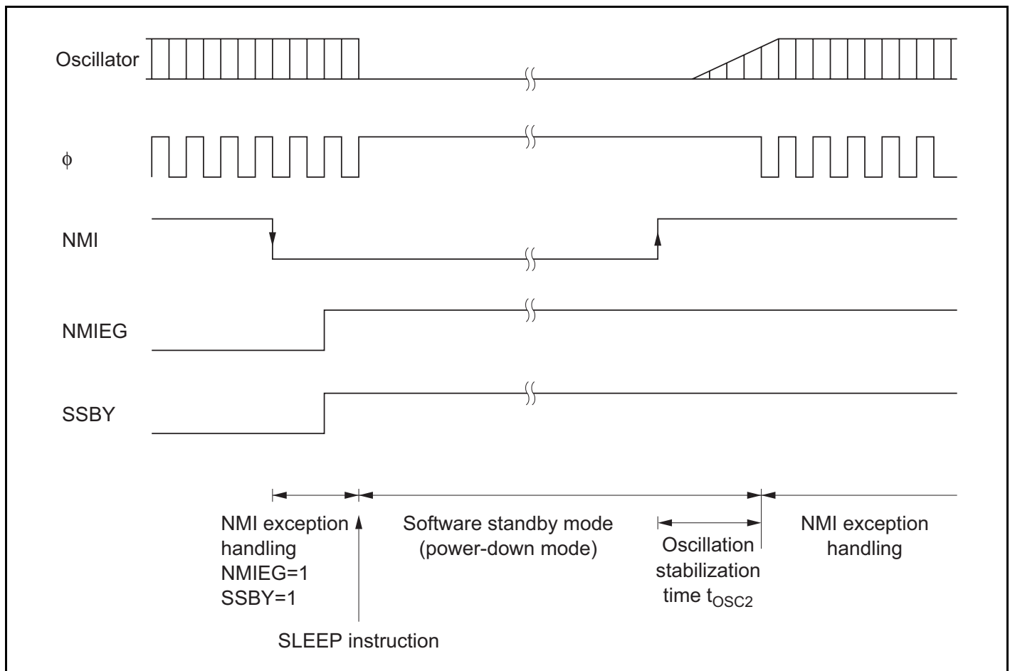
Figure 24.2 Software Standby Mode Application Example
