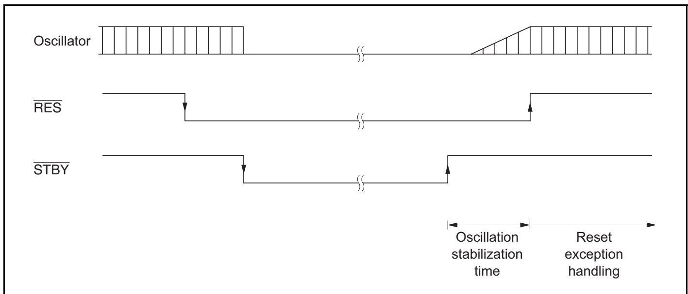
Figure 24.3 Hardware Standby Mode Timing
