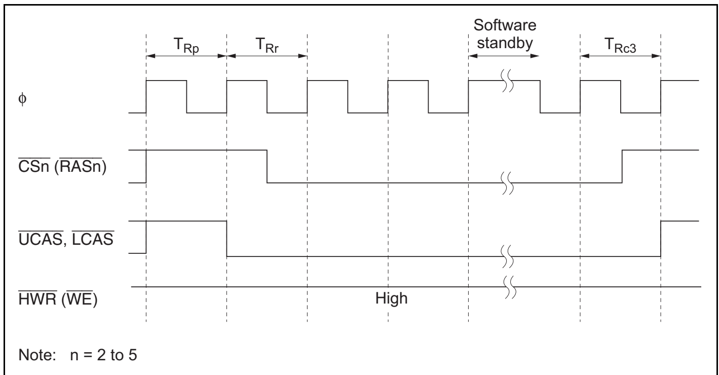
Figure 6.39 Self-Refresh Timing
