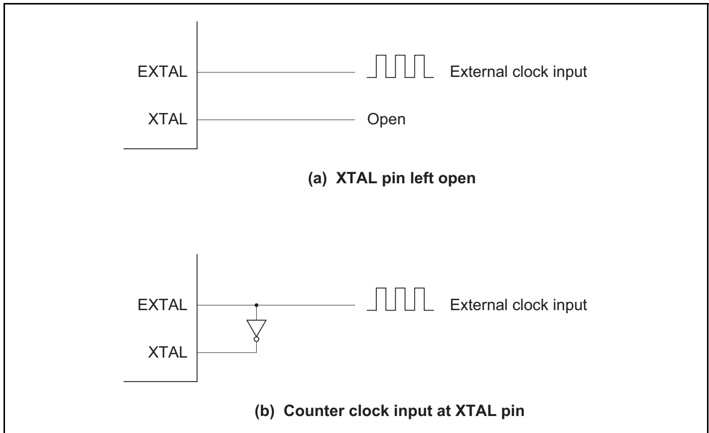
Figure 23.4 External Clock Input (Examples)
