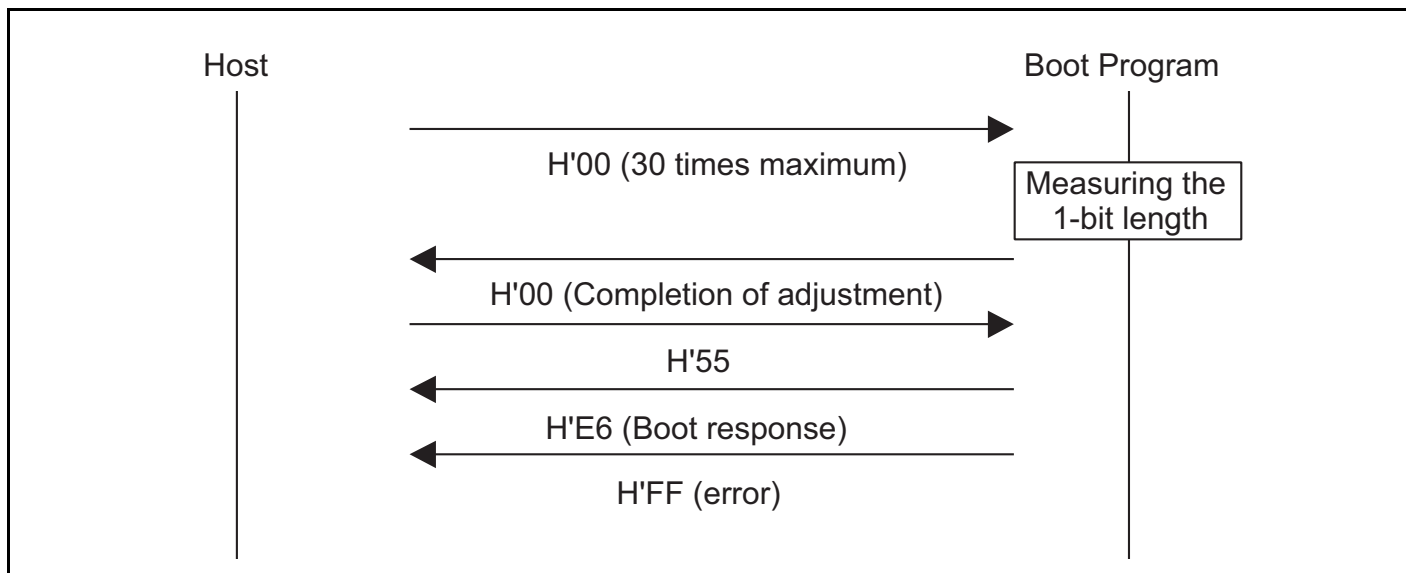
Figure 21.18 Bit-Rate-Adjustment Sequence
