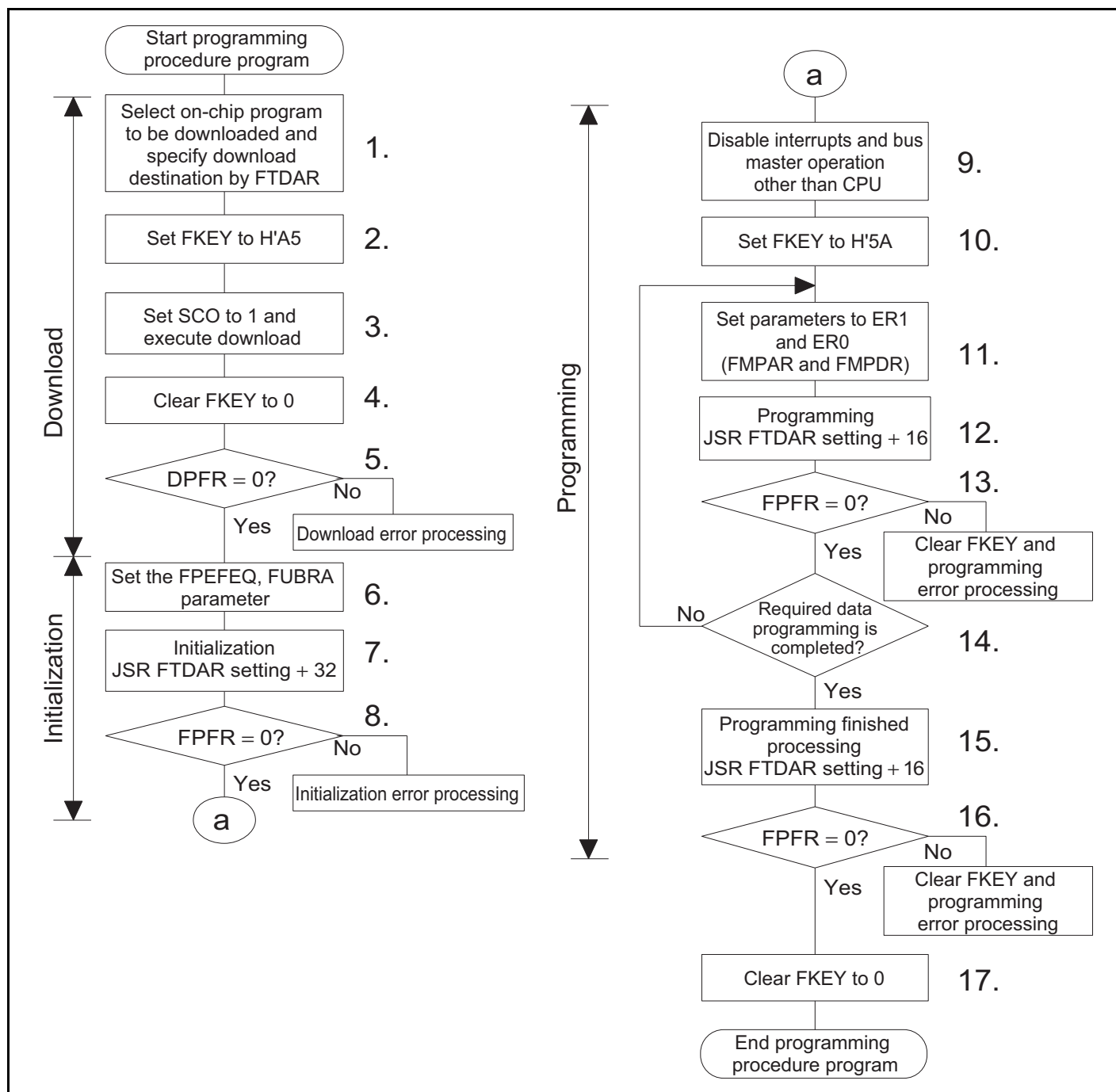
Figure 21.11 Programming Procedure
