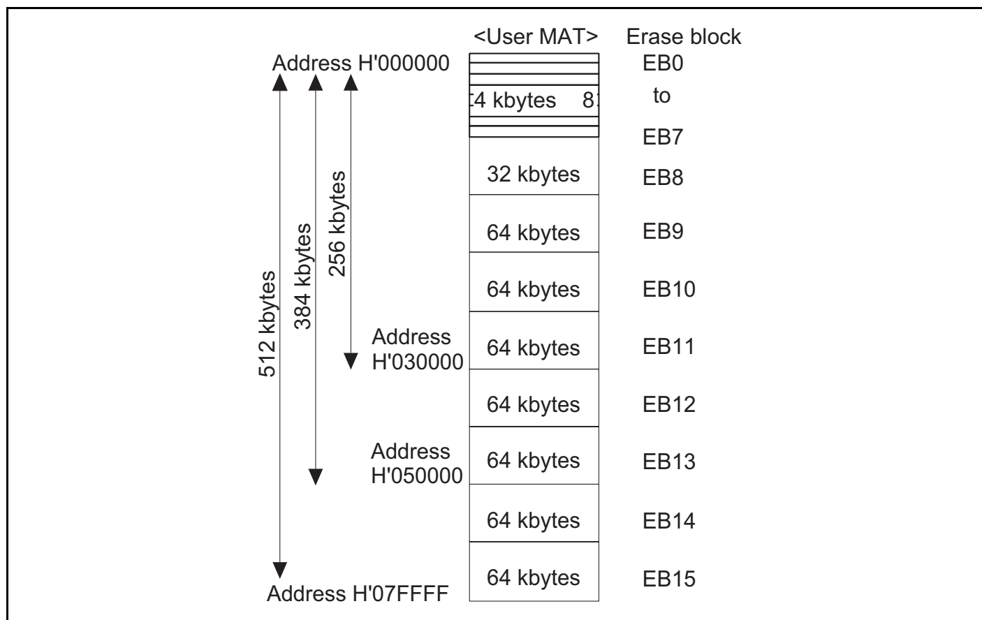
Figure 21.4 Block Division of User MAT
