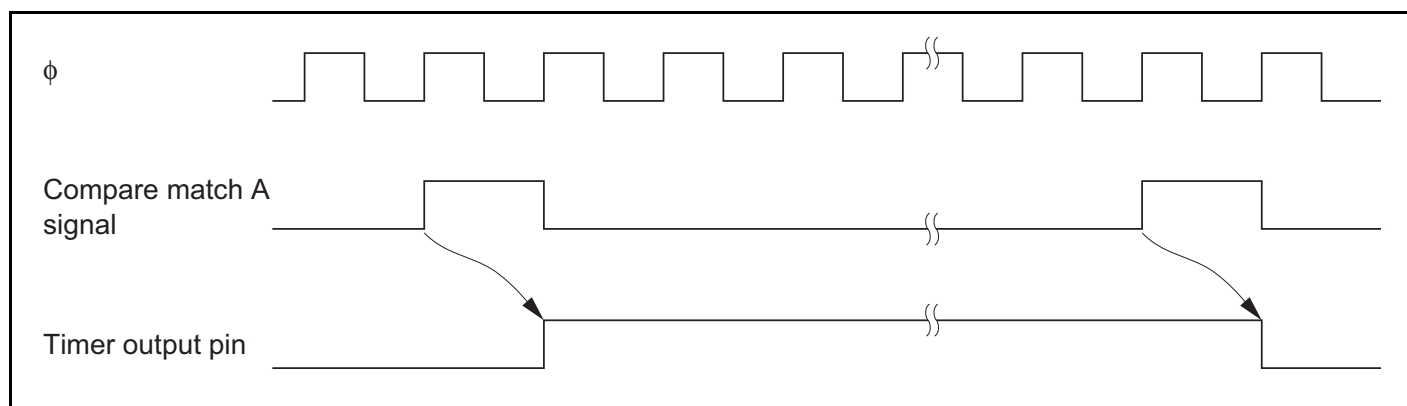
Figure 13.6 Timing of Timer Output
