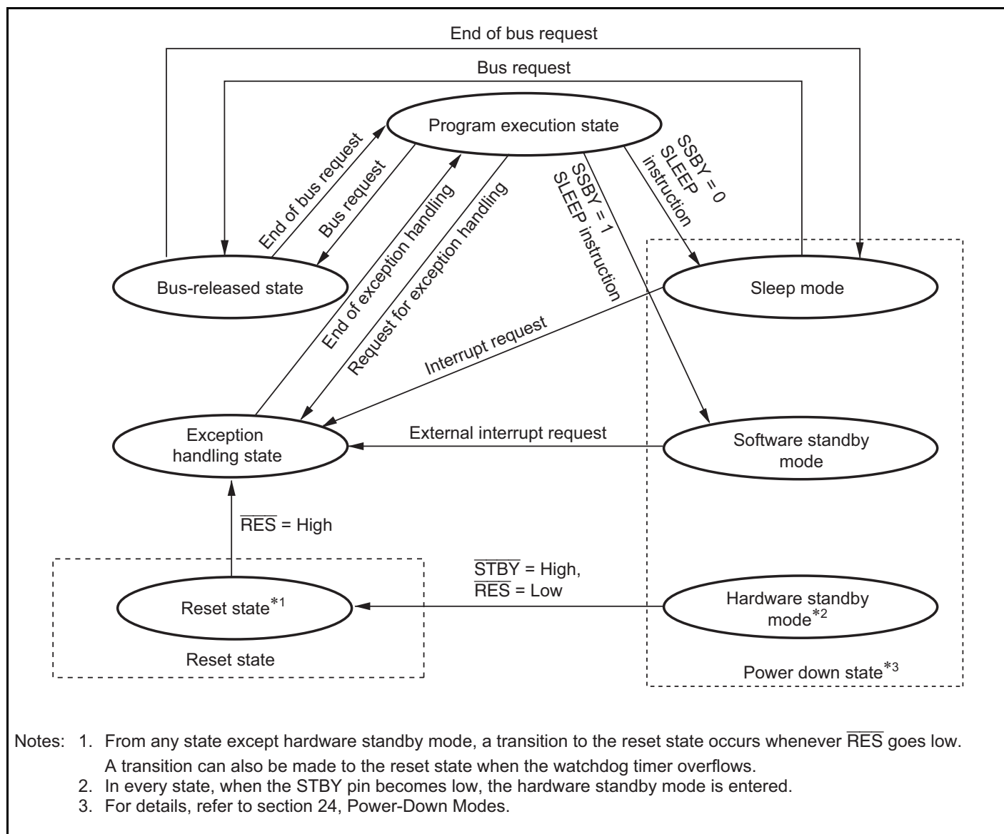
Figure 2.13 State Transitions
