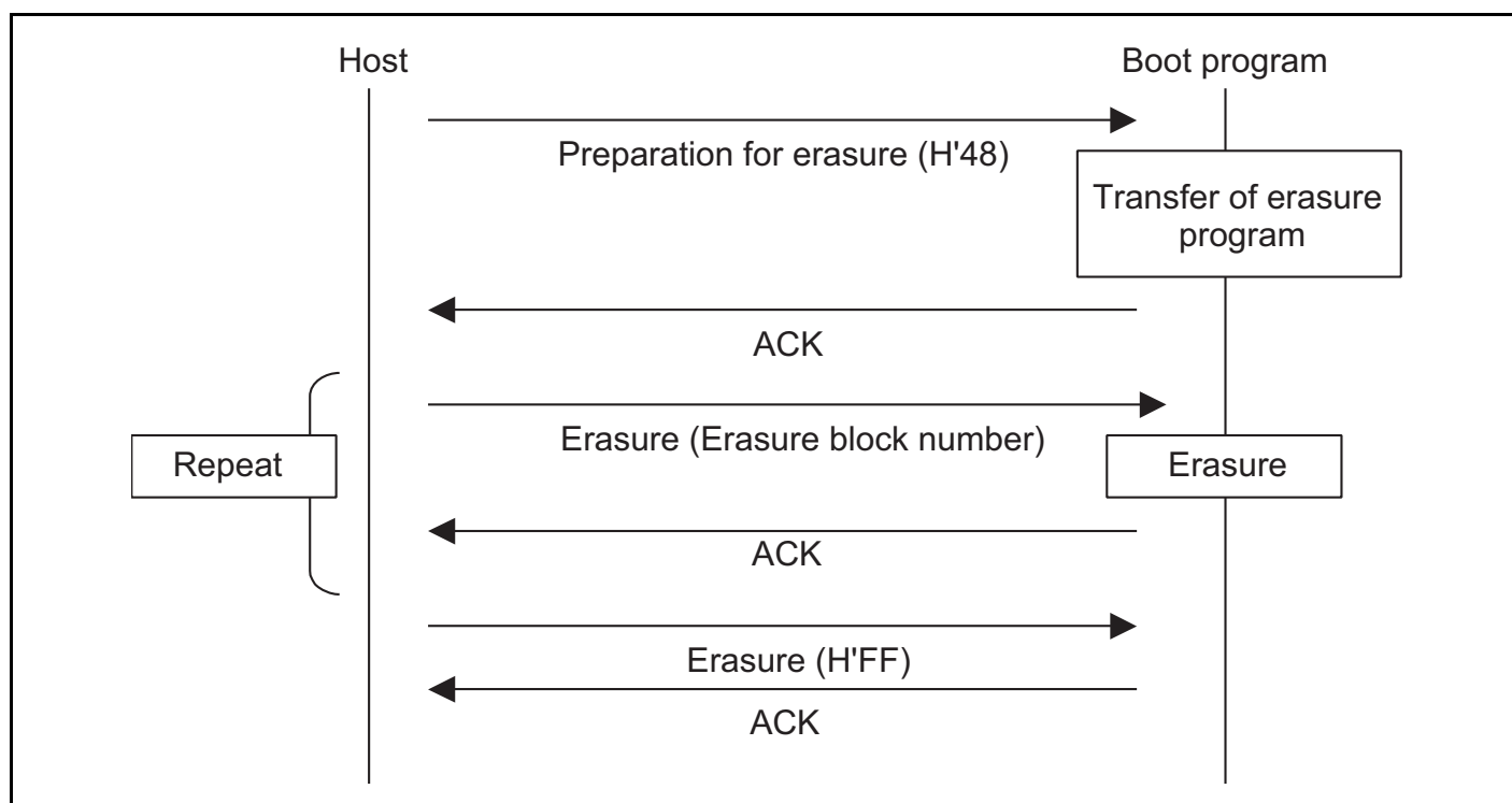
Figure 21.22 Erasure Sequence
