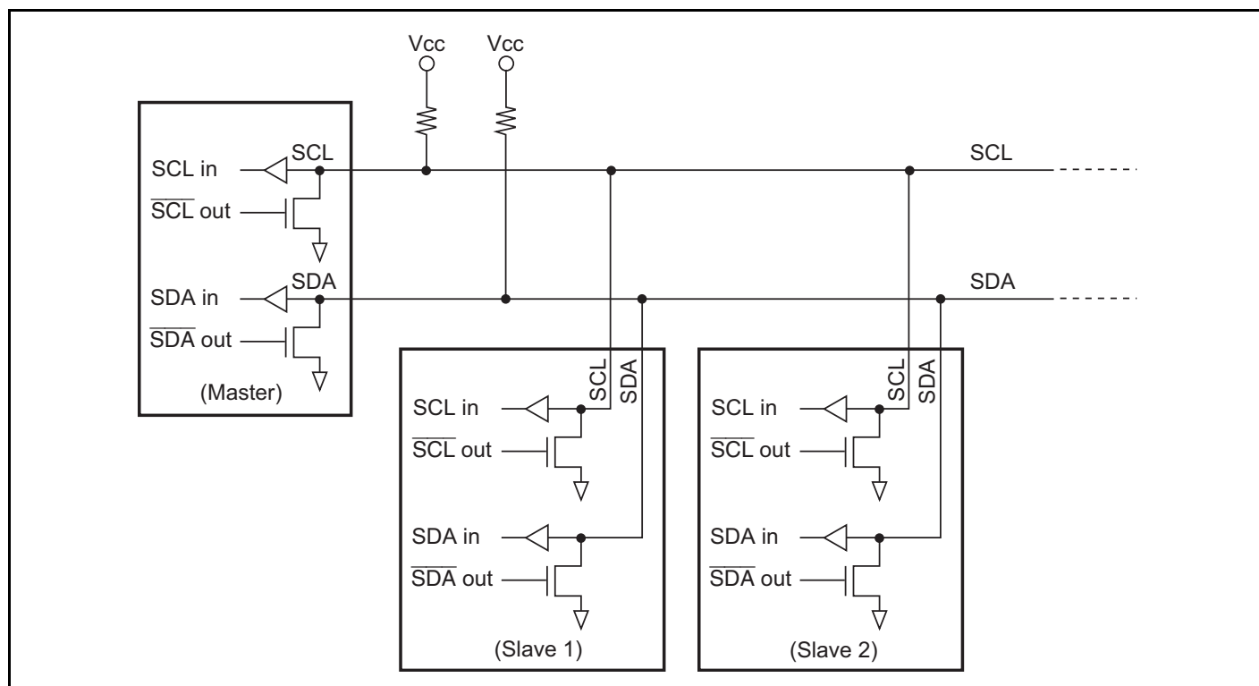
Figure 16.2 External Circuit Connections of I/O Pins
