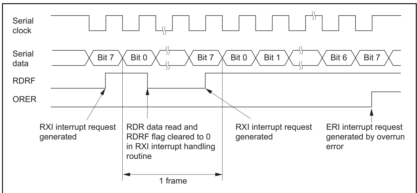
Figure 15.18 Example of SCI Operation in Reception
