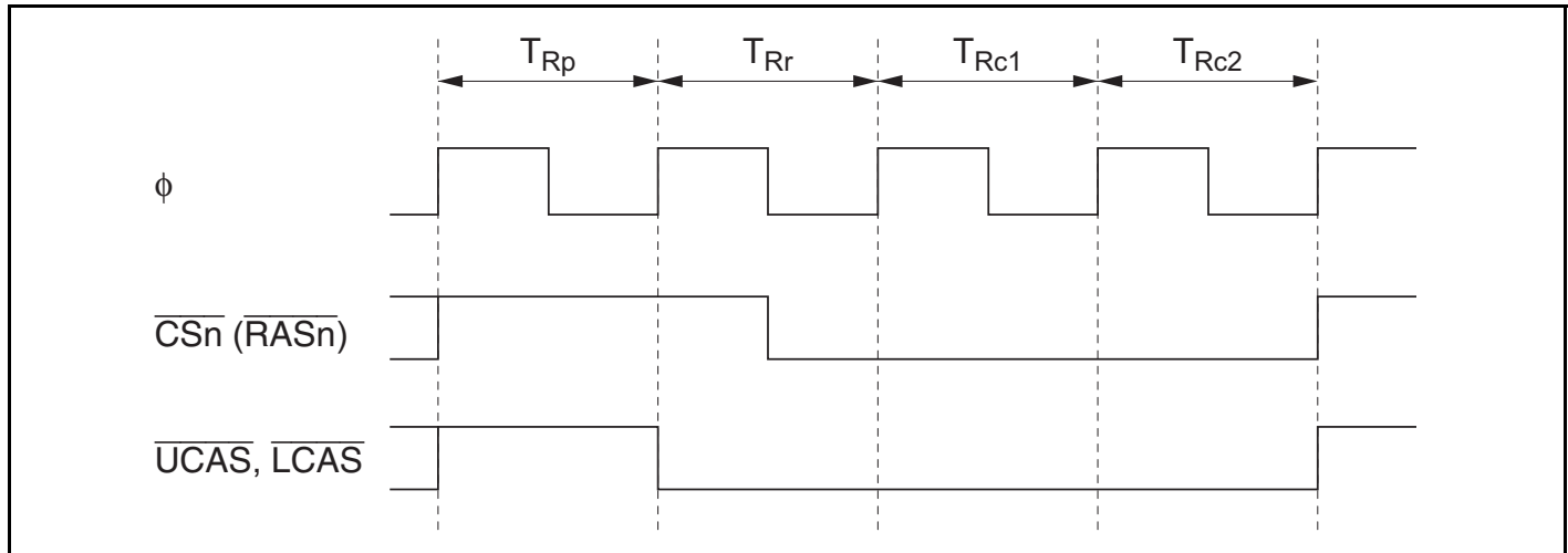
Figure 6.36 CBR Refresh Timing
