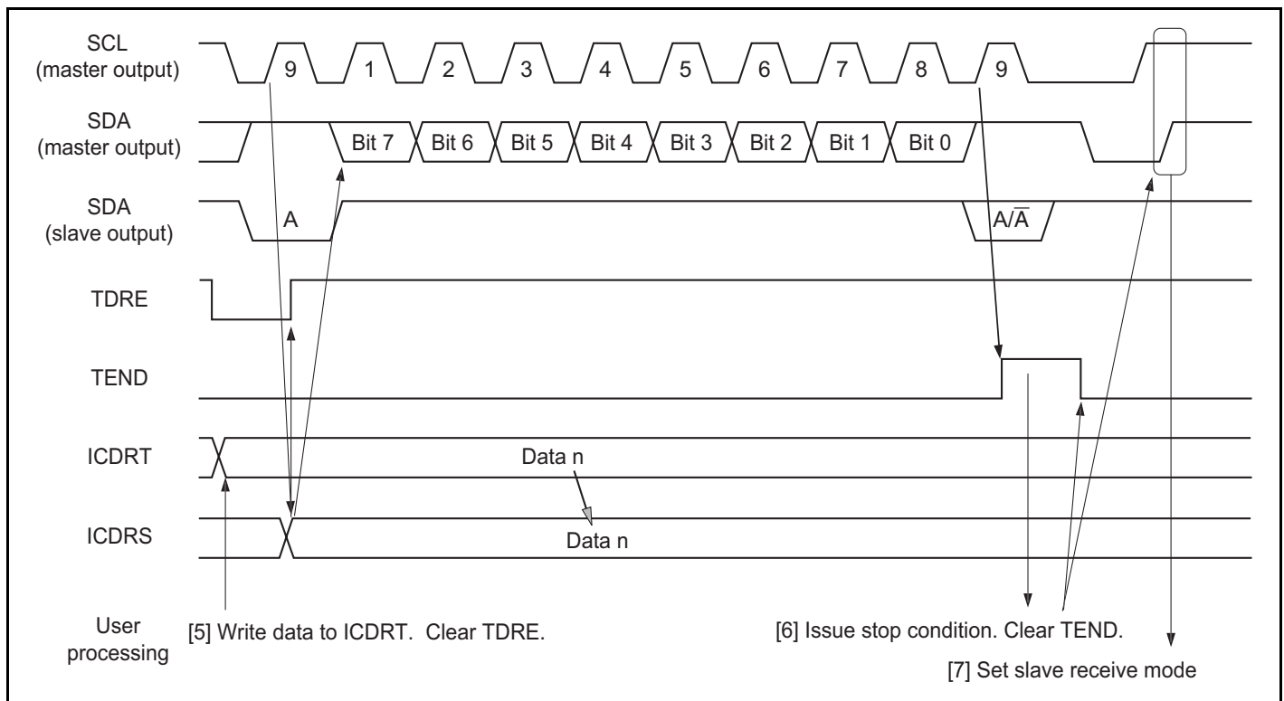
Figure 16.6 Master Transmit Mode Operation Timing 2
