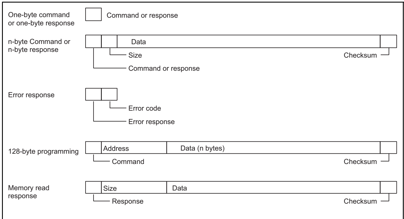
Figure 21.19 Communication Protocol Format
