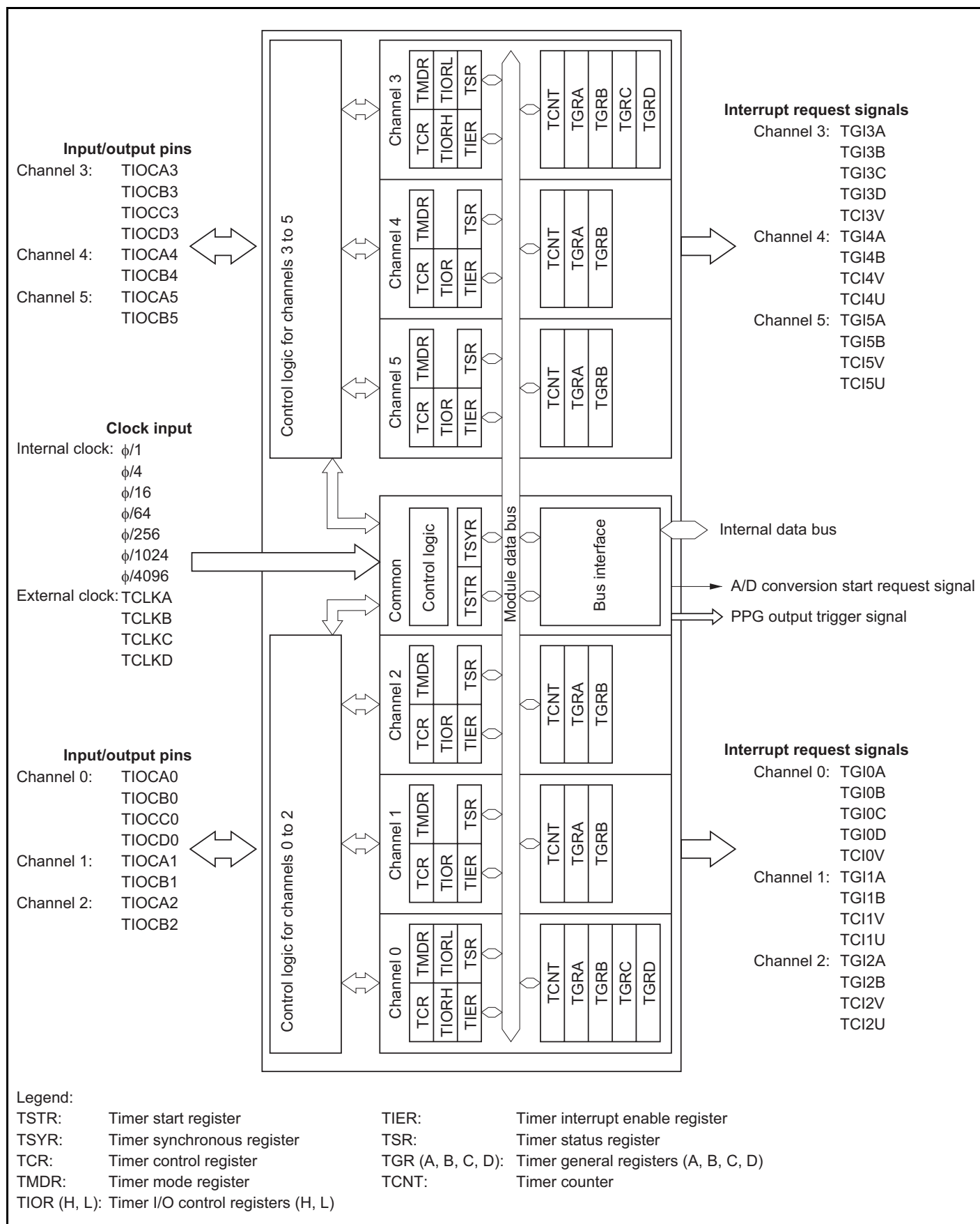
Figure 11.1 Block Diagram of TPU
