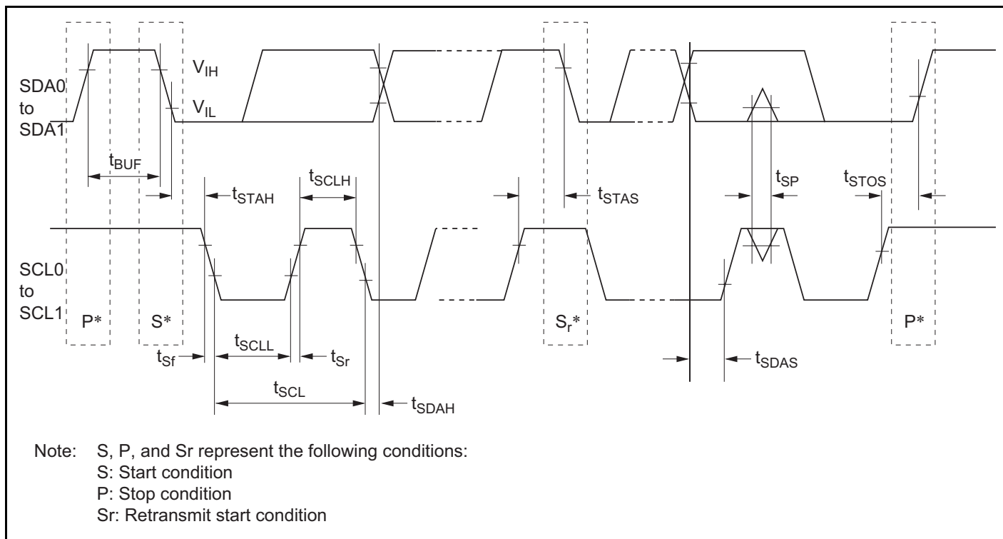
Figure 26.44 I 2 C Bus Interface 2 Input/Output Timing (Option)
