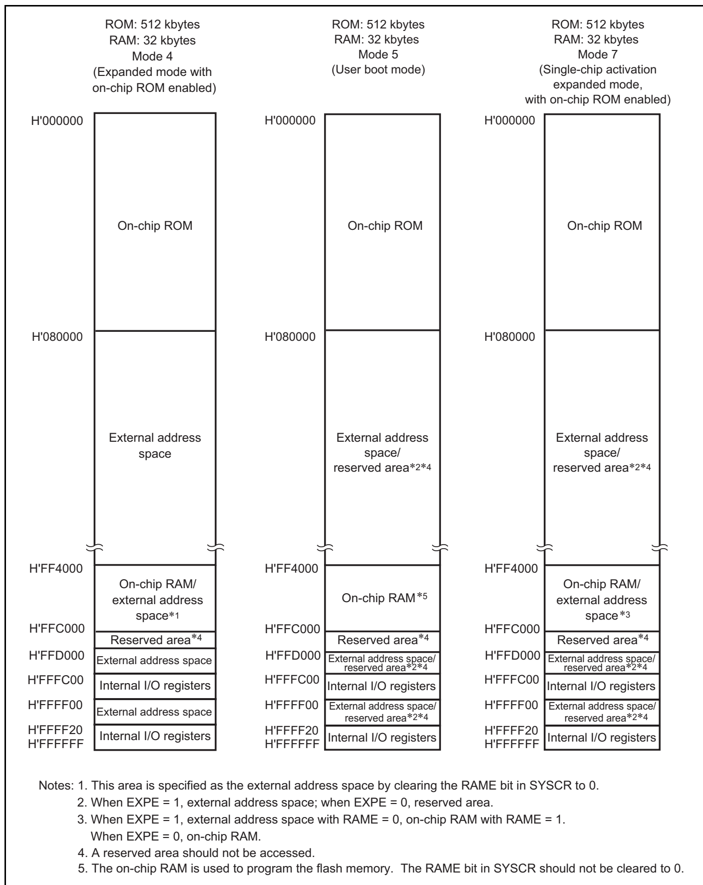
Figure 3.2 Memory Map for H8S/2378 and H8S/2378R (2)
