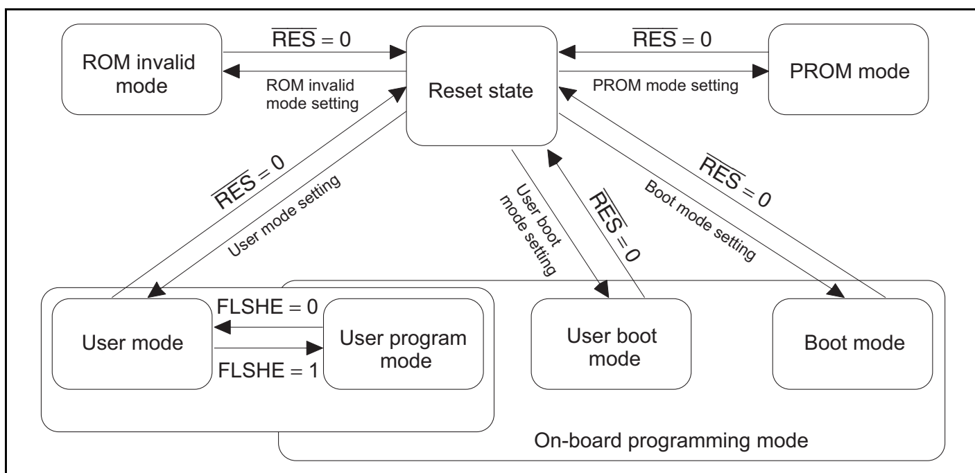
Figure 21.2 Mode Transition of Flash Memory
