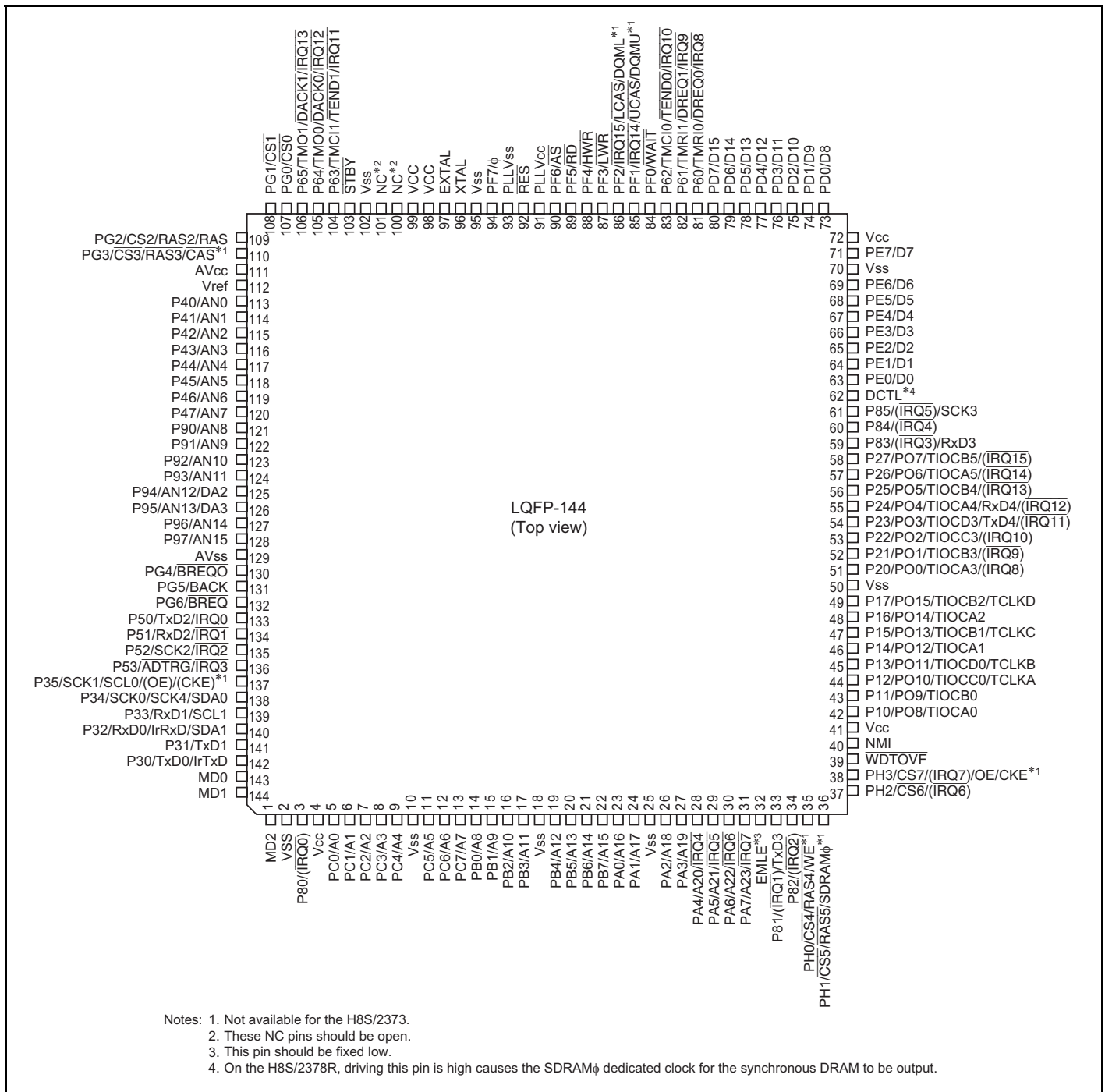
Figure 1.8 Pin Arrangement for H8S/2373 and H8S/2373R
