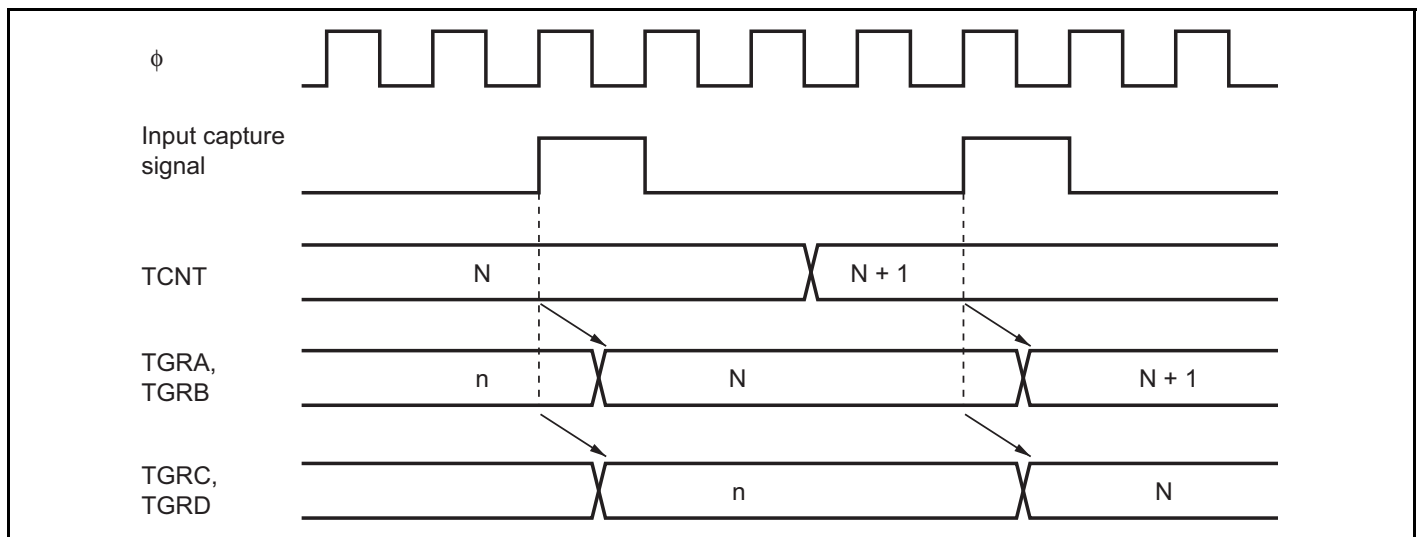
Figure 11.37 Buffer Operation Timing (Input Capture)
