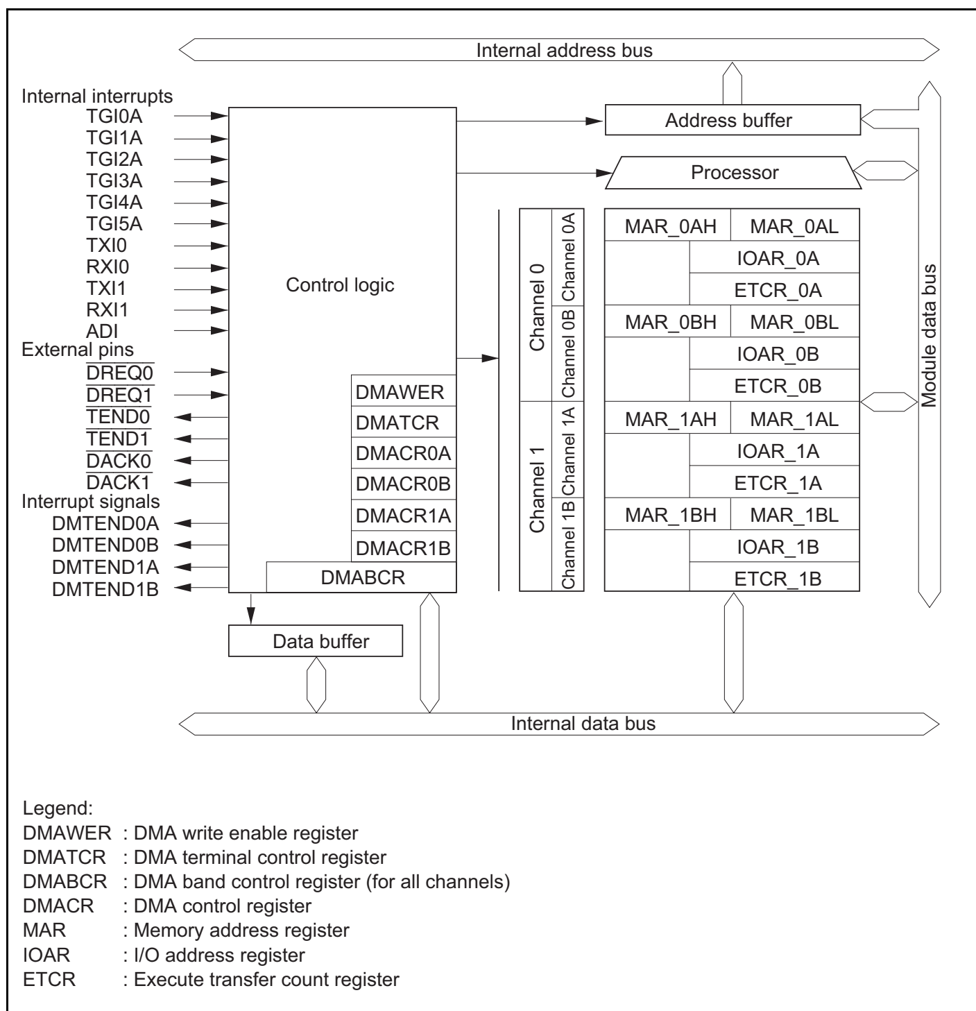
Figure 7.1 Block Diagram of DMAC
