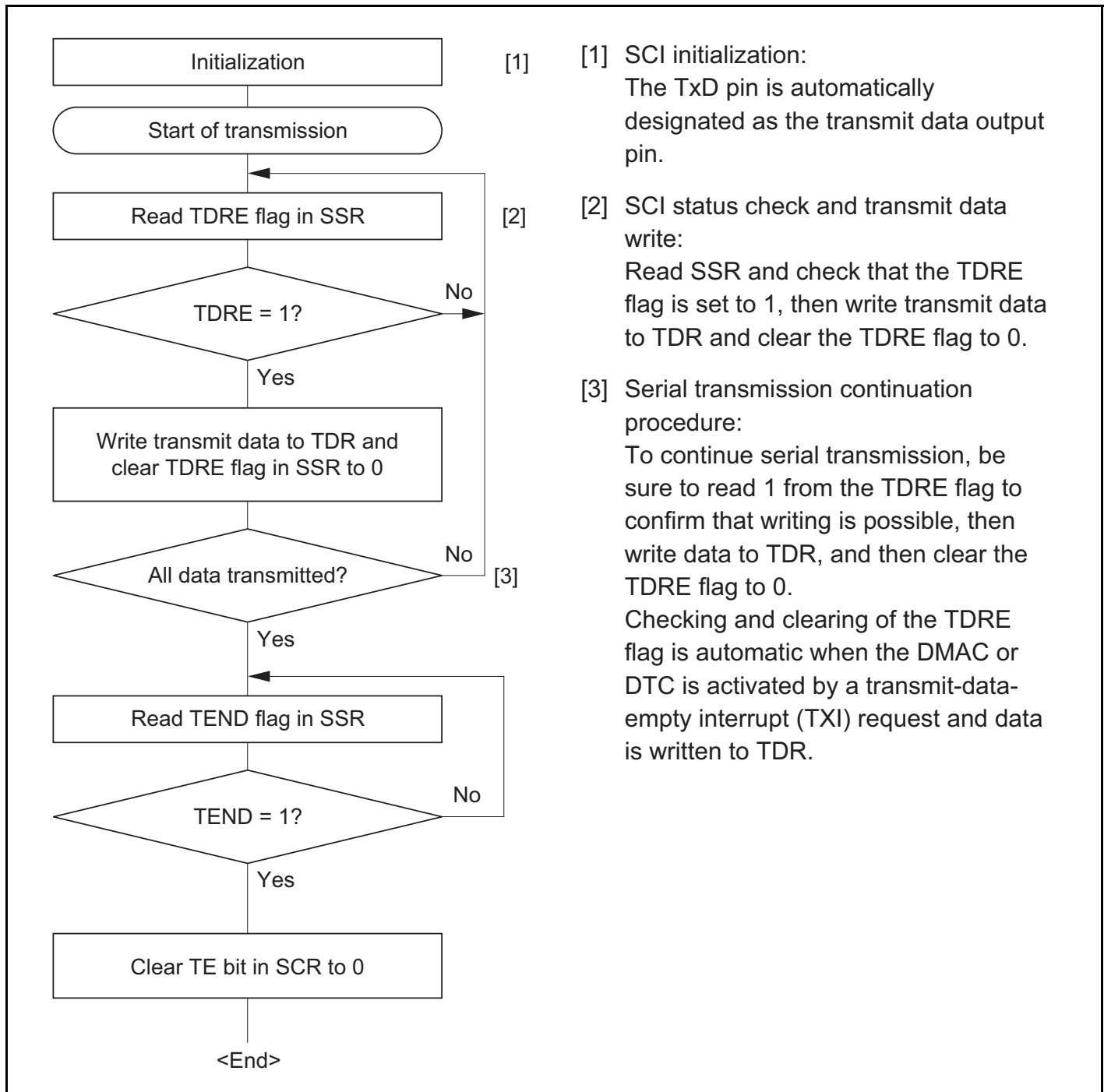
Figure 15.17 Sample Serial Transmission Flowchart
