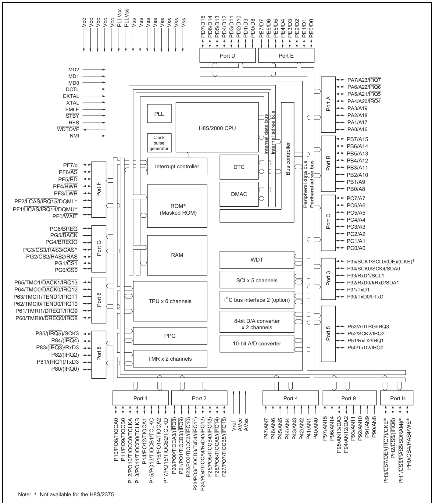
Figure 1.3 Internal Block Diagram for H8S/2375 and H8S/2375R
