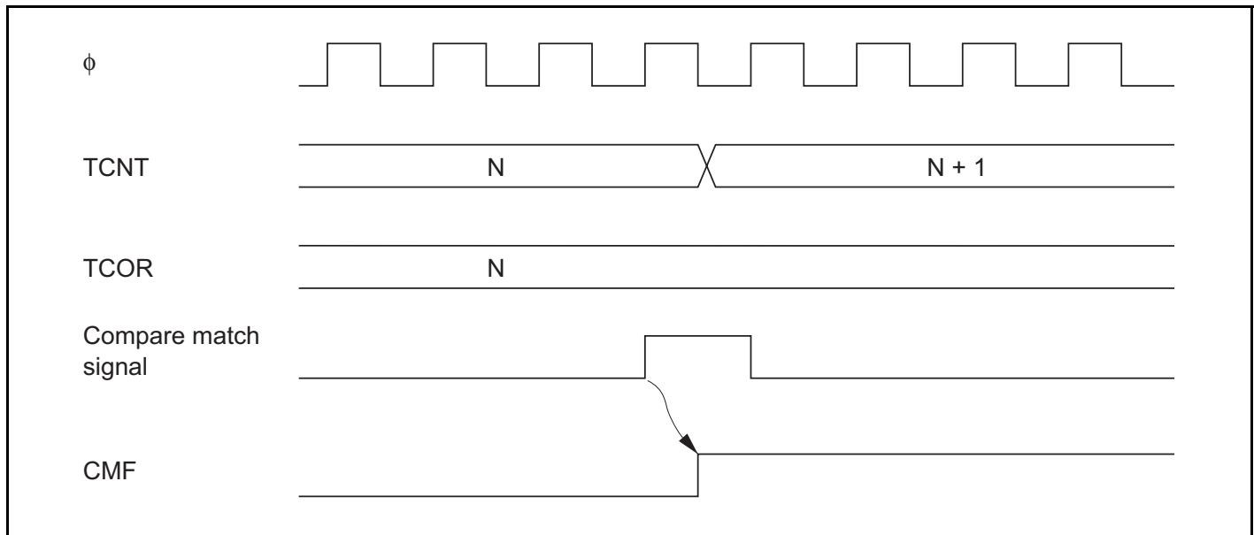
Figure 13.5 Timing of CMF Setting
