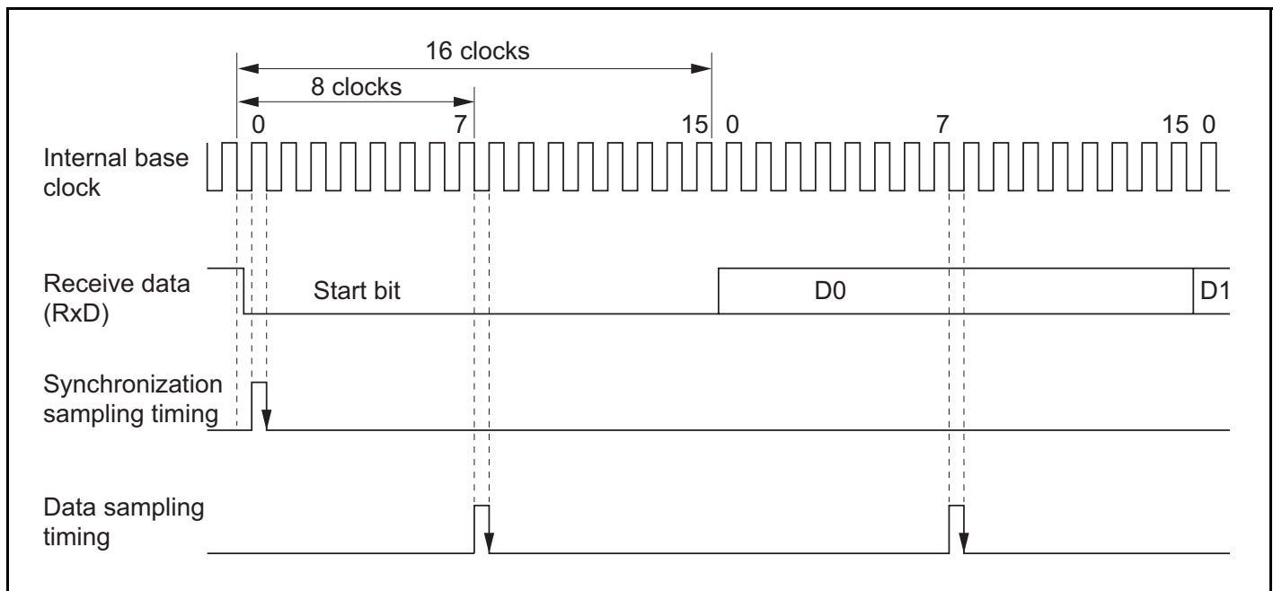
Figure 15.3 Receive Data Sampling Timing in Asynchronous Mode
