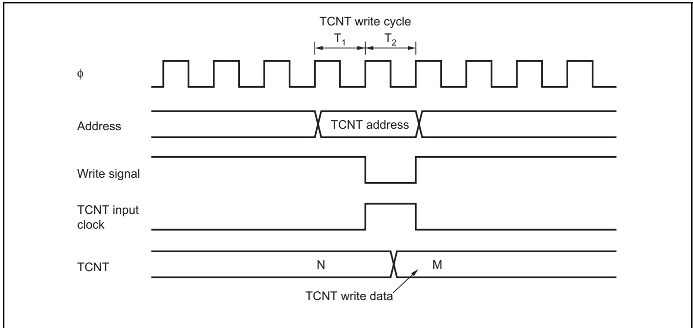
Figure 11.46 Contention between TCNT Write and Increment Operations
