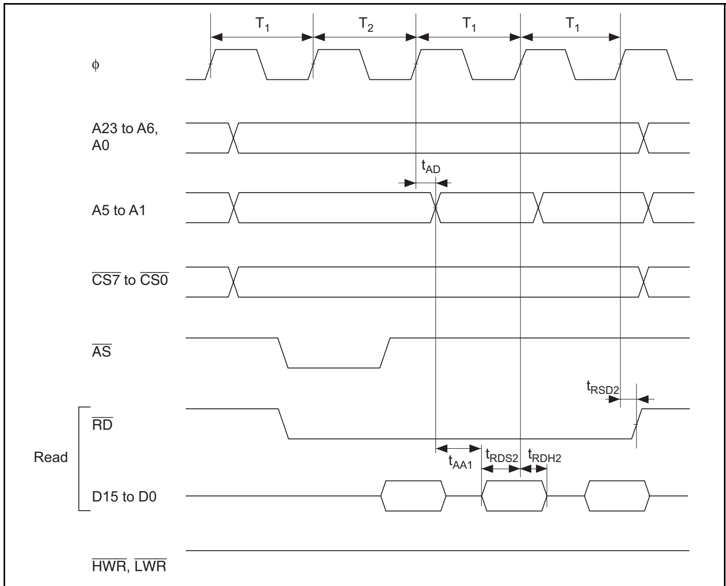
Figure 26.12 Burst ROM Access Timing: One-State Burst Access
