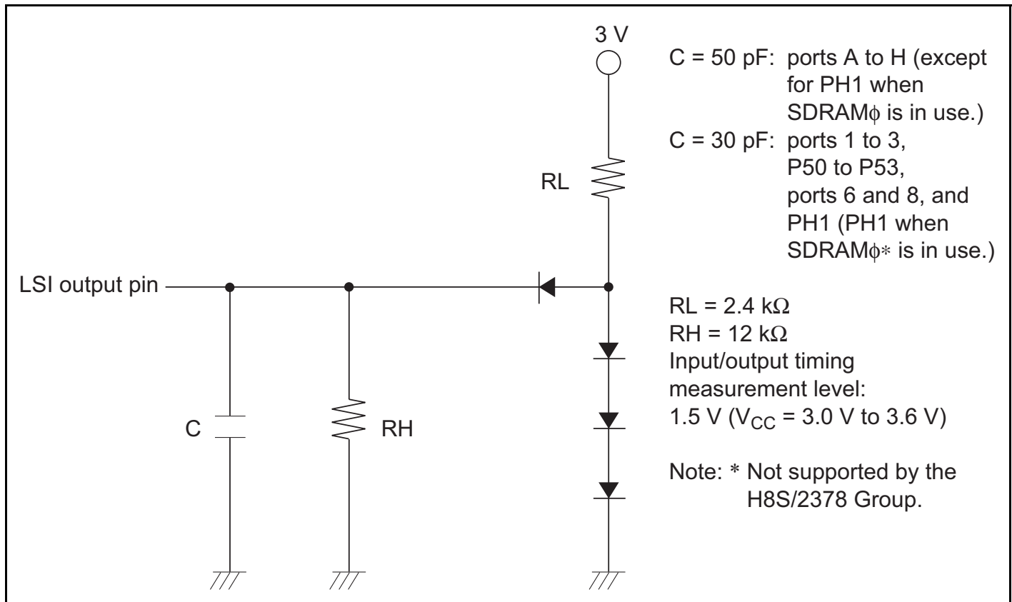
Figure 26.1 Output Load Circuit
