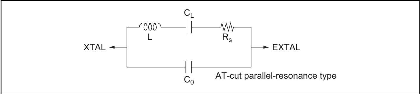
Figure 23.3 Crystal Resonator Equivalent Circuit
