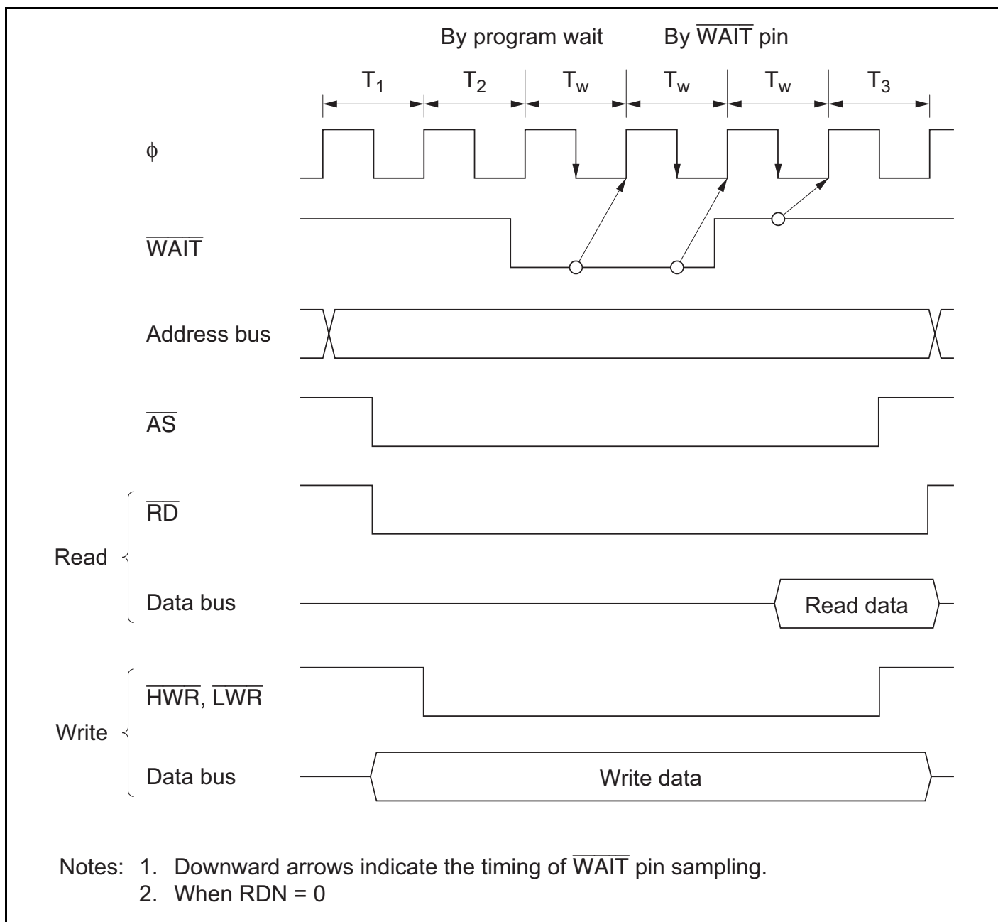
Figure 6.18 Example of Wait State Insertion Timing
