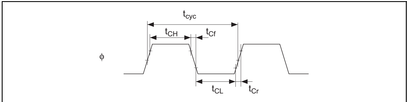
Figure 26.2 System Clock Timing
