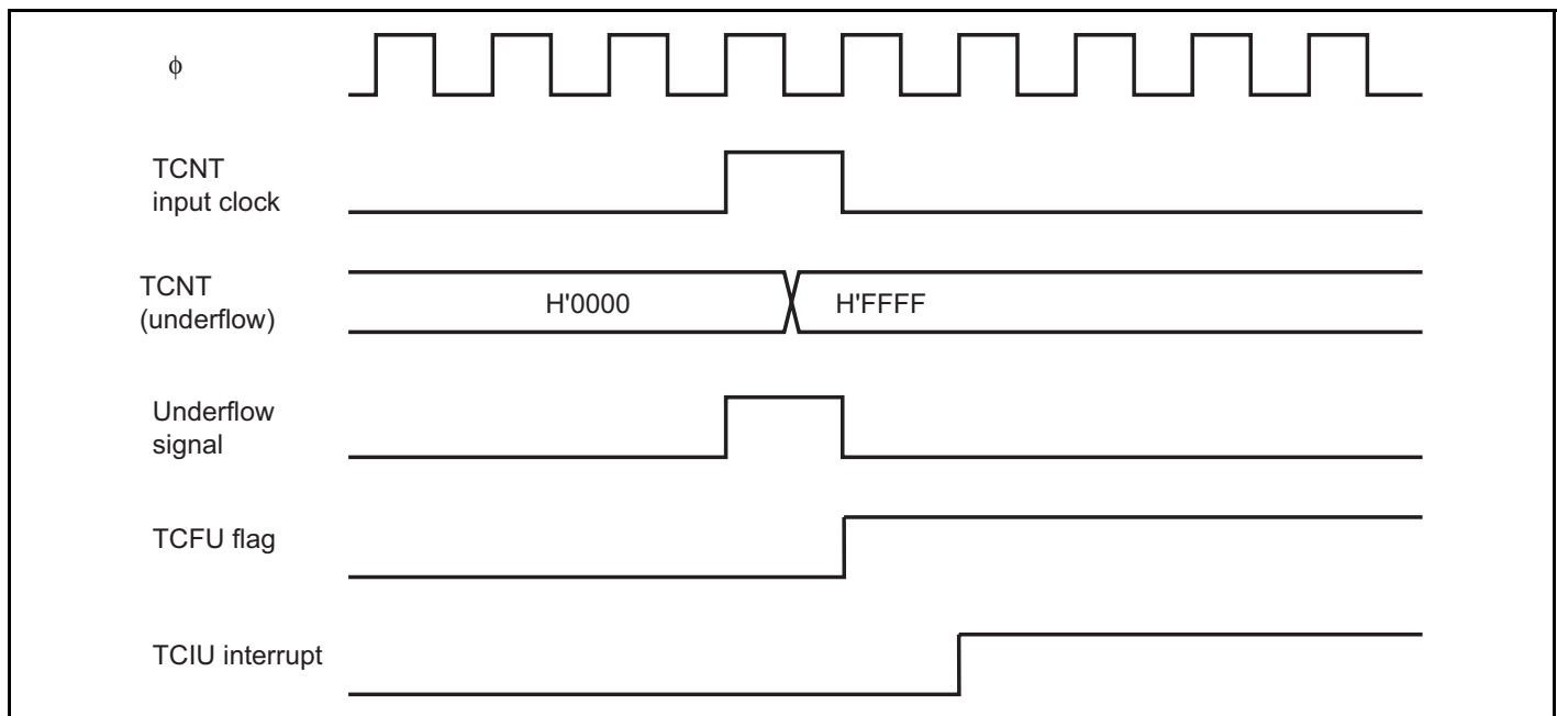
Figure 11.41 TCIU Interrupt Setting Timing
