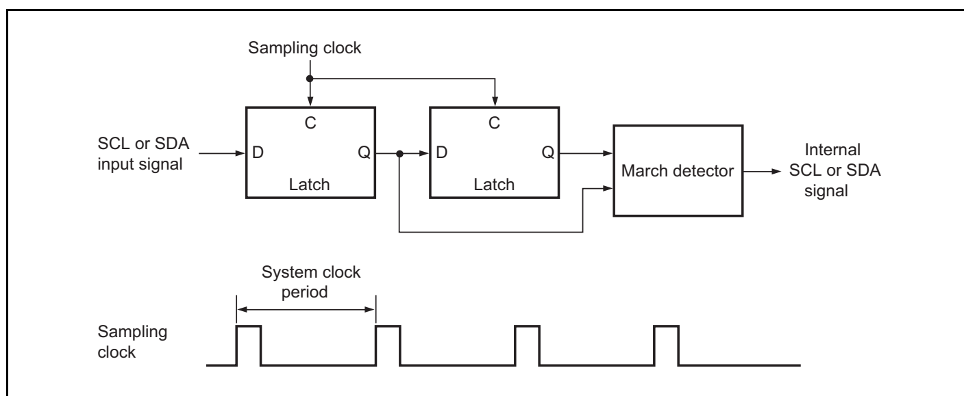
Figure 16.13 Block Diagram of Noise Canceler
