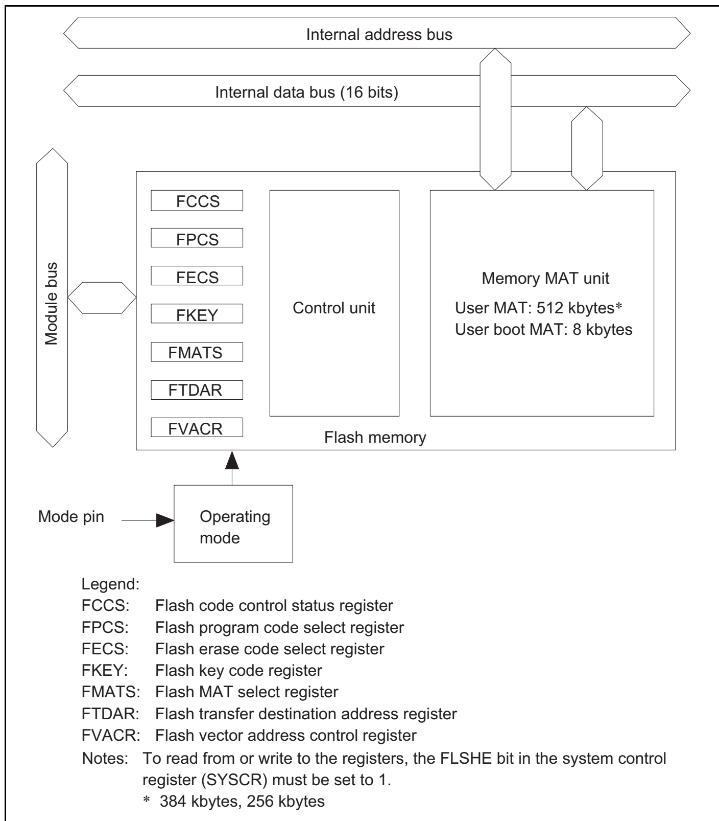
Figure 21.1 Block Diagram of Flash Memory
