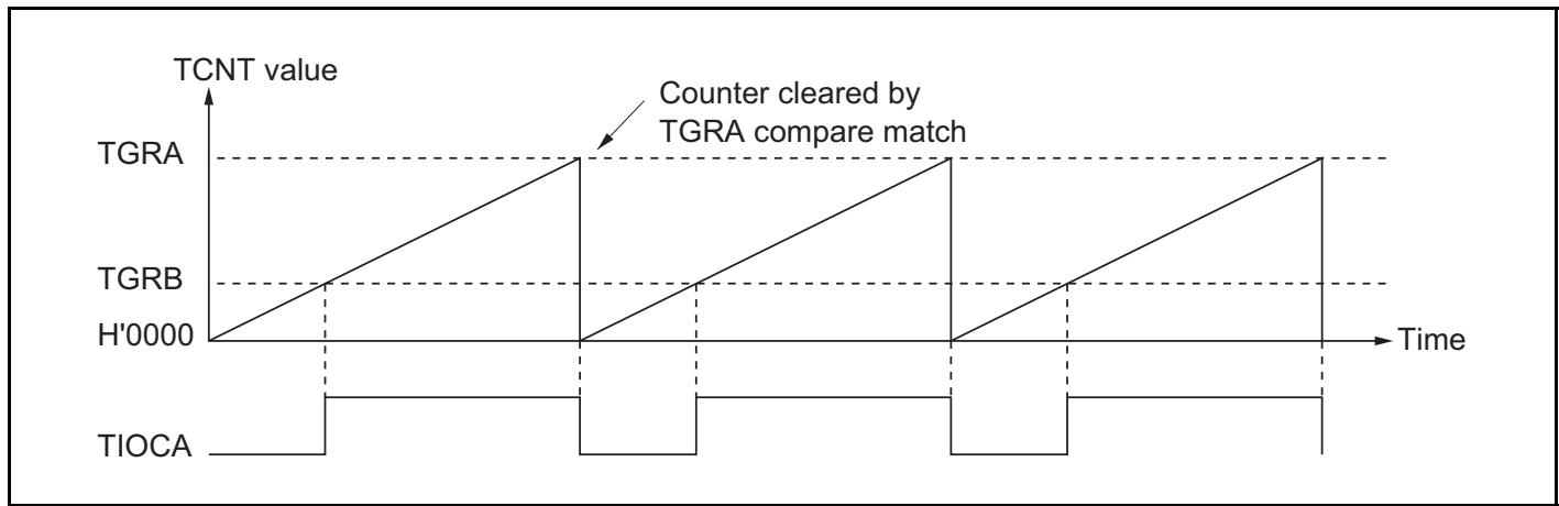
Figure 11.21 Example of PWM Mode Operation (1)
