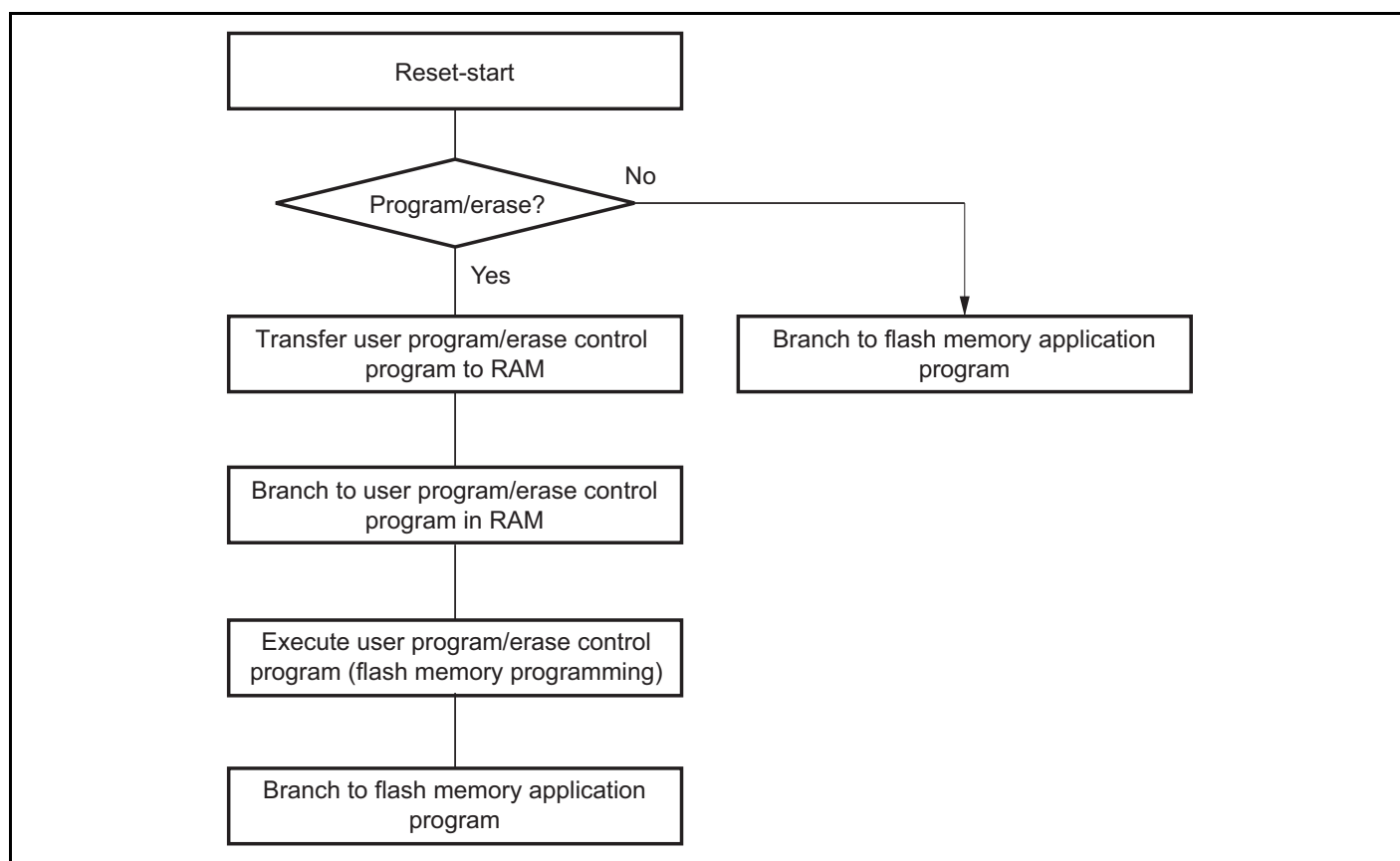
Figure 20.6 Programming/Erasing Flowchart Example in User Program Mode
