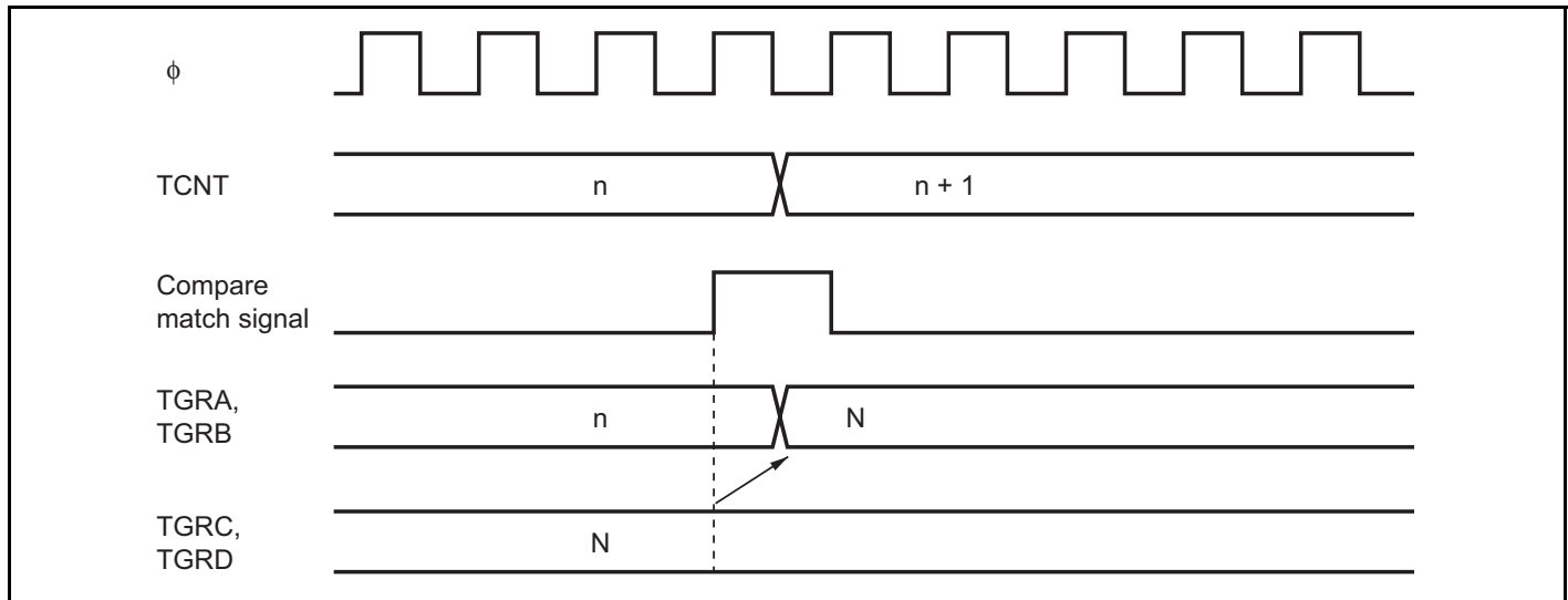
Figure 11.36 Buffer Operation Timing (Compare Match)
