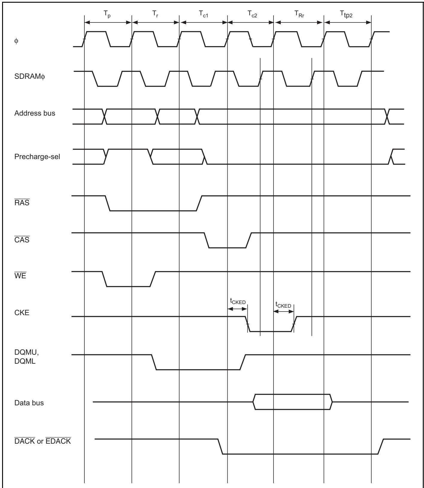
Figure 26.27 Read Data: Two-State Expansion (CAS Latency 2)
