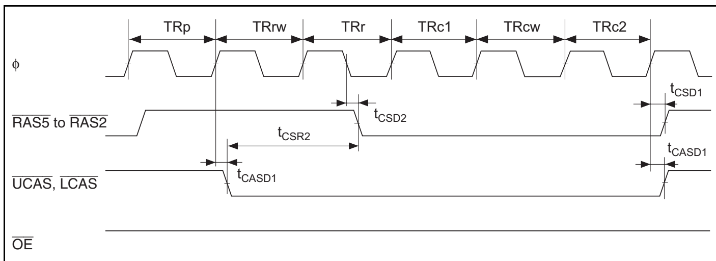
Figure 26.20 CAS-Before-RAS Refresh Timing (with Wait Cycle Insertion)
