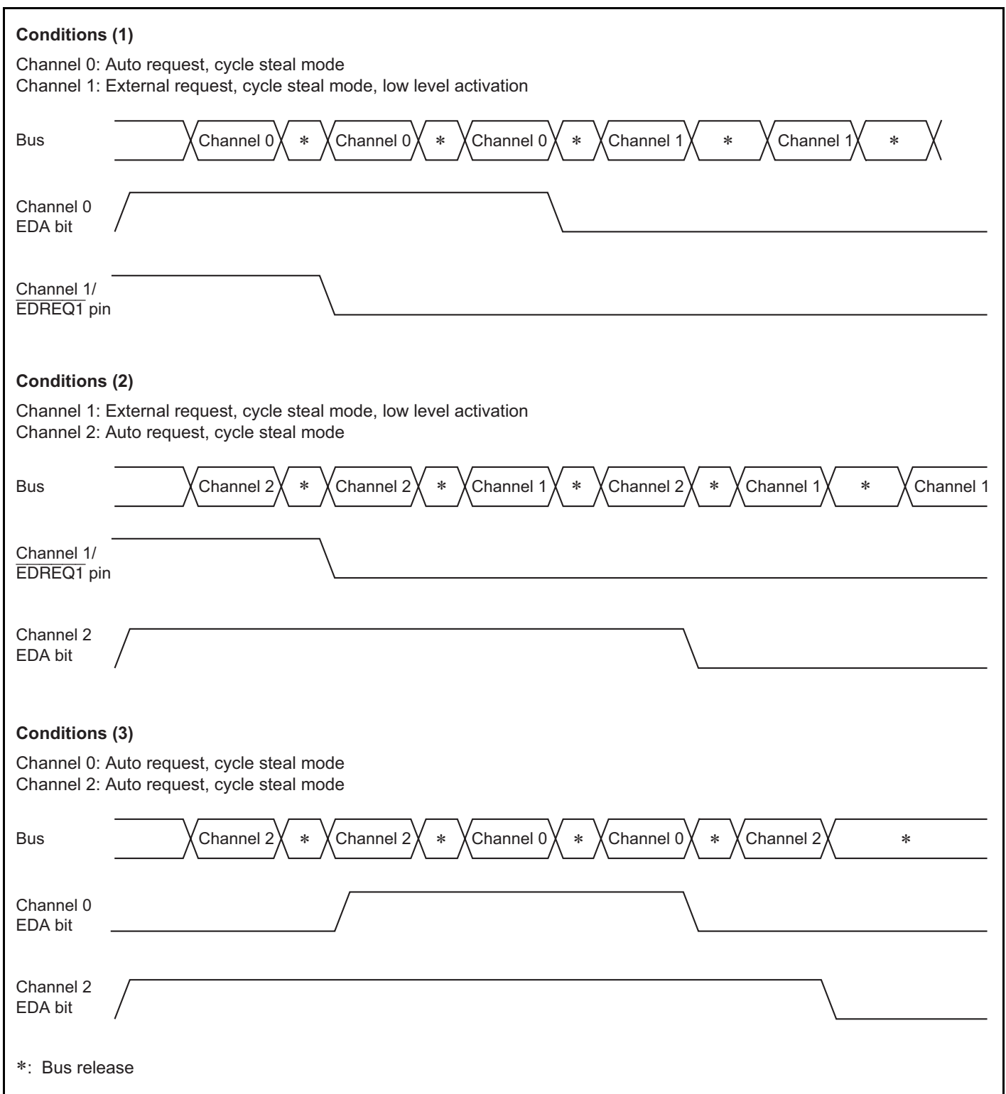
Figure 8.14 Examples of Channel Priority Timing
