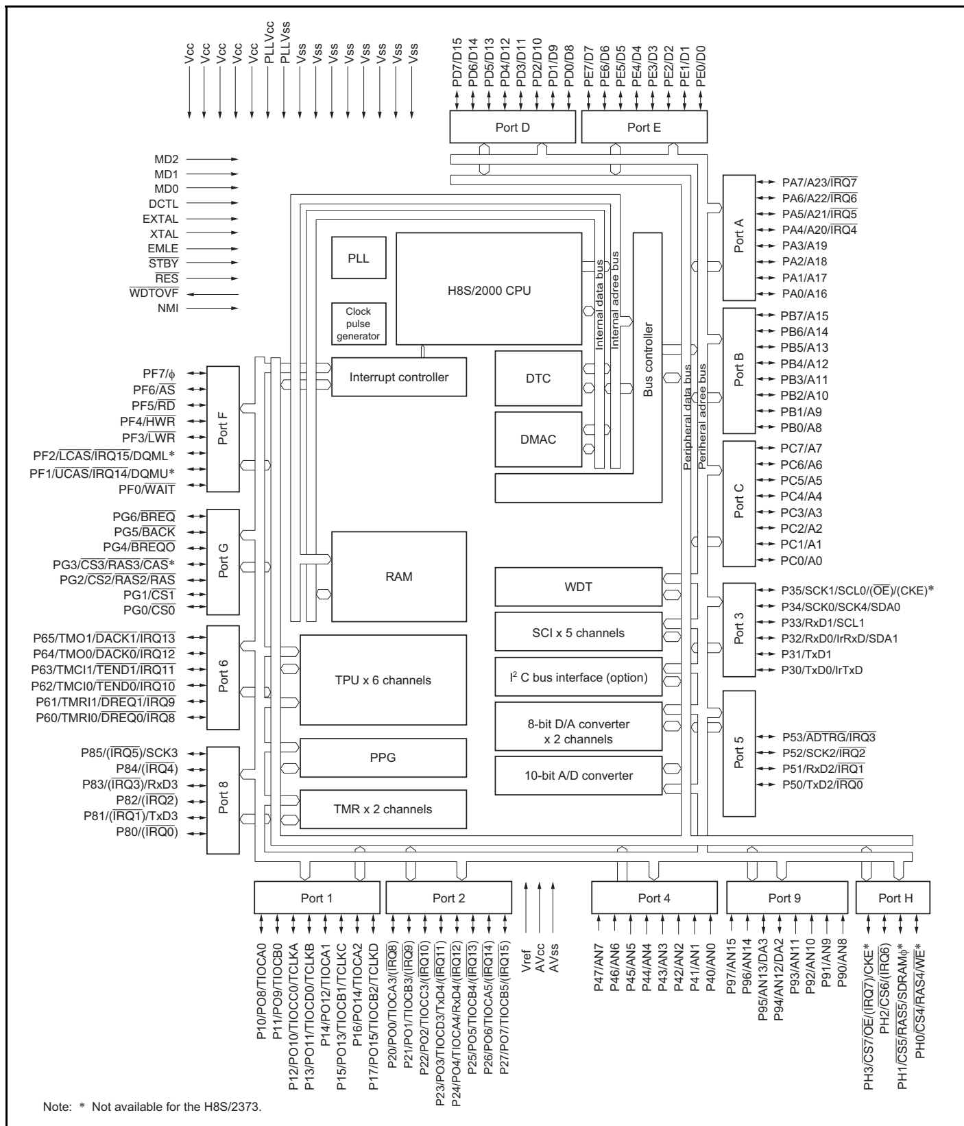
Figure 1.4 Internal Block Diagram for H8S/2373 and H8S/2373R
