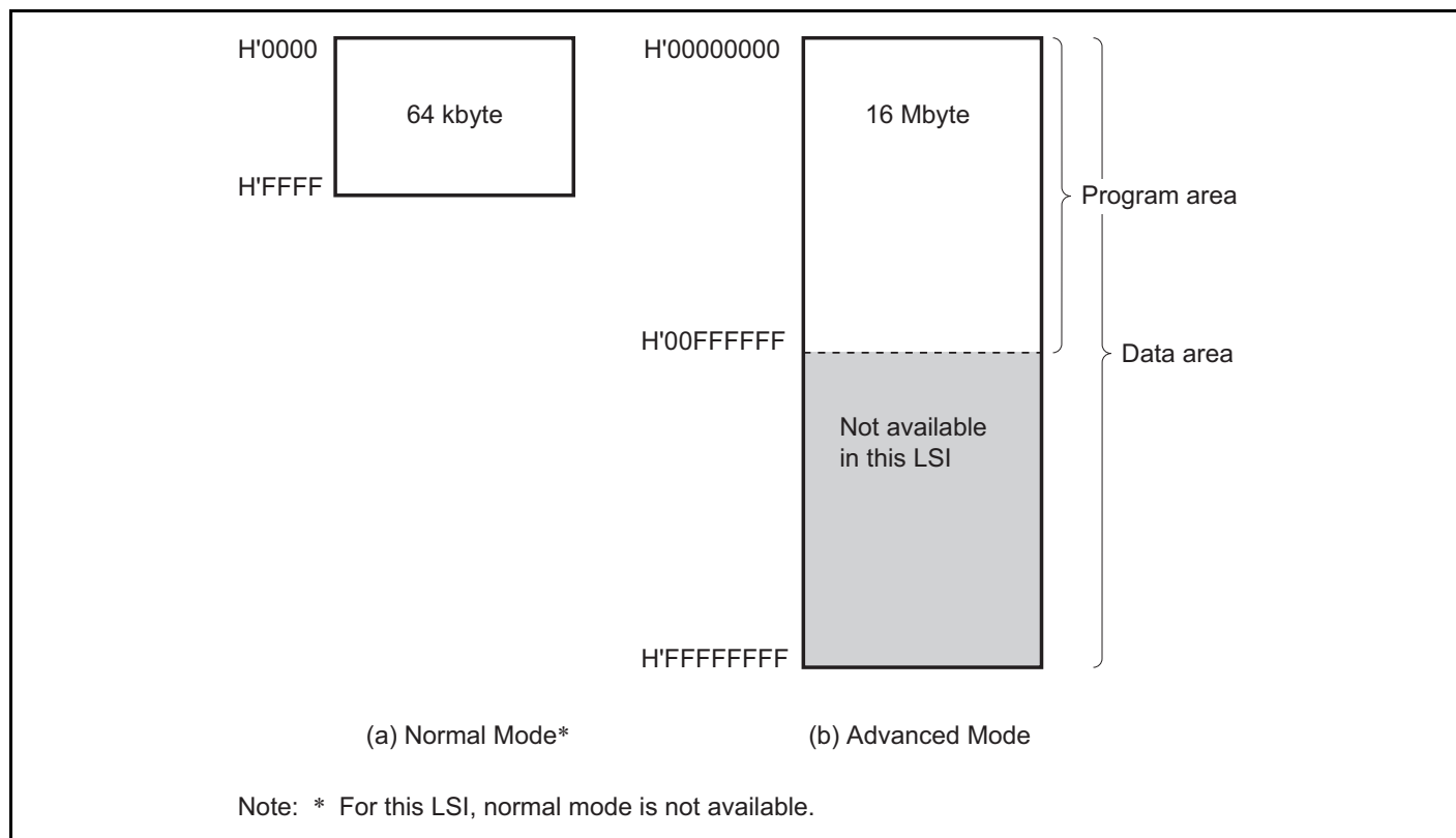
Figure 2.5 Memory Map
