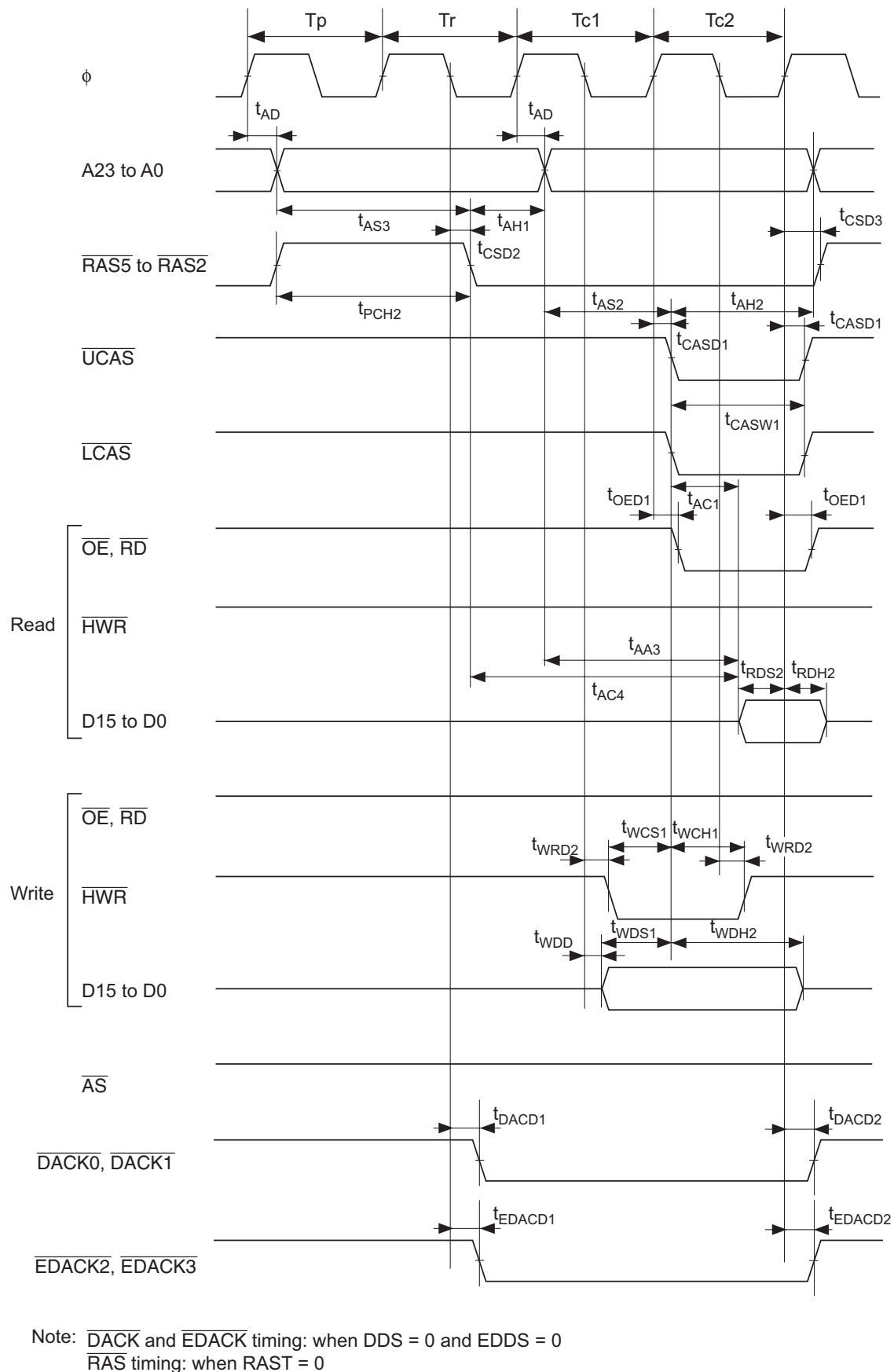
Figure 26.14 DRAM Access Timing: Two-State Access
