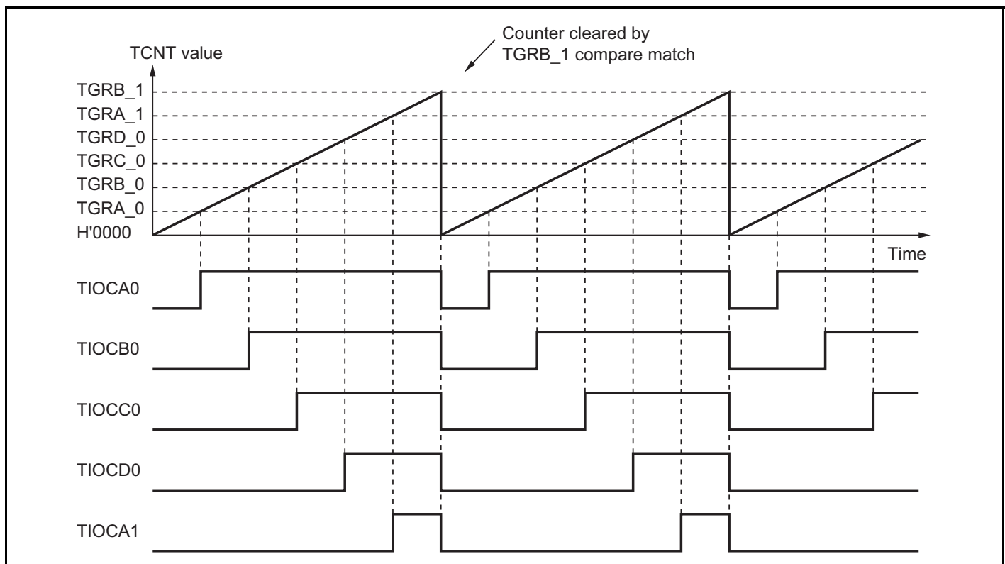
Figure 11.22 Example of PWM Mode Operation (2)
