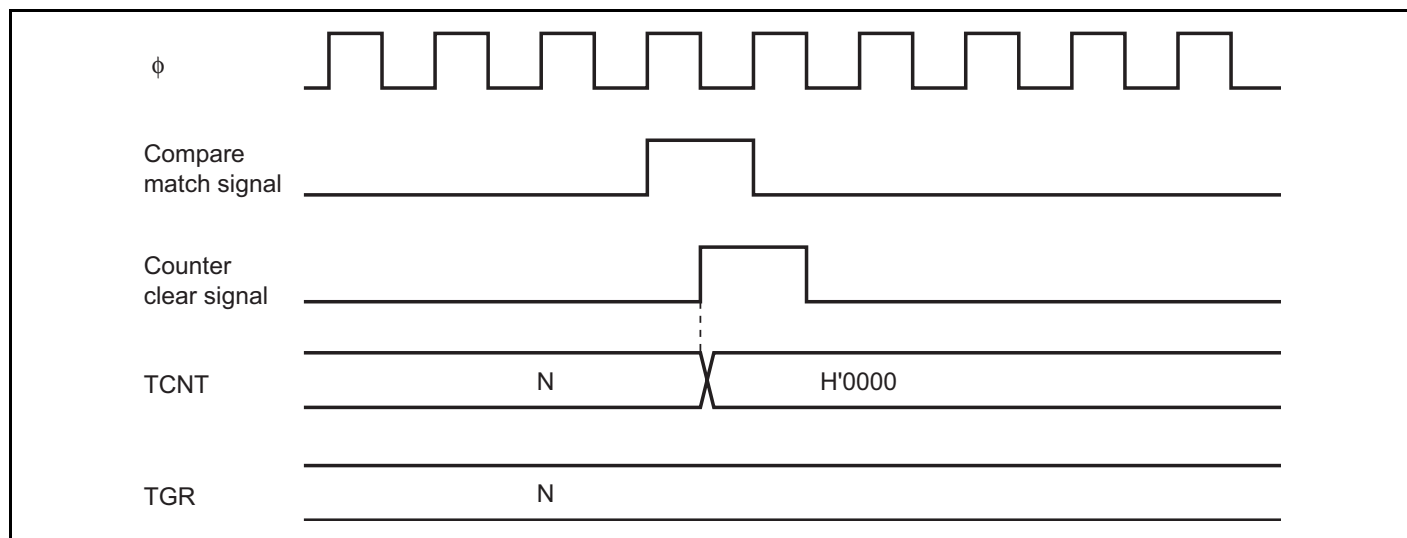
Figure 11.34 Counter Clear Timing (Compare Match)
