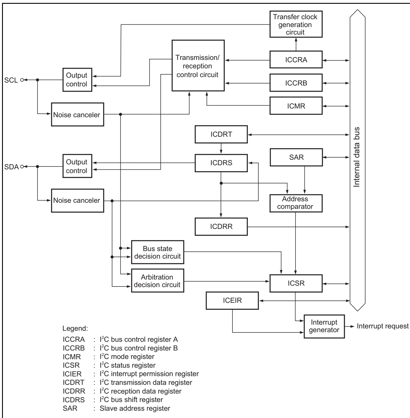
Figure 16.1 Block Diagram of I 2 C Bus Interface 2
