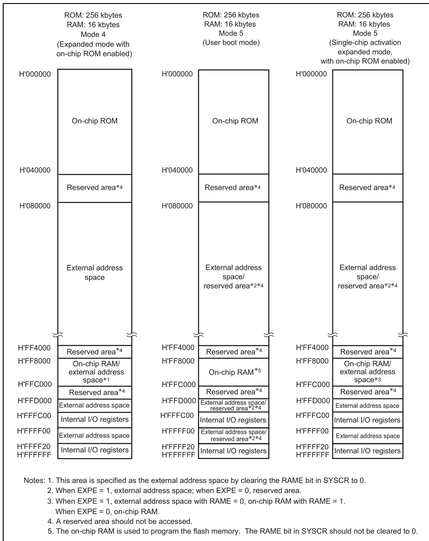
Figure 3.15 Memory Map for H8S/2370 and H8S/2370R (2)
