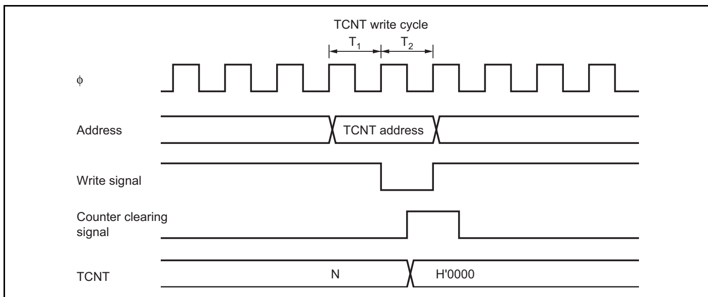
Figure 11.45 Contention between TCNT Write and Clear Operations
