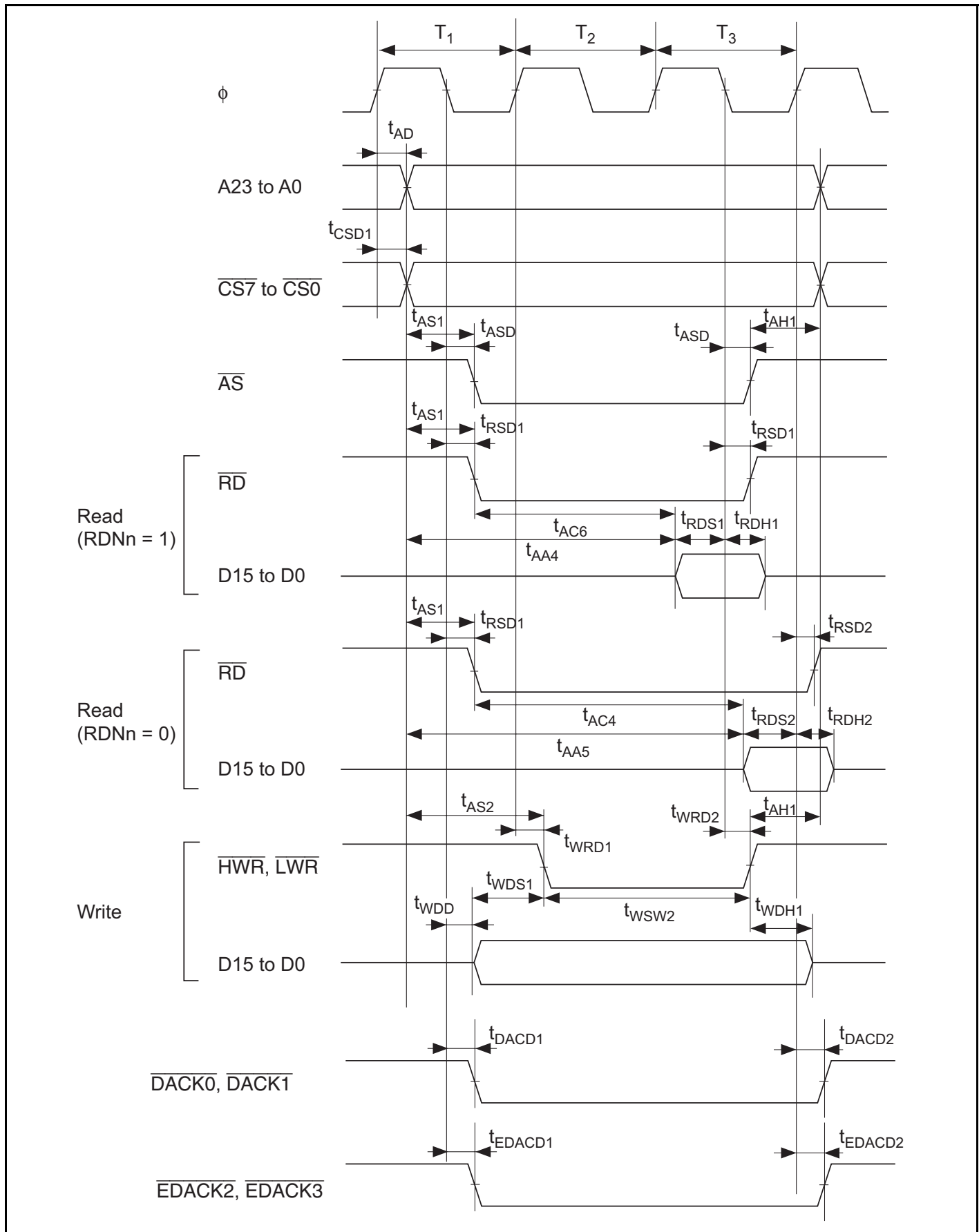
Figure 26.8 Basic Bus Timing: Three-State Access
