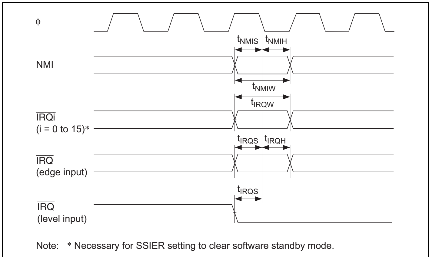
Figure 26.6 Interrupt Input Timing
