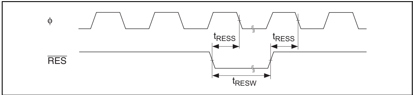
Figure 26.5 Reset Input Timing
