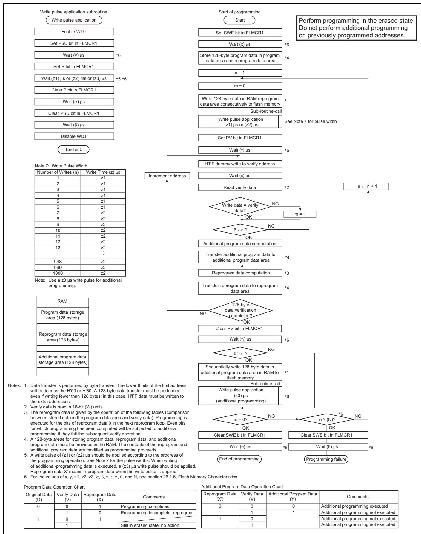
Figure 20.7 Program/Program-Verify Flowchart
