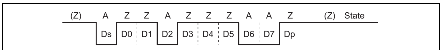
Figure 15.23 Direct Convention (SDIR = SINV = O/E = 0)
