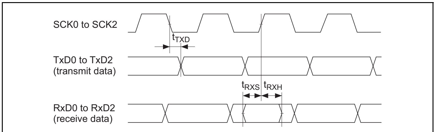
Figure 26.42 SCI Input/Output Timing: Synchronous Mode
