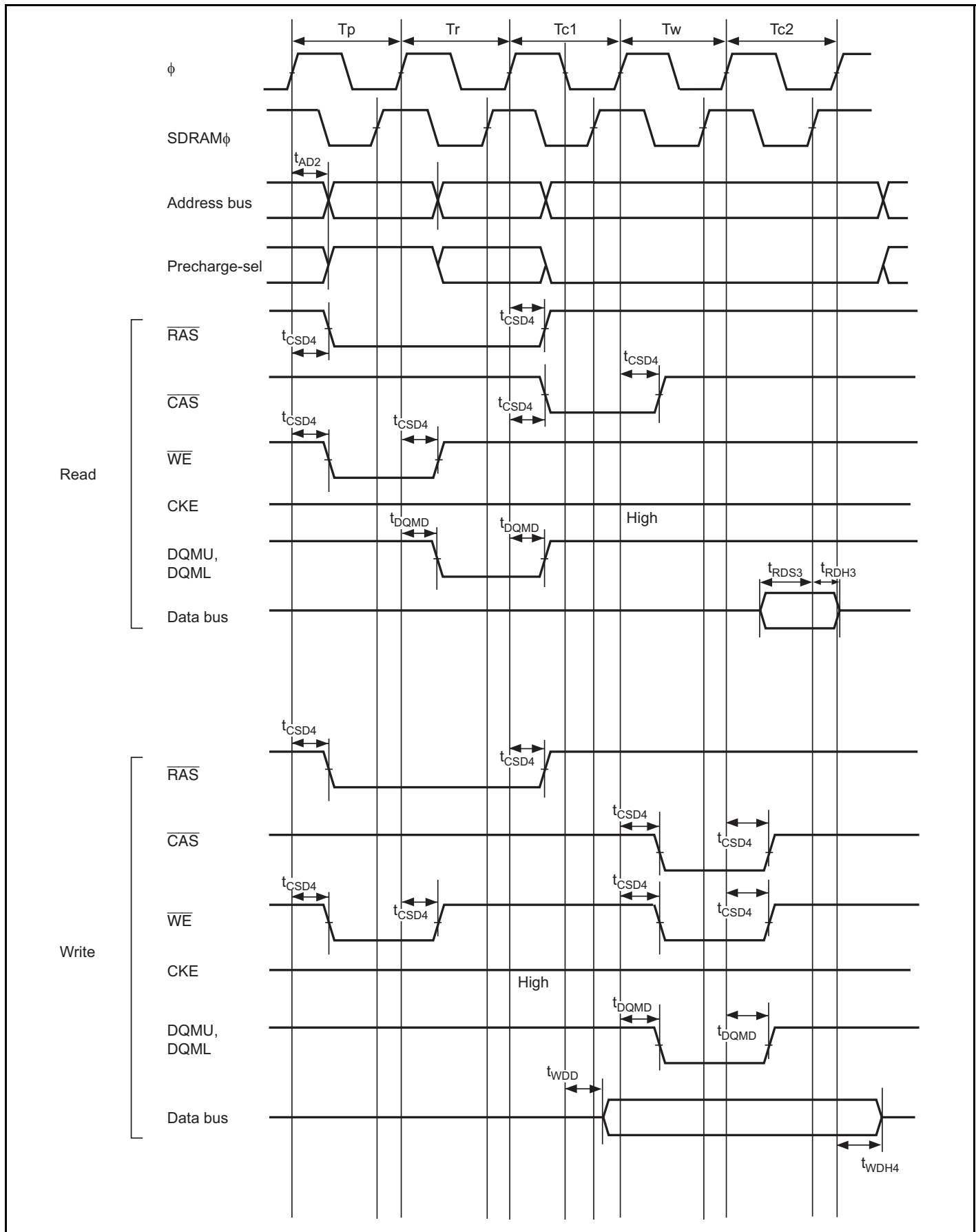
Figure 26.25 Synchronous DRAM Basic Access Timing (CAS Latency 2)
