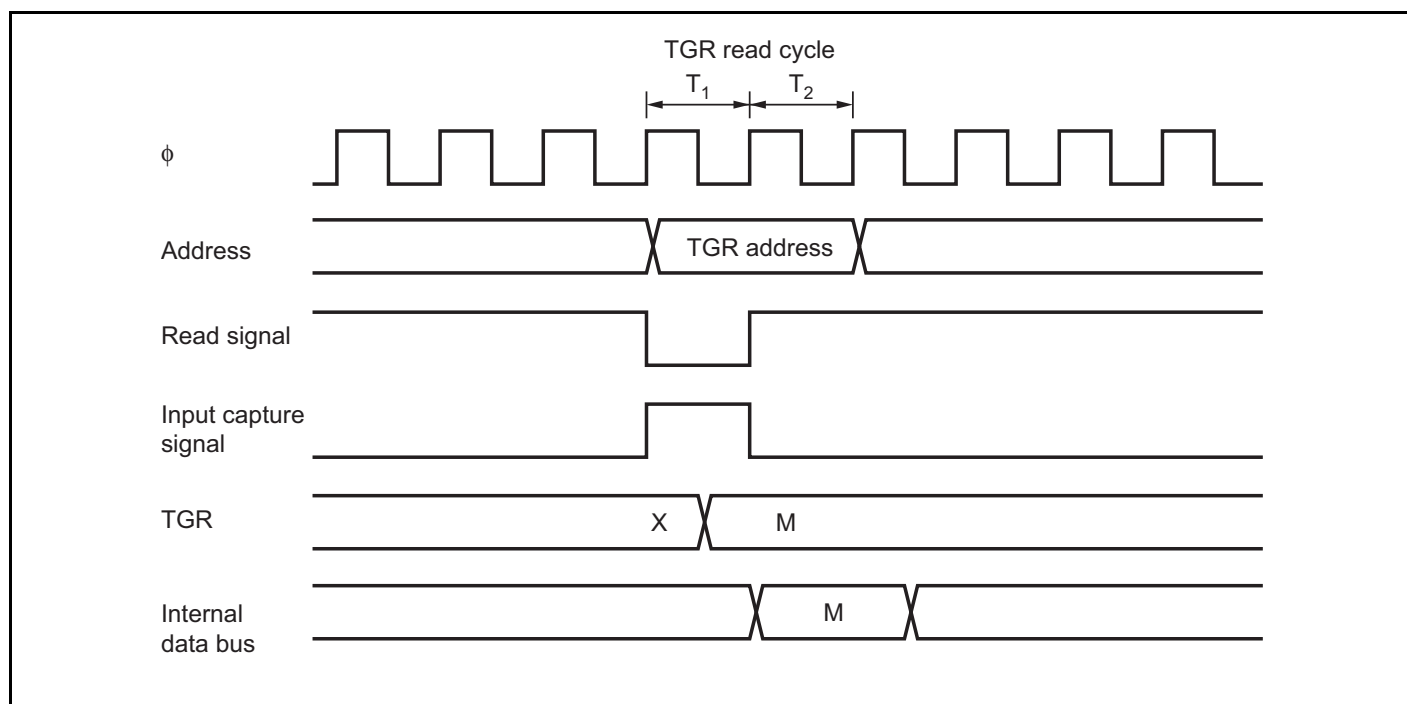
Figure 11.49 Contention between TGR Read and Input Capture
