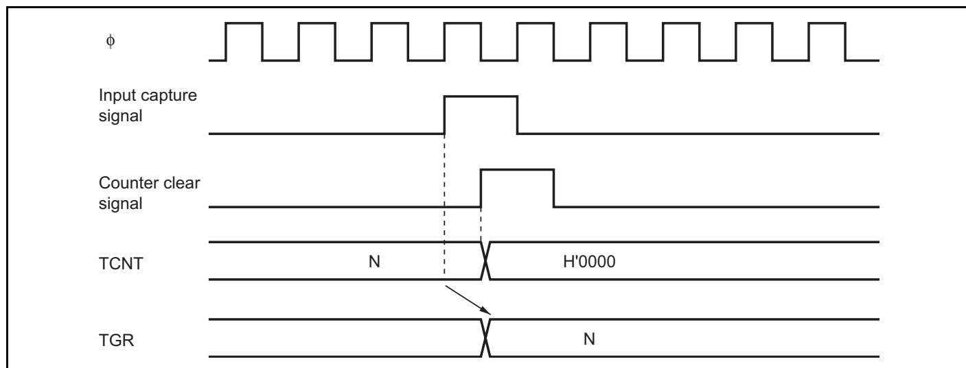
Figure 11.35 Counter Clear Timing (Input Capture)
