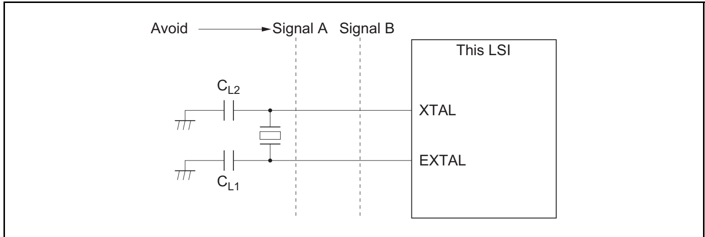
Figure 23.6 Note on Board Design for Oscillation Circuit
