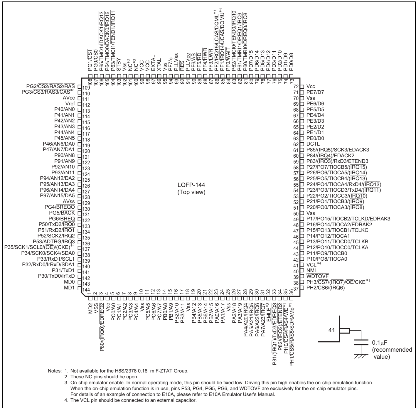
Figure 1.5 Pin Arrangement for H8S/2378 0.18 \mu m F-ZTAT Group and H8S/2378R 0.18 \mu m F-ZTAT Group
