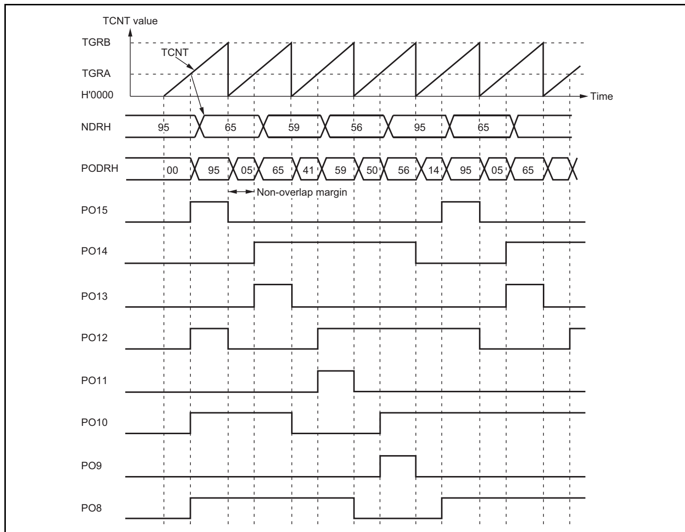
Figure 12.9 Non-Overlapping Pulse Output Example (Four-Phase Complementary)
