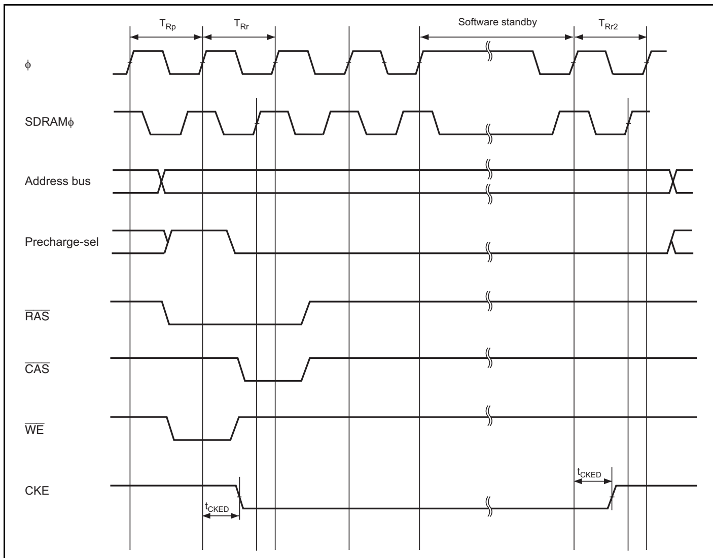
Figure 26.26 Synchronous DRAM Self-Refresh Timing
