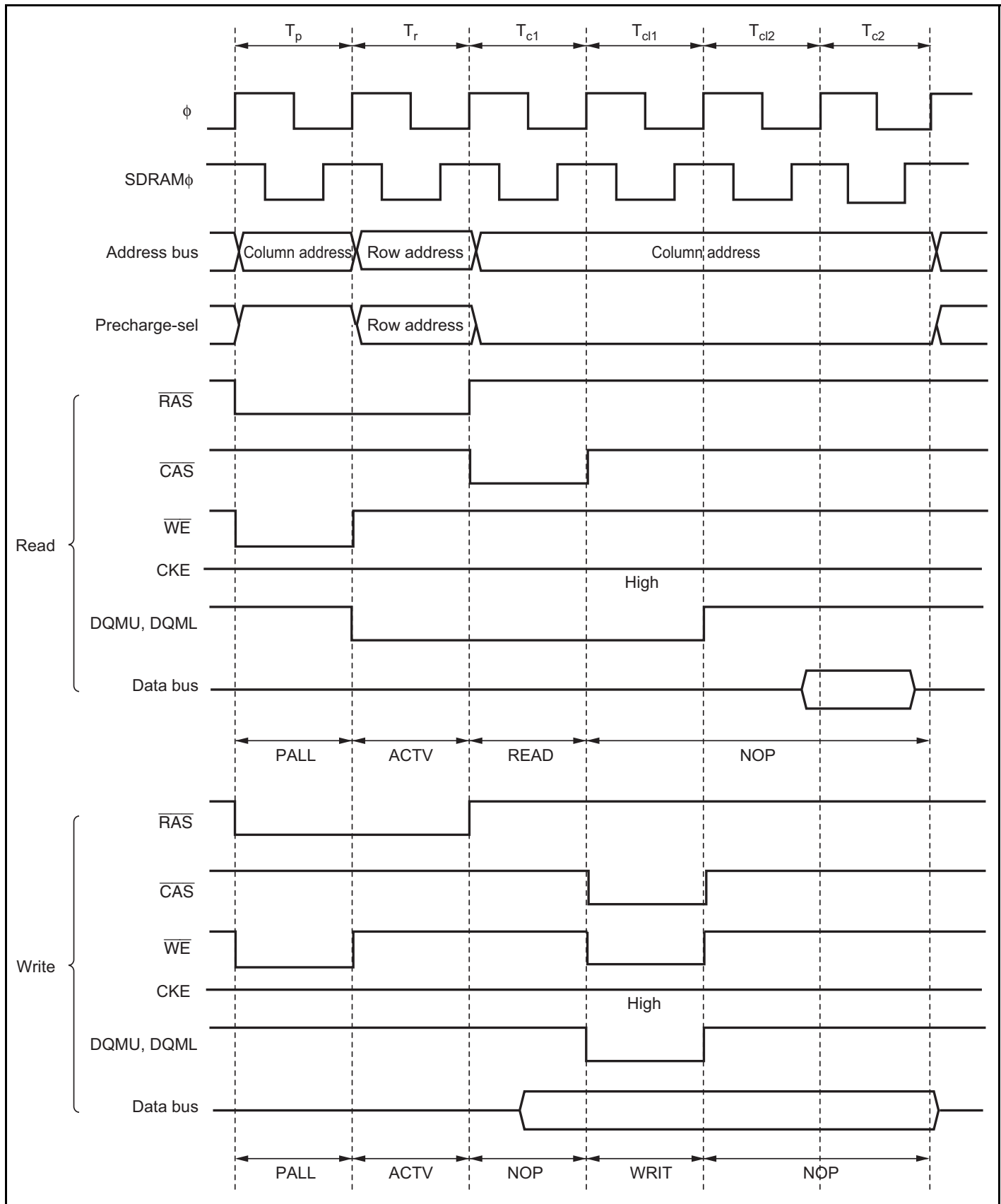
Figure 6.45 CAS Latency Control Timing (SDWCD = 0, CAS Latency 3)
