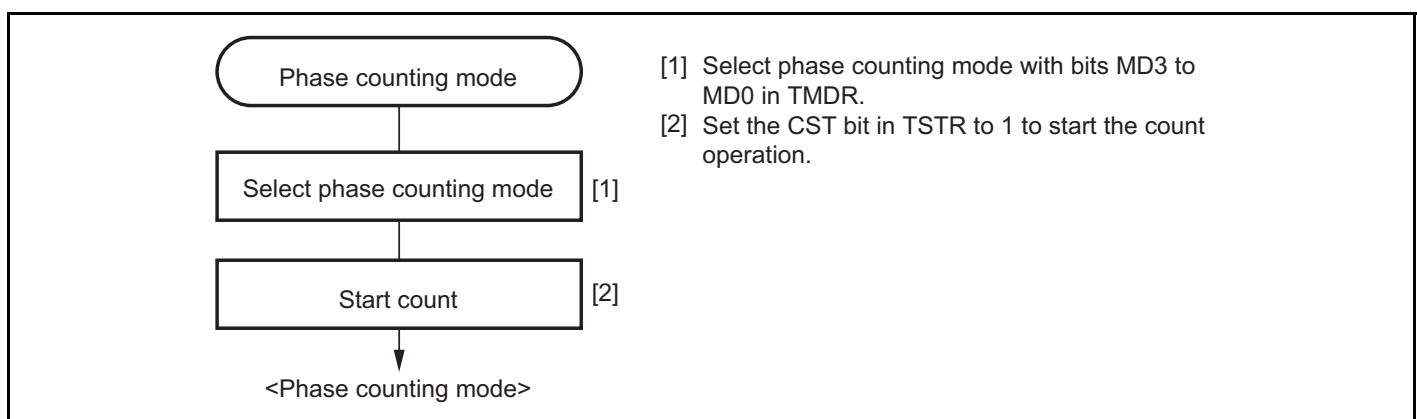
Figure 11.24 Example of Phase Counting Mode Setting Procedure
