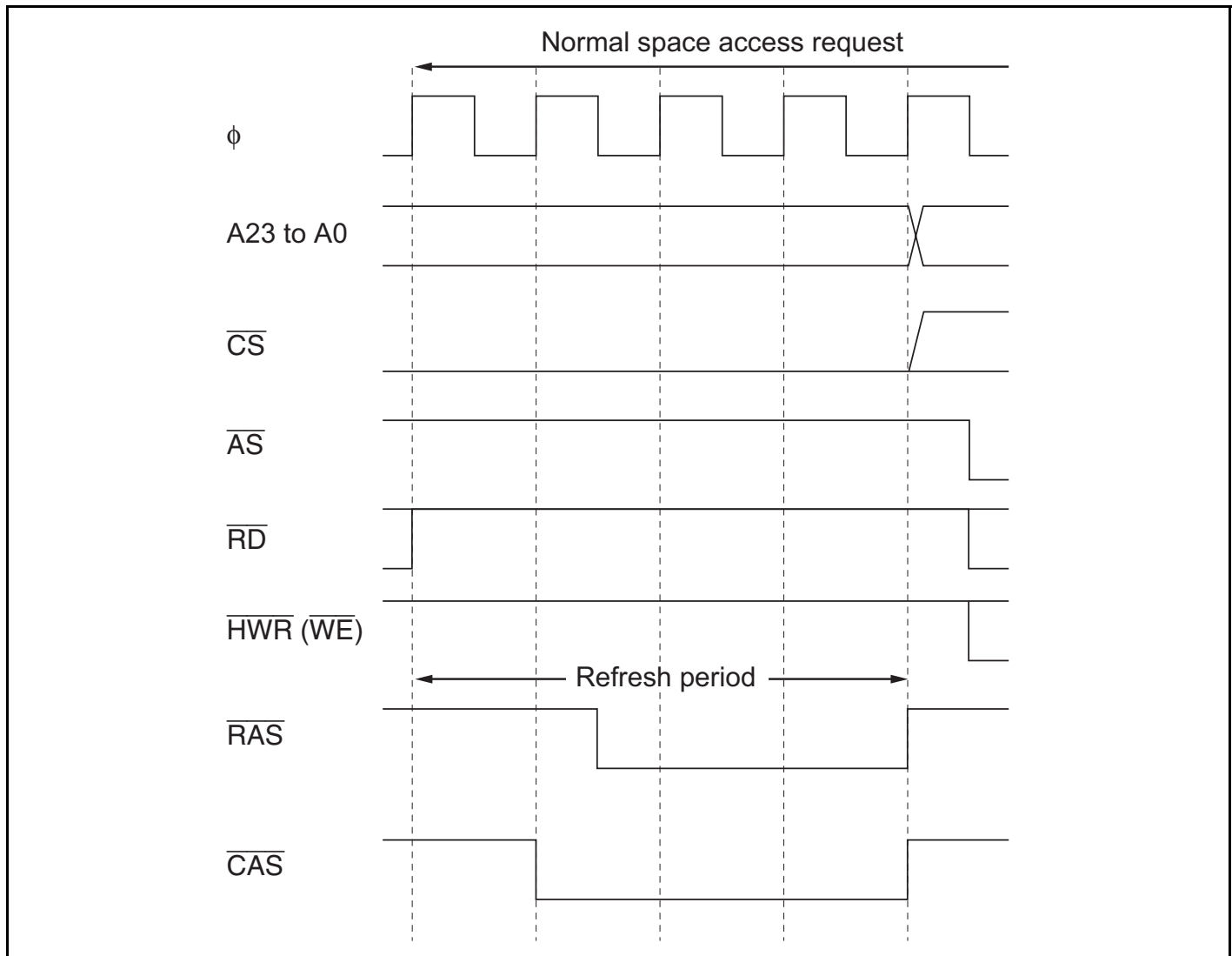
Figure 6.38 Example of CBR Refresh Timing (CBRM = 1)
