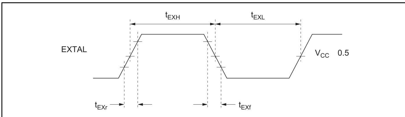
Figure 23.5 External Clock Input Timing
