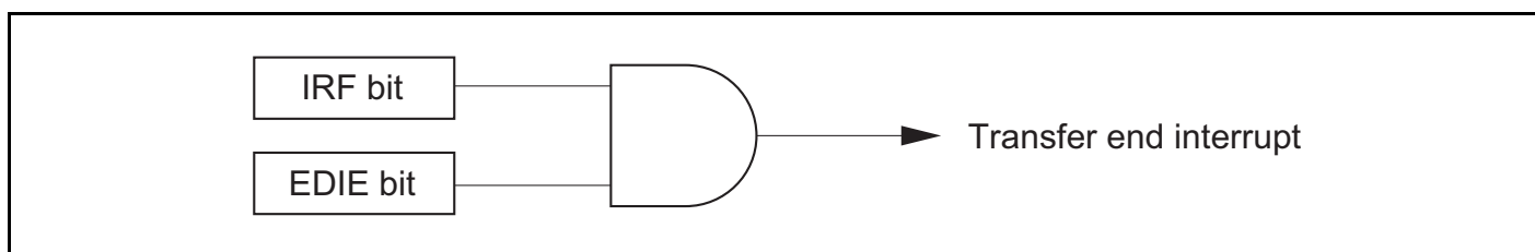
Figure 8.45 Transfer End Interrupt Logic
