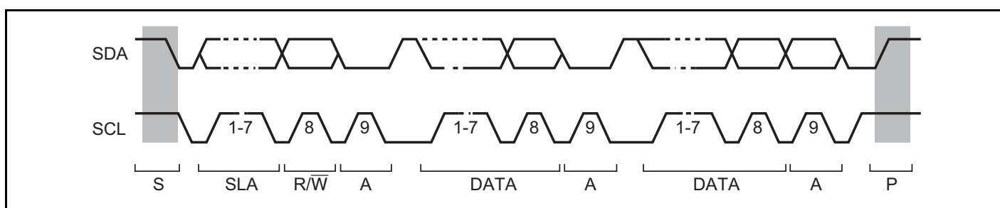
Figure 16.4 I 2 C Bus Timing
