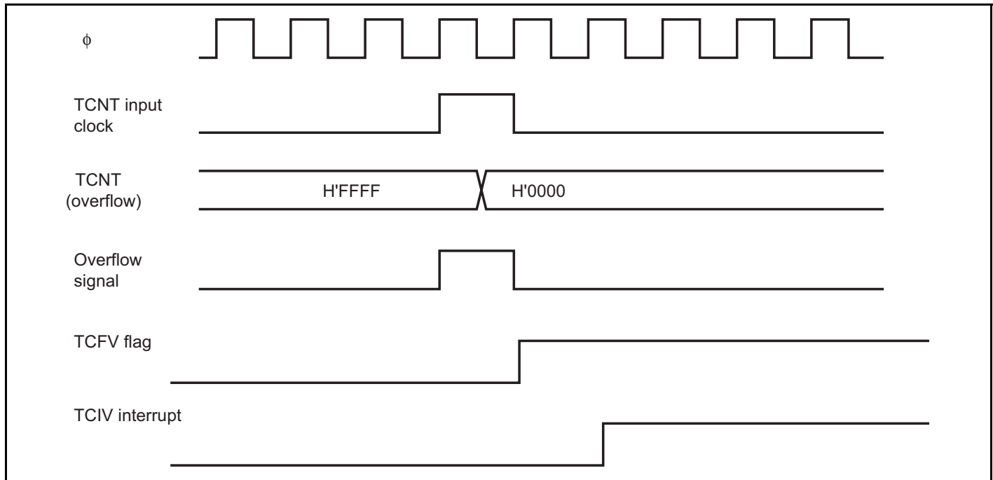
Figure 11.40 TCIV Interrupt Setting Timing
