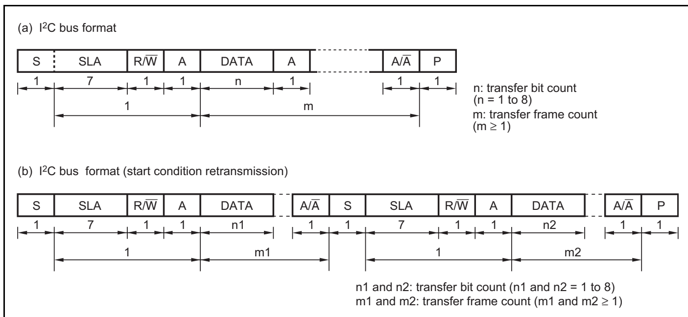
Figure 16.3 I 2 C Bus Formats
