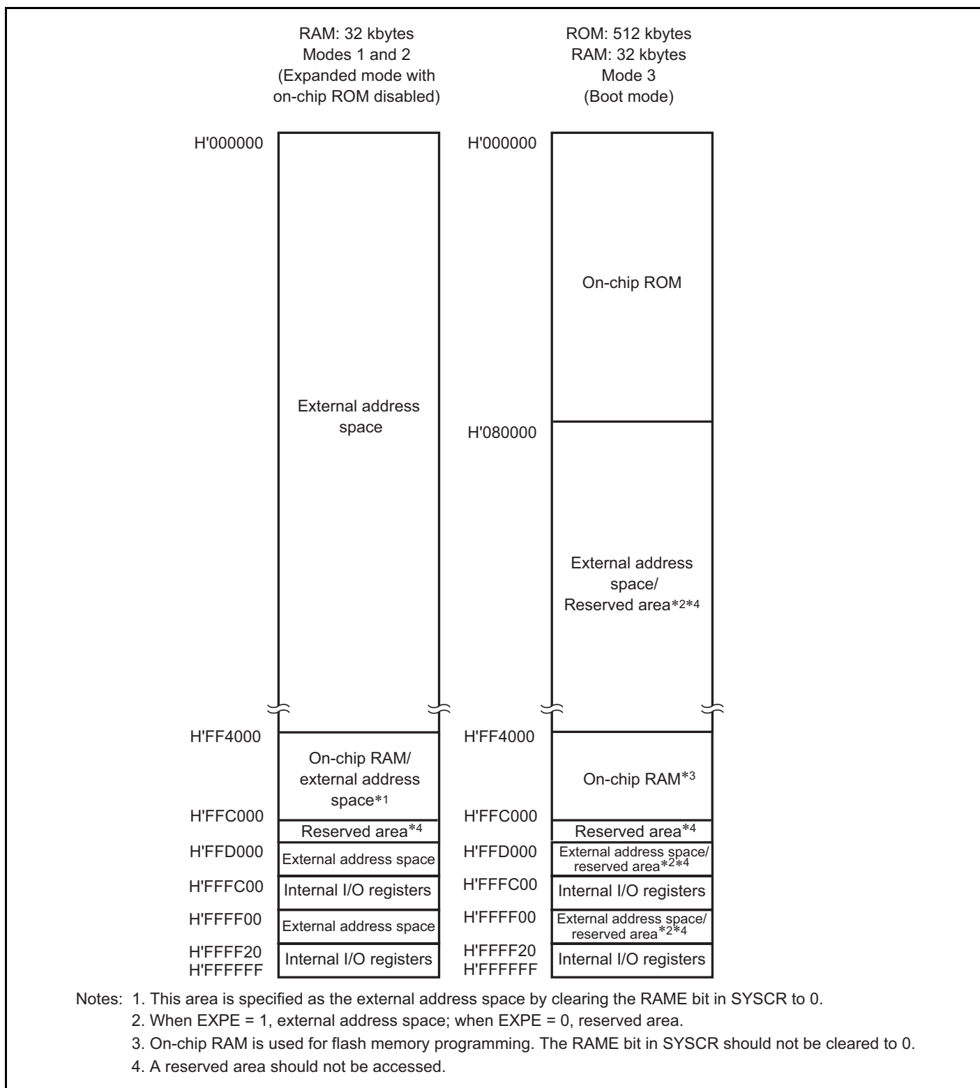
Figure 3.1 Memory Map for H8S/2378 and H8S/2378R (1)
