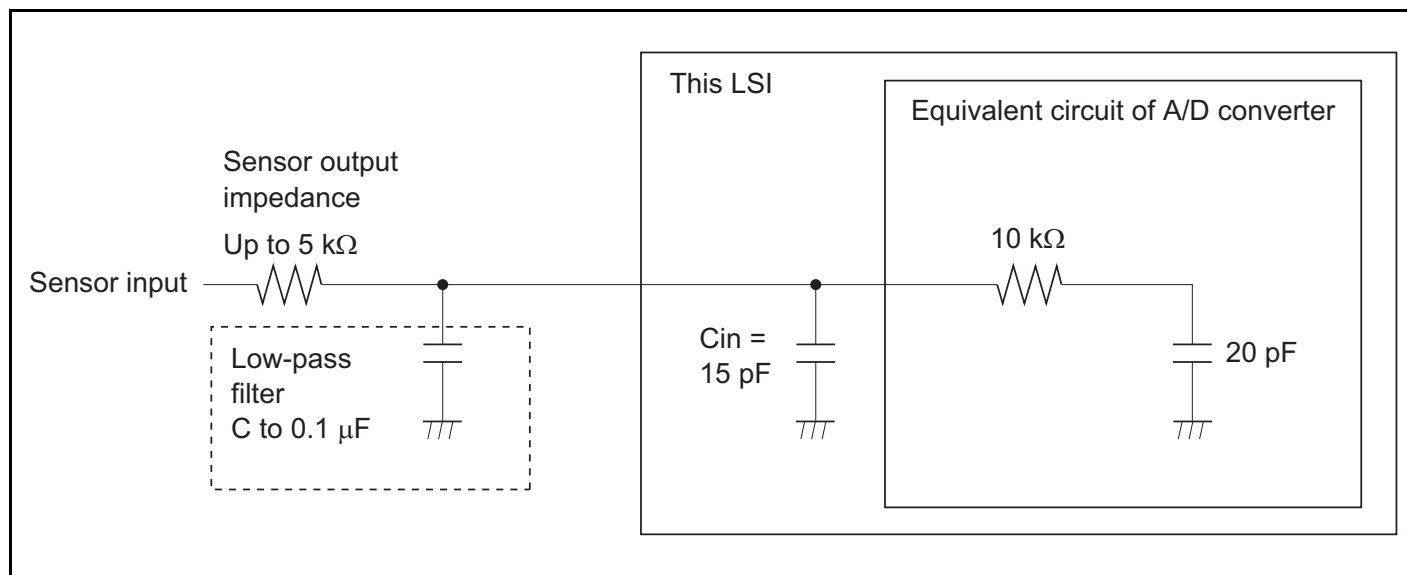
Figure 17.6 Example of Analog Input Circuit
