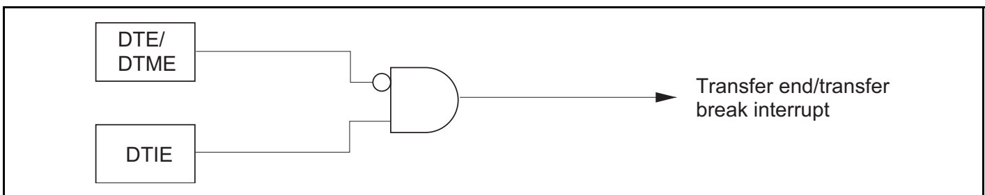
Figure 7.38 Block Diagram of Transfer End/Transfer Break Interrupt
