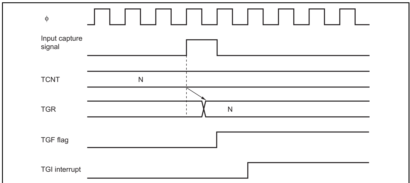
Figure 11.39 TGI Interrupt Timing (Input Capture)
