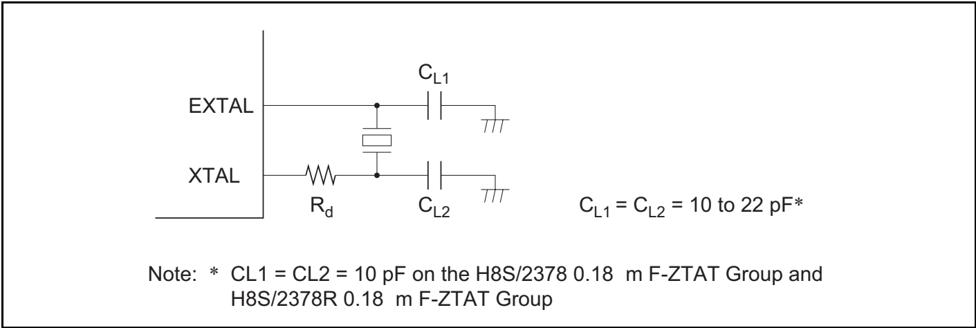
Figure 23.2 Connection of Crystal Resonator (Example)
