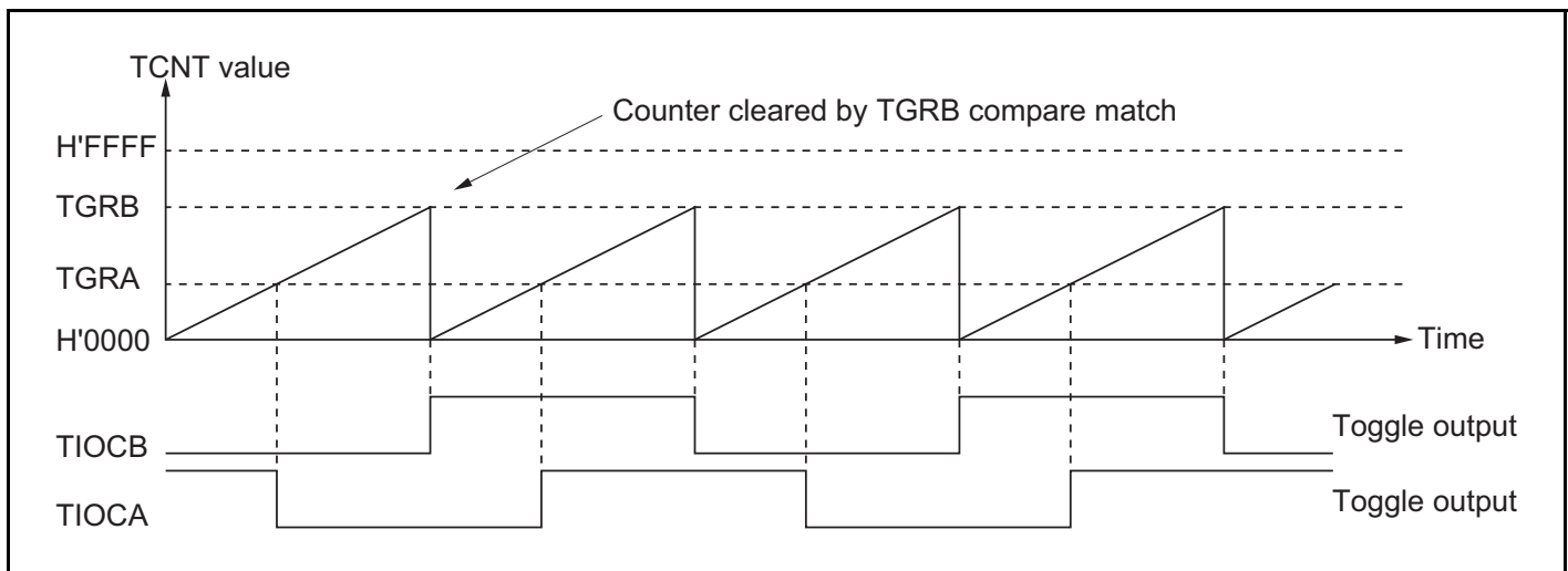
Figure 11.7 Example of Toggle Output Operation
