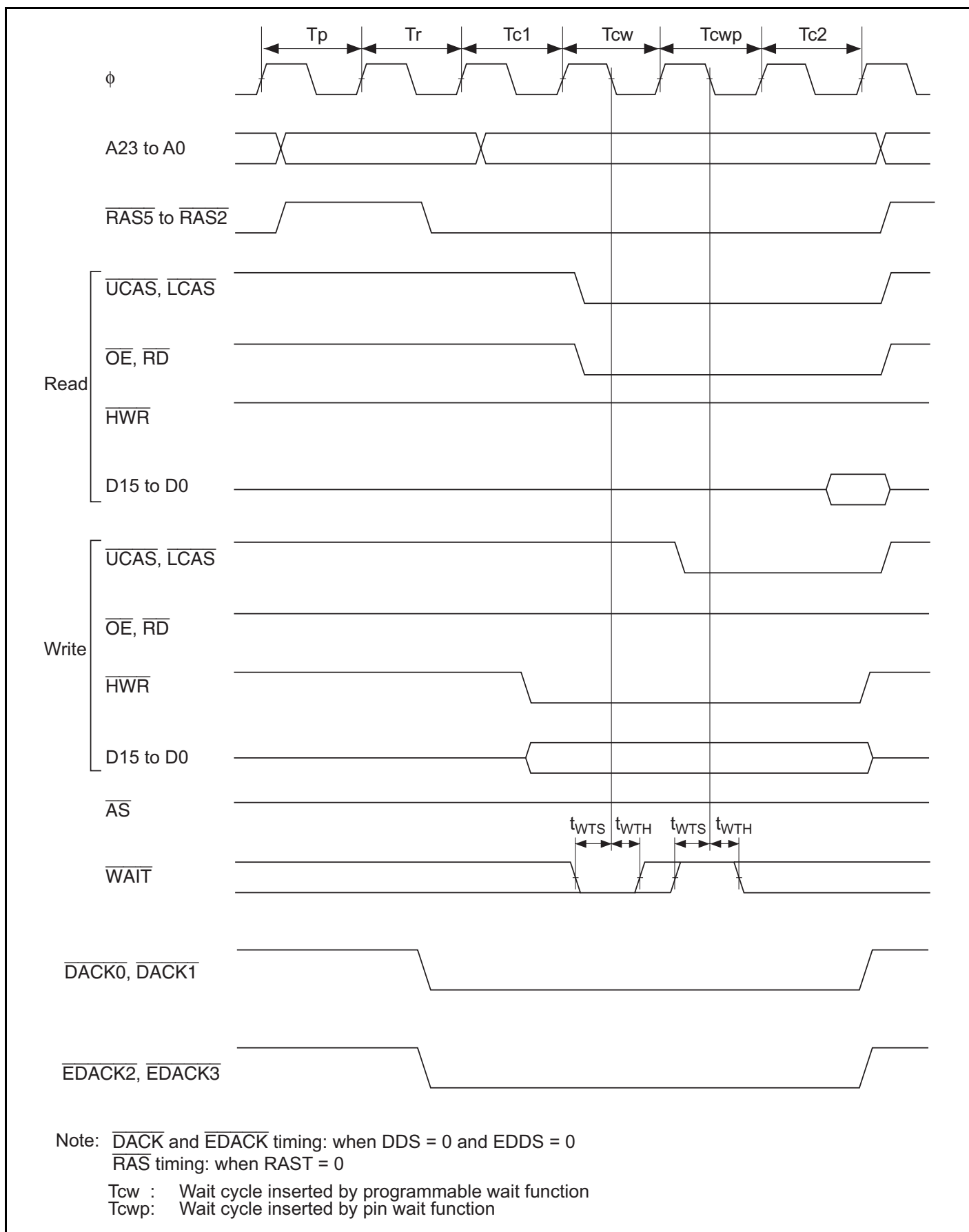
Figure 26.15 DRAM Access Timing: Two-State Access, One Wait
