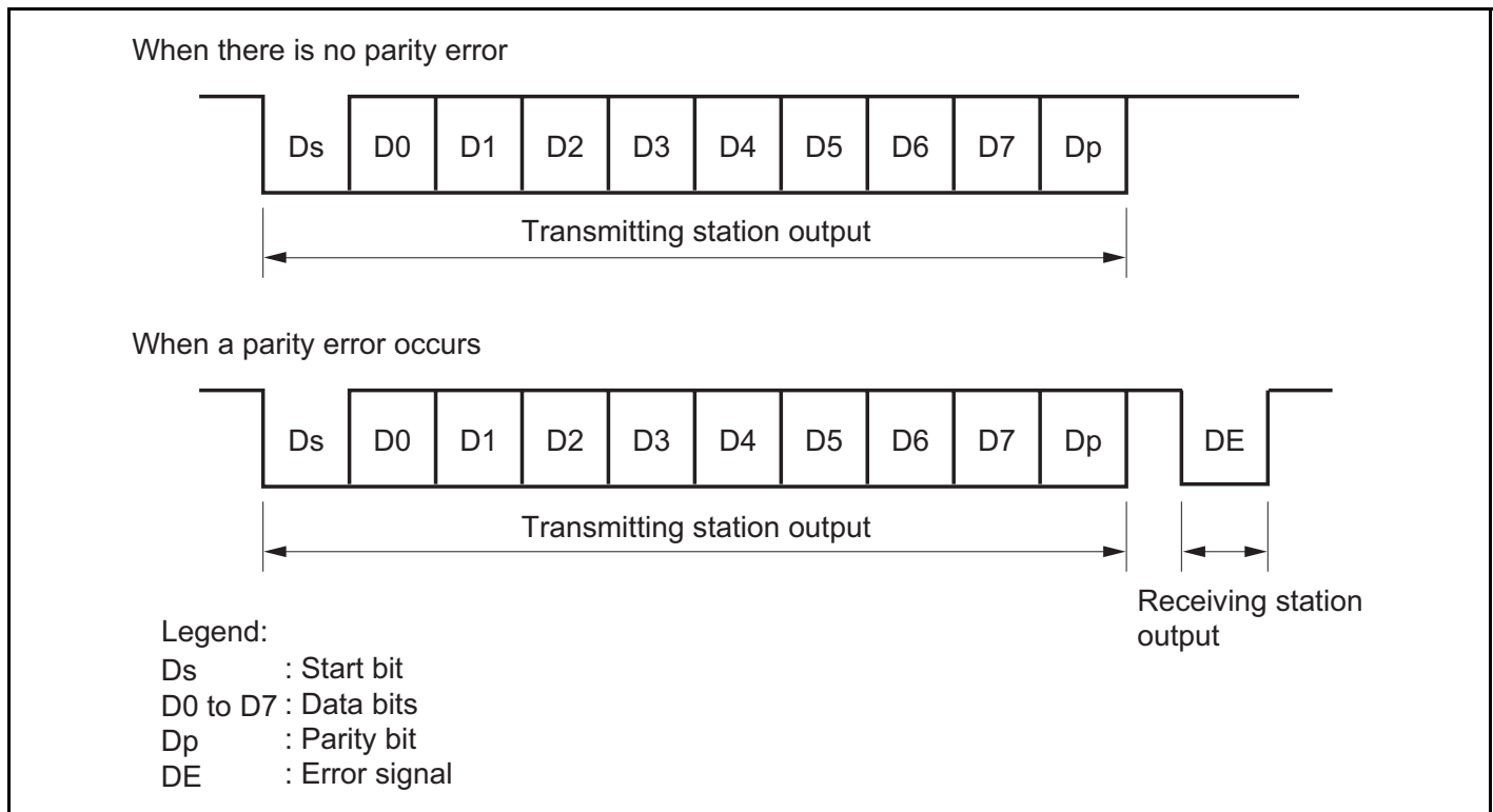
Figure 15.22 Normal Smart Card Interface Data Format
