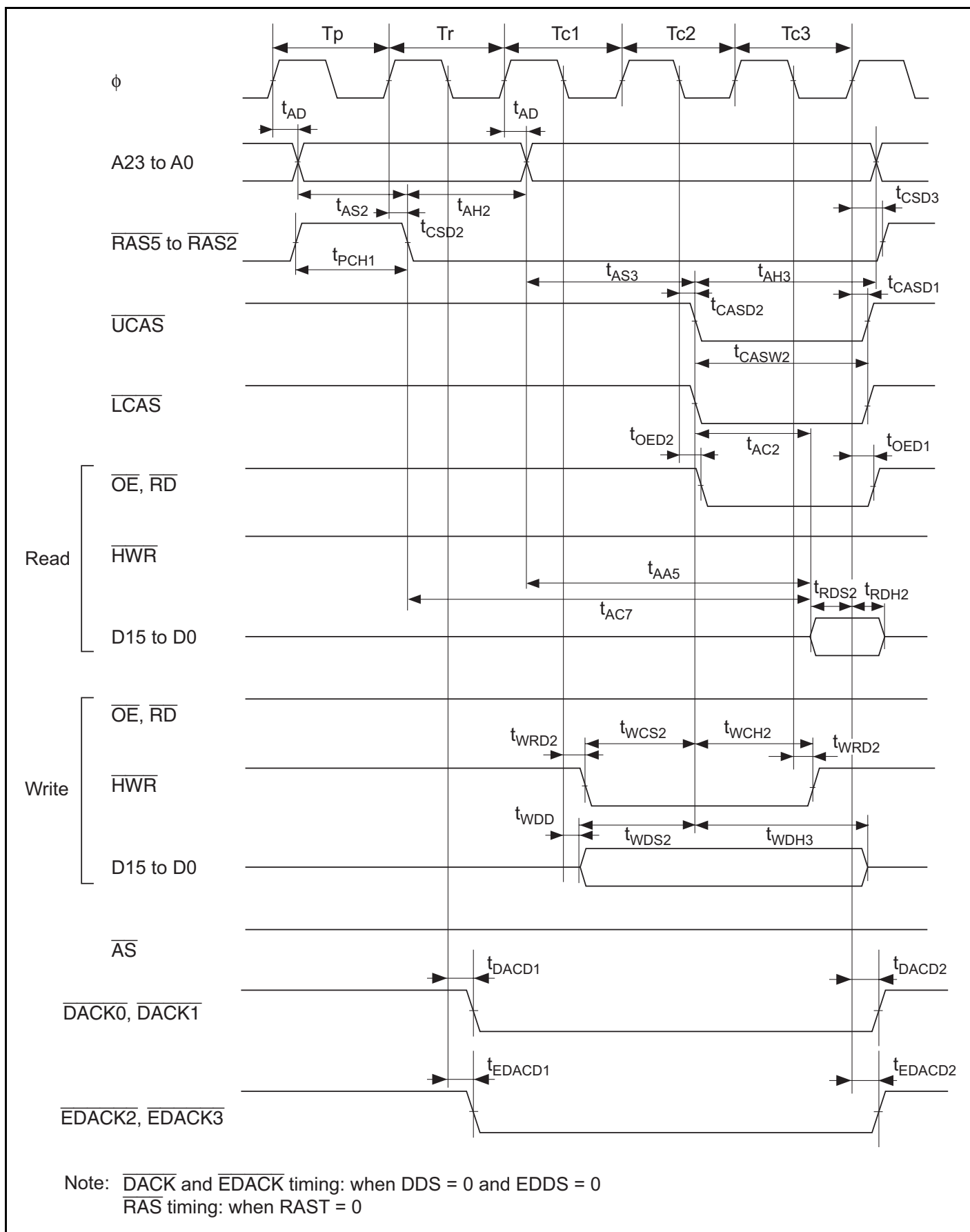
Figure 26.17 DRAM Access Timing: Three-State Access (RAST = 1)
