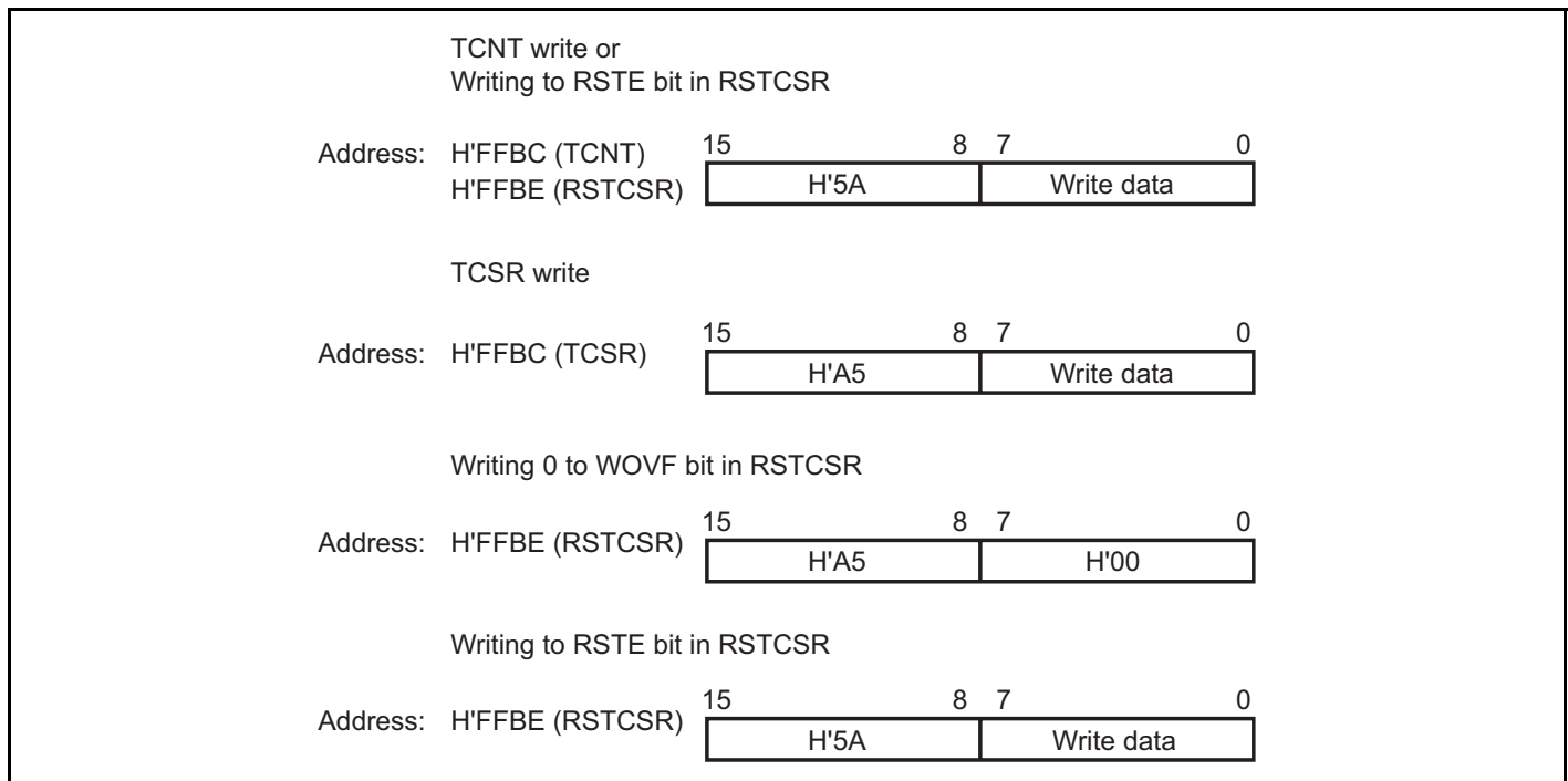
Figure 14.4 Writing to TCNT, TCSR, and RSTCSR
