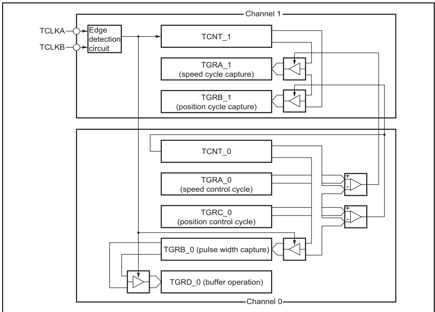
Figure 11.29 Phase Counting Mode Application Example
