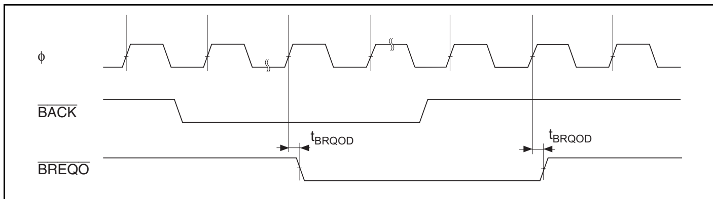
Figure 26.24 External Bus Request Output Timing
