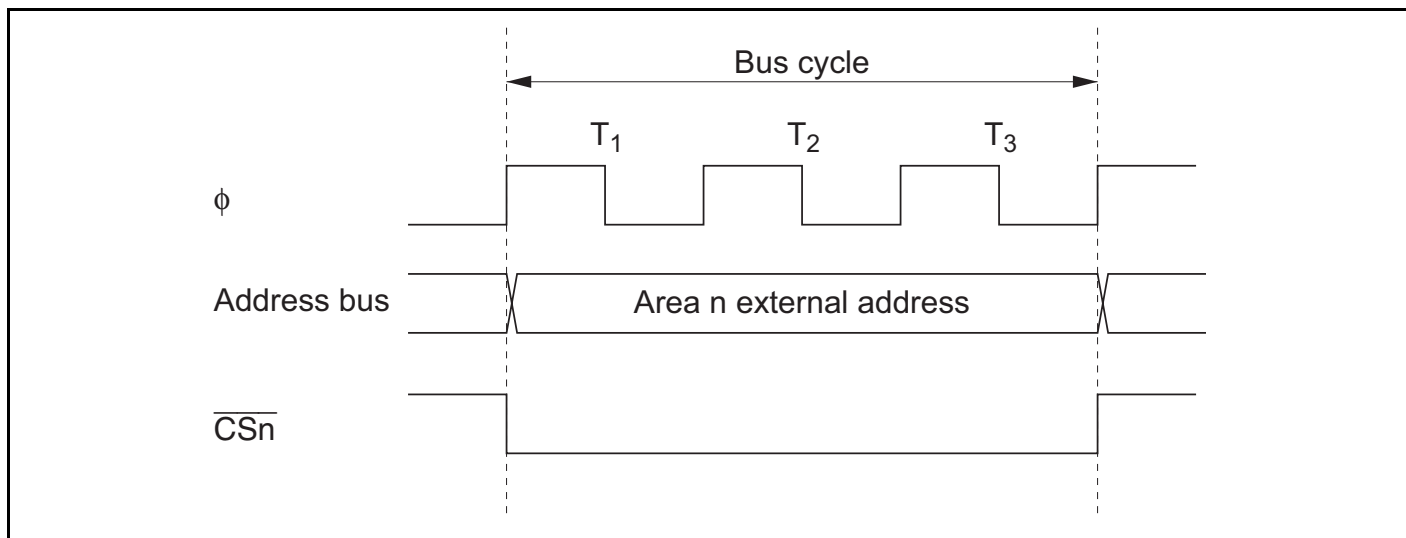
Figure 6.7 \overline{CSn} Signal Output Timing (n = 0 to 7)
