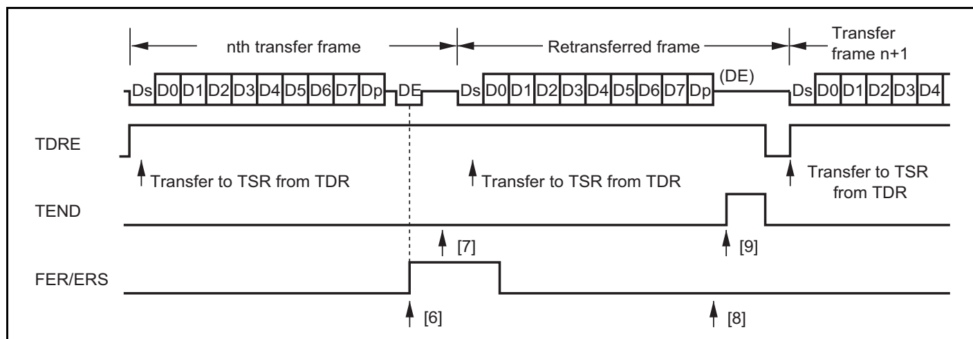
Figure 15.26 Retransfer Operation in SCI Transmit Mode
