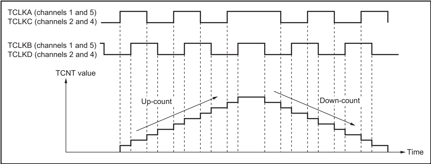
Figure 11.25 Example of Phase Counting Mode 1 Operation
