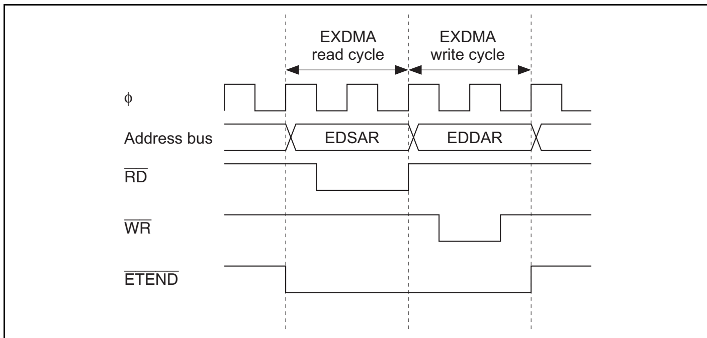
Figure 8.2 Example of Timing in Dual Address Mode
