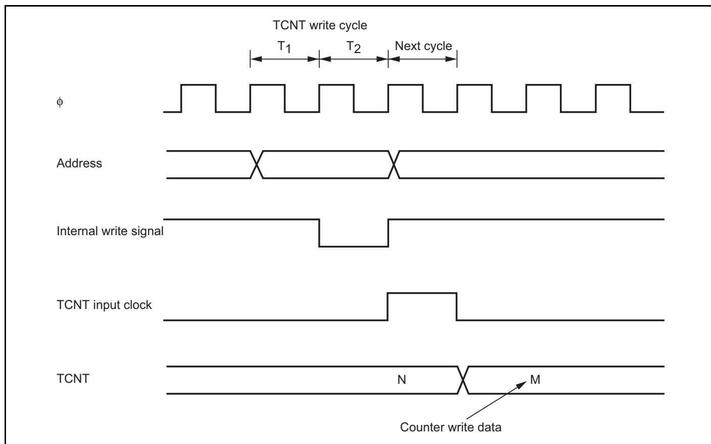
Figure 14.5 Contention between TCNT Write and Increment
