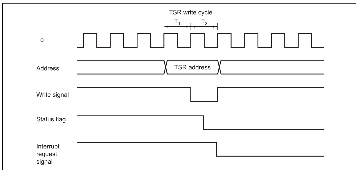
Figure 11.42 Timing for Status Flag Clearing by CPU
