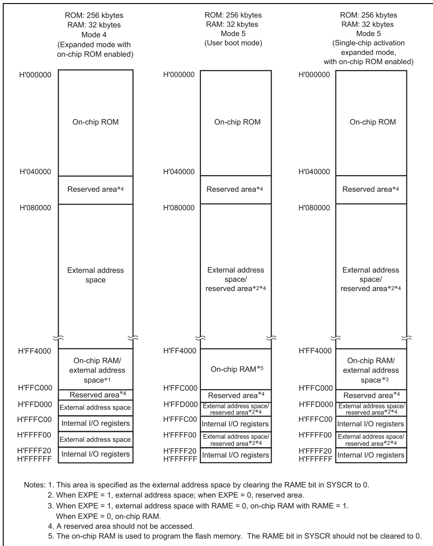
Figure 3.11 Memory Map for H8S/2372 and H8S/2372R (2)
