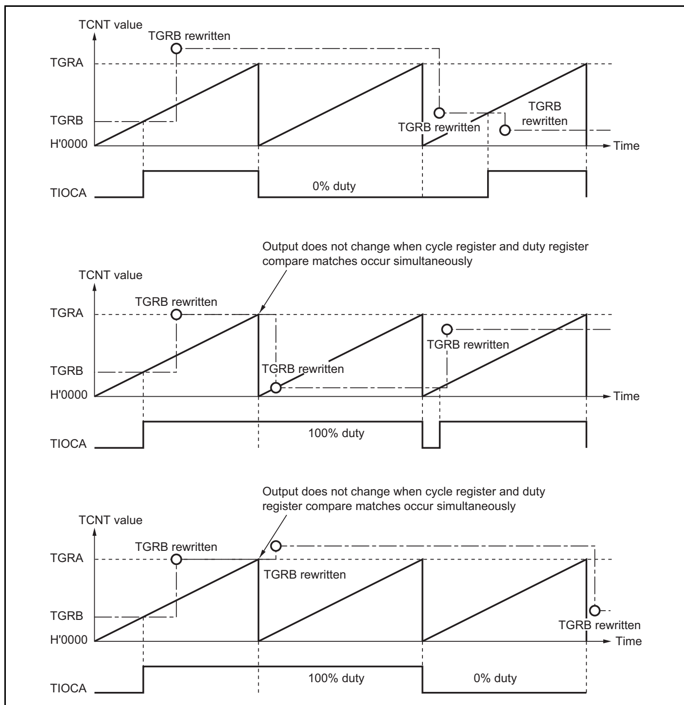
Figure 11.23 Example of PWM Mode Operation (3)
