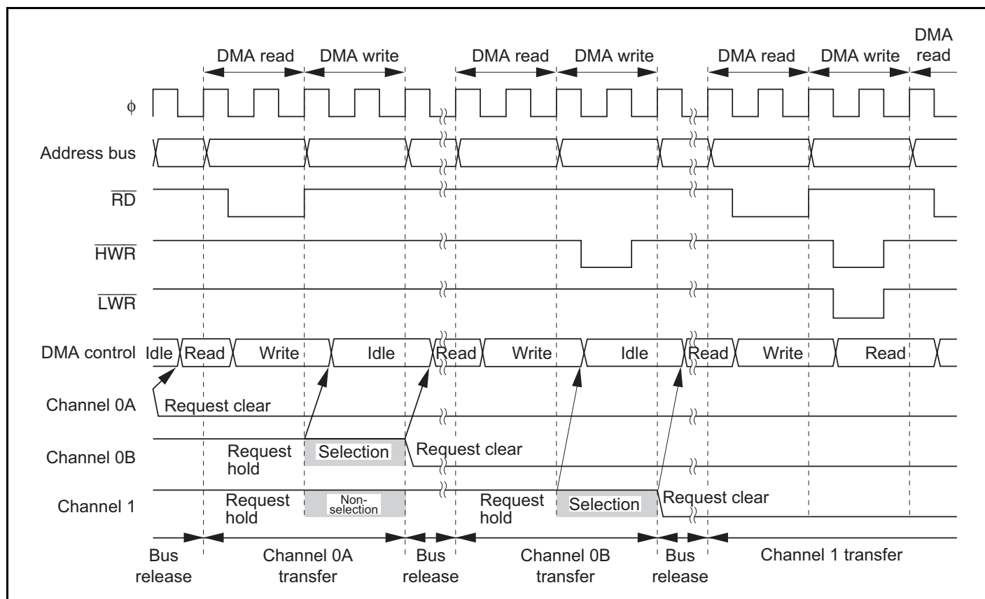
Figure 7.34 Example of Multi-Channel Transfer
