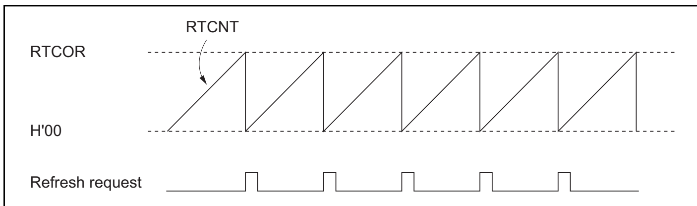
Figure 6.34 RTCNT Operation
