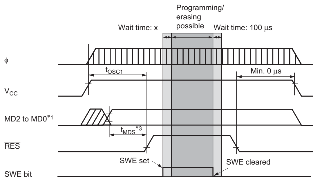
(1) Boot Mode
