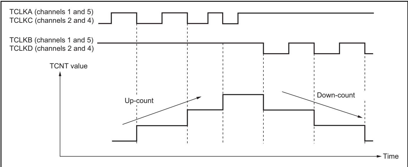
Figure 11.27 Example of Phase Counting Mode 3 Operation
