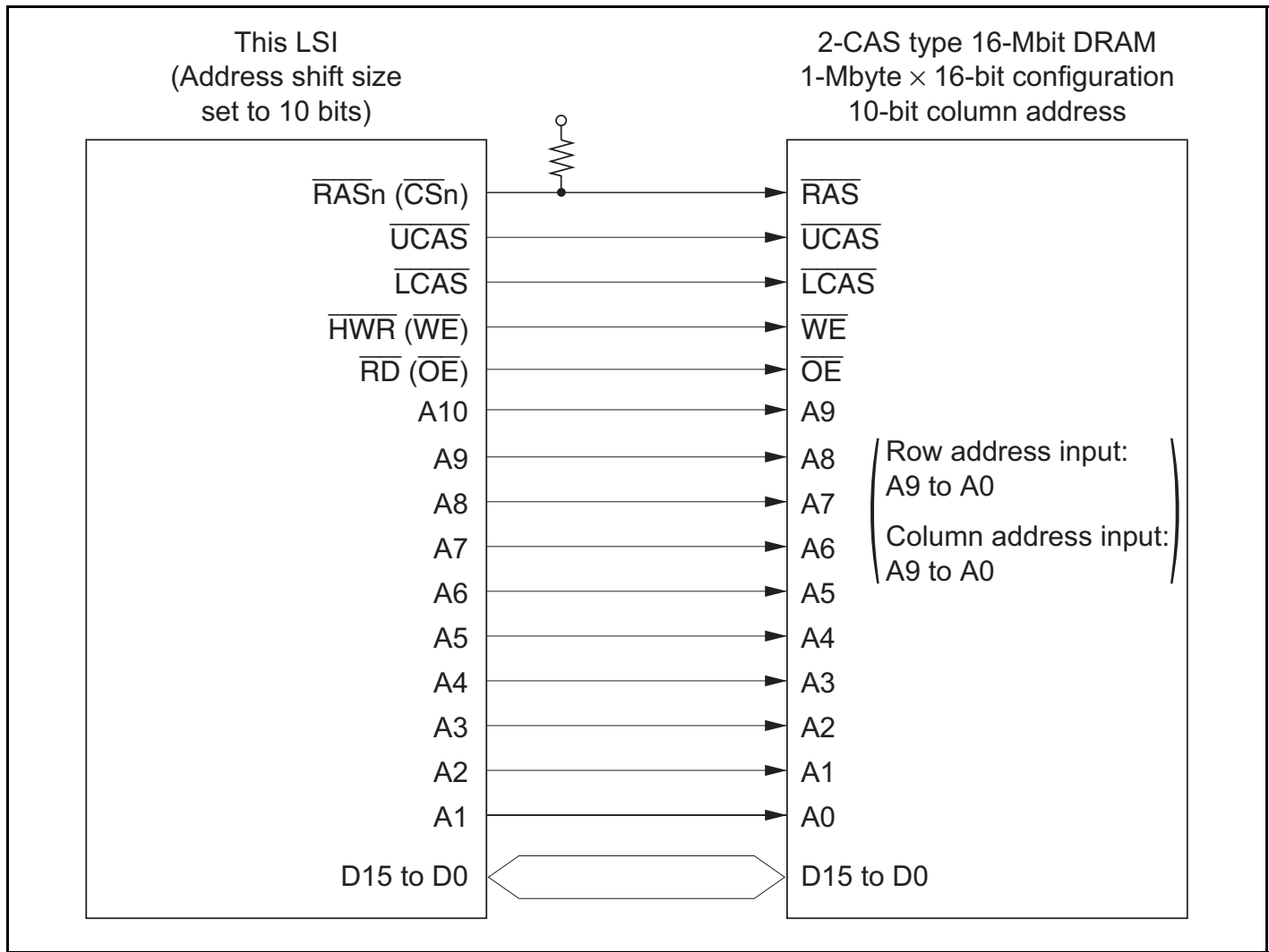
Figure 6.29 Example of 2-CAS DRAM Connection
