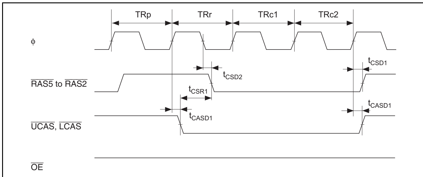
Figure 26.19 CAS-Before-RAS Refresh Timing
