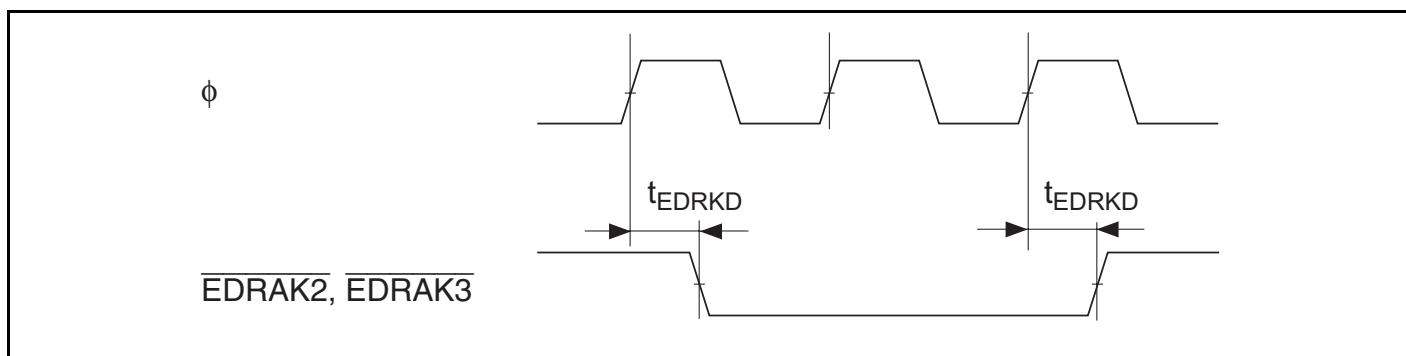
Figure 26.32 EXDMAC \overline{EDRAK} Output Timing
