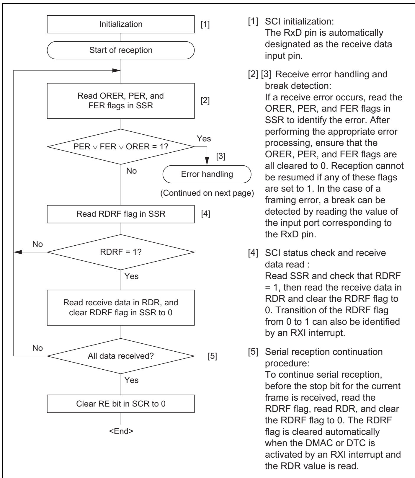
Figure 15.9 Sample Serial Reception Data Flowchart (1)
