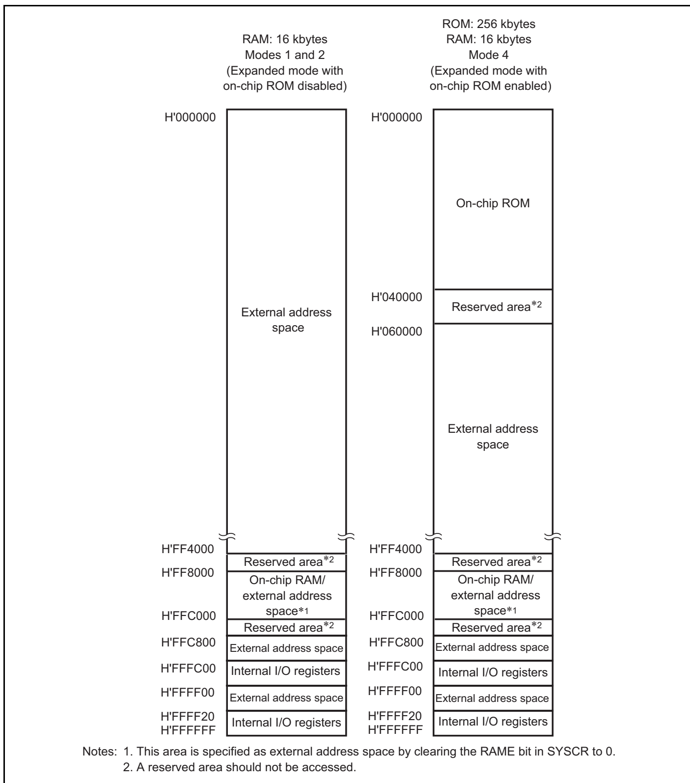
Figure 3.5 Memory Map for H8S/2375 and H8S/2375R (1)
