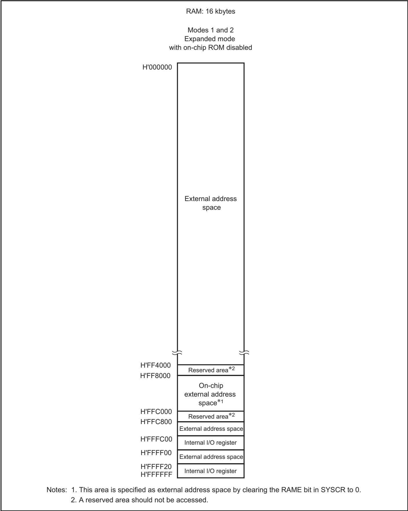
Figure 3.9 Memory Map for H8S/2373 and H8S/2373R
