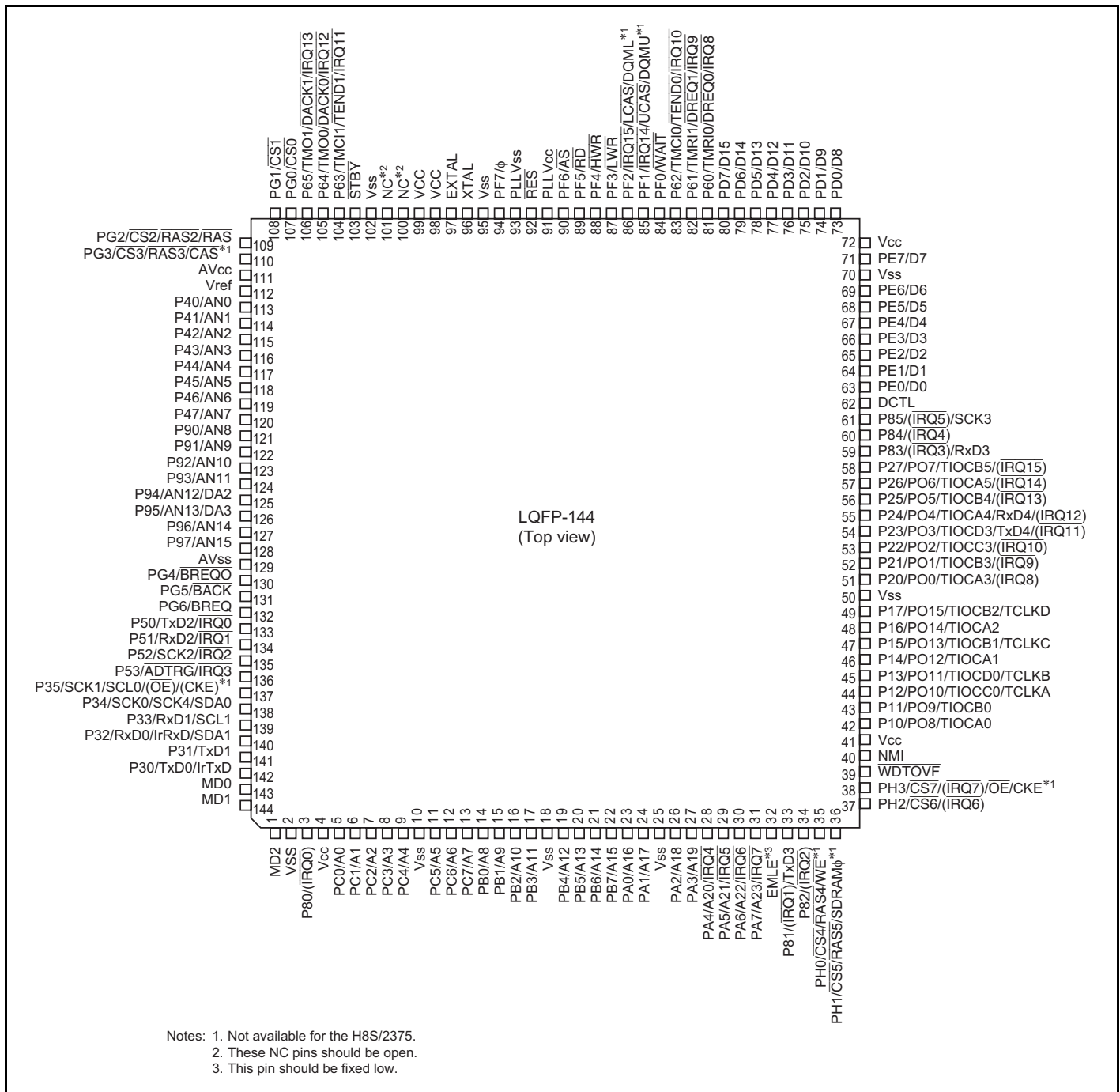
Figure 1.7 Pin Arrangement for H8S/2375 and H8S/2375R
