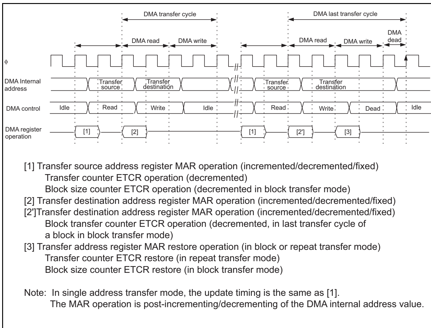
Figure 7.39 DMAC Register Update Timing
