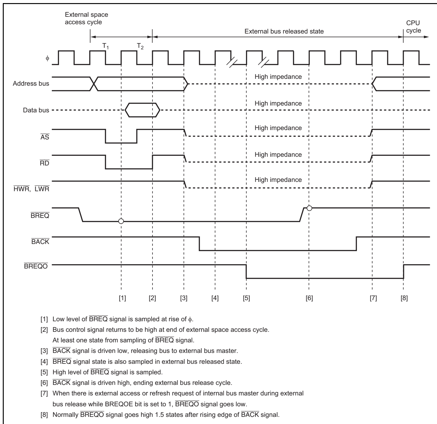
Figure 6.84 Bus Released State Transition Timing
