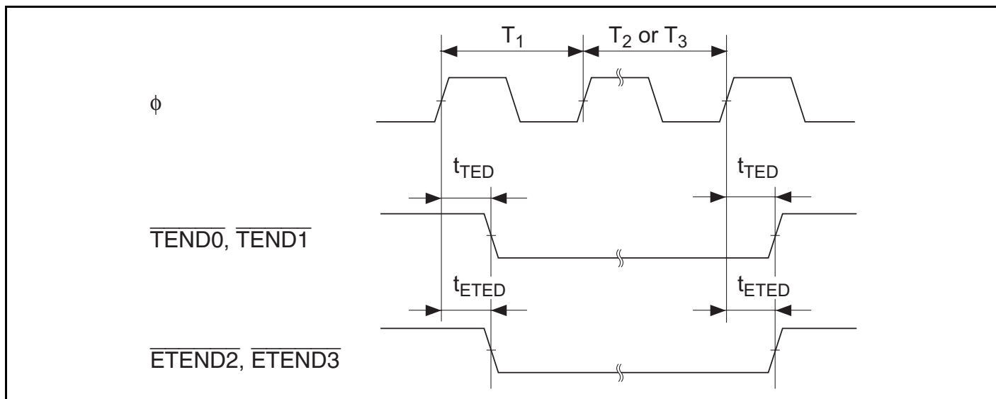
Figure 26.30 DMAC and EXDMAC \overline{TEND}/\overline{ETEND} Output Timing
