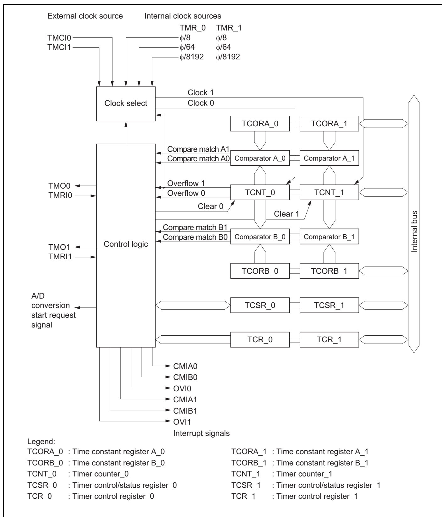
Figure 13.1 Block Diagram of 8-Bit Timer Module
