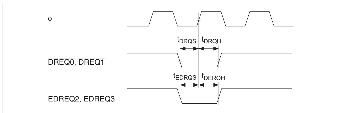
Figure 26.31 DMAC and EXDMAC \overline{DREQ}/\overline{EDREQ} Input Timing
