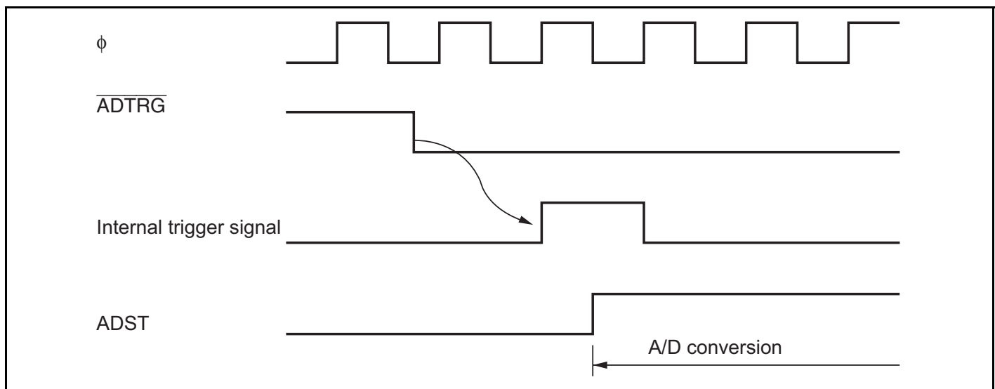
Figure 17.3 External Trigger Input Timing
