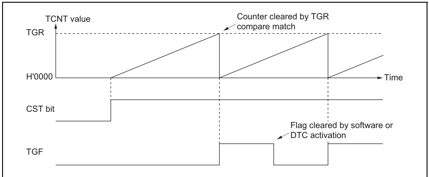
Figure 11.4 Periodic Counter Operation
