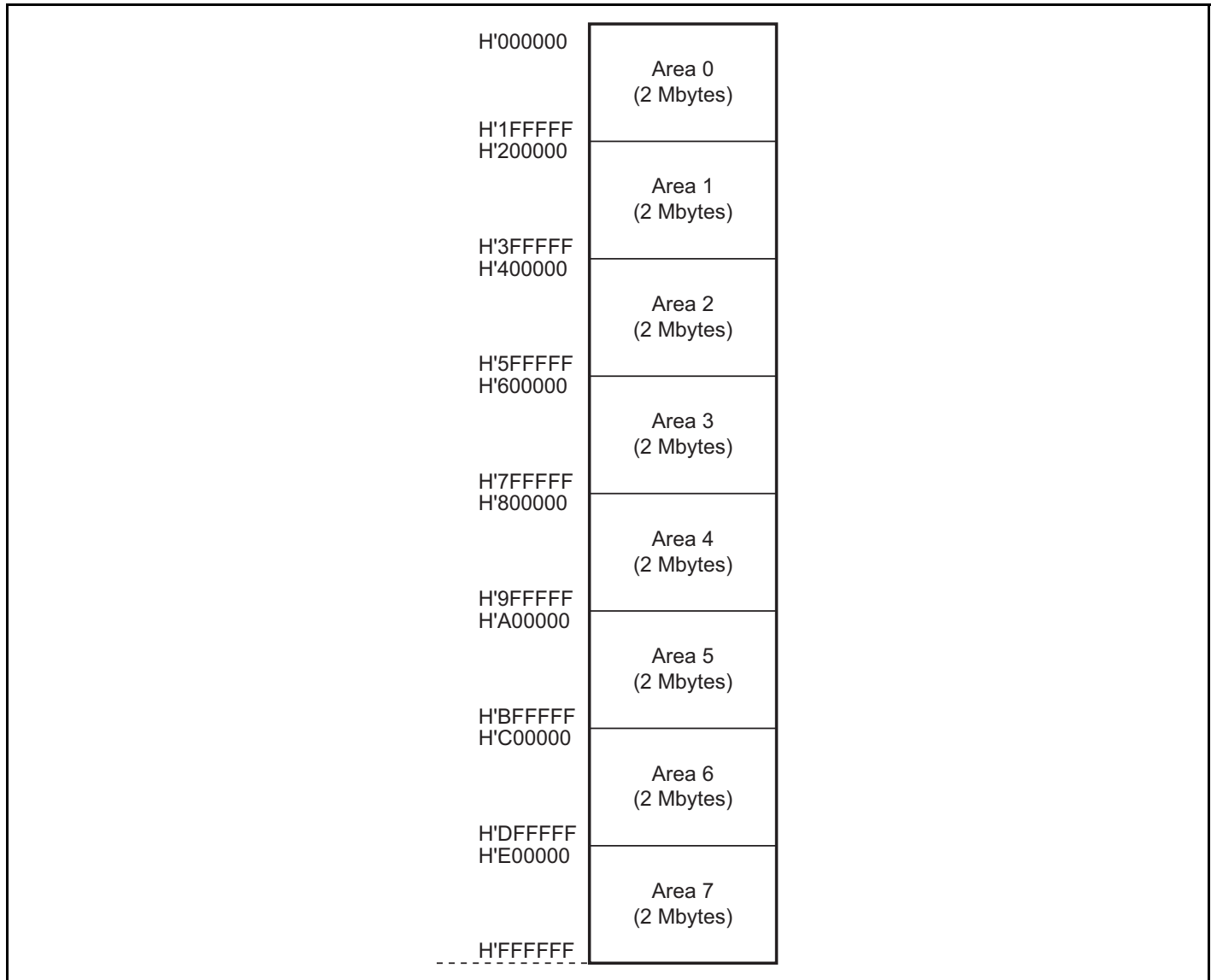
Figure 6.6 Area Divisions
