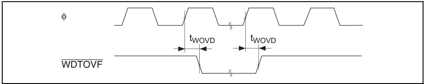
Figure 26.40 WDT Output Timing
