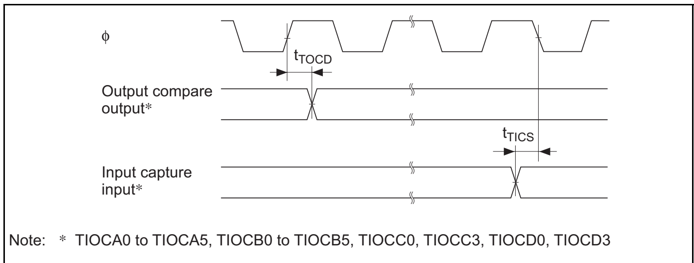
Figure 26.35 TPU Input/Output Timing
