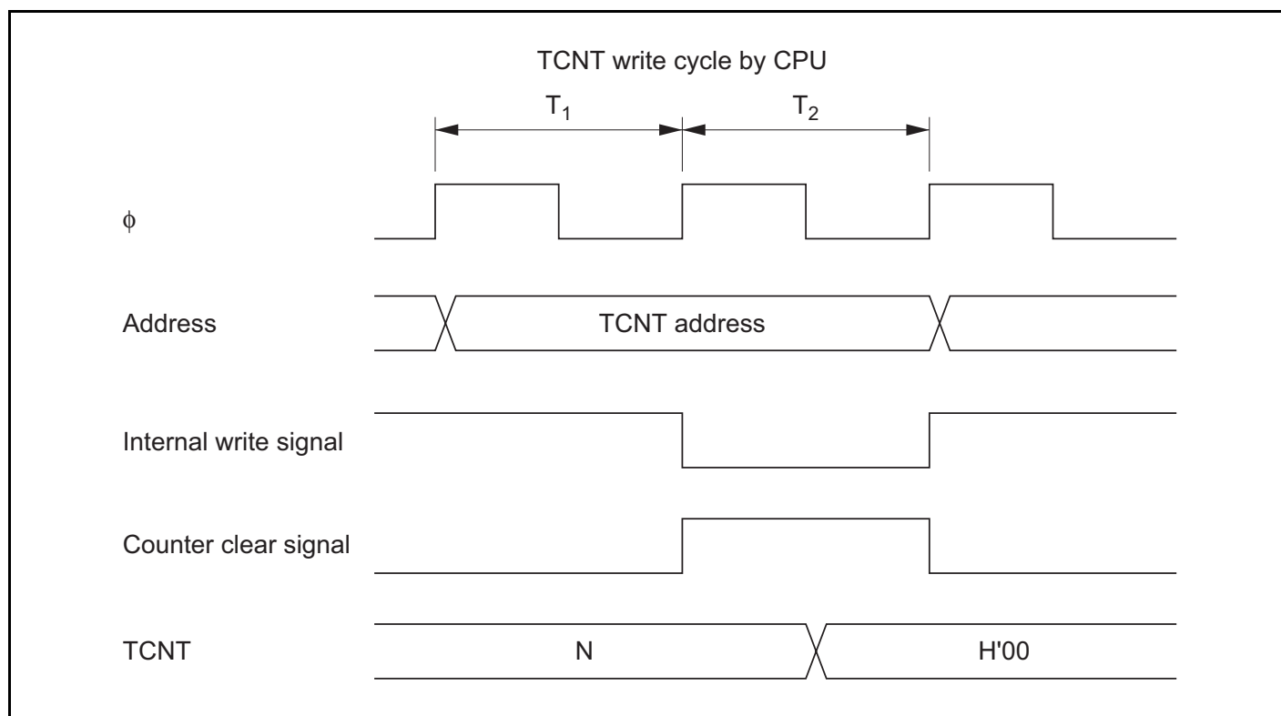
Figure 13.10 Contention between TCNT Write and Clear
