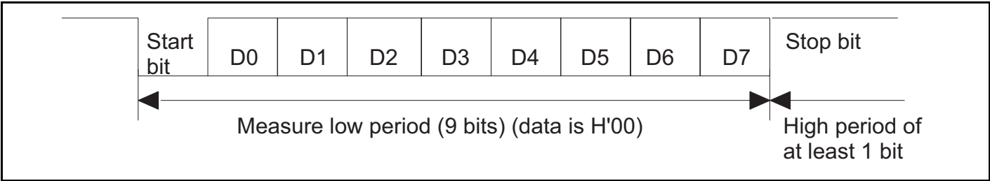
Figure 21.7 Automatic-Bit-Rate Adjustment Operation of SCI
