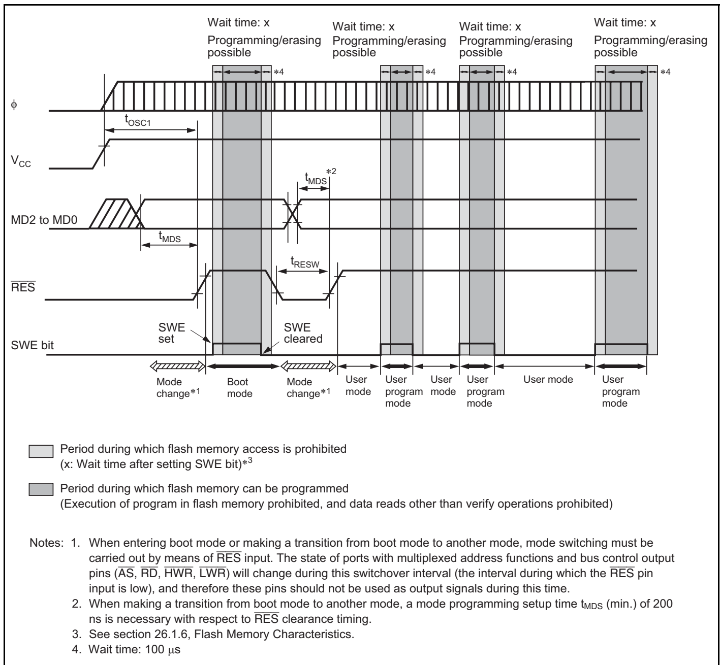
Figure 20.10 Mode Transition Timing (Example: Boot Mode → User Mode ↔ User Program Mode)
