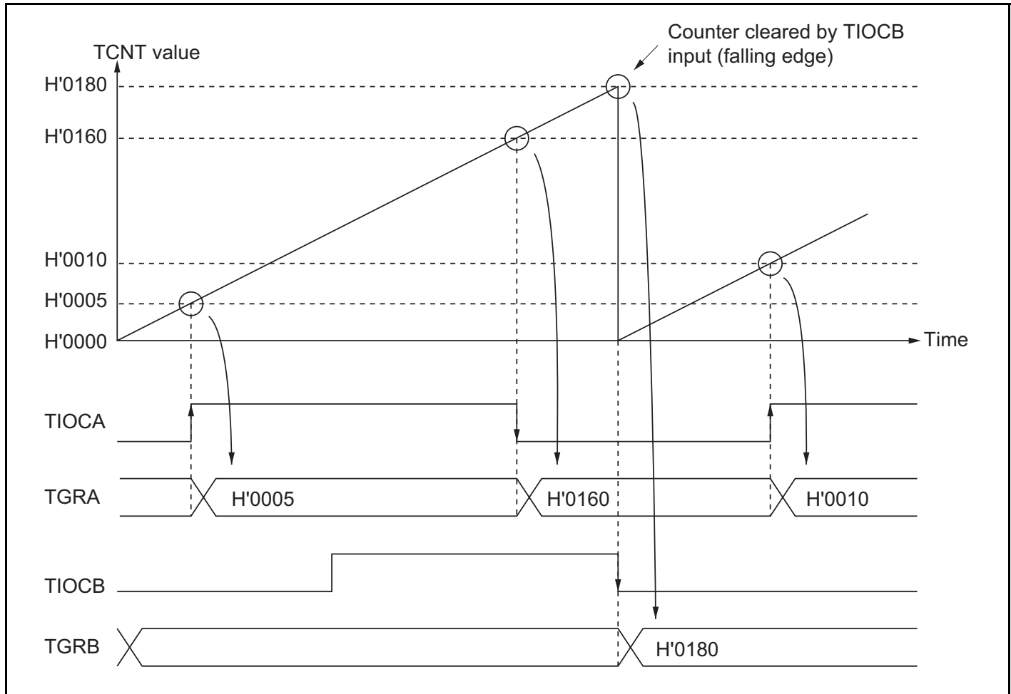
Figure 11.9 Example of Input Capture Operation
