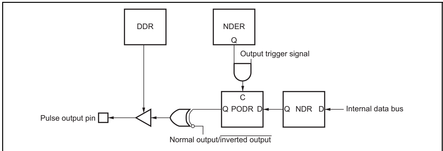
Figure 12.2 Overview Diagram of PPG
