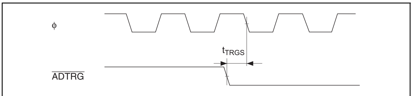
Figure 26.43 A/D Converter External Trigger Input Timing
