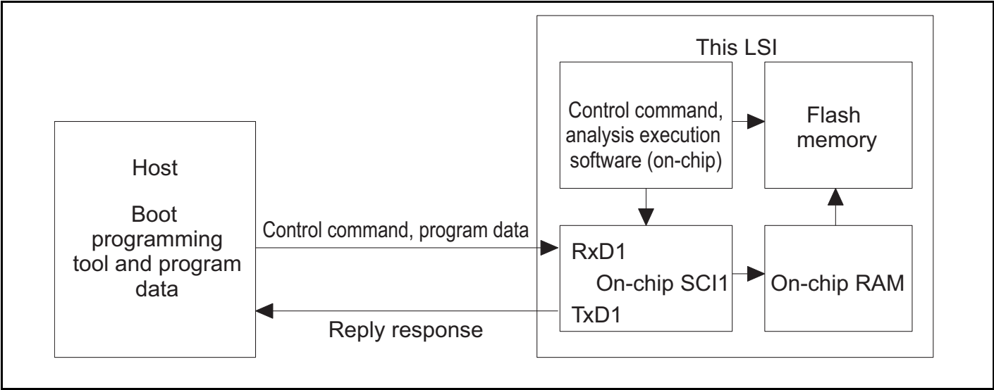
Figure 21.6 System Configuration in Boot Mode
