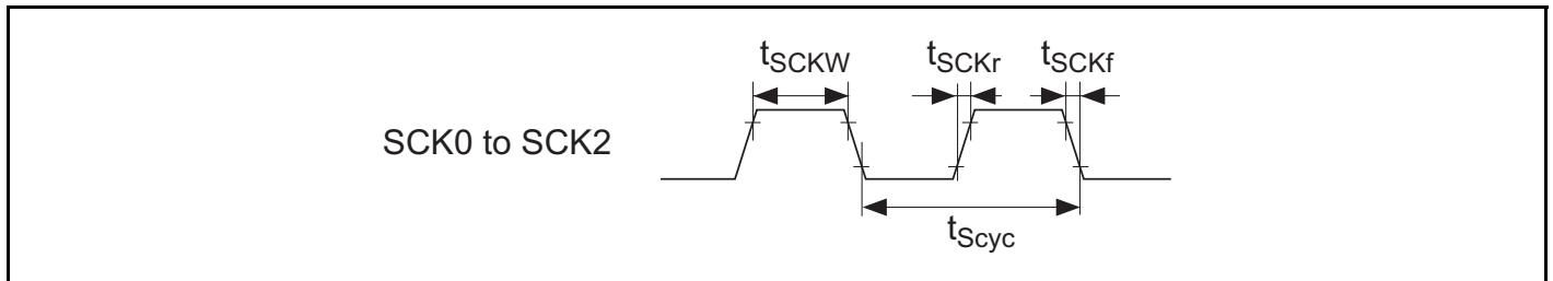
Figure 26.41 SCK Clock Input Timing
