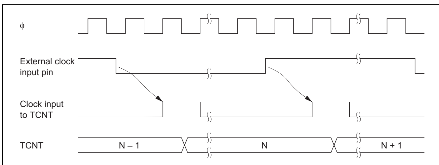
Figure 13.4 Count Timing for External Clock Input
