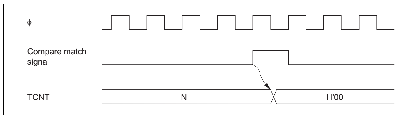
Figure 13.7 Timing of Compare Match Clear
