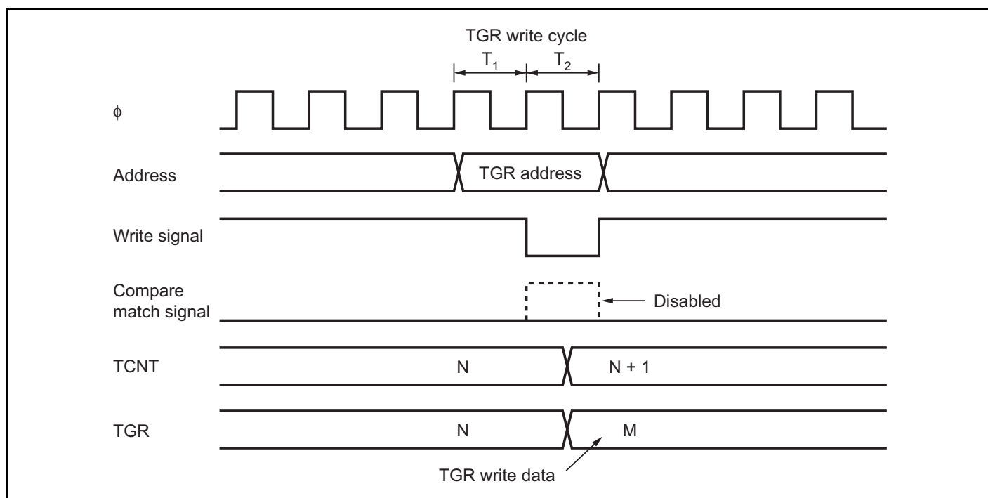
Figure 11.47 Contention between TGR Write and Compare Match
