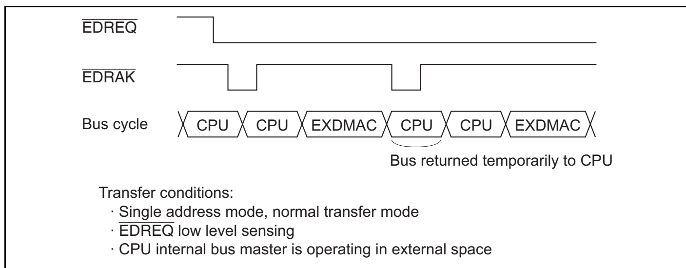
Figure 8.5 Example of Timing in Cycle Steal Mode
