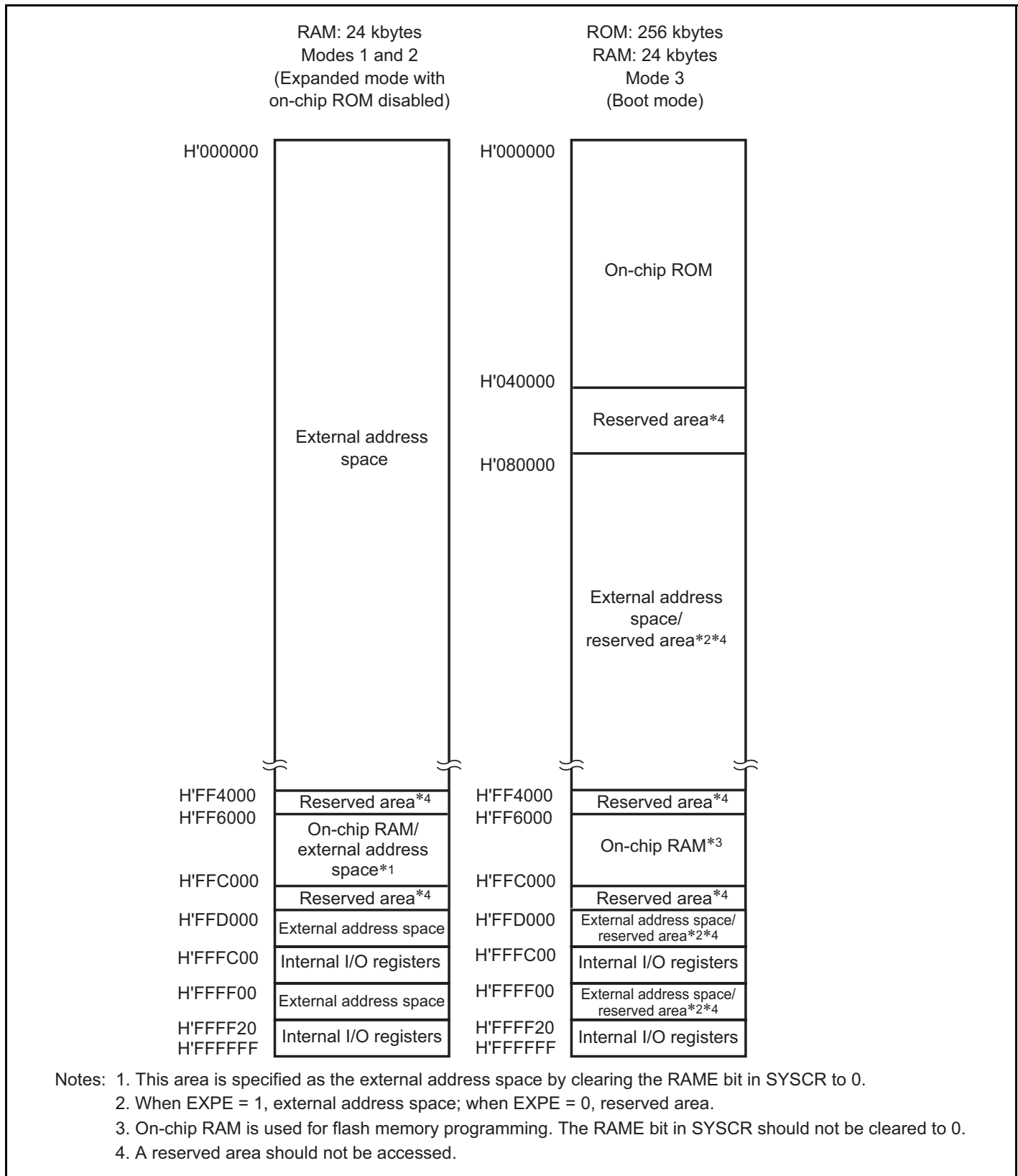
Figure 3.12 Memory Map for H8S/2371 and H8S/2371R (1)
