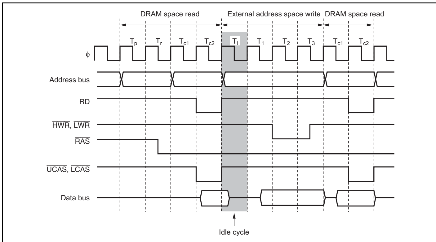
Figure 6.77 Example of Idle Cycle Operation after DRAM Access (Write after Read) (IDL = 0, RAST = 0, CAST = 0)
