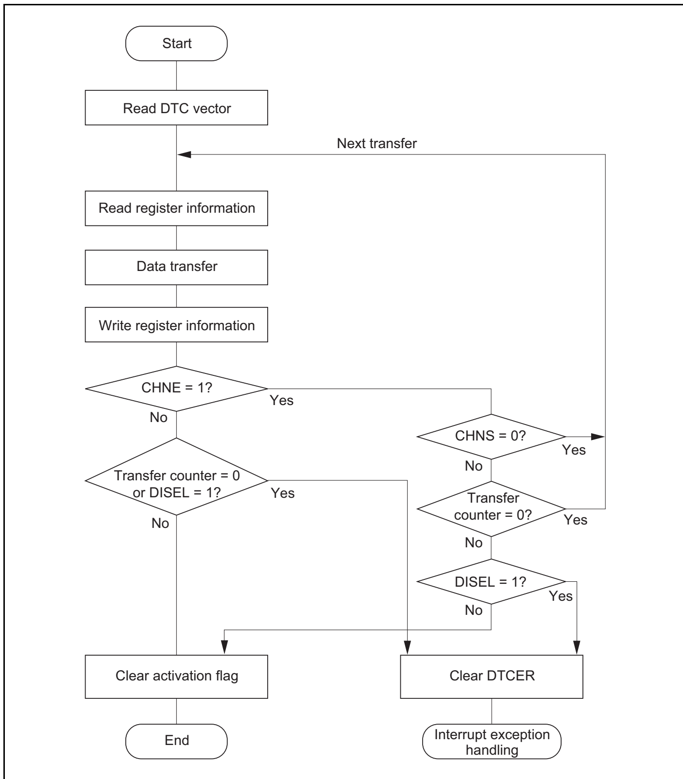
Figure 9.5 Flowchart of DTC Operation
