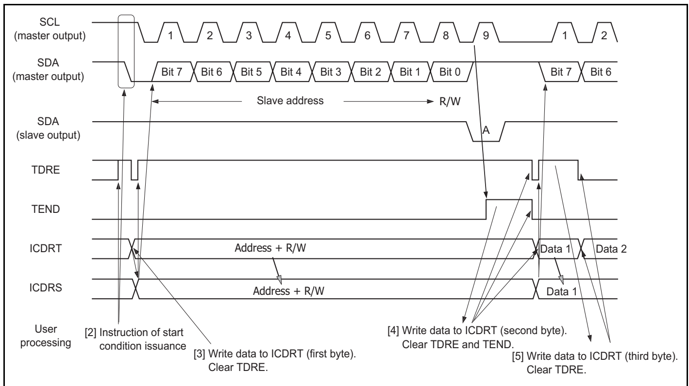
Figure 16.5 Master Transmit Mode Operation Timing 1
