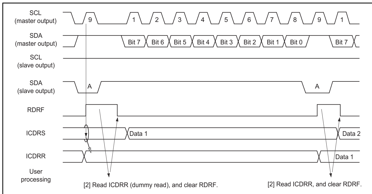
Figure 16.11 Slave Receive Mode Operation Timing 1
