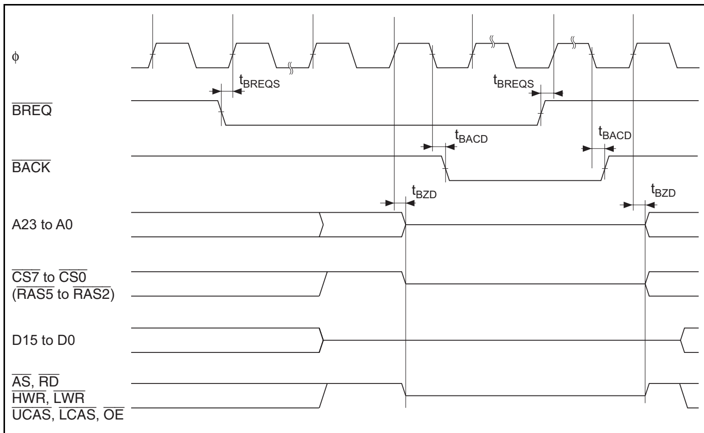
Figure 26.23 External Bus Release Timing
