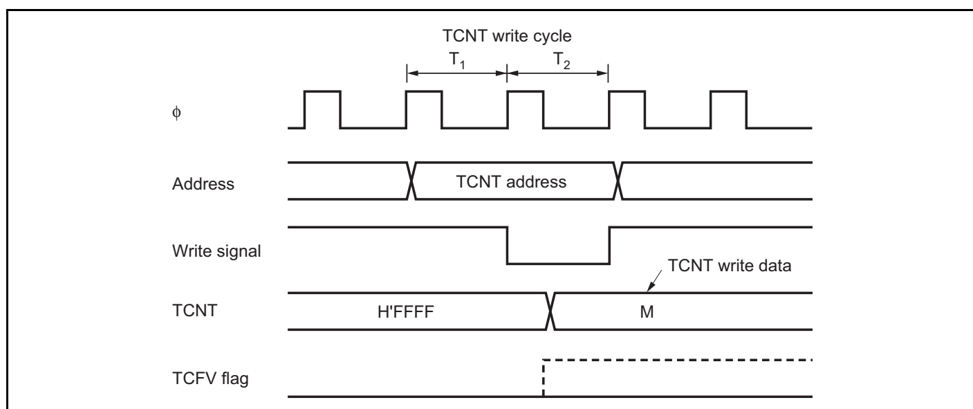
Figure 11.53 Contention between TCNT Write and Overflow
