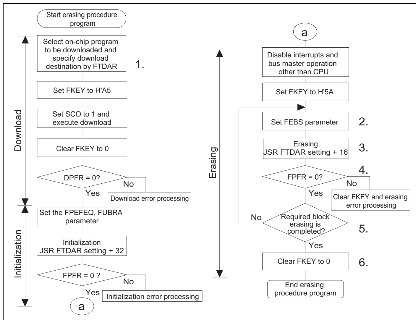
Figure 21.12 Erasing Procedure
