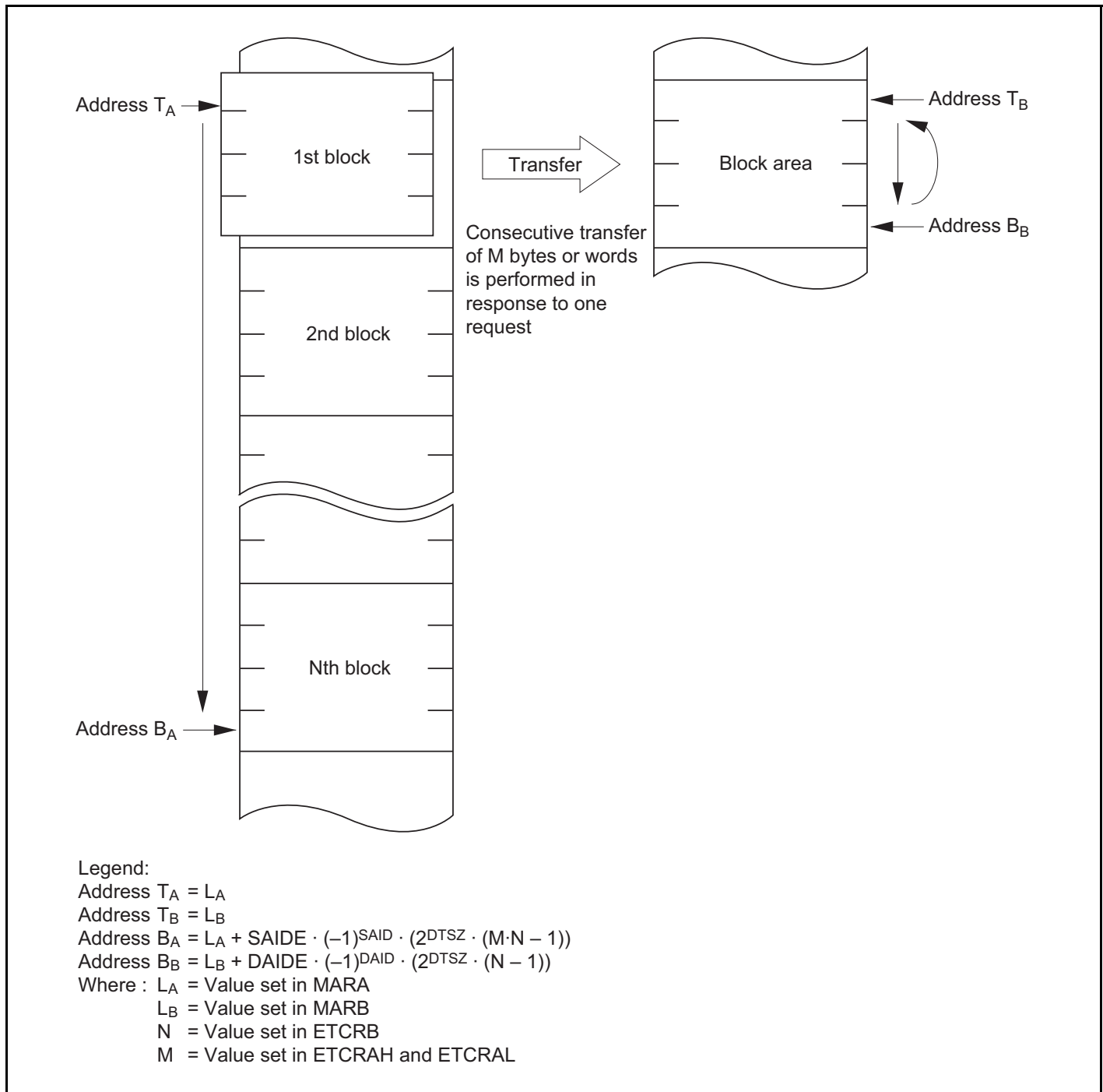
Figure 7.13 Operation in Block Transfer Mode (BLKDIR = 0)
