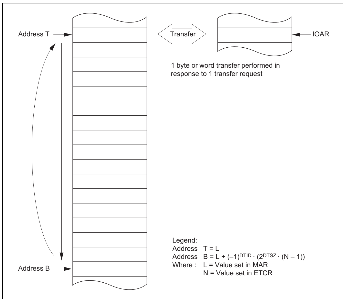
Figure 7.7 Operation in Repeat mode
