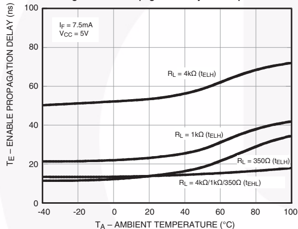
Fig. 9 Enable Propagation Delay vs. Temperature
