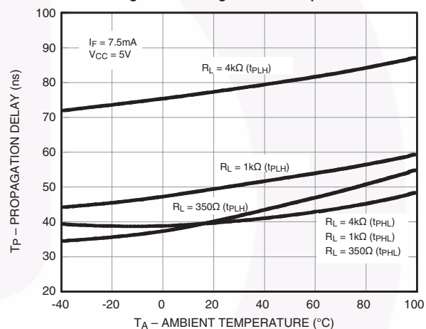
Fig. 10 Switching Time vs. Temperature
