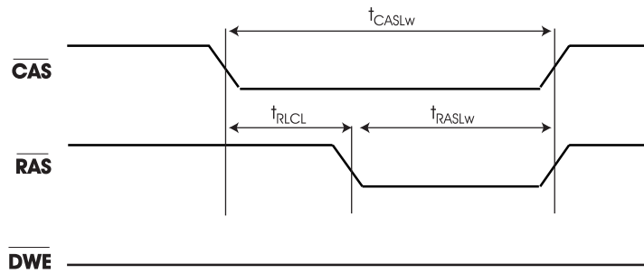
Figure 1-26: ARAM/DRAM Power-Down Refresh Cycle Timing
