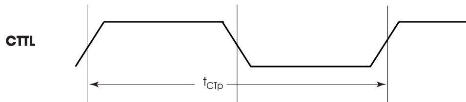
Figure 1-37: CCTL Timing
