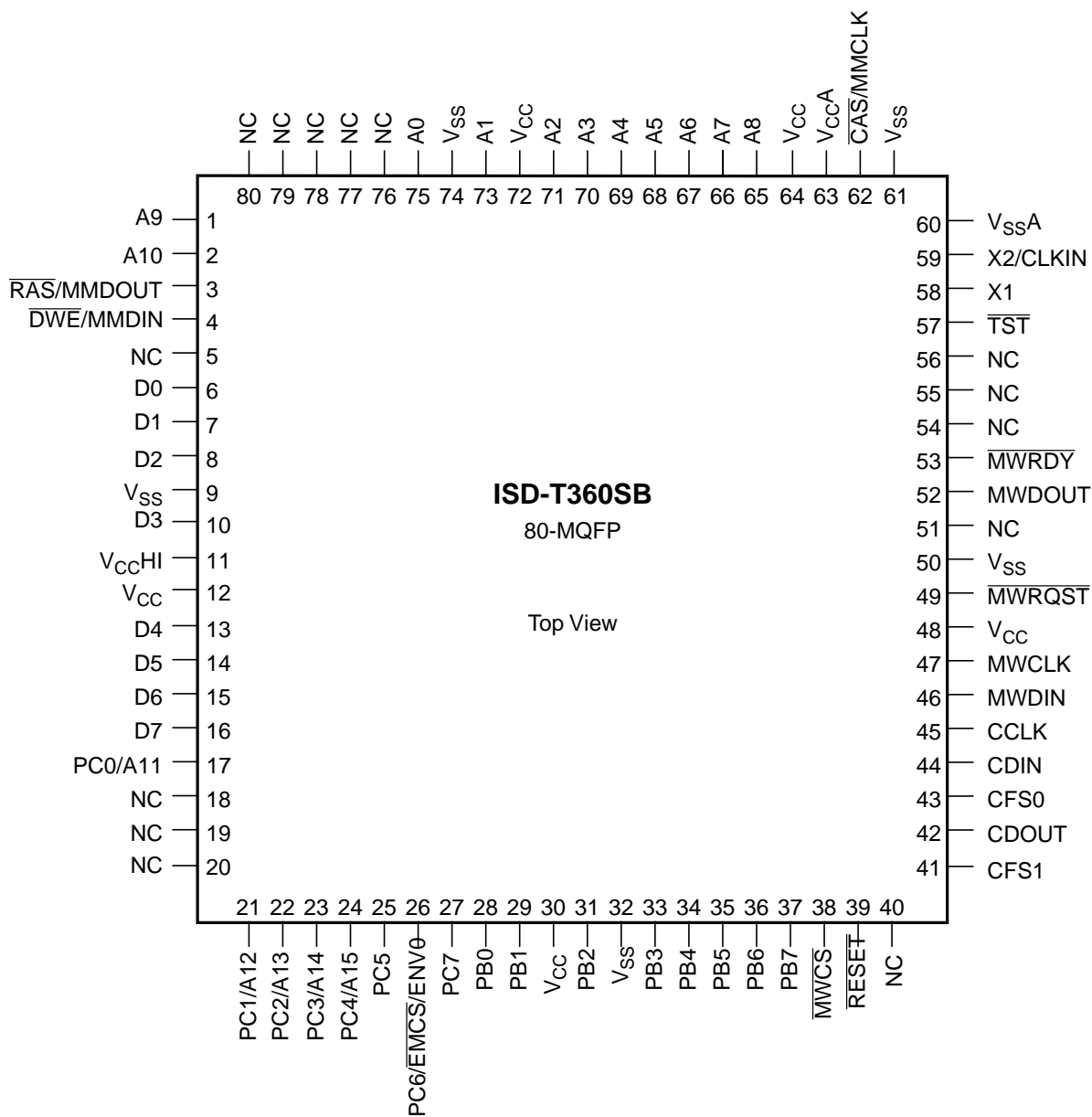
Figure 1-1: 80-MQFP Package Connection Diagram
