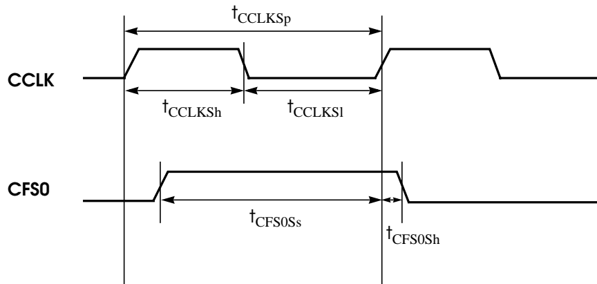
Figure 1-31: Slave Codec CCLK and CFS0 Timing
