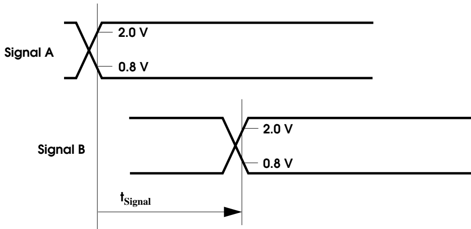
Figure 1-22: Asynchronous Signals
