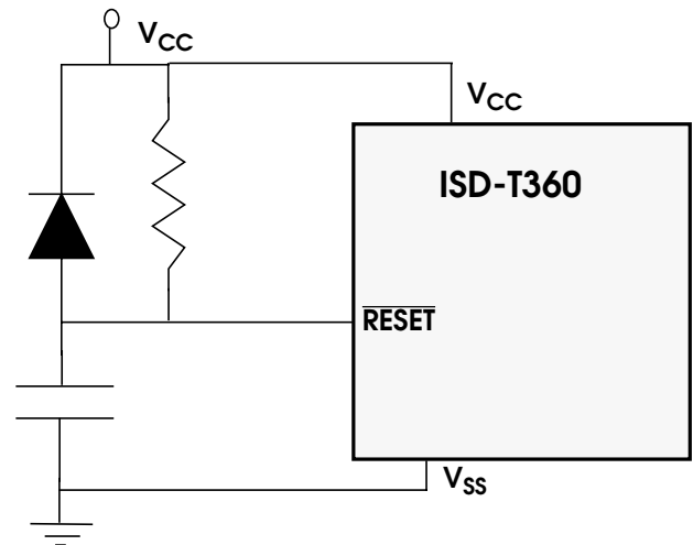
Figure 1-2: Recommended Power-On Reset Circuit
