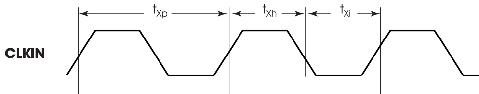
Figure 1-36: CLKIN Timing
