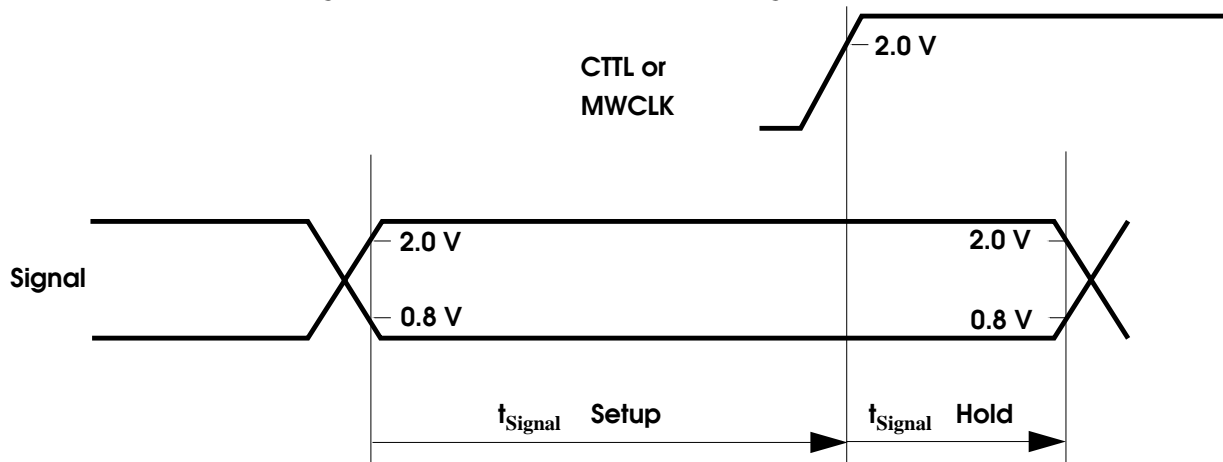
Figure 1-21: Synchronous Input Signals
