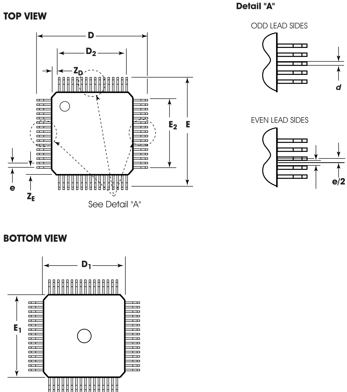
Figure 4-1: 80-Pin Plastic Quad Flat Package, Top and Bottom—Type: Metric PQFP, 14x14 Body
