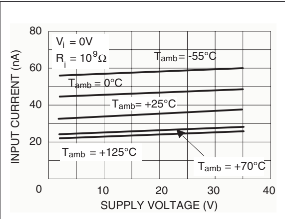
Figure 2. Input current vs. supply voltage
