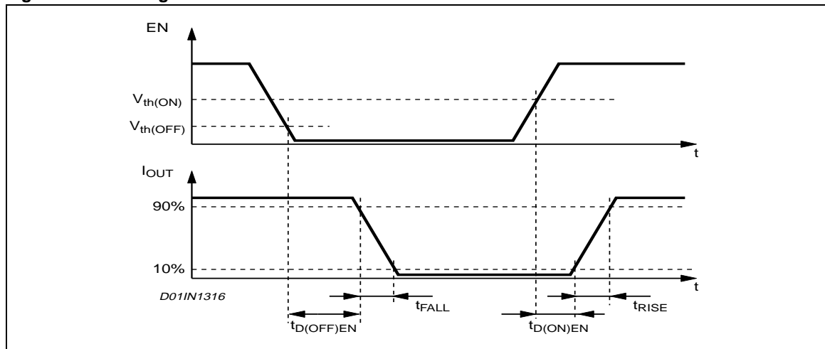
Figure 1. Switching Characteristic Definition
