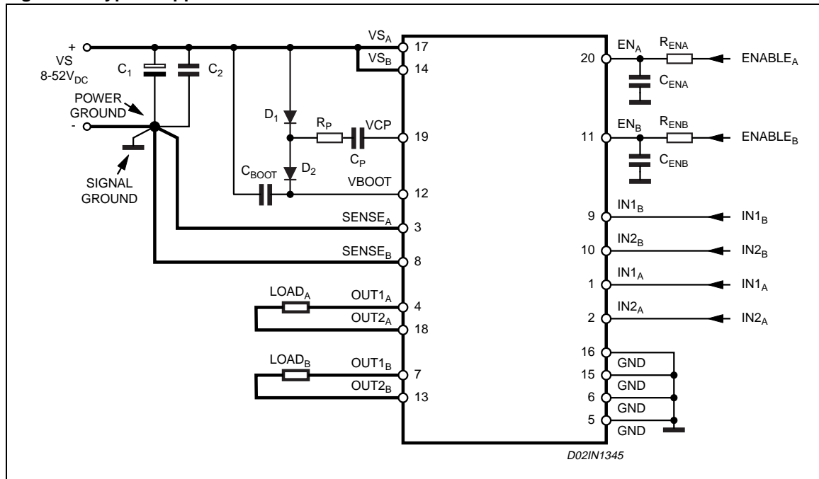
Figure 11. Typical Application
