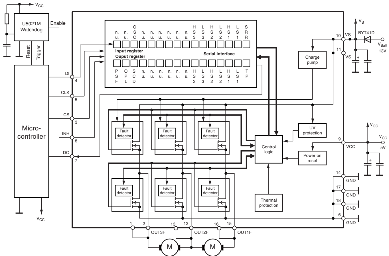
Figure 10-1. Application Circuit
