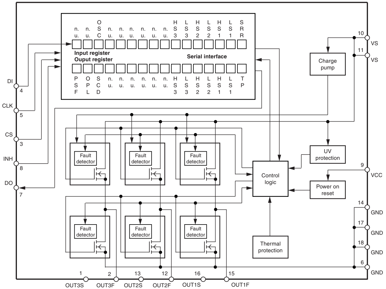
Figure 1-1. Block Diagram
