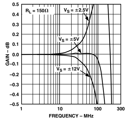
TPC 6. AD8130 Fine Scale Response vs. Supply, R_L = 150\ \Omega
