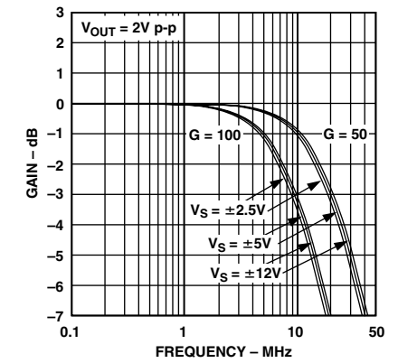
TPC 33. AD8129 Frequency Response vs. Supply, G = 50 , G = 100 , V_{OUT} = 2 V p-p
