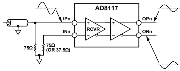
Figure 67. Example of Input Driven Single-Ended
