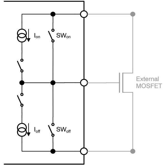
Figure 10. Pre-driver Topology
