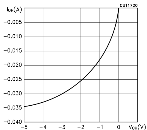
Figure 6 : Receiver Output Current vs Output Voltage (Output High)
