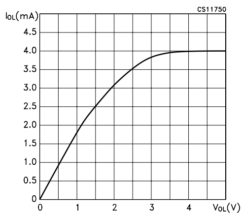
Figure 5 : Receiver Output Current vs Output Voltage (Output Low)
