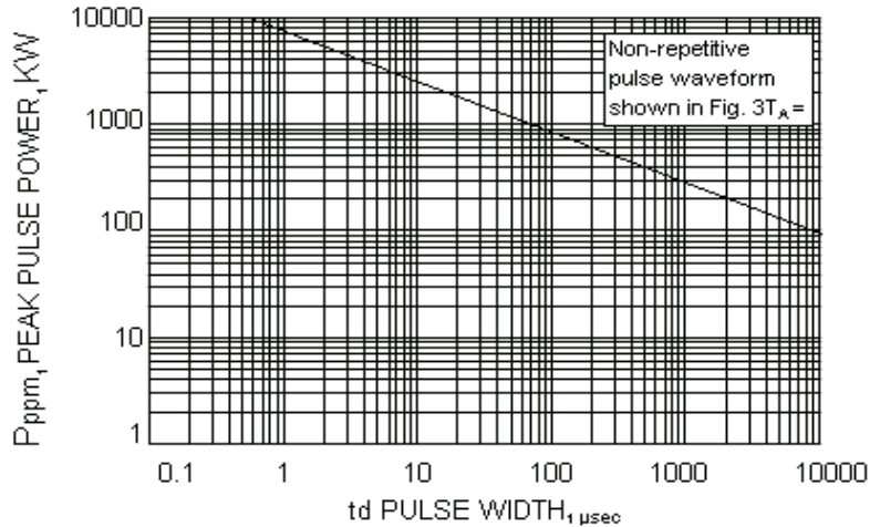
FIG. 1 PEAK PULSE POWER RATING
