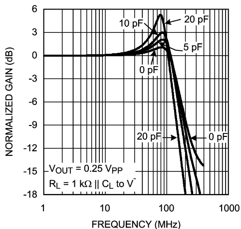
Frequency Response for Various Cap Load
