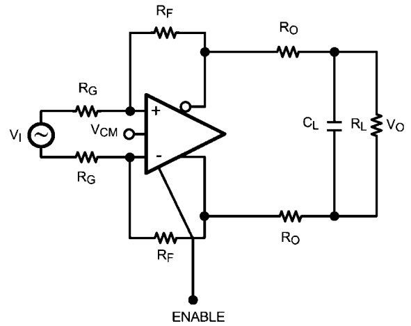
FIGURE 1. Typical Application
