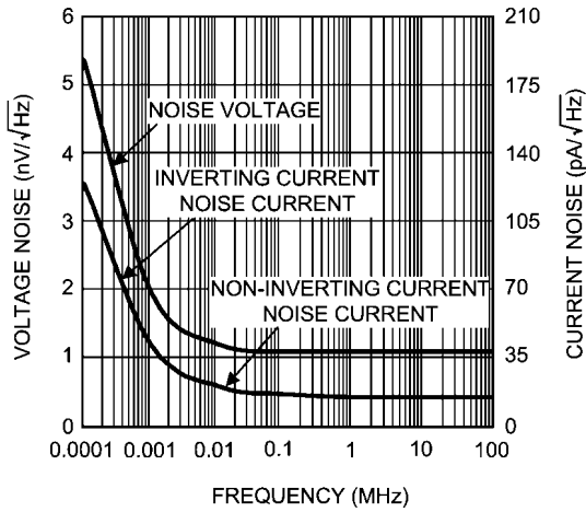
Input Noise vs. Frequency
