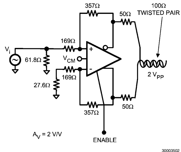
FIGURE 9. Fully Differential Cable Driver
