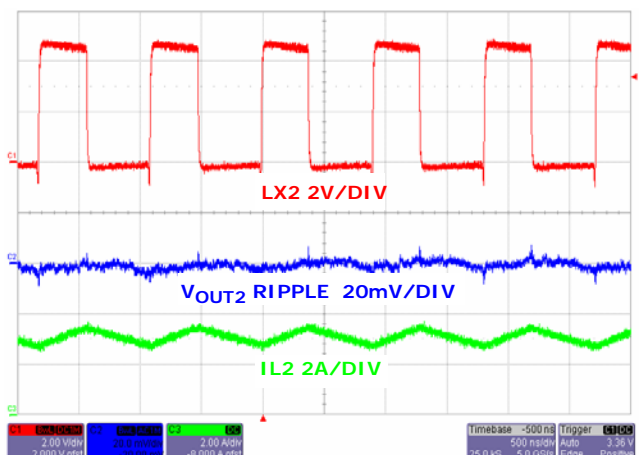
FIGURE 13. STEADY STATE OPERATION WITH FULL LOAD CHANNEL 2
