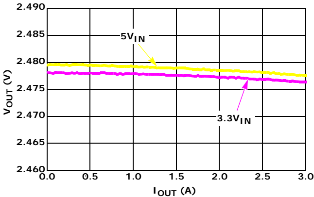
FIGURE 8. LOAD REGULATION, V_{OUT} = 2.5\text{V} T_A = +25^\circ\text{C}
