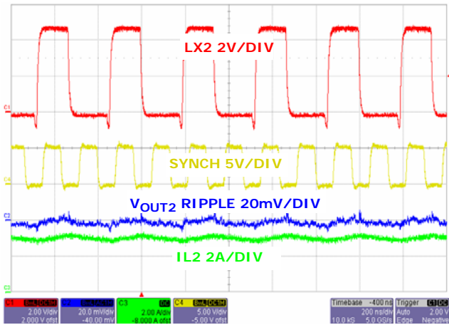
FIGURE 26. CHANNEL 2 STEADY STATE OPERATION AT FULL LOAD WITH FREQUENCY = 6MHz
