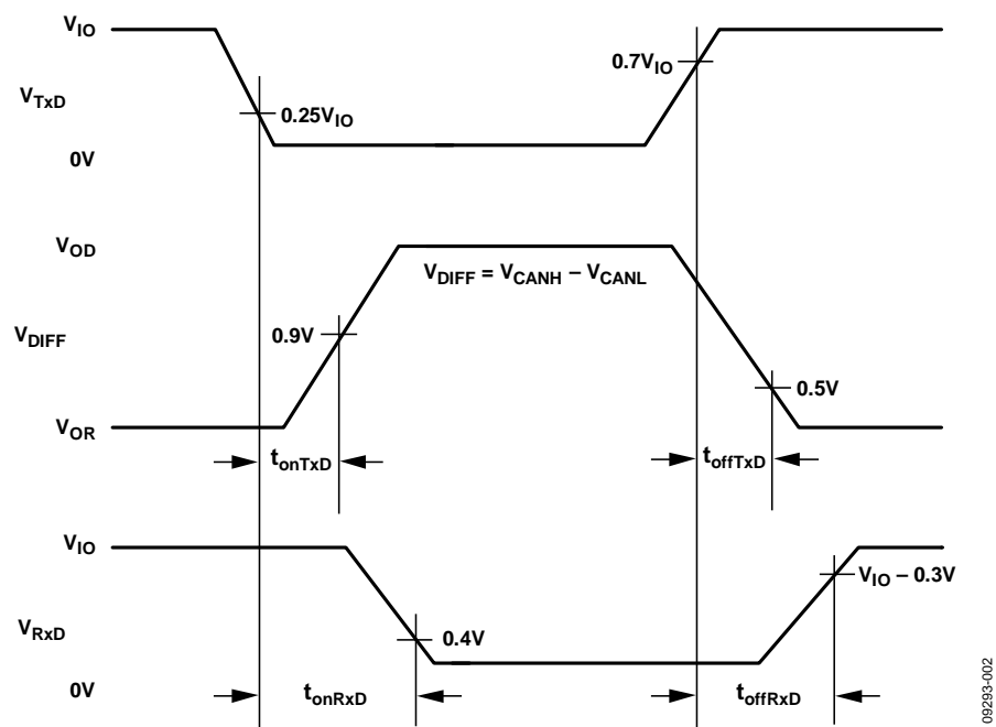
Figure 2. Driver Propagation Delay, Rise/Fall Timing
