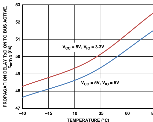
Figure 9. Propagation Delay from TxD On to Bus Active vs. Temperature
