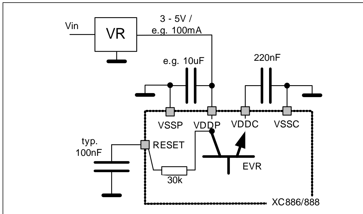
Figure 23 Reset Circuitry
