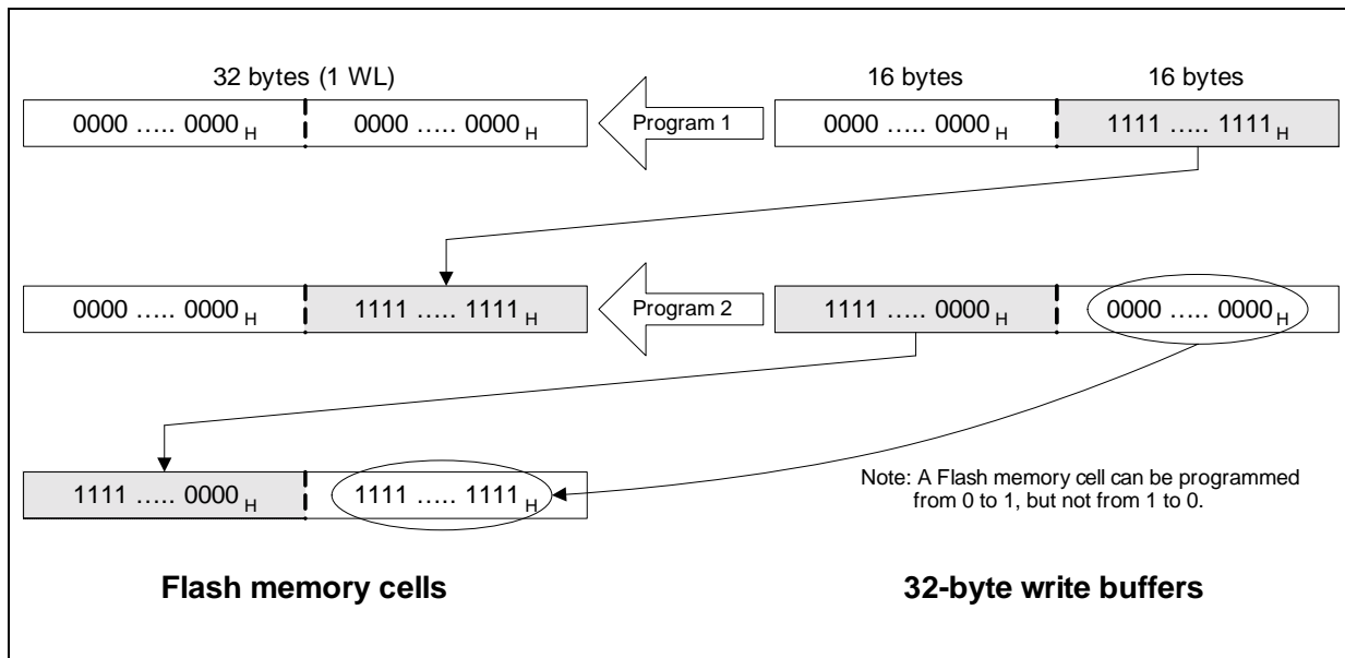
Figure 12 D-Flash Programming
