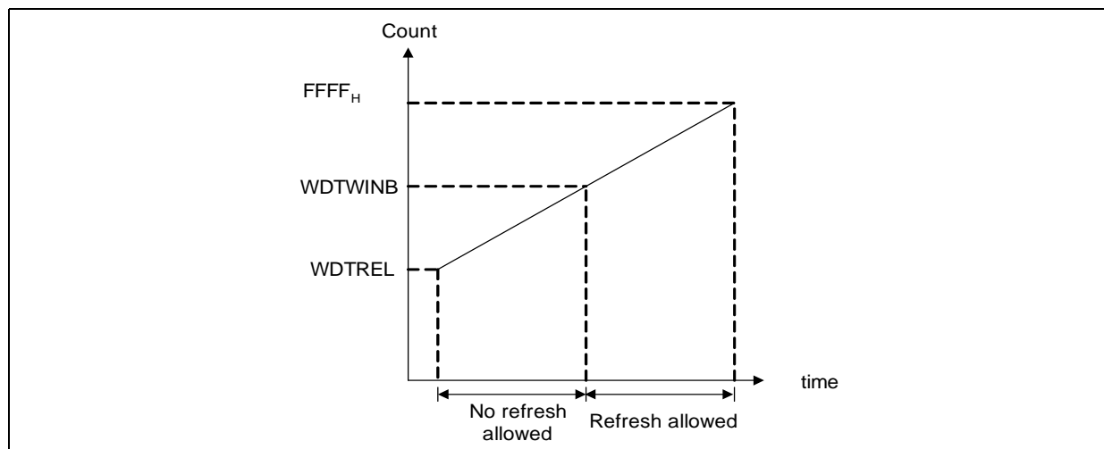
Figure 30 WDT Timing Diagram
