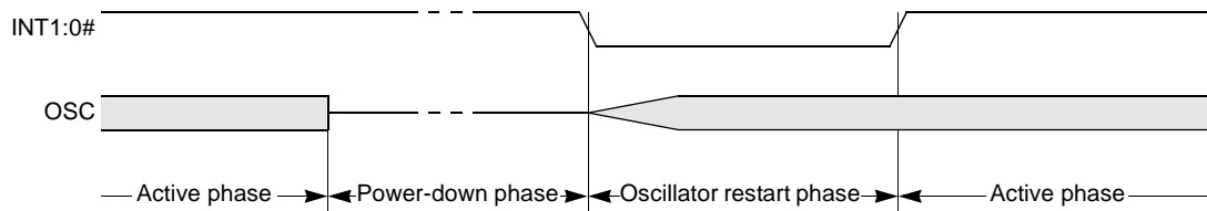
Figure 27. Power-Down Exit Waveform Using INT1:0#
