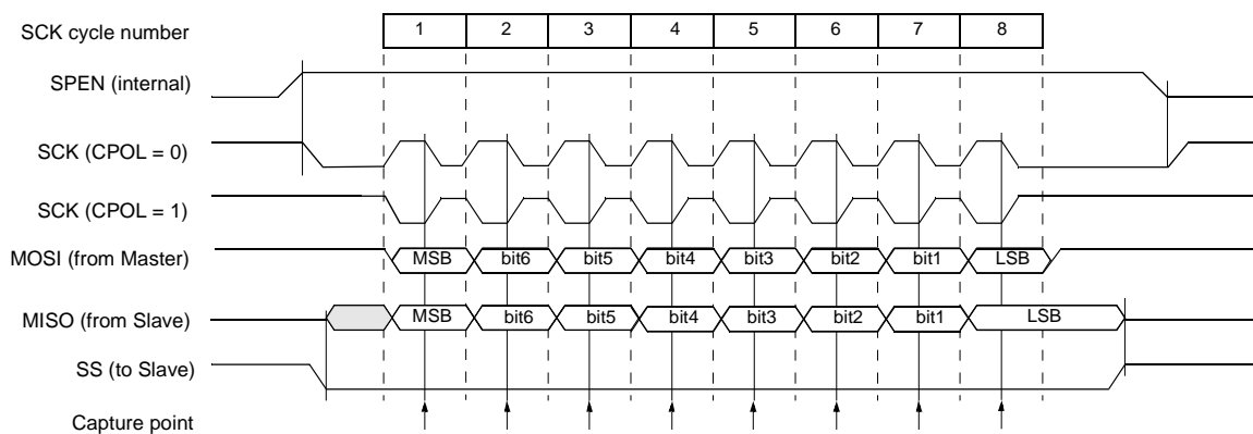
Figure 41. Data Transmission Format (CPHA = 1)
