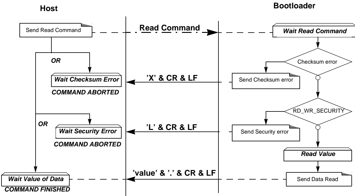
Figure 56. Read Flow
