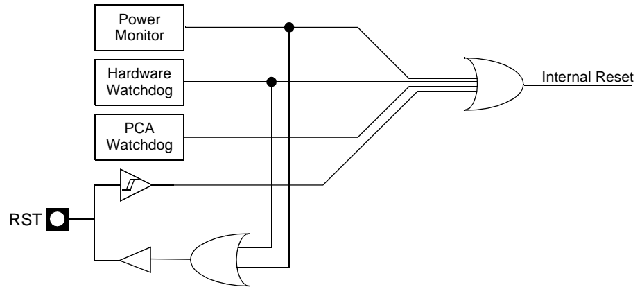
Figure 8. Reset schematic
