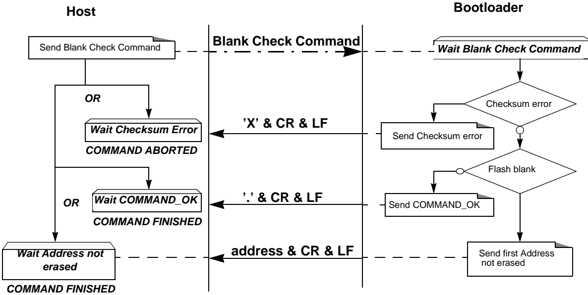
Figure 54. Blank Check Flow
