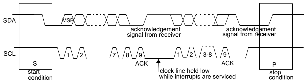
Figure 32. Complete Data Transfer on 2-wire Bus
