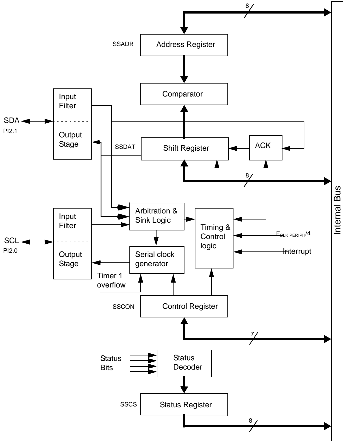
Figure 31. Block Diagram
