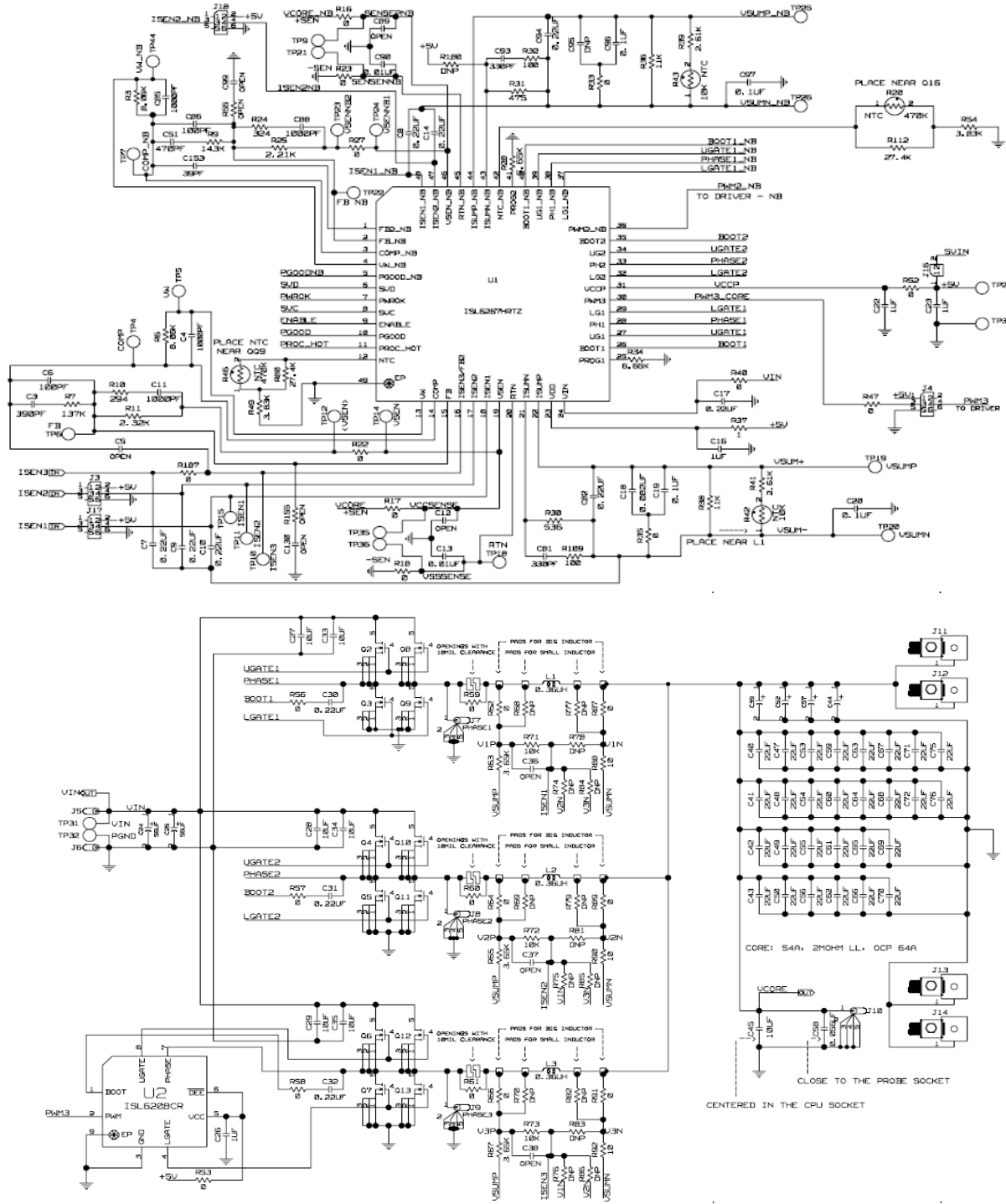
FIGURE 31. PORTION OF ISL6267EVAL12 EVALUATION BOARD SCHEMATIC
